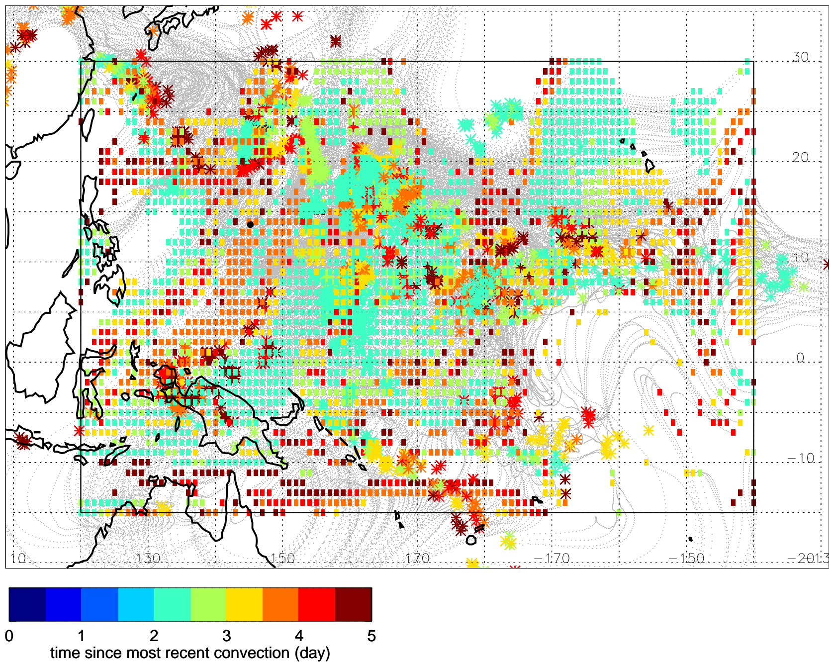
Fig. 2: Trajectories influenced by most recent convection (asterisks) between 0 and 5.0 days
