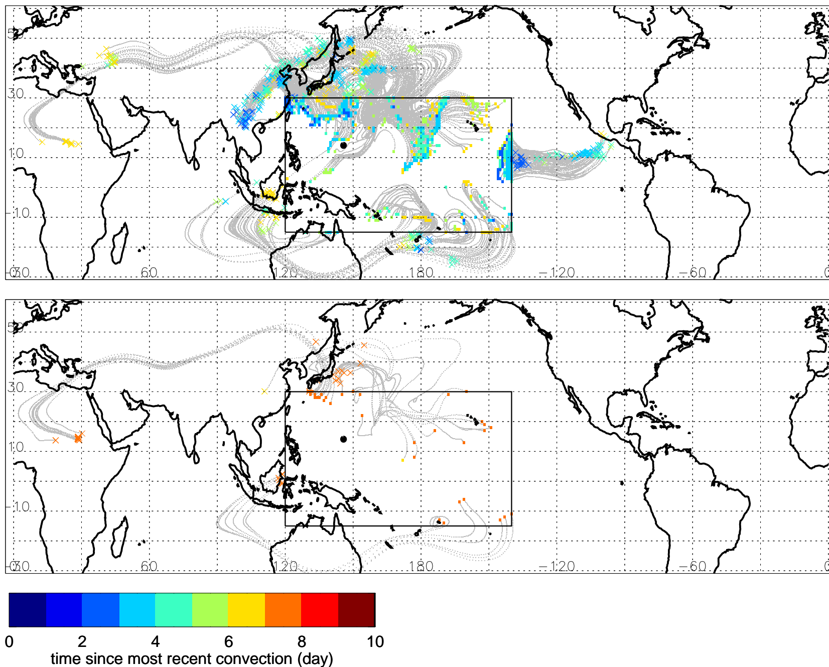
Fig. 5: Trajectories influenced by most recent convection that occurs outside of boxed region at location X.
