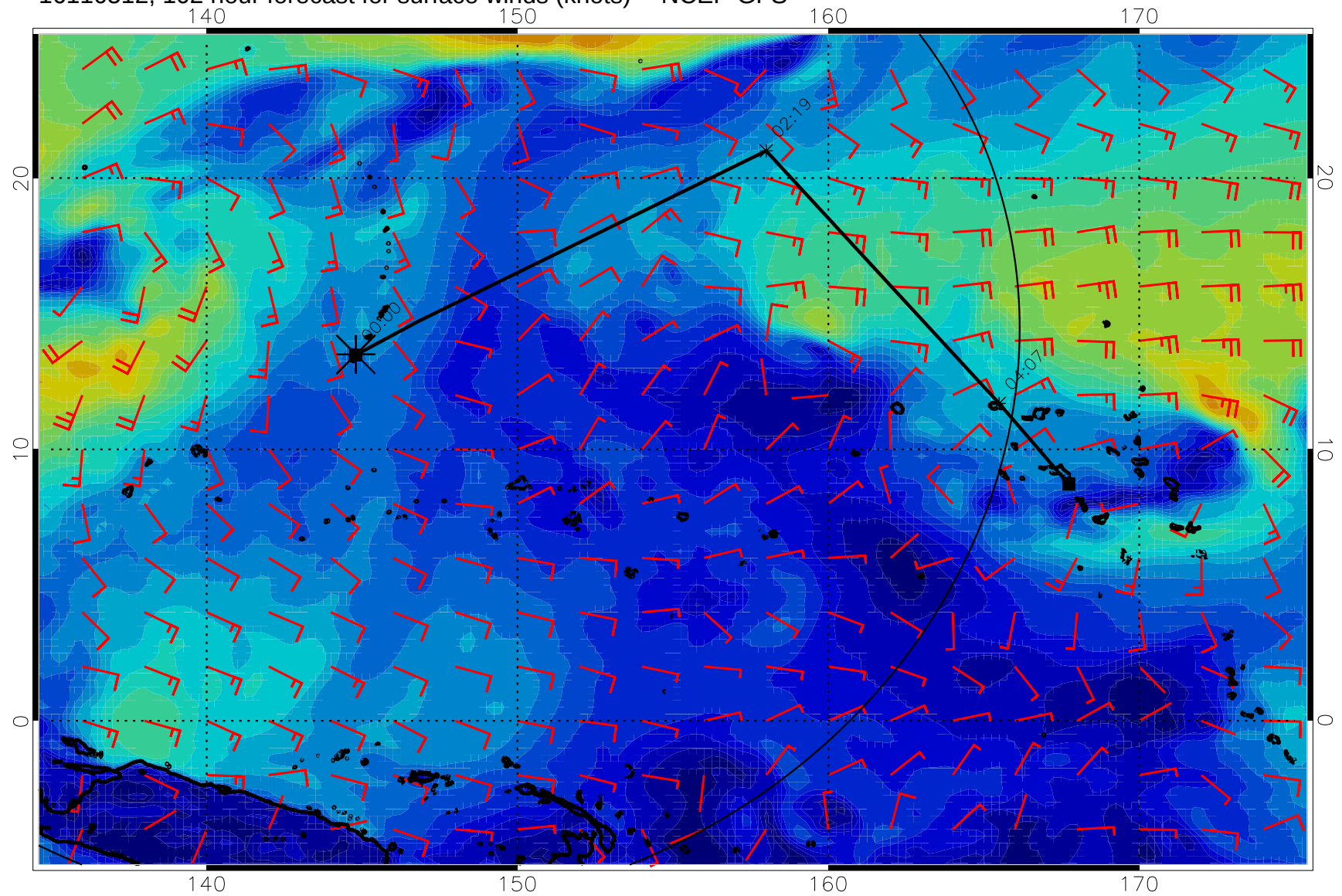
16110512, 102 hour forecast for surface winds (knots) -- NCEP GFS
