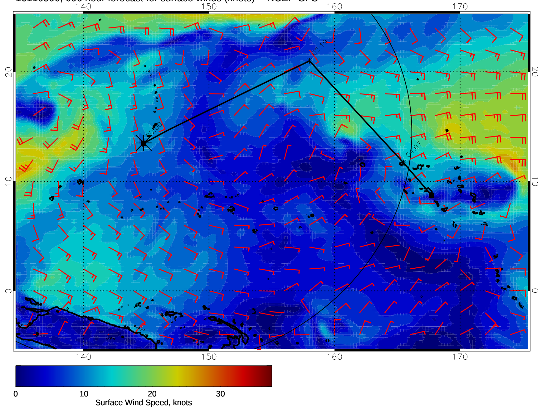
16110506, 096 hour forecast for surface winds (knots) -- NCEP GFS
