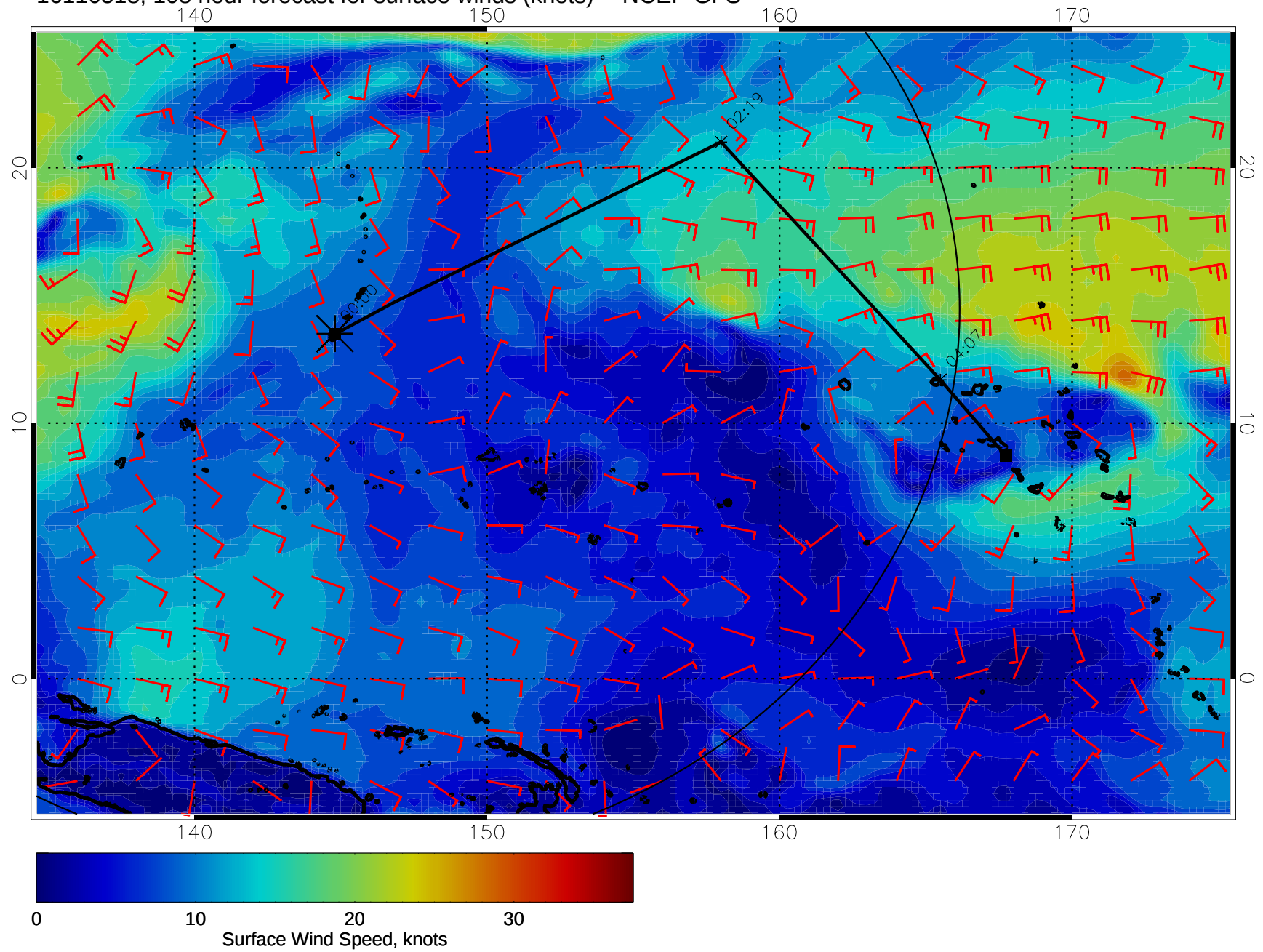
16110518, 108 hour forecast for surface winds (knots) -- NCEP GFS
