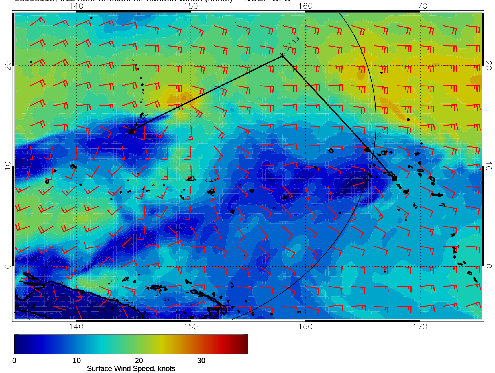
16110118, 012 hour forecast for surface winds (knots) -- NCEP GFS
