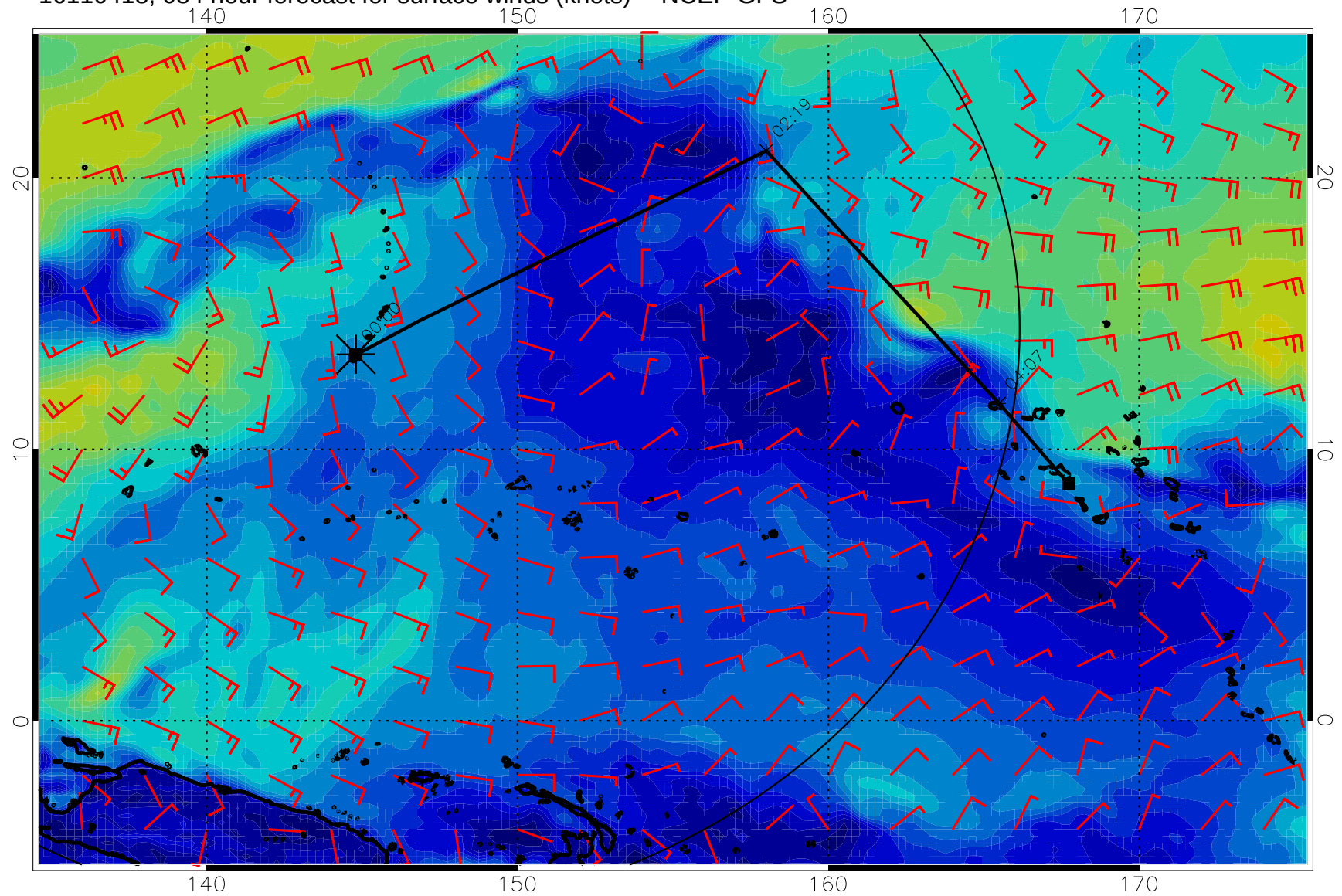
16110418, 084 hour forecast for surface winds (knots) -- NCEP GFS
