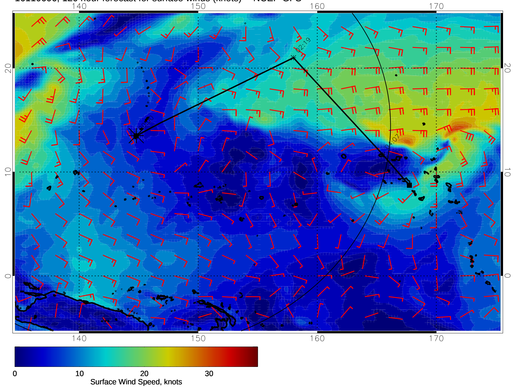
16110606, 120 hour forecast for surface winds (knots) -- NCEP GFS
