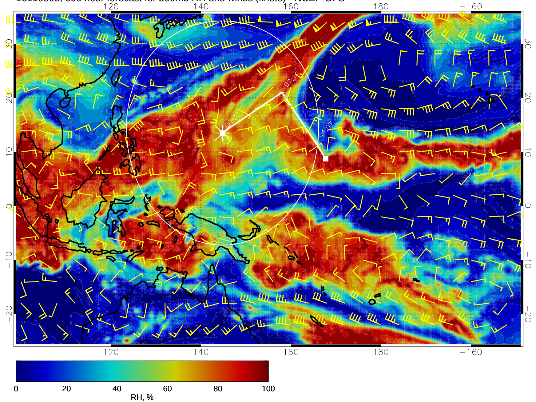
16110500, 090 hour forecast for 500mb RH and winds (knots) - NCEP GFS
