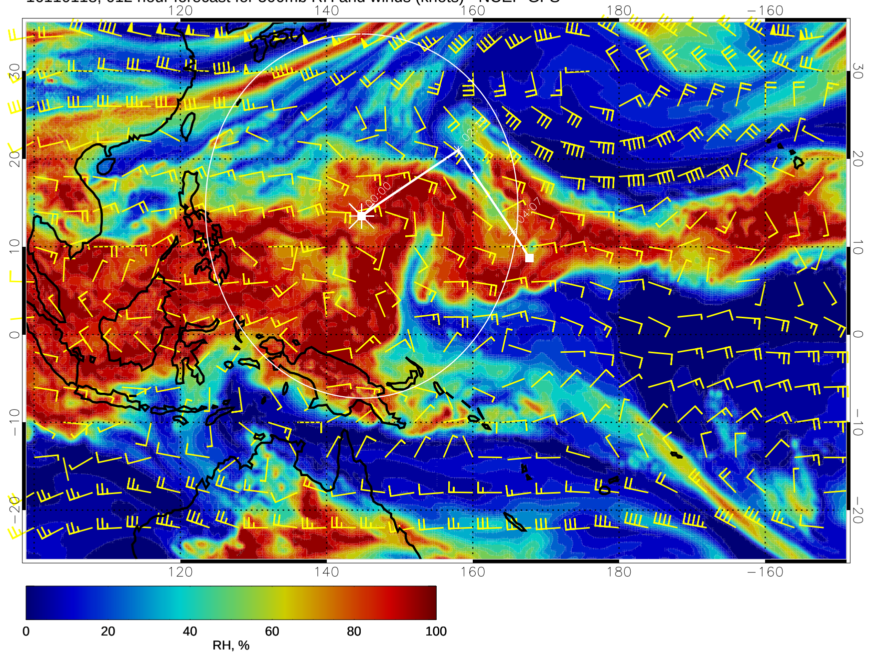
16110118, 012 hour forecast for 500mb RH and winds (knots) - NCEP GFS
