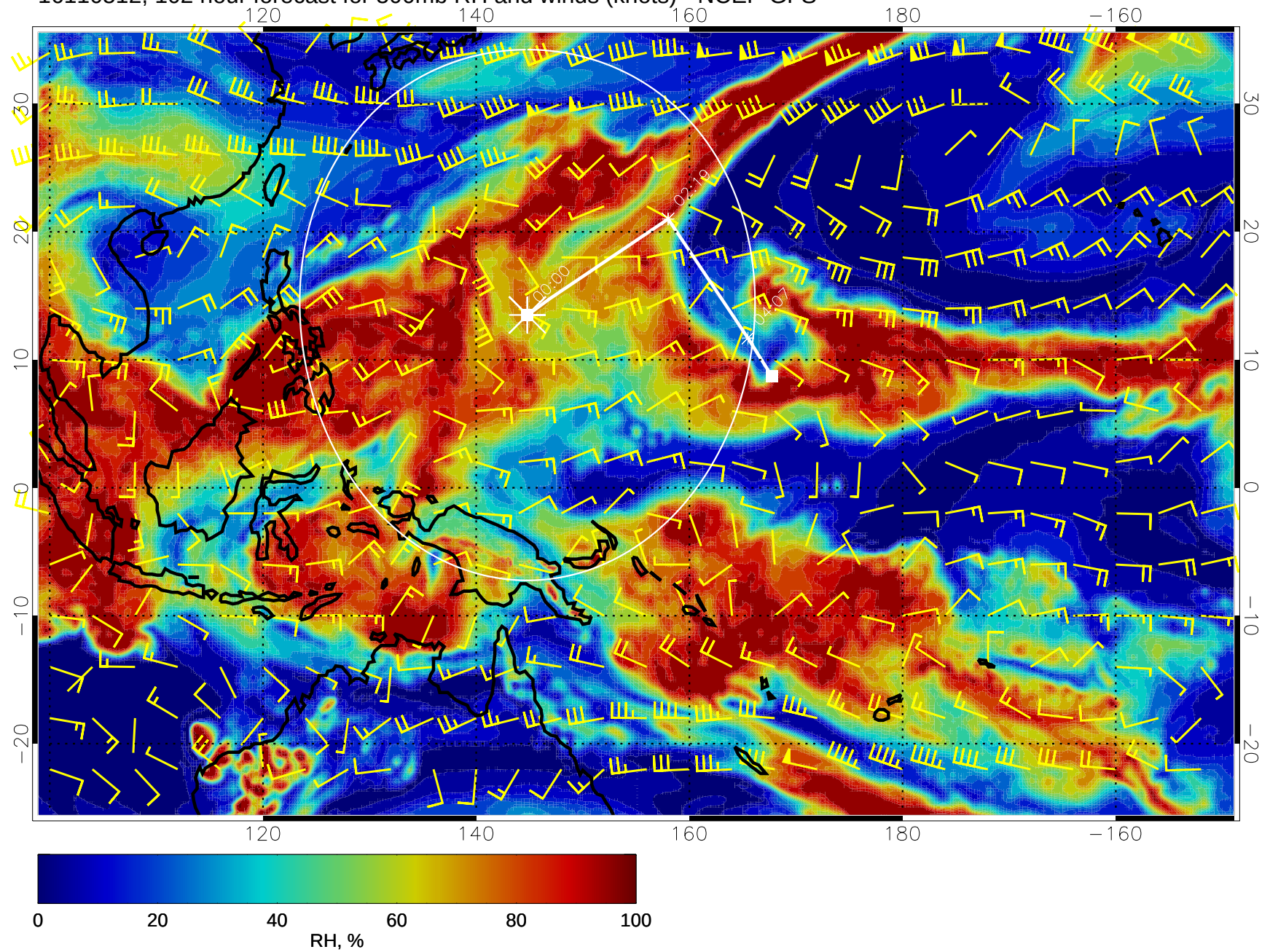
16110512, 102 hour forecast for 500mb RH and winds (knots) - NCEP GFS
