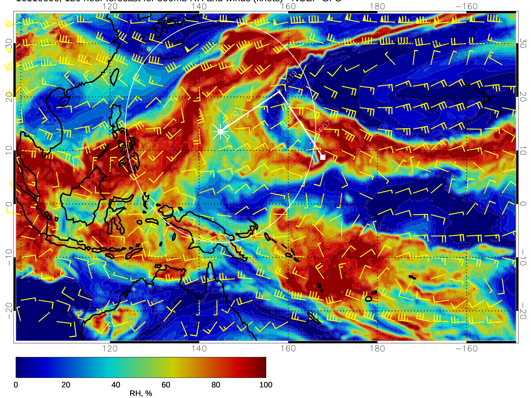
16110606, 120 hour forecast for 500mb RH and winds (knots) - NCEP GFS
