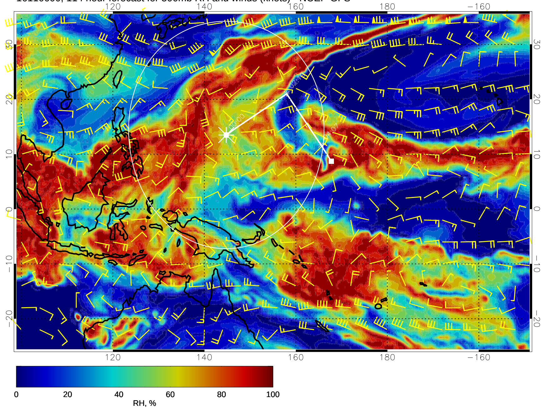
16110600, 114 hour forecast for 500mb RH and winds (knots) - NCEP GFS
