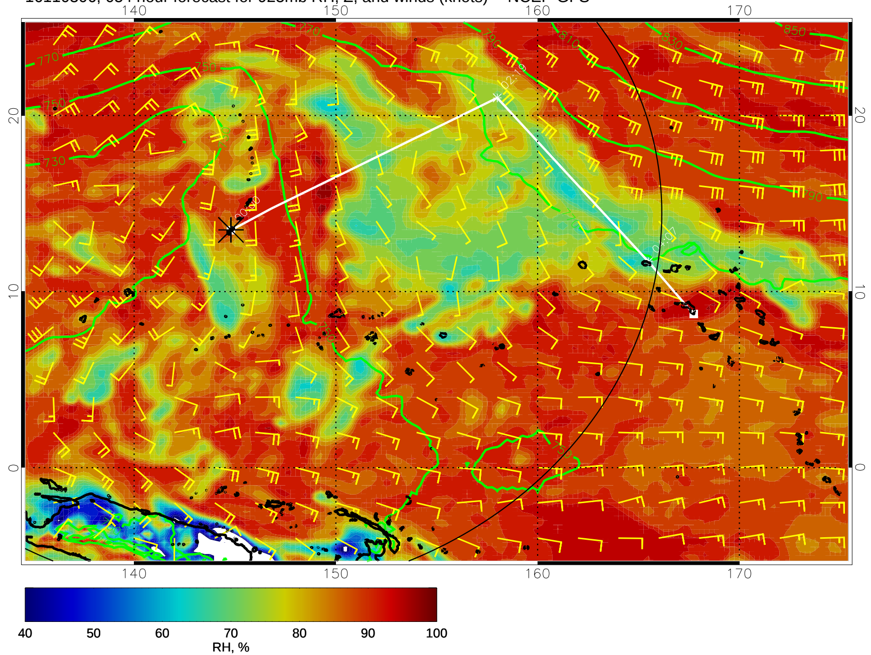
16110306, 054 hour forecast for 925mb RH, Z, and winds (knots) -- NCEP GFS
