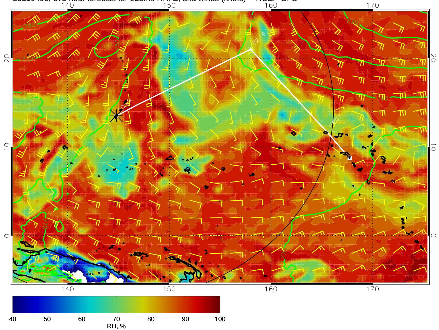
16110400, 072 hour forecast for 925mb RH, Z, and winds (knots) -- NCEP GFS
