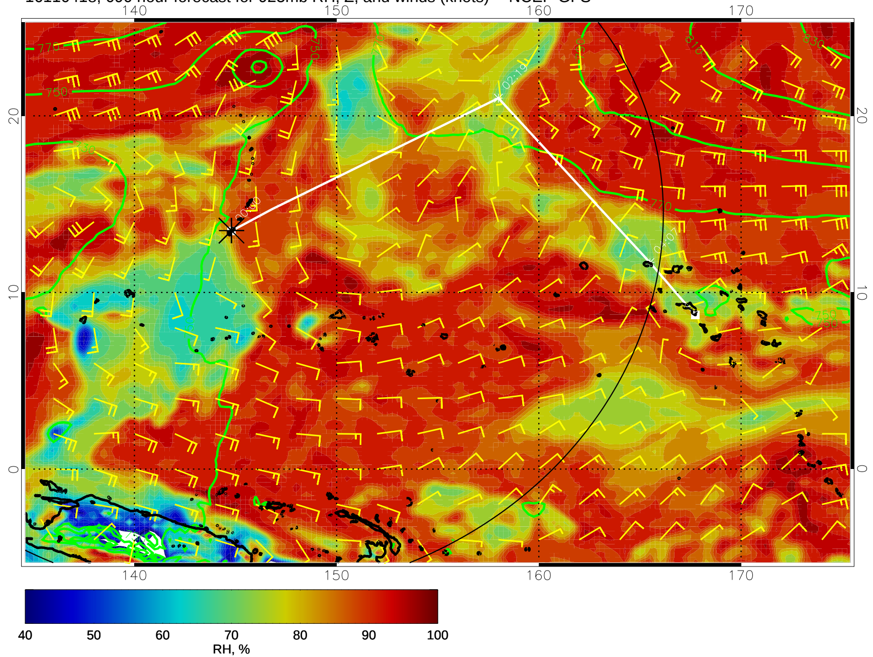
16110418, 090 hour forecast for 925mb RH, Z, and winds (knots) -- NCEP GFS
