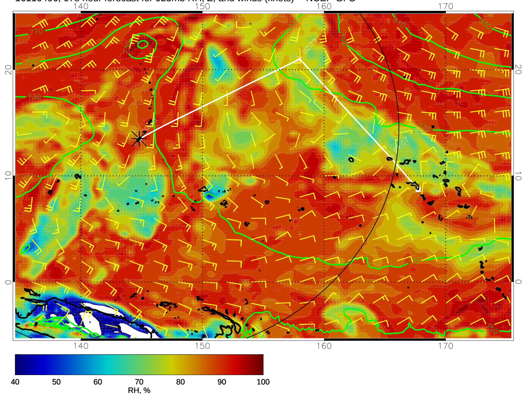
16110406, 078 hour forecast for 925mb RH, Z, and winds (knots) -- NCEP GFS
