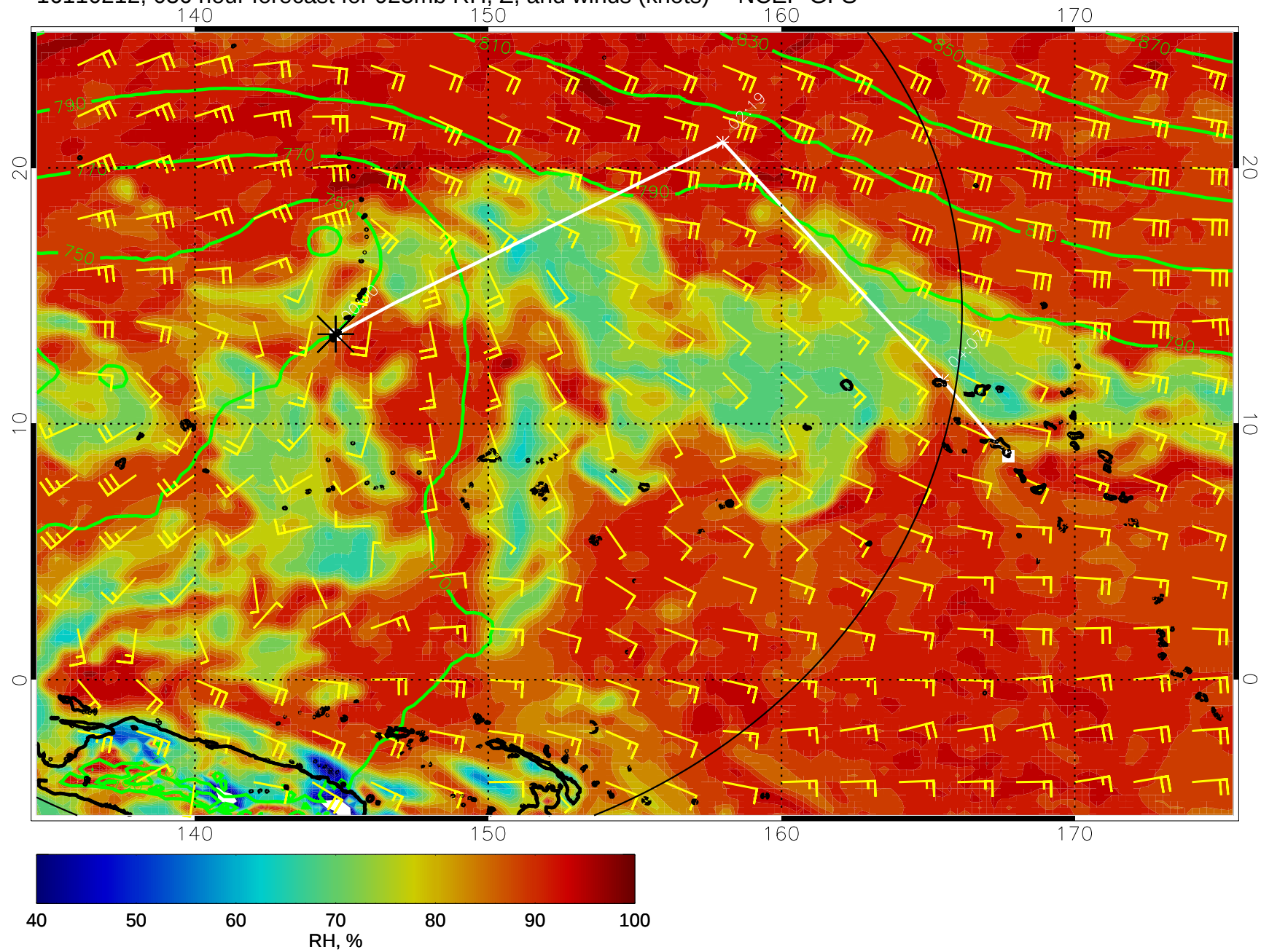
16110212, 036 hour forecast for 925mb RH, Z, and winds (knots) -- NCEP GFS
