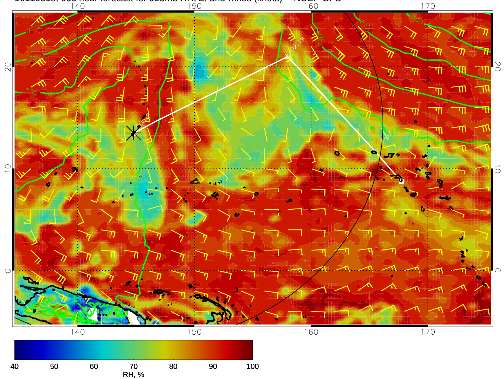
16110318, 066 hour forecast for 925mb RH, Z, and winds (knots) -- NCEP GFS
