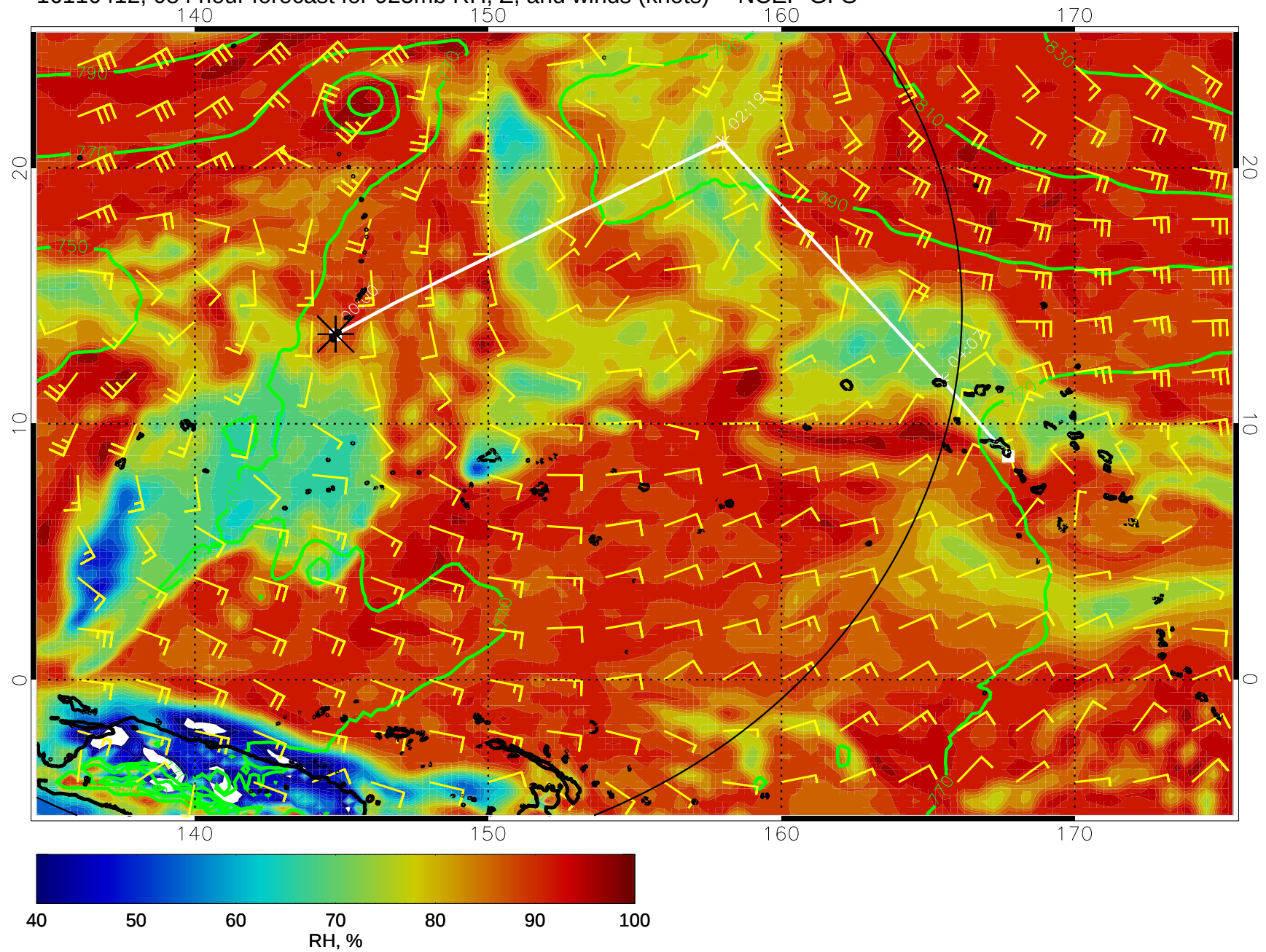
16110412, 084 hour forecast for 925mb RH, Z, and winds (knots) -- NCEP GFS
