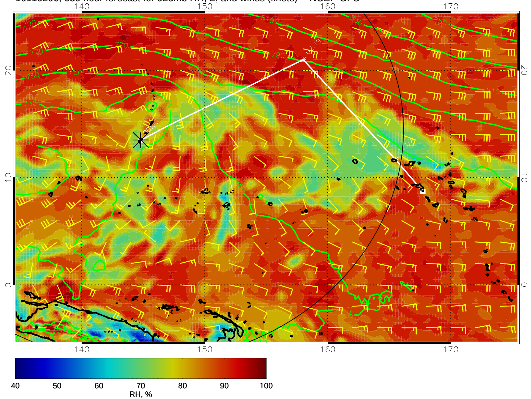
16110206, 030 hour forecast for 925mb RH, Z, and winds (knots) -- NCEP GFS
