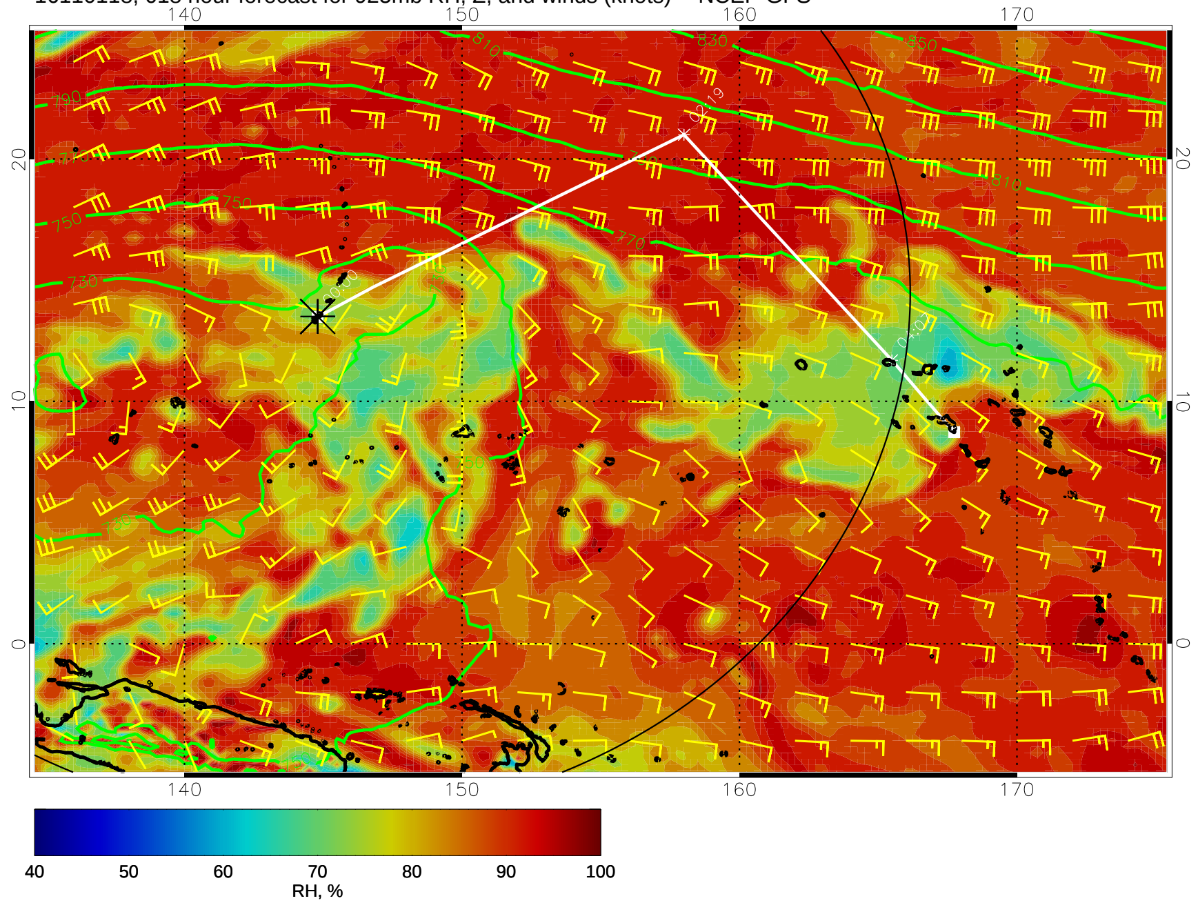
16110118, 018 hour forecast for 925mb RH, Z, and winds (knots) -- NCEP GFS
