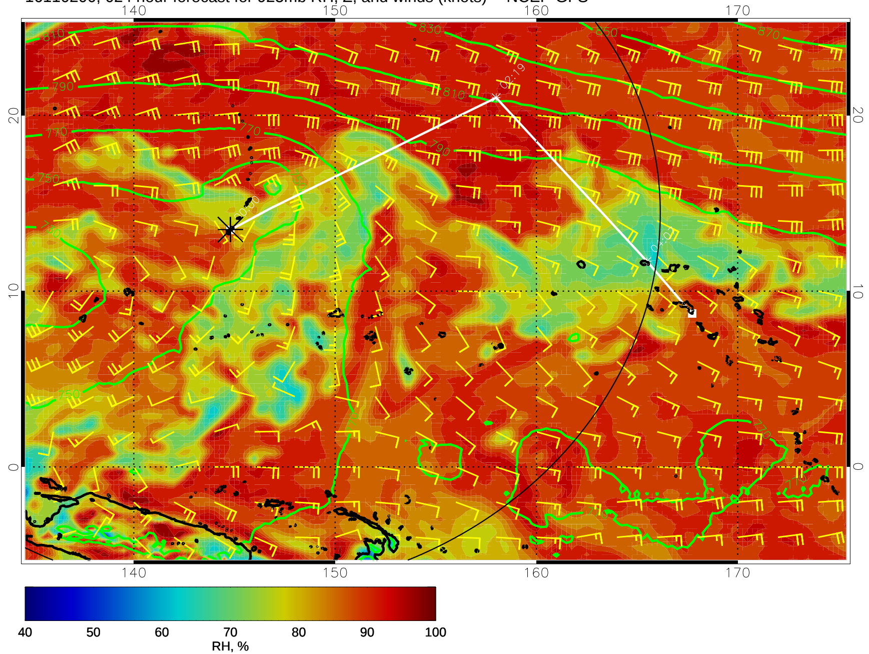
16110200, 024 hour forecast for 925mb RH, Z, and winds (knots) -- NCEP GFS
