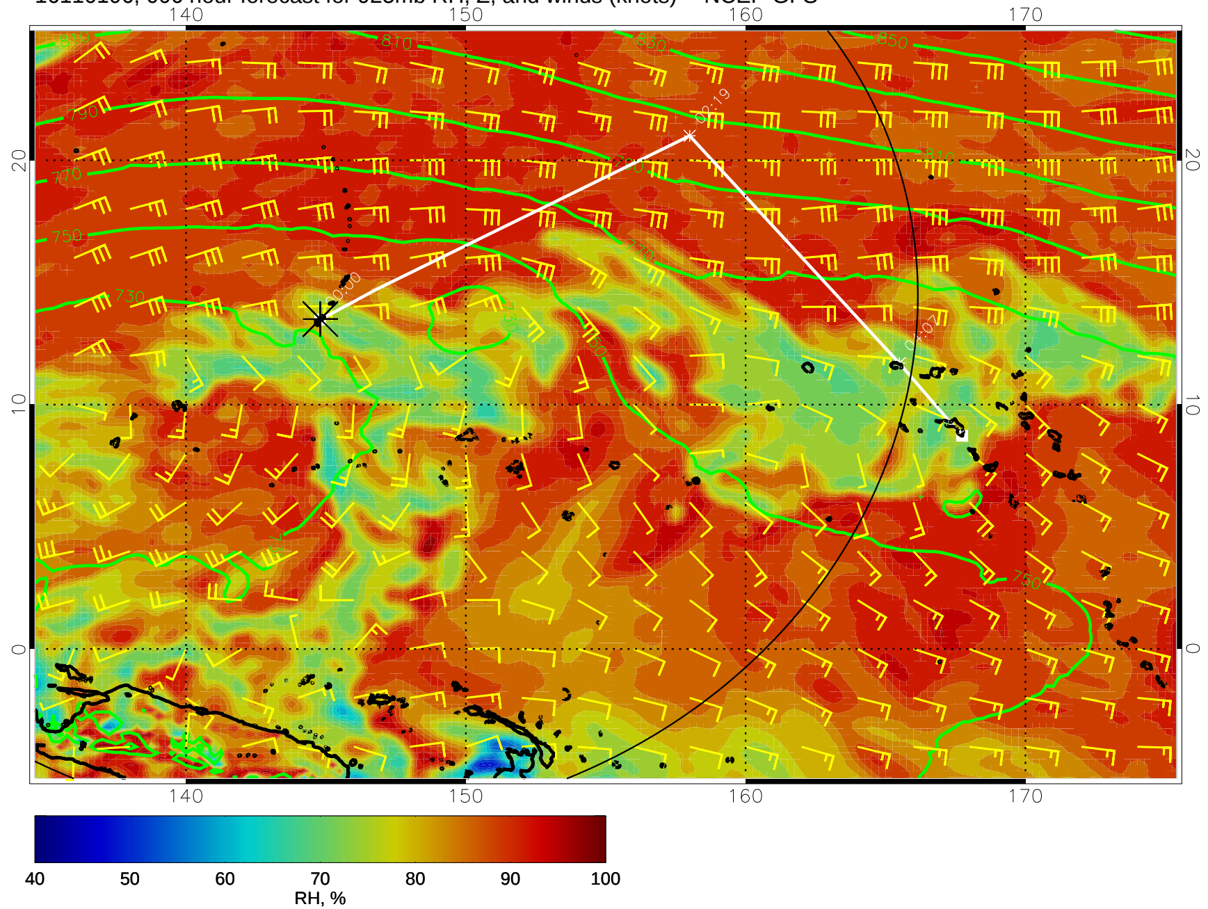
16110106, 006 hour forecast for 925mb RH, Z, and winds (knots) -- NCEP GFS
