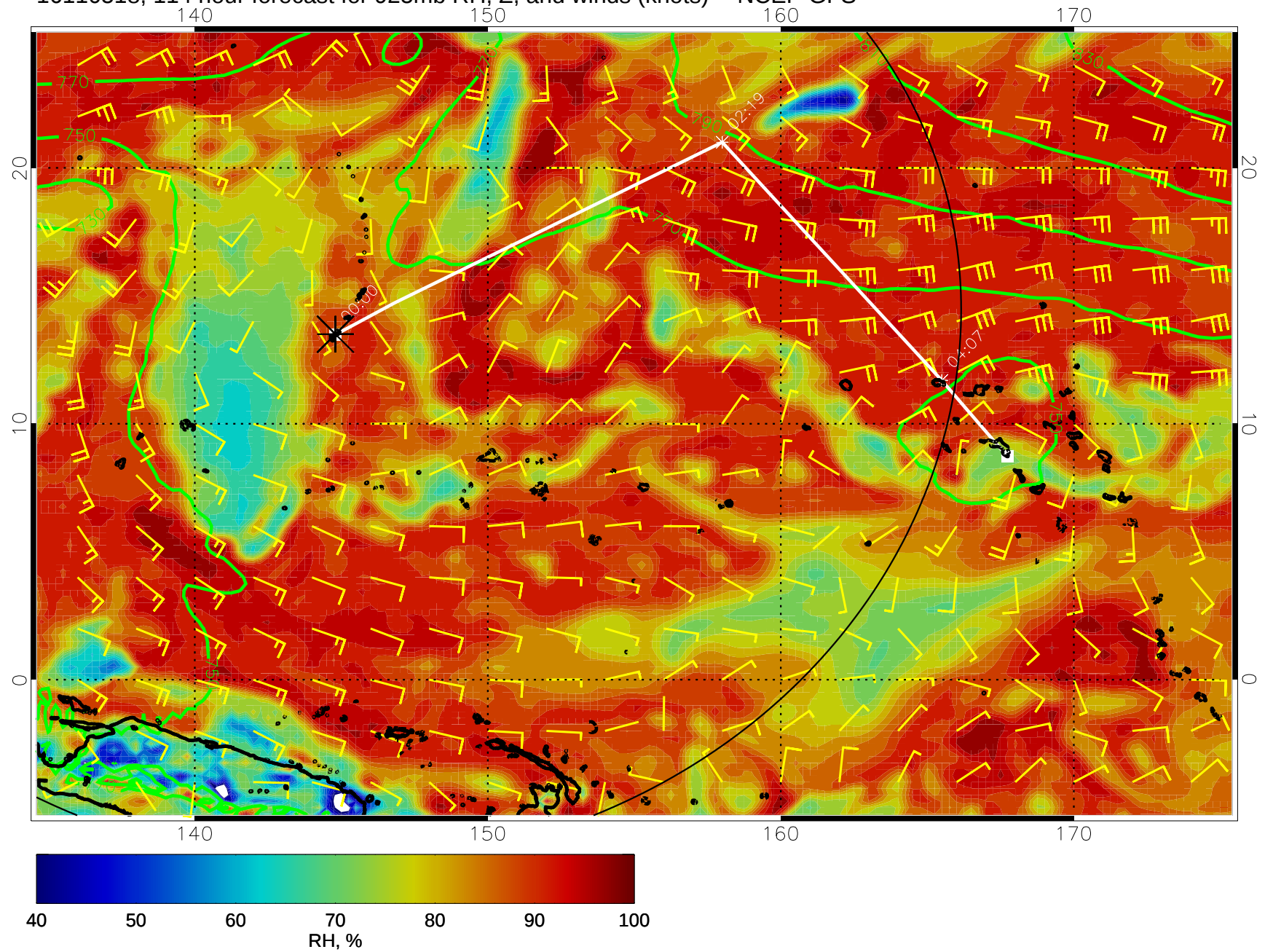
16110518, 114 hour forecast for 925mb RH, Z, and winds (knots) -- NCEP GFS
