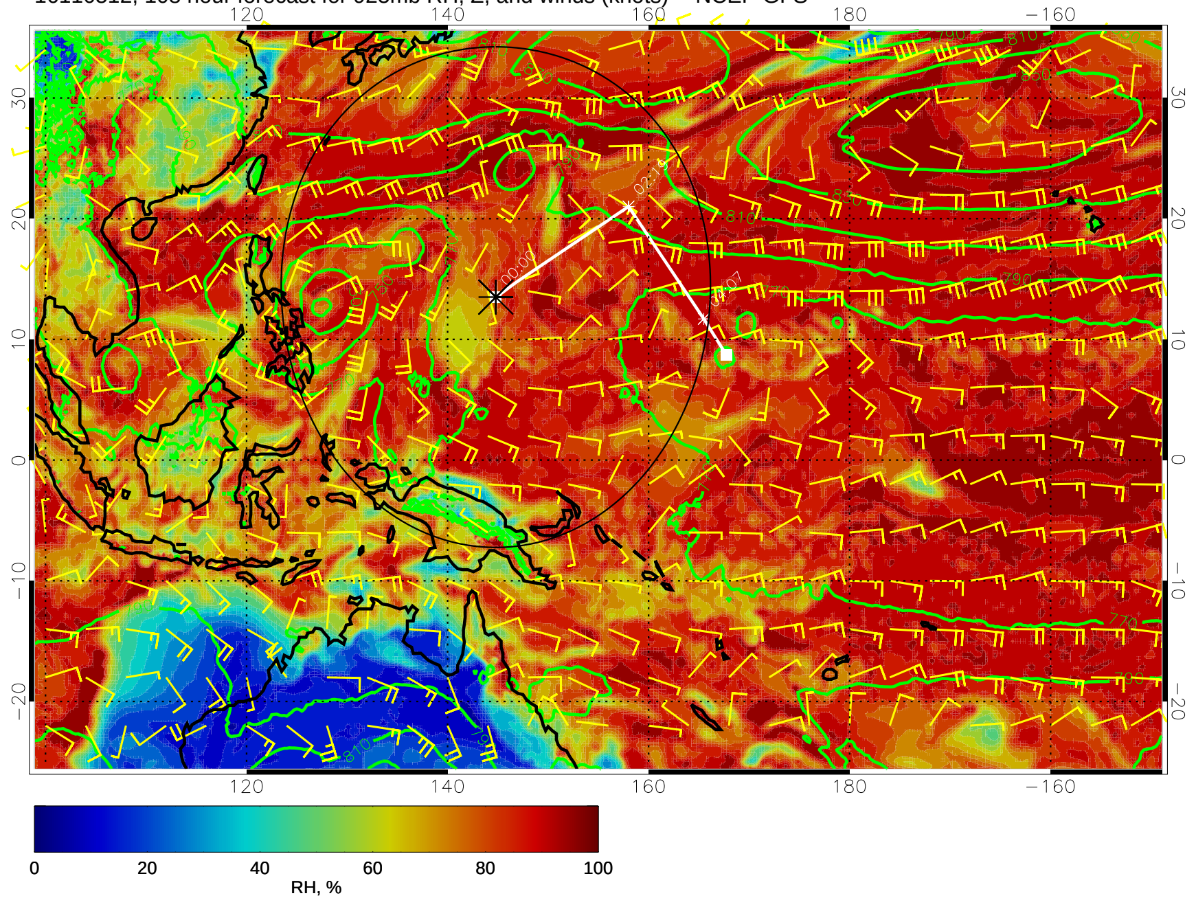
16110512, 108 hour forecast for 925mb RH, Z, and winds (knots) -- NCEP GFS
