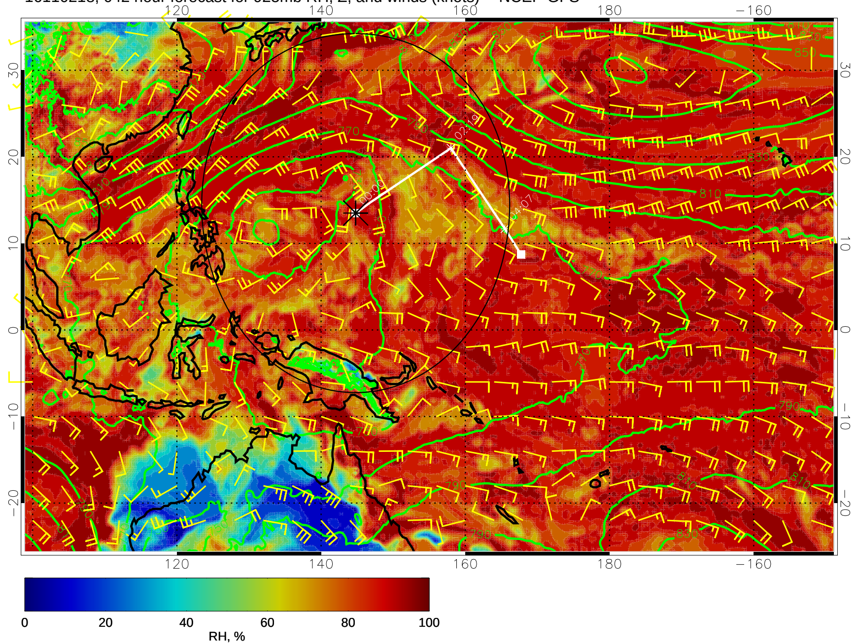
16110218, 042 hour forecast for 925mb RH, Z, and winds (knots) -- NCEP GFS
