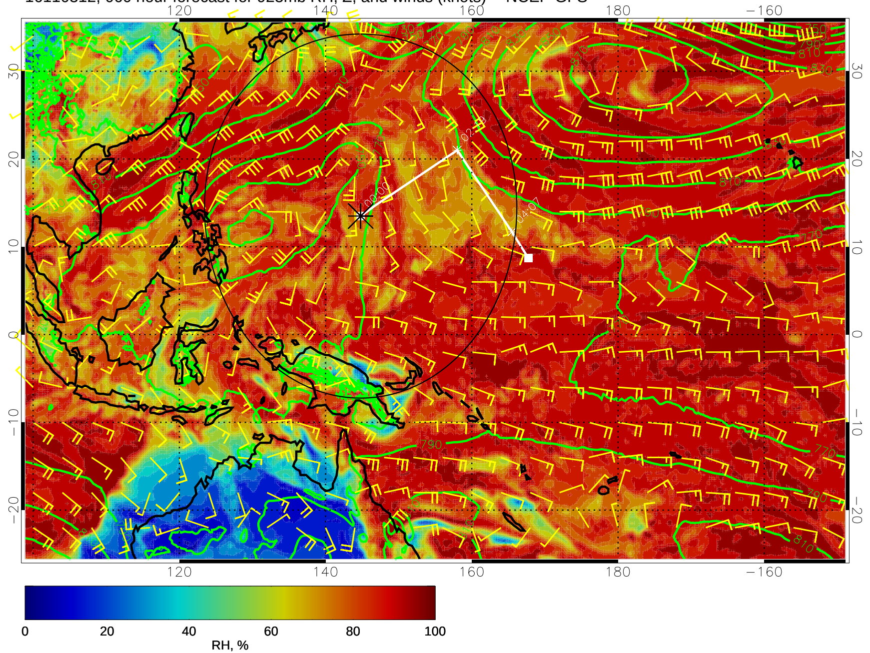
16110312, 060 hour forecast for 925mb RH, Z, and winds (knots) -- NCEP GFS
