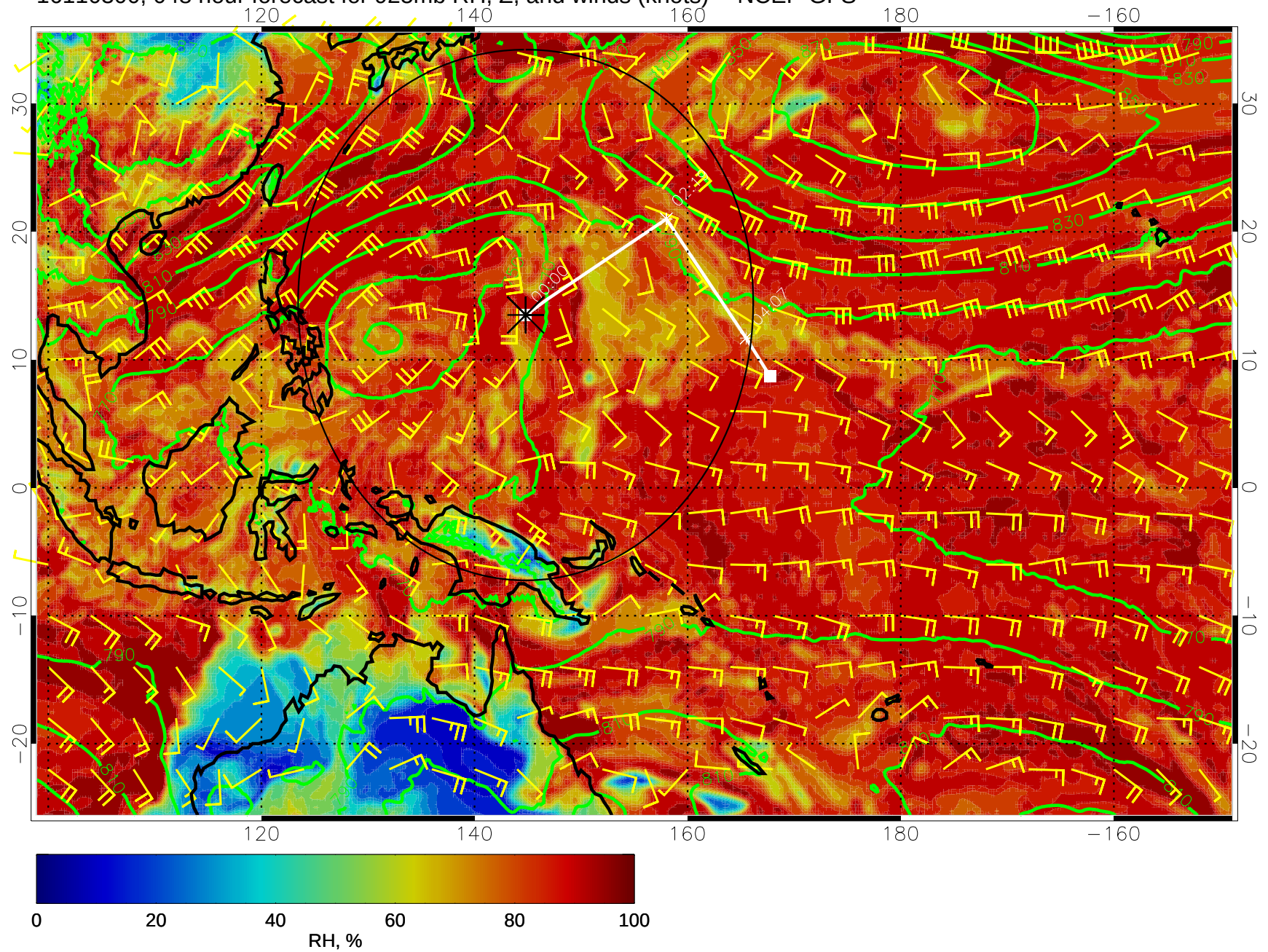
16110300, 048 hour forecast for 925mb RH, Z, and winds (knots) -- NCEP GFS
