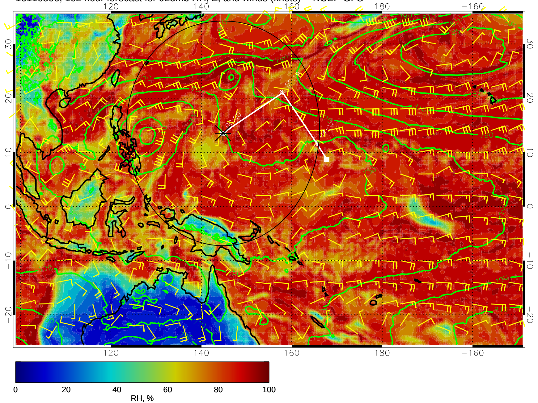
16110506, 102 hour forecast for 925mb RH, Z, and winds (knots) -- NCEP GFS
