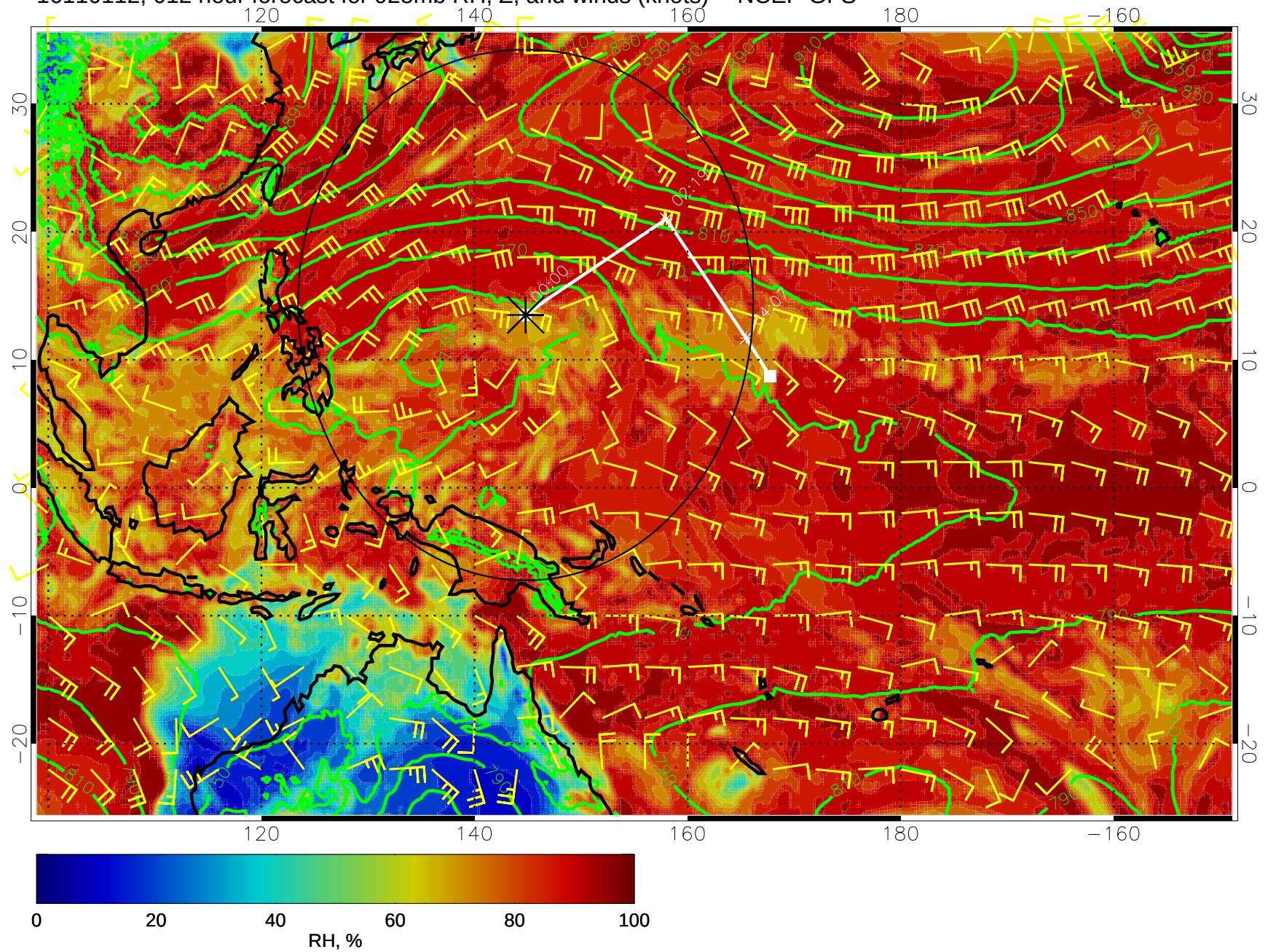
16110112, 012 hour forecast for 925mb RH, Z, and winds (knots) -- NCEP GFS
