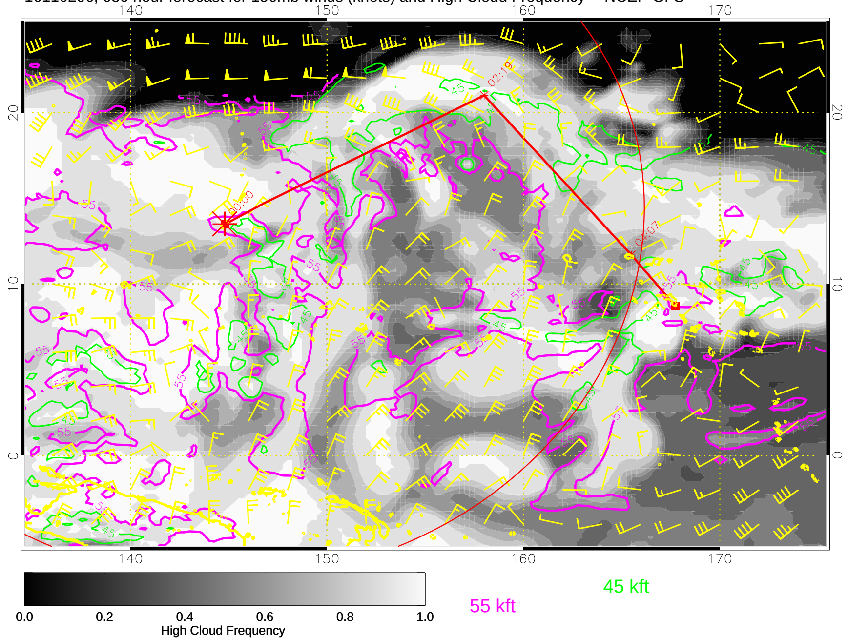
16110206, 030 hour forecast for 150mb winds (knots) and High Cloud Frequency -- NCEP GFS
