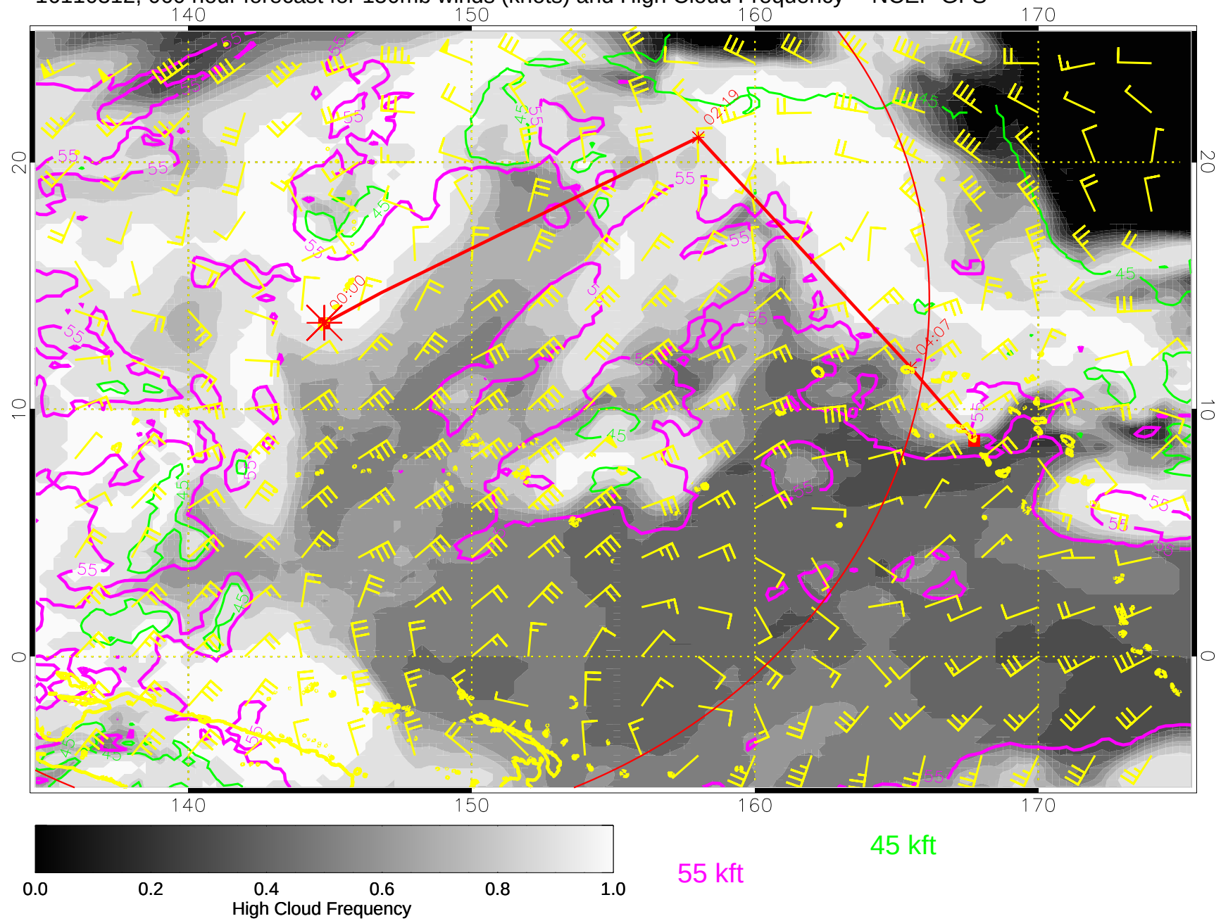
16110312, 060 hour forecast for 150mb winds (knots) and High Cloud Frequency -- NCEP GFS
