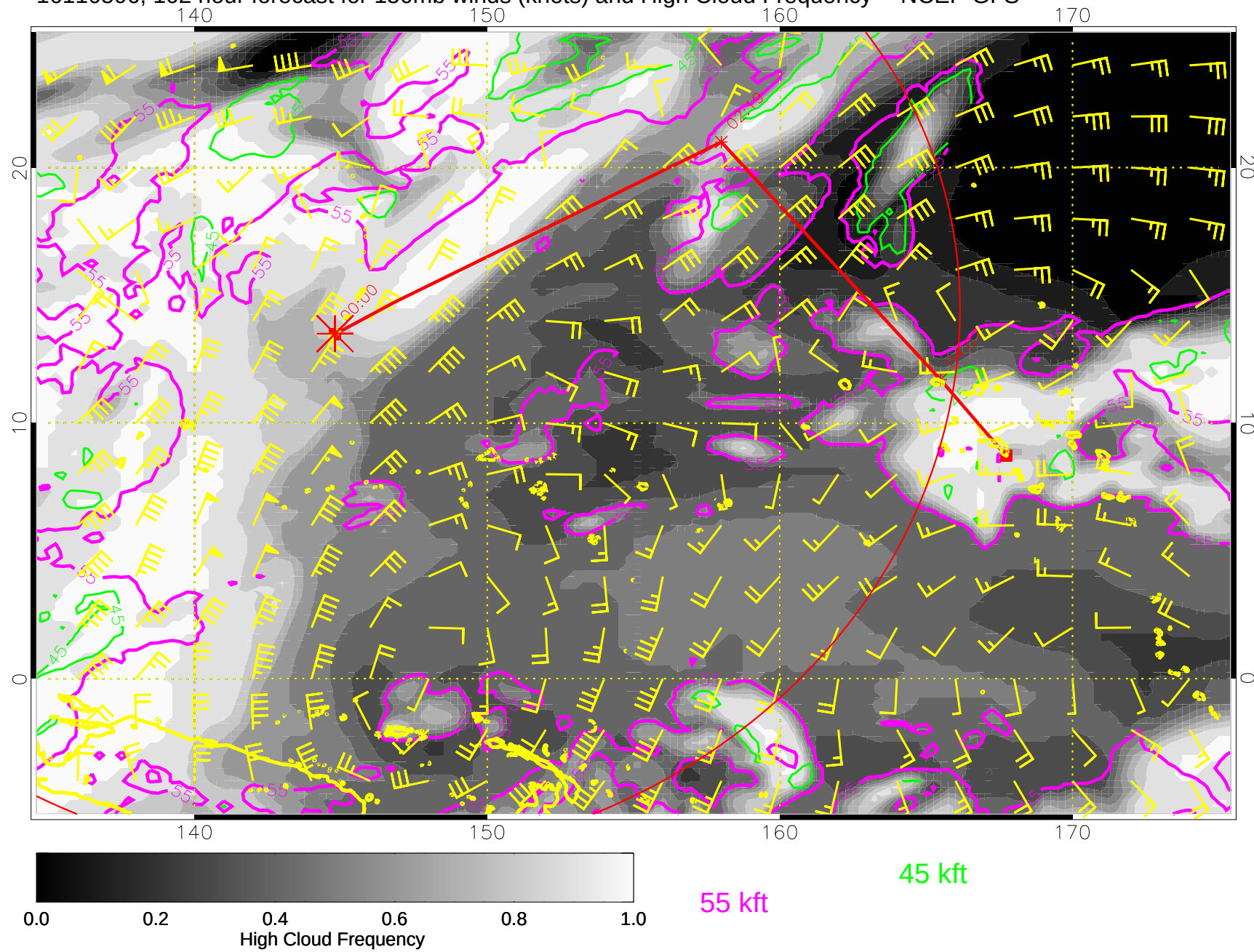
16110506, 102 hour forecast for 150mb winds (knots) and High Cloud Frequency -- NCEP GFS
