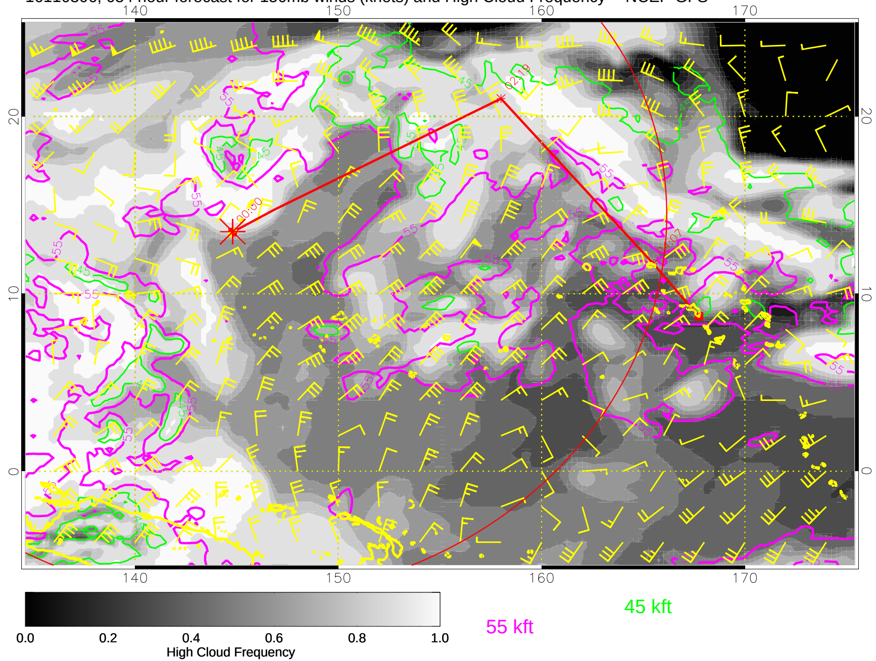
16110306, 054 hour forecast for 150mb winds (knots) and High Cloud Frequency -- NCEP GFS
