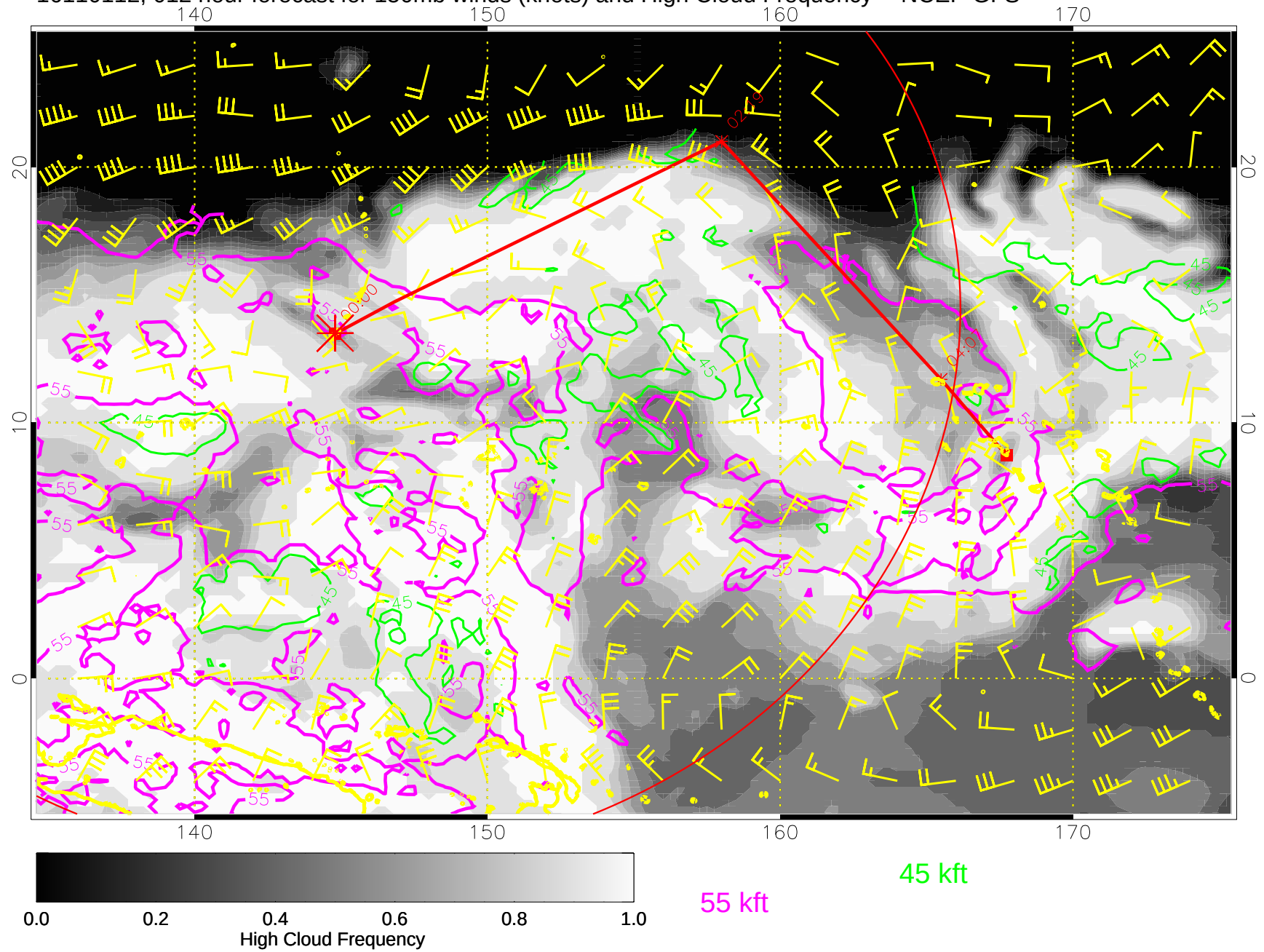
16110112, 012 hour forecast for 150mb winds (knots) and High Cloud Frequency -- NCEP GFS
