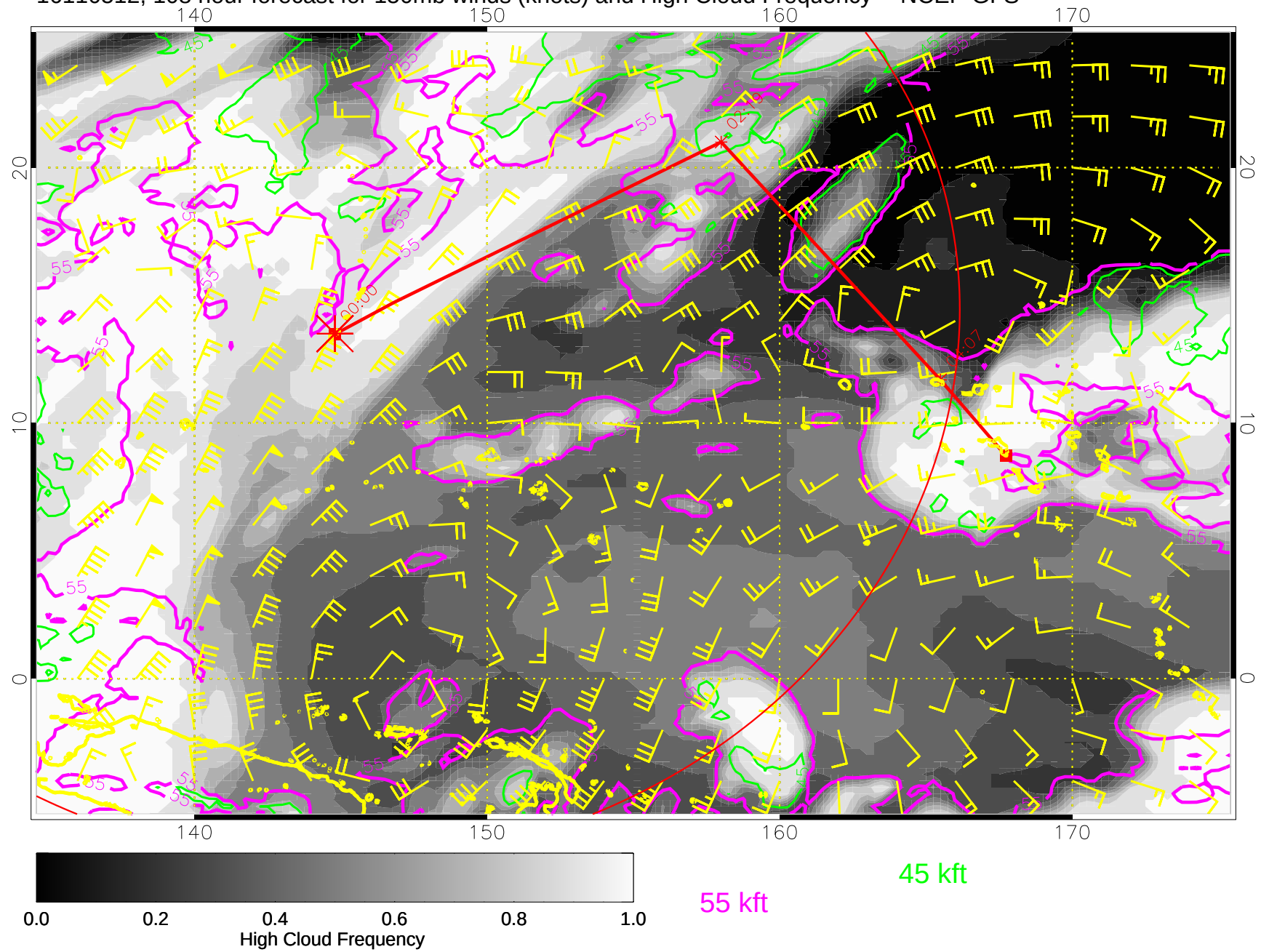
16110512, 108 hour forecast for 150mb winds (knots) and High Cloud Frequency -- NCEP GFS
