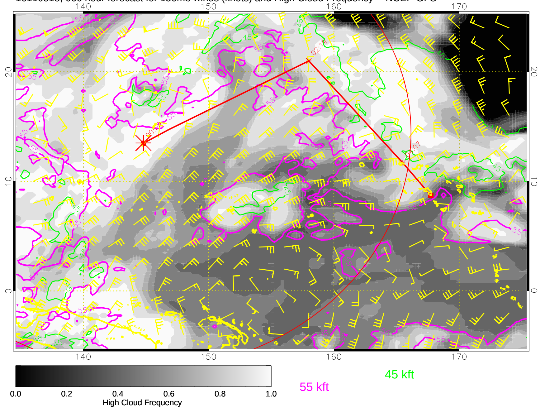
16110318, 066 hour forecast for 150mb winds (knots) and High Cloud Frequency -- NCEP GFS
