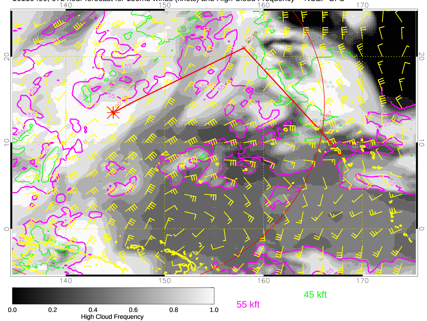
16110400, 072 hour forecast for 150mb winds (knots) and High Cloud Frequency -- NCEP GFS
