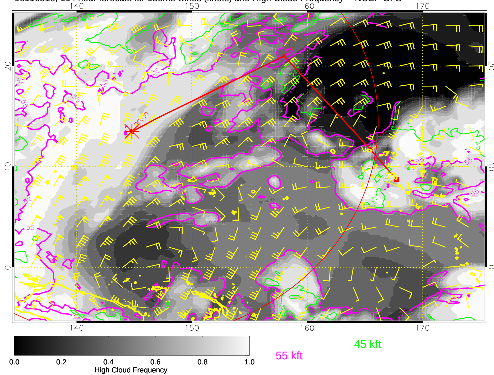
16110518, 114 hour forecast for 150mb winds (knots) and High Cloud Frequency -- NCEP GFS
