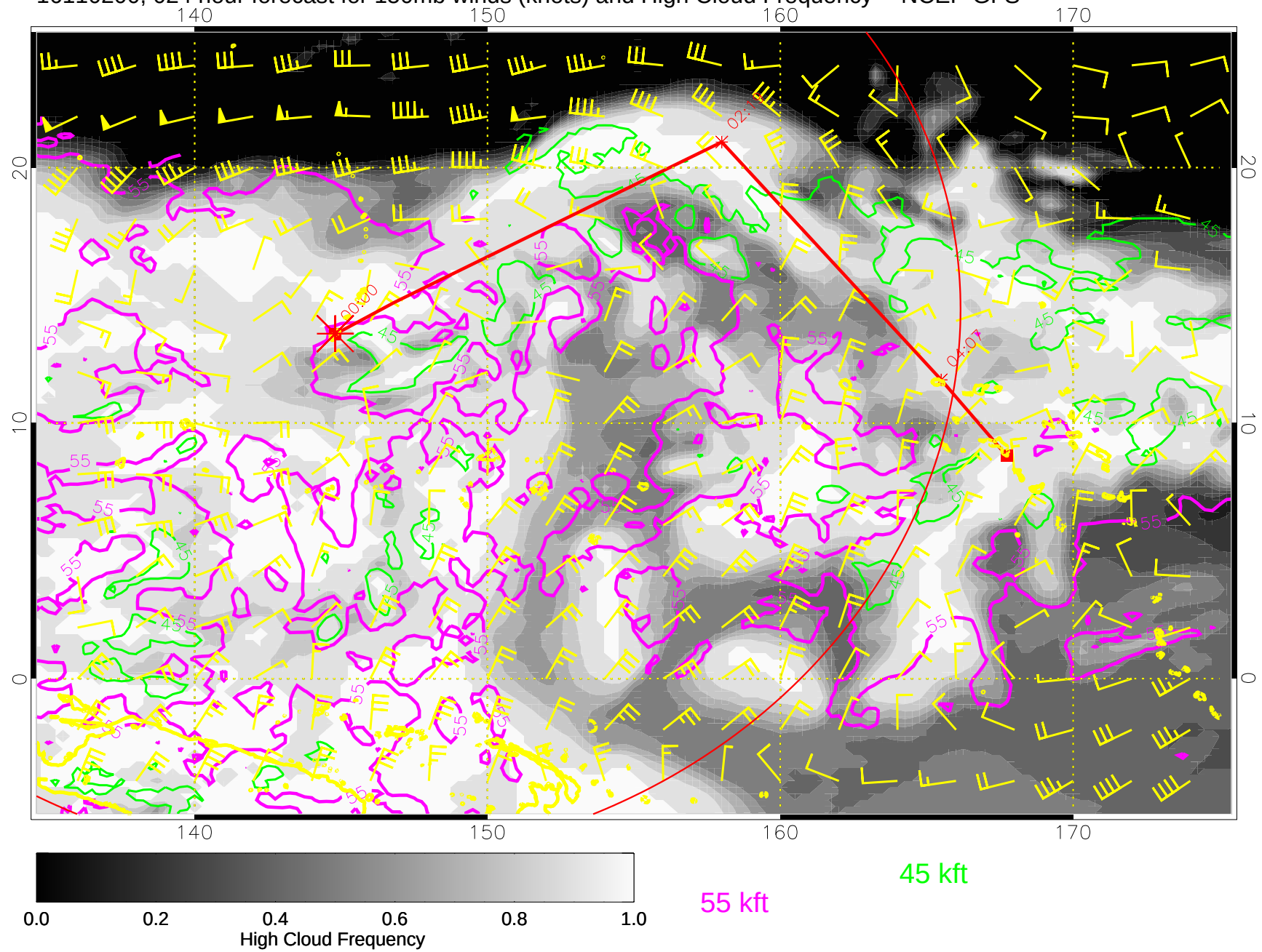
16110200, 024 hour forecast for 150mb winds (knots) and High Cloud Frequency -- NCEP GFS
