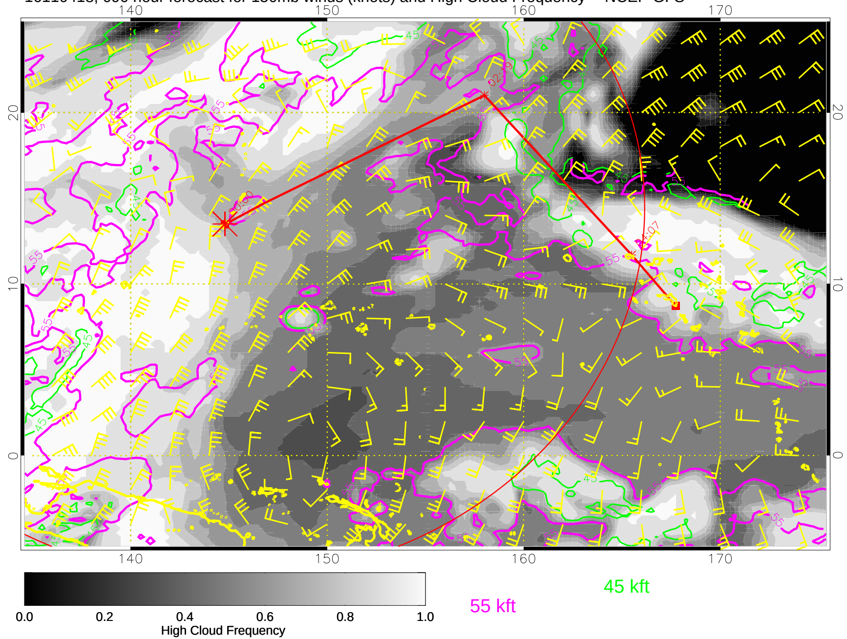
16110418, 090 hour forecast for 150mb winds (knots) and High Cloud Frequency -- NCEP GFS
