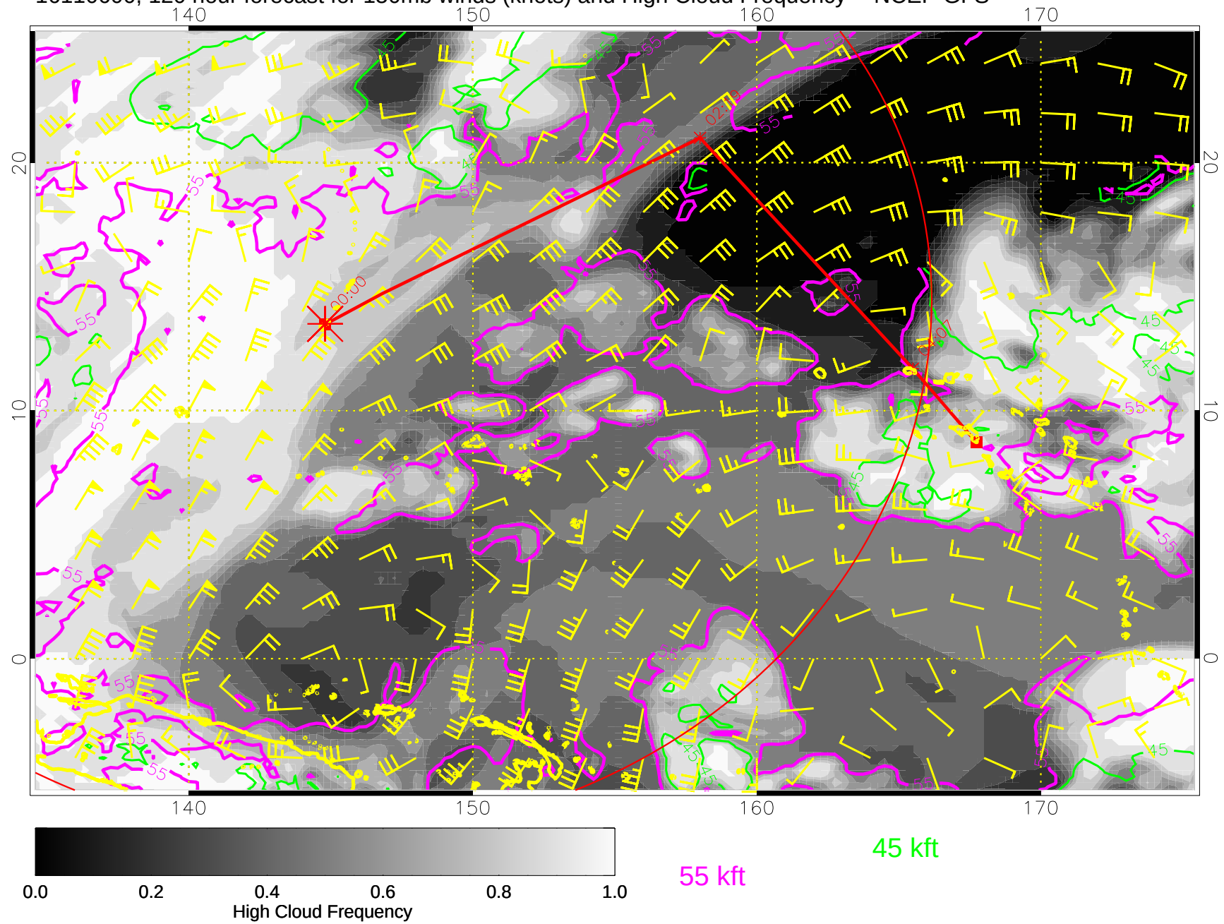
16110600, 120 hour forecast for 150mb winds (knots) and High Cloud Frequency -- NCEP GFS
