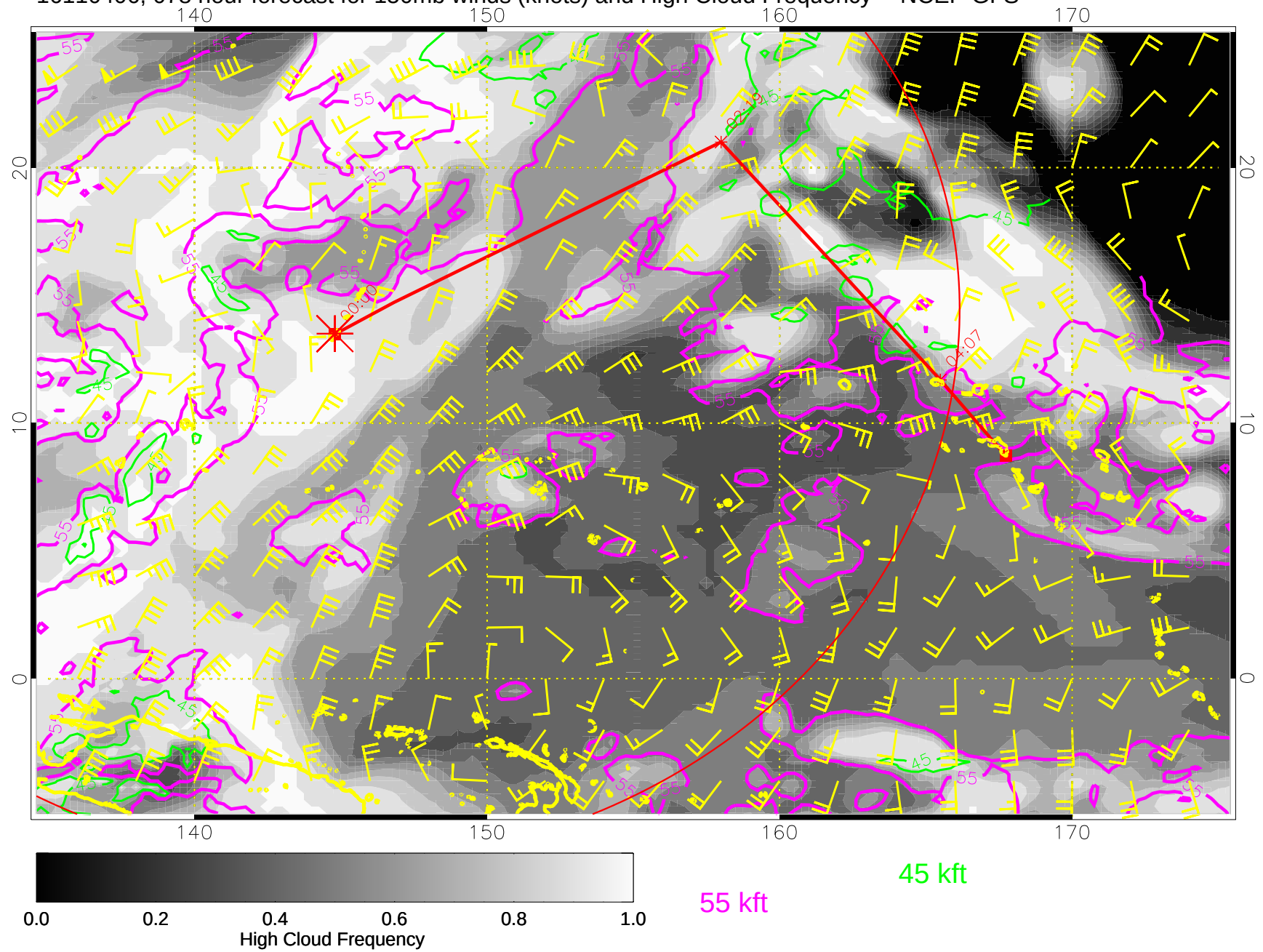
16110406, 078 hour forecast for 150mb winds (knots) and High Cloud Frequency -- NCEP GFS
