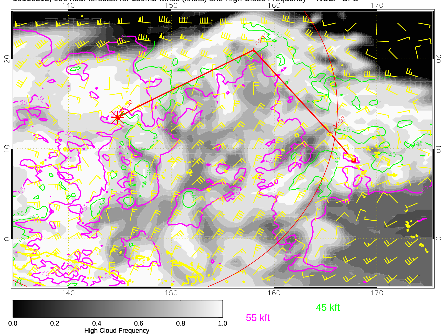
16110212, 036 hour forecast for 150mb winds (knots) and High Cloud Frequency -- NCEP GFS
