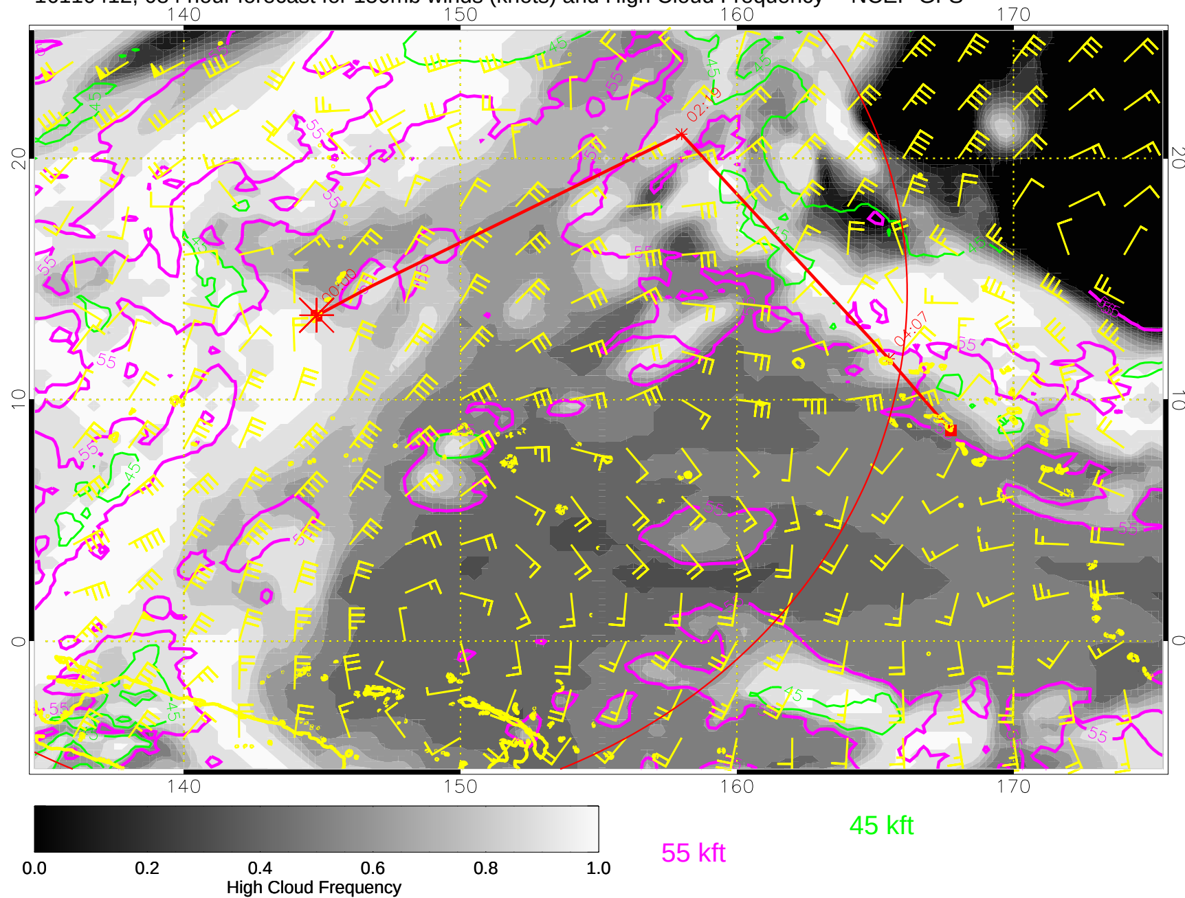
16110412, 084 hour forecast for 150mb winds (knots) and High Cloud Frequency -- NCEP GFS
