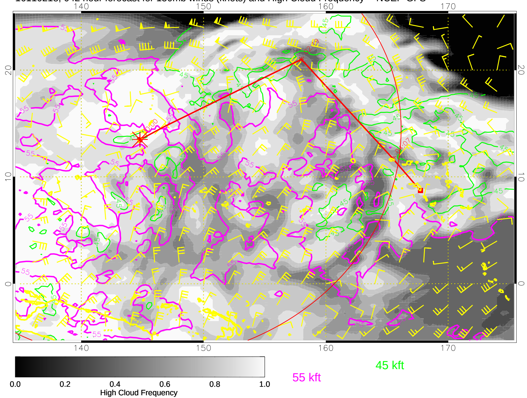
16110218, 04Z hour forecast for 150mb winds (knots) and High Cloud Frequency -- NCEP GFS
