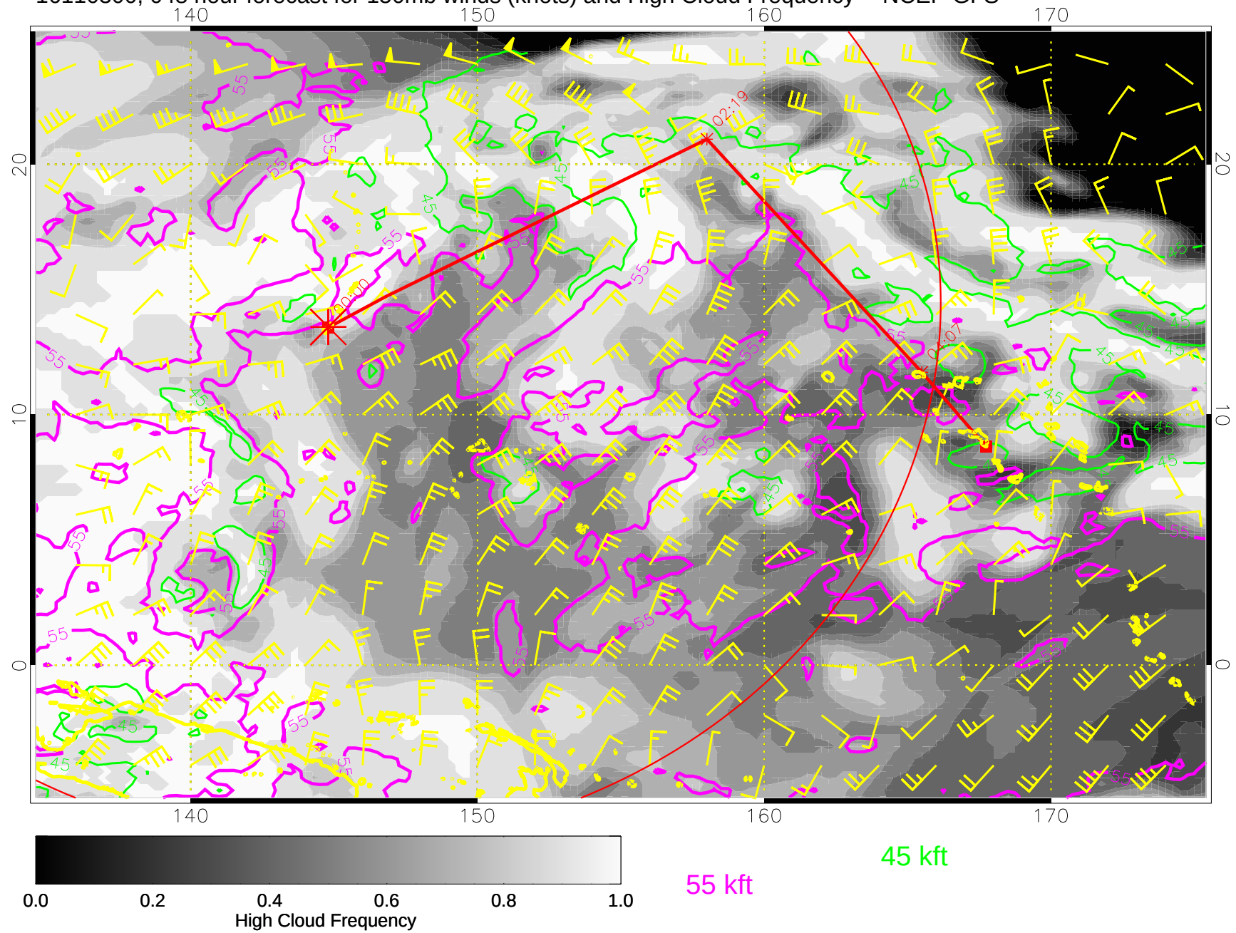
16110300, 048 hour forecast for 150mb winds (knots) and High Cloud Frequency -- NCEP GFS
