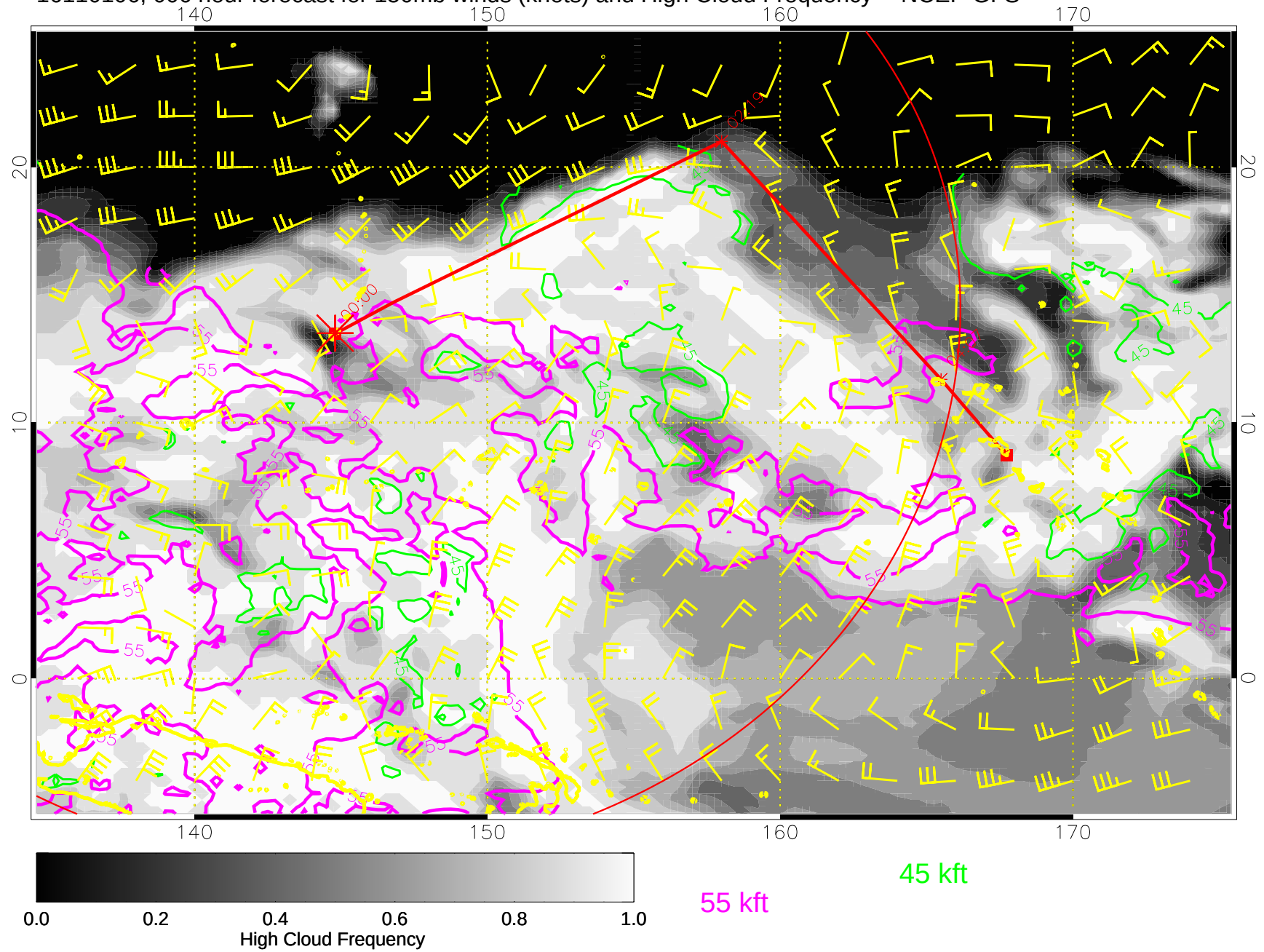
16110106, 006 hour forecast for 150mb winds (knots) and High Cloud Frequency -- NCEP GFS
