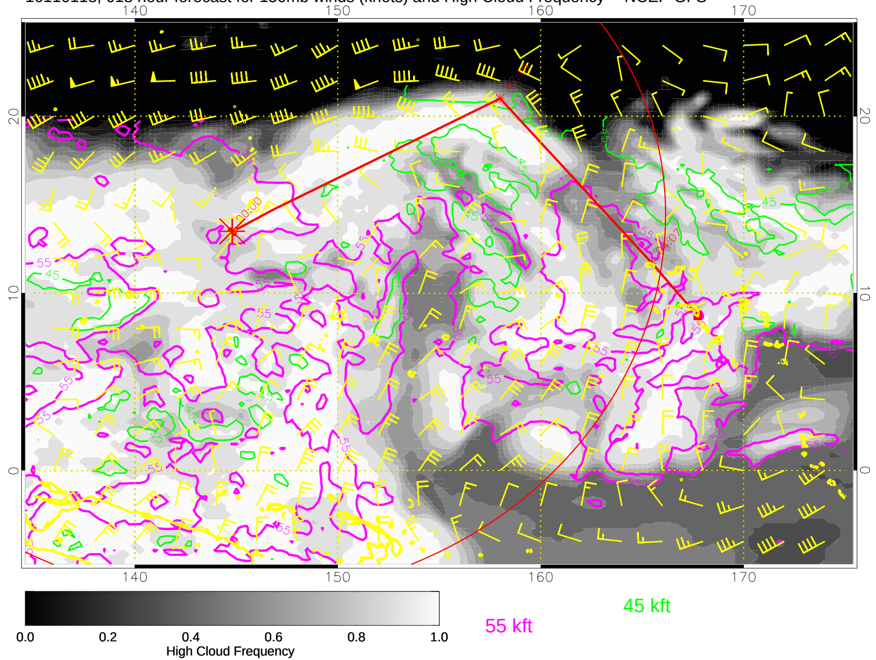
16110118, 018 hour forecast for 150mb winds (knots) and High Cloud Frequency -- NCEP GFS
