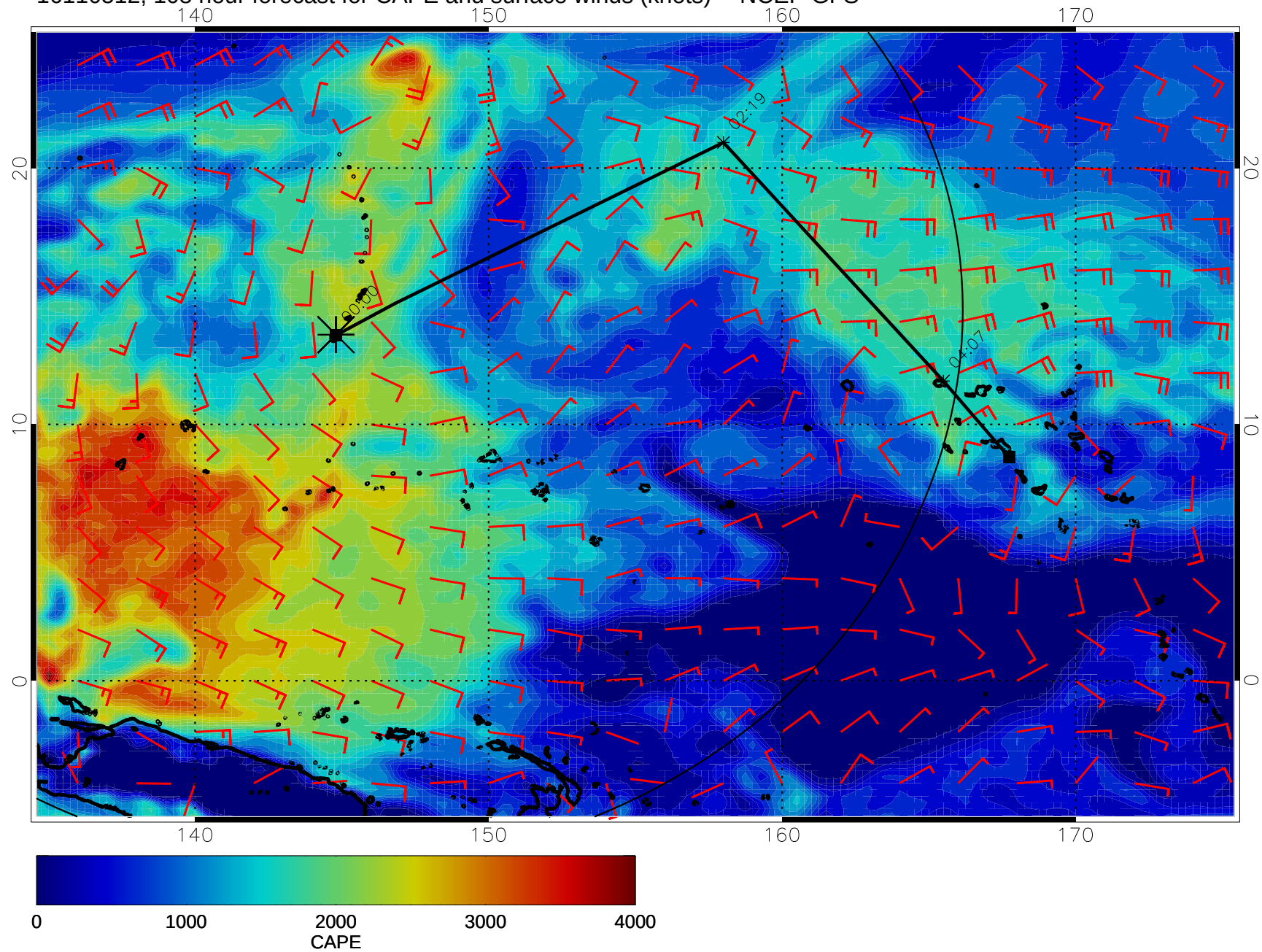
16110512, 108 hour forecast for CAPE and surface winds (knots) -- NCEP GFS
