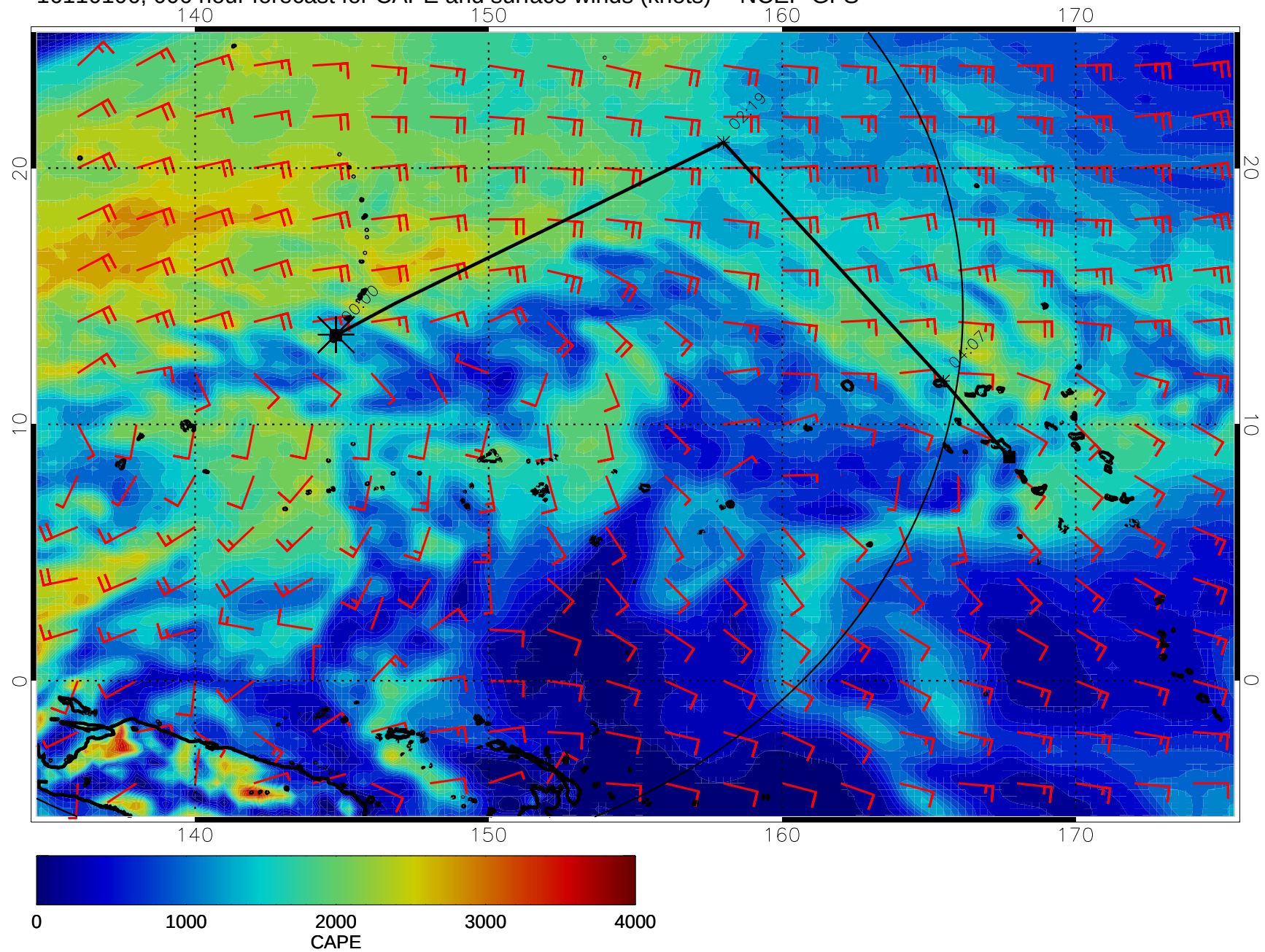
16110106, 006 hour forecast for CAPE and surface winds (knots) -- NCEP GFS
