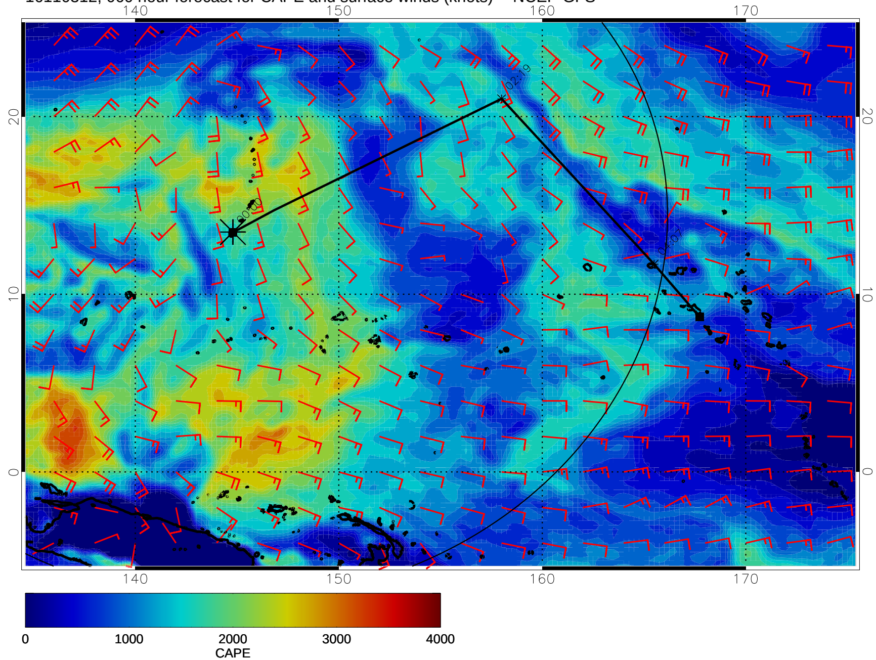
16110312, 060 hour forecast for CAPE and surface winds (knots) -- NCEP GFS
