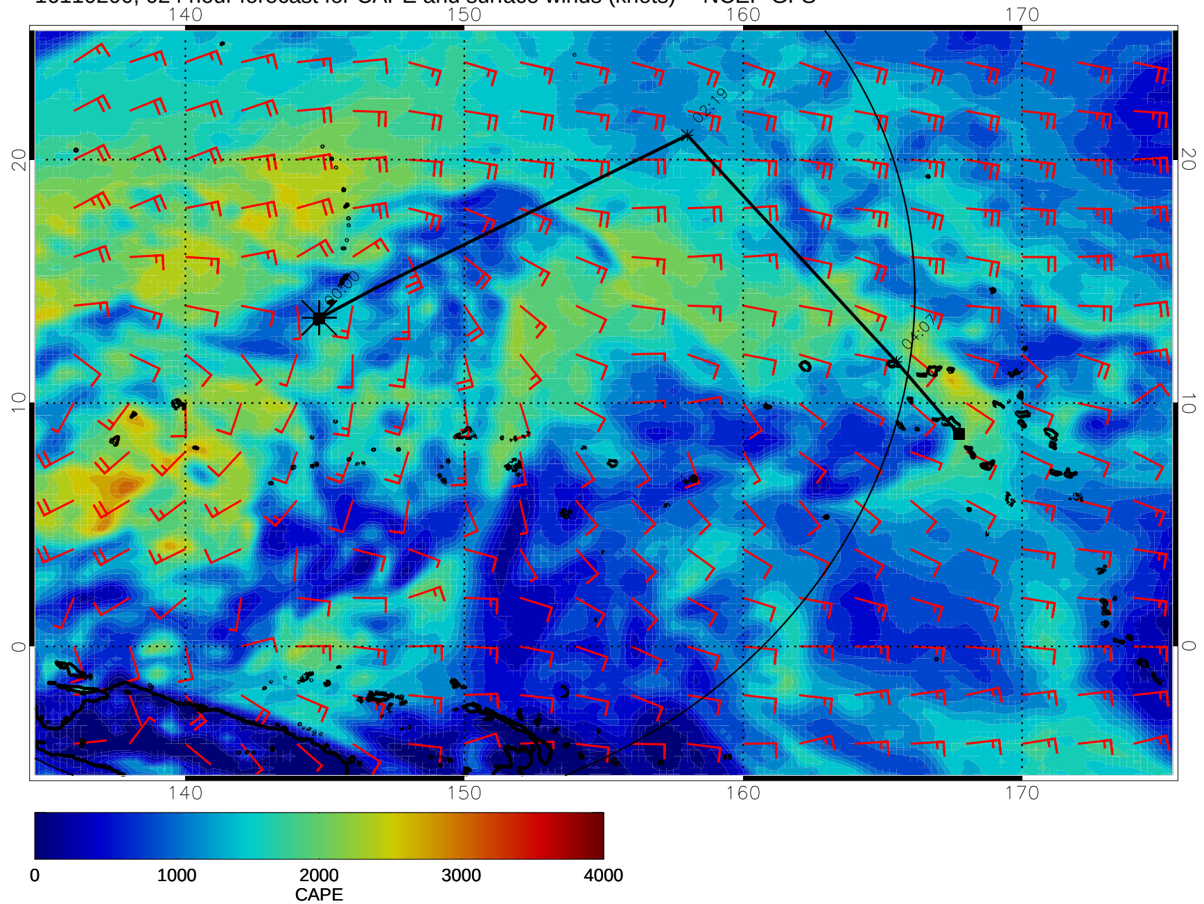
16110200, 024 hour forecast for CAPE and surface winds (knots) -- NCEP GFS
