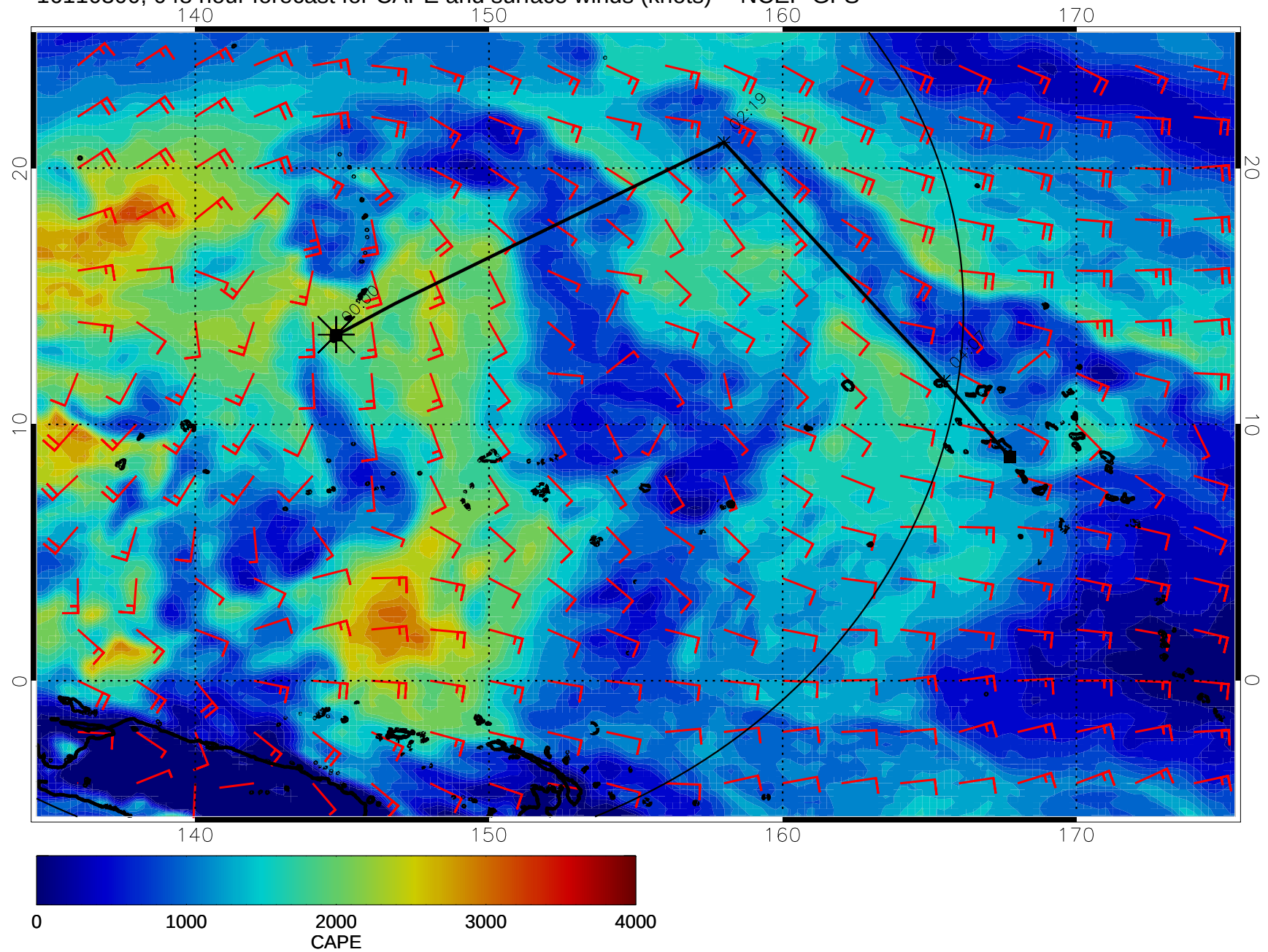
16110300, 048 hour forecast for CAPE and surface winds (knots) -- NCEP GFS
