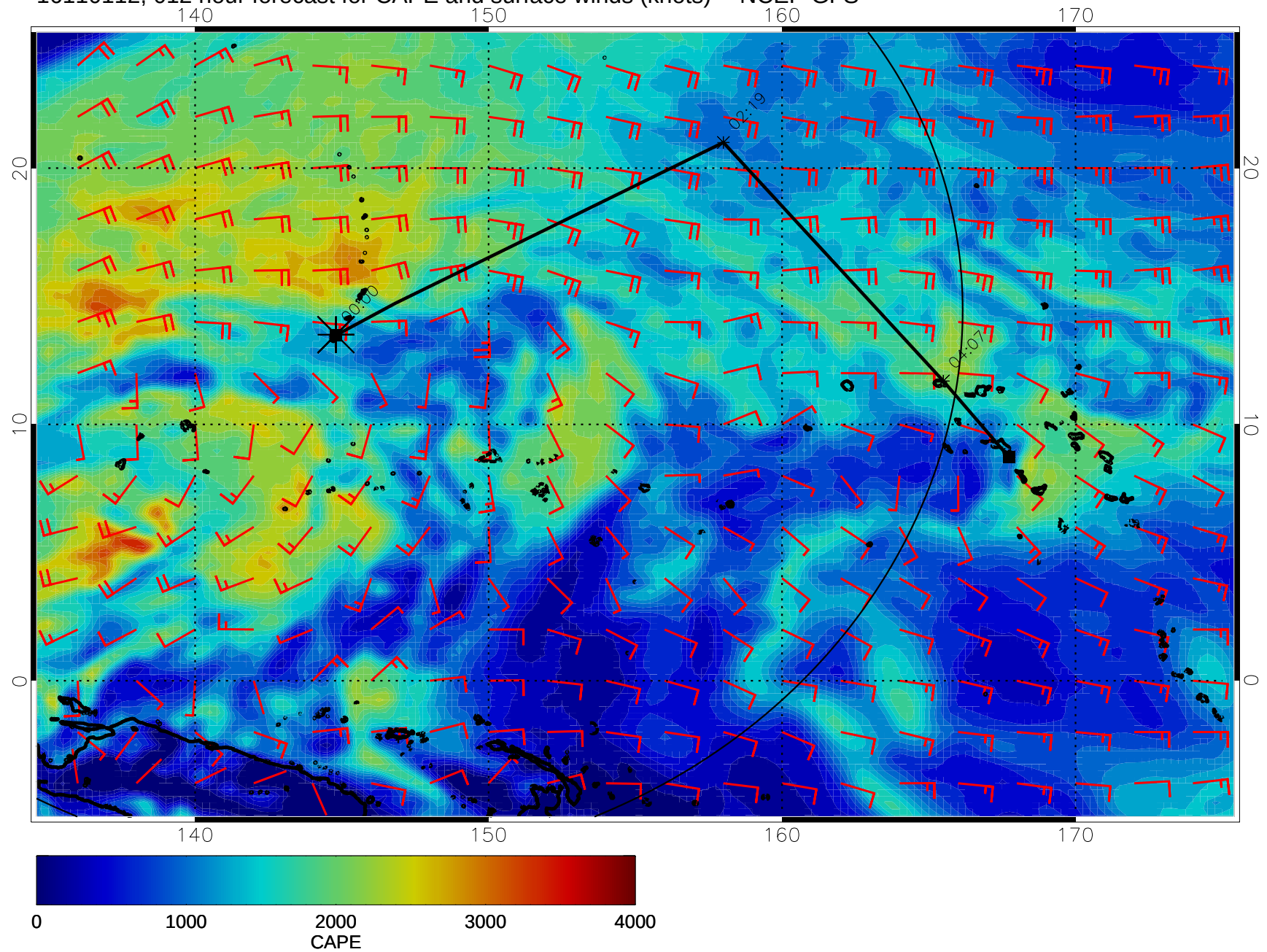
16110112, 012 hour forecast for CAPE and surface winds (knots) -- NCEP GFS
