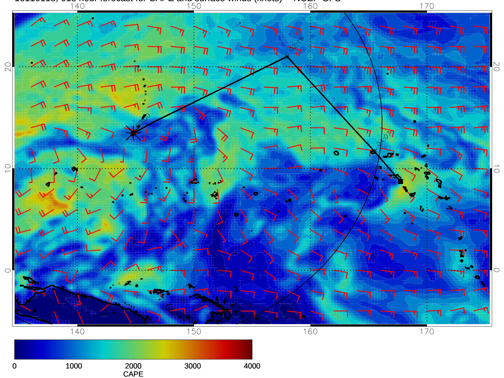
16110118, 018 hour forecast for CAPE and surface winds (knots) -- NCEP GFS
