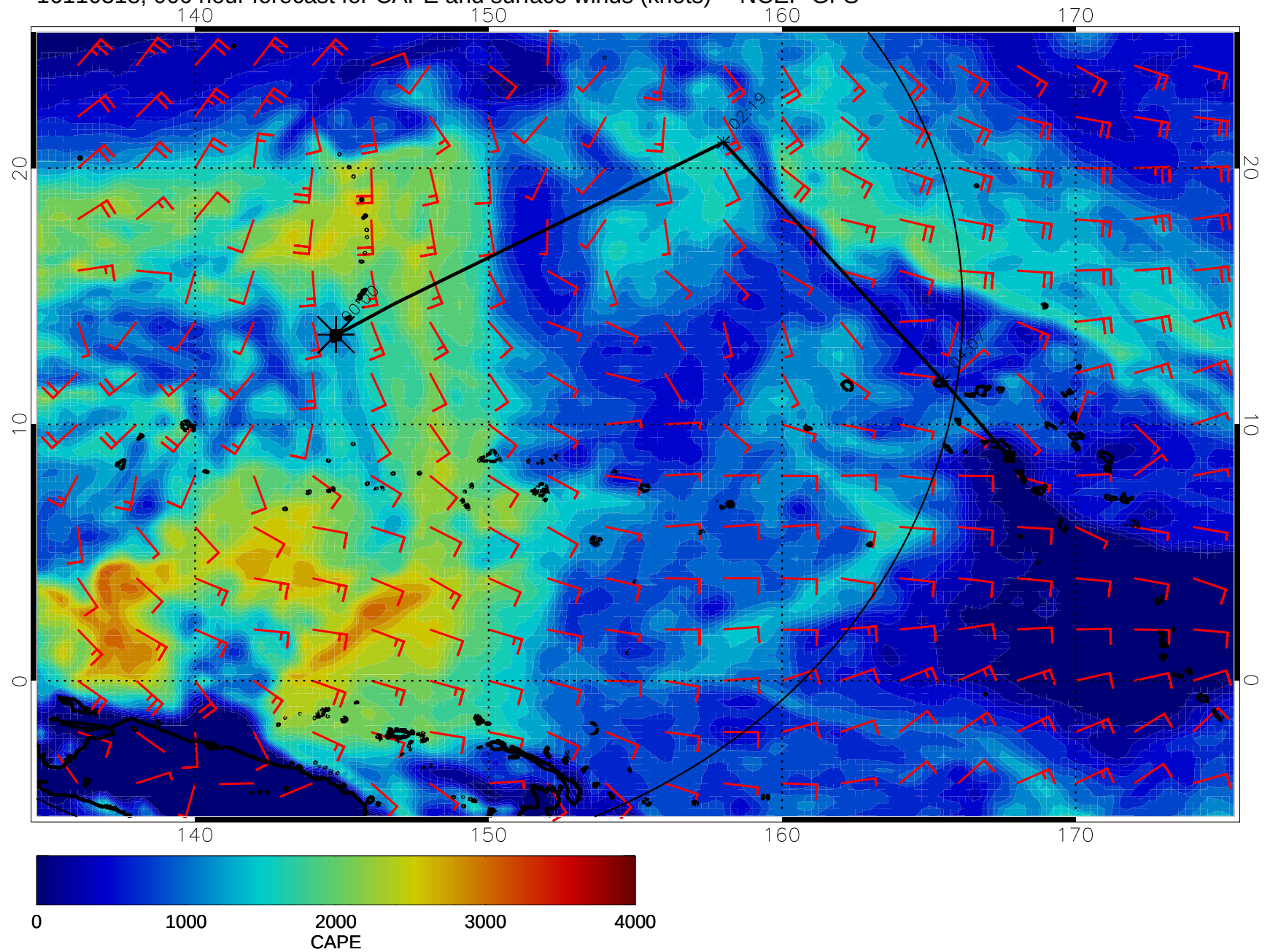
16110318, 066 hour forecast for CAPE and surface winds (knots) -- NCEP GFS
