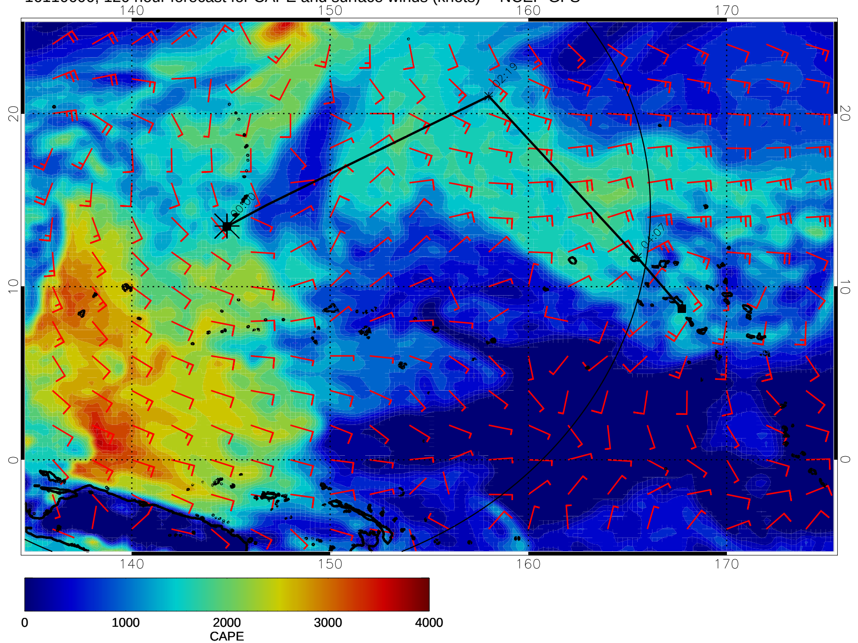
16110600, 120 hour forecast for CAPE and surface winds (knots) -- NCEP GFS
