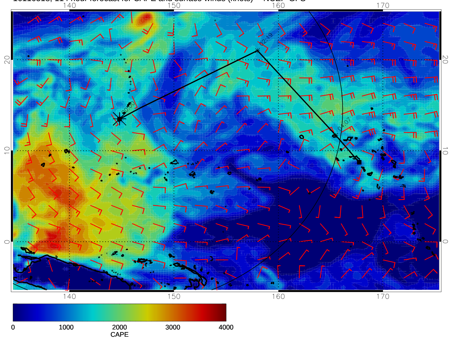
16110518, 114 hour forecast for CAPE and surface winds (knots) -- NCEP GFS
