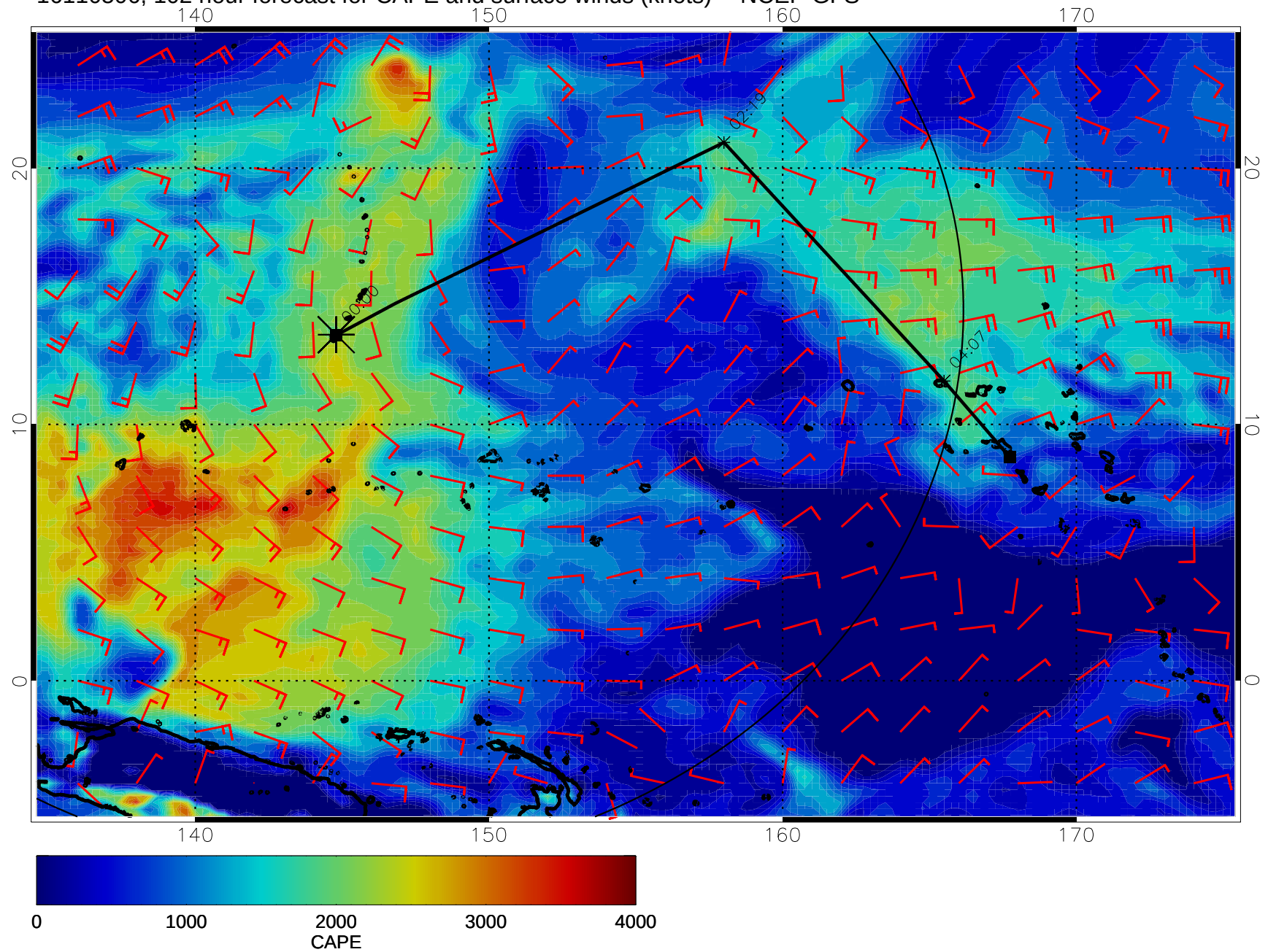
16110506, 102 hour forecast for CAPE and surface winds (knots) -- NCEP GFS
