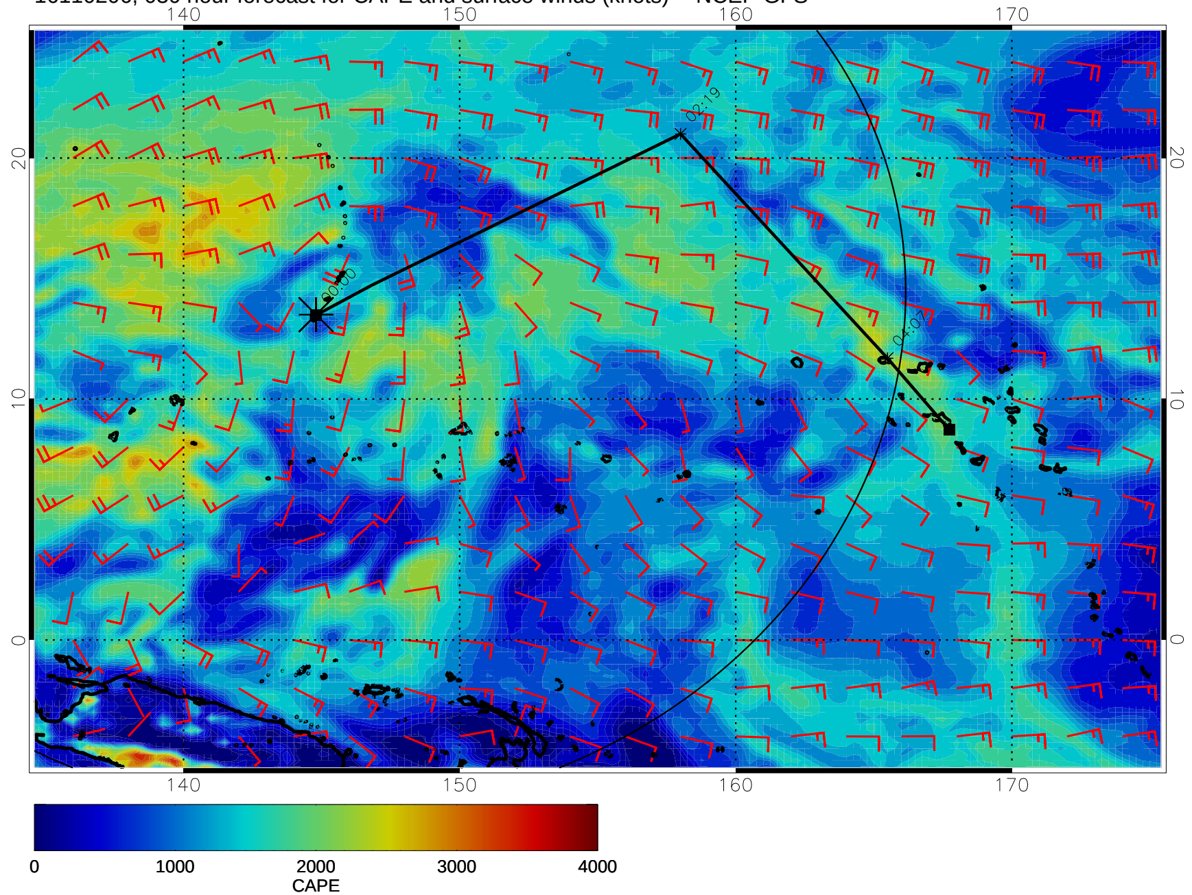
16110206, 0300 hour forecast for CAPE and surface winds (knots) -- NCEP GFS
