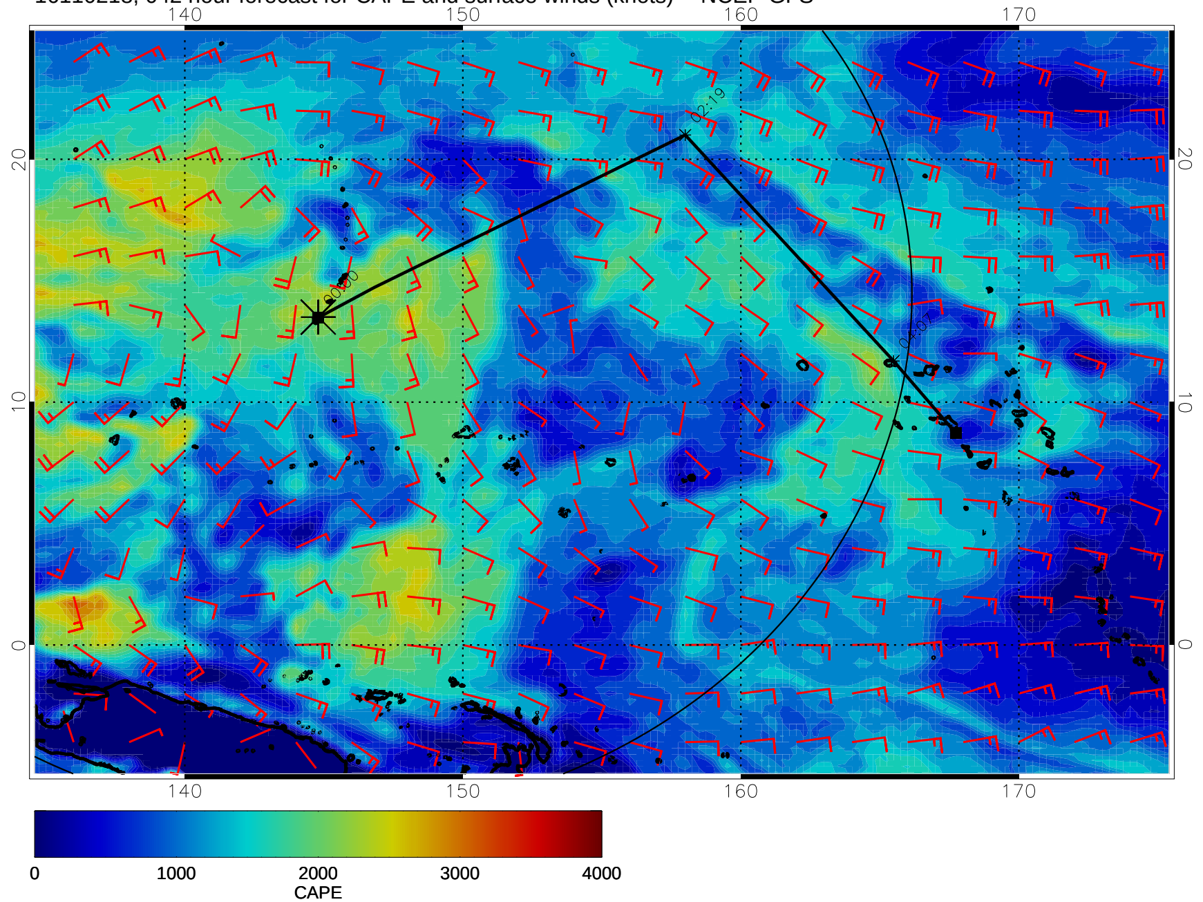
16110218, 042 hour forecast for CAPE and surface winds (knots) -- NCEP GFS
