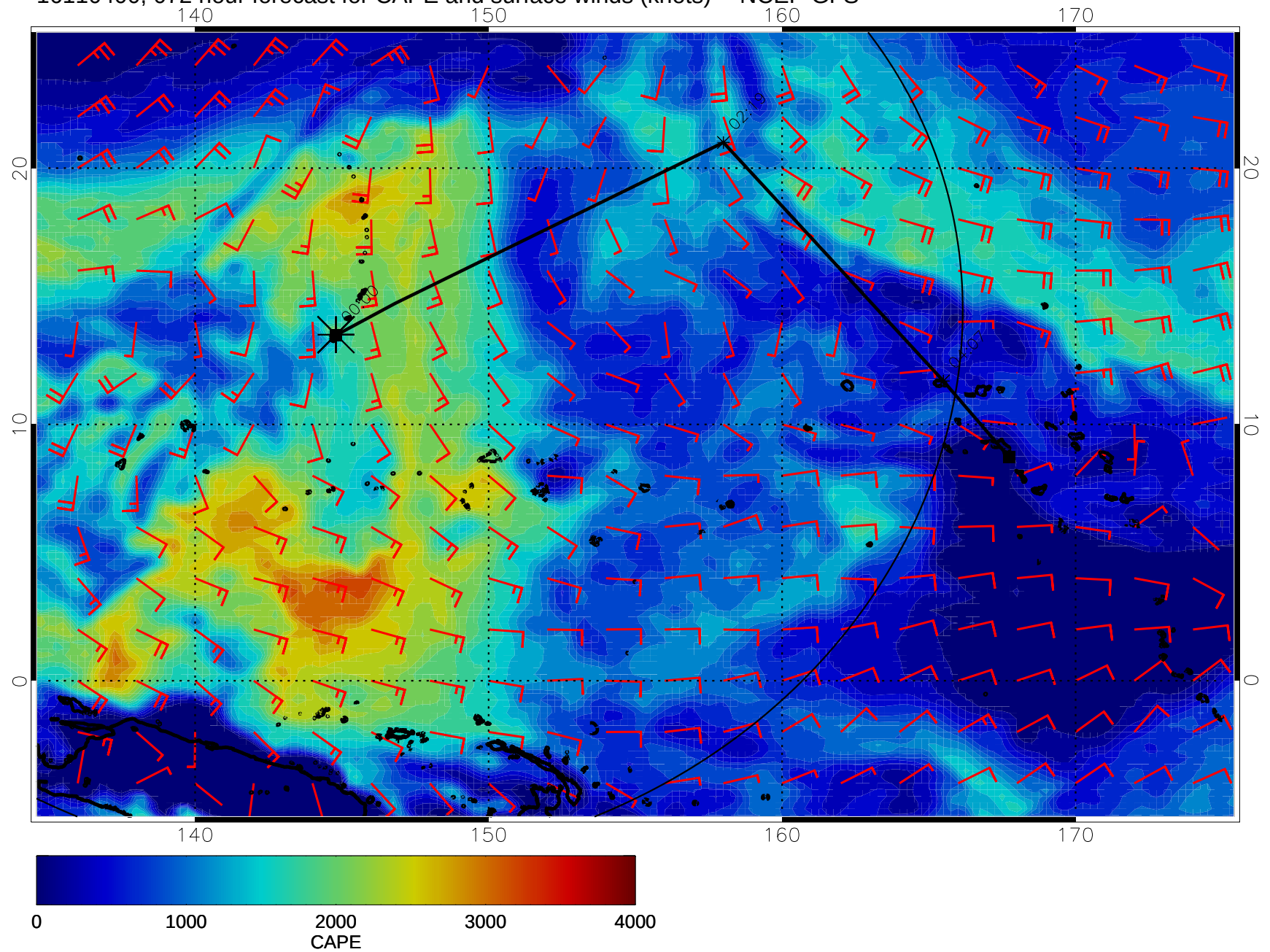
16110400, 072 hour forecast for CAPE and surface winds (knots) -- NCEP GFS
