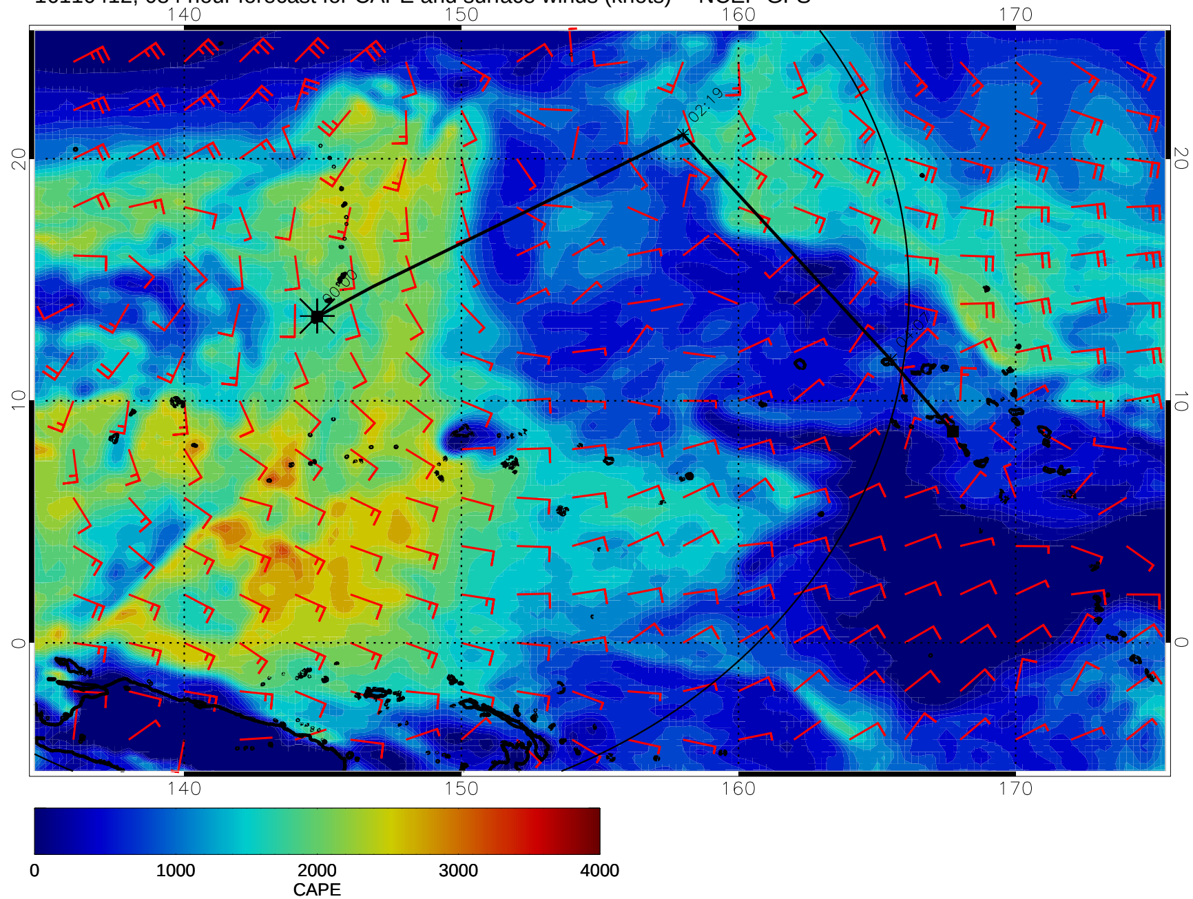
16110412, 084 hour forecast for CAPE and surface winds (knots) -- NCEP GFS
