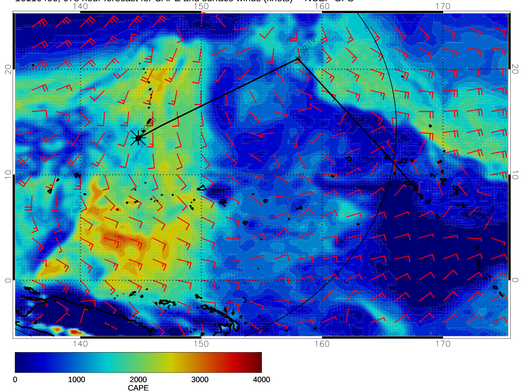
16110406, 078 hour forecast for CAPE and surface winds (knots) -- NCEP GFS
