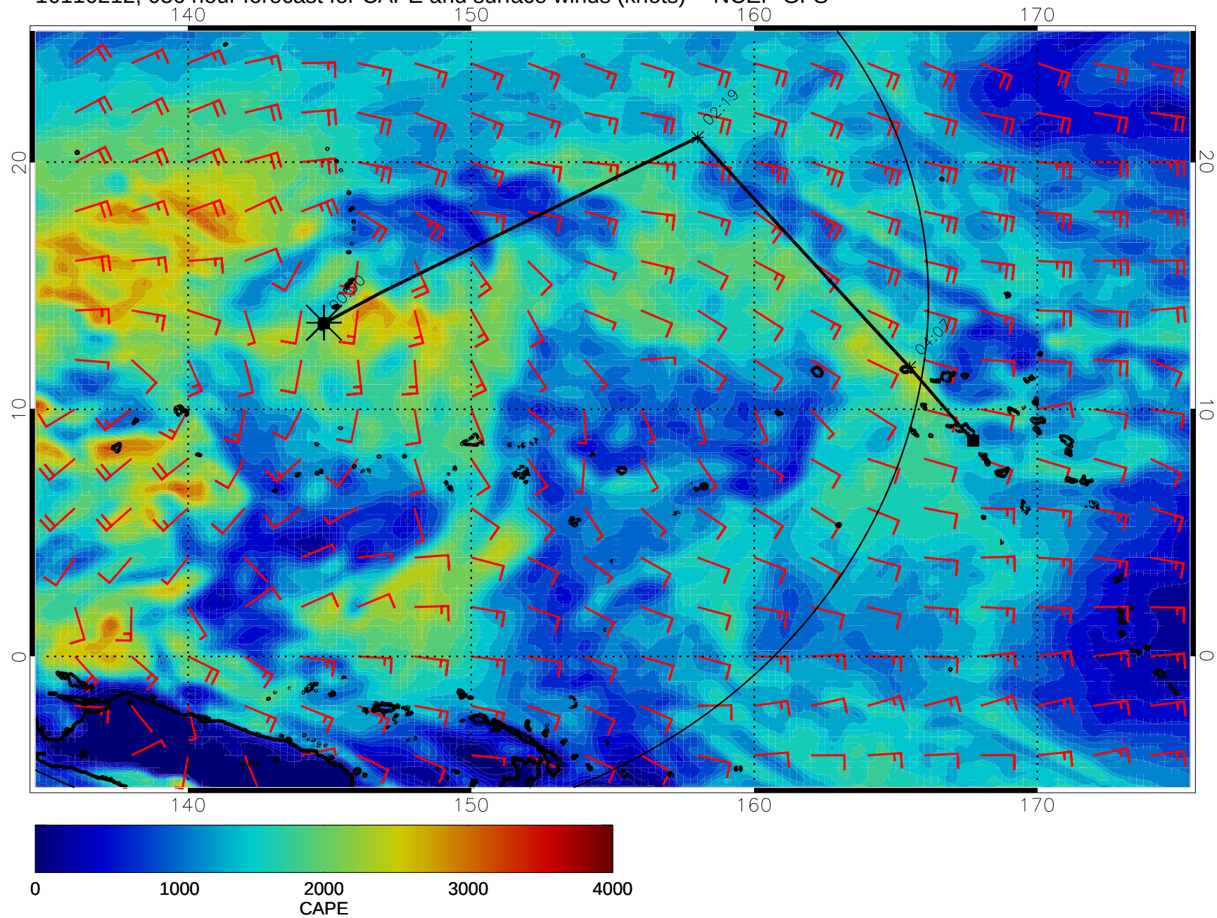
16110212, 036 hour forecast for CAPE and surface winds (knots) -- NCEP GFS
