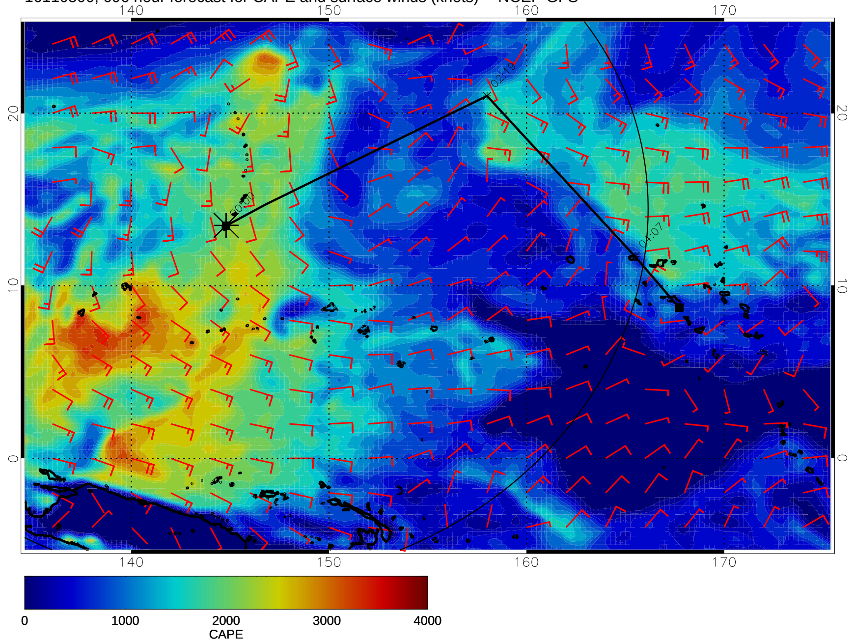
16110500, 096 hour forecast for CAPE and surface winds (knots) -- NCEP GFS
