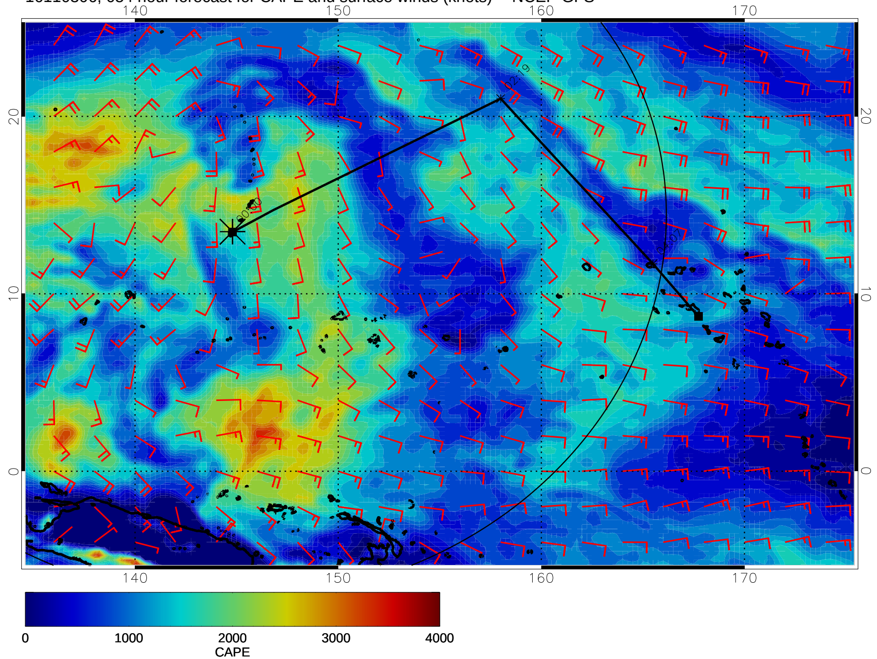
16110306, 054 hour forecast for CAPE and surface winds (knots) -- NCEP GFS
