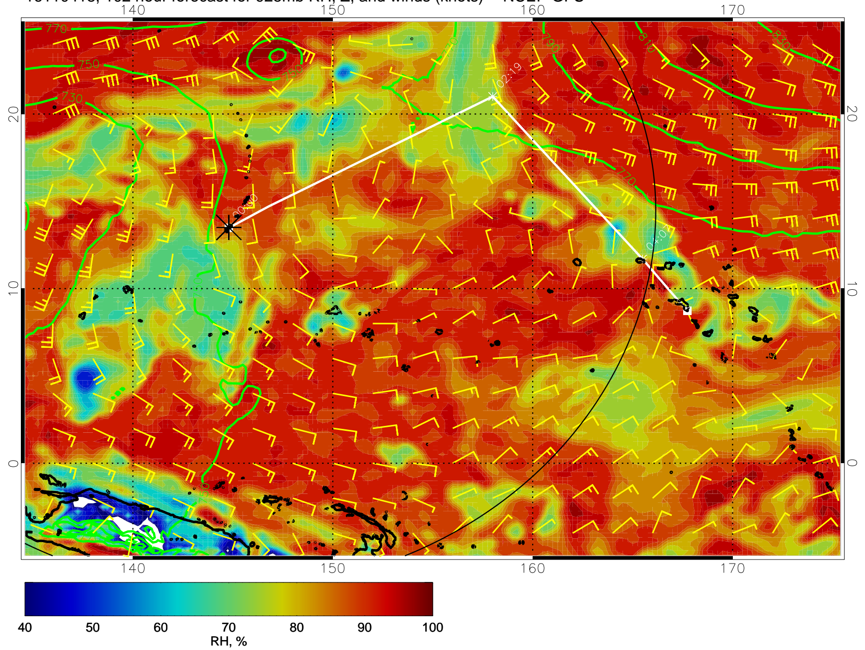
16110418, 102 hour forecast for 925mb RH, Z, and winds (knots) -- NCEP GFS
