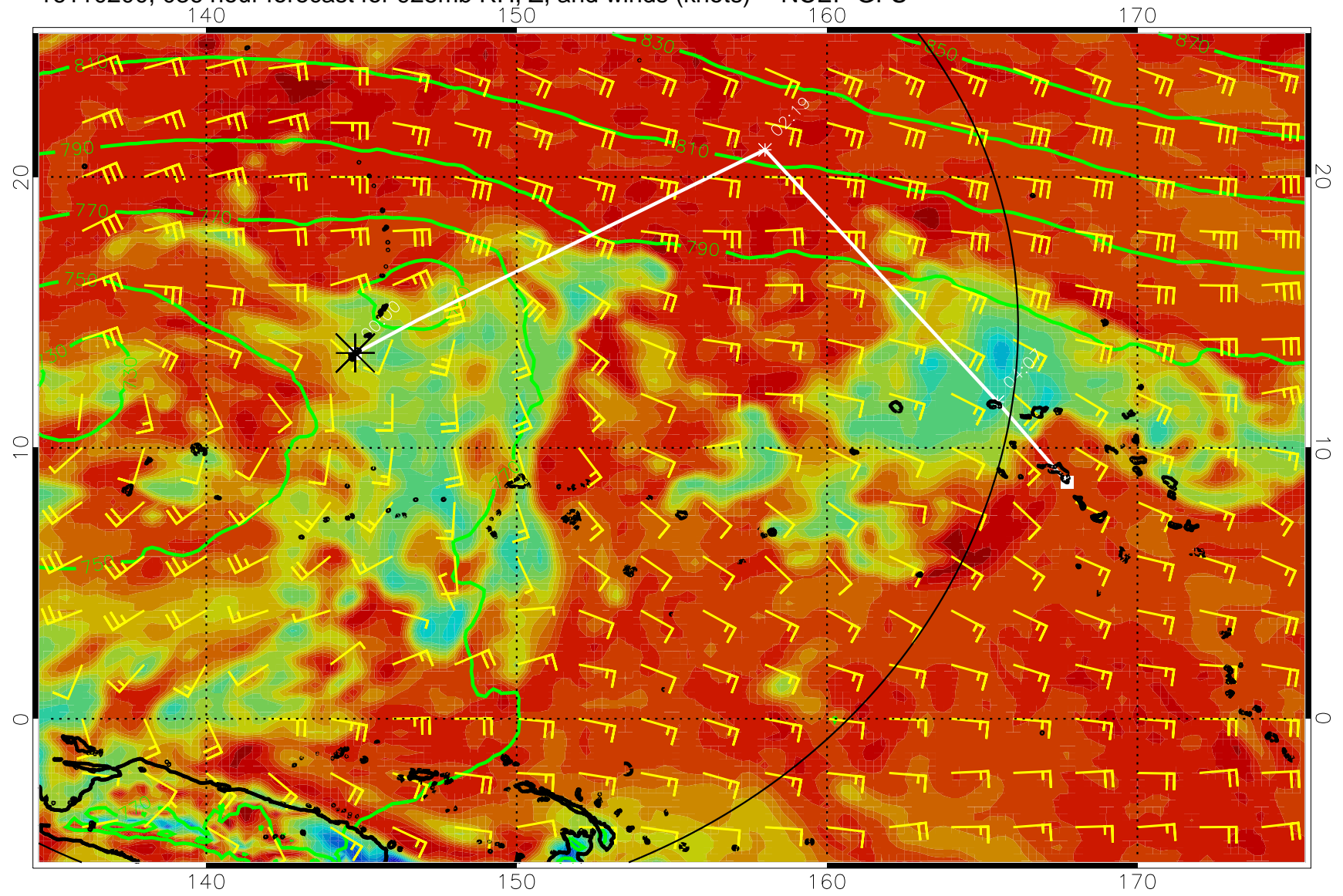
16110200, 036 hour forecast for 925mb RH, Z, and winds (knots) -- NCEP GFS
