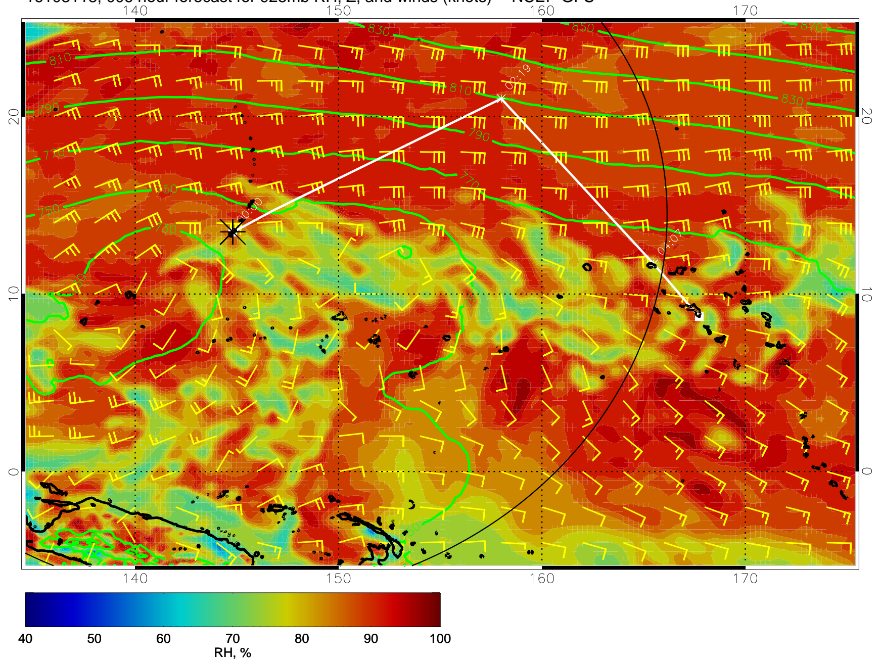
16103118, 006 hour forecast for 925mb RH, Z, and winds (knots) -- NCEP GFS
