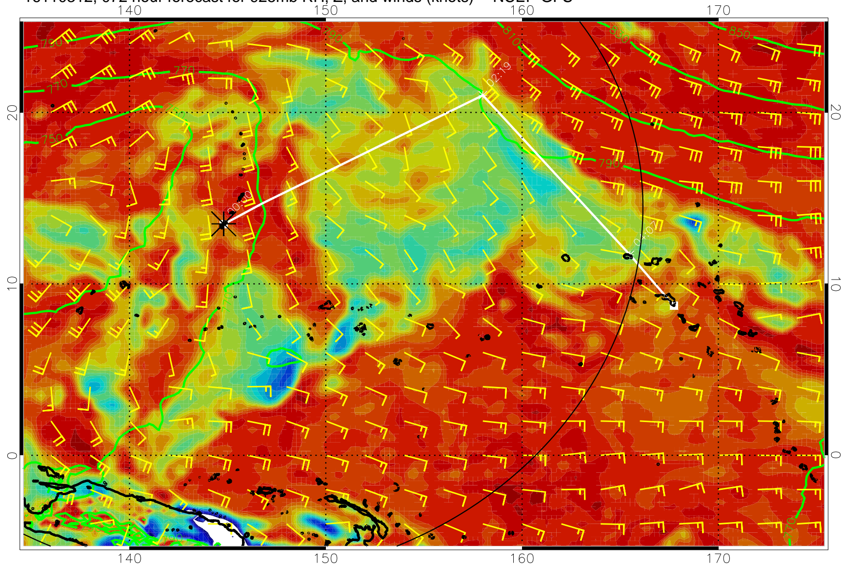
16110312, 072 hour forecast for 925mb RH, Z, and winds (knots) -- NCEP GFS
