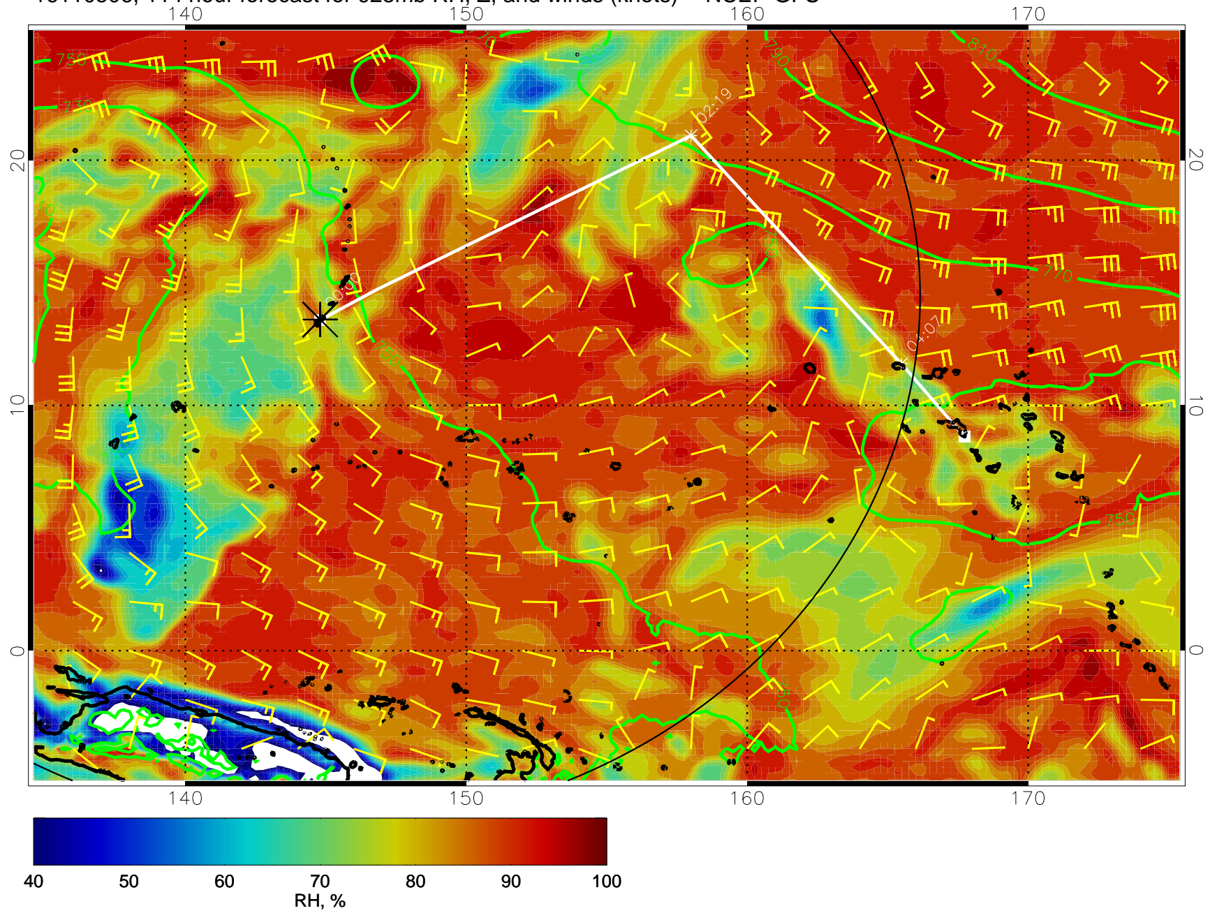
16110506, 114 hour forecast for 925mb RH, Z, and winds (knots) -- NCEP GFS
