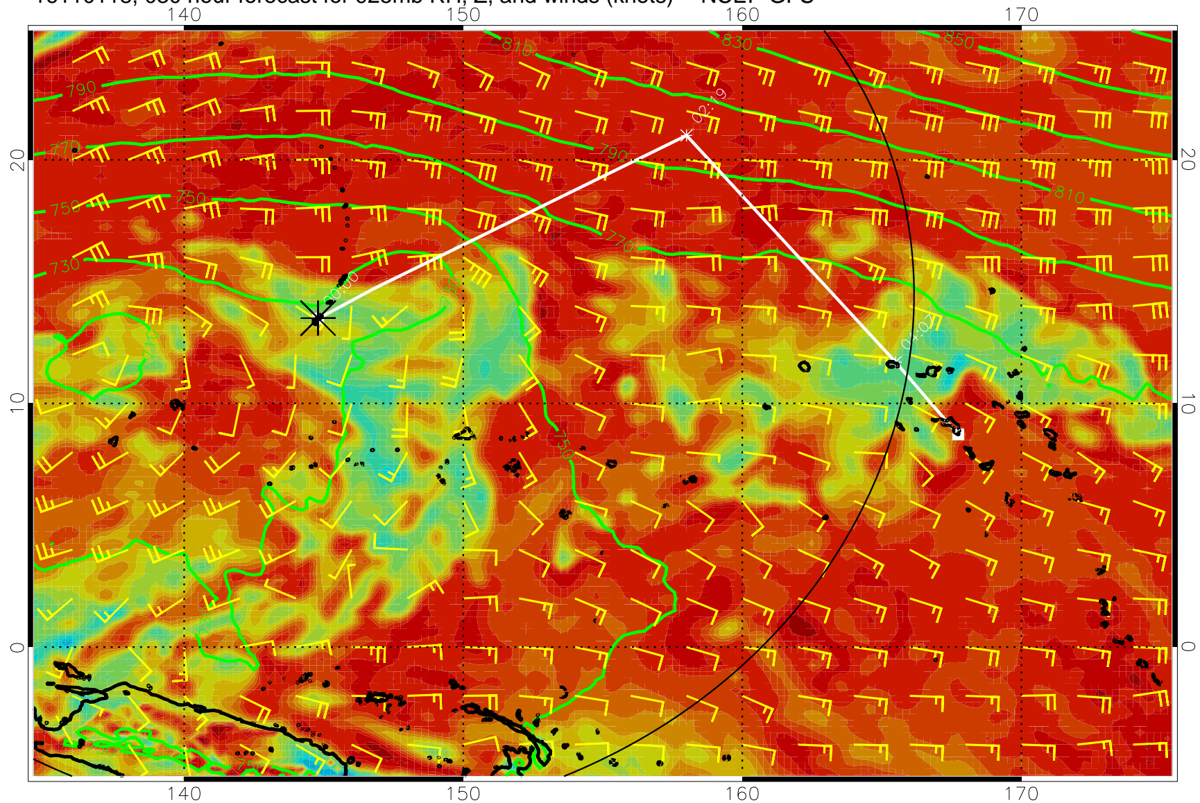
16110118, 030 hour forecast for 925mb RH, Z, and winds (knots) -- NCEP GFS
