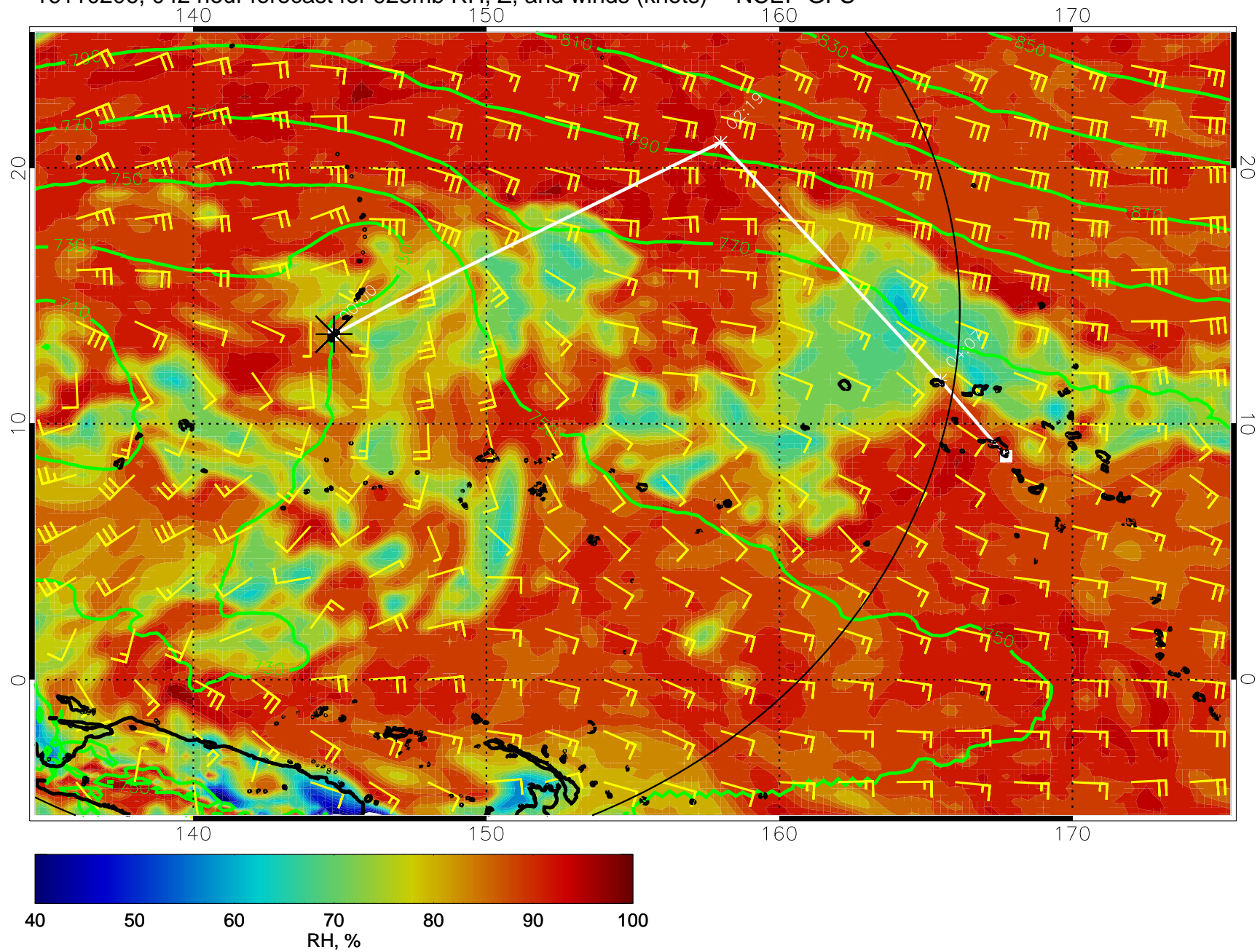
16110206, 042 hour forecast for 925mb RH, Z, and winds (knots) -- NCEP GFS
