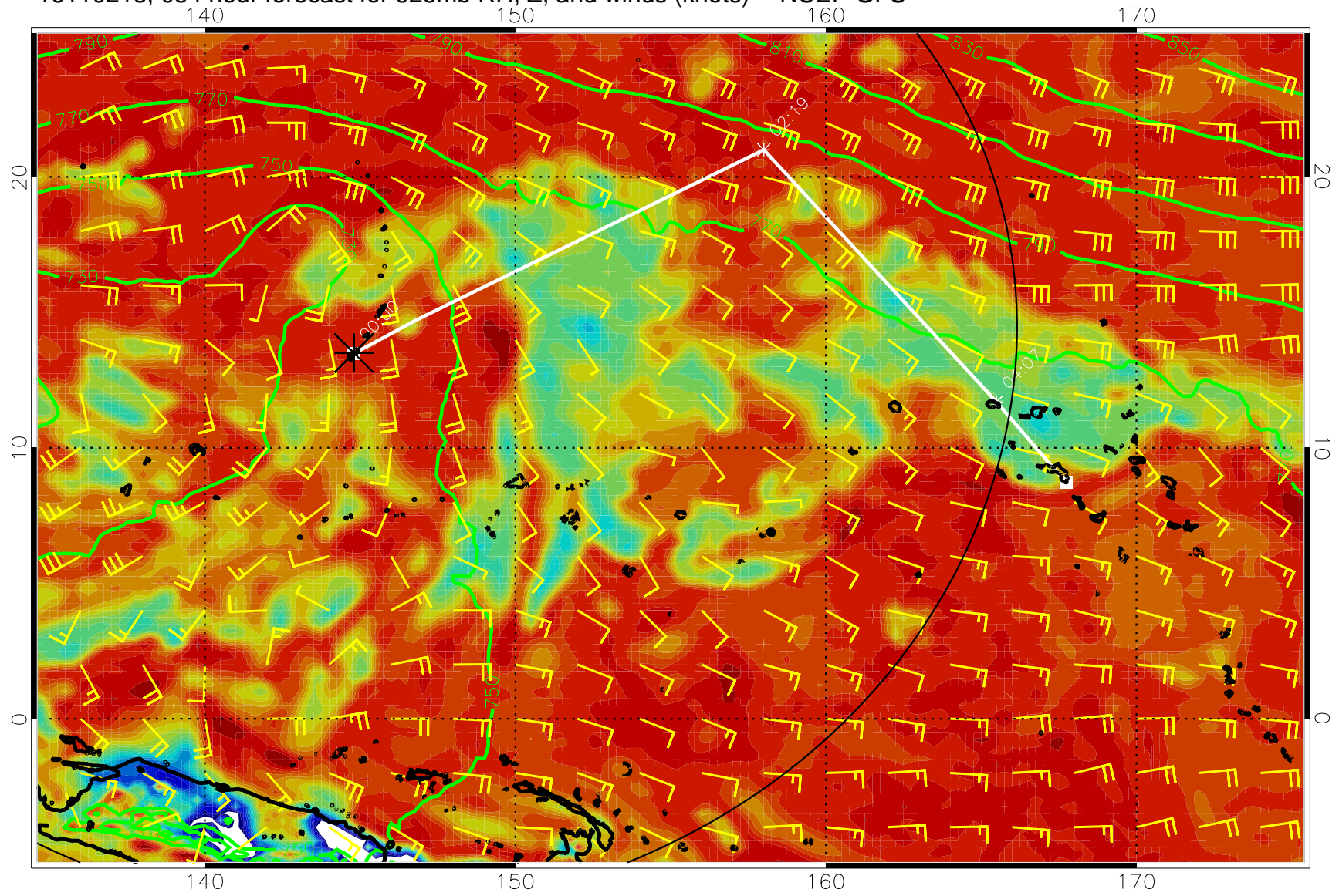
16110218, 054 hour forecast for 925mb RH, Z, and winds (knots) -- NCEP GFS
