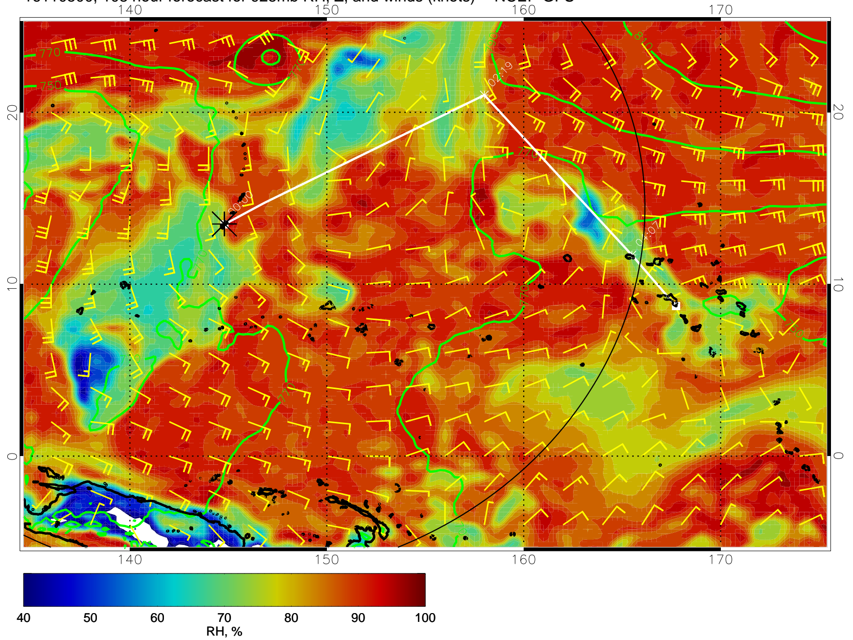
16110500, 108 hour forecast for 925mb RH, Z, and winds (knots) -- NCEP GFS
