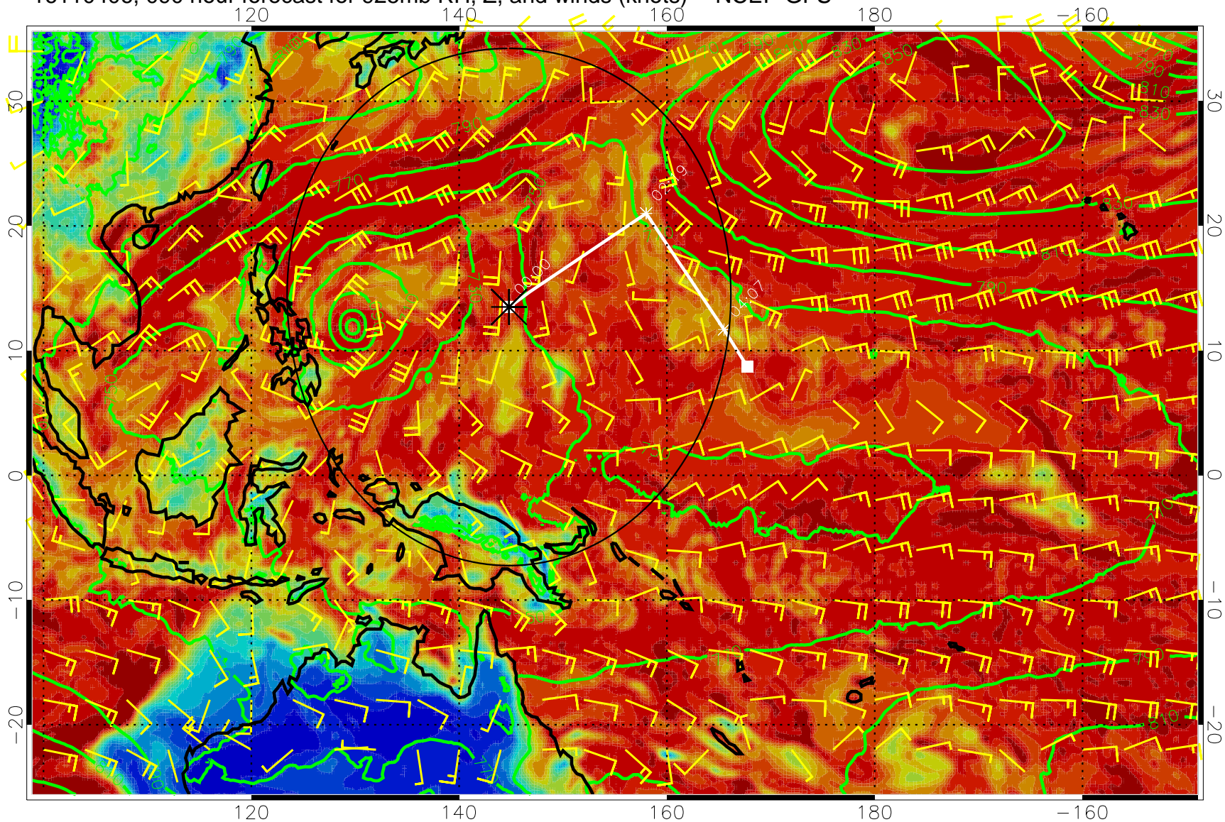
16110406, 090 hour forecast for 925mb RH, Z, and winds (knots) -- NCEP GFS
