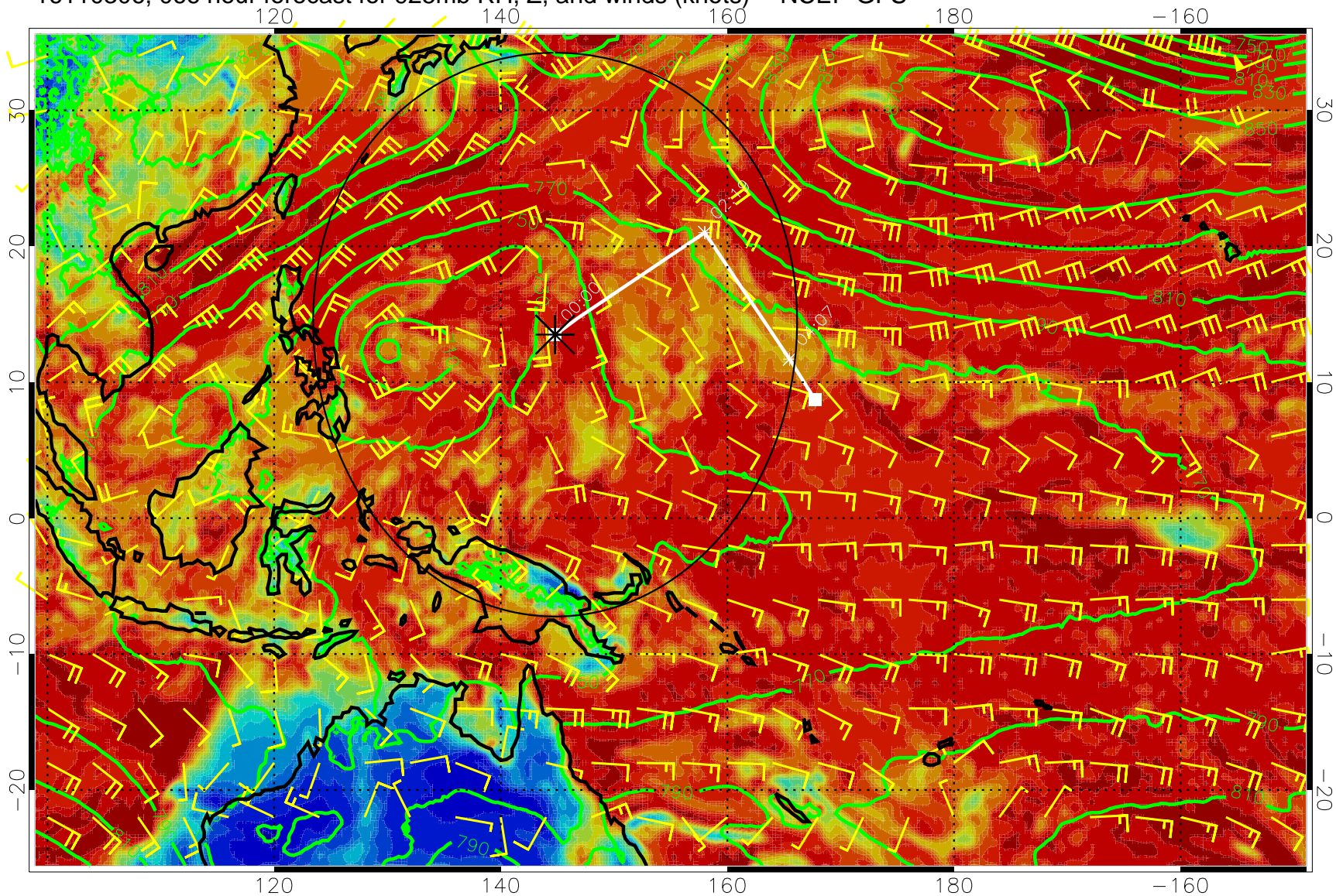
16110306, 066 hour forecast for 925mb RH, Z, and winds (knots) -- NCEP GFS
