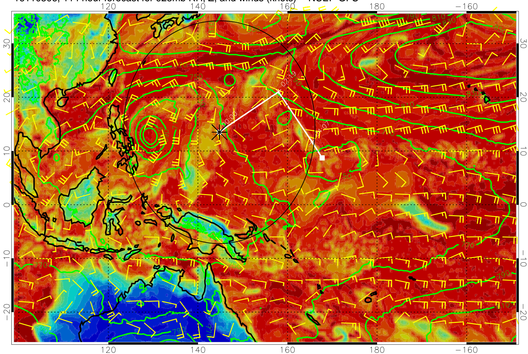
16110506, 114 hour forecast for 925mb RH, Z, and winds (knots) -- NCEP GFS
