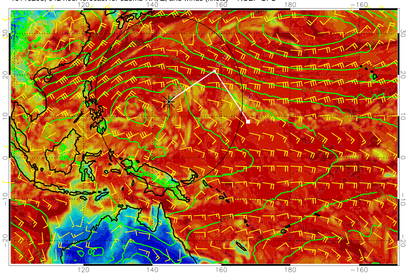
16110206, 042 hour forecast for 925mb RH, Z, and winds (knots) -- NCEP GFS
