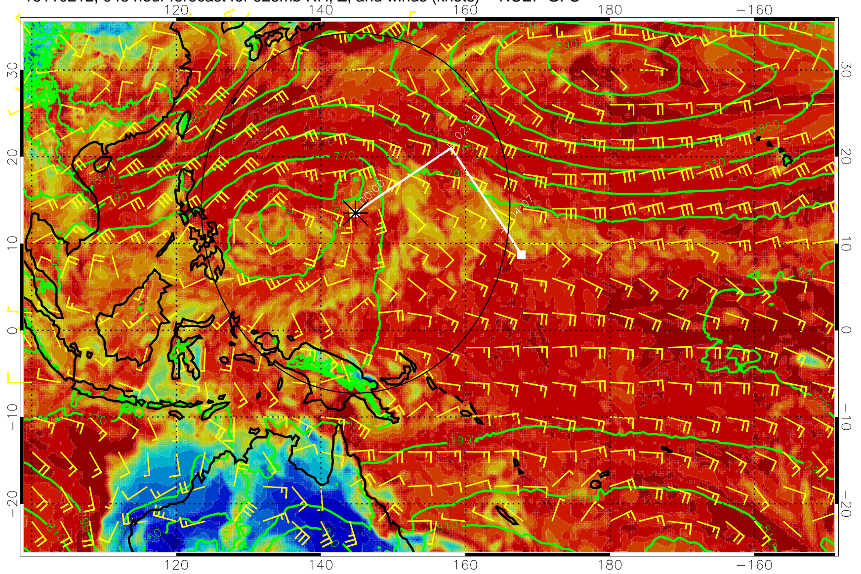
16110212, 048 hour forecast for 925mb RH, Z, and winds (knots) -- NCEP GFS
