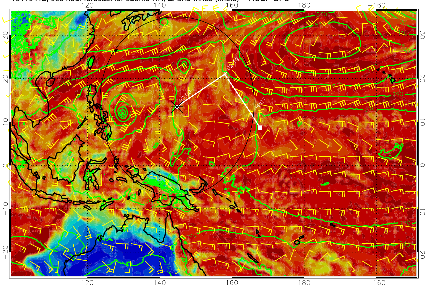
16110412, 096 hour forecast for 925mb RH, Z, and winds (knots) -- NCEP GFS
