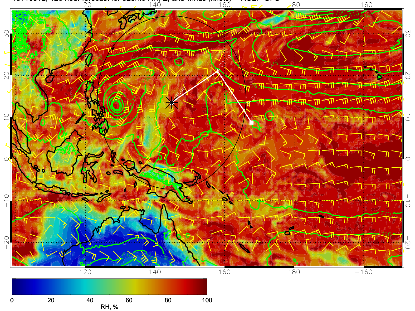
16110512, 120 hour forecast for 925mb RH, Z, and winds (knots) -- NCEP GFS
