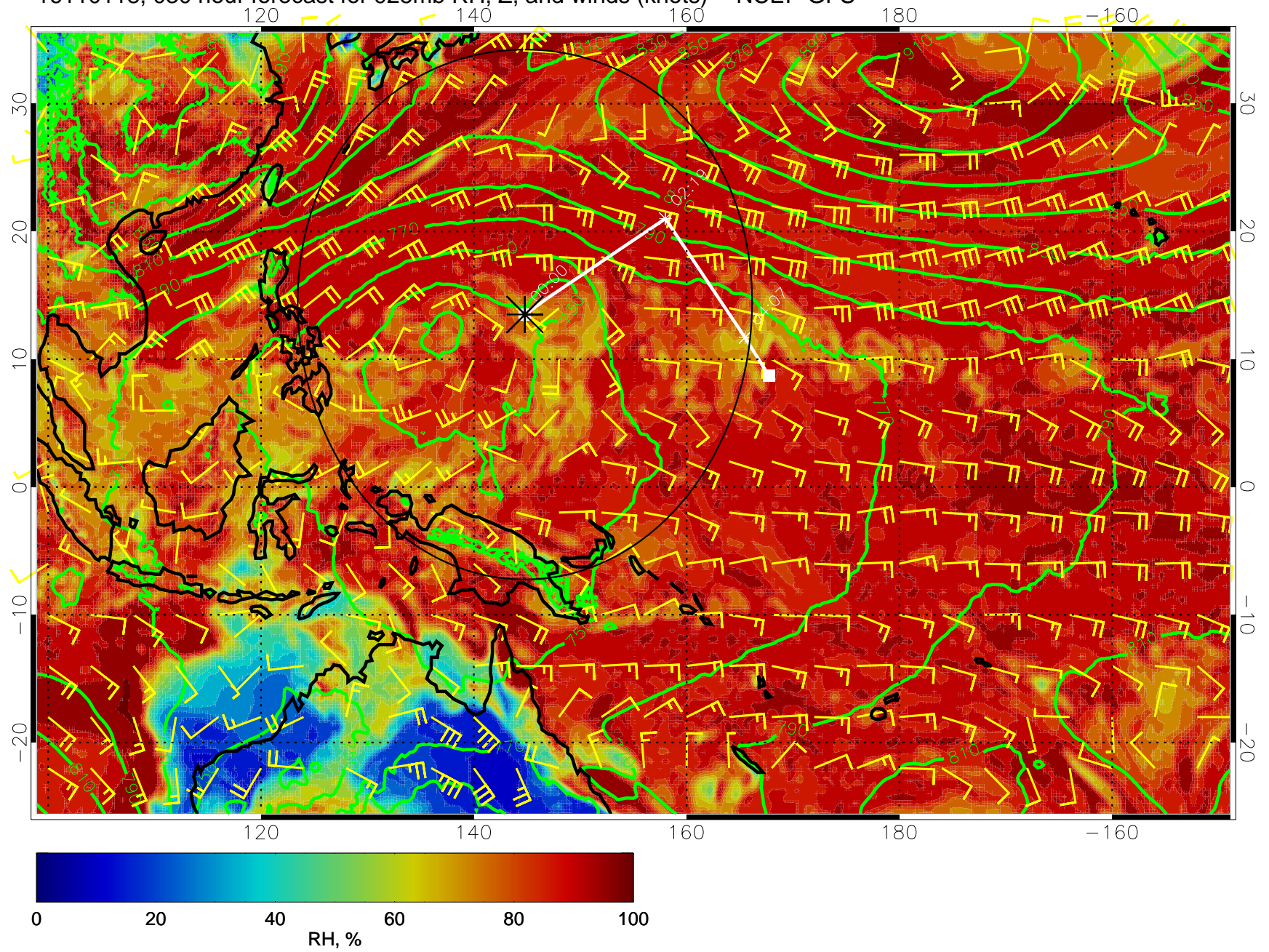
16110118, 030 hour forecast for 925mb RH, Z, and winds (knots) -- NCEP GFS
