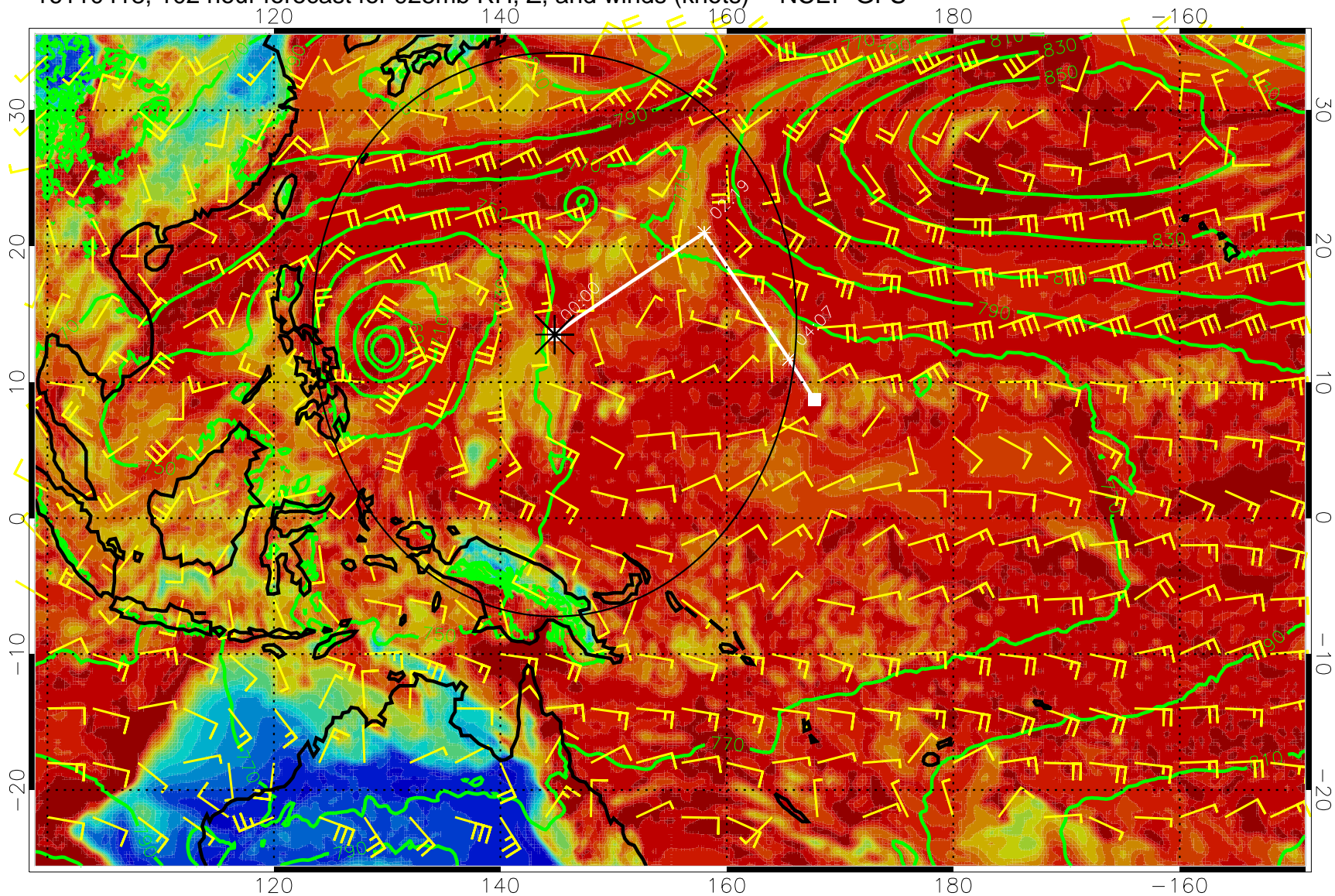
16110418, 102 hour forecast for 925mb RH, Z, and winds (knots) -- NCEP GFS
