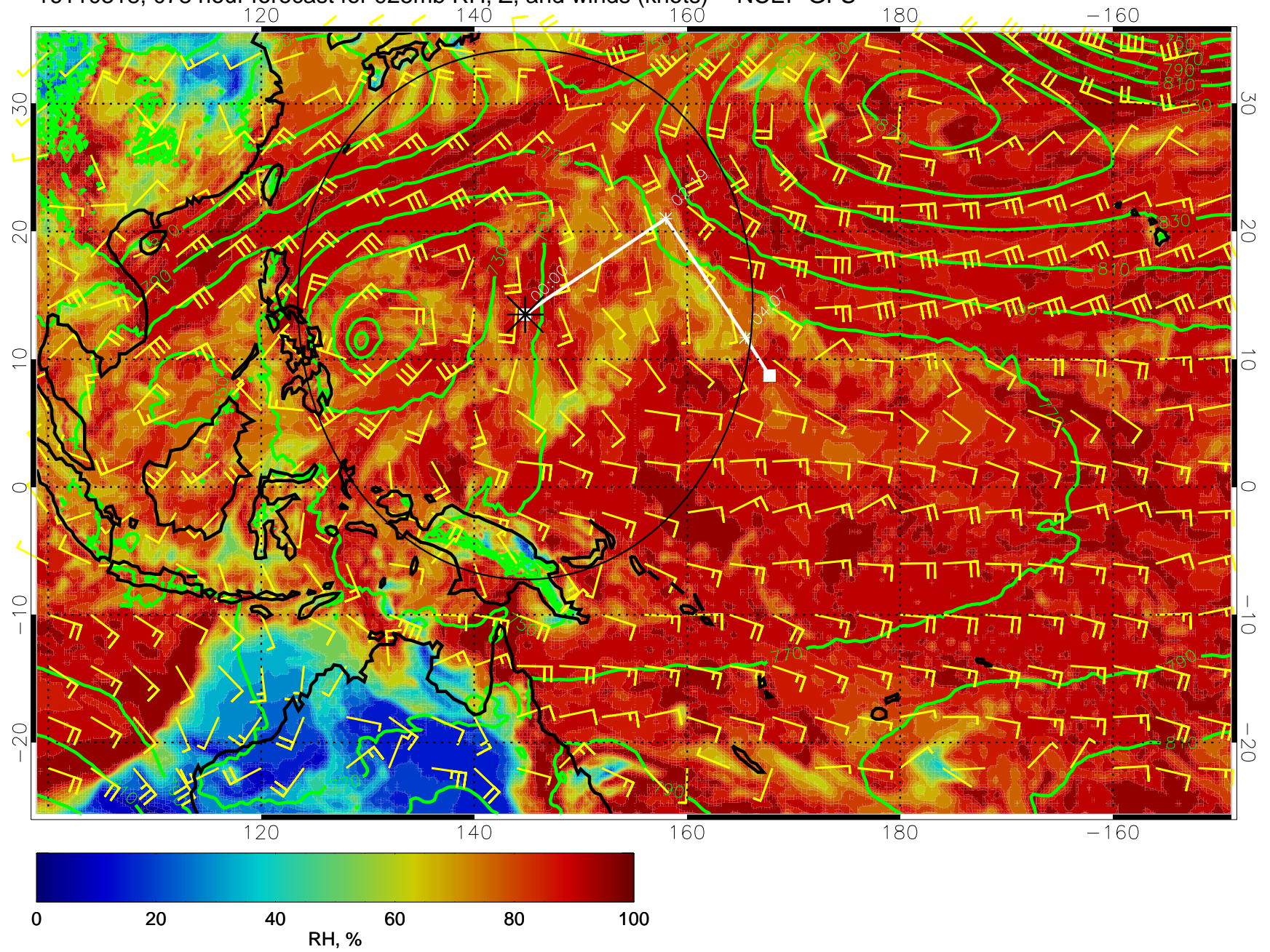
16110318, 078 hour forecast for 925mb RH, Z, and winds (knots) -- NCEP GFS
