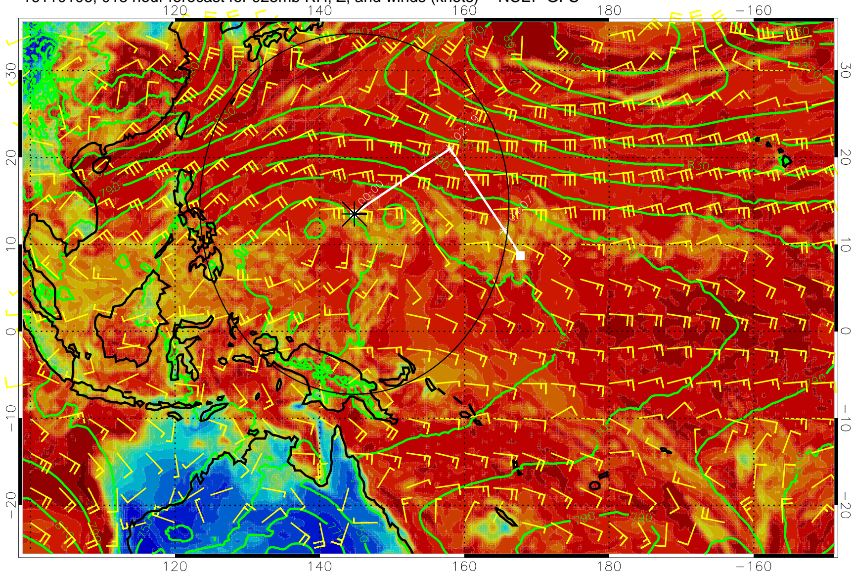
16110106, 018 hour forecast for 925mb RH, Z, and winds (knots) -- NCEP GFS
