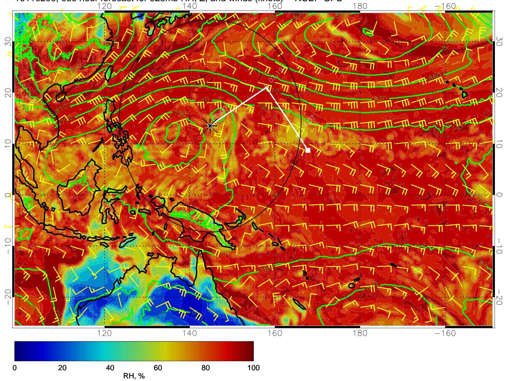
16110200, 036 hour forecast for 925mb RH, Z, and winds (knots) -- NCEP GFS
