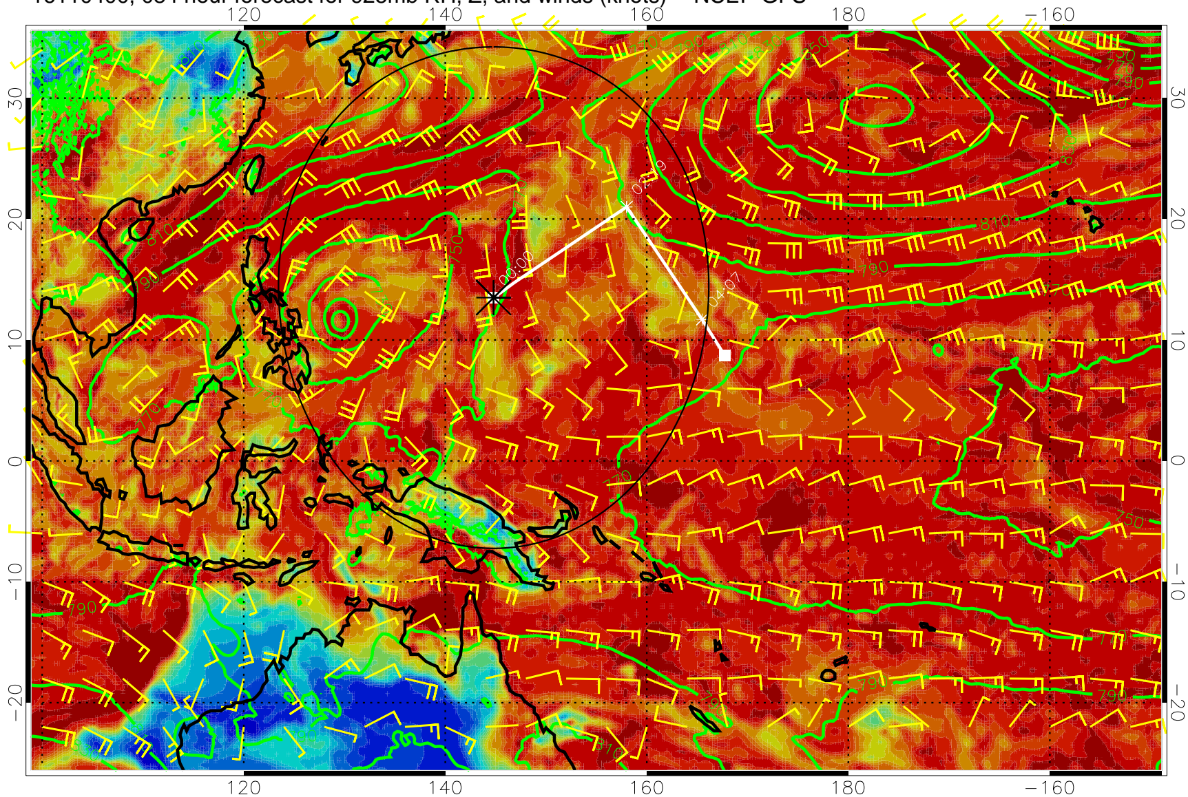
16110400, 084 hour forecast for 925mb RH, Z, and winds (knots) -- NCEP GFS
