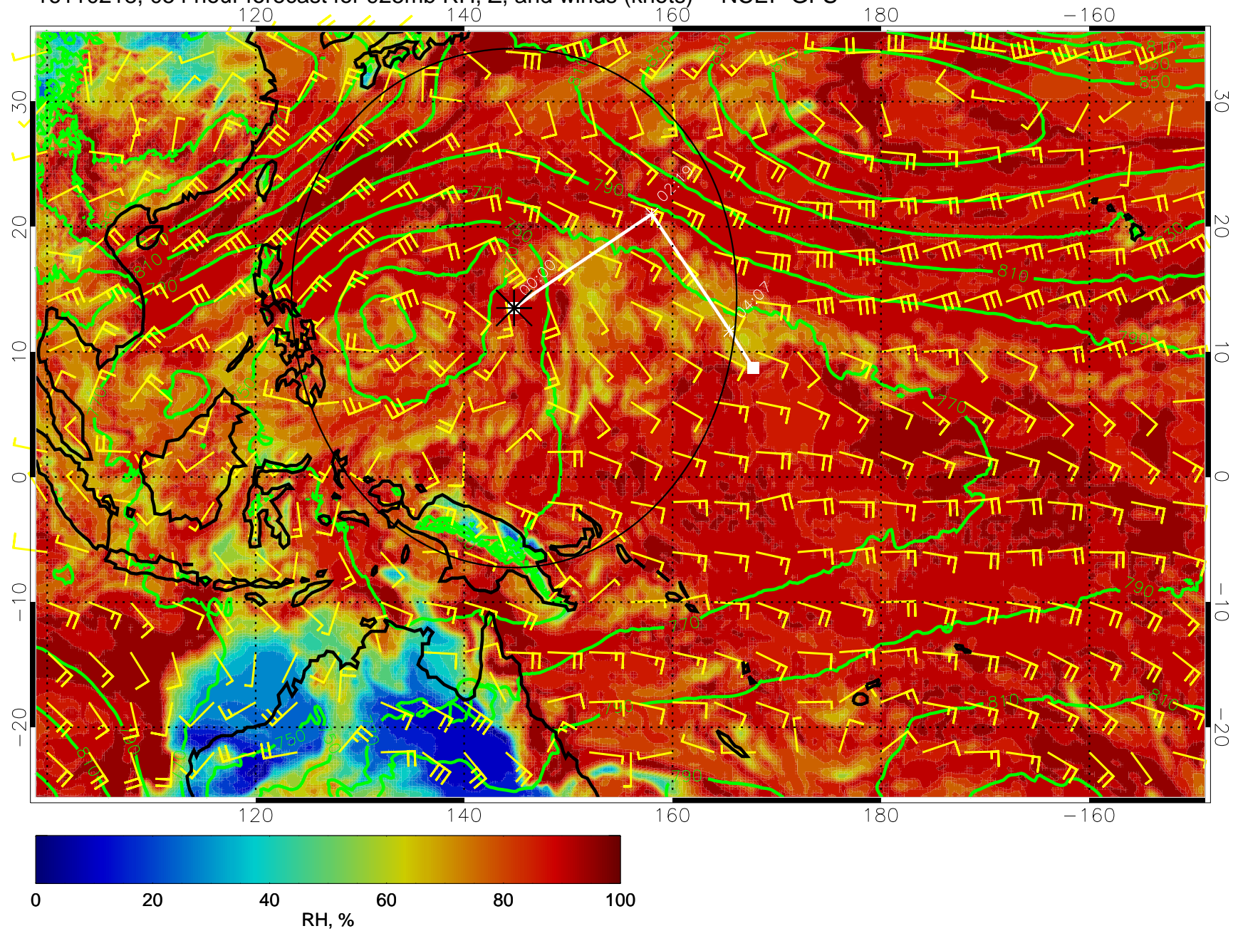
16110218, 054 hour forecast for 925mb RH, Z, and winds (knots) -- NCEP GFS
