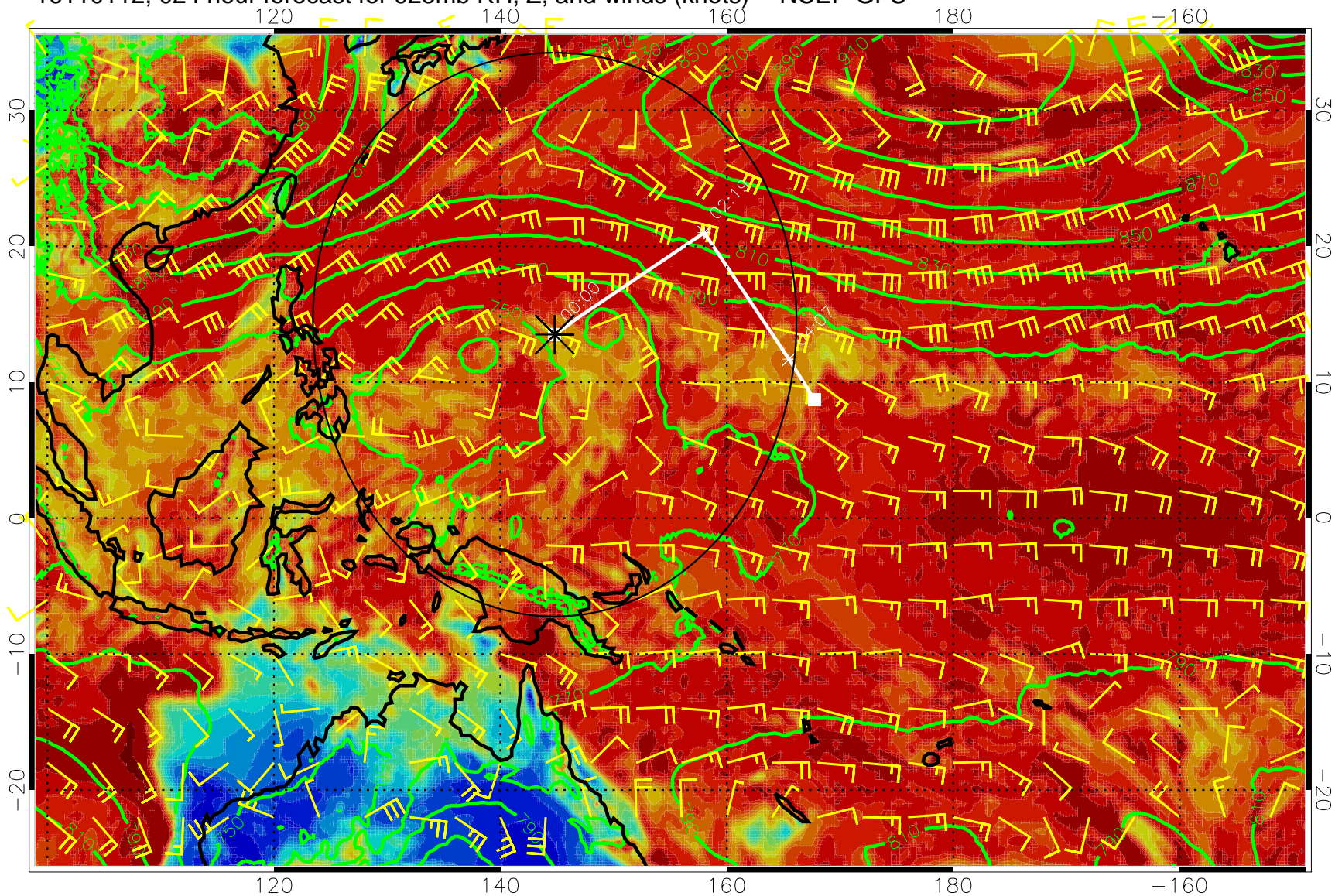
16110112, 024 hour forecast for 925mb RH, Z, and winds (knots) -- NCEP GFS
