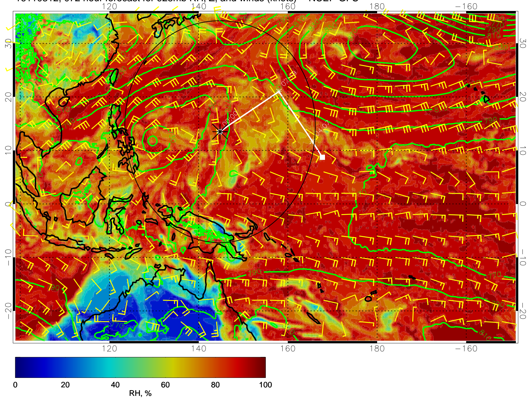
16110312, 072 hour forecast for 925mb RH, Z, and winds (knots) -- NCEP GFS
