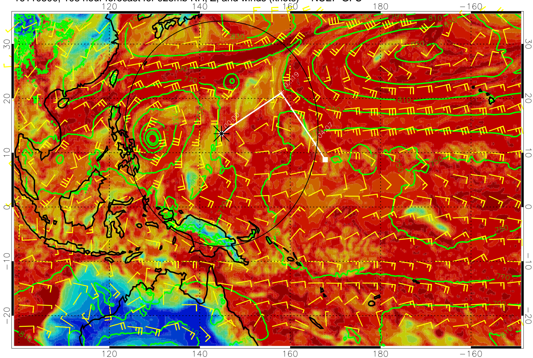
16110500, 108 hour forecast for 925mb RH, Z, and winds (knots) -- NCEP GFS
