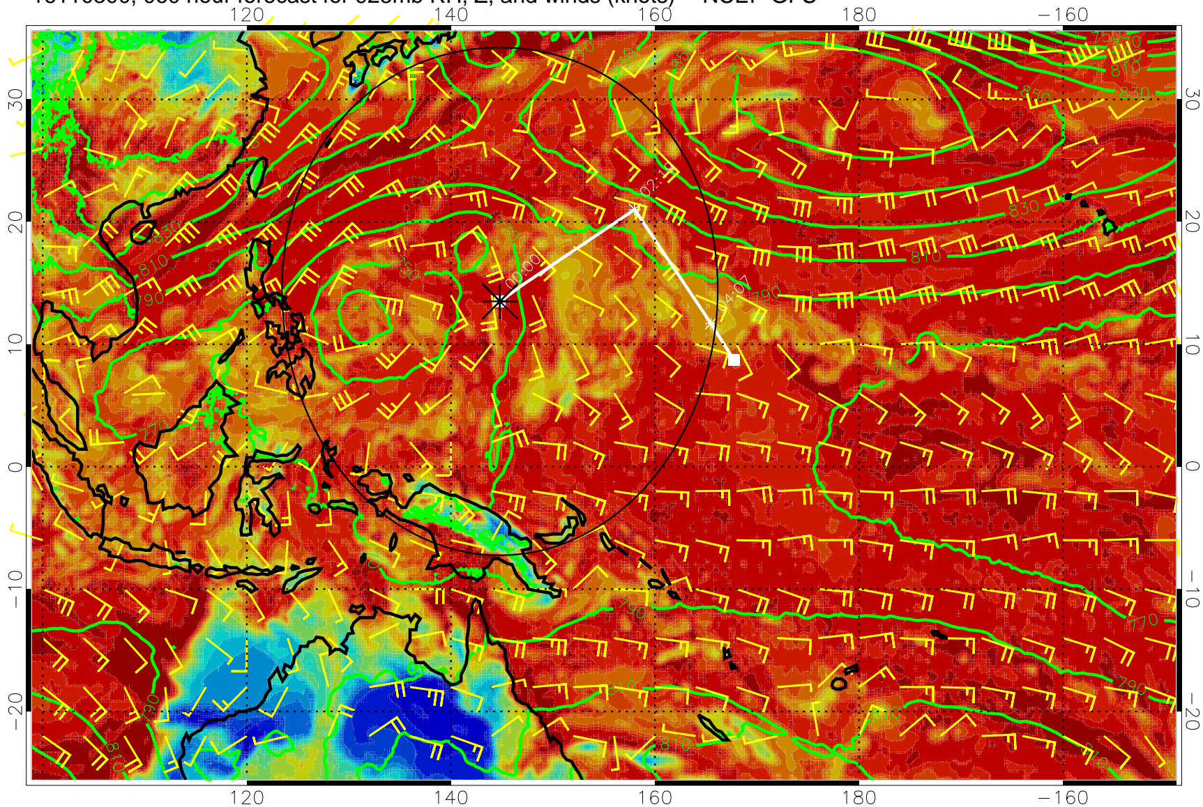
16110300, 060 hour forecast for 925mb RH, Z, and winds (knots) -- NCEP GFS
