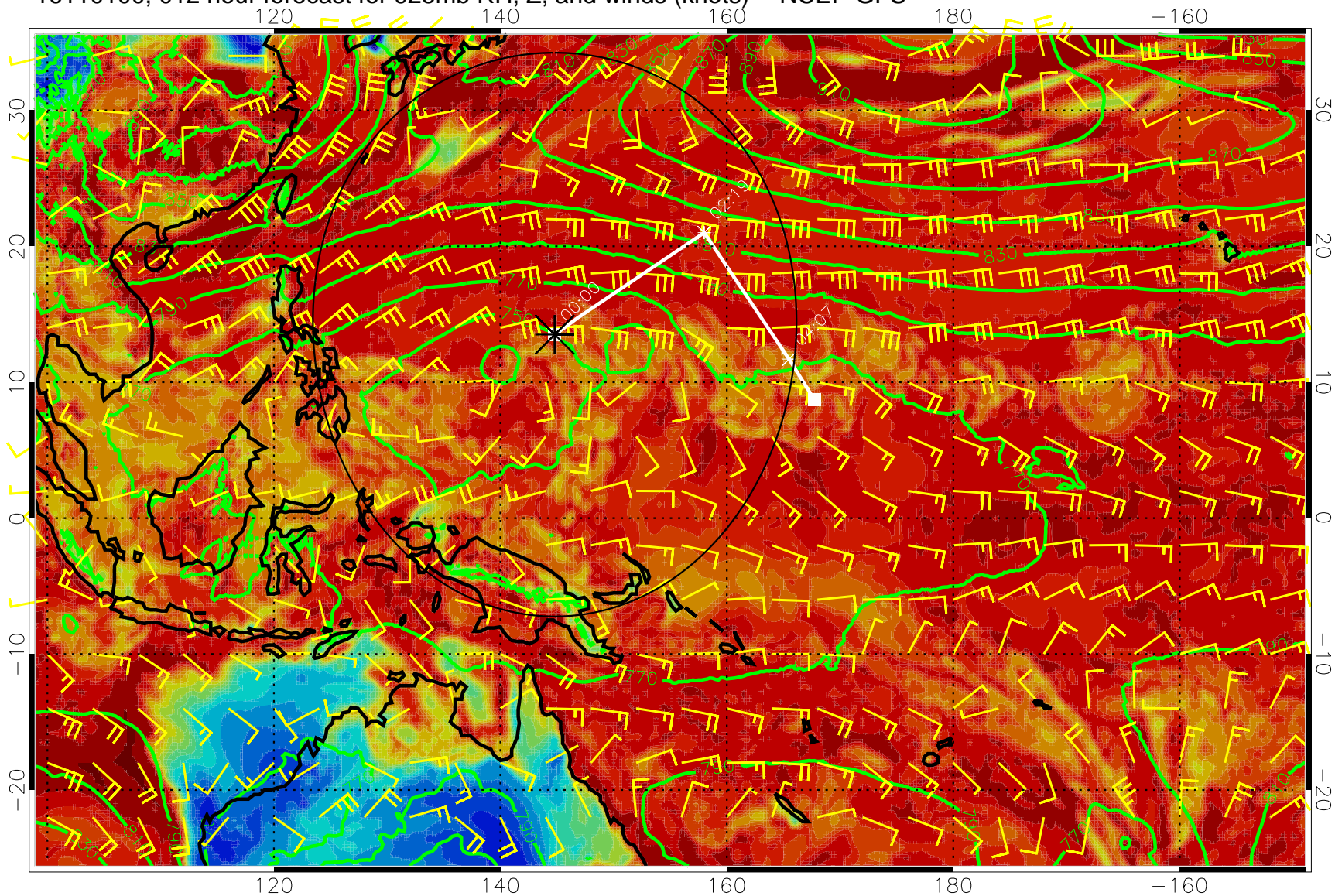
16110100, 012 hour forecast for 925mb RH, Z, and winds (knots) -- NCEP GFS
