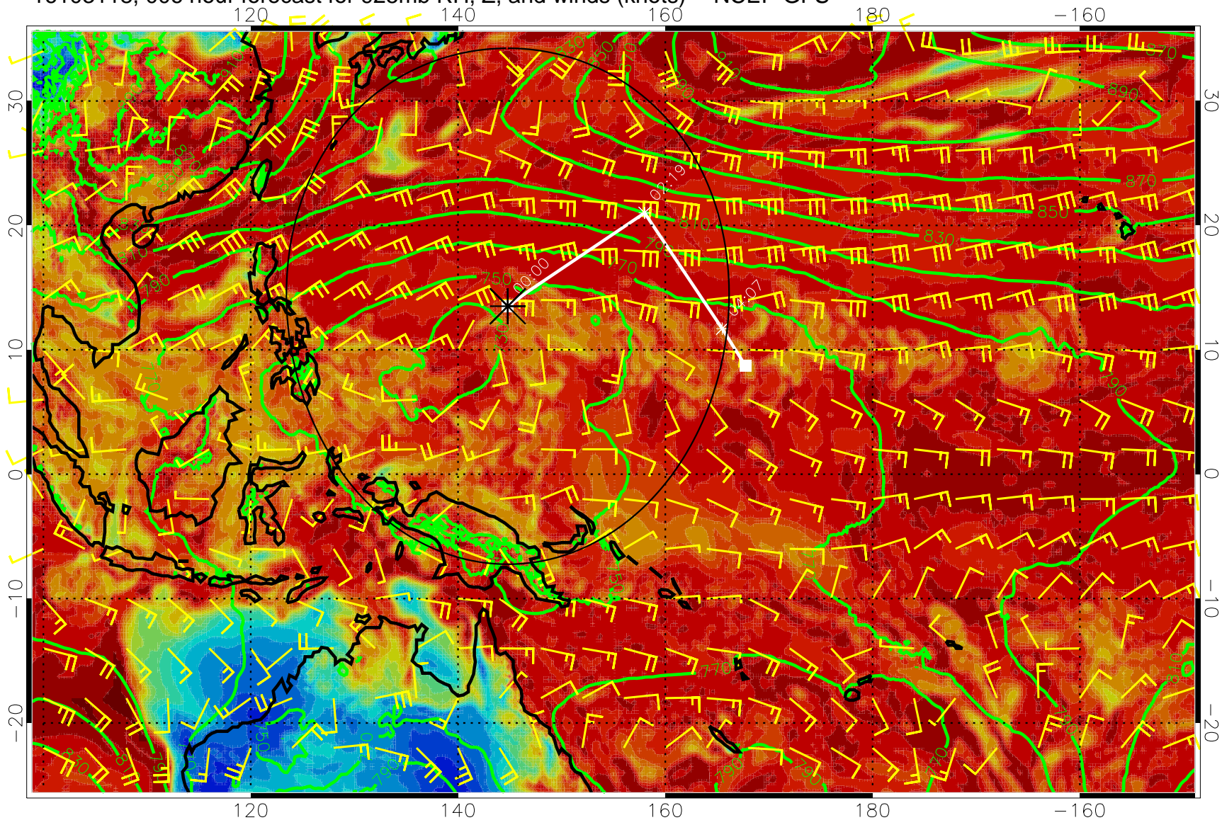
16103118, 006 hour forecast for 925mb RH, Z, and winds (knots) -- NCEP GFS
