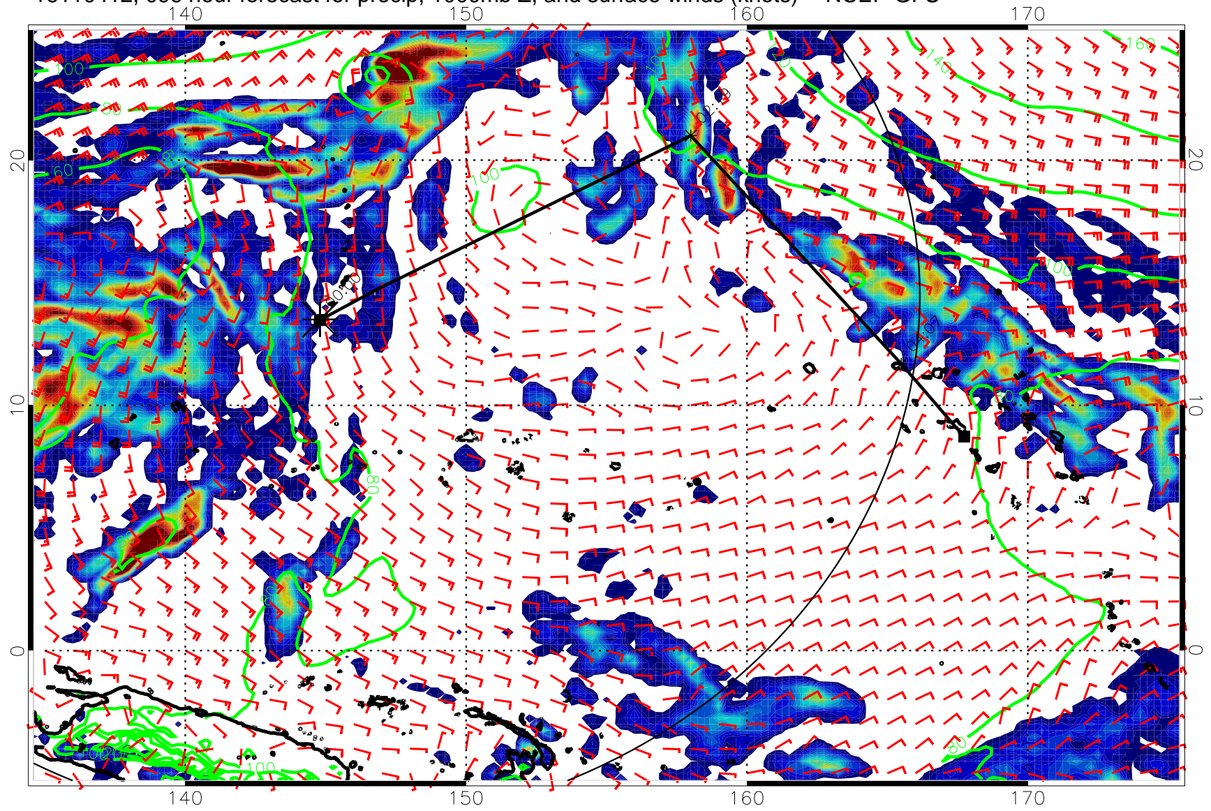
16110412, 096 hour forecast for precip, 1000mb Z, and surface winds (knots) -- NCEP GFS
