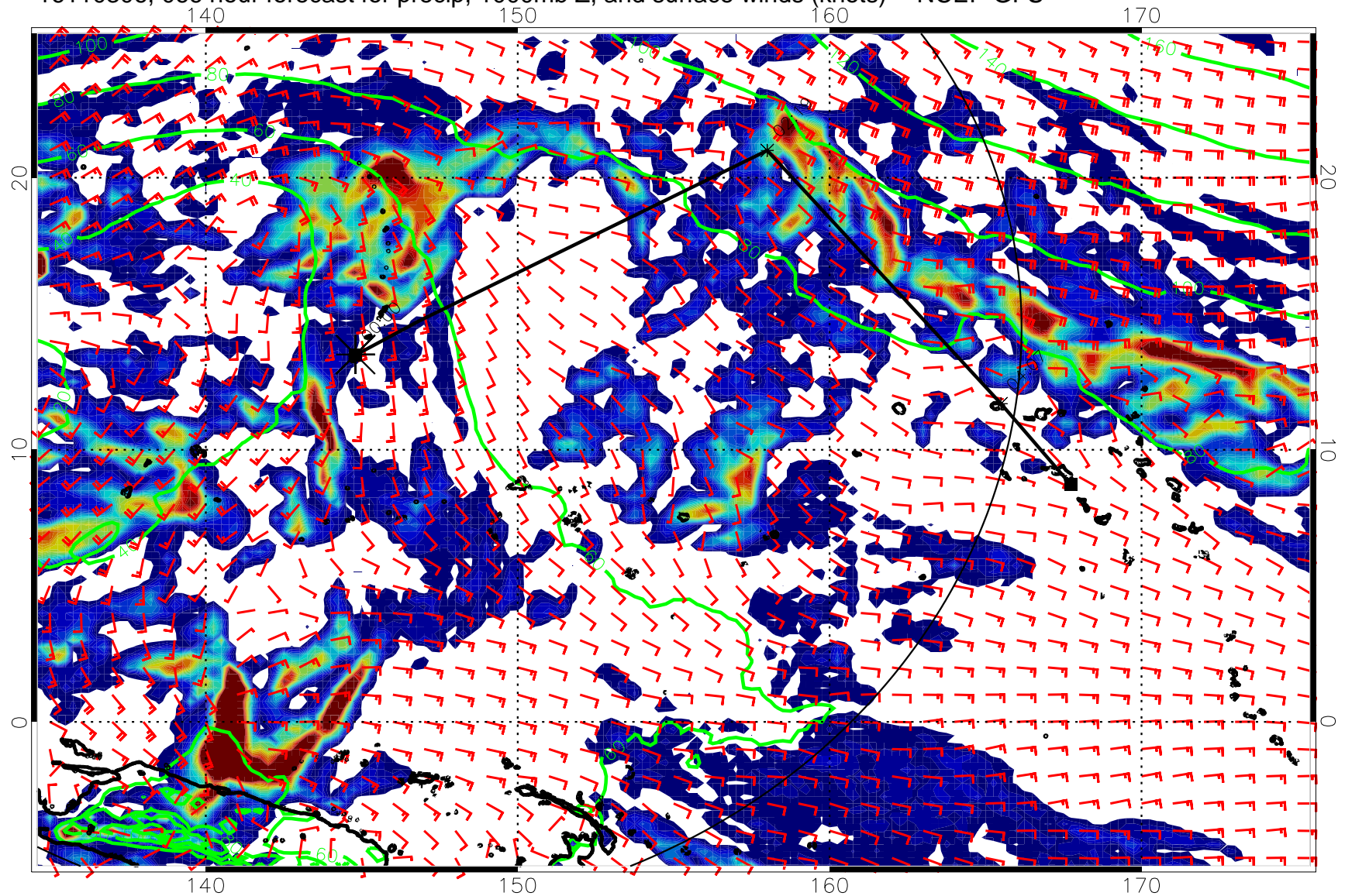
16110306, 066 hour forecast for precip, 1000mb Z, and surface winds (knots) -- NCEP GFS
