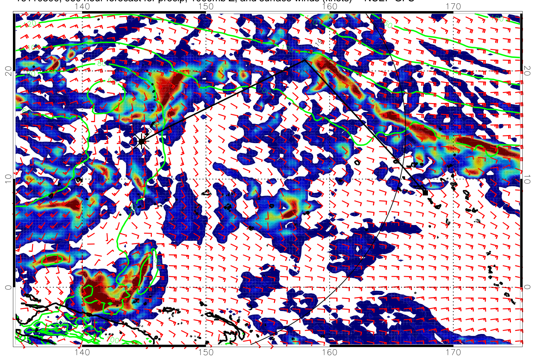
16110300, 060 hour forecast for precip, 1000mb Z, and surface winds (knots) -- NCEP GFS
