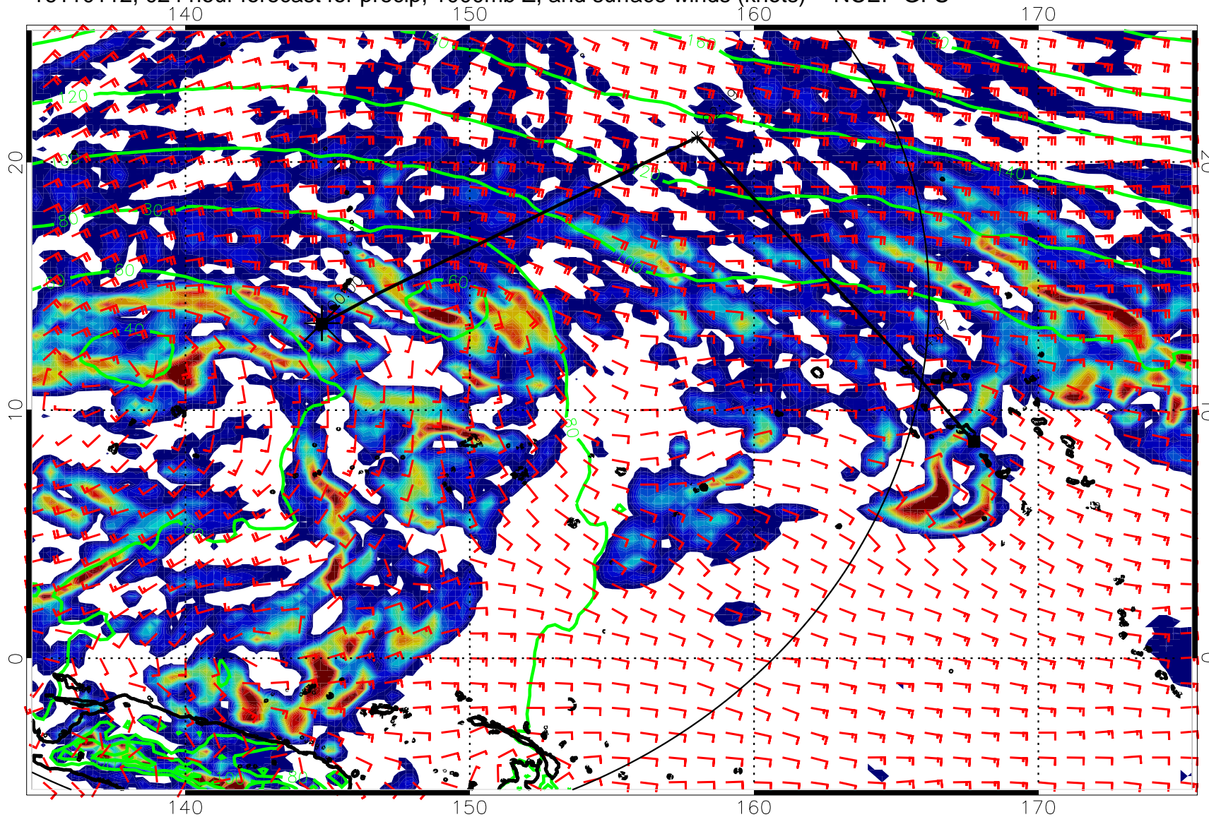
16110112, 024 hour forecast for precip, 1000mb Z, and surface winds (knots) -- NCEP GFS
