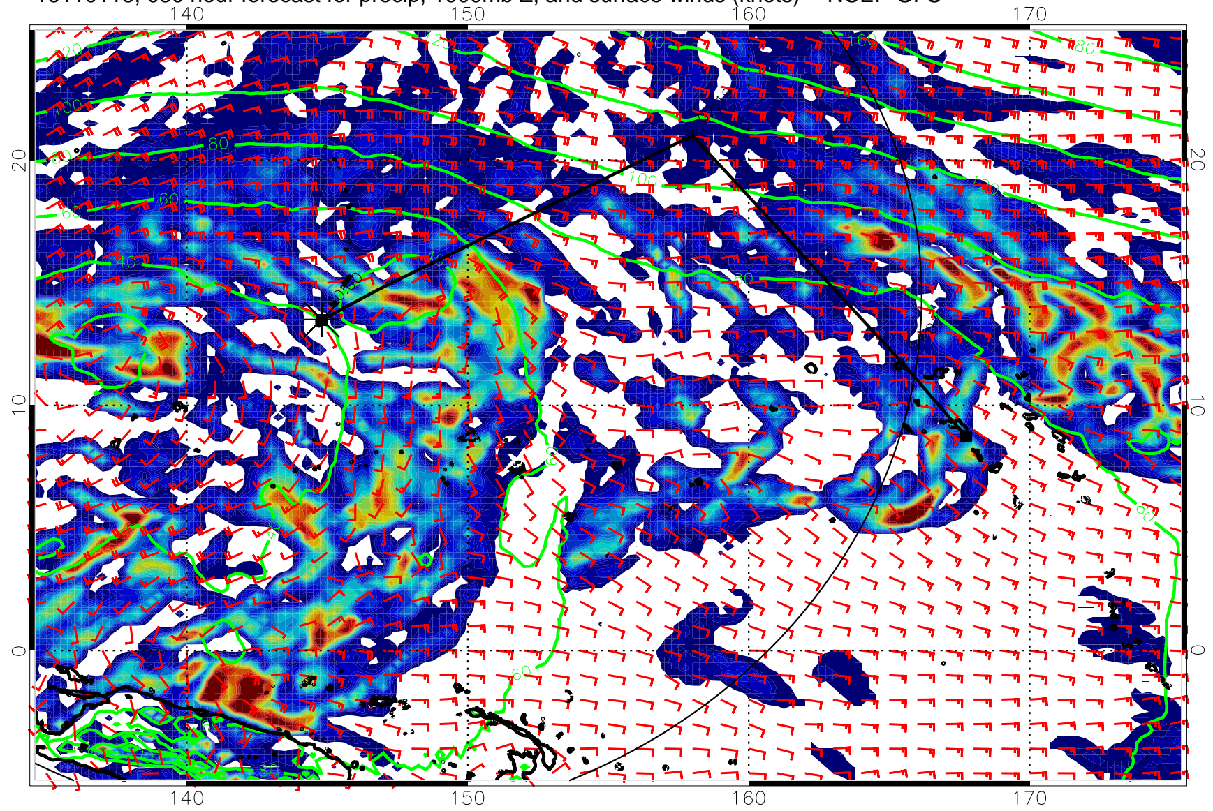
16110118, 030 hour forecast for precip, 1000mb Z, and surface winds (knots) -- NCEP GFS
