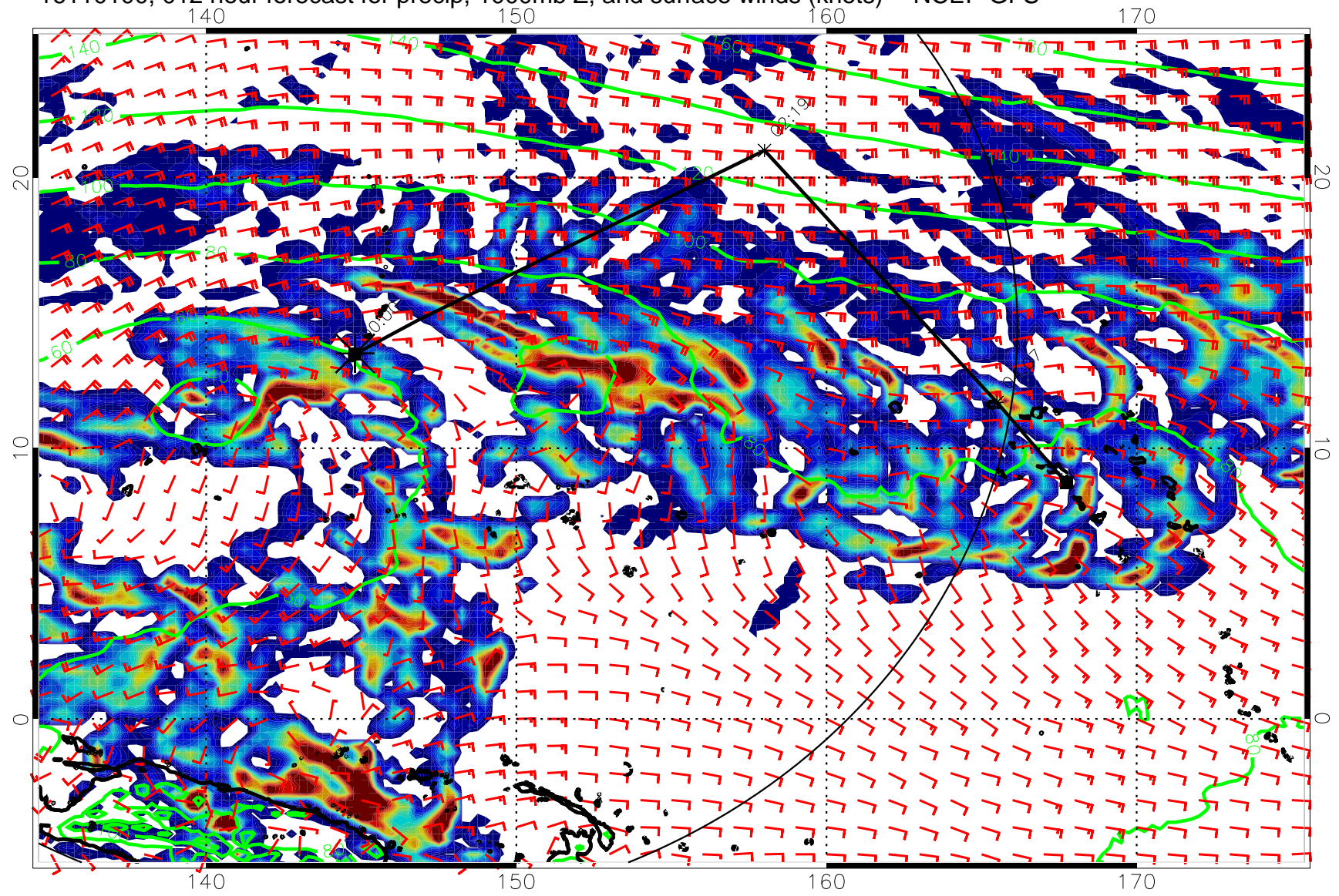
16110100, 012 hour forecast for precip, 1000mb Z, and surface winds (knots) -- NCEP GFS
