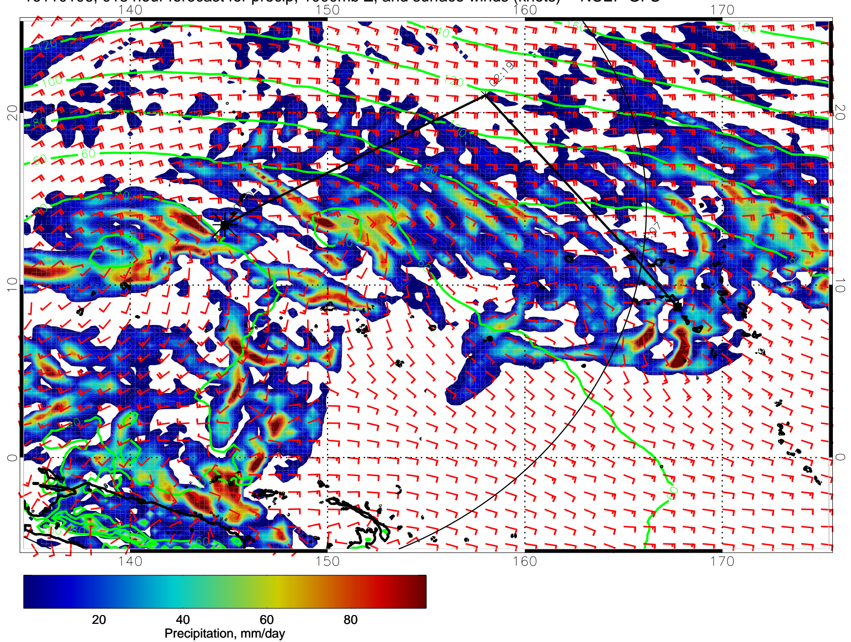
16110106, 018 hour forecast for precip, 1000mb Z, and surface winds (knots) -- NCEP GFS
