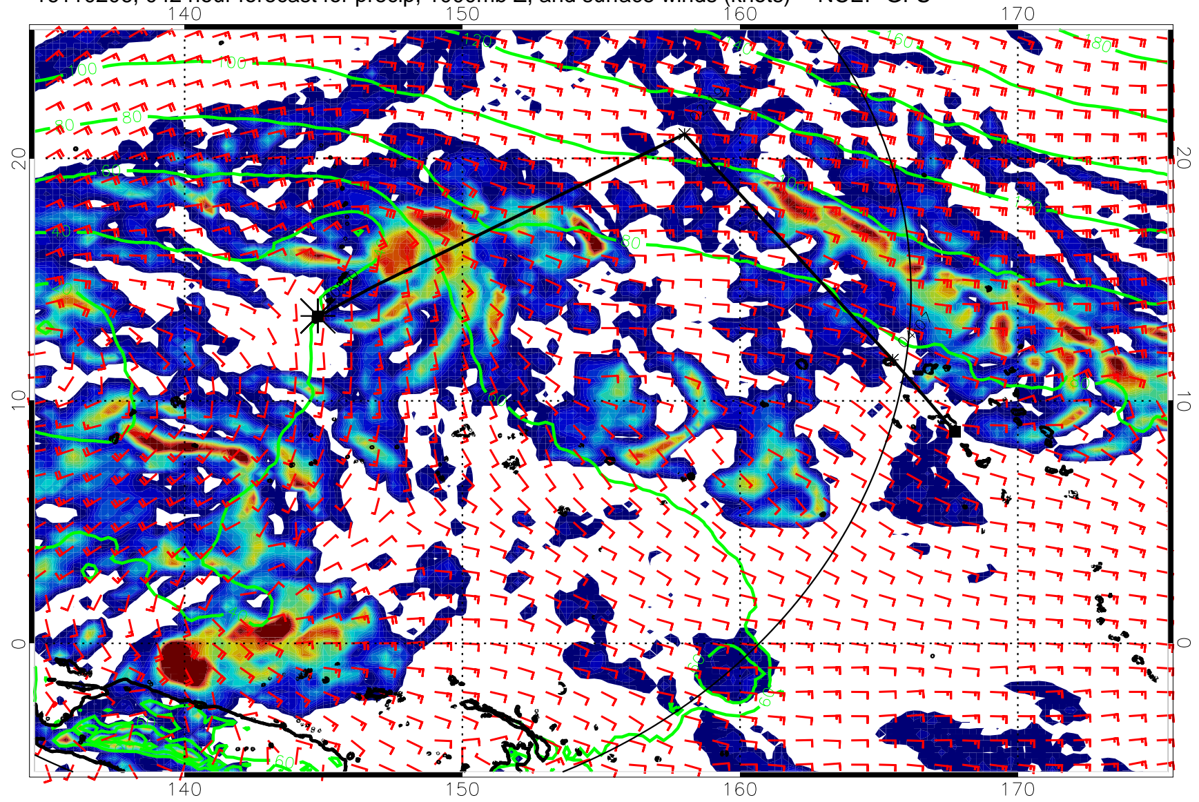
16110206, 042 hour forecast for precip, 1000mb Z, and surface winds (knots) -- NCEP GFS
