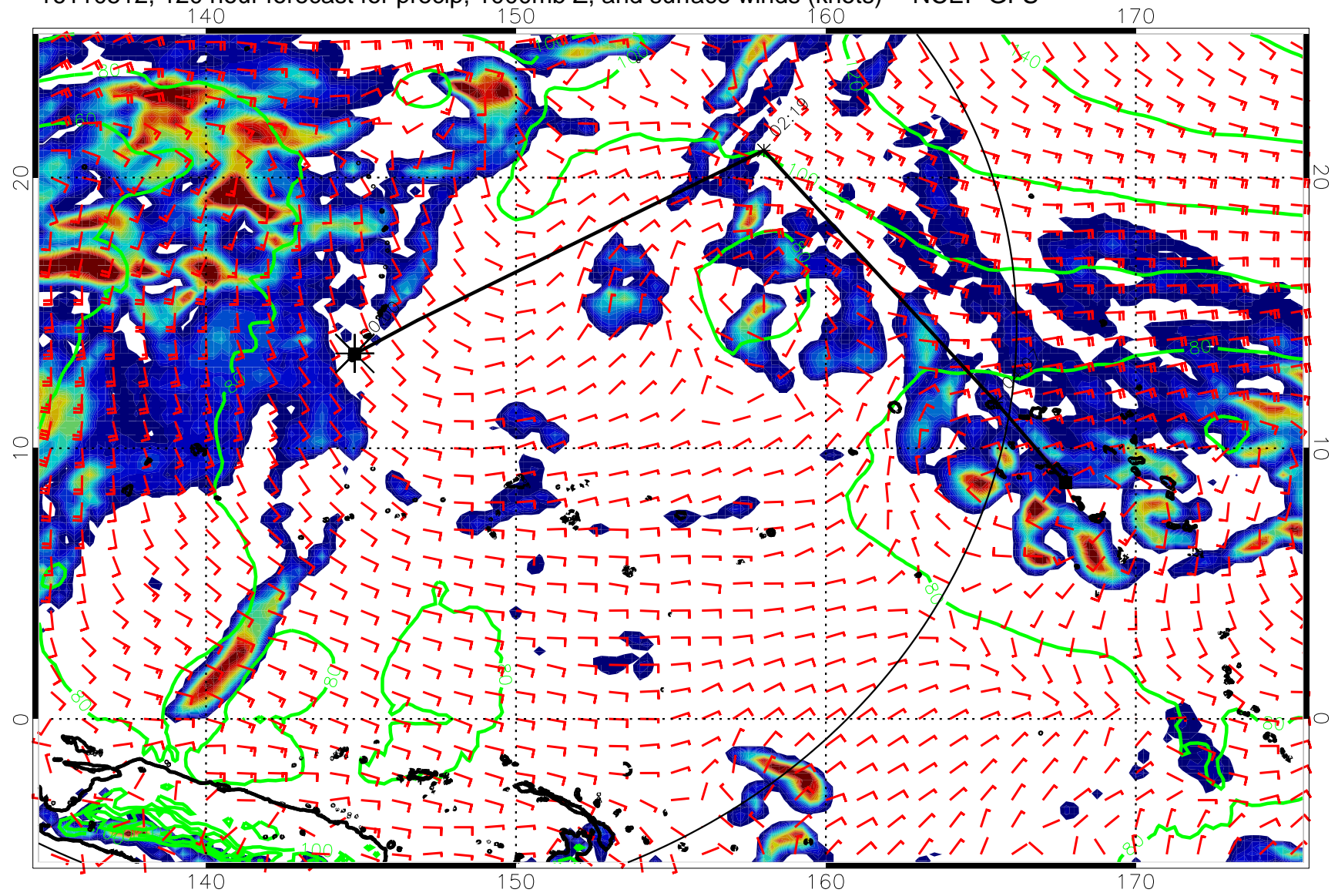
16110512, 120 hour forecast for precip, 1000mb Z, and surface winds (knots) -- NCEP GFS
