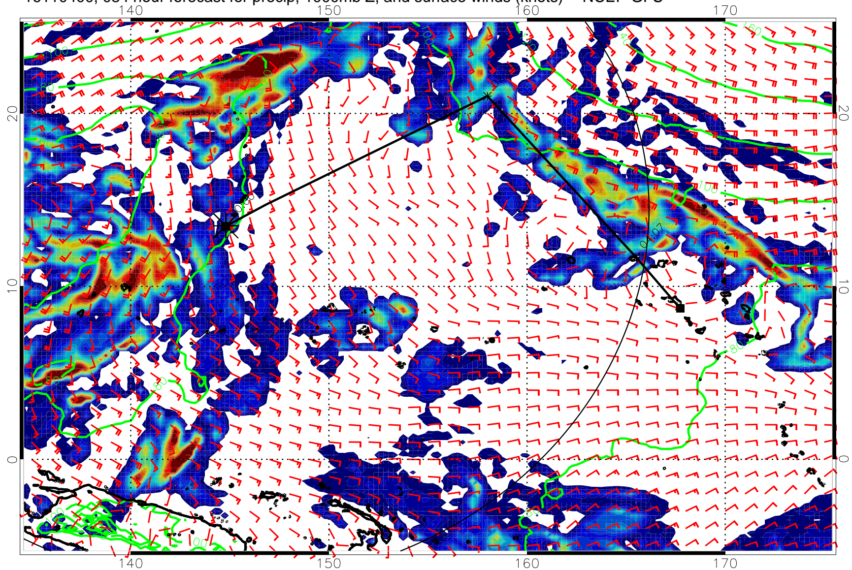
16110400, 084 hour forecast for precip, 1000mb Z, and surface winds (knots) -- NCEP GFS
