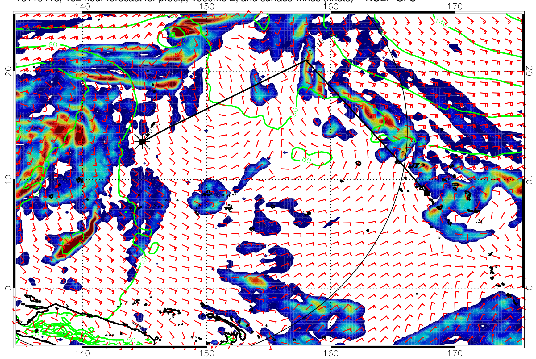
16110418, 102 hour forecast for precip, 1000mb Z, and surface winds (knots) -- NCEP GFS
