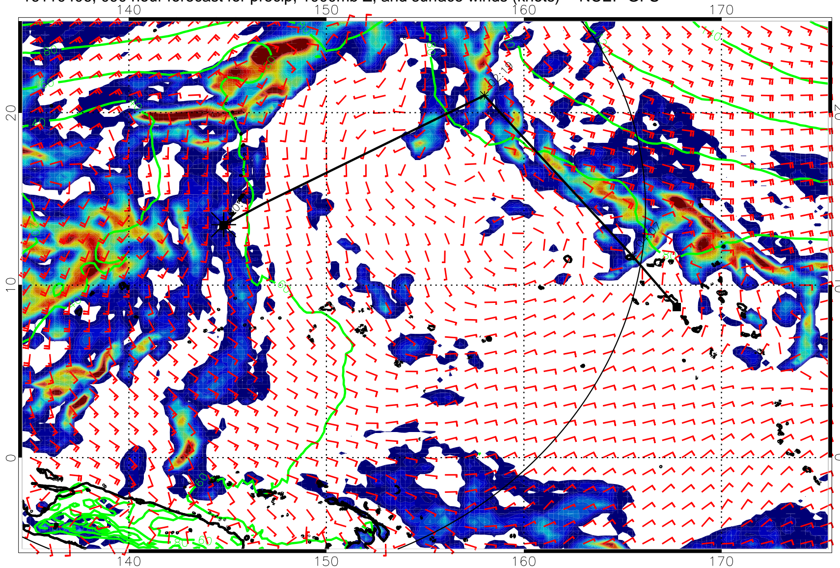
16110406, 090 hour forecast for precip, 1000mb Z, and surface winds (knots) -- NCEP GFS
