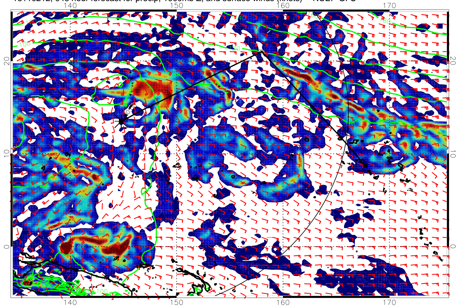
16110212, 048 hour forecast for precip, 1000mb Z, and surface winds (knots) -- NCEP GFS
