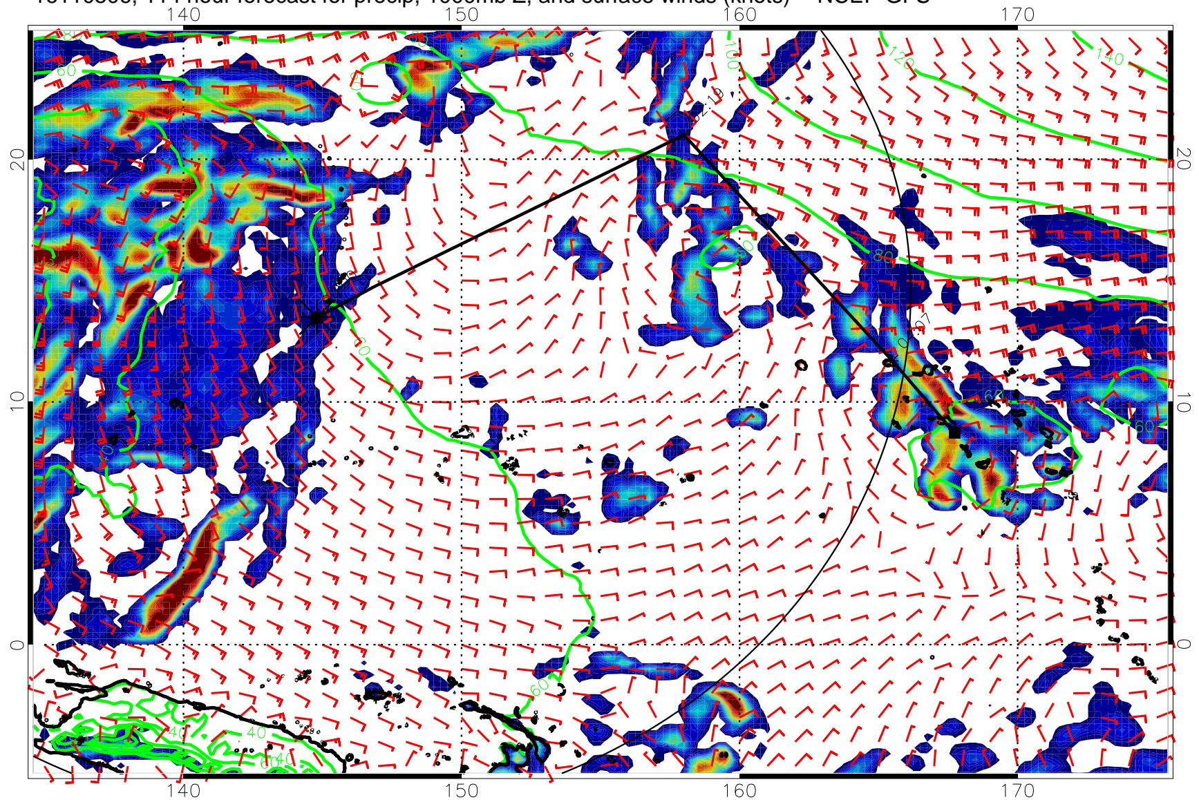
16110506, 114 hour forecast for precip, 1000mb Z, and surface winds (knots) -- NCEP GFS
