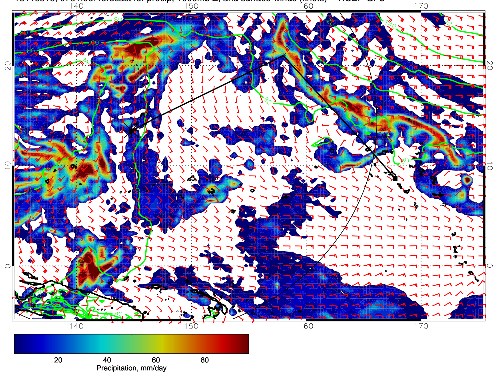
16110318, 078 hour forecast for precip, 1000mb Z, and surface winds (knots) -- NCEP GFS
