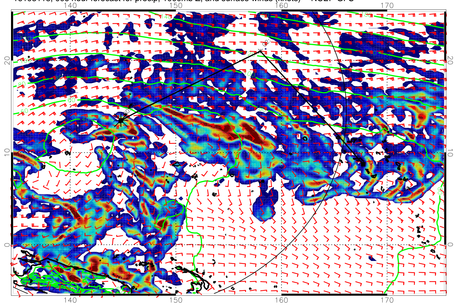
16103118, 006 hour forecast for precip, 1000mb Z, and surface winds (knots) -- NCEP GFS
