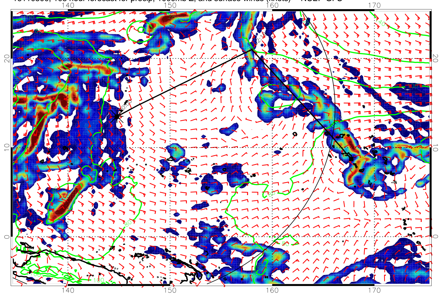
16110500, 108 hour forecast for precip, 1000mb Z, and surface winds (knots) -- NCEP GFS
