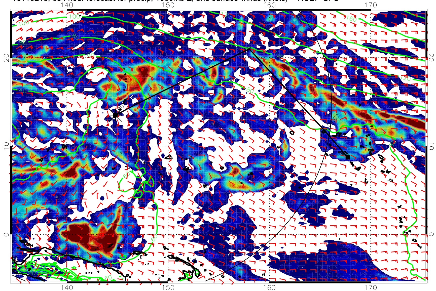
16110218, 054 hour forecast for precip, 1000mb Z, and surface winds (knots) -- NCEP GFS
