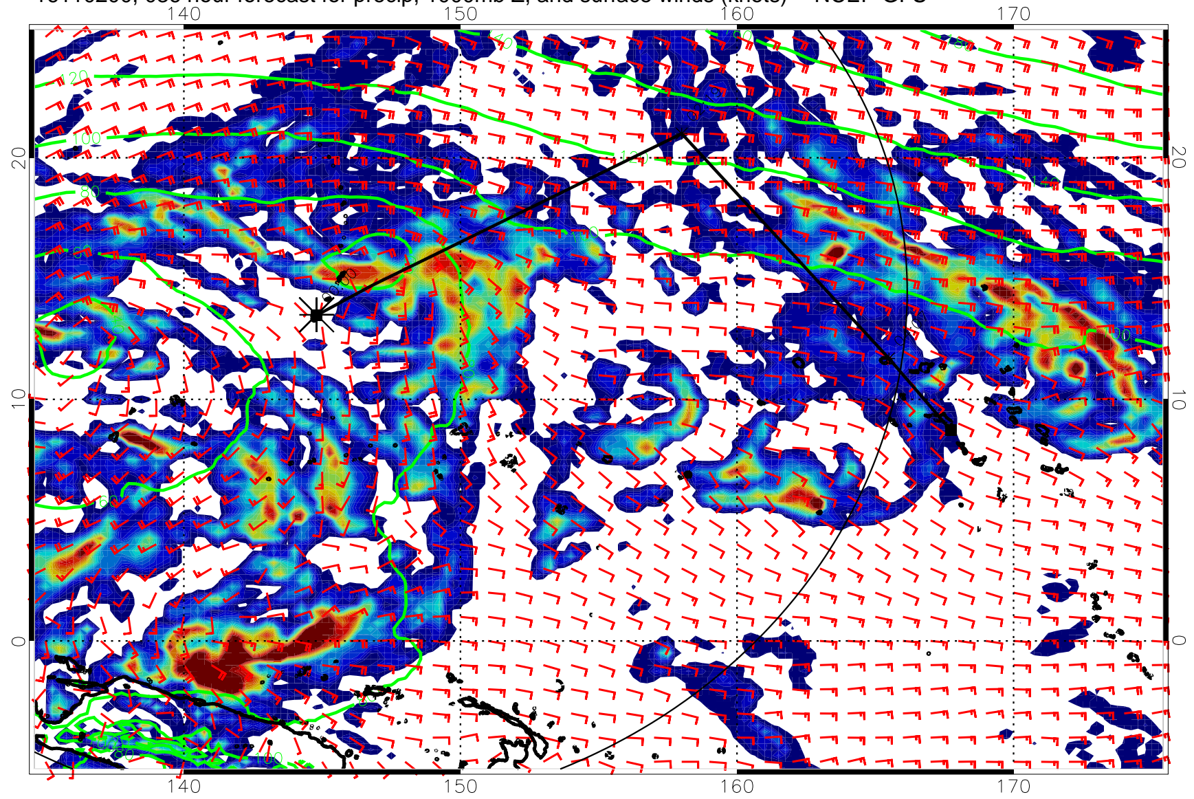
16110200, 036 hour forecast for precip, 1000mb Z, and surface winds (knots) -- NCEP GFS
