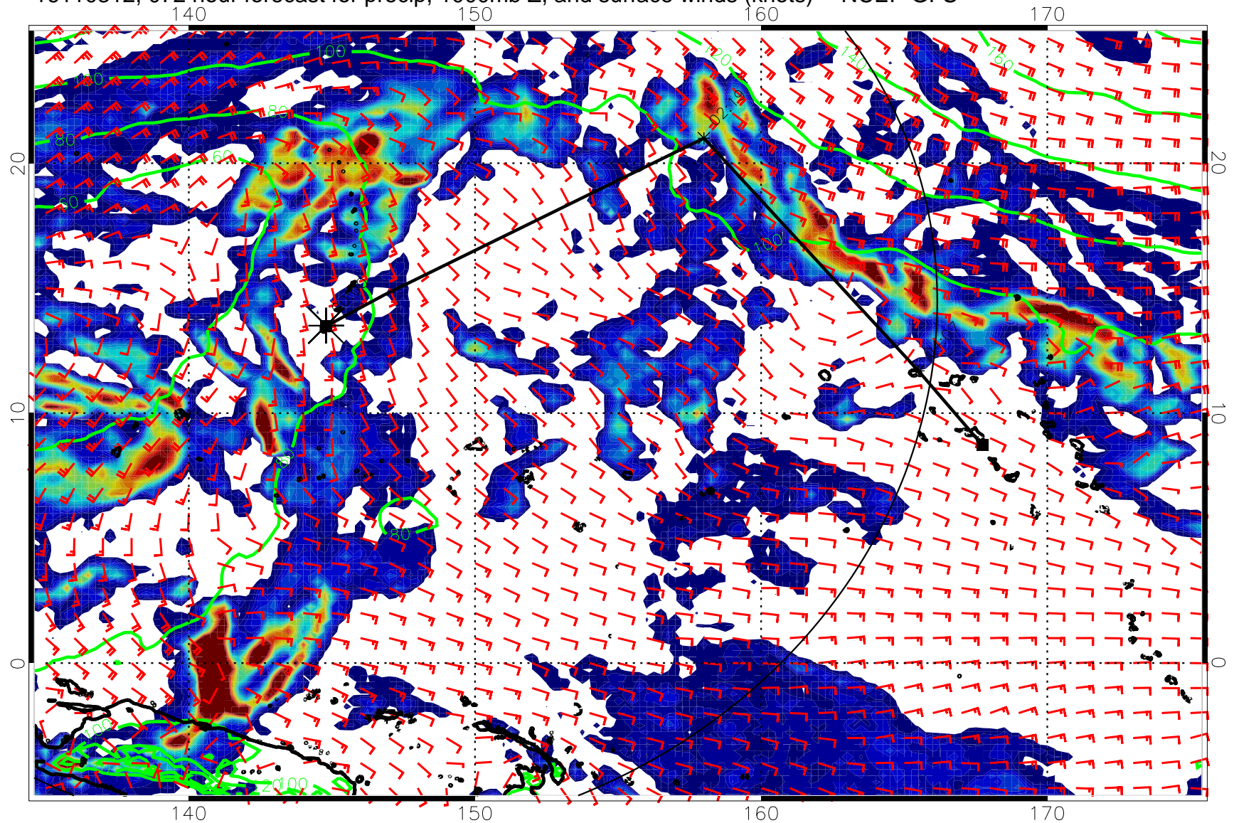
16110312, 072 hour forecast for precip, 1000mb Z, and surface winds (knots) -- NCEP GFS
