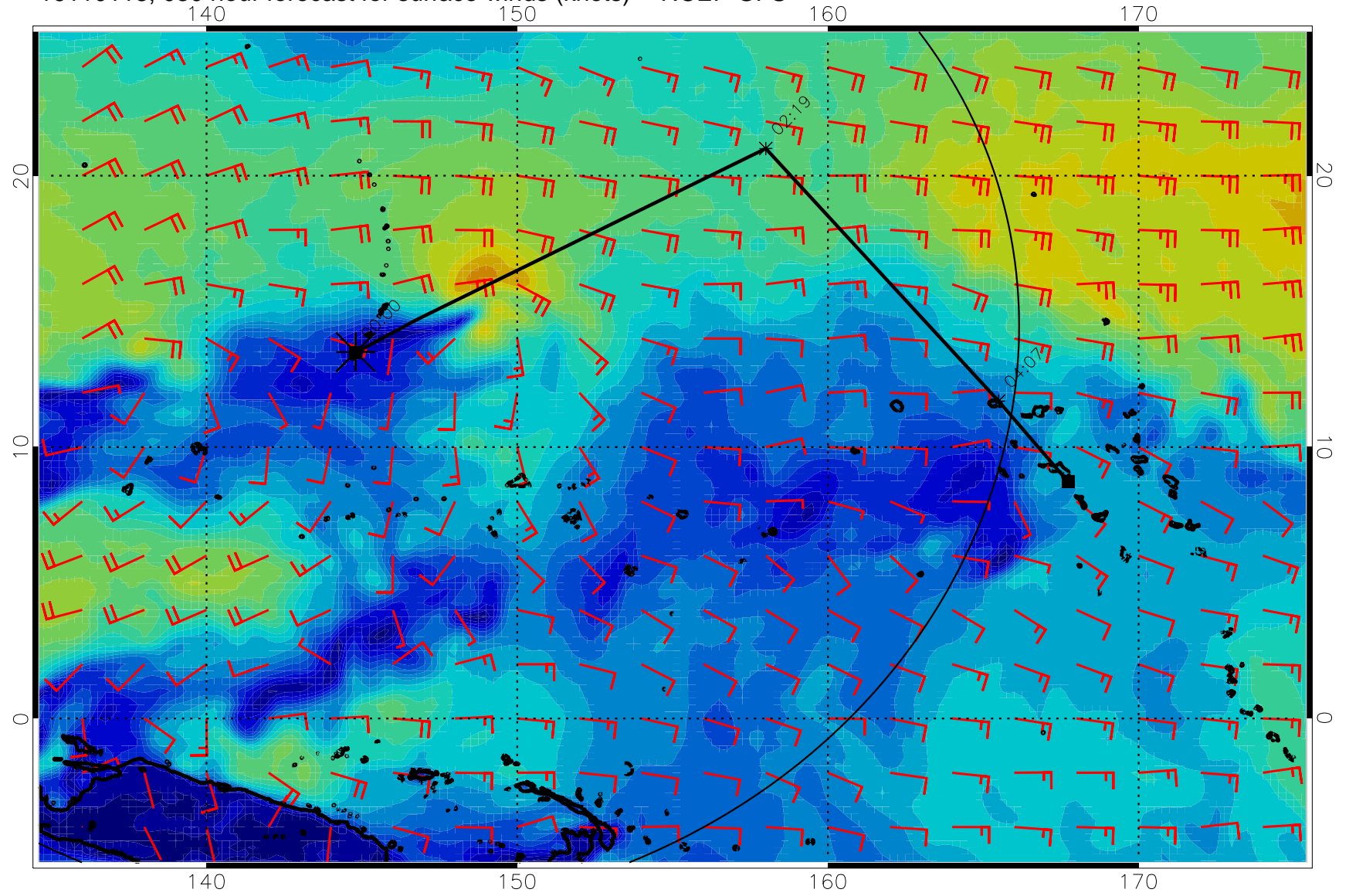
16110118, 0300 hour forecast for surface winds (knots) -- NCEP GFS
