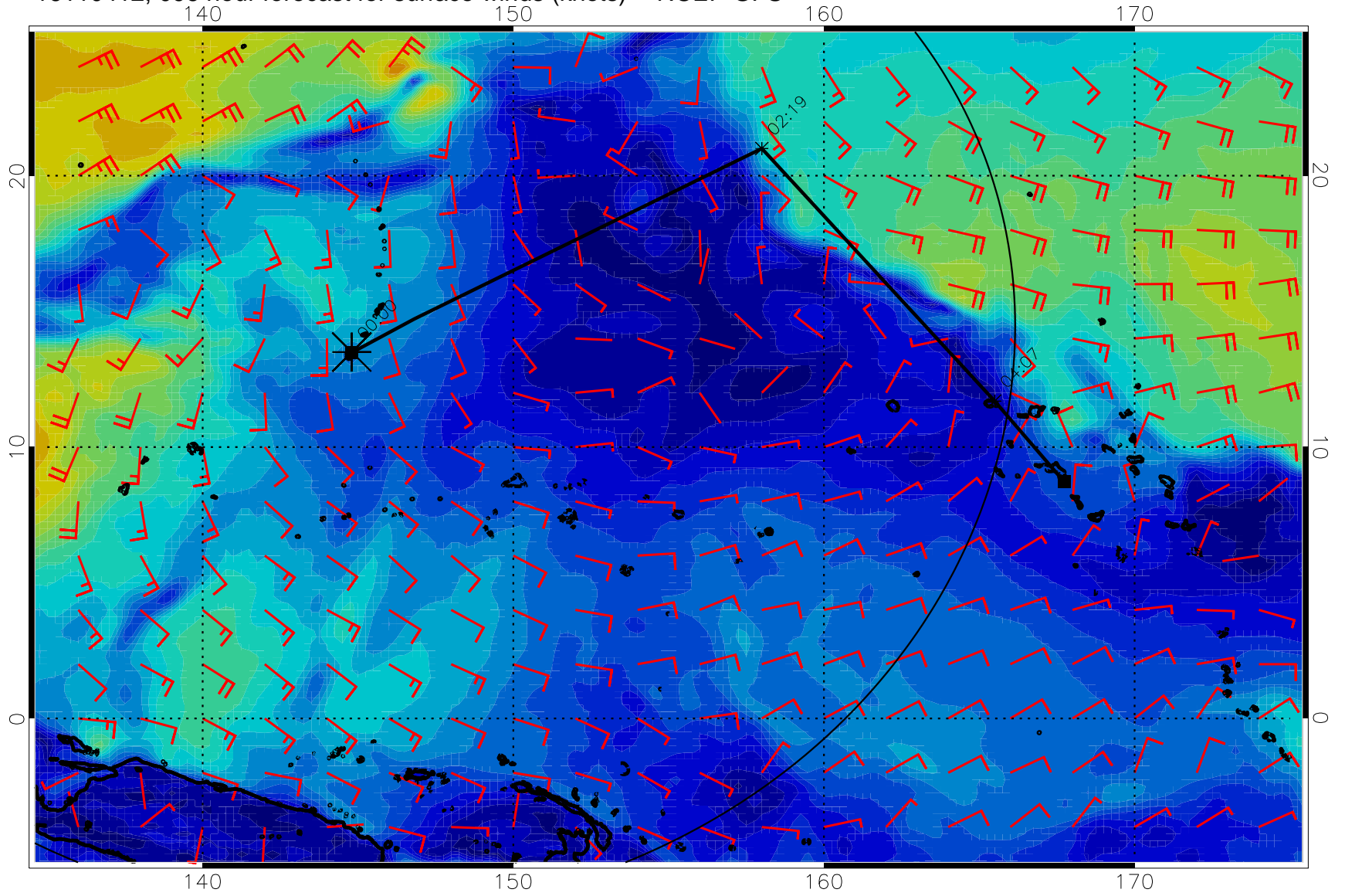
16110412, 096 hour forecast for surface winds (knots) -- NCEP GFS
