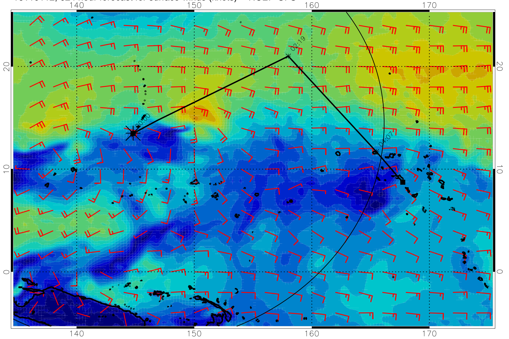
16110112, 024 hour forecast for surface winds (knots) -- NCEP GFS
