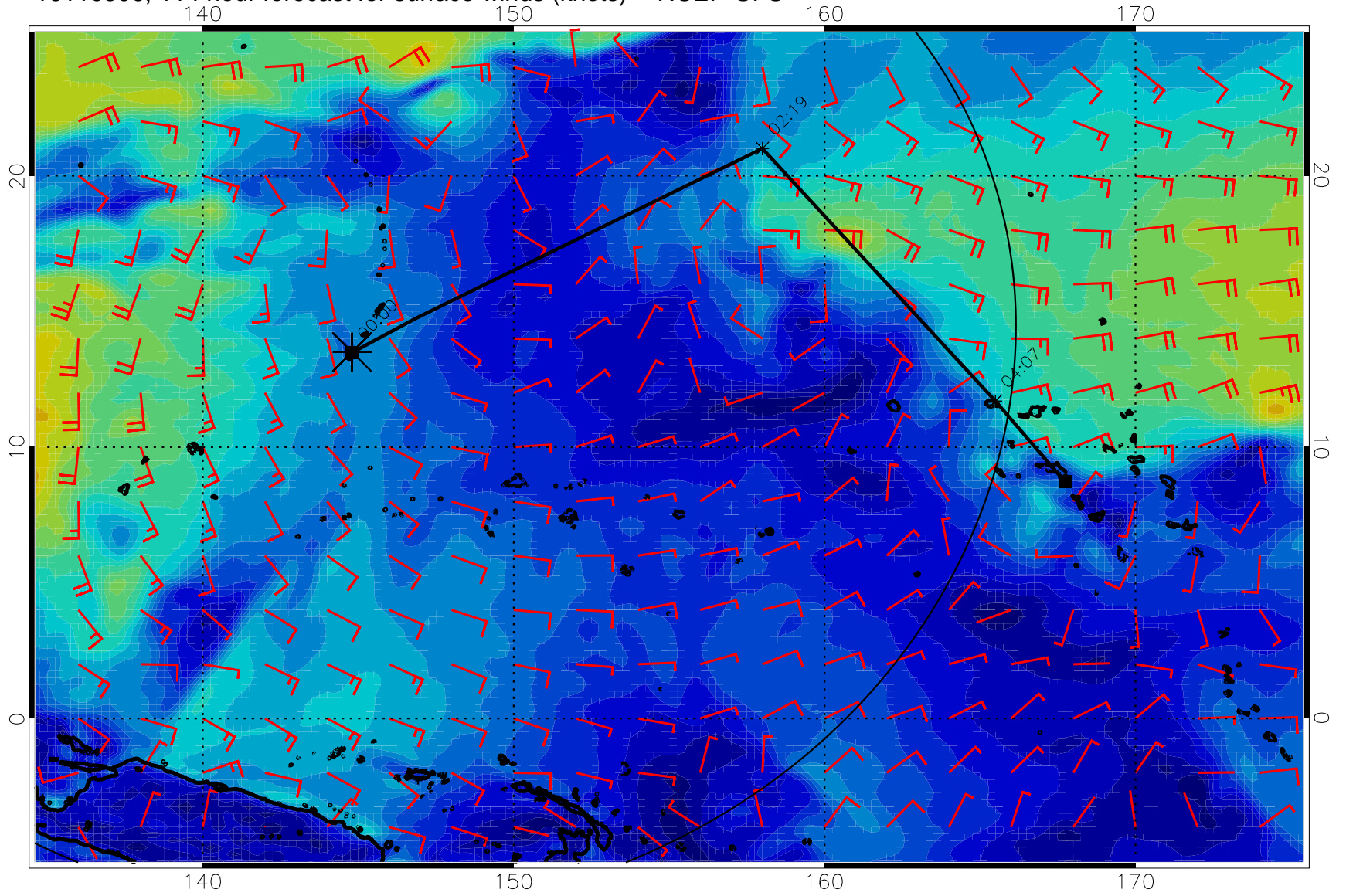
16110506, 114 hour forecast for surface winds (knots) -- NCEP GFS
