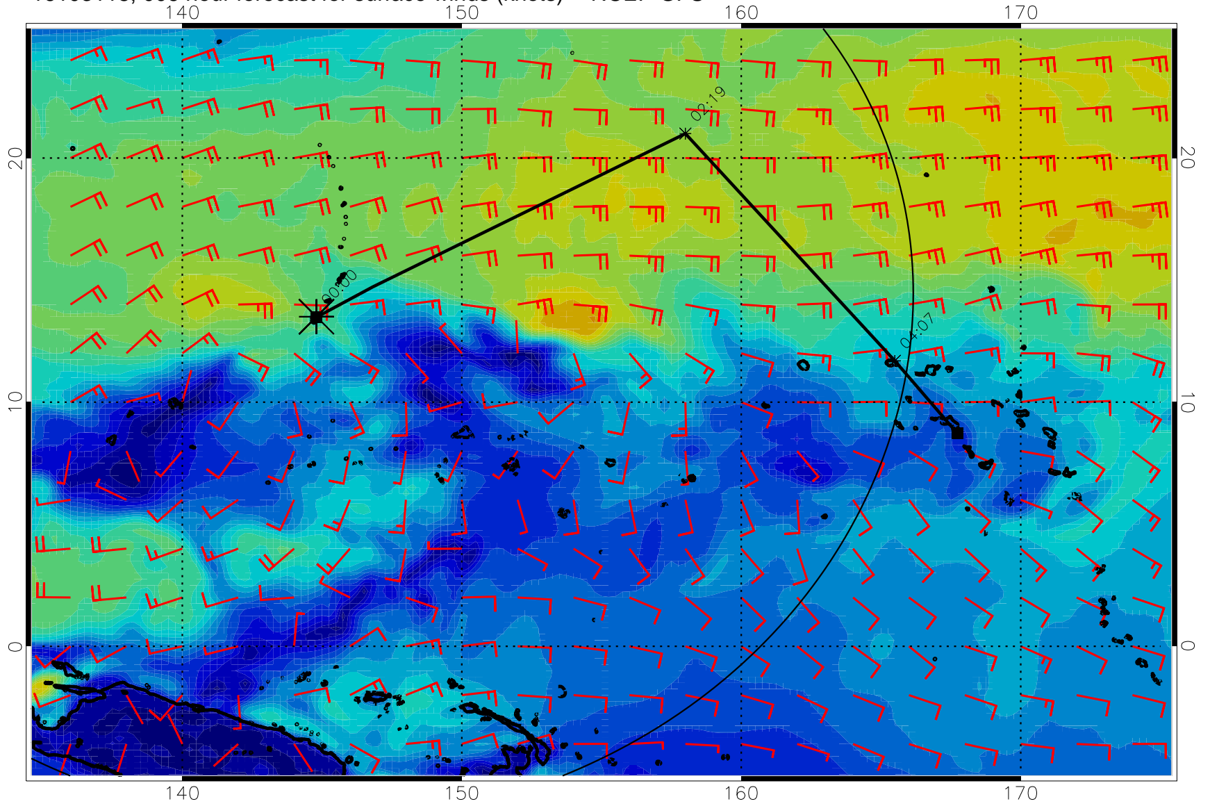
16103118, 006 hour forecast for surface winds (knots) -- NCEP GFS
