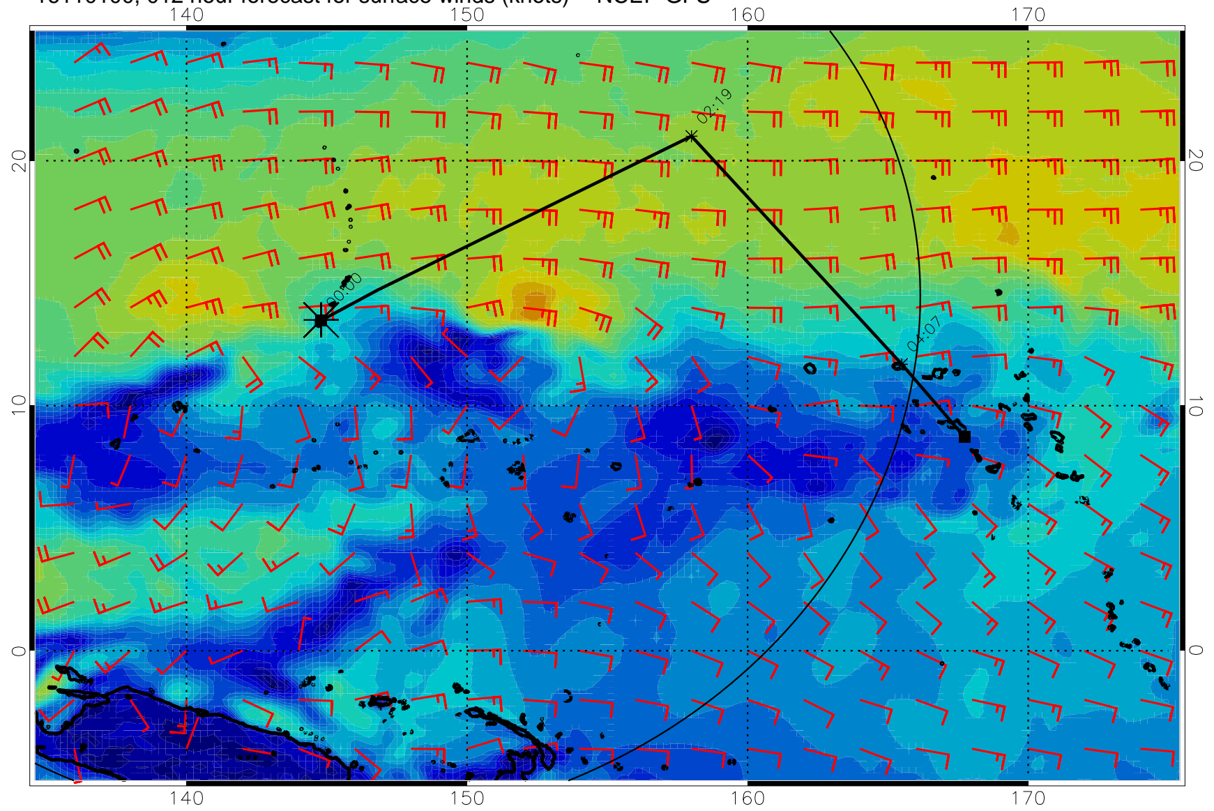
16110100, 012 hour forecast for surface winds (knots) -- NCEP GFS
