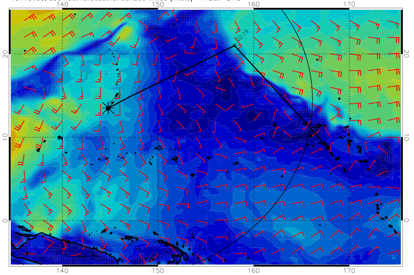
16110406, 090 hour forecast for surface winds (knots) -- NCEP GFS
