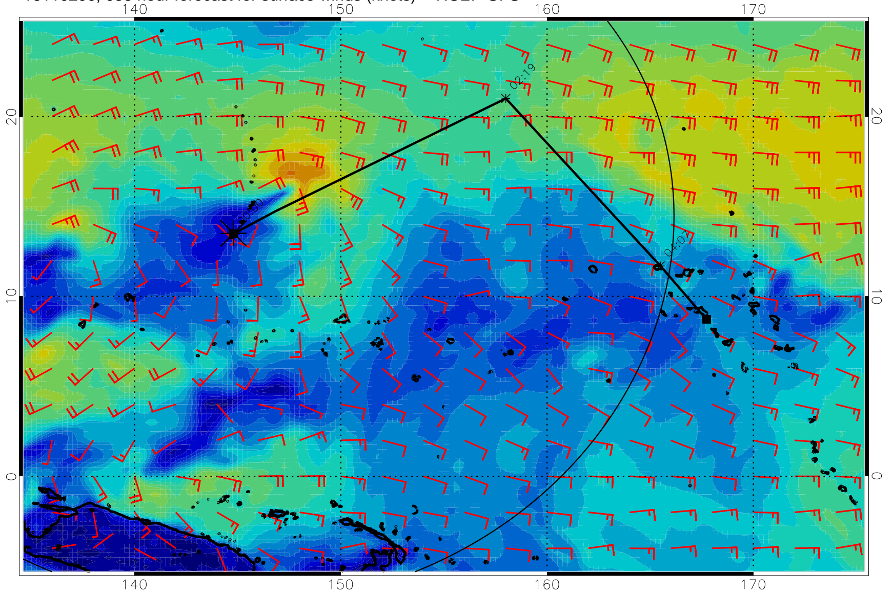
16110200, 036 hour forecast for surface winds (knots) -- NCEP GFS
