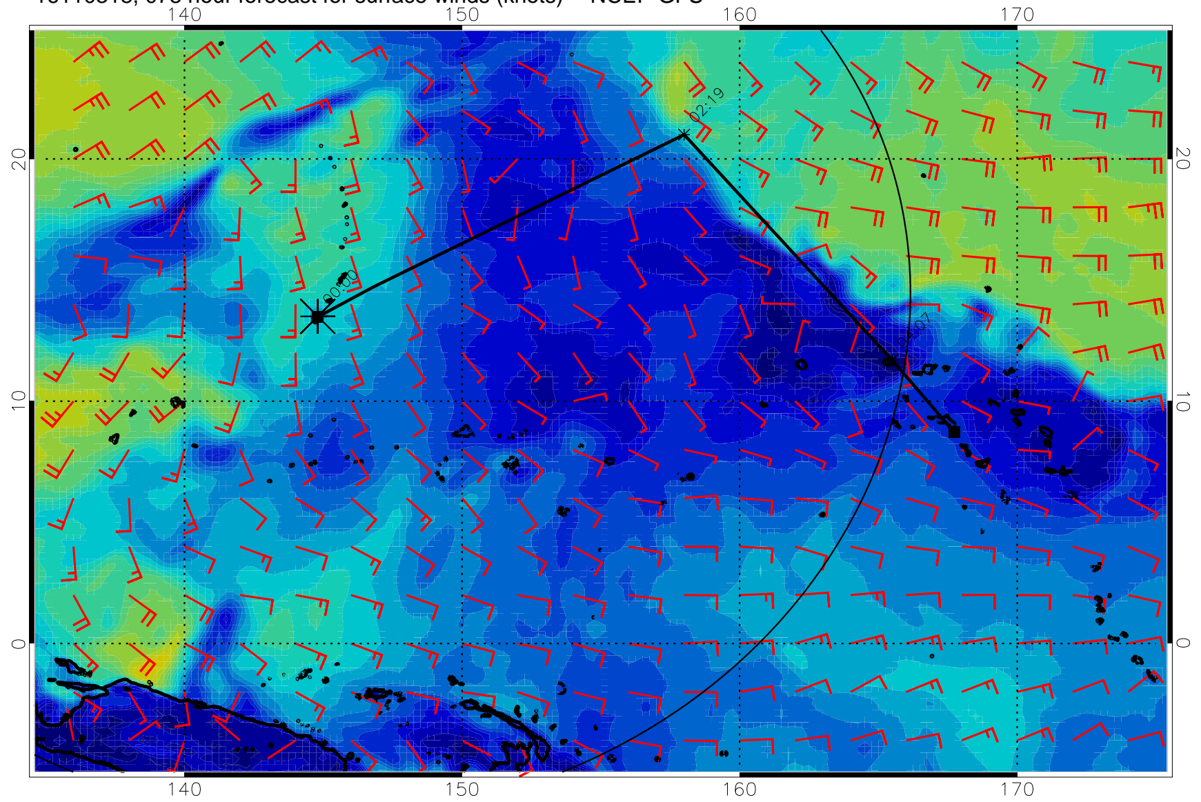
16110318, 078 hour forecast for surface winds (knots) -- NCEP GFS
