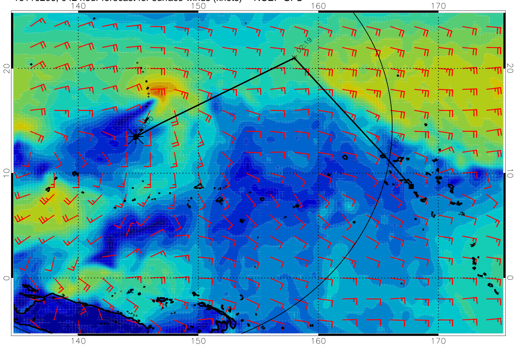
16110206, 042 hour forecast for surface winds (knots) -- NCEP GFS
