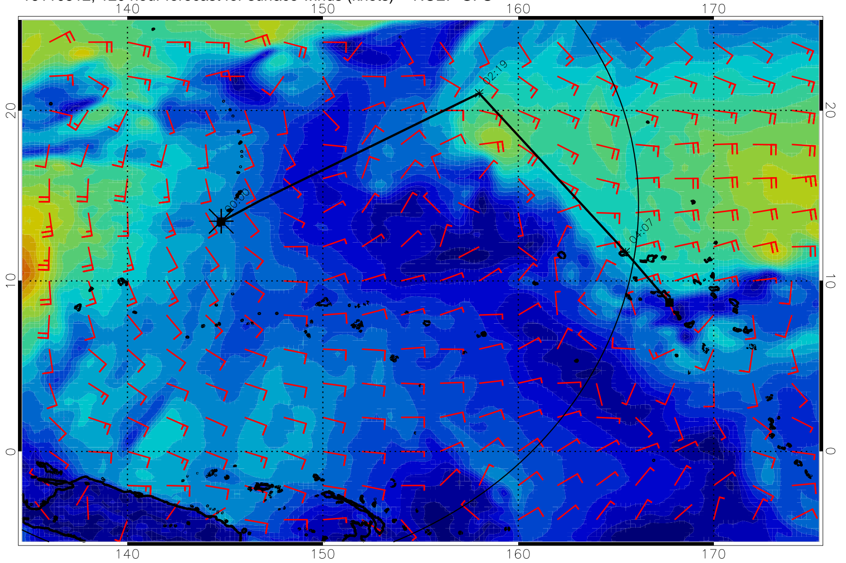
16110512, 120 hour forecast for surface winds (knots) -- NCEP GFS
