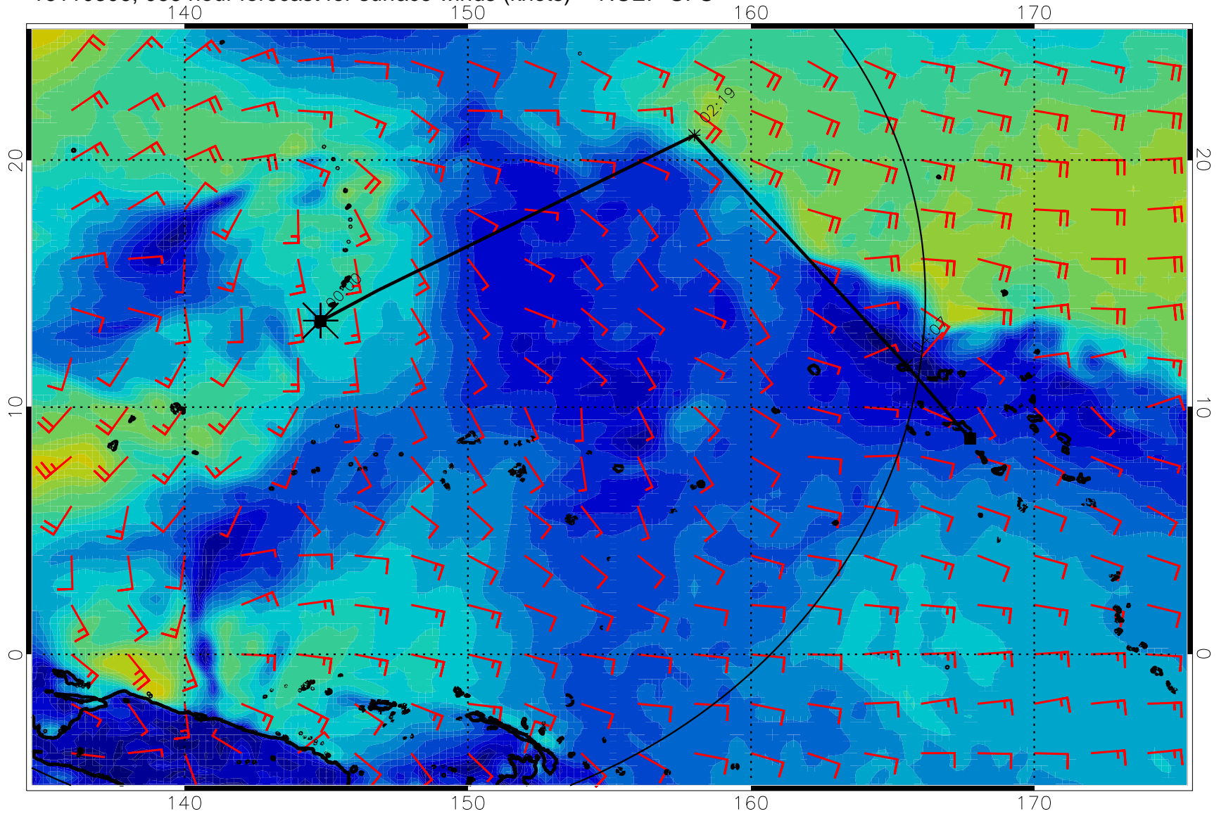
16110306, 066 hour forecast for surface winds (knots) -- NCEP GFS
