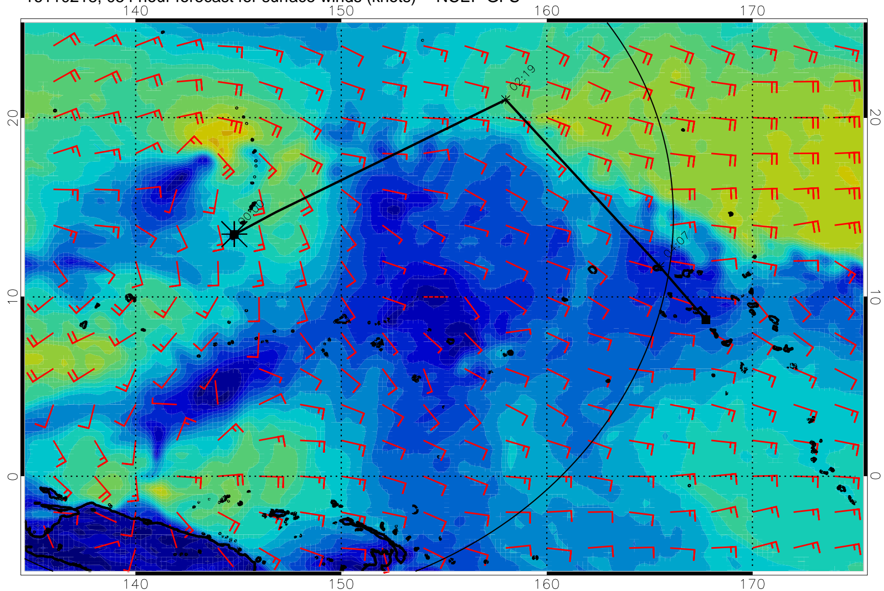
16110218, 054 hour forecast for surface winds (knots) -- NCEP GFS
