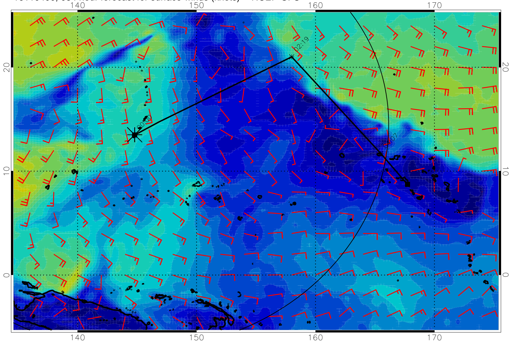
16110400, 084 hour forecast for surface winds (knots) -- NCEP GFS
