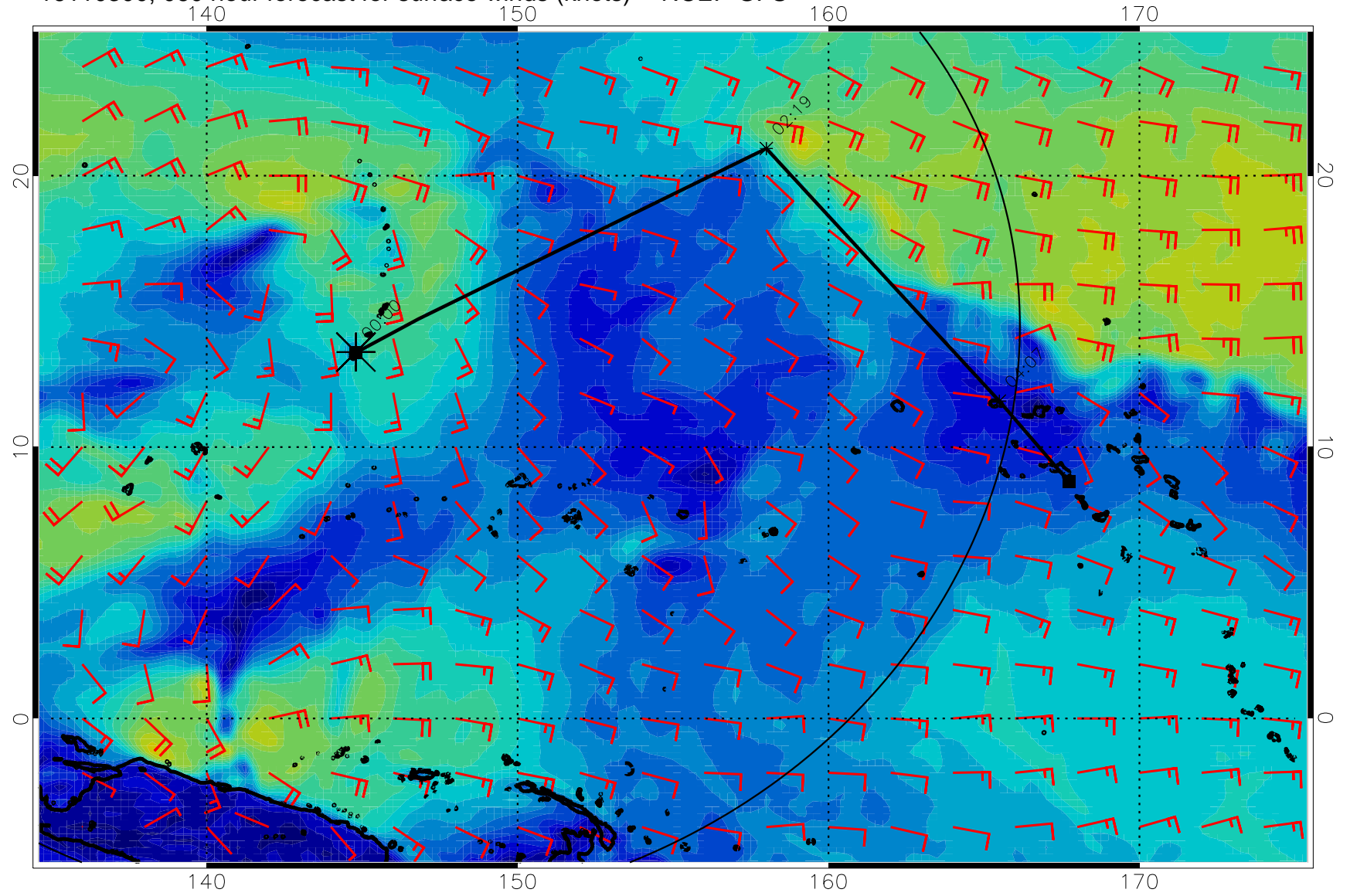
16110300, 060 hour forecast for surface winds (knots) -- NCEP GFS
