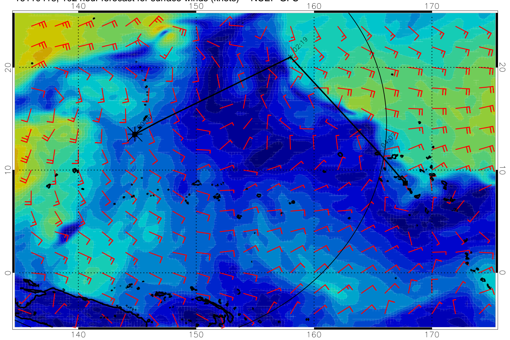
16110418, 102 hour forecast for surface winds (knots) -- NCEP GFS
