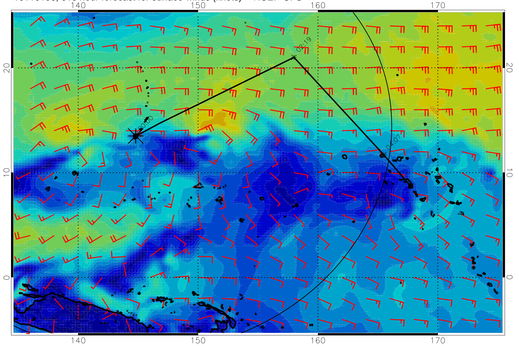
16110106, 018 hour forecast for surface winds (knots) -- NCEP GFS
