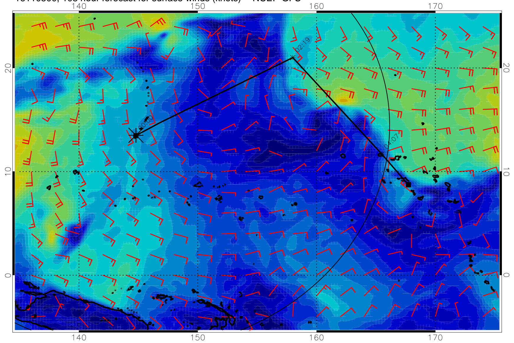
16110500, 108 hour forecast for surface winds (knots) -- NCEP GFS
