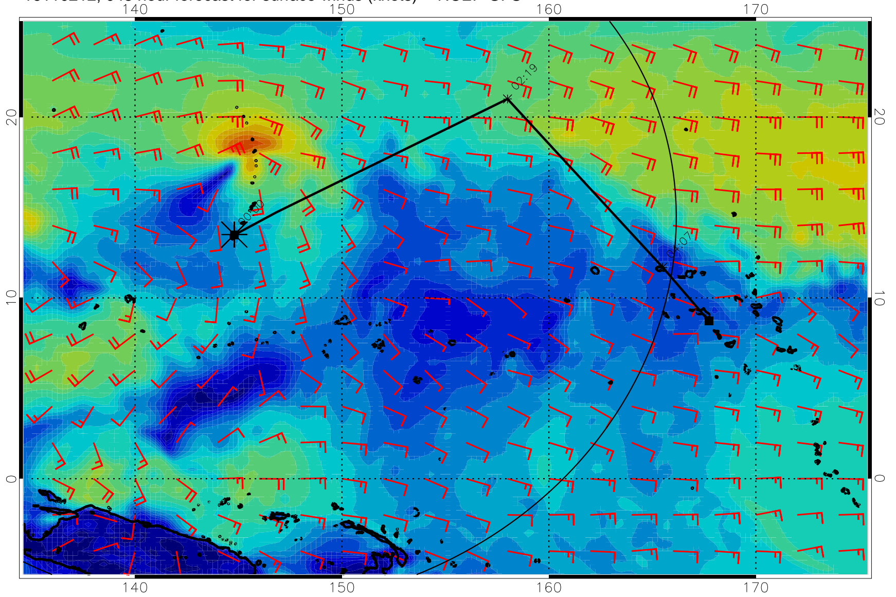
16110212, 048 hour forecast for surface winds (knots) -- NCEP GFS
