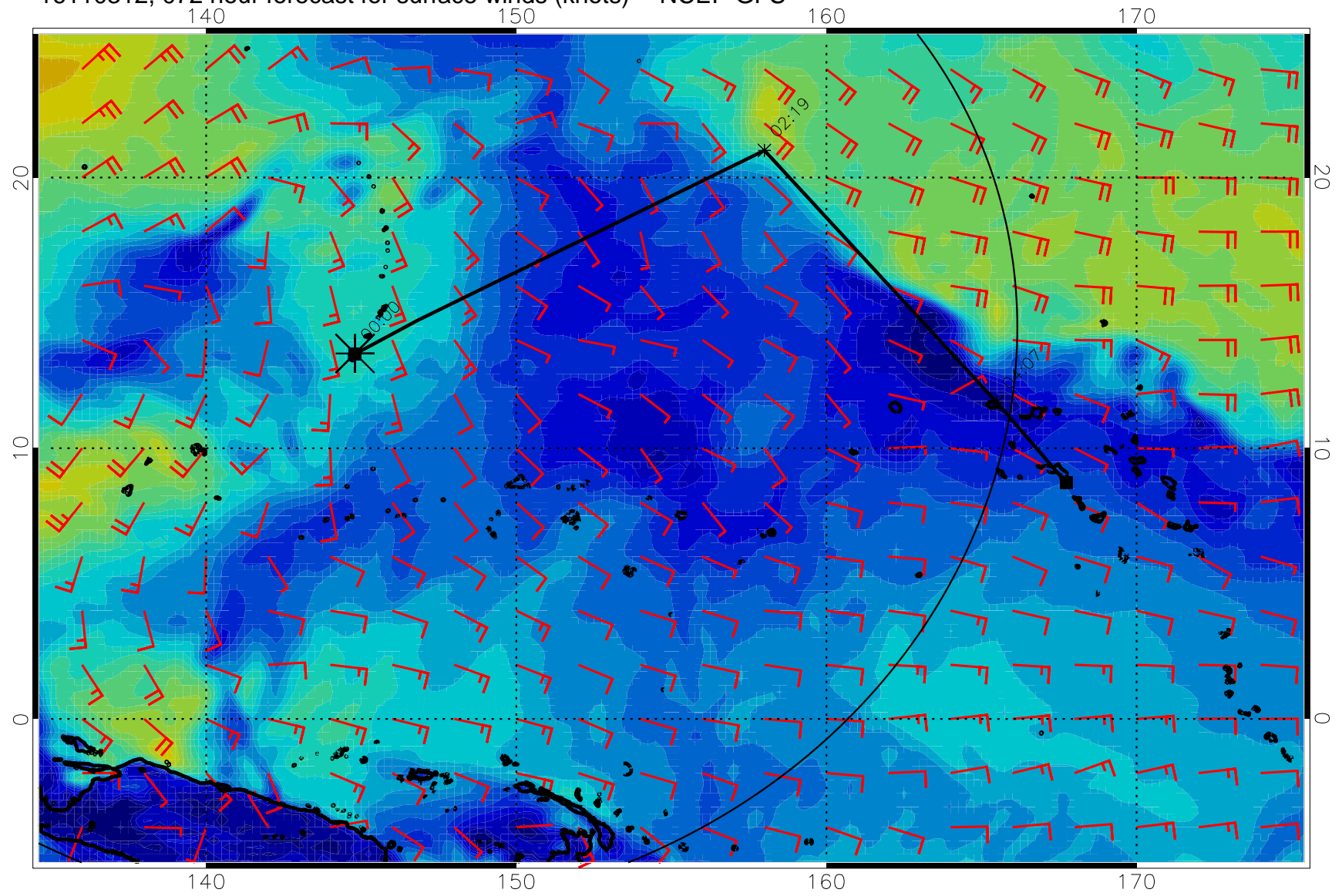
16110312, 072 hour forecast for surface winds (knots) -- NCEP GFS
