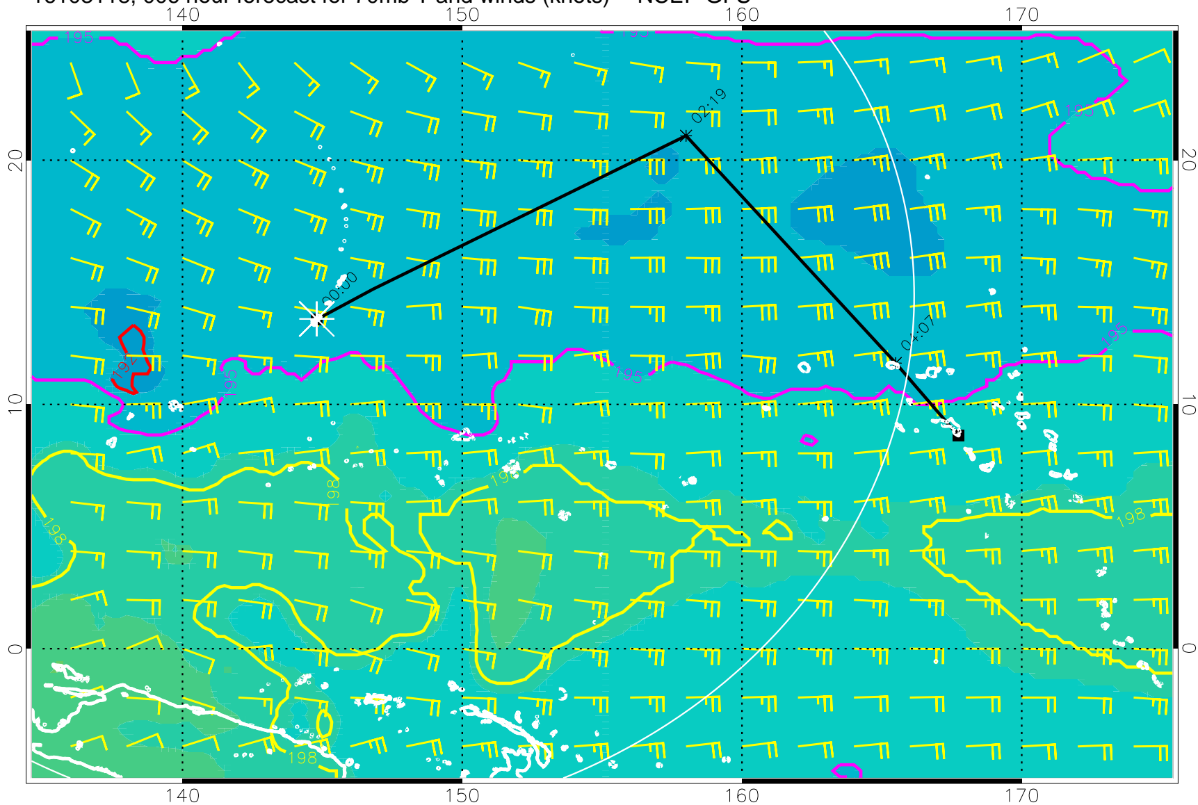
16103118, 006 hour forecast for 70mb T and winds (knots) -- NCEP GFS
