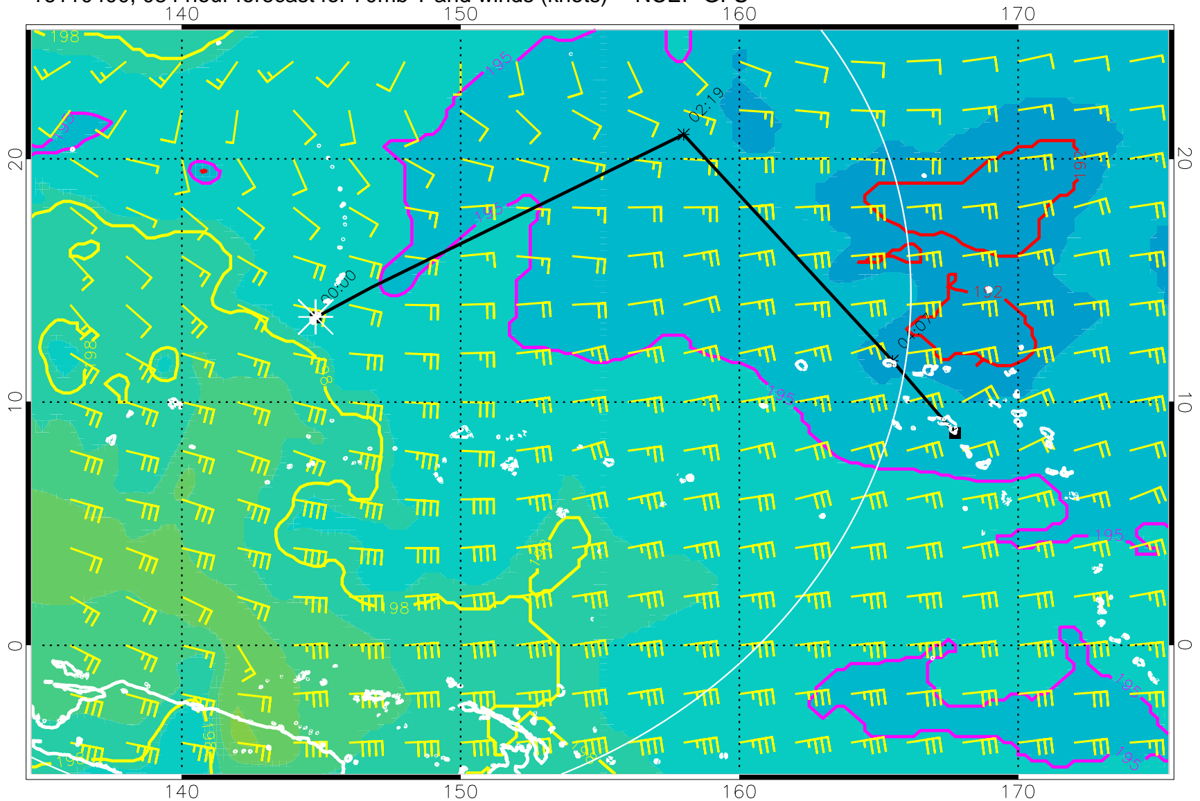
16110400, 084 hour forecast for 70mb T and winds (knots) -- NCEP GFS
