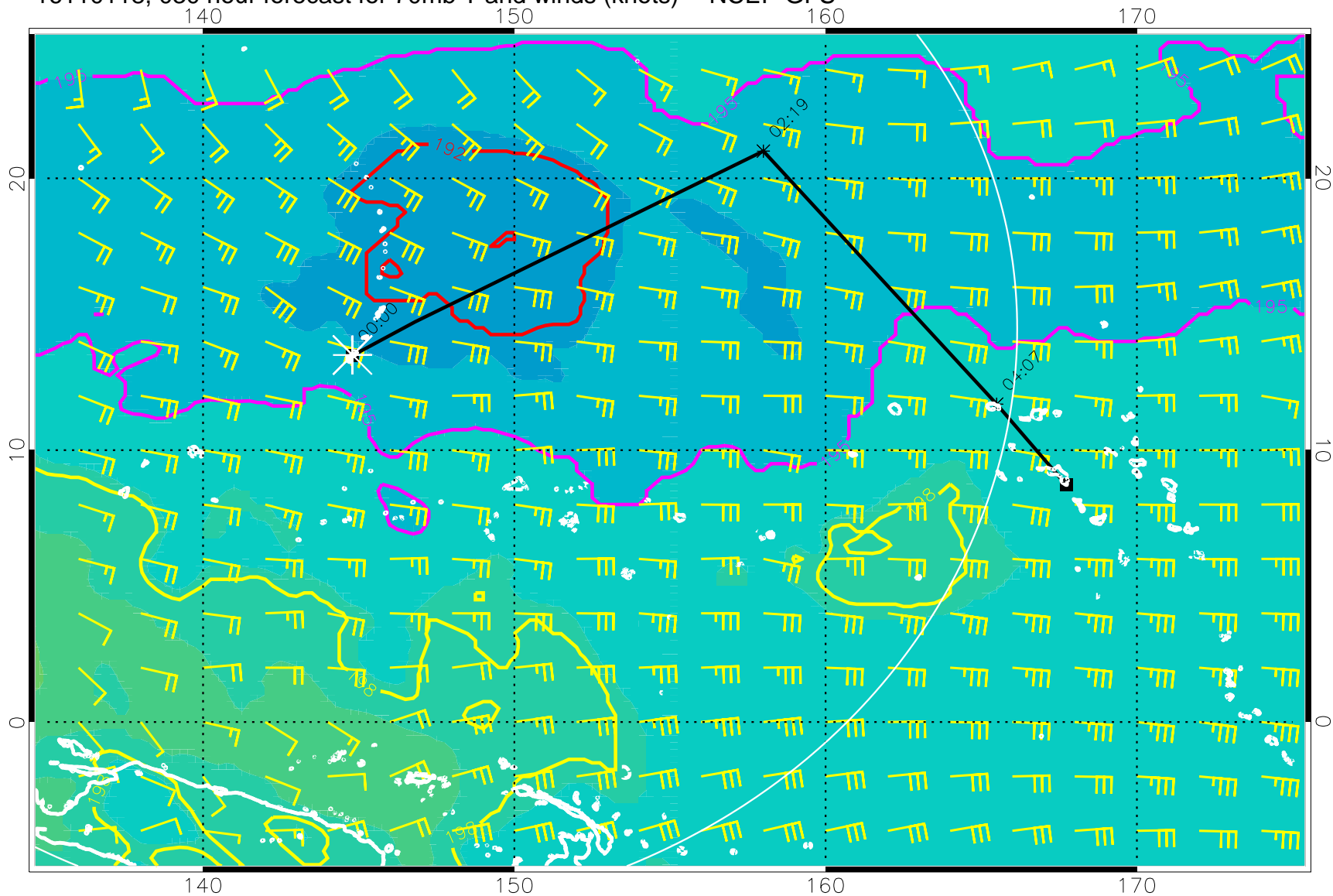
16110118, 030 hour forecast for 70mb T and winds (knots) -- NCEP GFS
