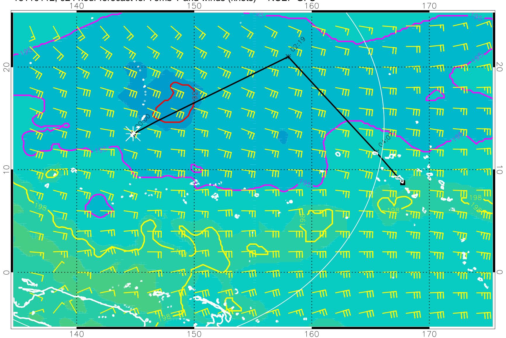
16110112, 024 hour forecast for 70mb T and winds (knots) -- NCEP GFS
