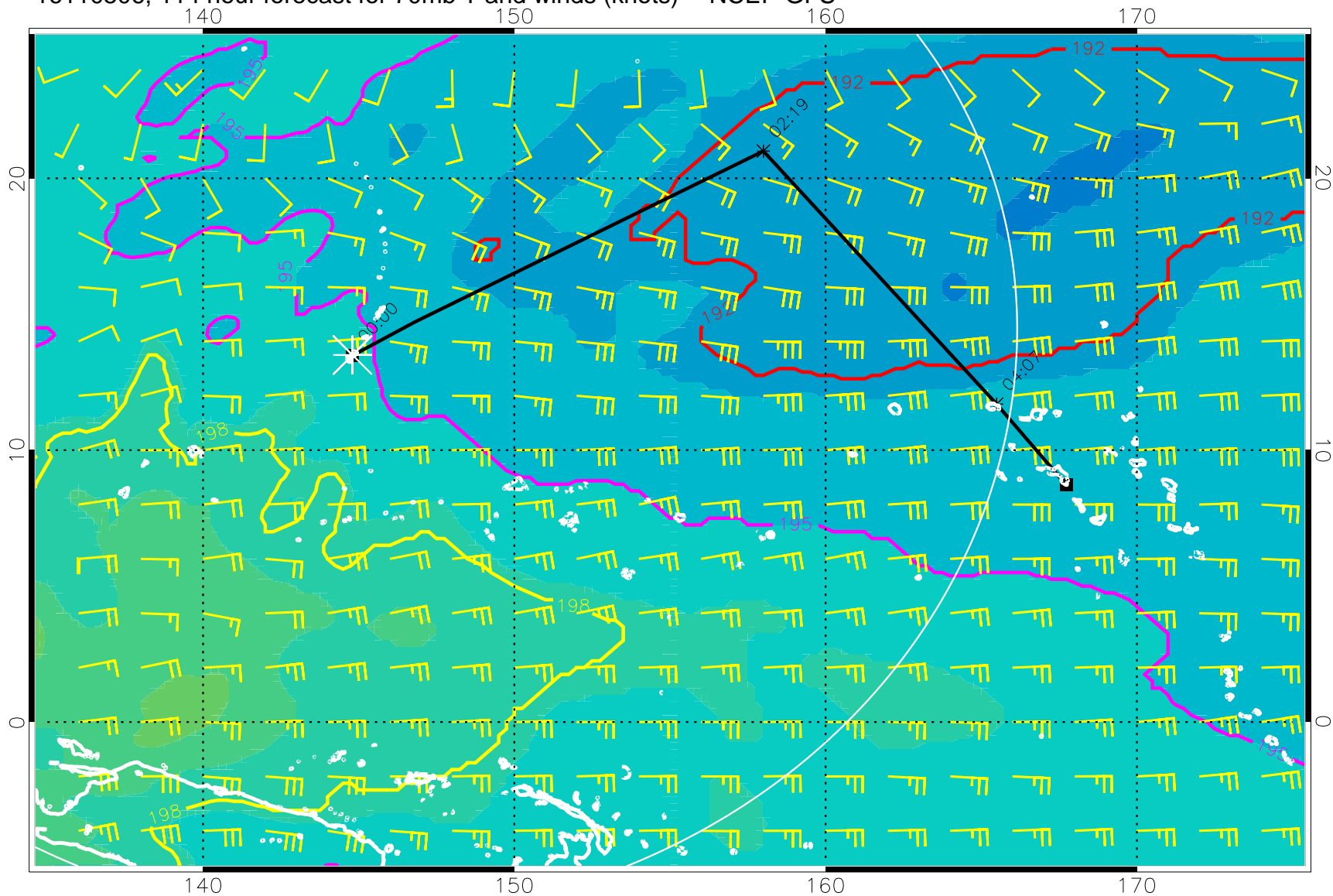
16110506, 114 hour forecast for 70mb T and winds (knots) -- NCEP GFS
