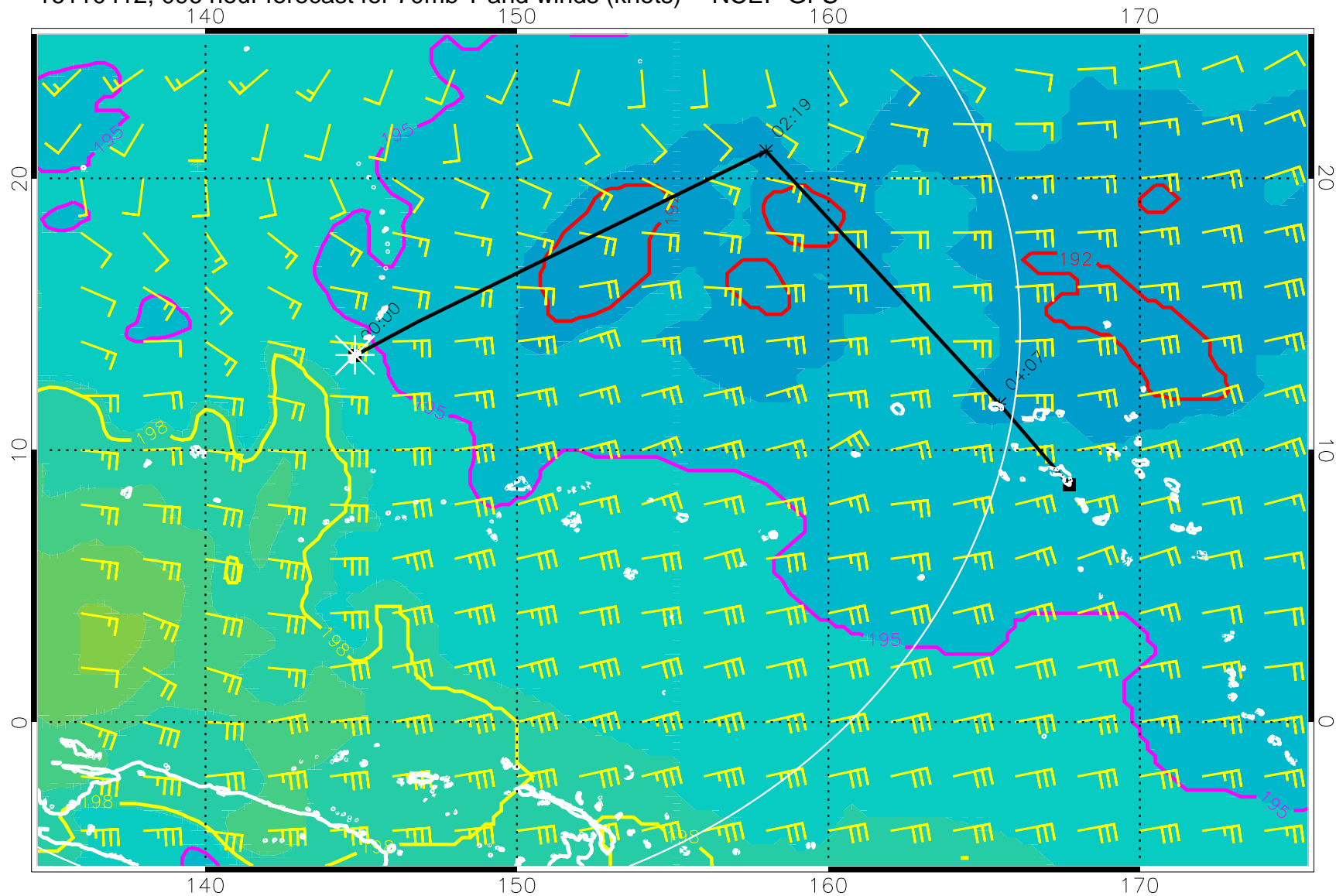
16110412, 096 hour forecast for 70mb T and winds (knots) -- NCEP GFS
