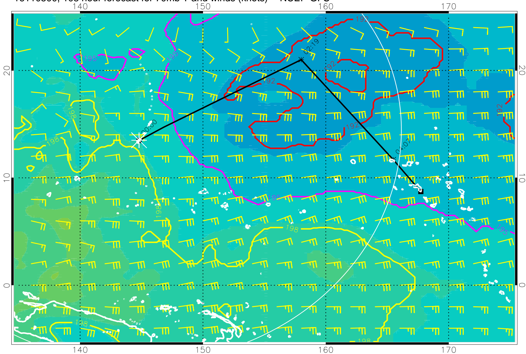
16110500, 108 hour forecast for 70mb T and winds (knots) -- NCEP GFS
