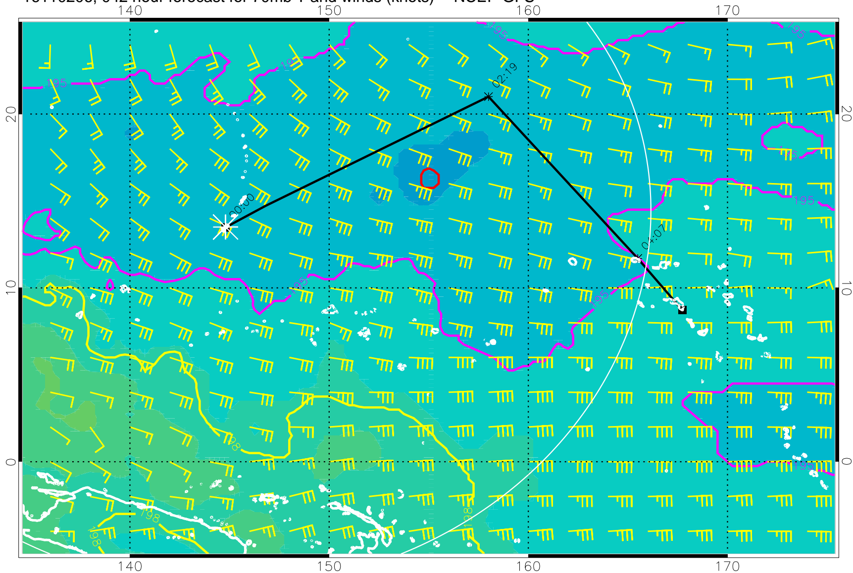
16110206, 042 hour forecast for 70mb T and winds (knots) -- NCEP GFS
