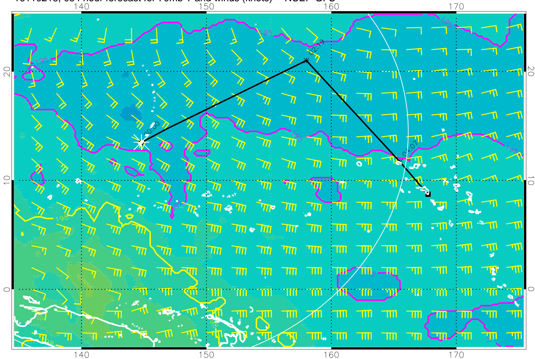
16110218, 054 hour forecast for 70mb T and winds (knots) -- NCEP GFS
