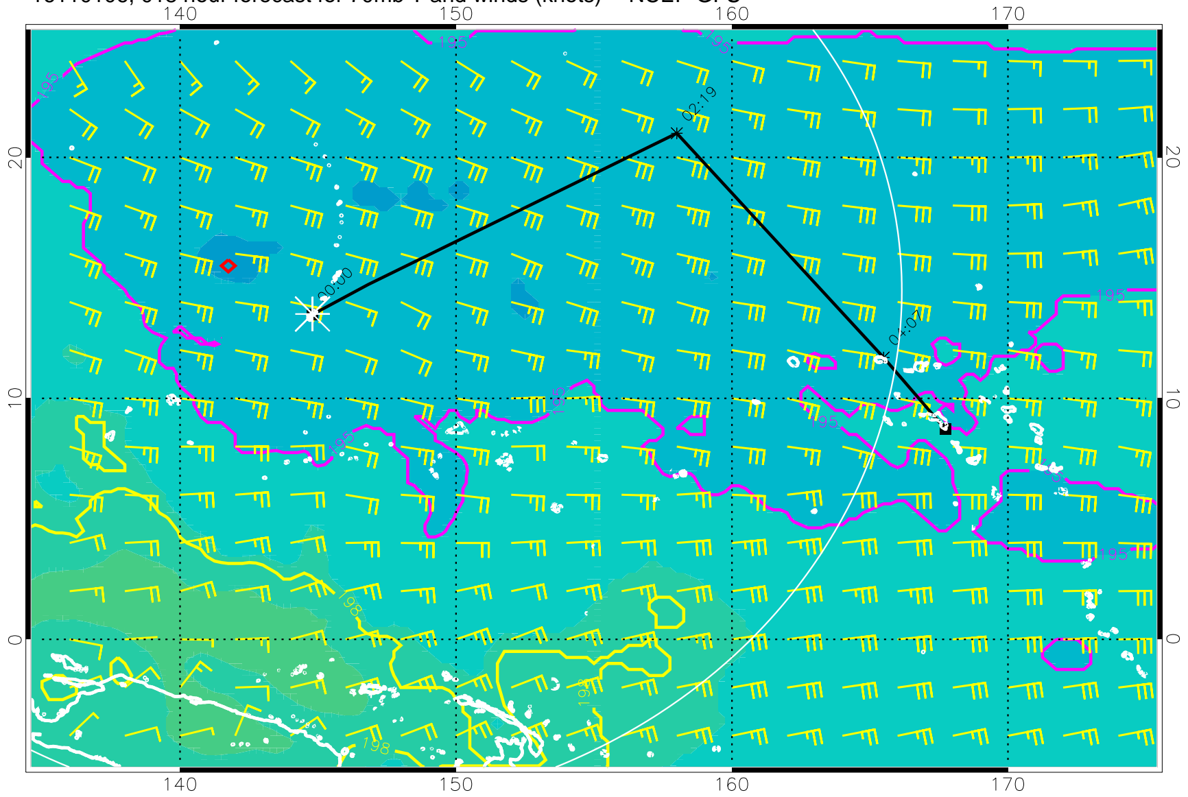
16110106, 018 hour forecast for 70mb T and winds (knots) -- NCEP GFS
