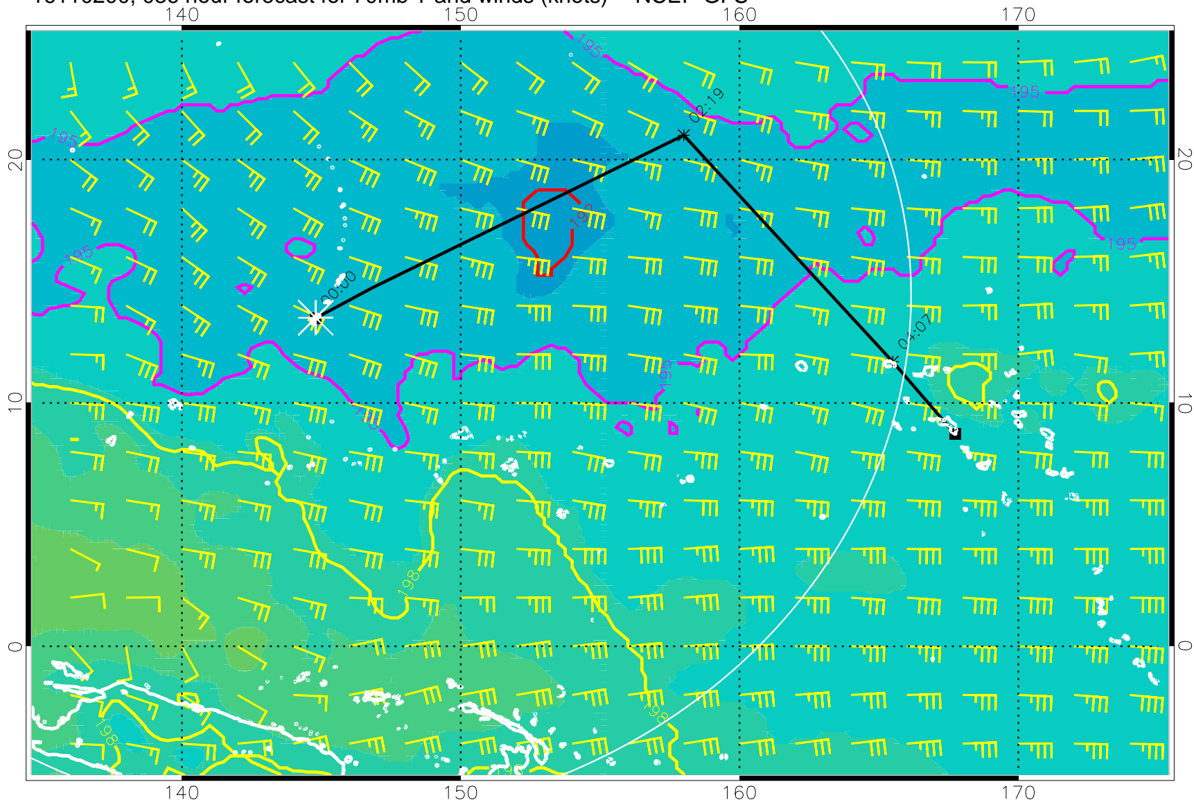
16110200, 036 hour forecast for 70mb T and winds (knots) -- NCEP GFS
