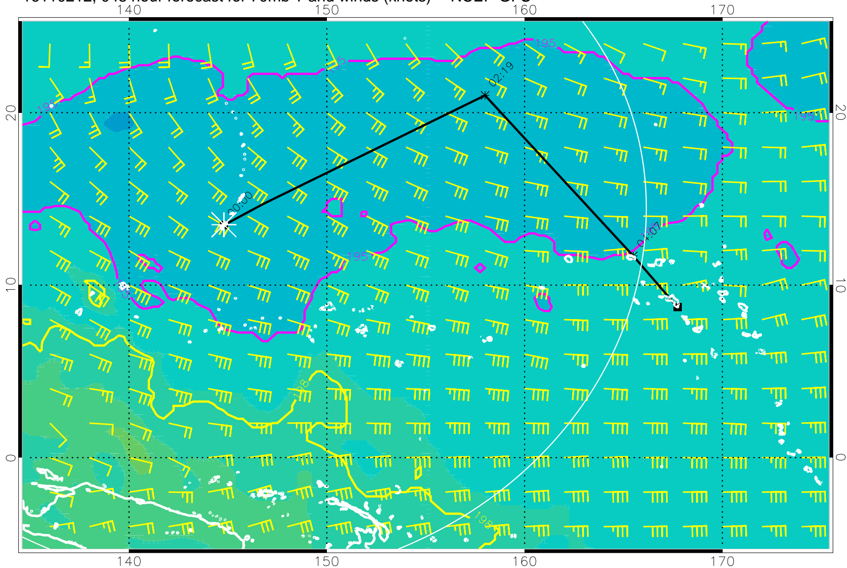
16110212, 048 hour forecast for 70mb T and winds (knots) -- NCEP GFS
