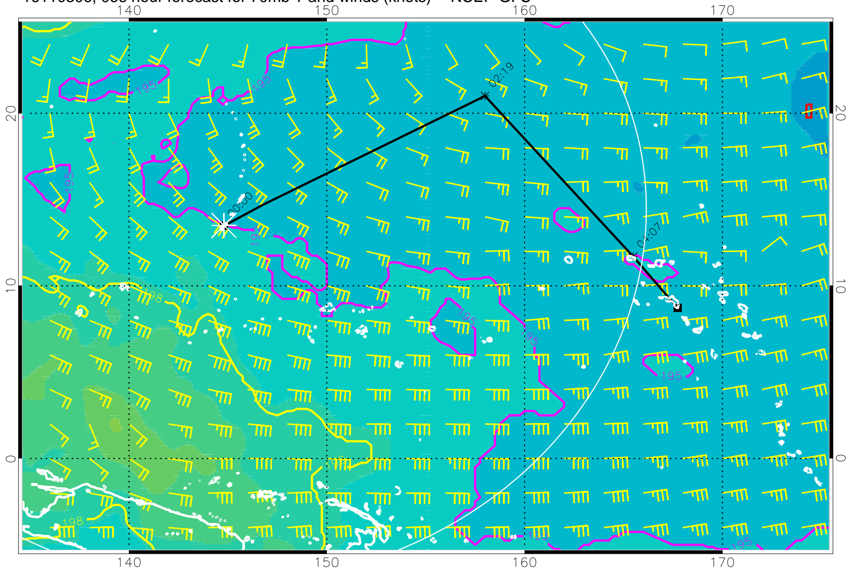
16110306, 066 hour forecast for 70mb T and winds (knots) -- NCEP GFS
