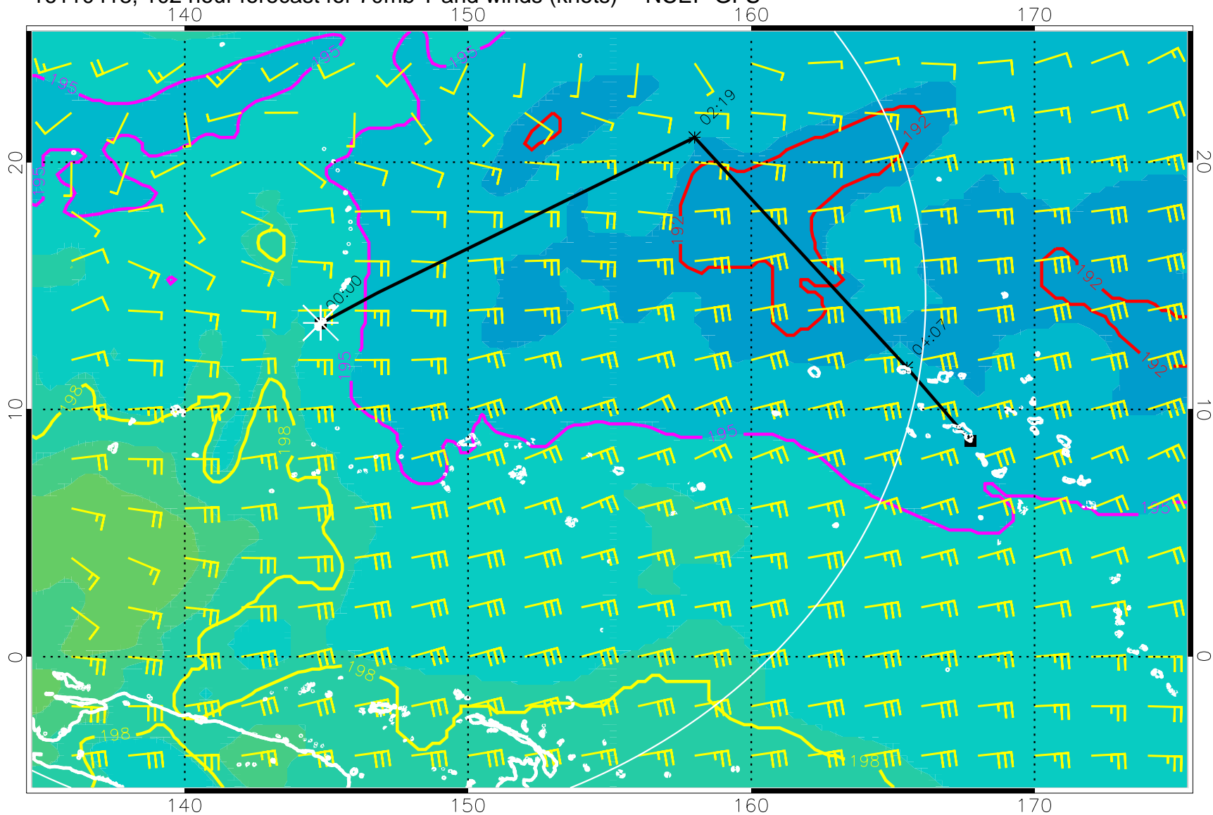
16110418, 102 hour forecast for 70mb T and winds (knots) -- NCEP GFS
