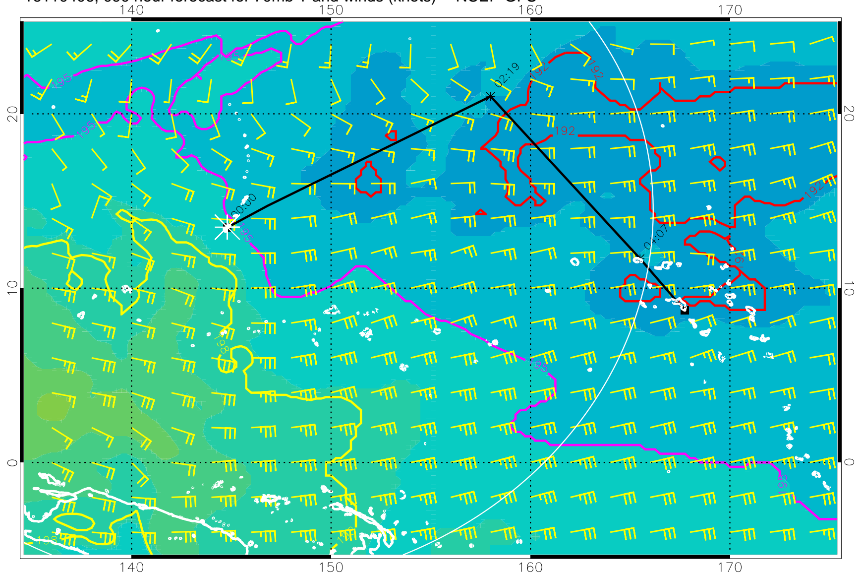
16110406, 090 hour forecast for 70mb T and winds (knots) -- NCEP GFS
