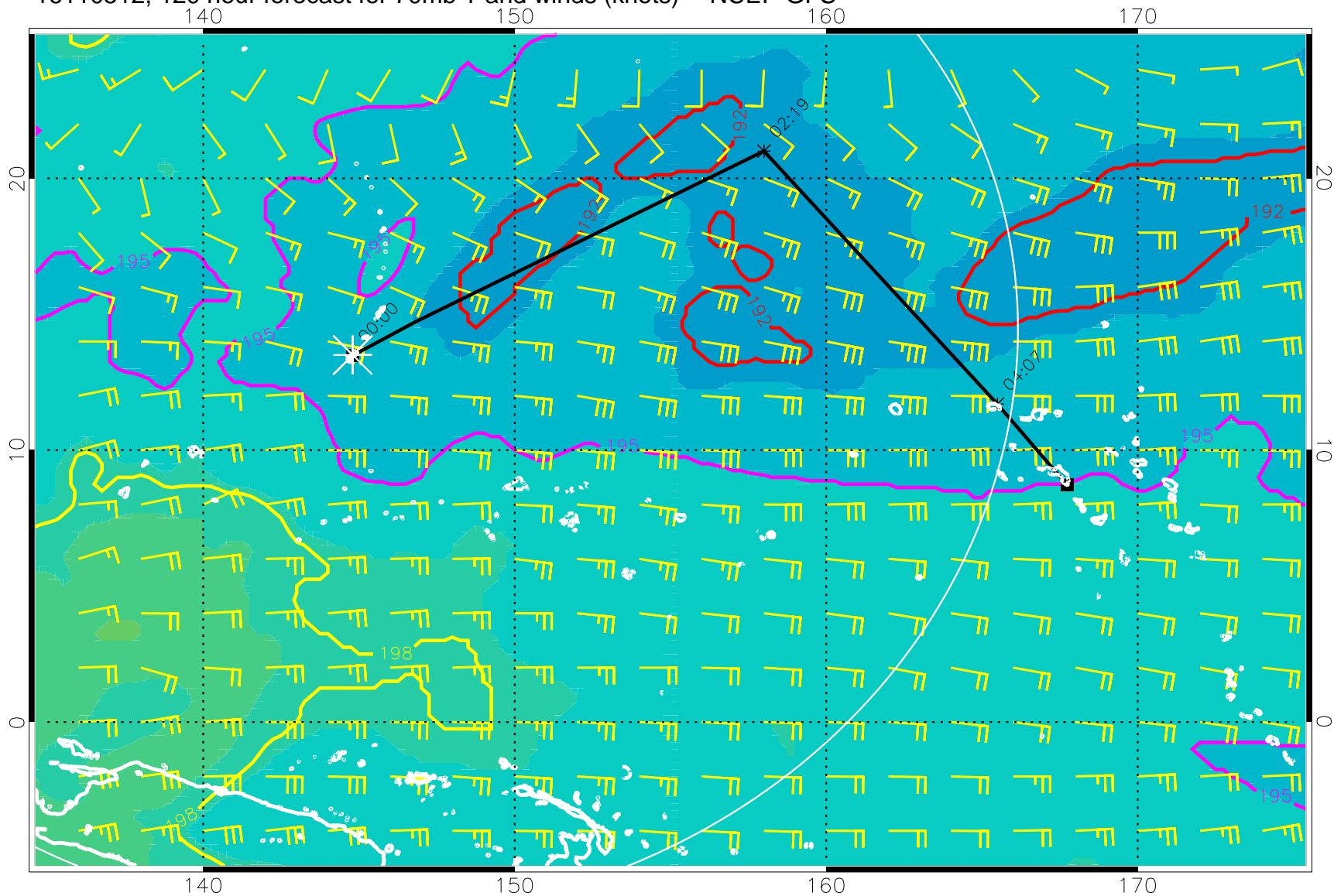
16110512, 120 hour forecast for 70mb T and winds (knots) -- NCEP GFS
