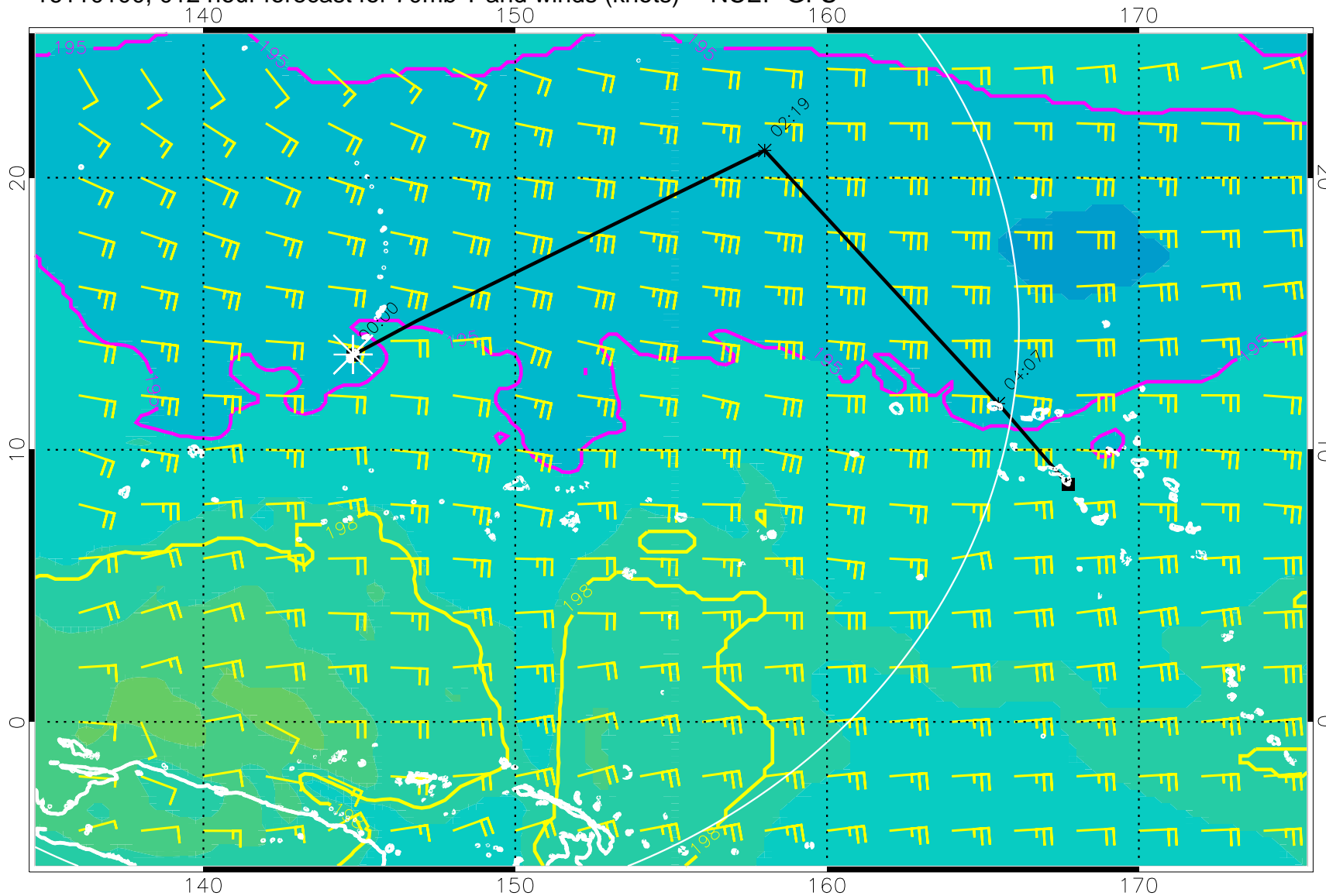
16110100, 012 hour forecast for 70mb T and winds (knots) -- NCEP GFS
