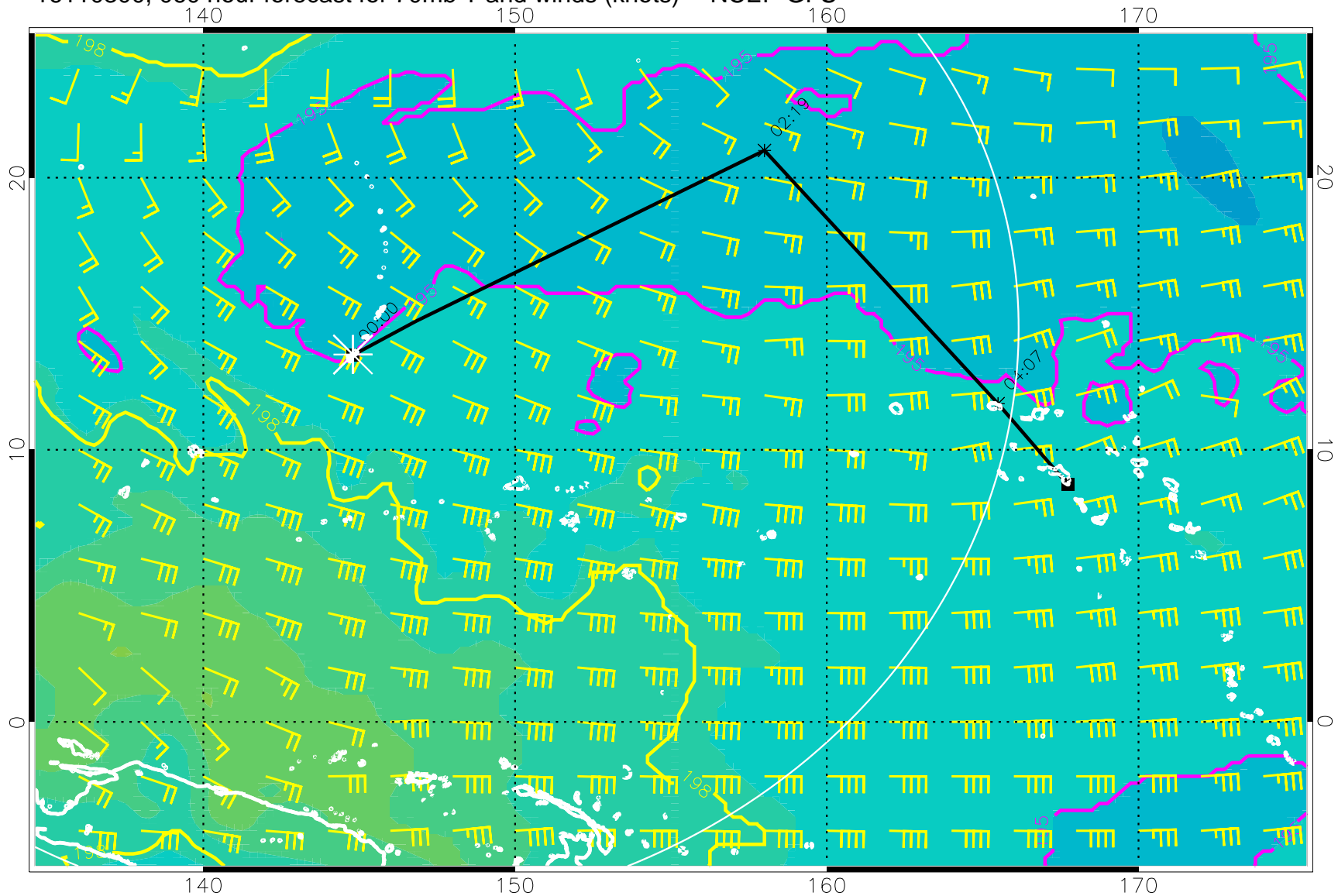
16110300, 060 hour forecast for 70mb T and winds (knots) -- NCEP GFS
