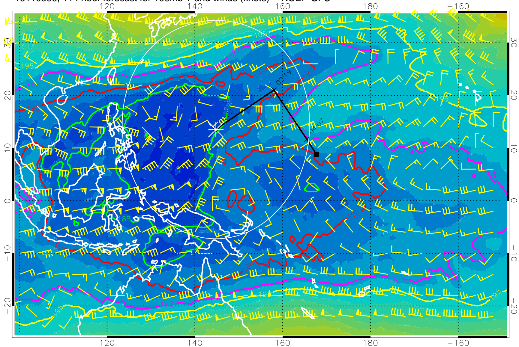
16110506, 114 hour forecast for 100mb T and winds (knots) -- NCEP GFS
