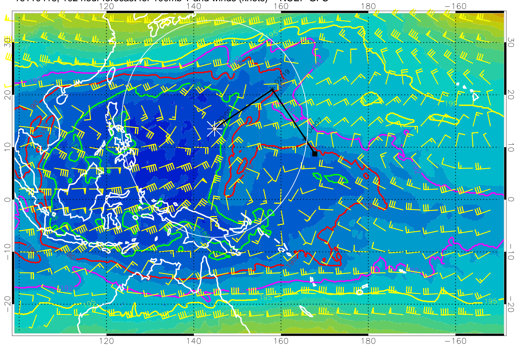
16110418, 102 hour forecast for 100mb T and winds (knots) -- NCEP GFS
