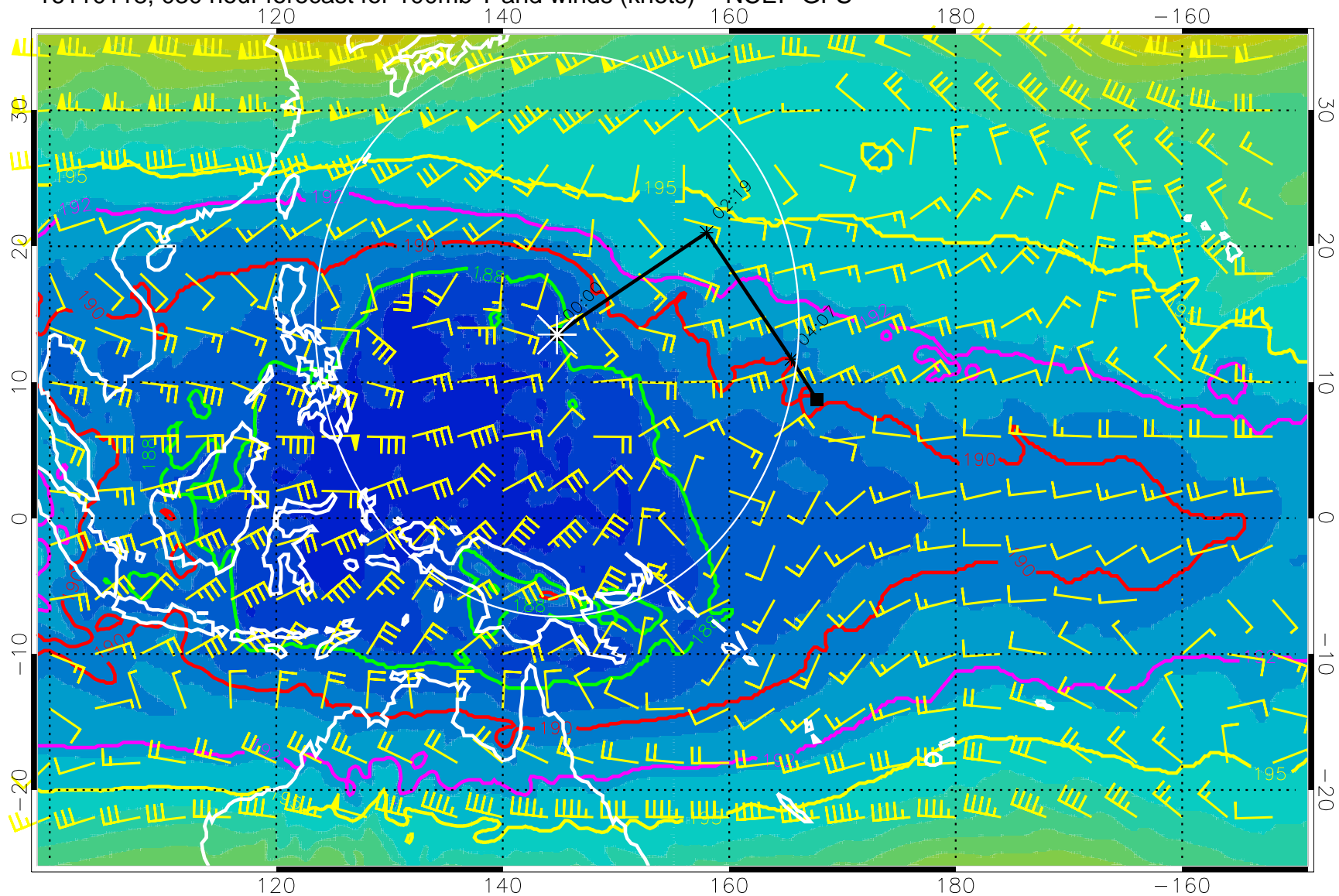
16110118, 030 hour forecast for 100mb T and winds (knots) -- NCEP GFS
