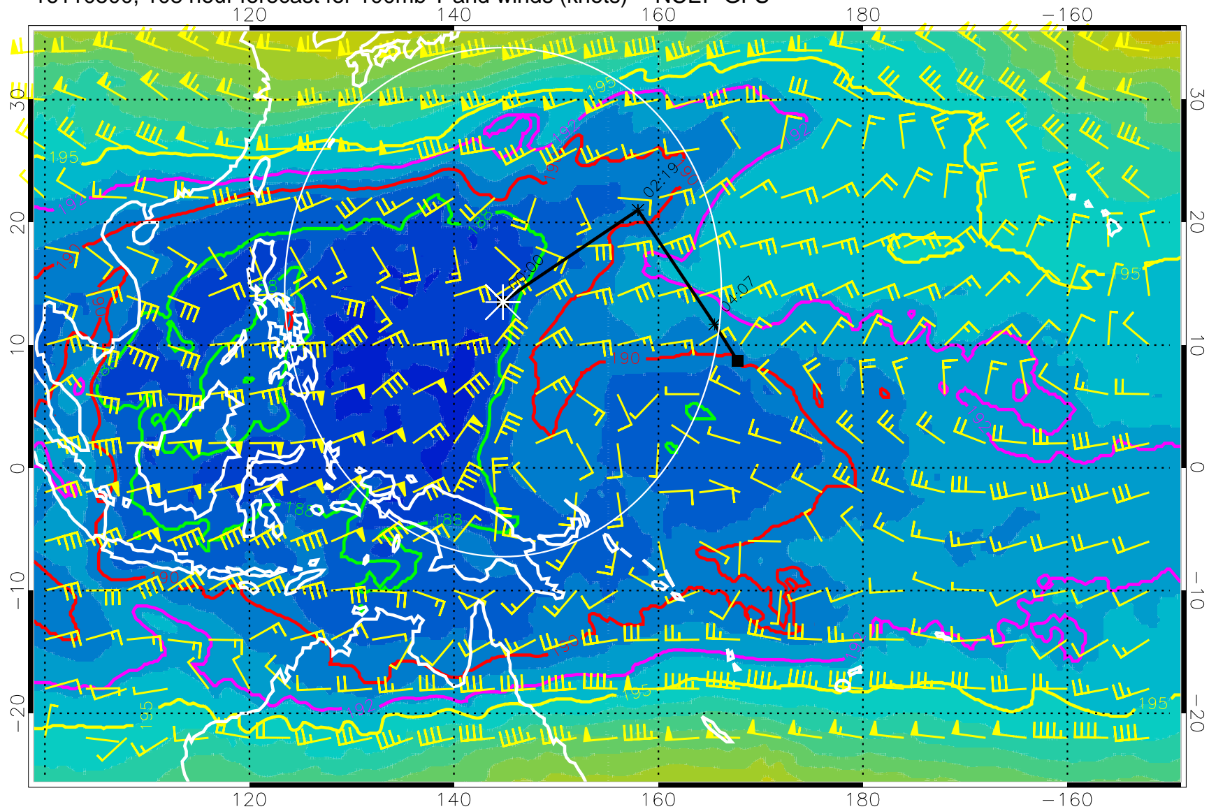
16110500, 108 hour forecast for 100mb T and winds (knots) -- NCEP GFS
