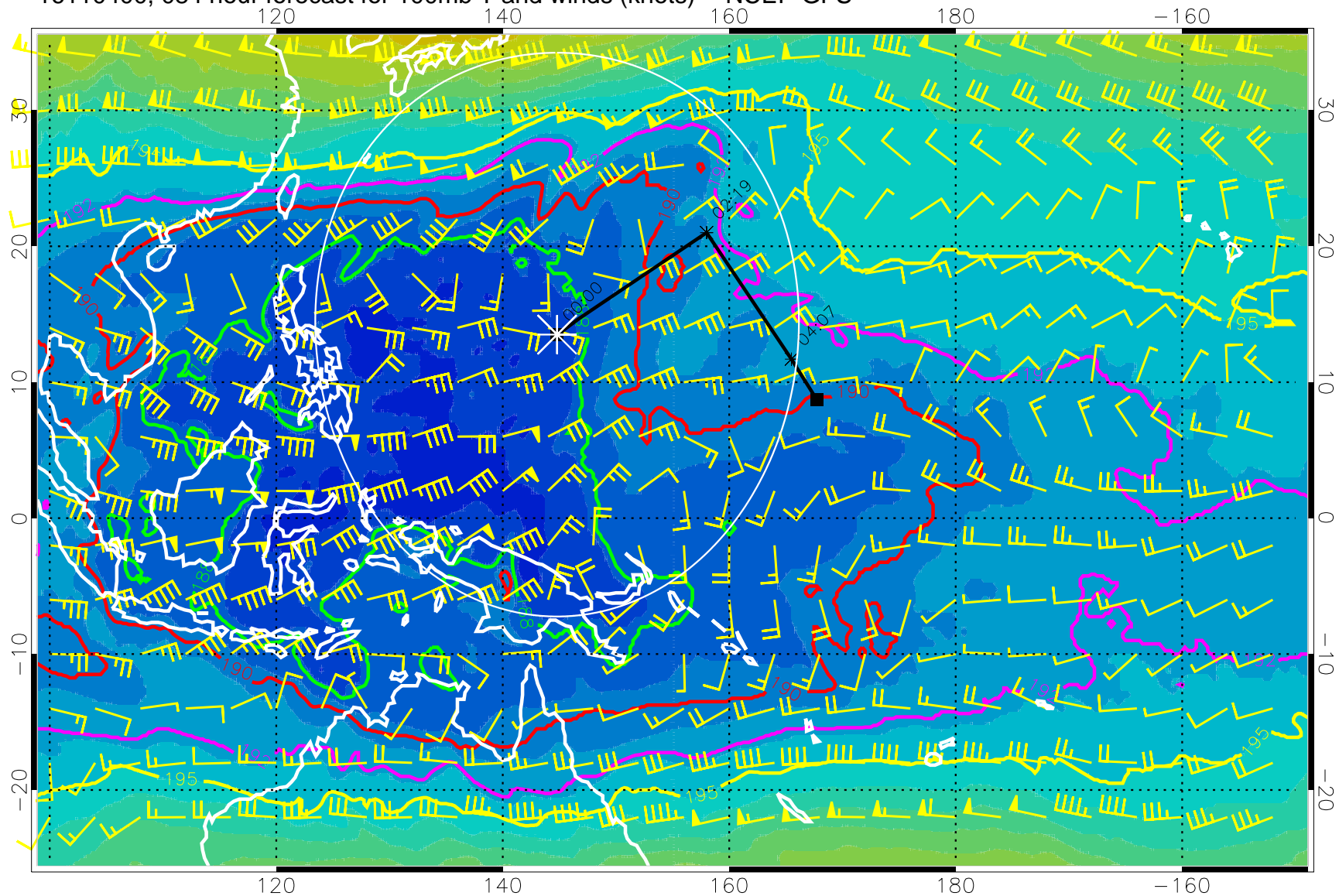
16110400, 084 hour forecast for 100mb T and winds (knots) -- NCEP GFS
