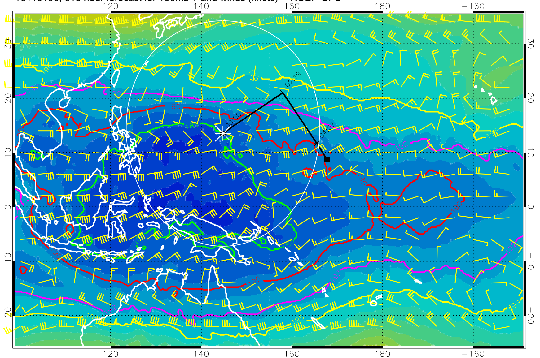
16110106, 018 hour forecast for 100mb T and winds (knots) -- NCEP GFS
