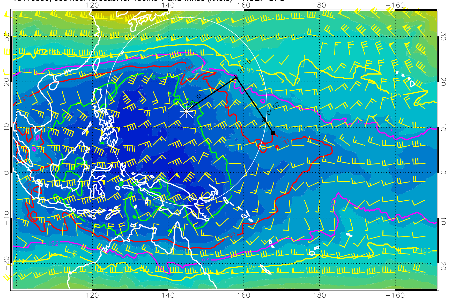
16110300, 060 hour forecast for 100mb T and winds (knots) -- NCEP GFS
