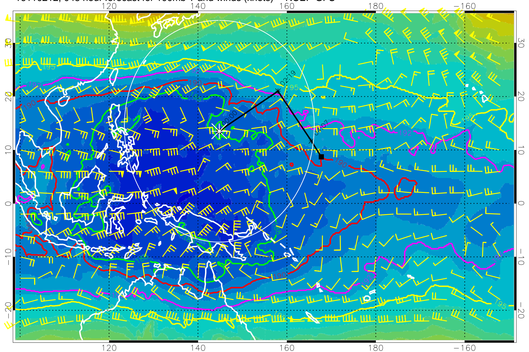
16110212, 048 hour forecast for 100mb T and winds (knots) -- NCEP GFS
