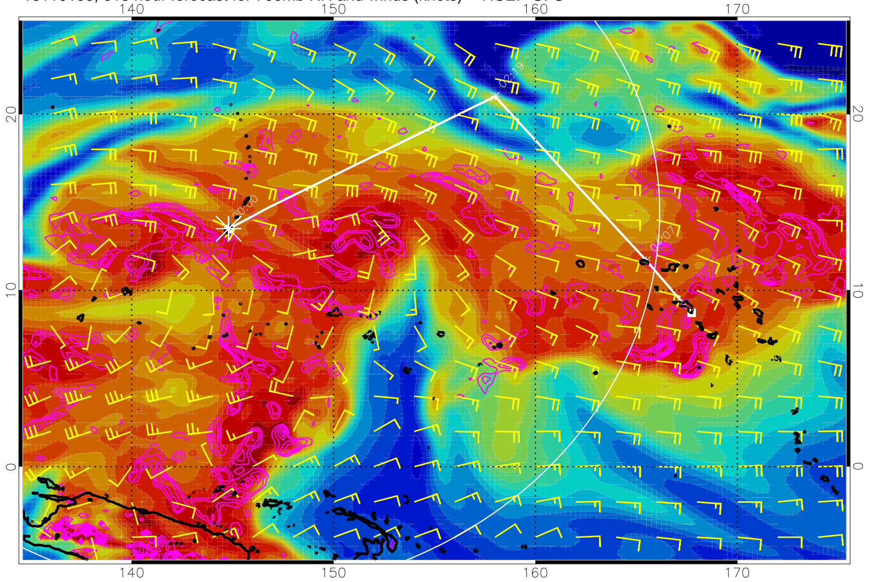
16110106, 018 hour forecast for 700mb RH and winds (knots) -- NCEP GFS
