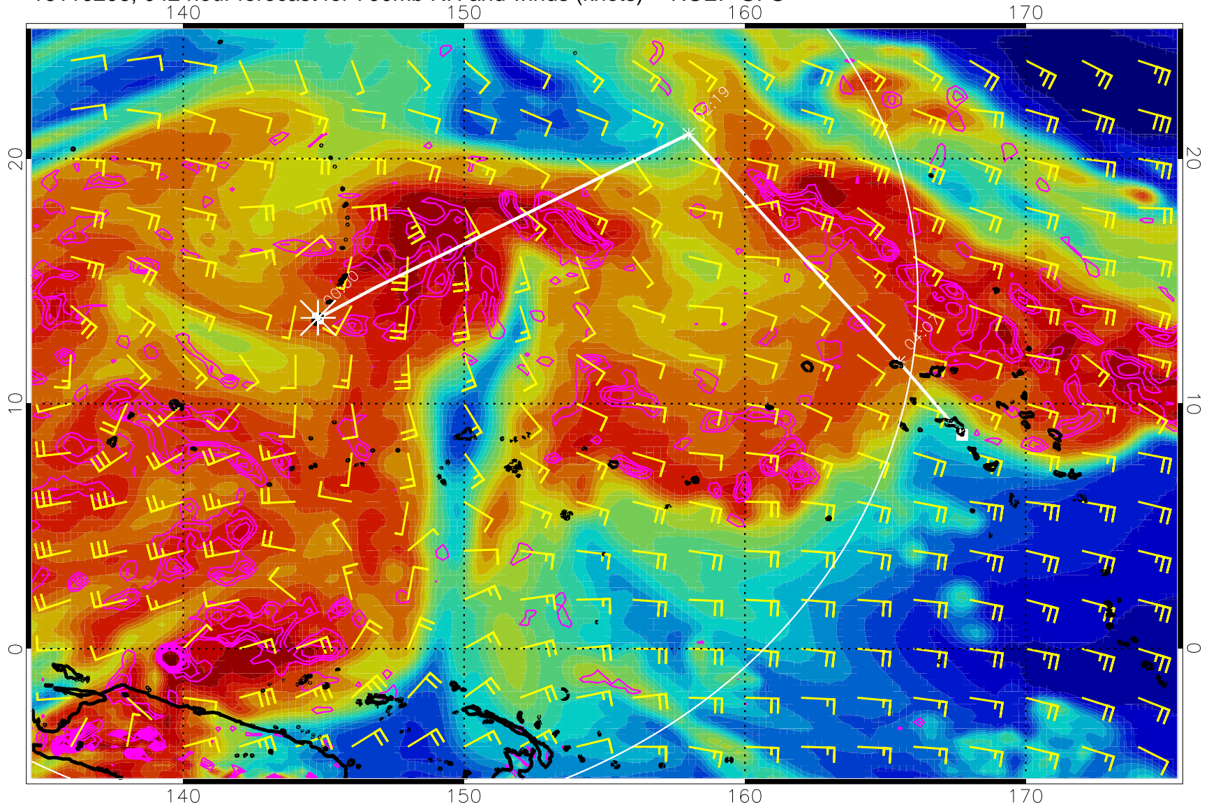
16110206, 042 hour forecast for 700mb RH and winds (knots) -- NCEP GFS
