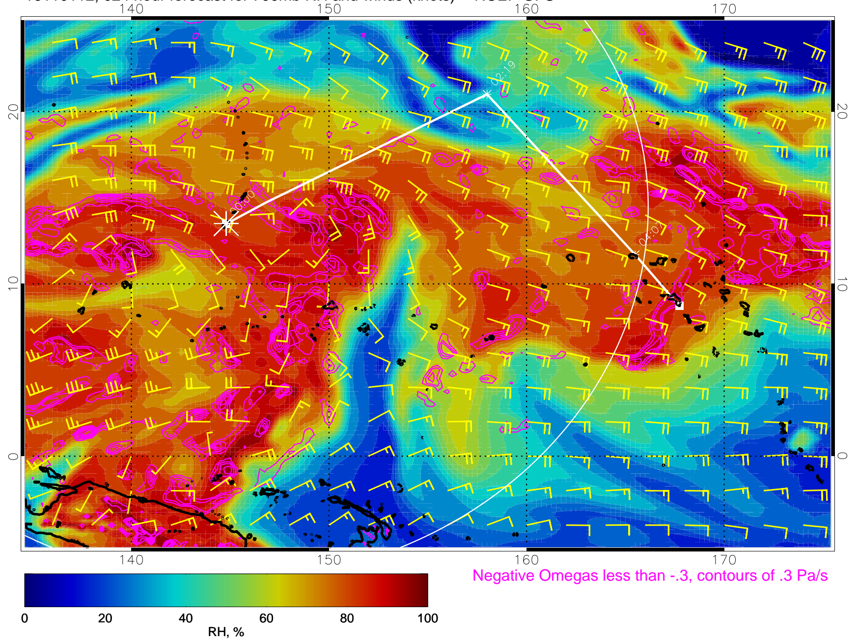
16110112, 024 hour forecast for 700mb RH and winds (knots) -- NCEP GFS
