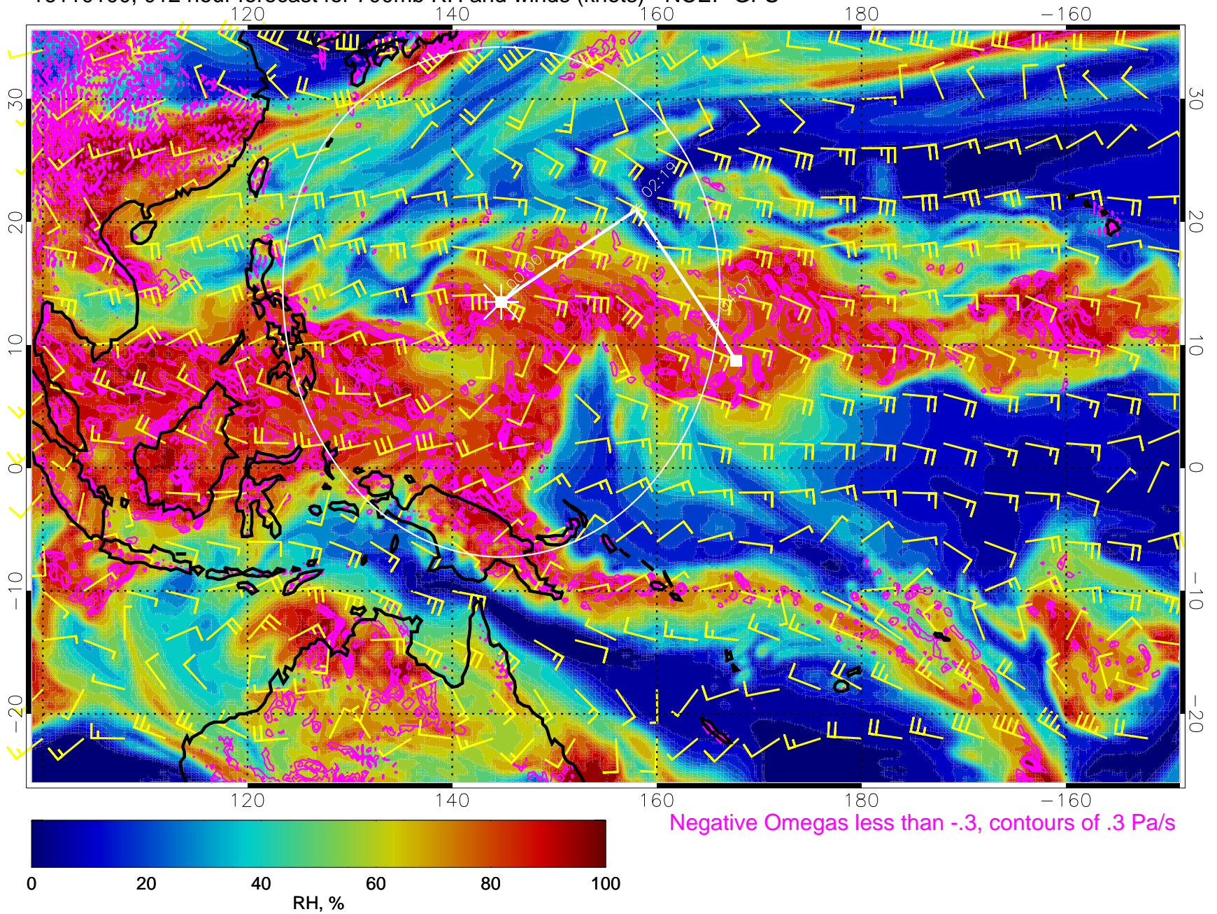
16110100, 012 hour forecast for 700mb RH and winds (knots) - NCEP GFS
