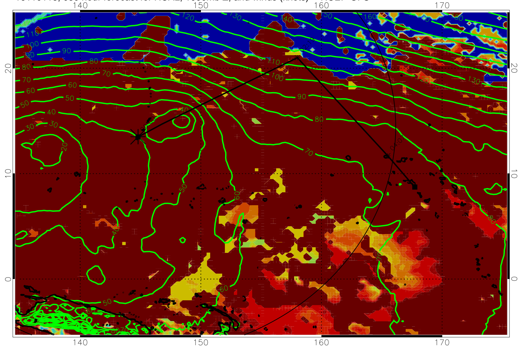
16110118, 030 hour forecast for HCAL, 1000mb Z, and winds (knots) -- NCEP GFS
