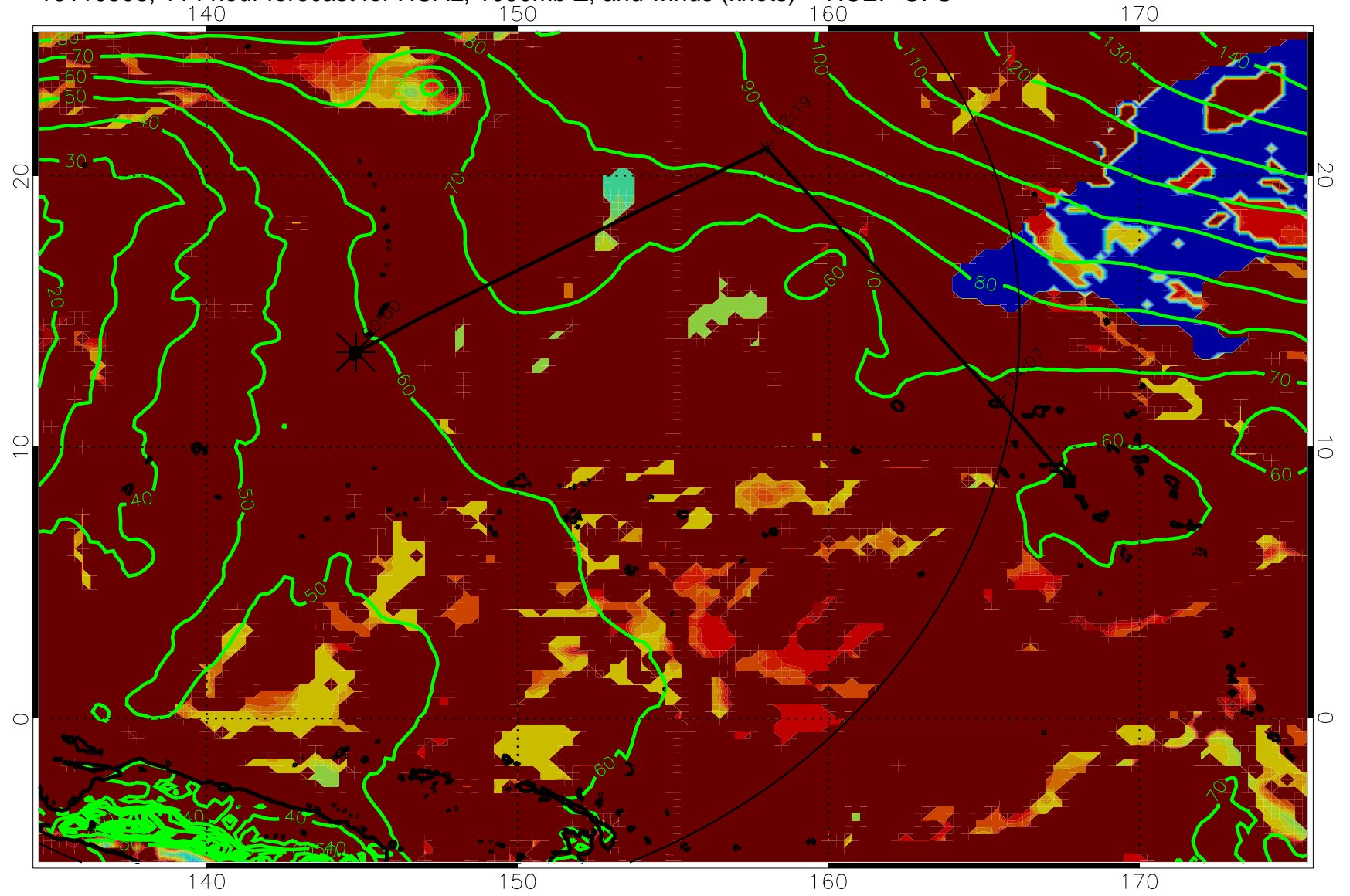
16110506, 114 hour forecast for HCAL, 1000mb Z, and winds (knots) -- NCEP GFS
