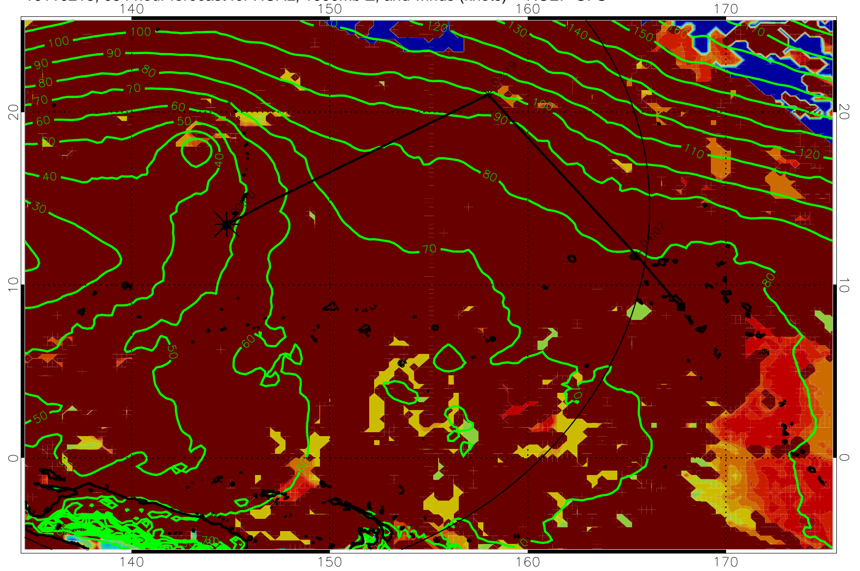
16110218, 054 hour forecast for HCAL, 1000mb Z, and winds (knots) -- NCEP GFS
