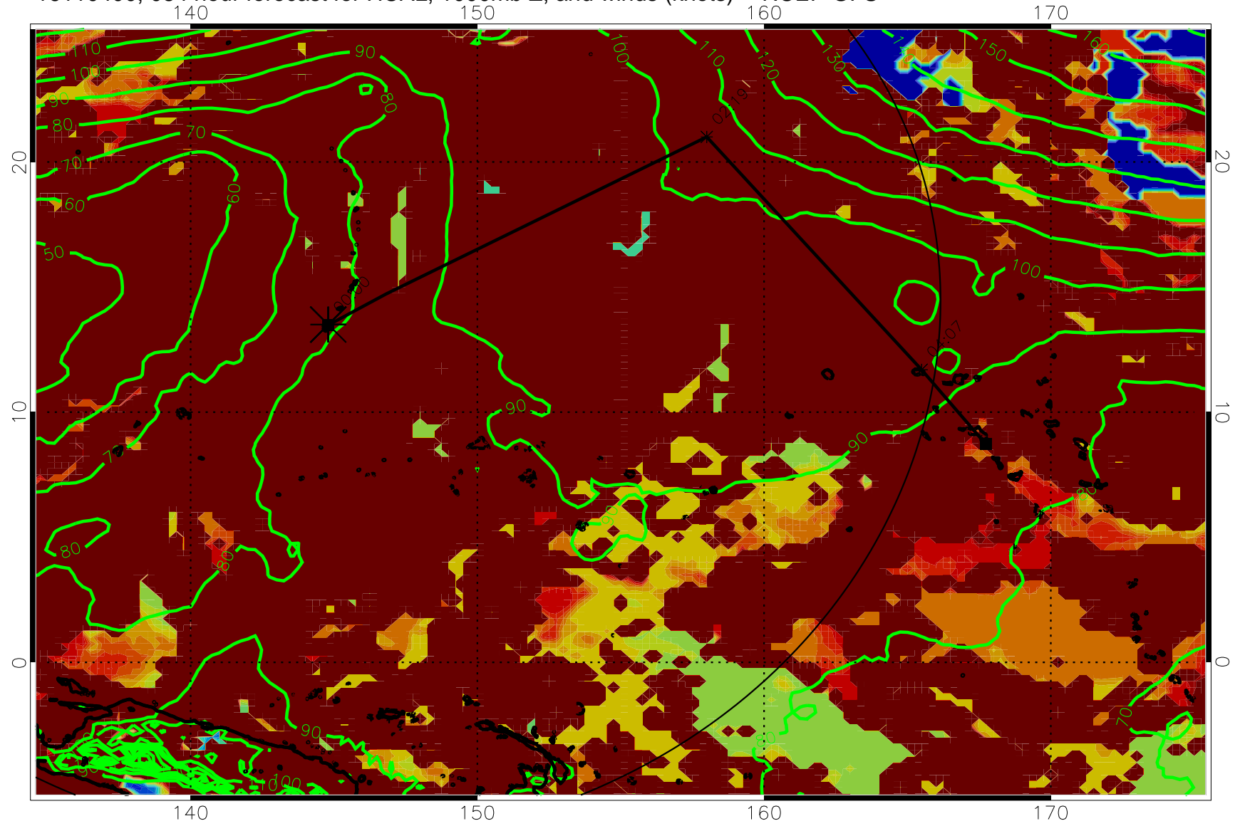
16110400, 084 hour forecast for HCAL, 1000mb Z, and winds (knots) -- NCEP GFS
