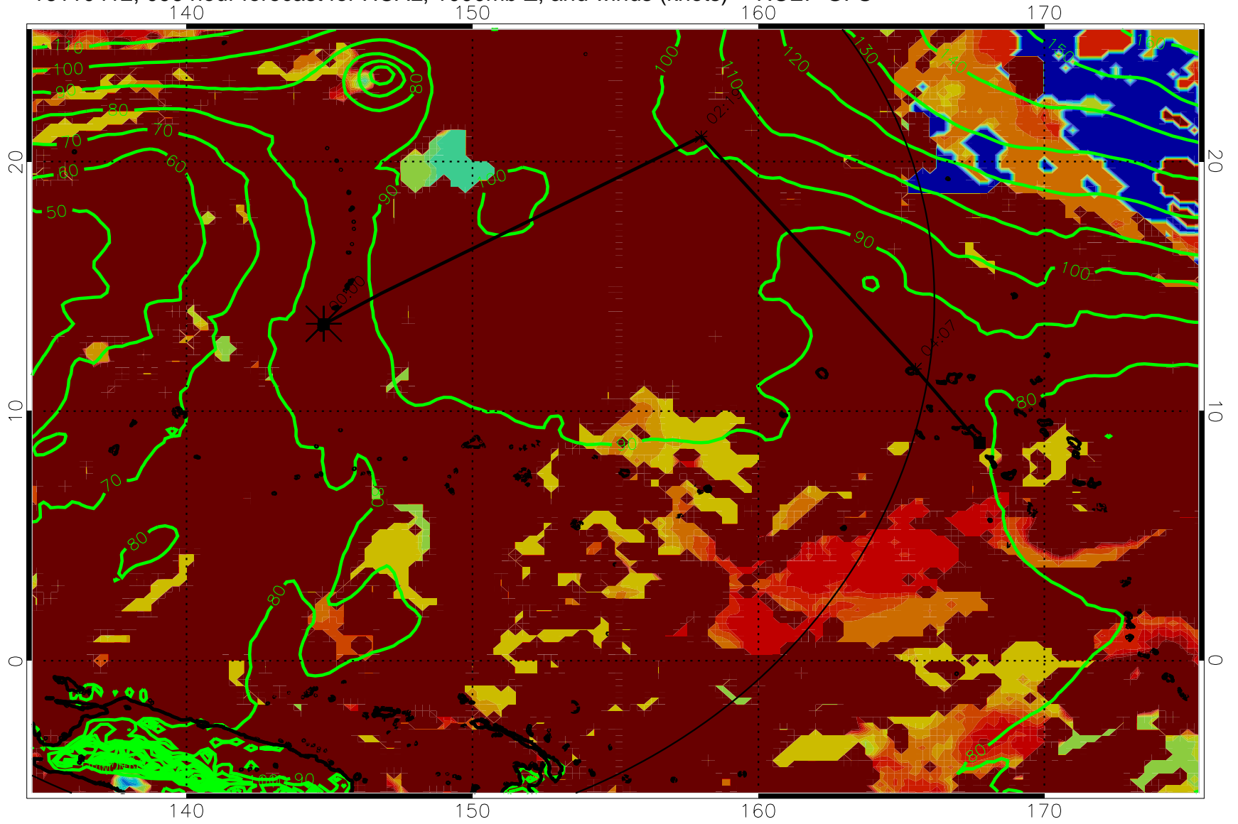
16110412, 096 hour forecast for HCAL, 1000mb Z, and winds (knots) -- NCEP GFS
