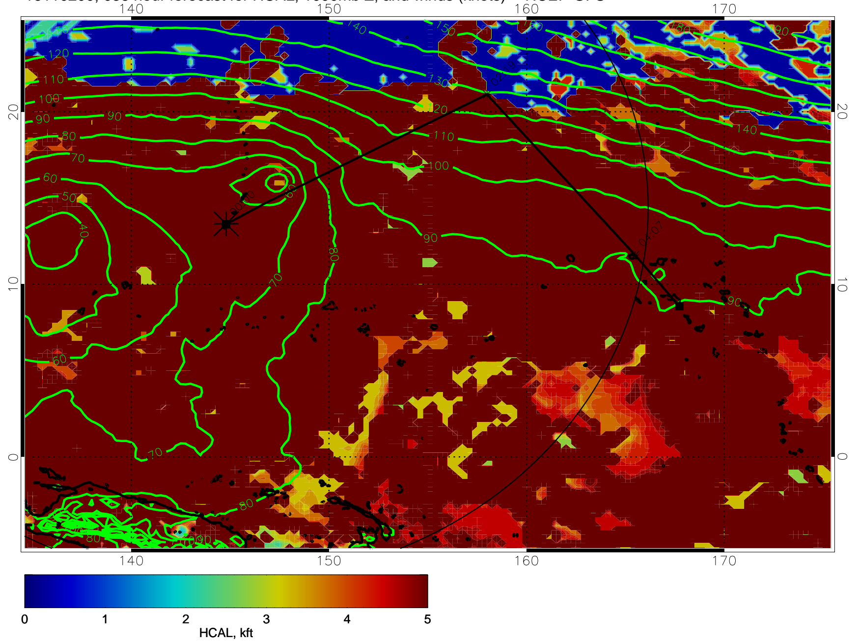
16110200, 036 hour forecast for HCAL, 1000mb Z, and winds (knots) -- NCEP GFS
