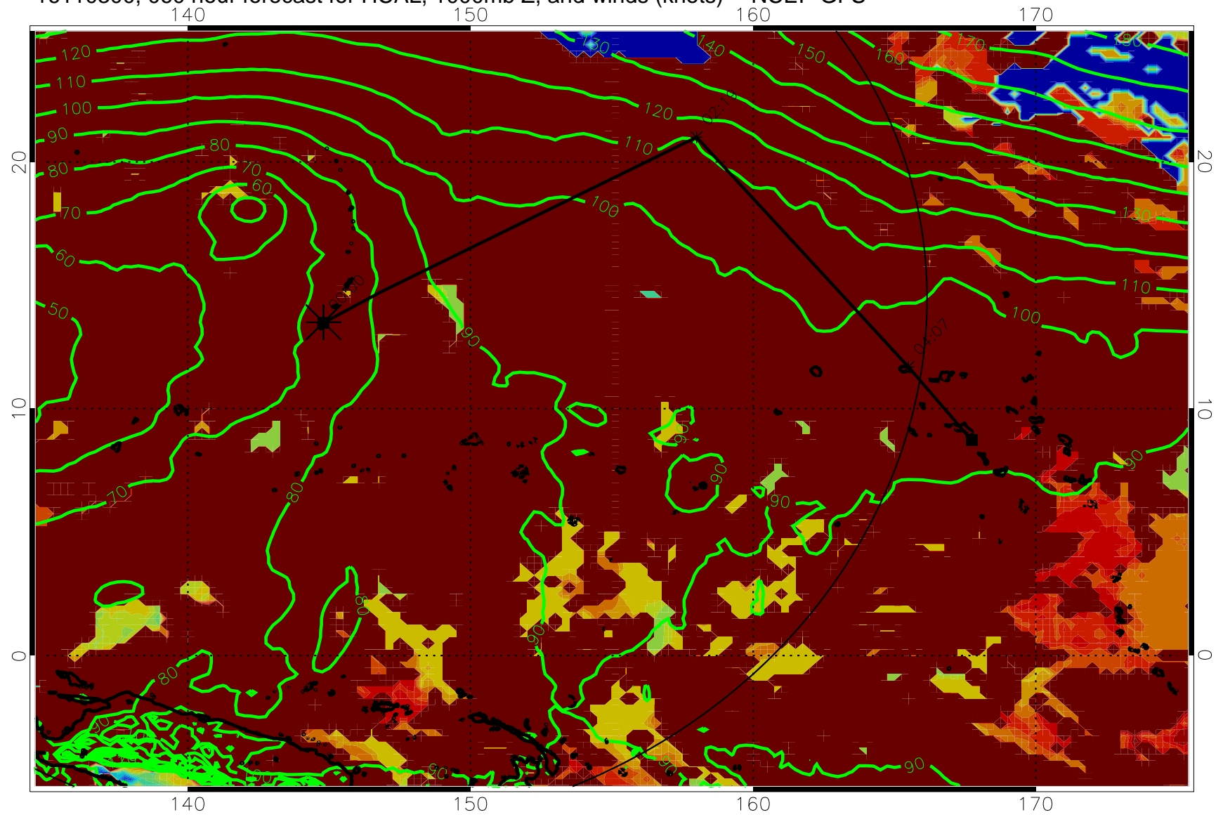
16110300, 060 hour forecast for HCAL, 1000mb Z, and winds (knots) -- NCEP GFS
