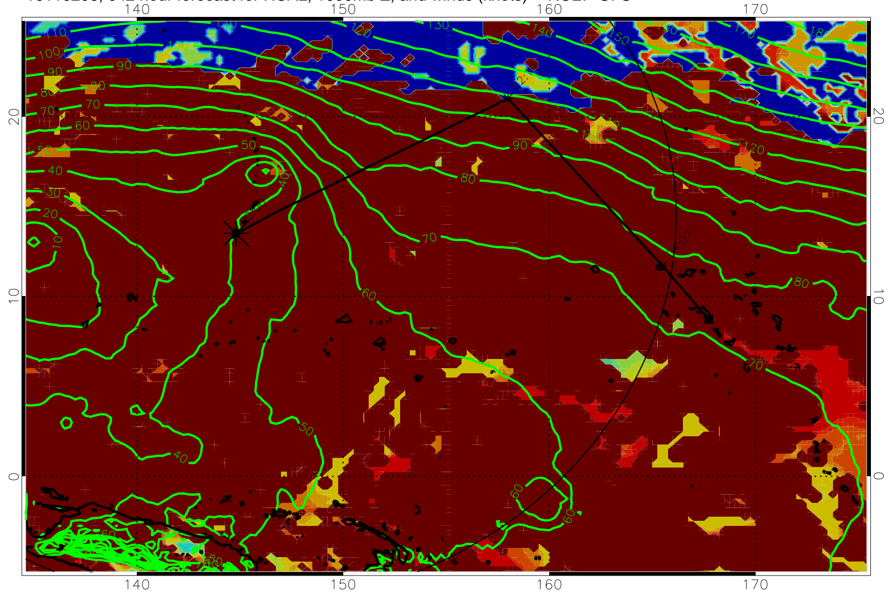
16110206, 042 hour forecast for HCAL, 1000mb Z, and winds (knots) -- NCEP GFS
