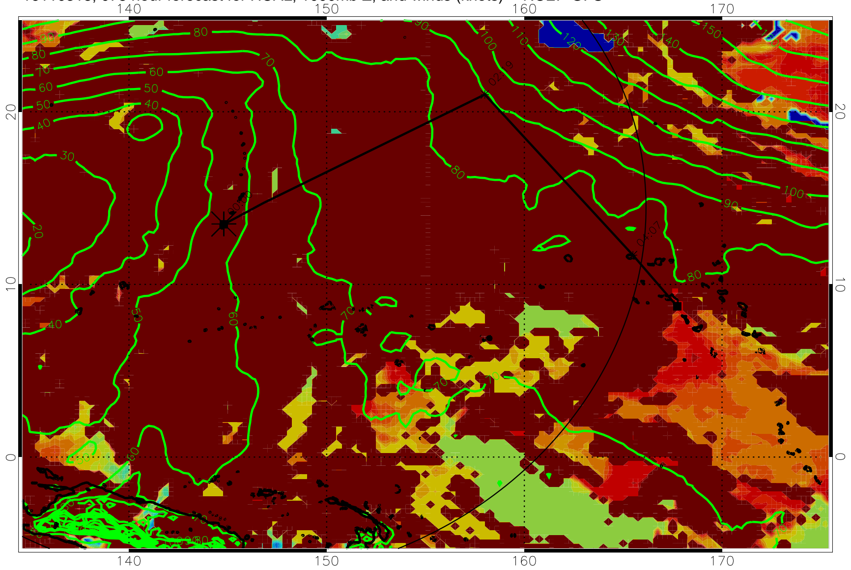
16110318, 078 hour forecast for HCAL, 1000mb Z, and winds (knots) -- NCEP GFS
