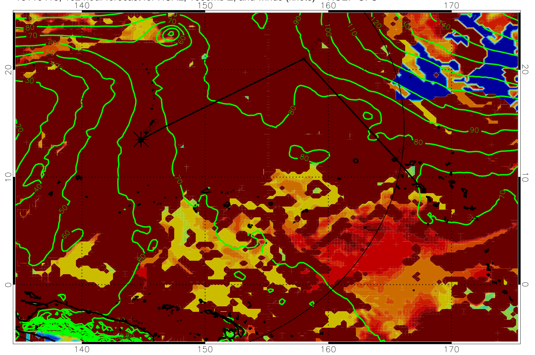
16110418, 102 hour forecast for HCAL, 1000mb Z, and winds (knots) -- NCEP GFS
