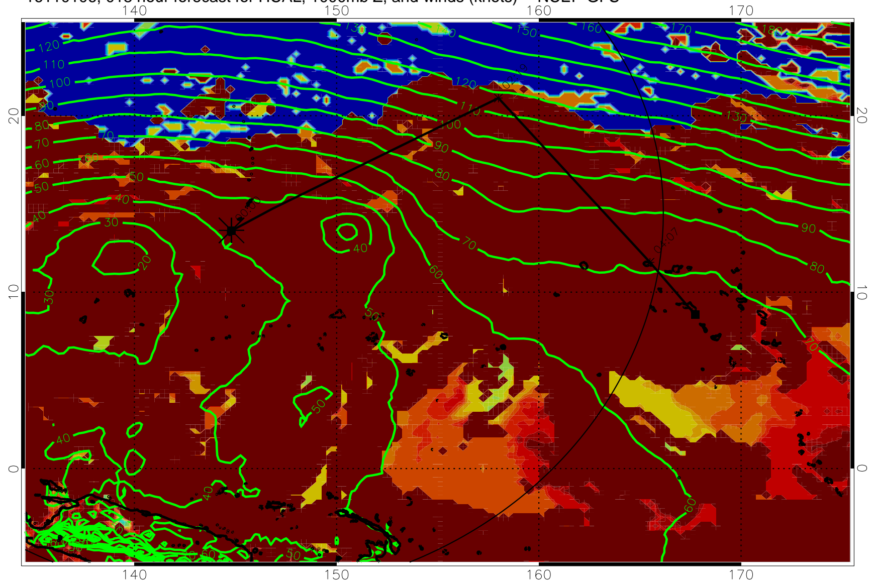
16110106, 018 hour forecast for HCAL, 1000mb Z, and winds (knots) -- NCEP GFS
