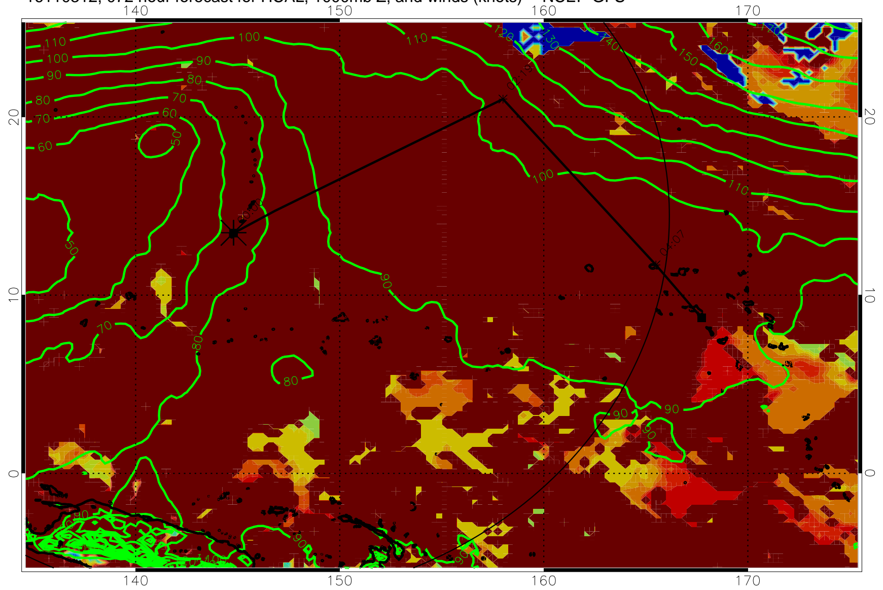
16110312, 072 hour forecast for HCAL, 1000mb Z, and winds (knots) -- NCEP GFS
