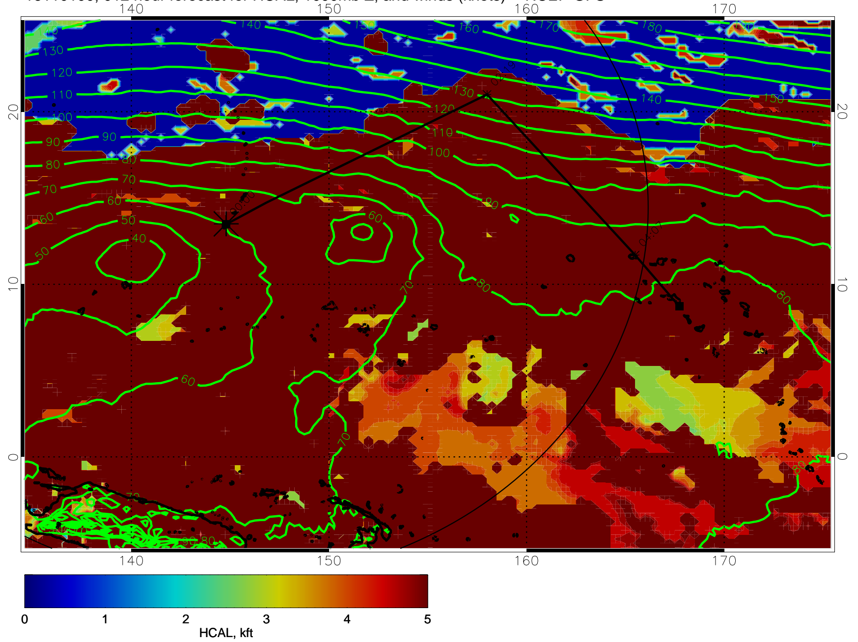
16110100, 012 hour forecast for HCAL, 1000mb Z, and winds (knots) -- NCEP GFS
