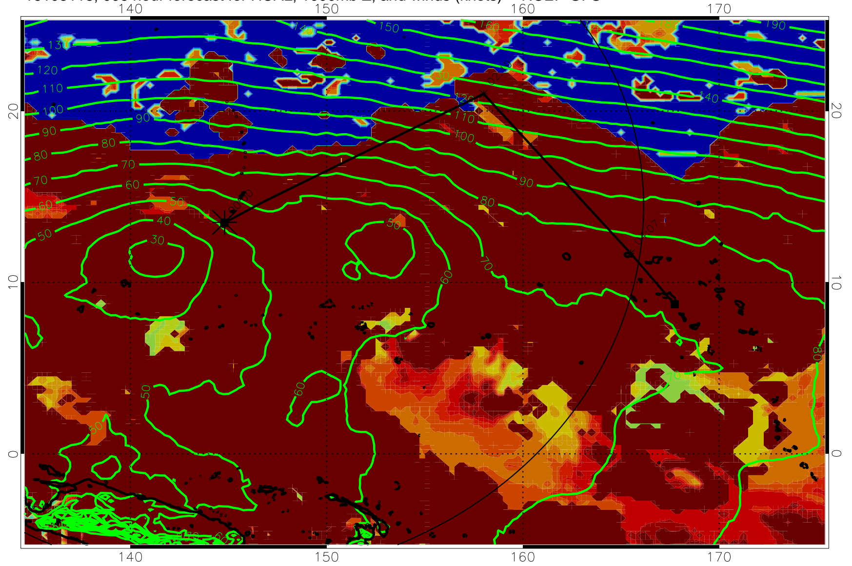
16103118, 006 hour forecast for HCAL, 1000mb Z, and winds (knots) -- NCEP GFS
