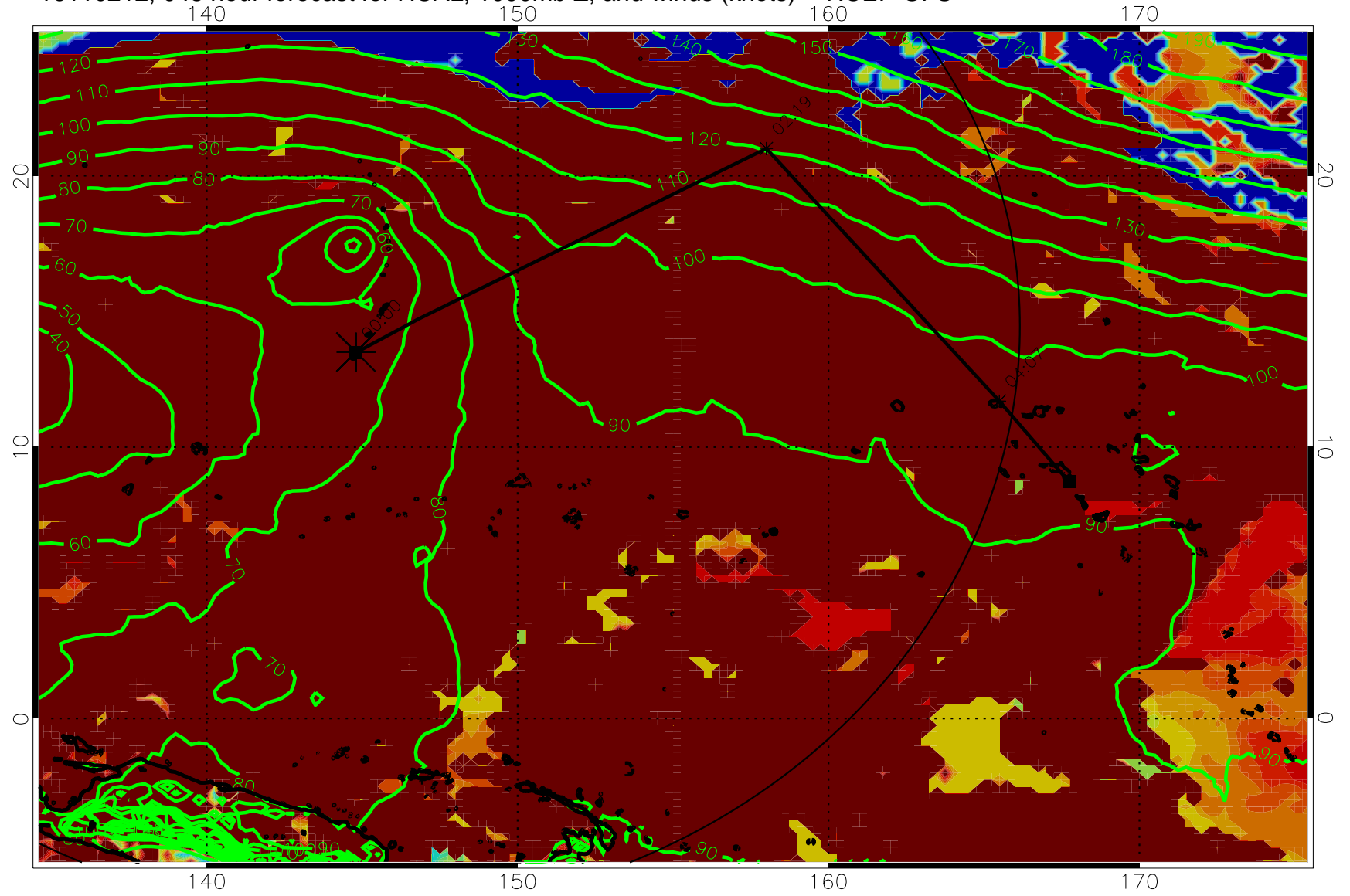
16110212, 048 hour forecast for HCAL, 1000mb Z, and winds (knots) -- NCEP GFS
