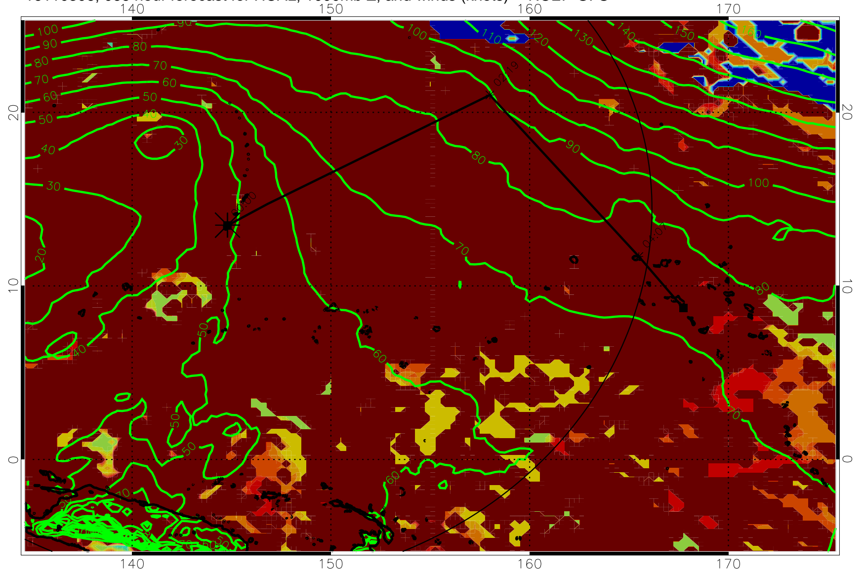
16110306, 066 hour forecast for HCAL, 1000mb Z, and winds (knots) -- NCEP GFS
