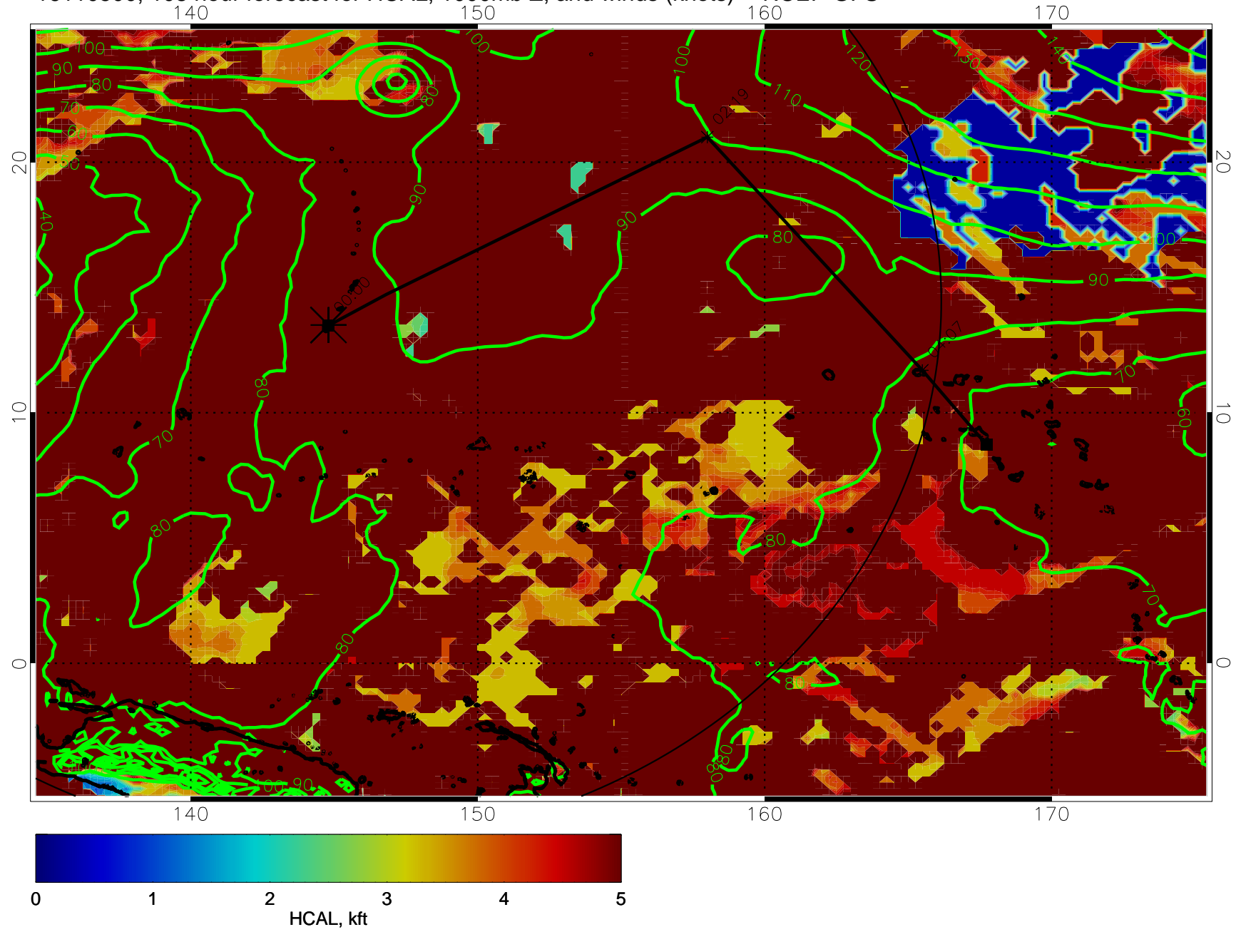
16110500, 108 hour forecast for HCAL, 1000mb Z, and winds (knots) -- NCEP GFS
