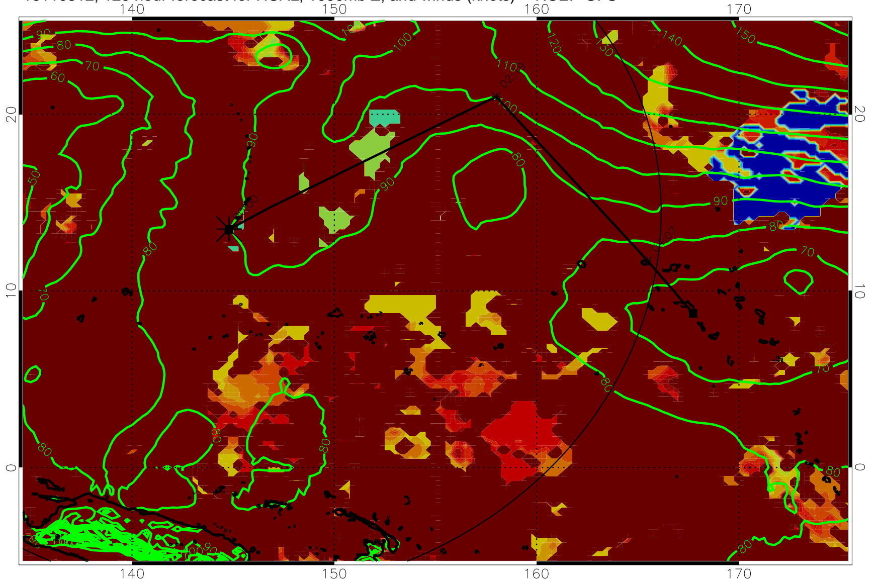
16110512, 120 hour forecast for HCAL, 1000mb Z, and winds (knots) -- NCEP GFS
