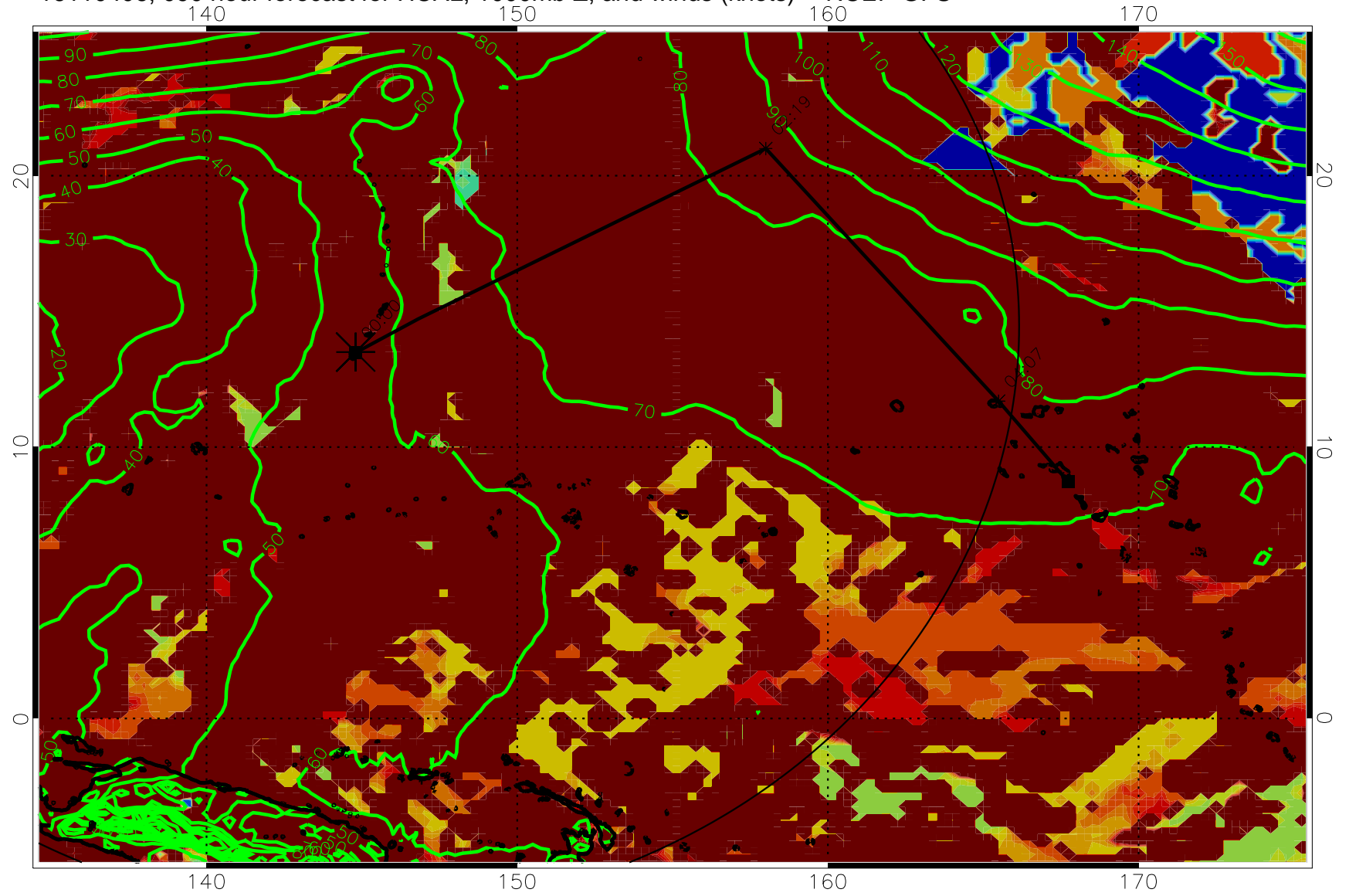
16110406, 090 hour forecast for HCAL, 1000mb Z, and winds (knots) -- NCEP GFS
