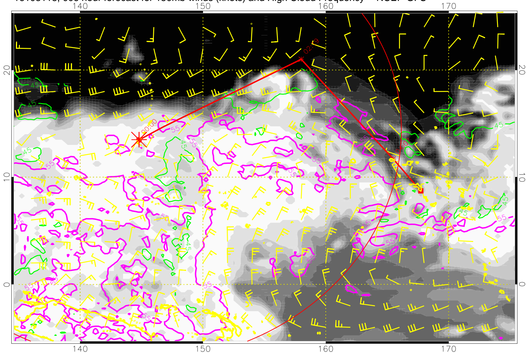
16103118, 006 hour forecast for 150mb winds (knots) and High Cloud Frequency -- NCEP GFS
