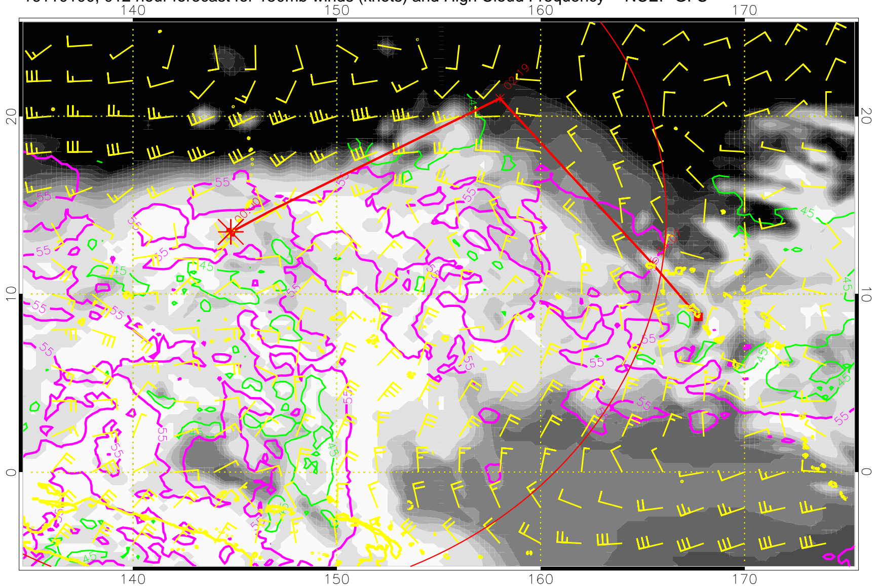
16110100, 012 hour forecast for 150mb winds (knots) and High Cloud Frequency -- NCEP GFS
