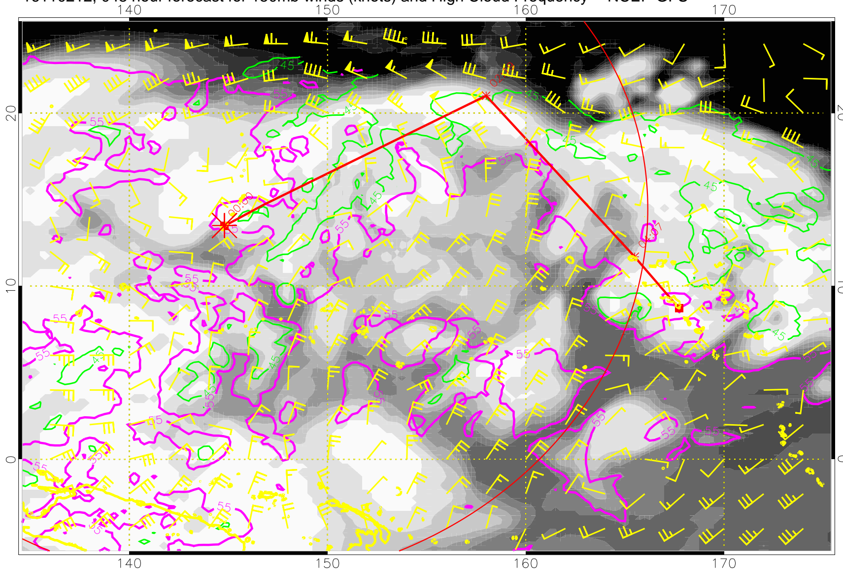
16110212, 048 hour forecast for 150mb winds (knots) and High Cloud Frequency -- NCEP GFS
