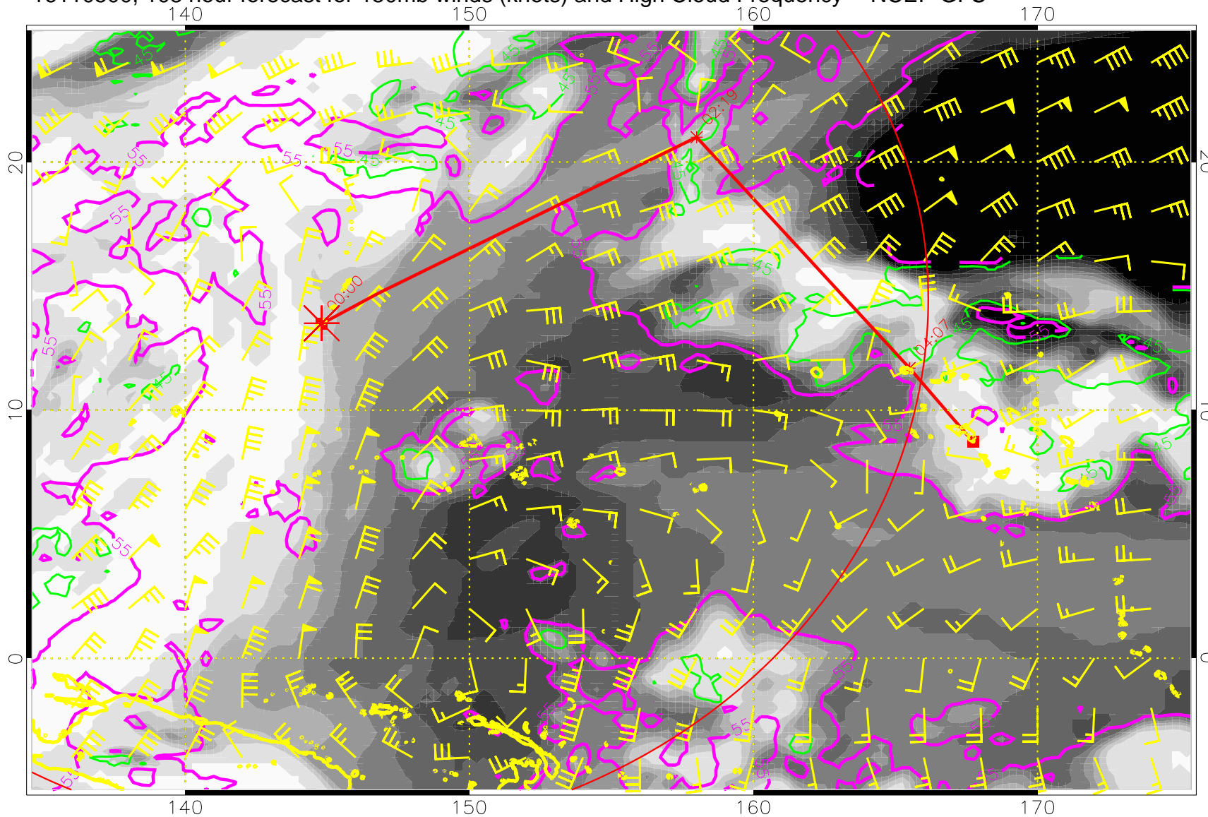
16110500, 108 hour forecast for 150mb winds (knots) and High Cloud Frequency -- NCEP GFS
