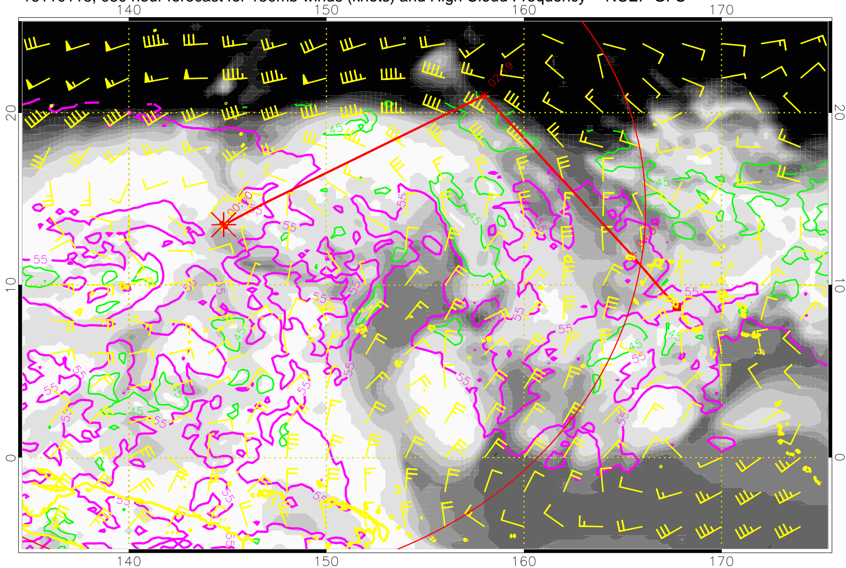
16110118, 030 hour forecast for 150mb winds (knots) and High Cloud Frequency -- NCEP GFS
