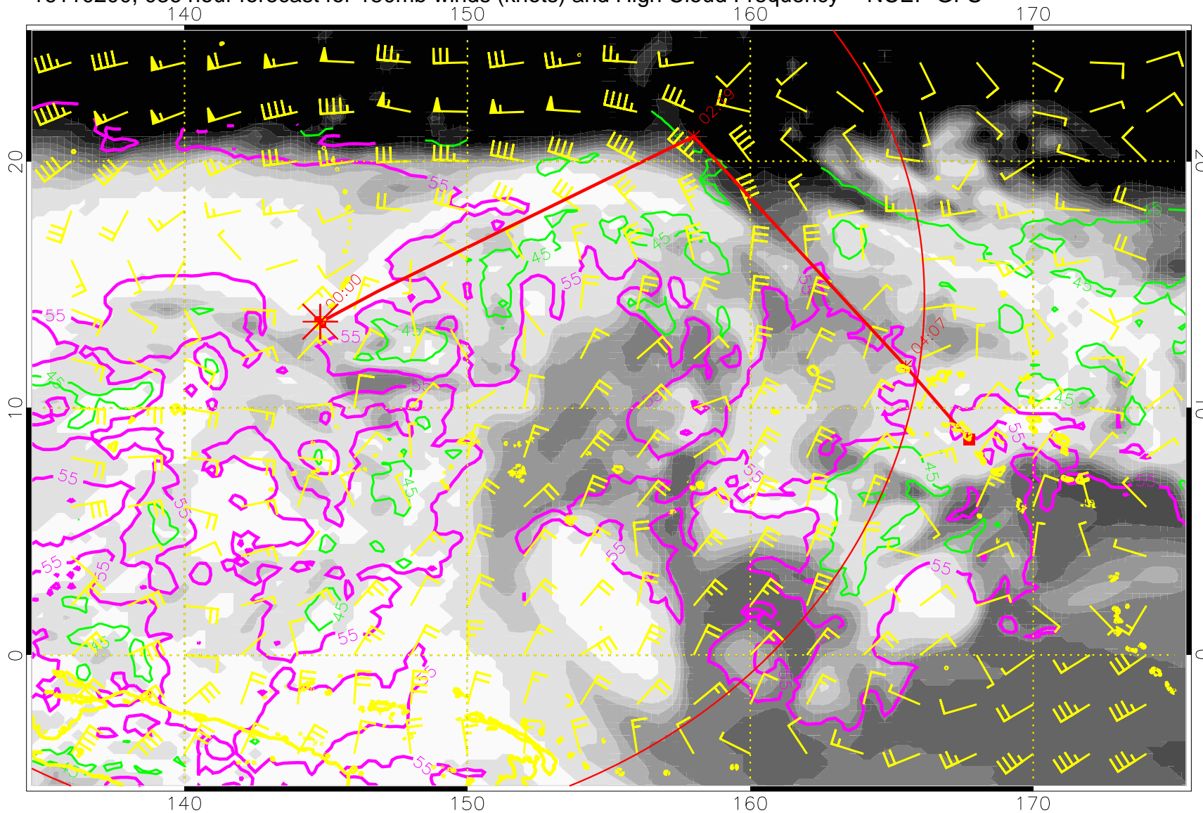
16110200, 036 hour forecast for 150mb winds (knots) and High Cloud Frequency -- NCEP GFS
