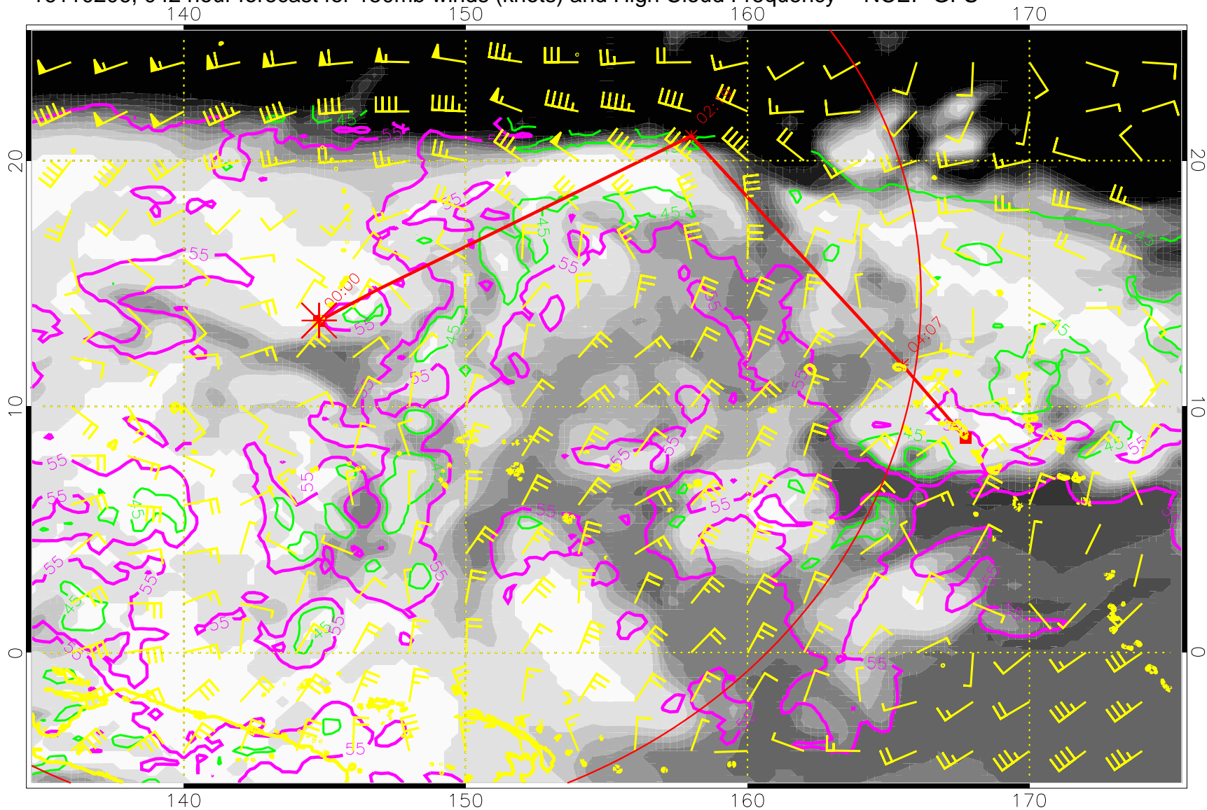
16110206, 04Z hour forecast for 150mb winds (knots) and High Cloud Frequency -- NCEP GFS
