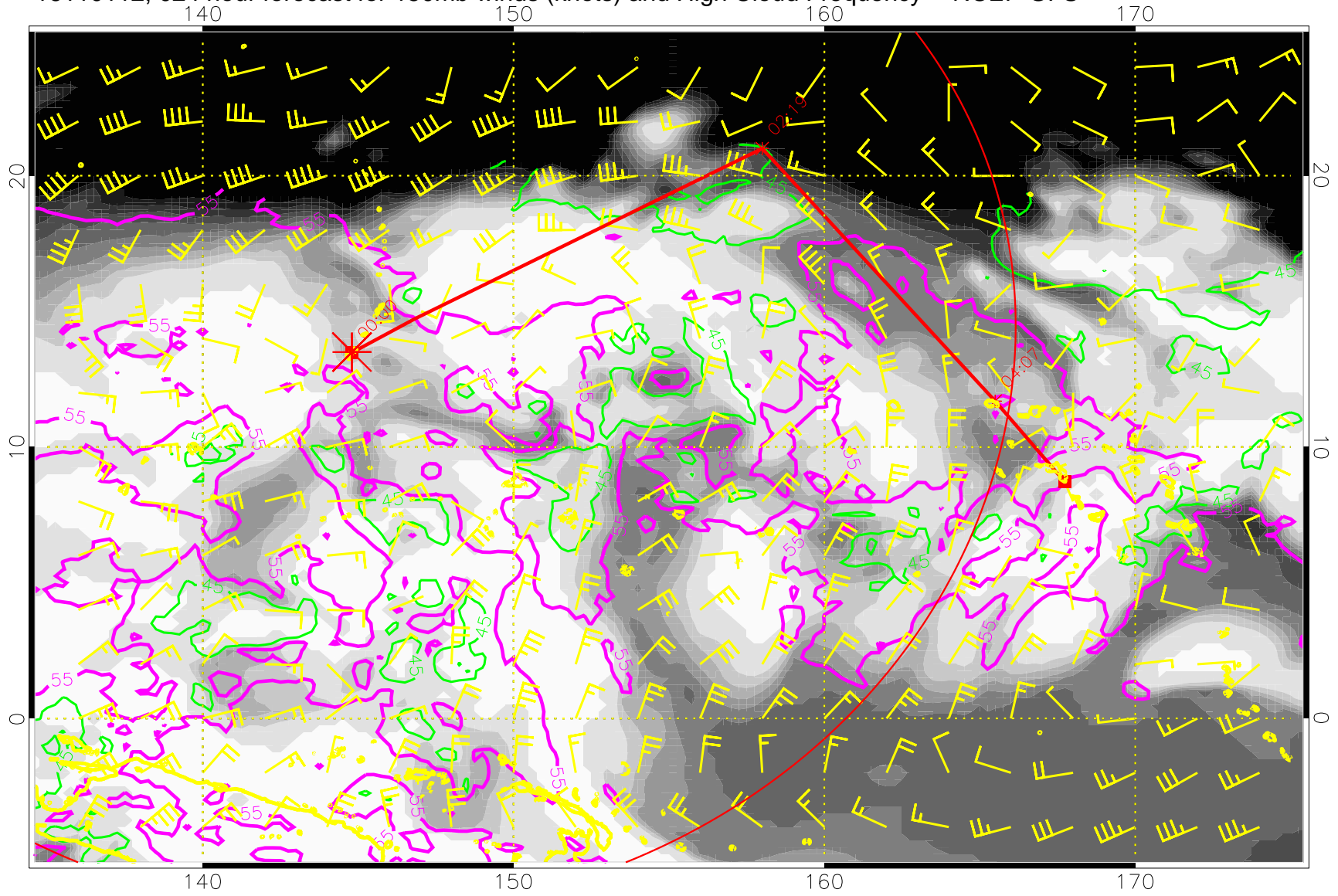
16110112, 024 hour forecast for 150mb winds (knots) and High Cloud Frequency -- NCEP GFS
