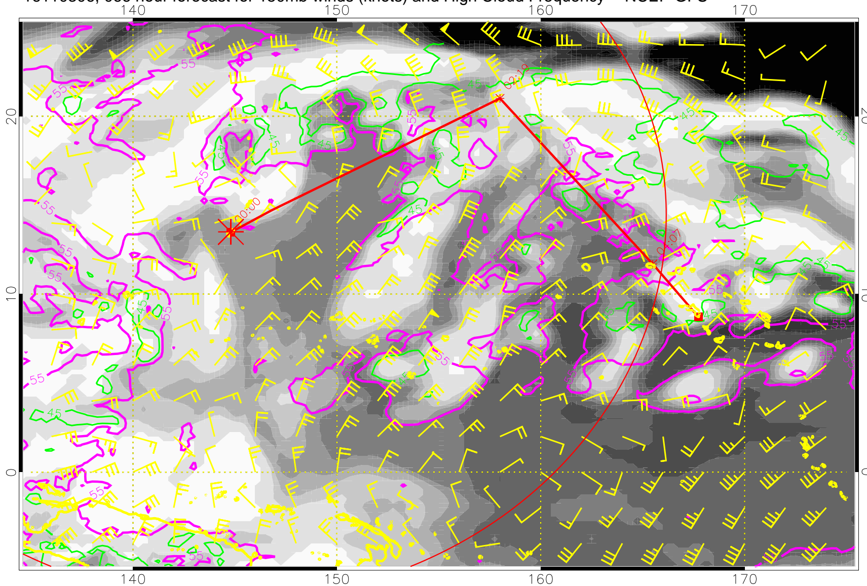
16110306, 066 hour forecast for 150mb winds (knots) and High Cloud Frequency -- NCEP GFS
