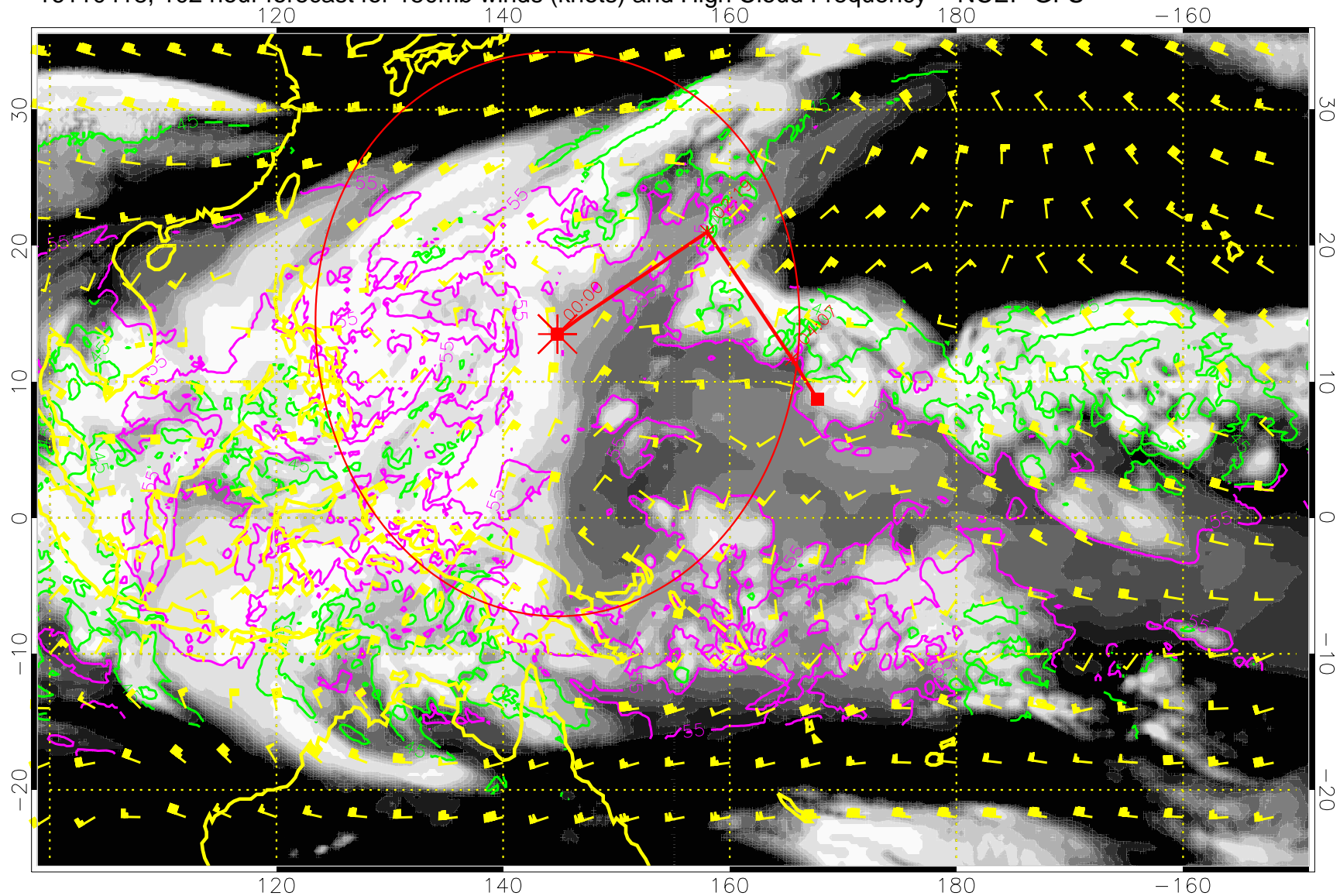
16110418, 102 hour forecast for 150mb winds (knots) and High Cloud Frequency -- NCEP GFS
