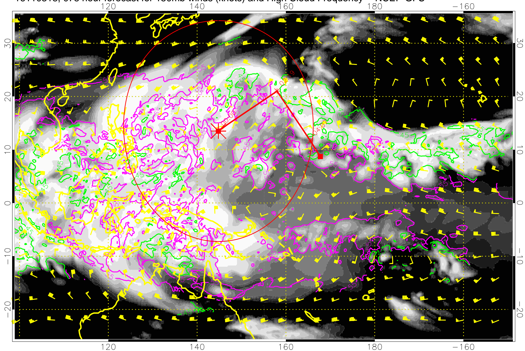
16110318, 078 hour forecast for 150mb winds (knots) and High Cloud Frequency -- NCEP GFS
