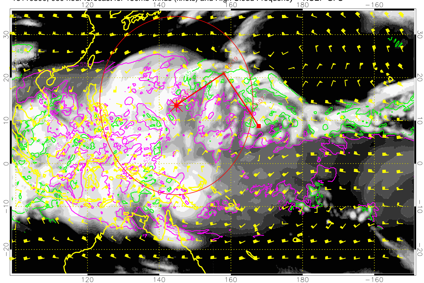
16110300, 060 hour forecast for 150mb winds (knots) and High Cloud Frequency -- NCEP GFS
