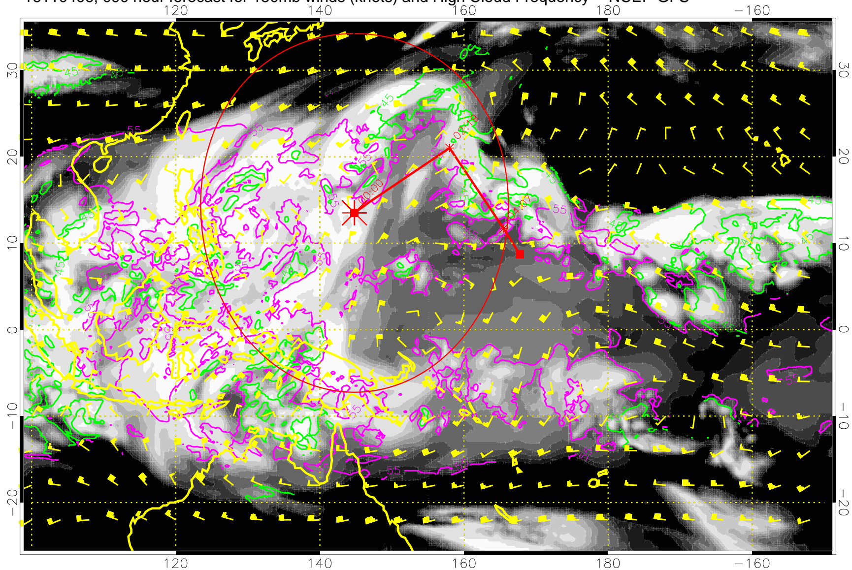
16110406, 090 hour forecast for 150mb winds (knots) and High Cloud Frequency -- NCEP GFS
