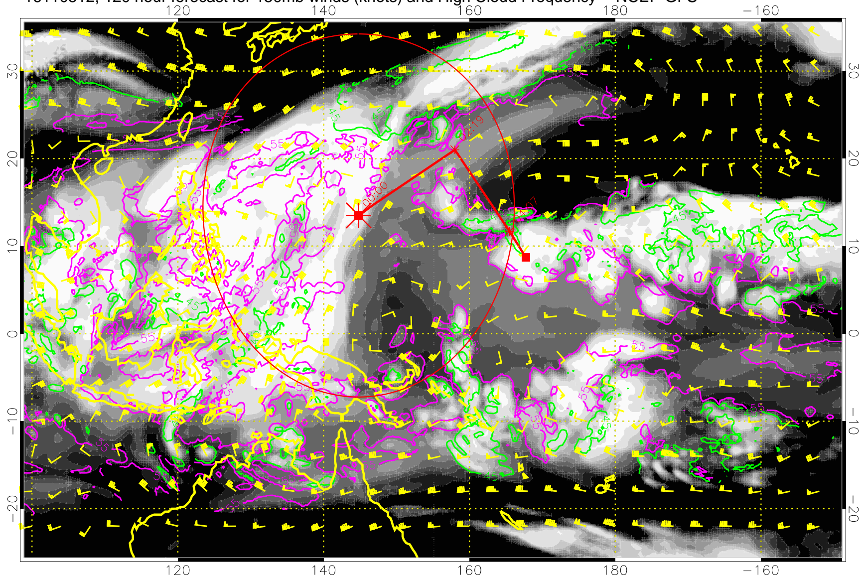
16110512, 120 hour forecast for 150mb winds (knots) and High Cloud Frequency -- NCEP GFS
