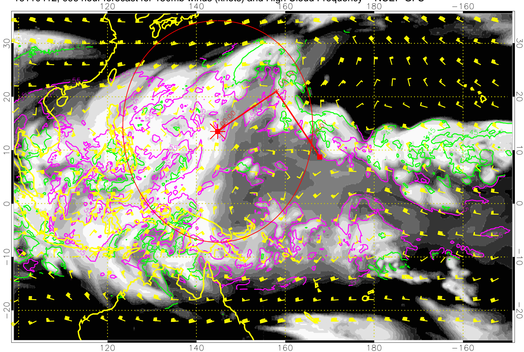
16110412, 096 hour forecast for 150mb winds (knots) and High Cloud Frequency -- NCEP GFS
