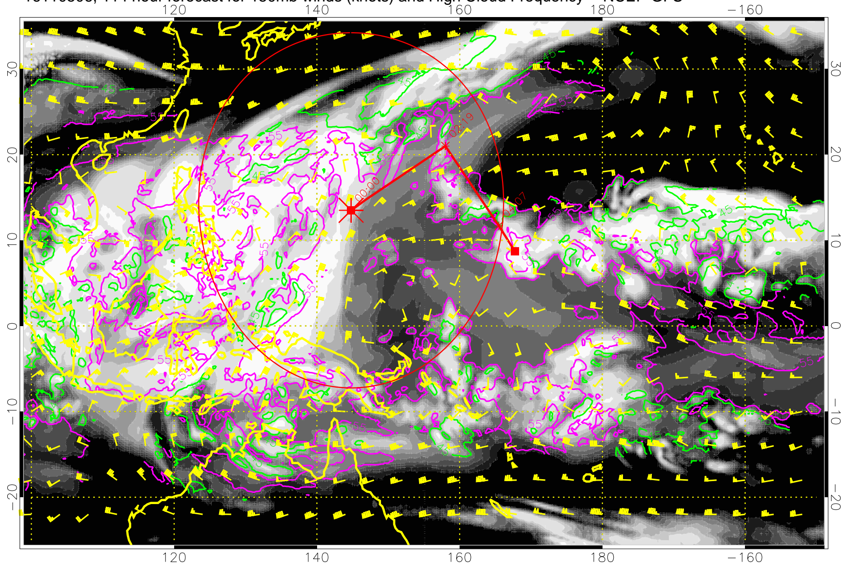
16110506, 114 hour forecast for 150mb winds (knots) and High Cloud Frequency -- NCEP GFS
