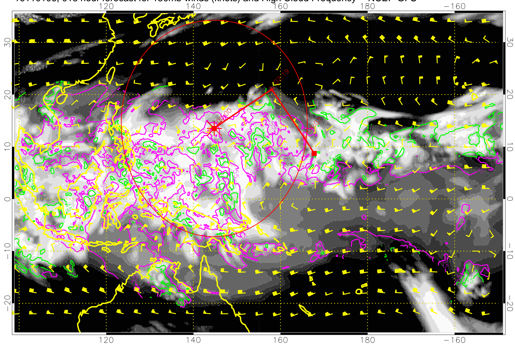
16110106, 018 hour forecast for 150mb winds (knots) and High Cloud Frequency -- NCEP GFS
