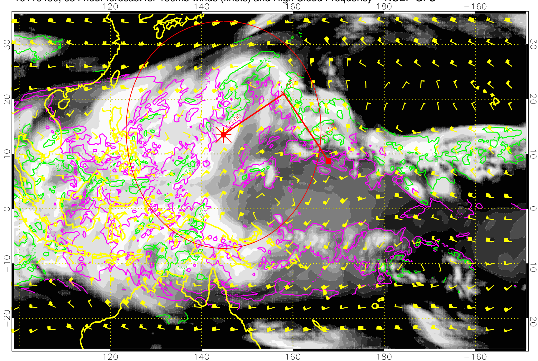
16110400, 084 hour forecast for 150mb winds (knots) and High Cloud Frequency -- NCEP GFS
