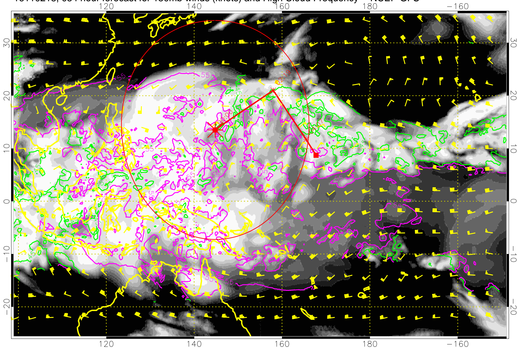
16110218, 054 hour forecast for 150mb winds (knots) and High Cloud Frequency -- NCEP GFS
