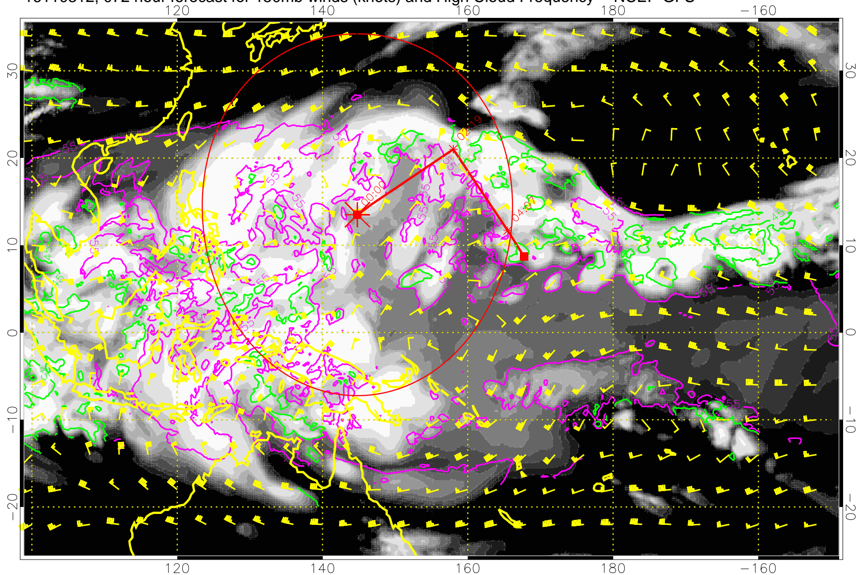
16110312, 072 hour forecast for 150mb winds (knots) and High Cloud Frequency -- NCEP GFS
