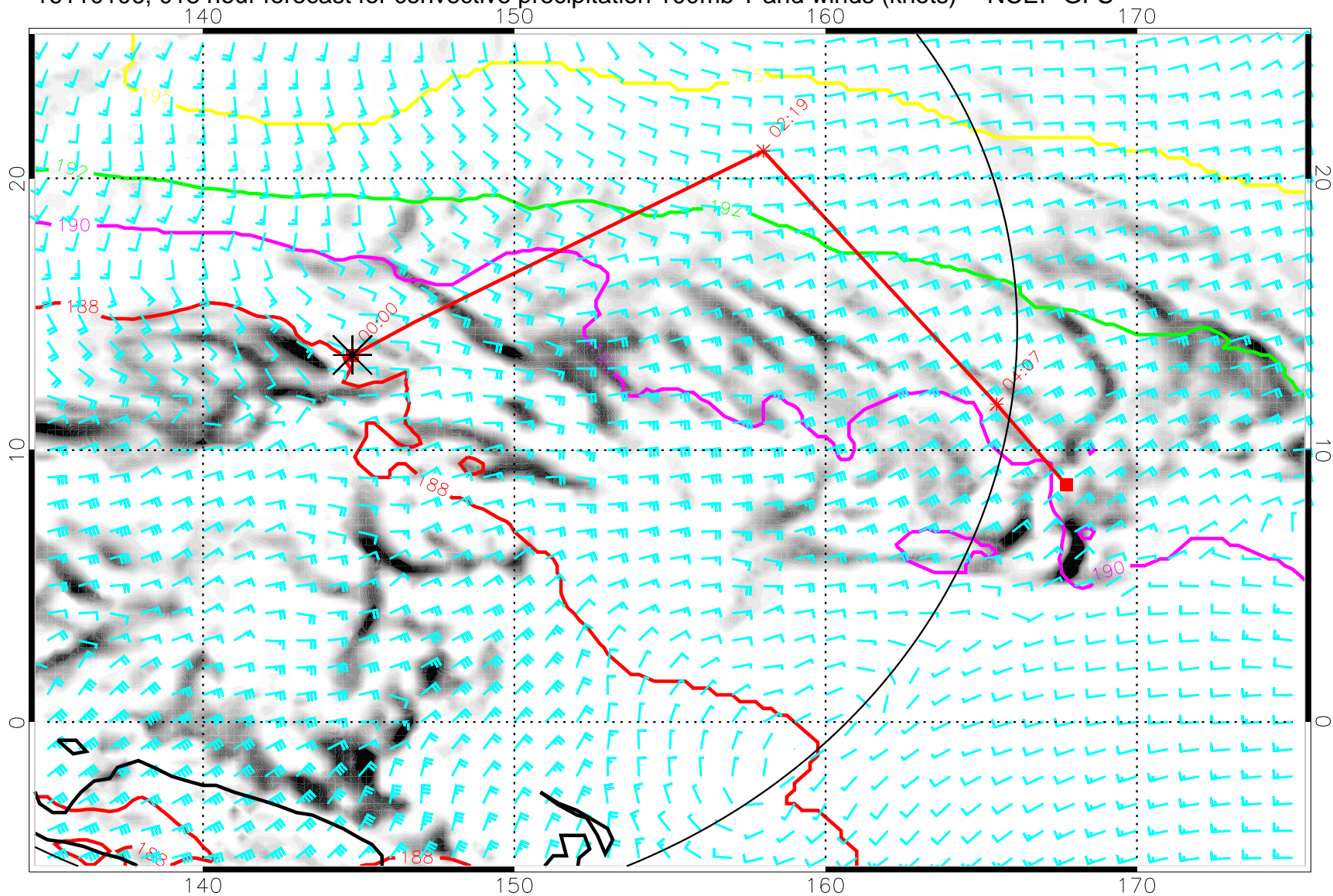
16110106, 018 hour forecast for convective precipitation 100mb T and winds (knots) -- NCEP GFS
