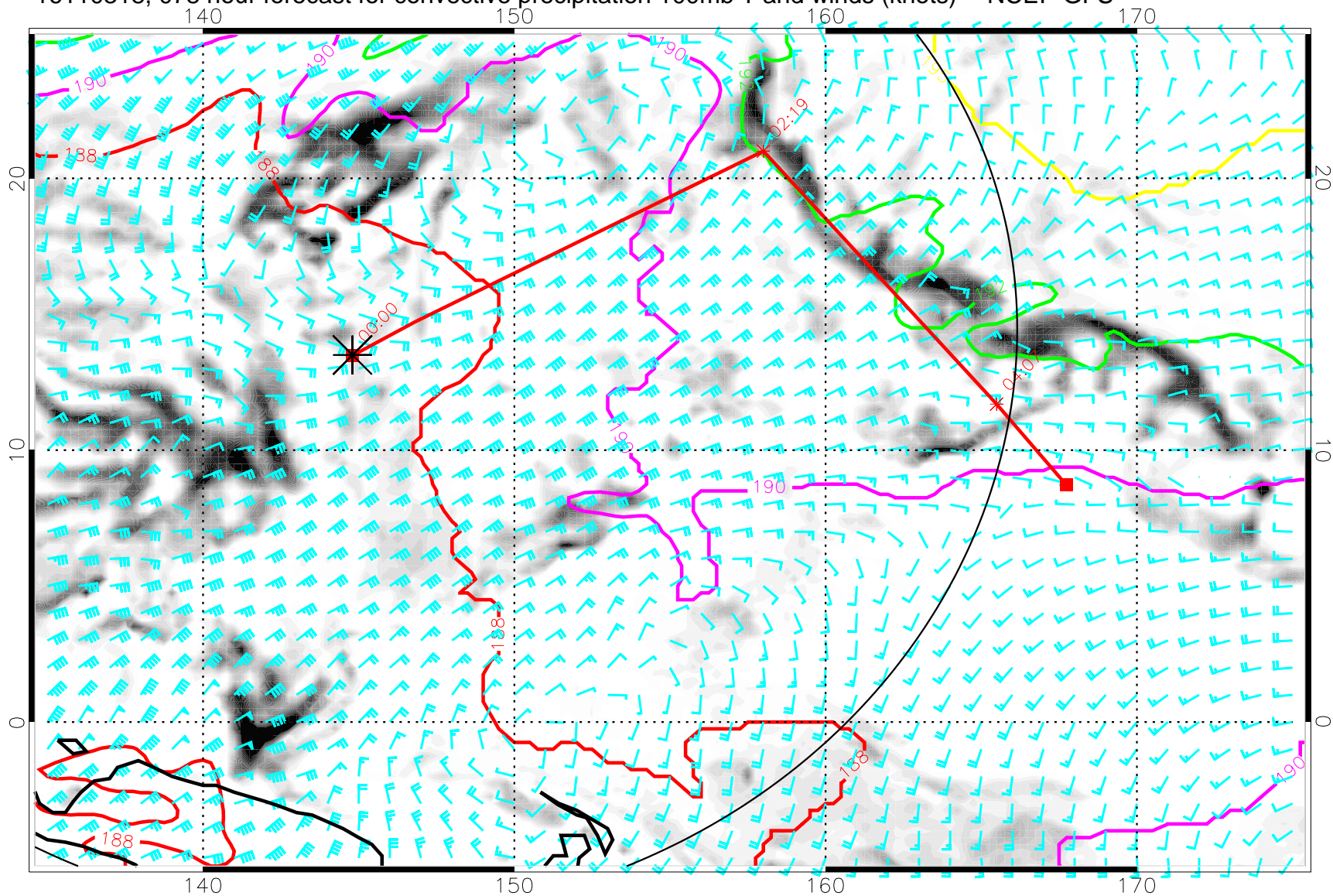
16110318, 078 hour forecast for convective precipitation 100mb T and winds (knots) -- NCEP GFS
