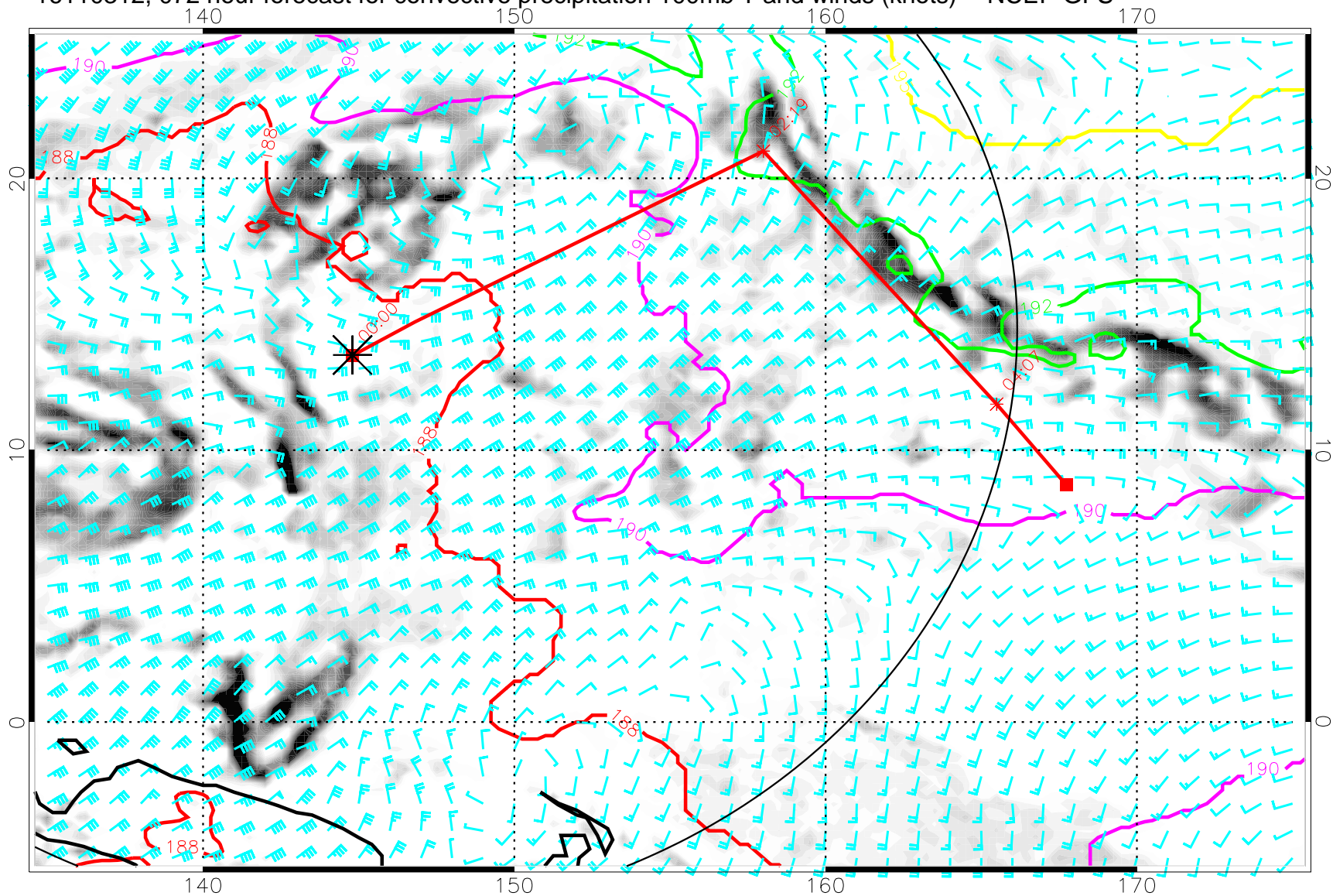
16110312, 072 hour forecast for convective precipitation 100mb T and winds (knots) -- NCEP GFS
