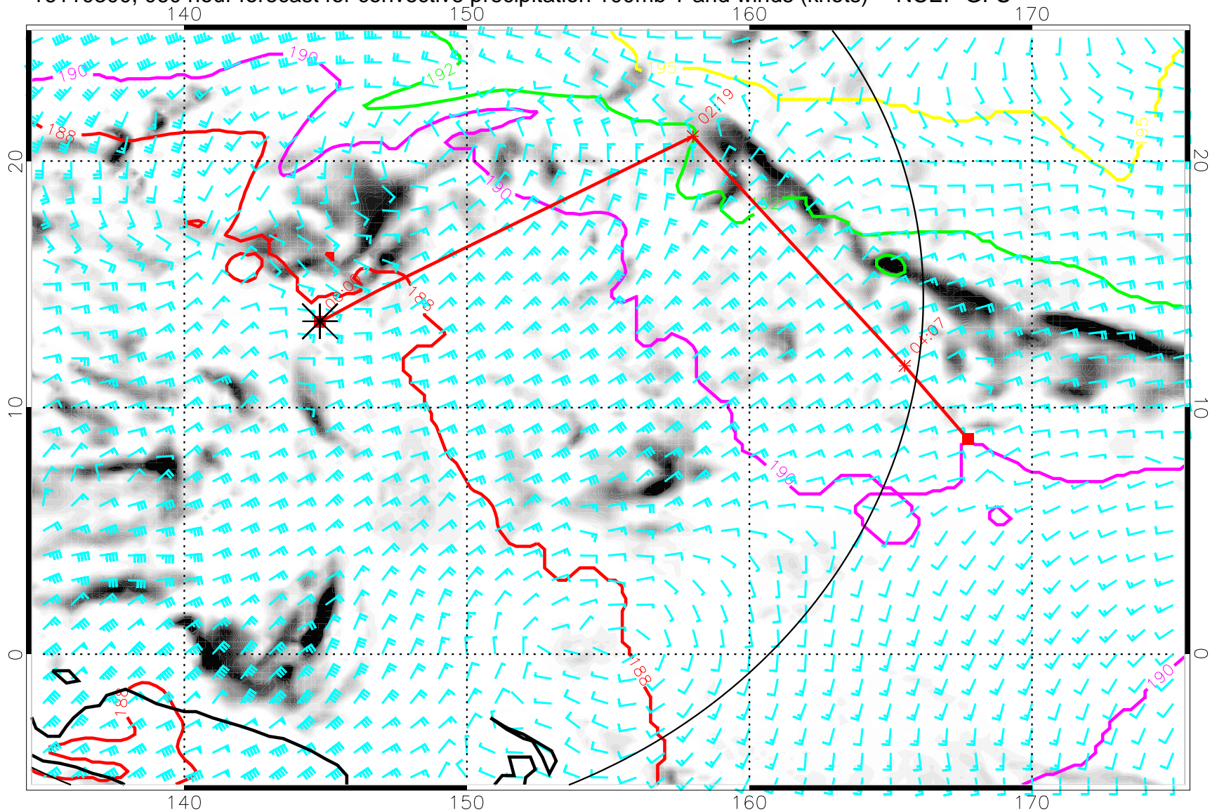
16110300, 060 hour forecast for convective precipitation 100mb T and winds (knots) -- NCEP GFS
