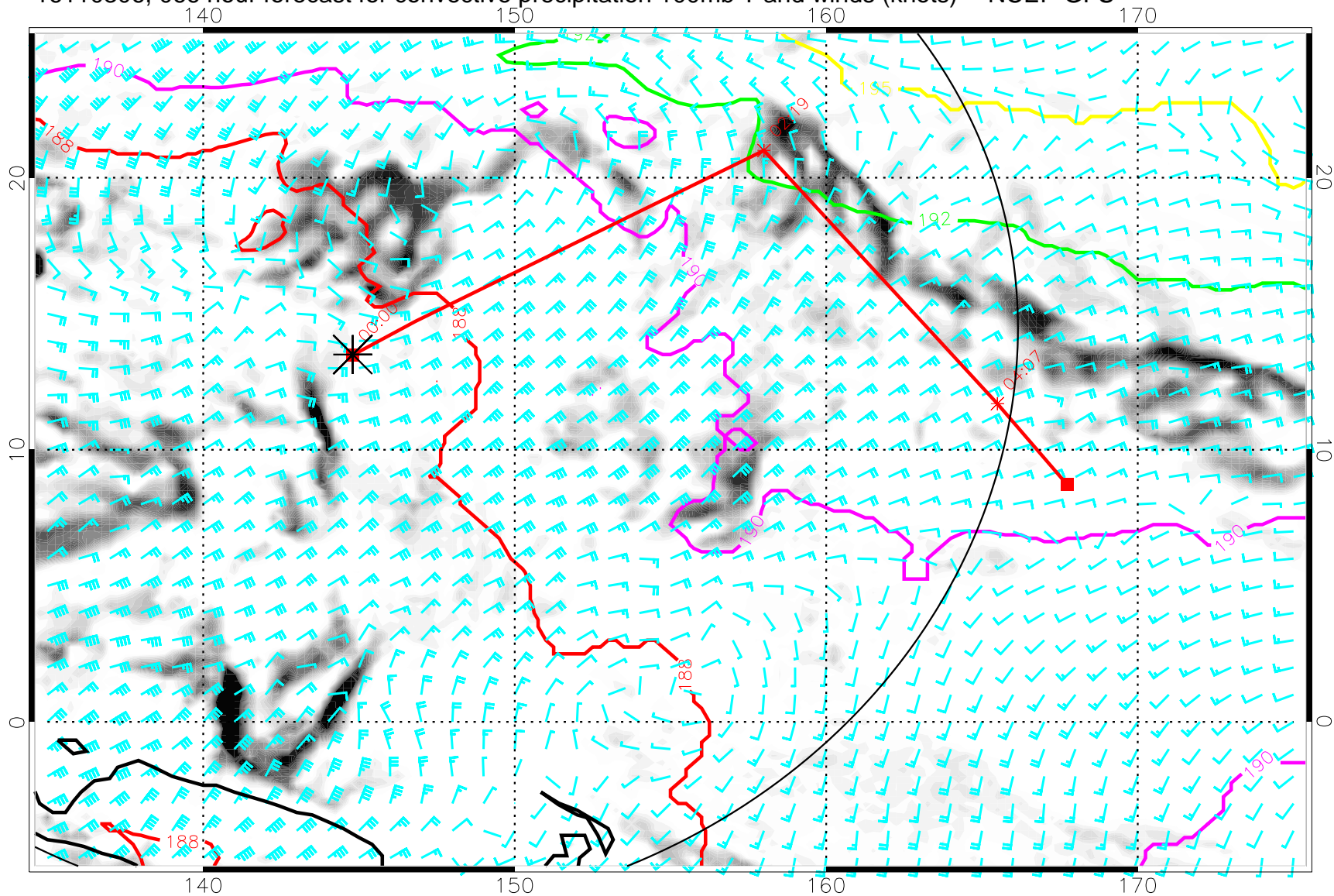
16110306, 066 hour forecast for convective precipitation 100mb T and winds (knots) -- NCEP GFS
