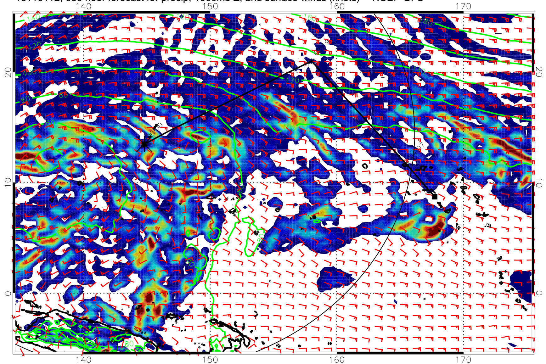
16110112, 030 hour forecast for precip, 1000mb Z, and surface winds (knots) -- NCEP GFS
