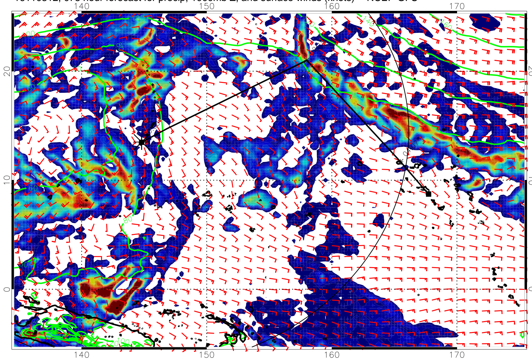
16110312, 078 hour forecast for precip, 1000mb Z, and surface winds (knots) -- NCEP GFS
