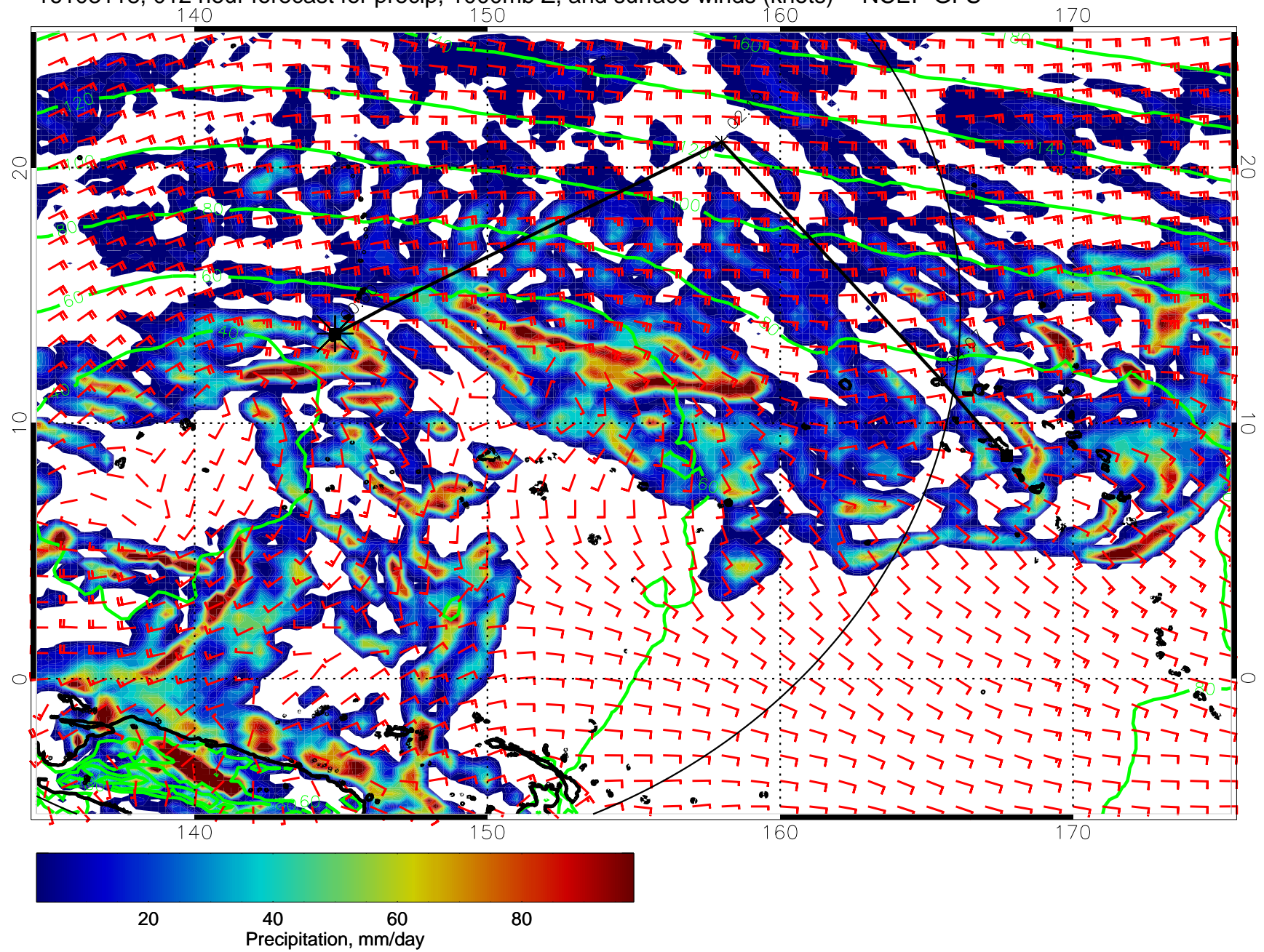
16103118, 012 hour forecast for precip, 1000mb Z, and surface winds (knots) -- NCEP GFS
