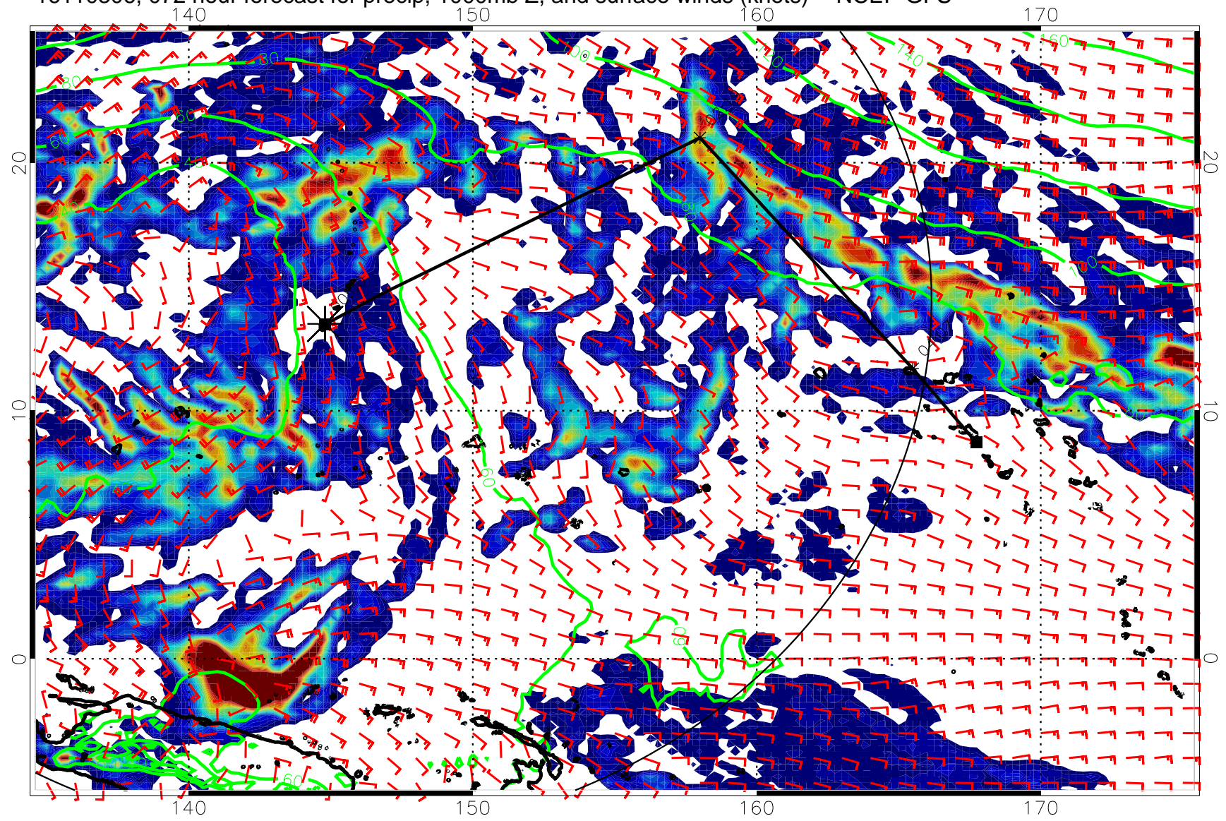
16110306, 072 hour forecast for precip, 1000mb Z, and surface winds (knots) -- NCEP GFS
