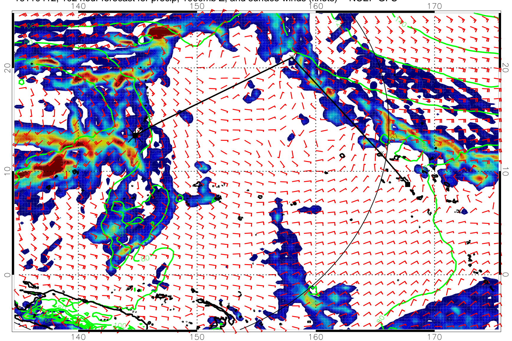
16110412, 102 hour forecast for precip, 1000mb Z, and surface winds (knots) -- NCEP GFS
