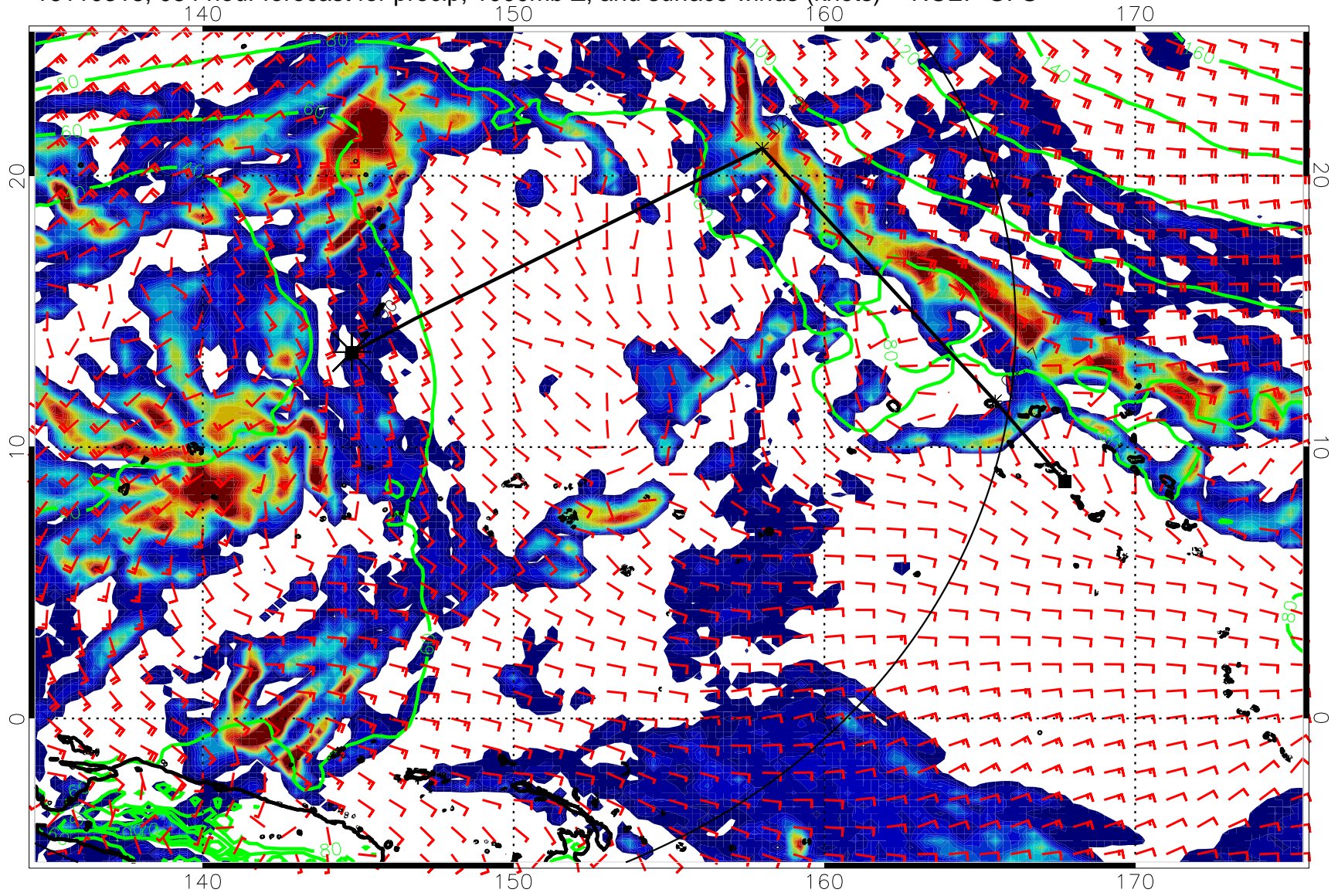
16110318, 084 hour forecast for precip, 1000mb Z, and surface winds (knots) -- NCEP GFS
