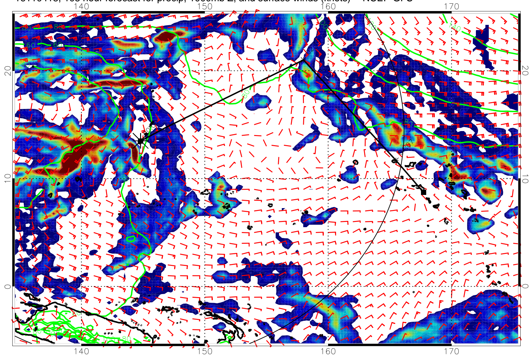
16110418, 108 hour forecast for precip, 1000mb Z, and surface winds (knots) -- NCEP GFS
