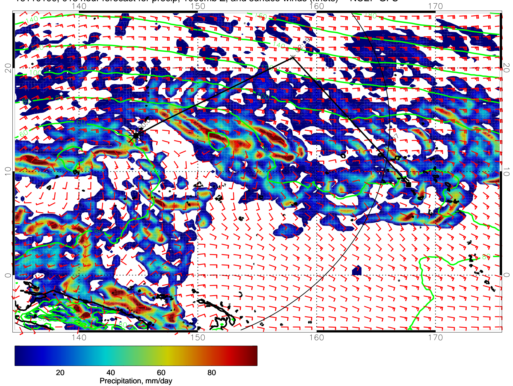
16110100, 018 hour forecast for precip, 1000mb Z, and surface winds (knots) -- NCEP GFS
