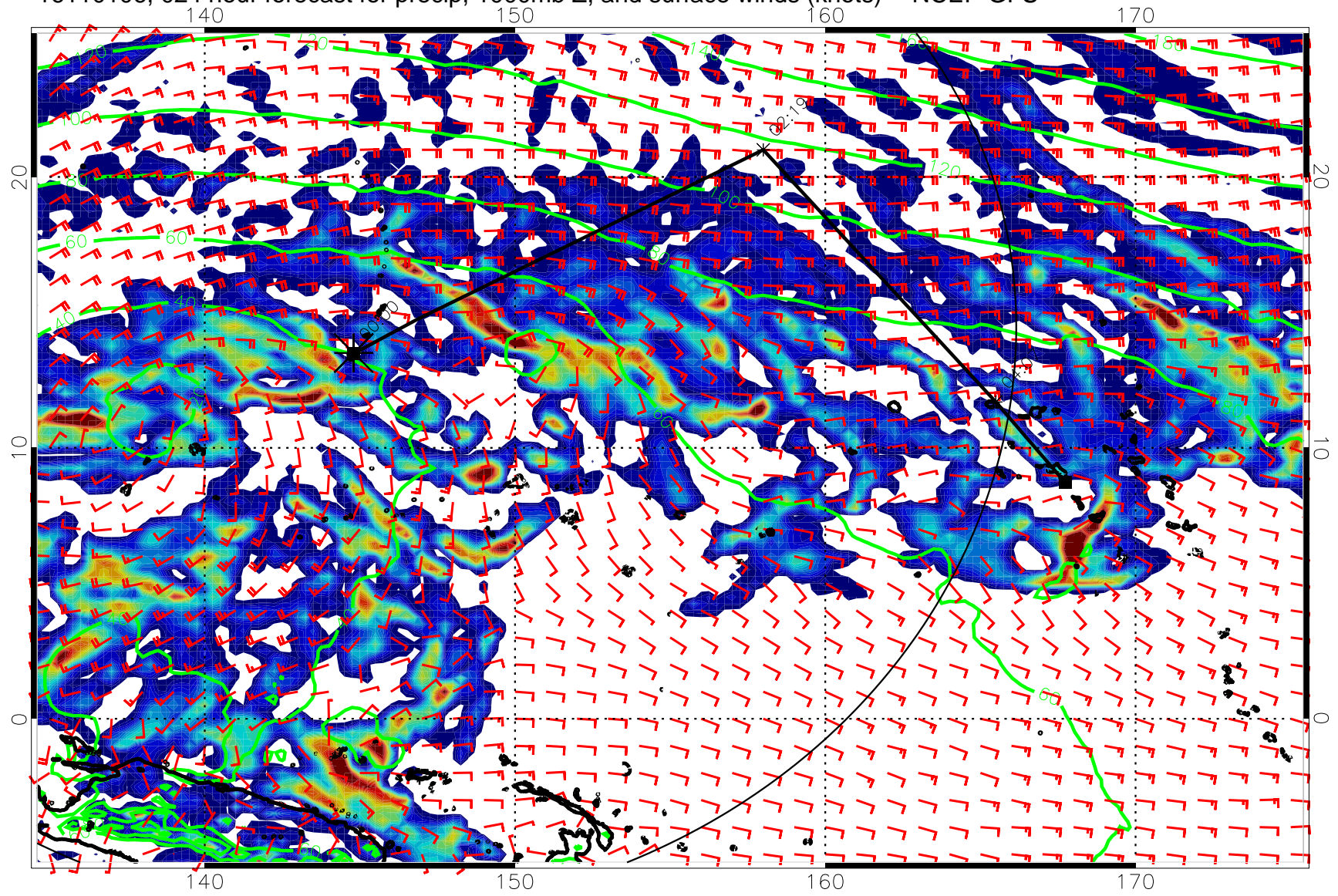
16110106, 024 hour forecast for precip, 1000mb Z, and surface winds (knots) -- NCEP GFS
