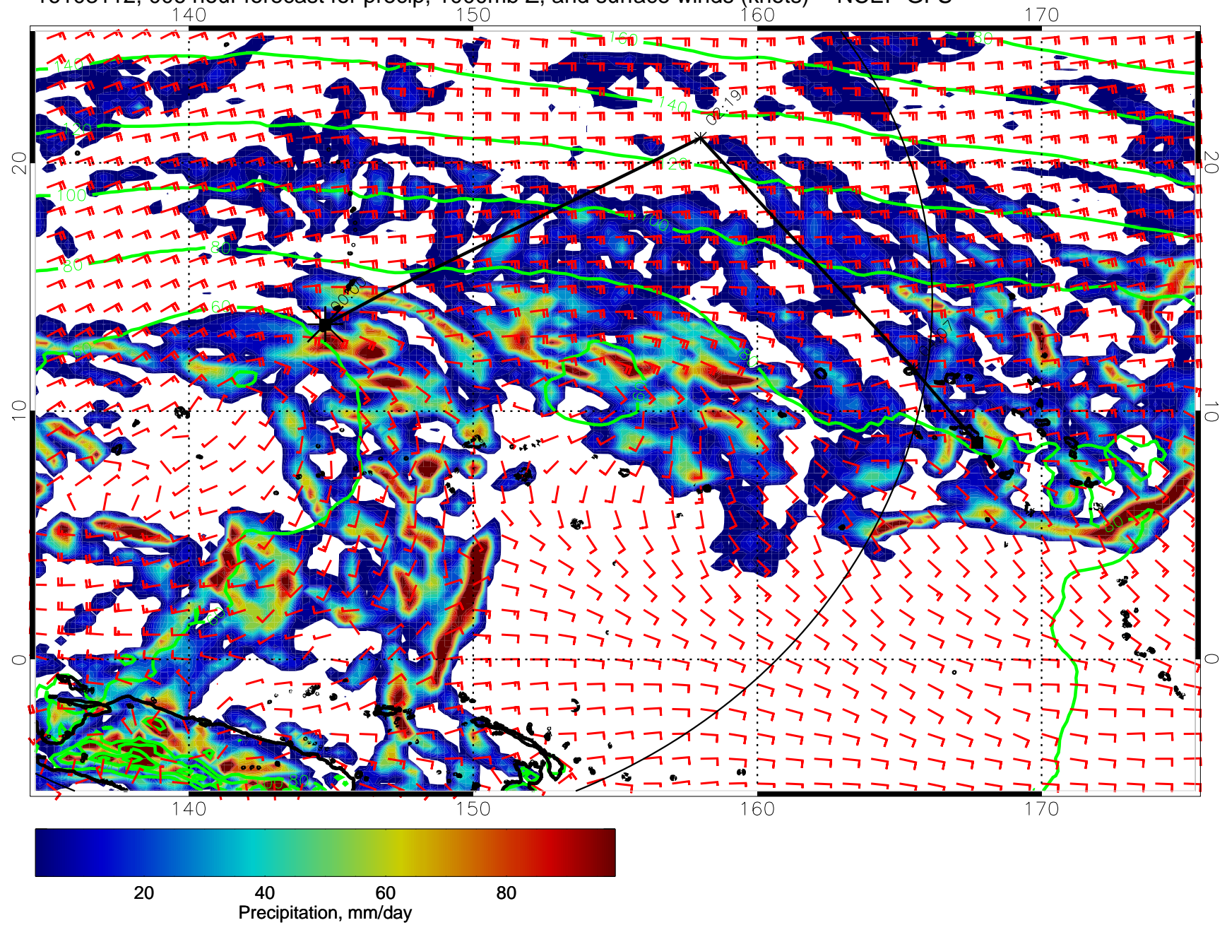
16103112, 006 hour forecast for precip, 1000mb Z, and surface winds (knots) -- NCEP GFS
