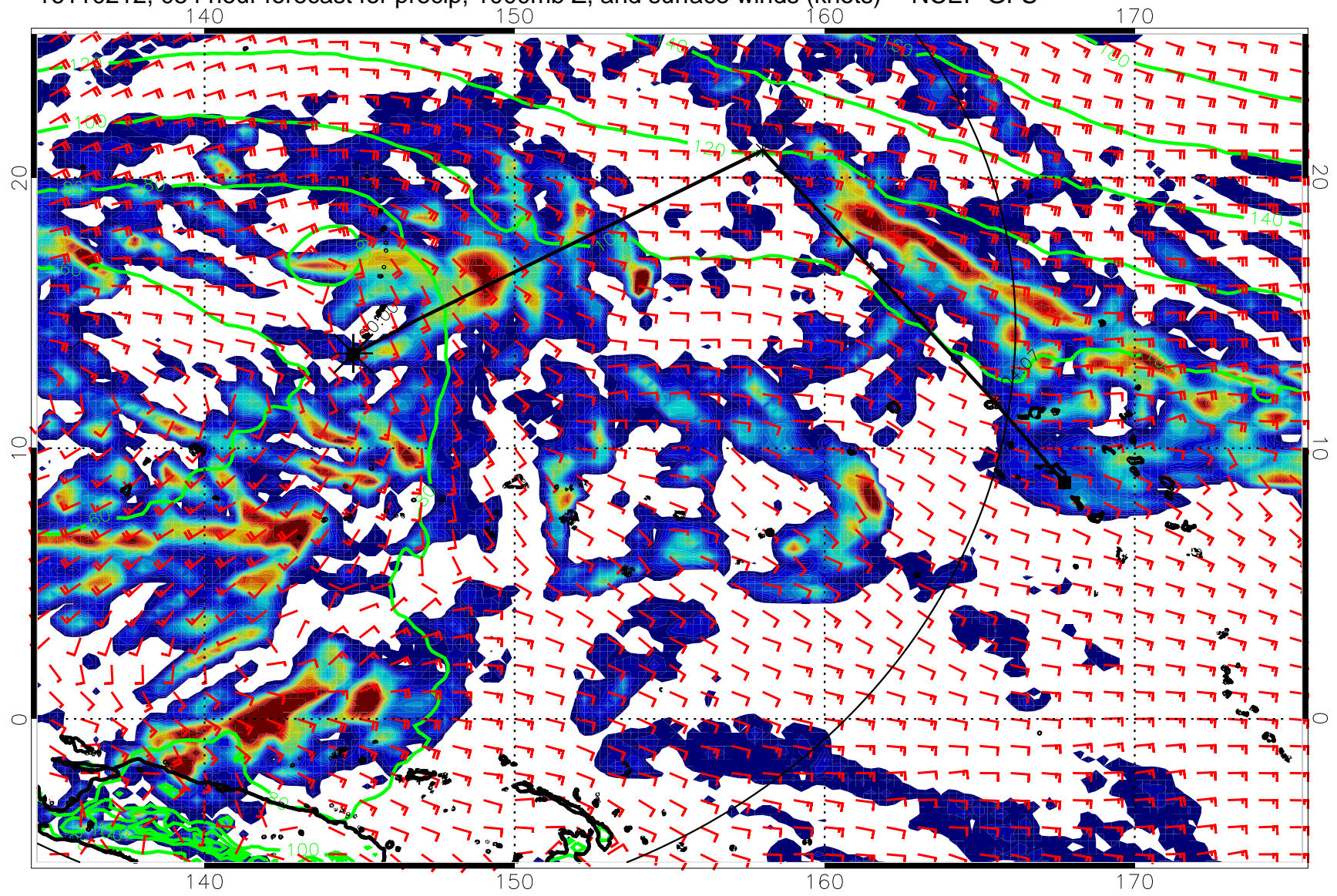
16110212, 054 hour forecast for precip, 1000mb Z, and surface winds (knots) -- NCEP GFS
