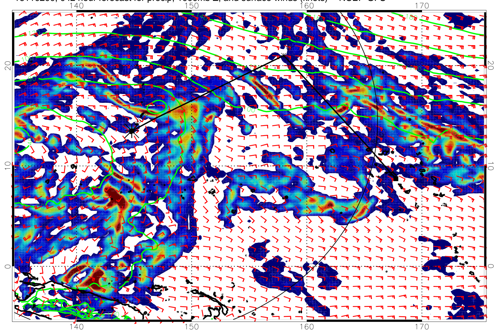
16110200, 042 hour forecast for precip, 1000mb Z, and surface winds (knots) -- NCEP GFS
