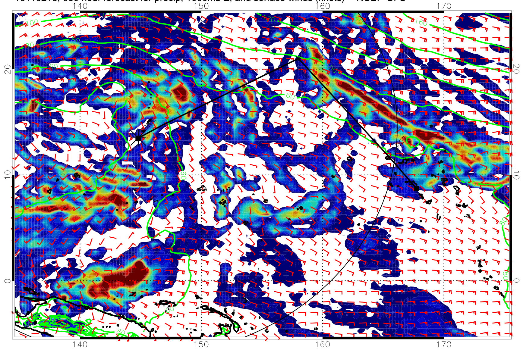
16110218, 060 hour forecast for precip, 1000mb Z, and surface winds (knots) -- NCEP GFS
