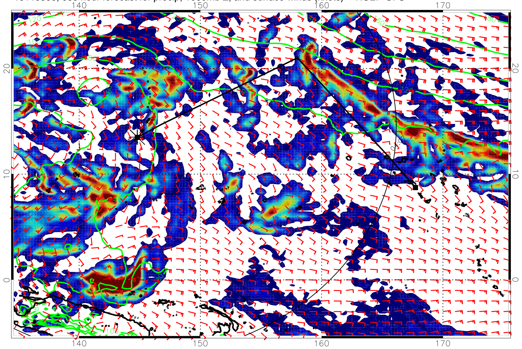
16110300, 066 hour forecast for precip, 1000mb Z, and surface winds (knots) -- NCEP GFS
