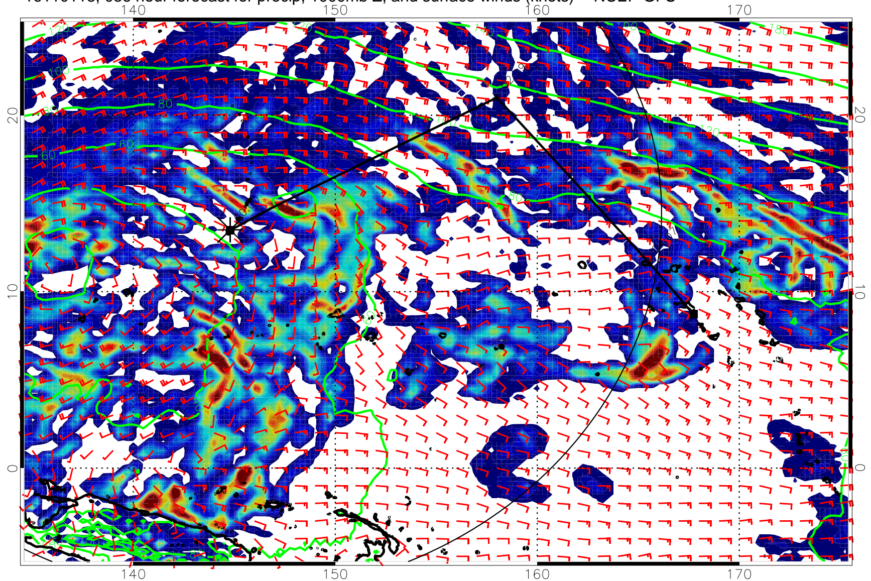
16110118, 036 hour forecast for precip, 1000mb Z, and surface winds (knots) -- NCEP GFS
