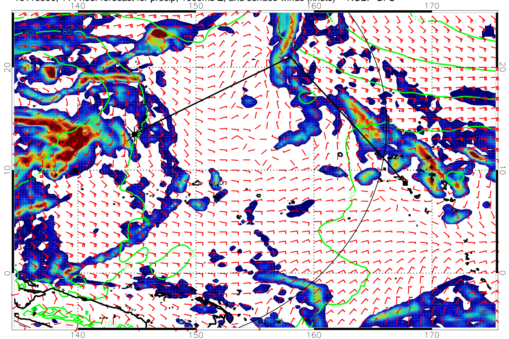
16110500, 114 hour forecast for precip, 1000mb Z, and surface winds (knots) -- NCEP GFS
