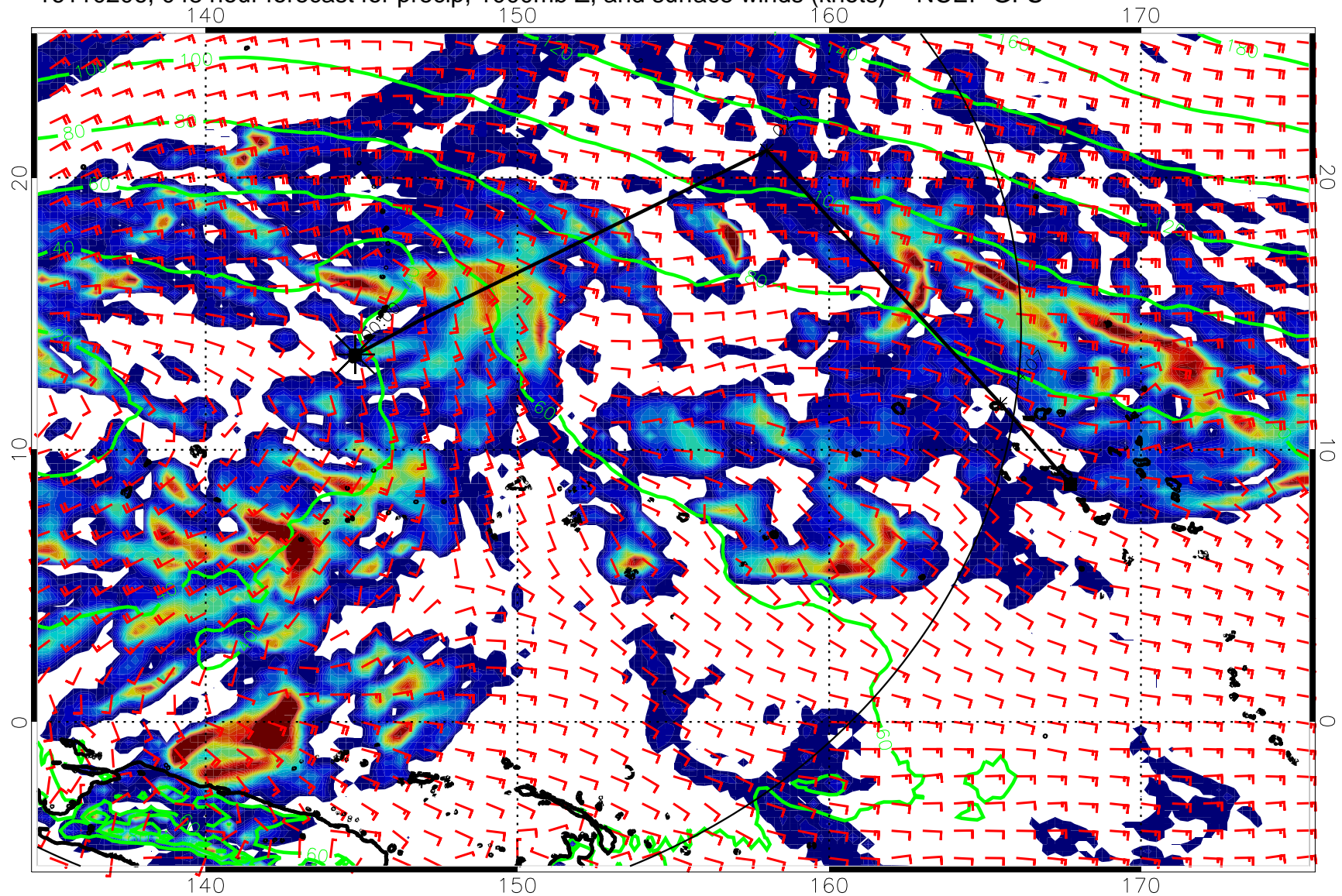
16110206, 048 hour forecast for precip, 1000mb Z, and surface winds (knots) -- NCEP GFS
