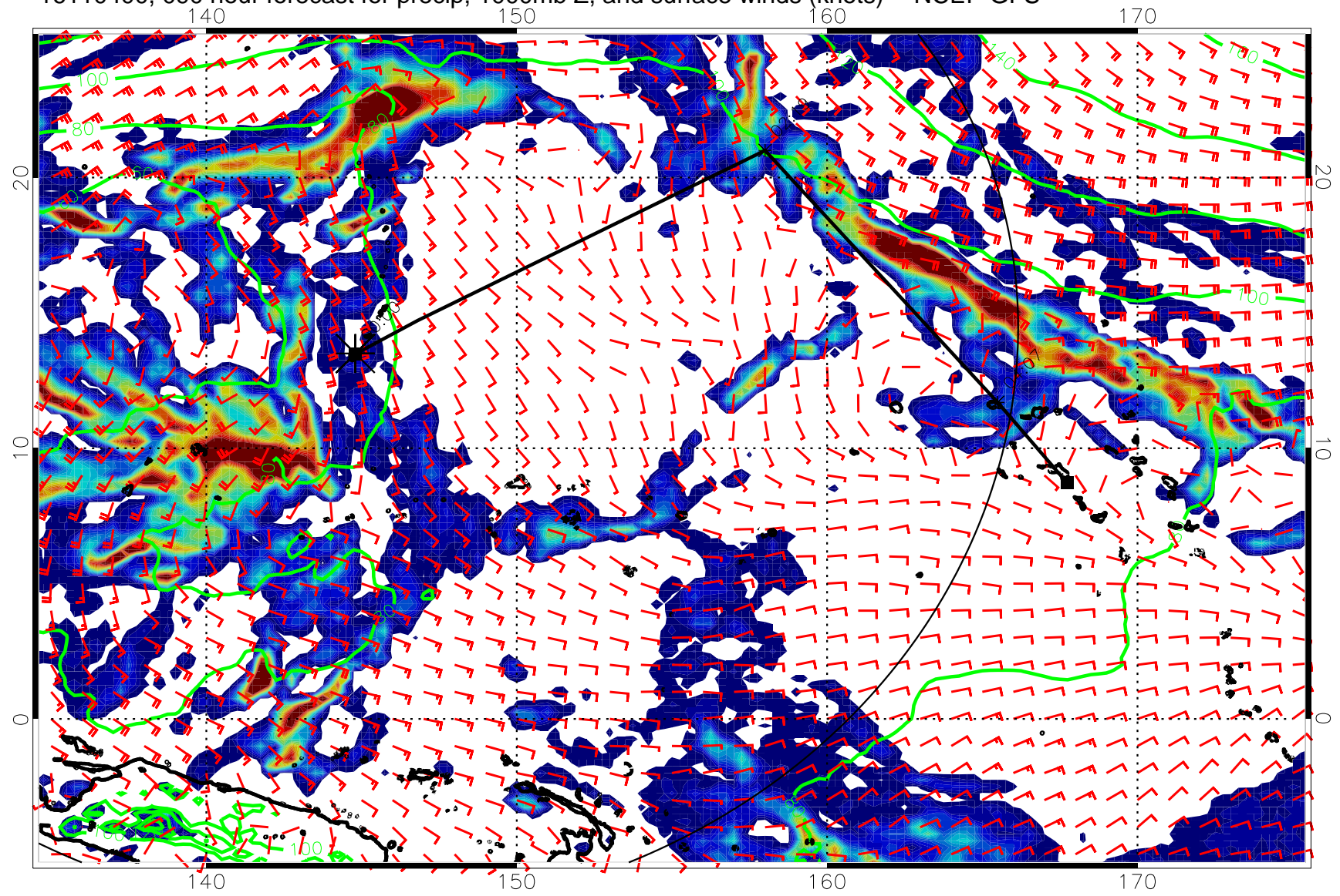
16110400, 090 hour forecast for precip, 1000mb Z, and surface winds (knots) -- NCEP GFS
