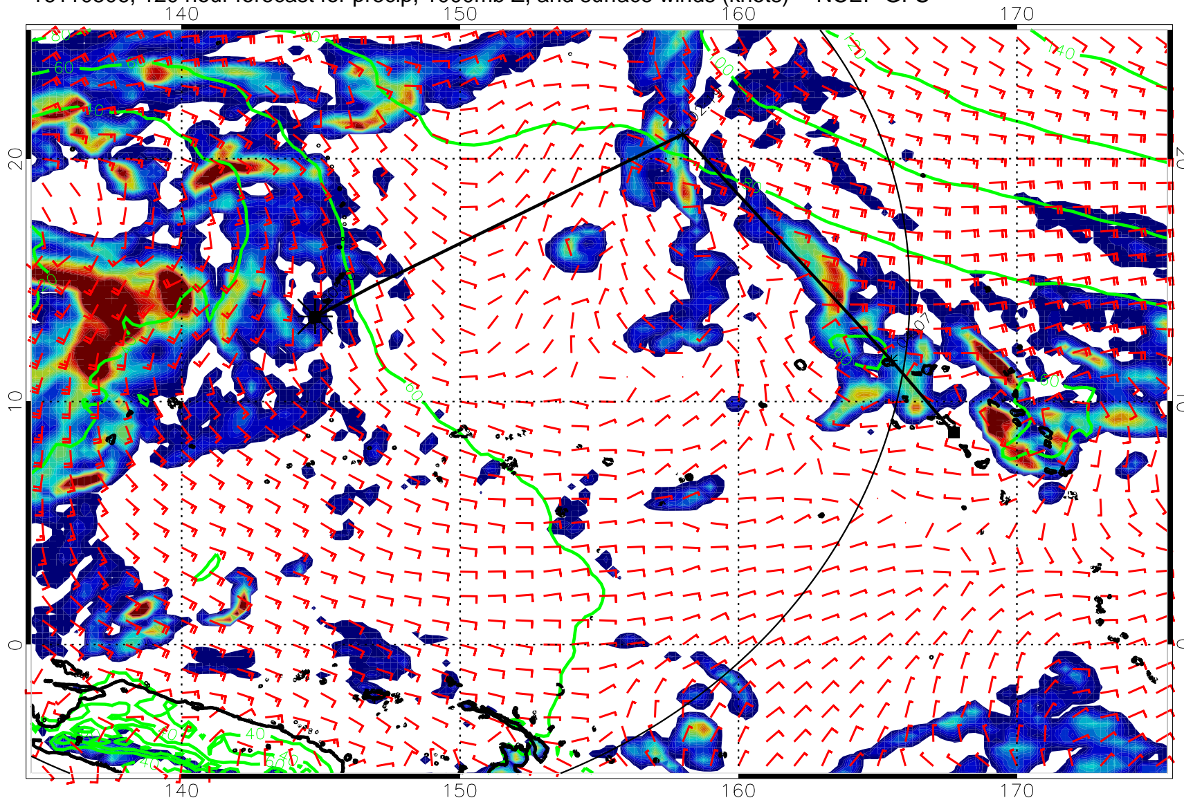
16110506, 120 hour forecast for precip, 1000mb Z, and surface winds (knots) -- NCEP GFS
