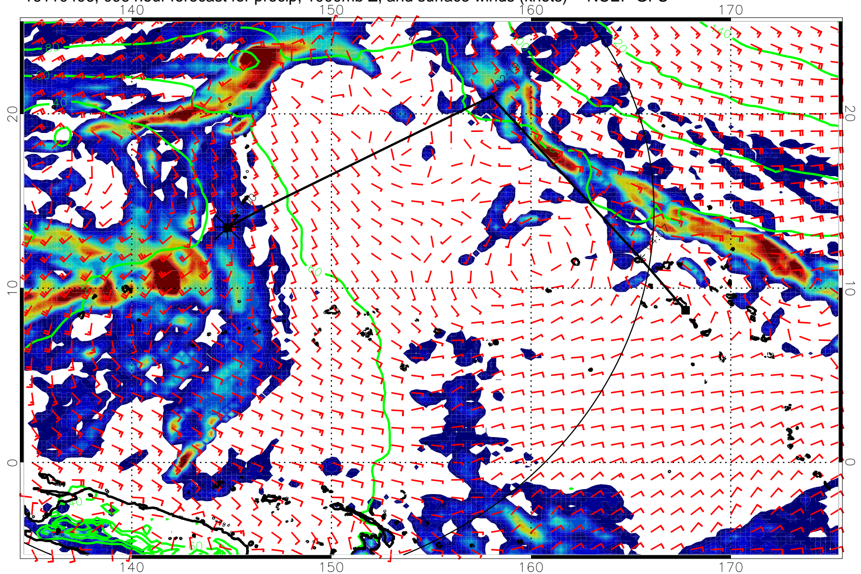
16110406, 096 hour forecast for precip, 1000mb Z, and surface winds (knots) -- NCEP GFS
