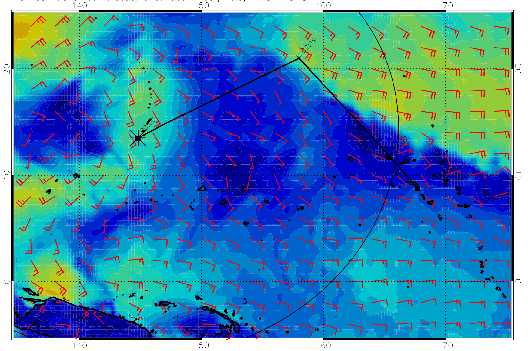
16110312, 078 hour forecast for surface winds (knots) -- NCEP GFS
