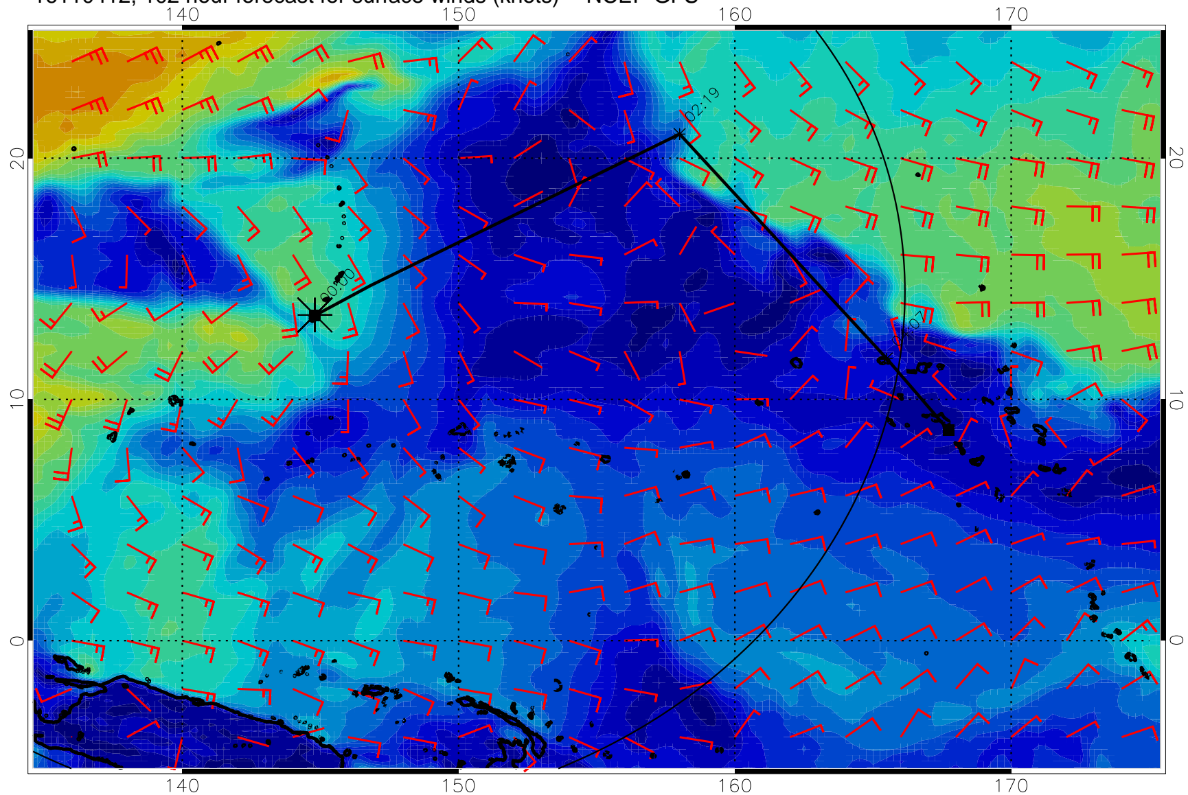
16110412, 102 hour forecast for surface winds (knots) -- NCEP GFS
