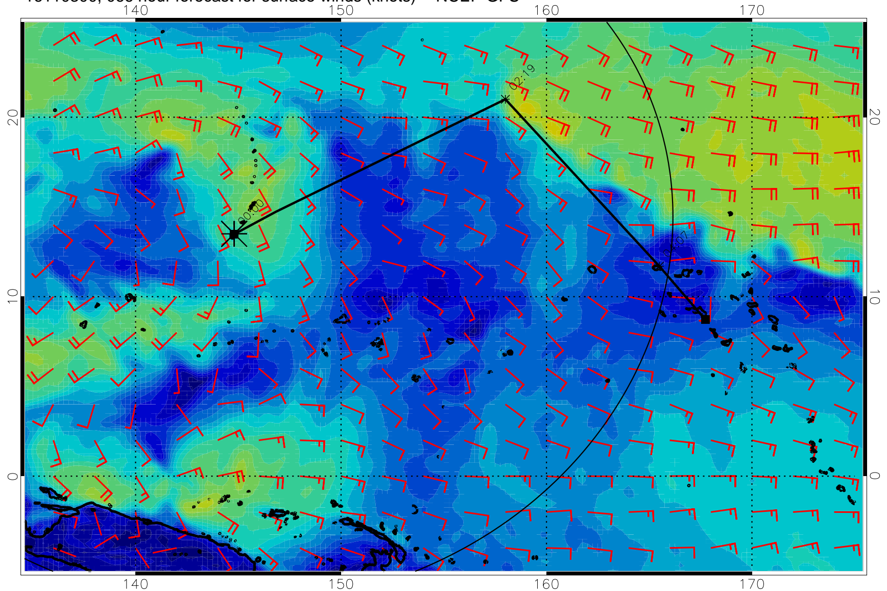
16110300, 066 hour forecast for surface winds (knots) -- NCEP GFS
