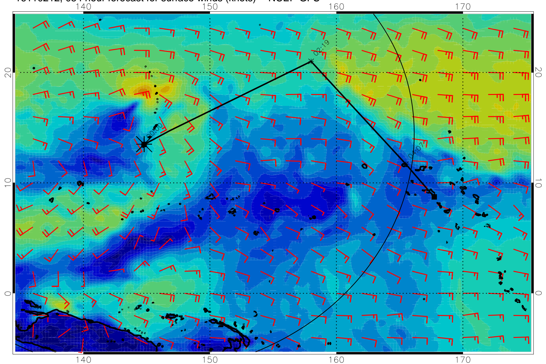
16110212, 054 hour forecast for surface winds (knots) -- NCEP GFS
