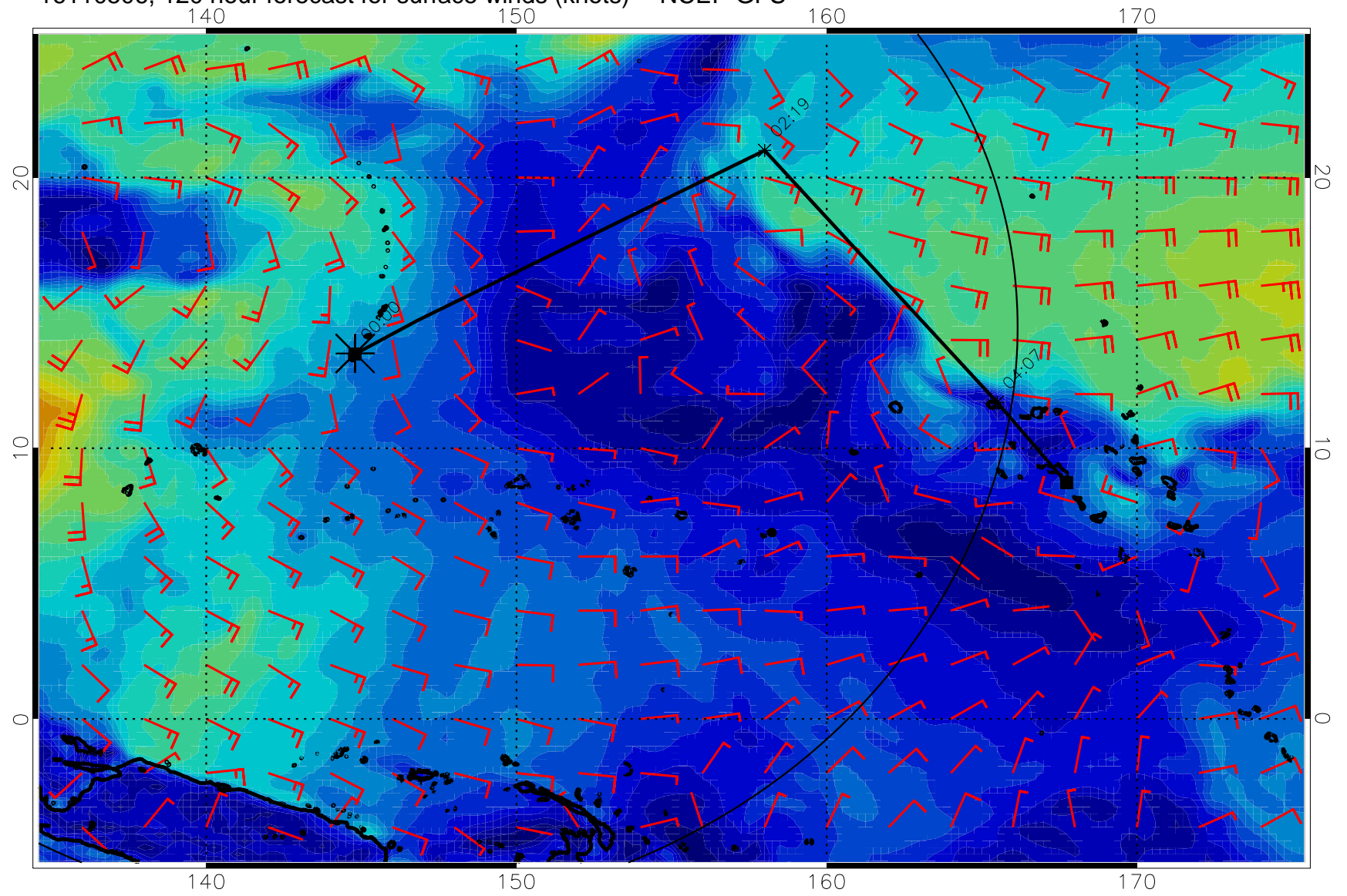
16110506, 120 hour forecast for surface winds (knots) -- NCEP GFS
