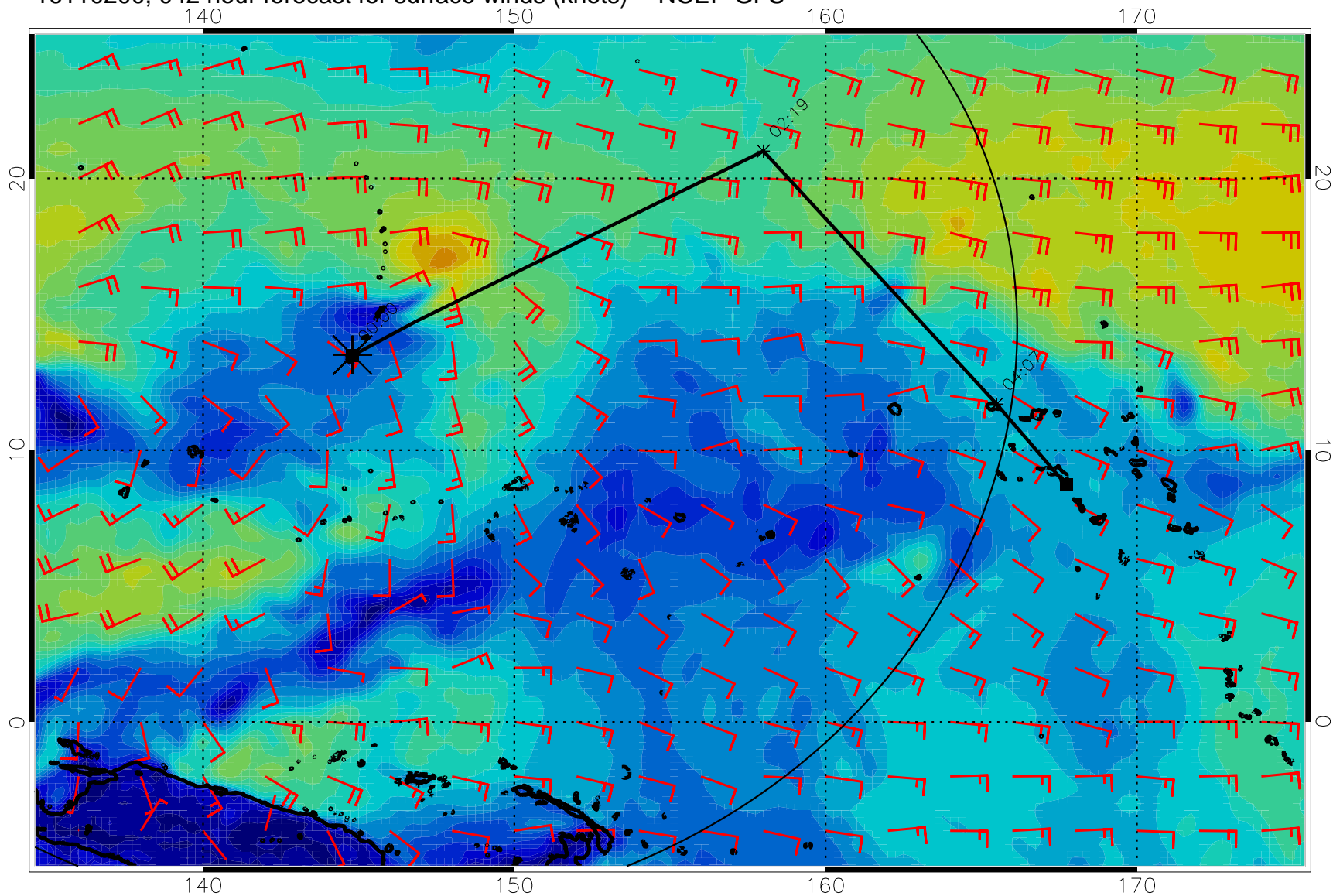
16110200, 042 hour forecast for surface winds (knots) -- NCEP GFS
