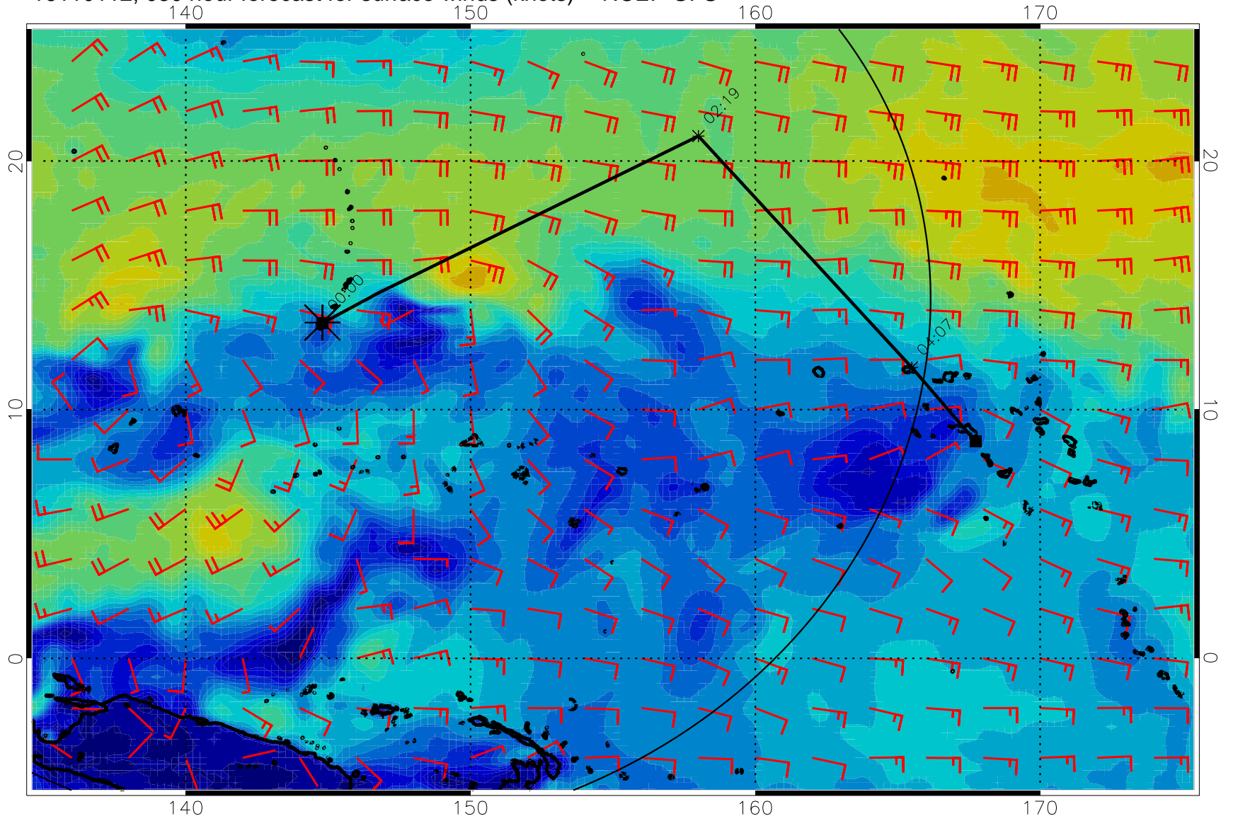
16110112, 0300 hour forecast for surface winds (knots) -- NCEP GFS
