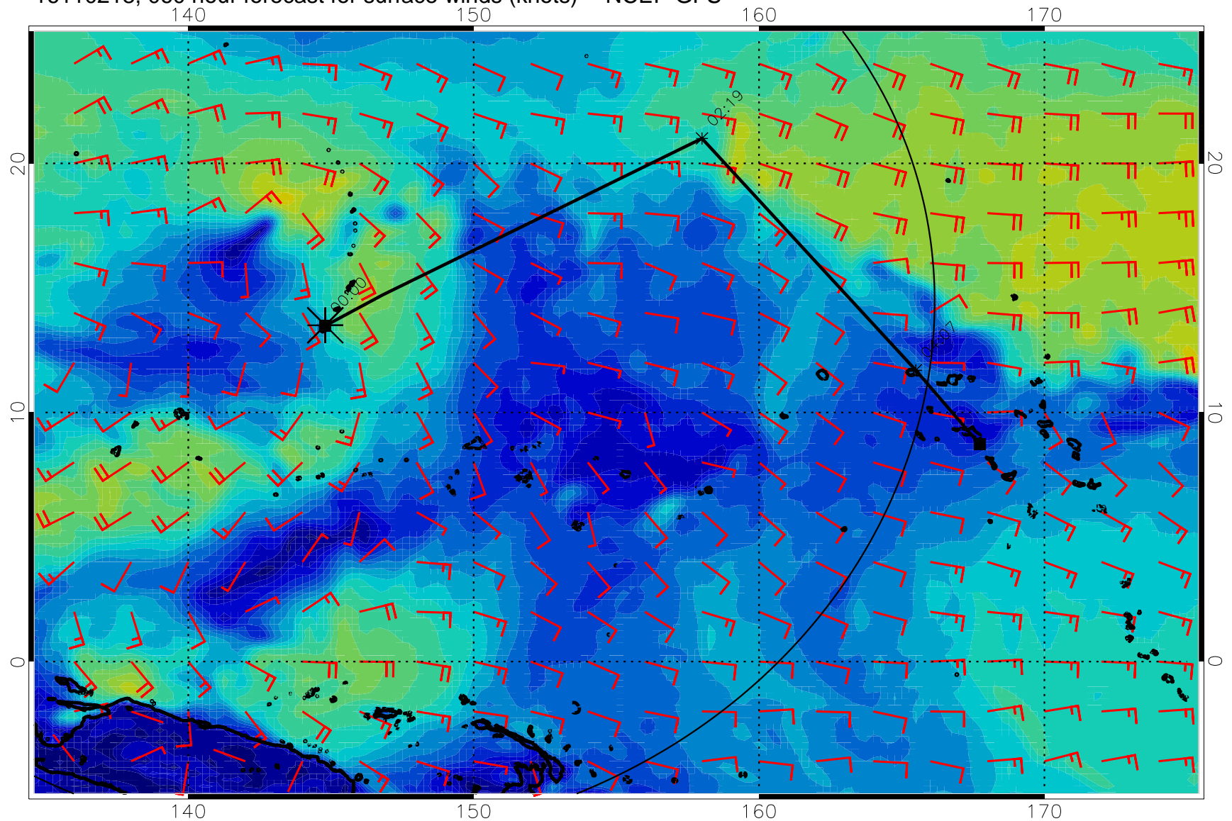
16110218, 060 hour forecast for surface winds (knots) -- NCEP GFS
