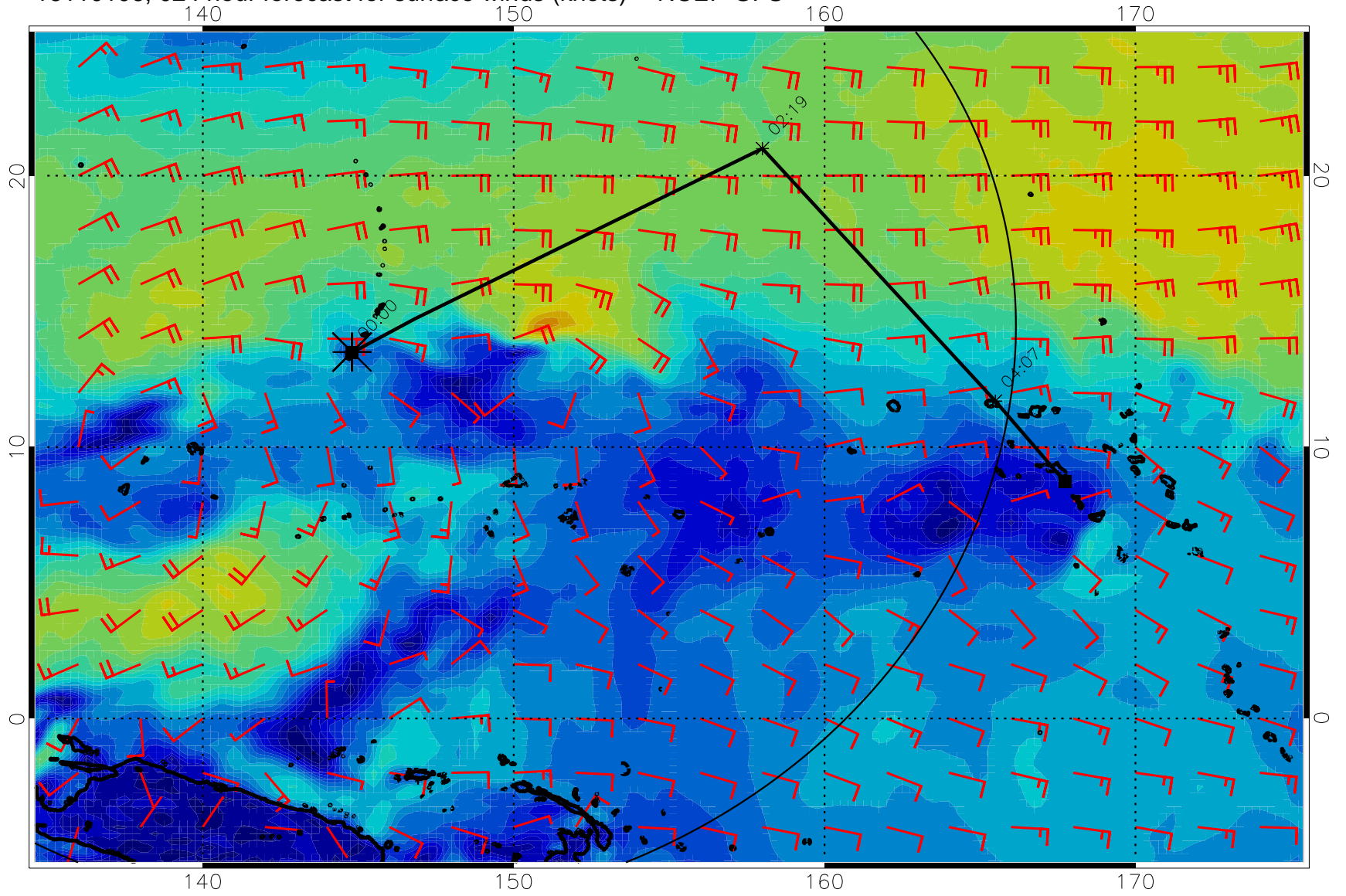
16110106, 024 hour forecast for surface winds (knots) -- NCEP GFS
