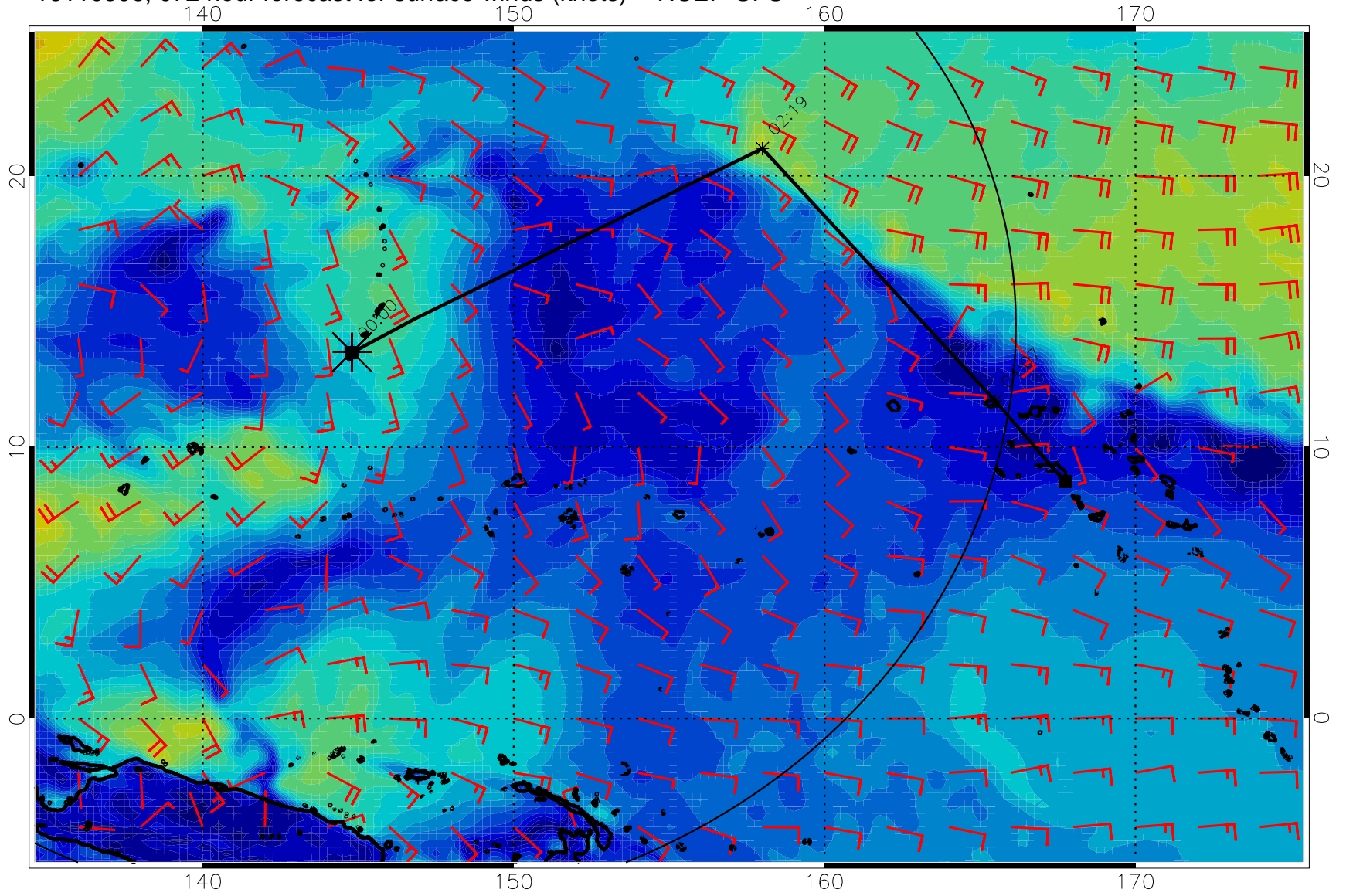
16110306, 072 hour forecast for surface winds (knots) -- NCEP GFS
