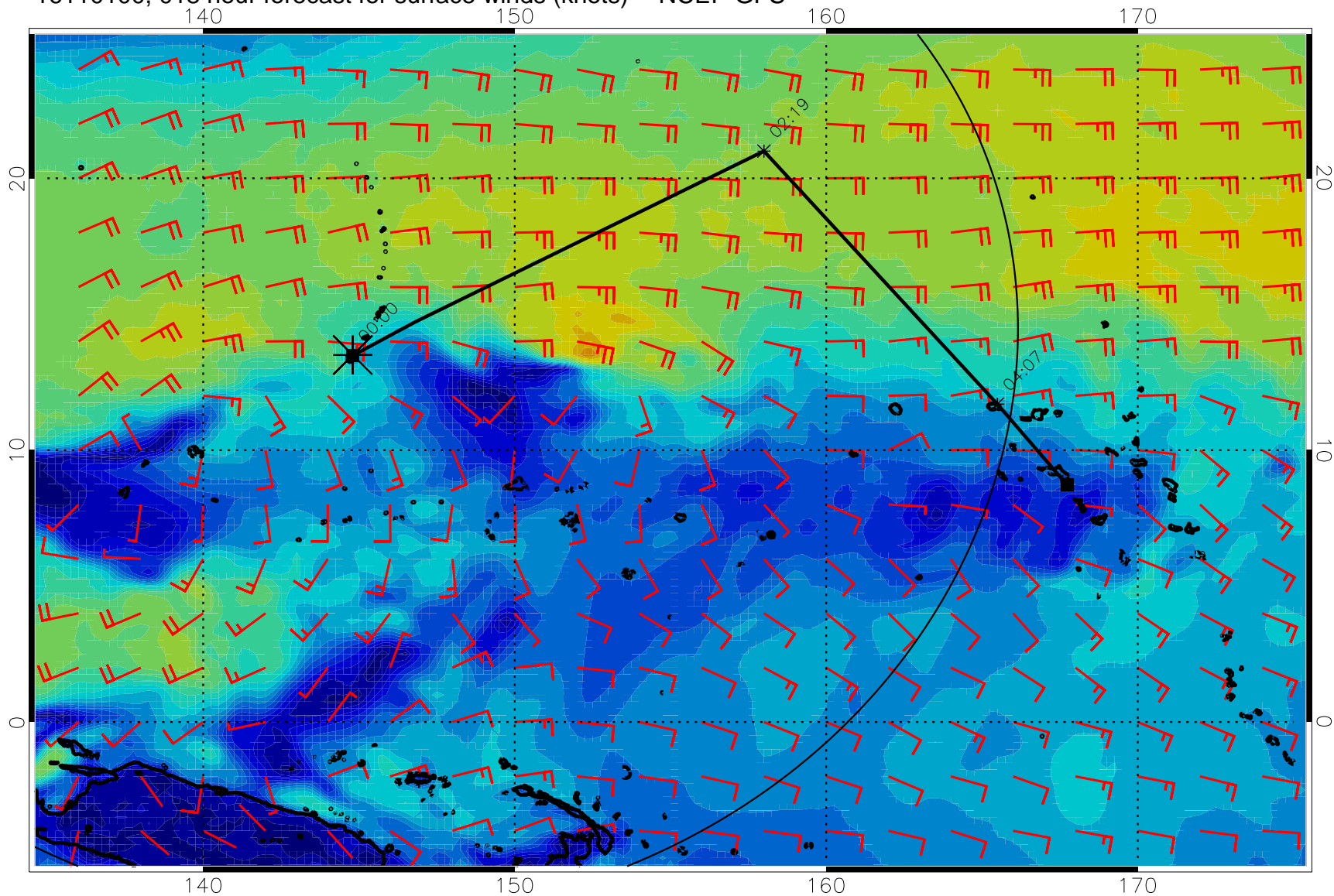
16110100, 018 hour forecast for surface winds (knots) -- NCEP GFS
