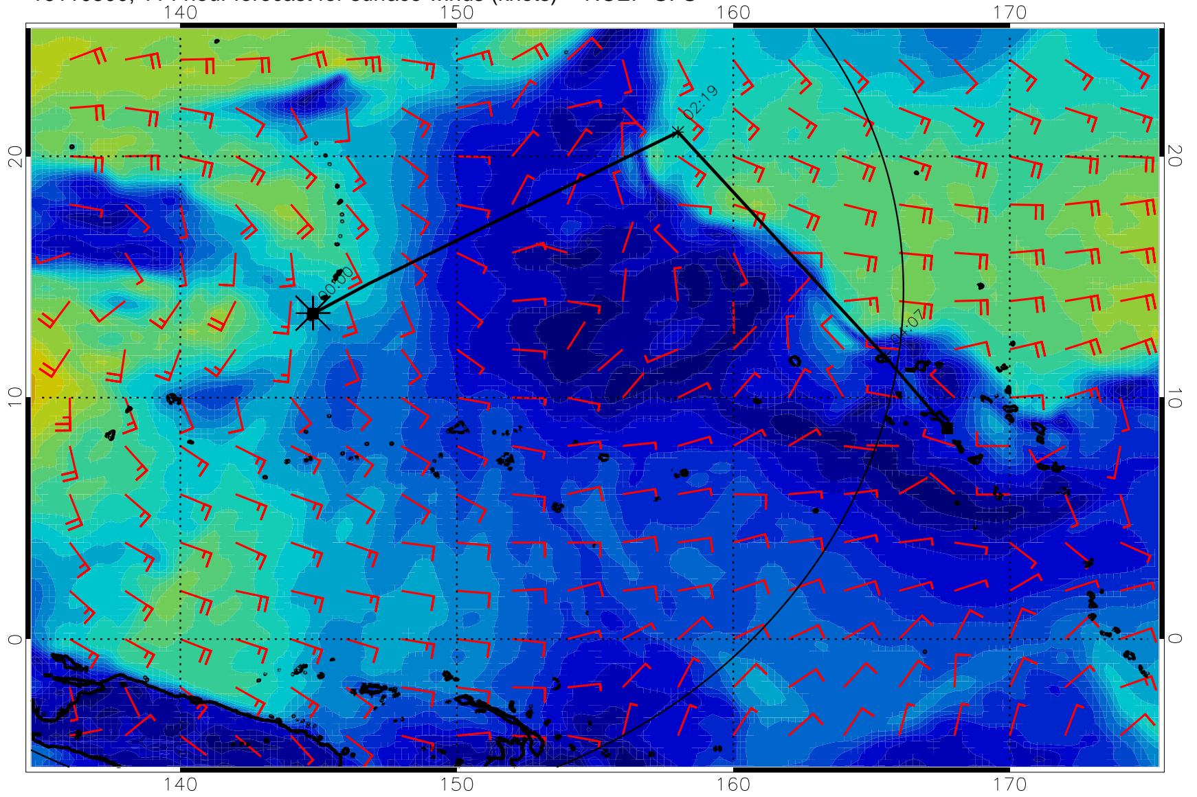
16110500, 114 hour forecast for surface winds (knots) -- NCEP GFS
