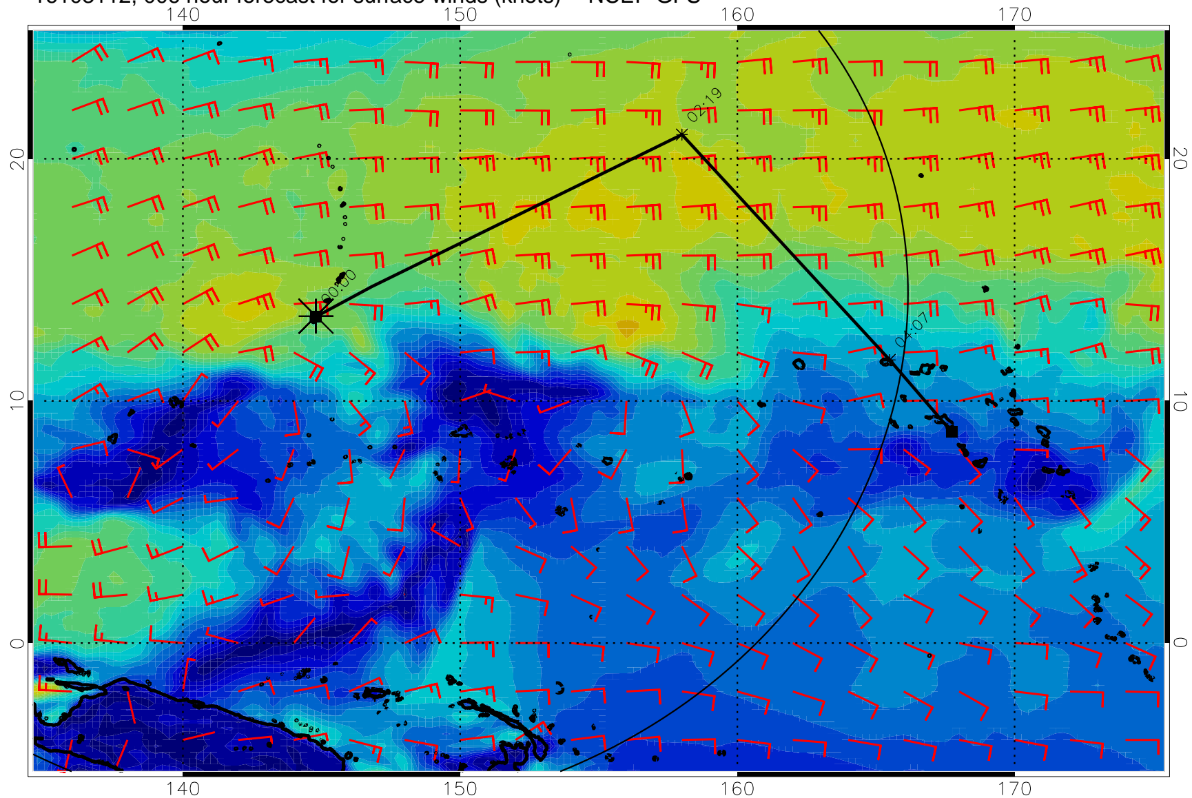
16103112, 006 hour forecast for surface winds (knots) -- NCEP GFS
