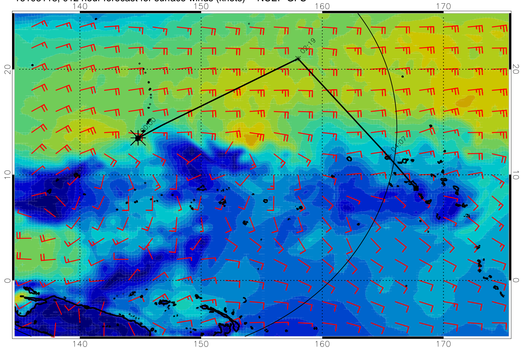
16103118, 012 hour forecast for surface winds (knots) -- NCEP GFS
