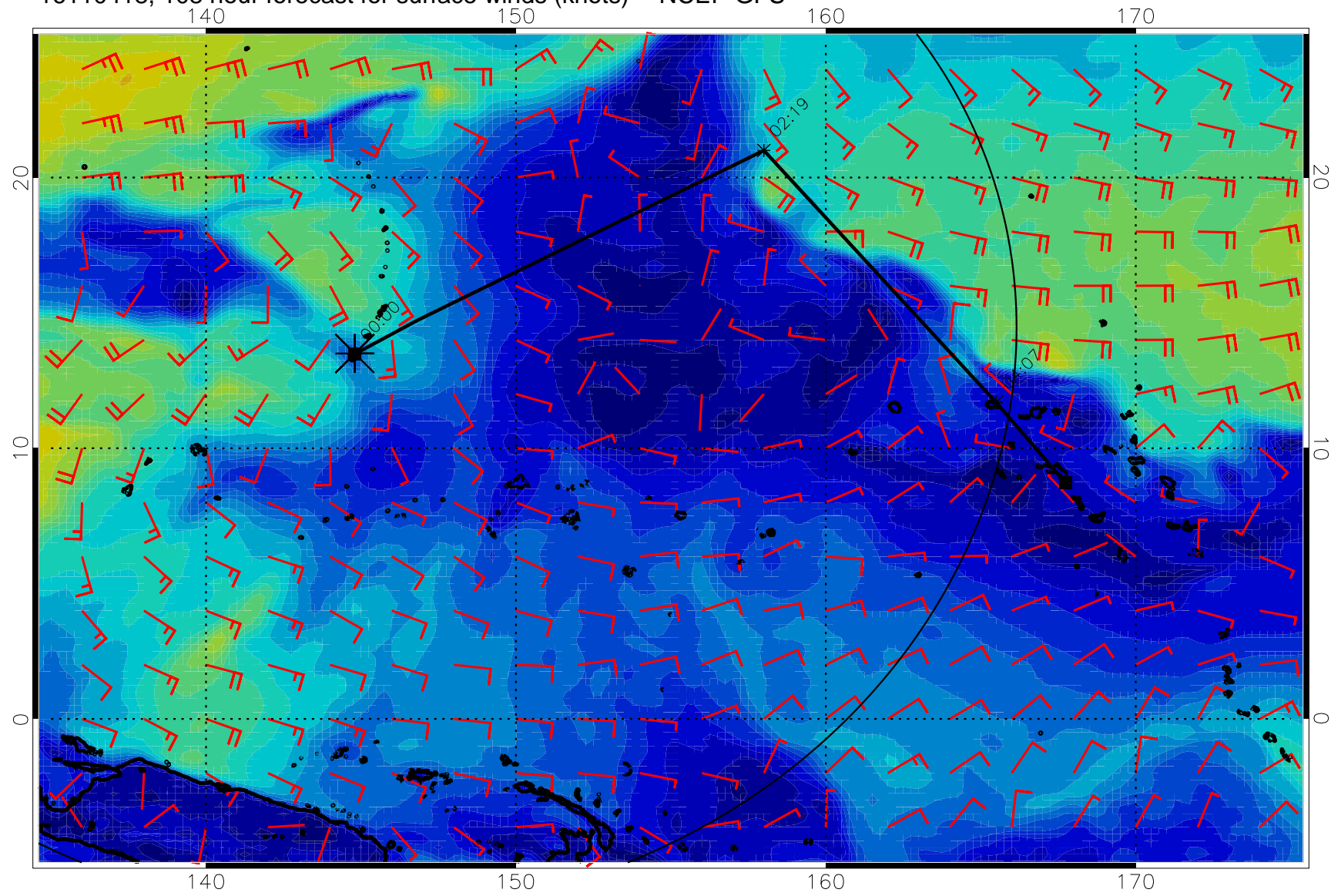
16110418, 108 hour forecast for surface winds (knots) -- NCEP GFS
