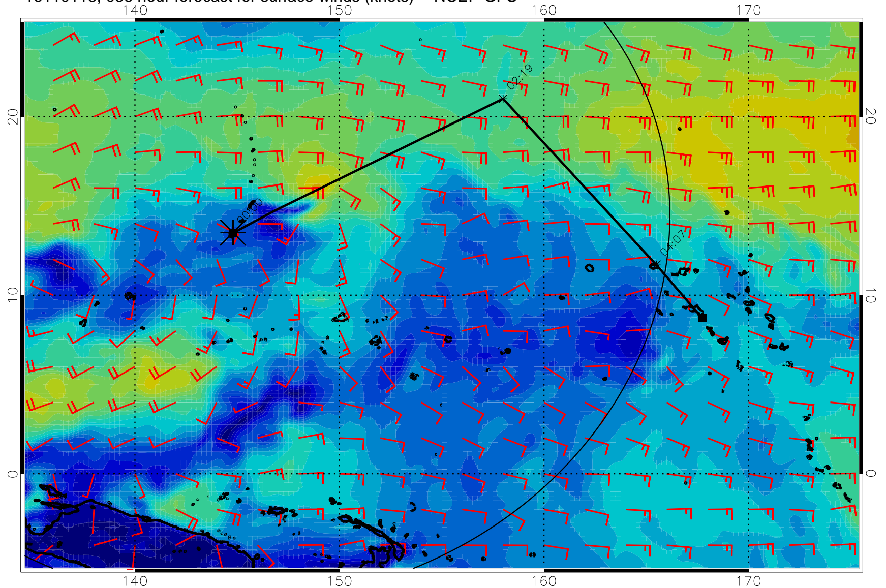
16110118, 036 hour forecast for surface winds (knots) -- NCEP GFS
