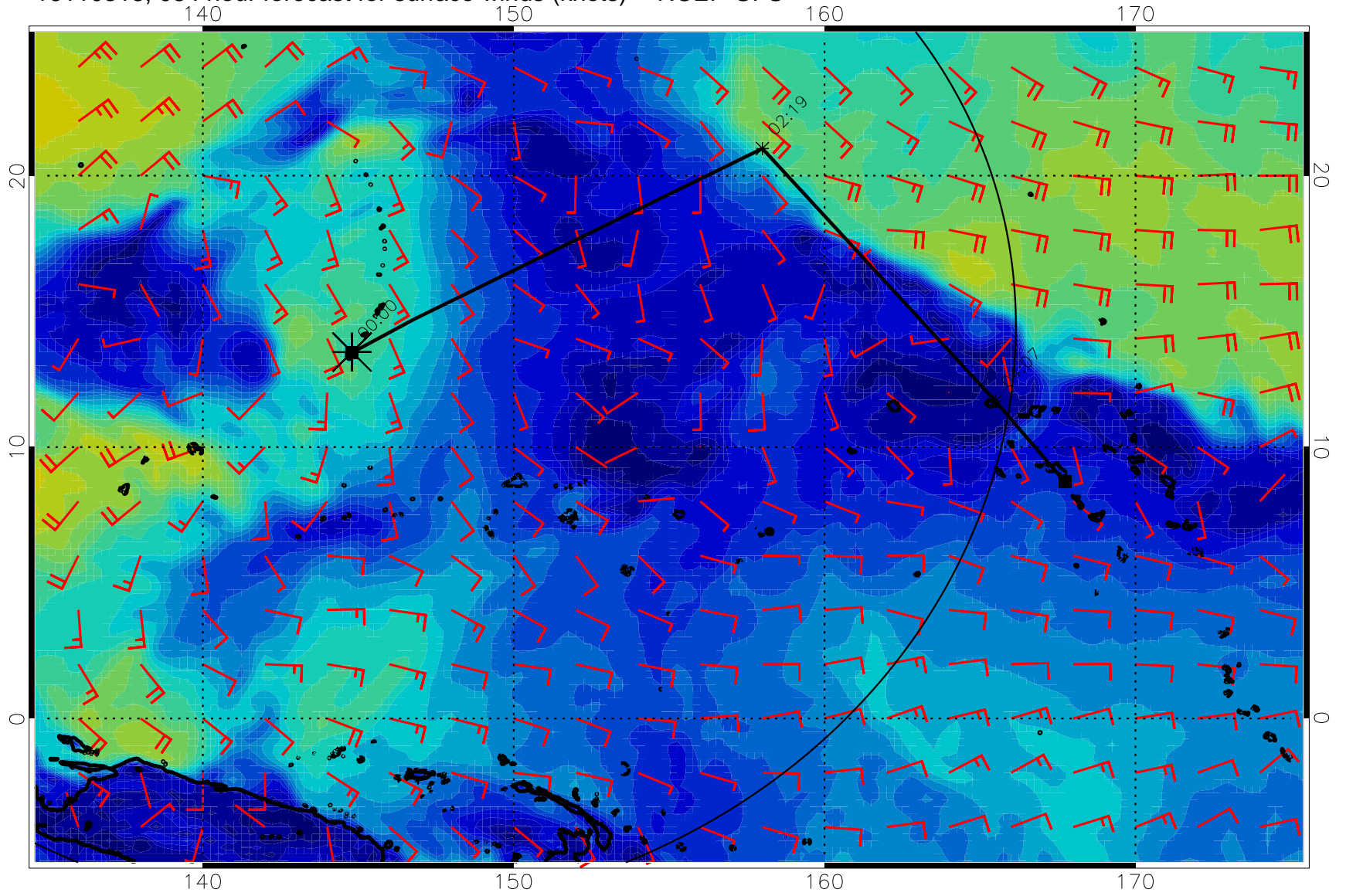
16110318, 084 hour forecast for surface winds (knots) -- NCEP GFS
