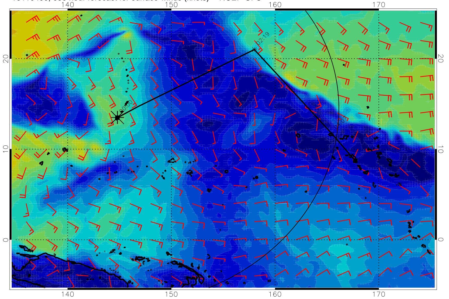
16110400, 090 hour forecast for surface winds (knots) -- NCEP GFS
