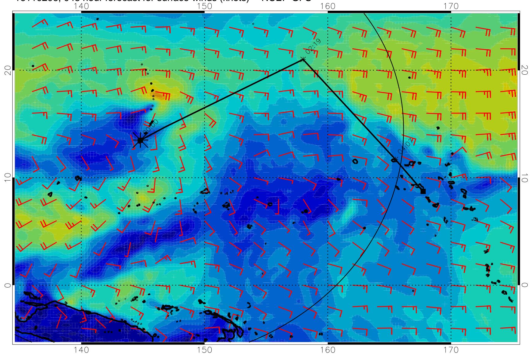
16110206, 048 hour forecast for surface winds (knots) -- NCEP GFS
