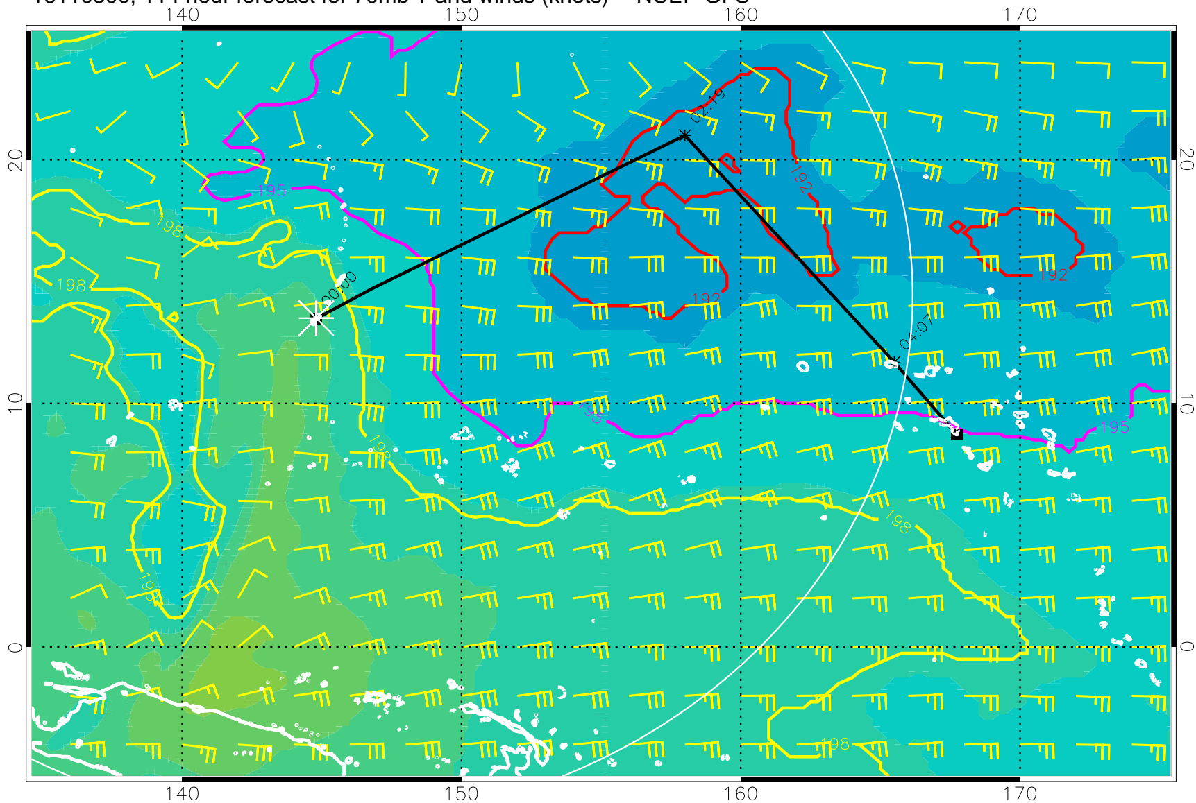
16110500, 114 hour forecast for 70mb T and winds (knots) -- NCEP GFS
