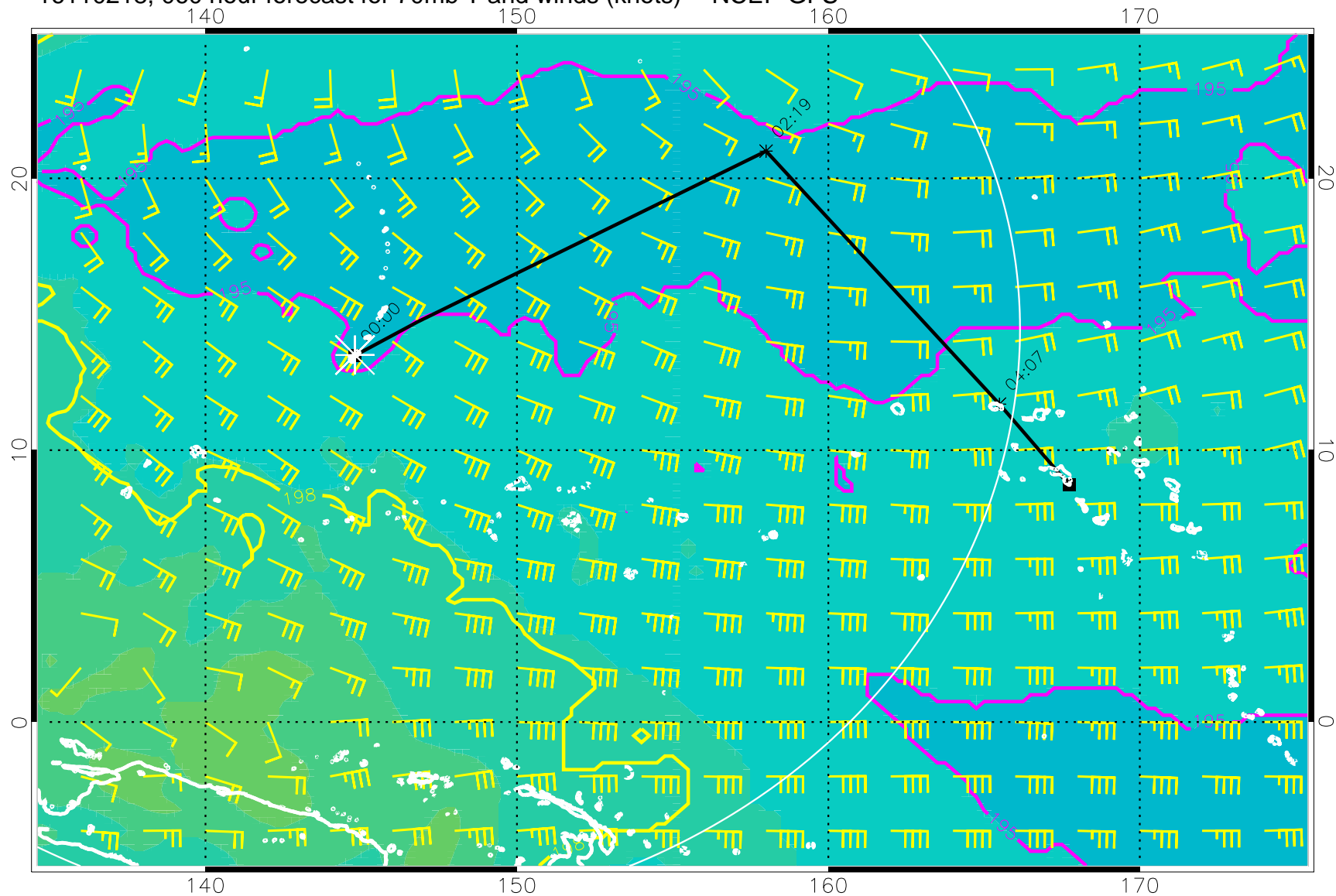
16110218, 060 hour forecast for 70mb T and winds (knots) -- NCEP GFS
