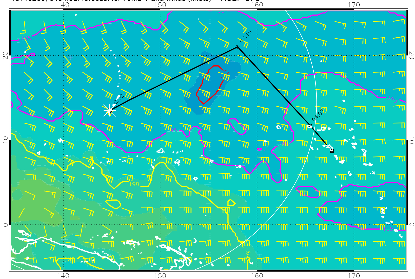
16110206, 048 hour forecast for 70mb T and winds (knots) -- NCEP GFS
