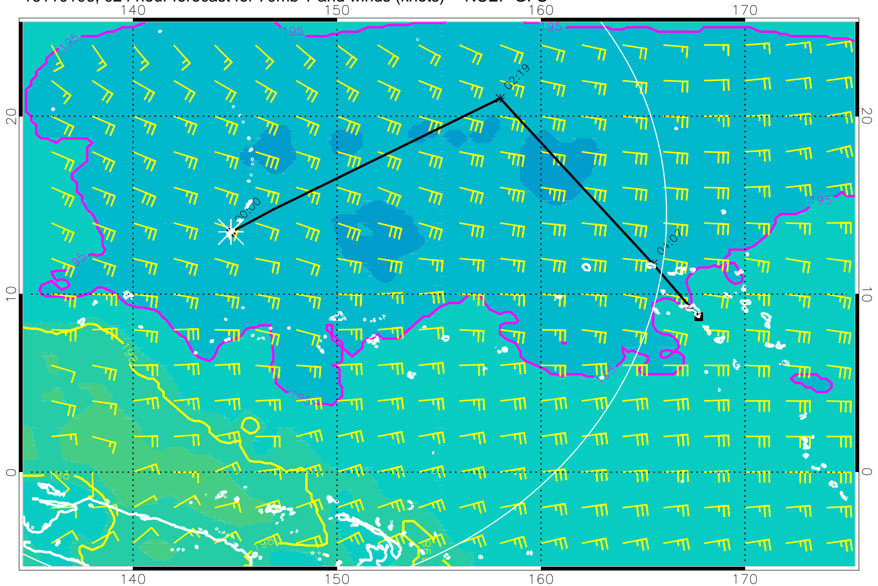
16110106, 024 hour forecast for 70mb T and winds (knots) -- NCEP GFS
