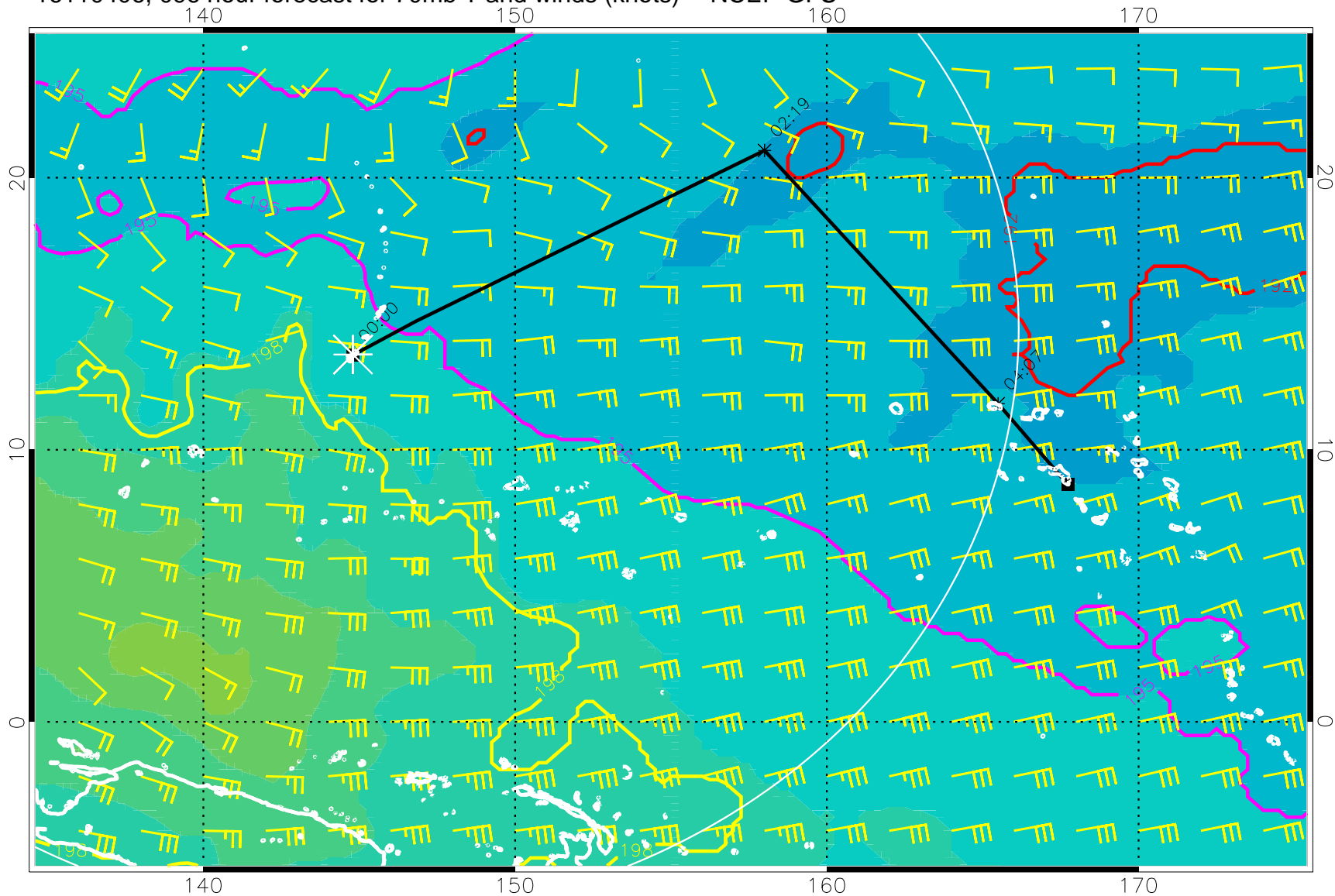
16110406, 096 hour forecast for 70mb T and winds (knots) -- NCEP GFS
