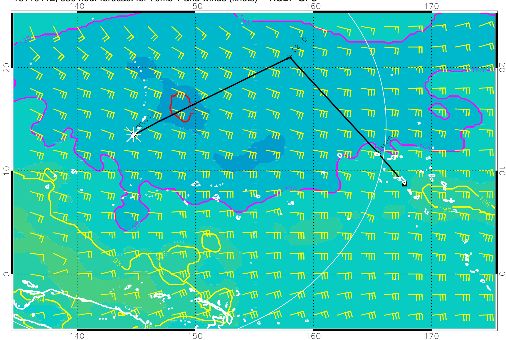
16110112, 0300 hour forecast for 70mb T and winds (knots) -- NCEP GFS
