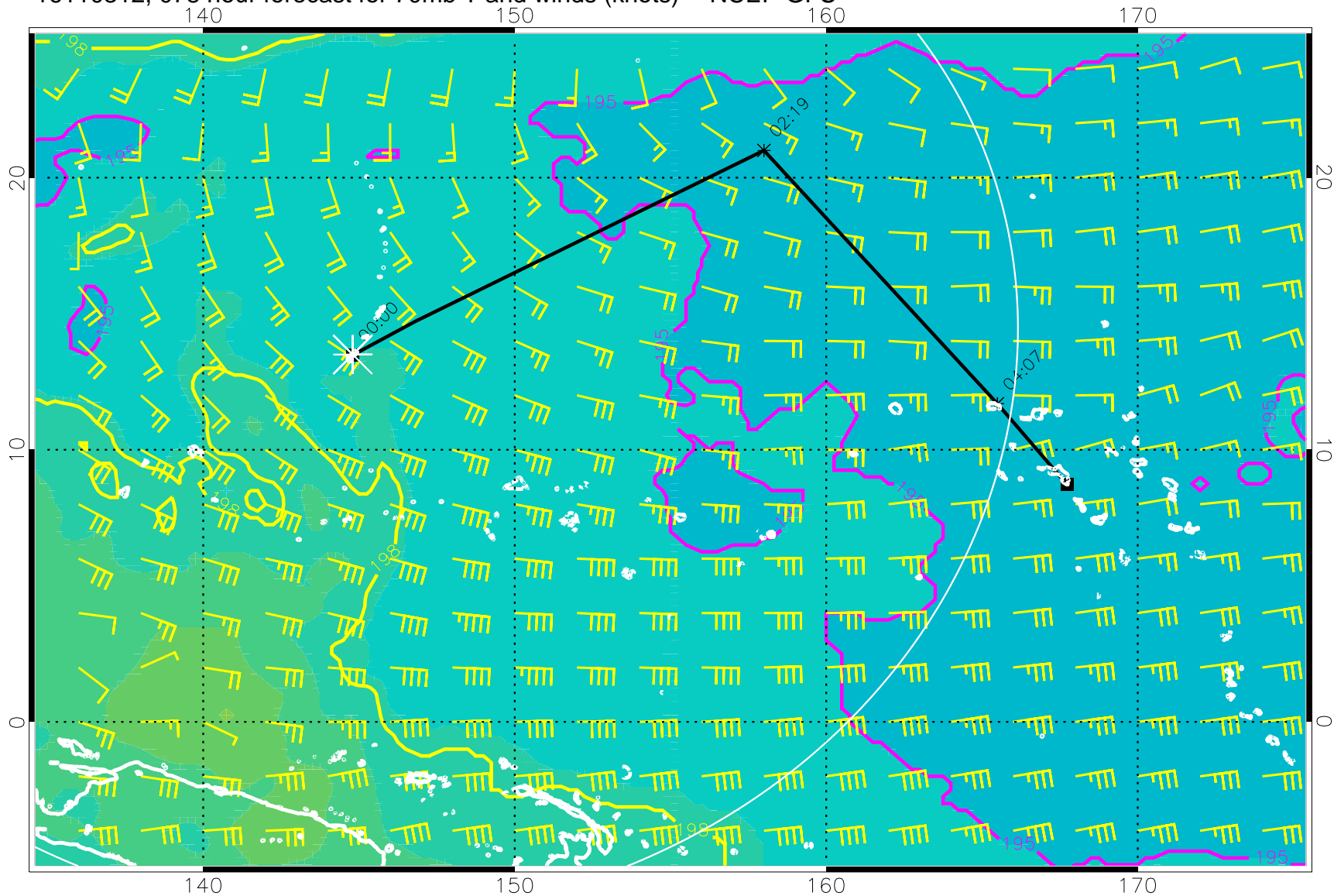
16110312, 078 hour forecast for 70mb T and winds (knots) -- NCEP GFS
