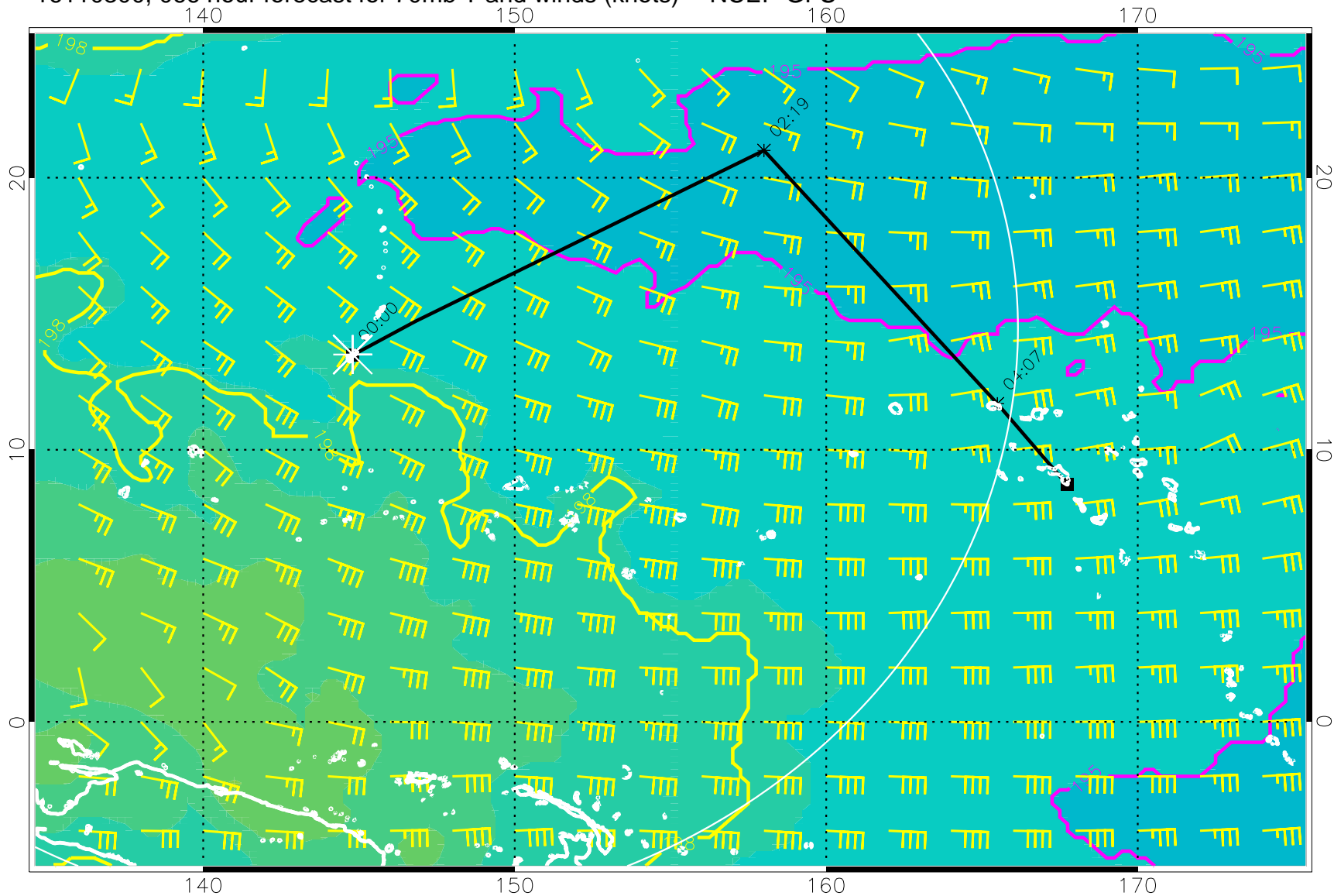
16110300, 066 hour forecast for 70mb T and winds (knots) -- NCEP GFS
