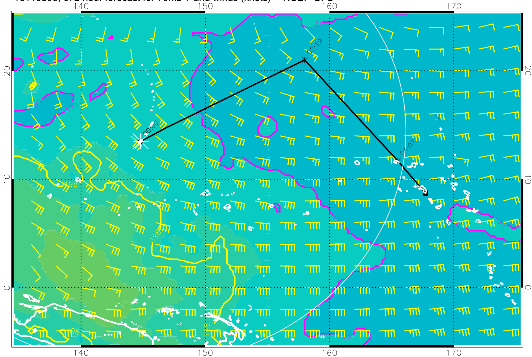
16110306, 072 hour forecast for 70mb T and winds (knots) -- NCEP GFS
