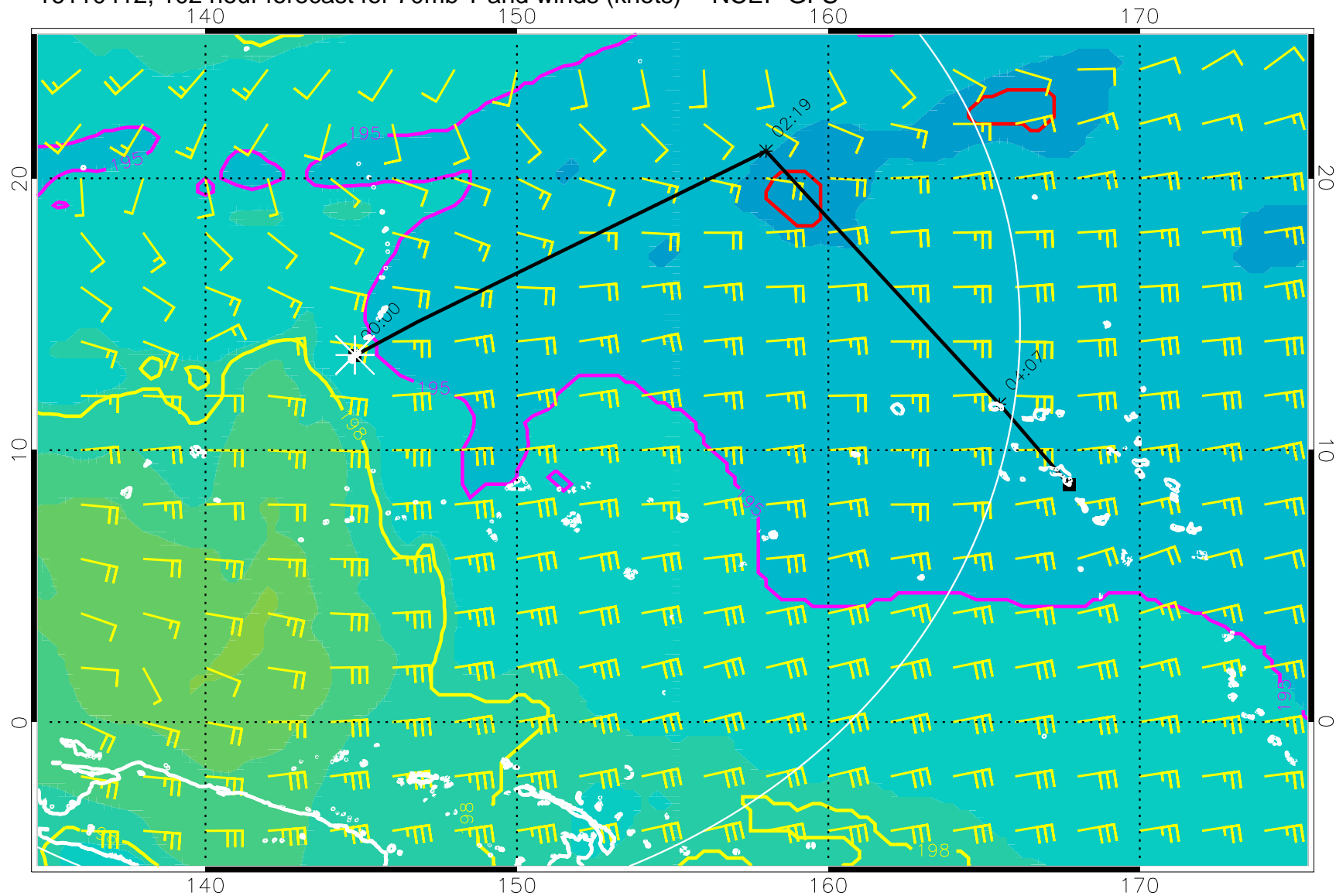
16110412, 102 hour forecast for 70mb T and winds (knots) -- NCEP GFS
