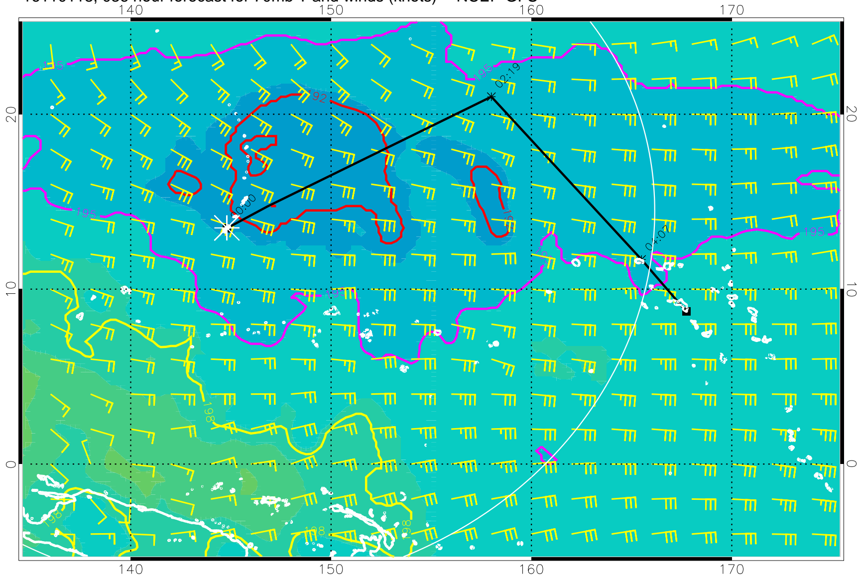
16110118, 036 hour forecast for 70mb T and winds (knots) -- NCEP GFS
