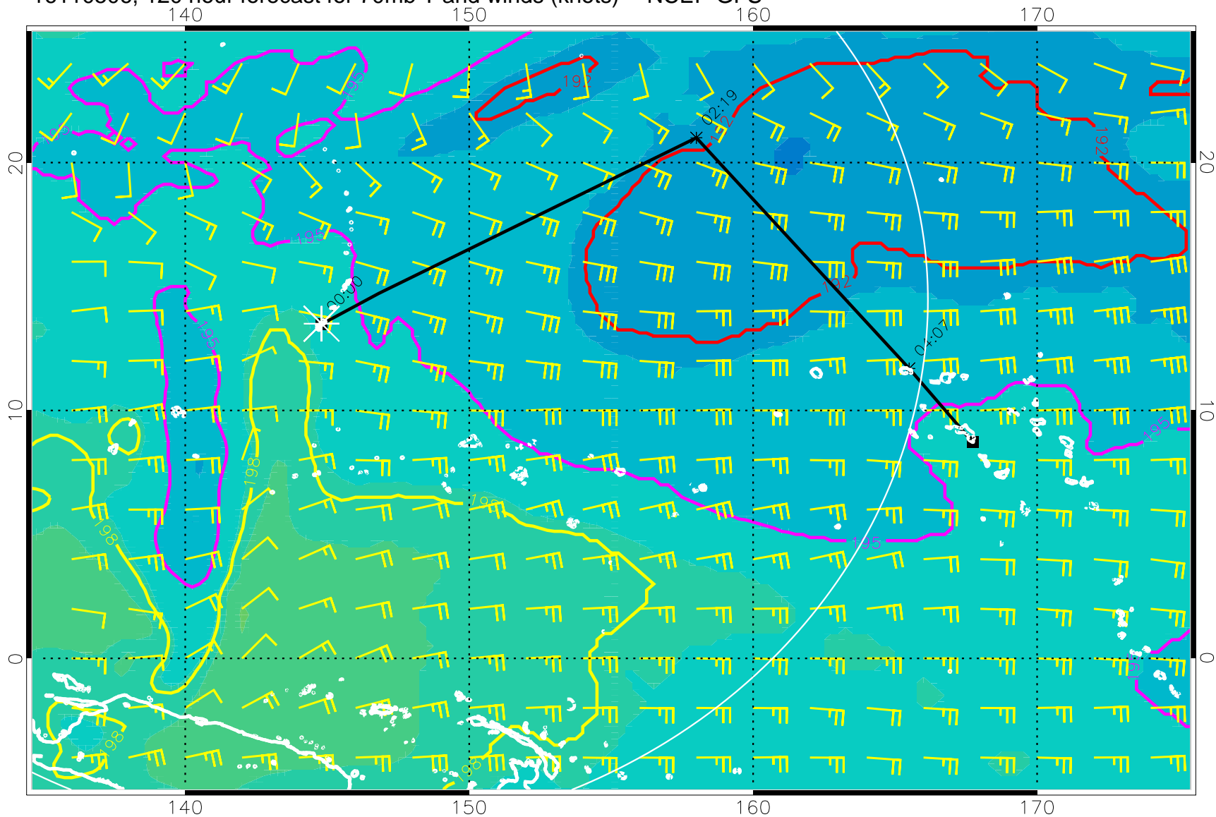
16110506, 120 hour forecast for 70mb T and winds (knots) -- NCEP GFS
