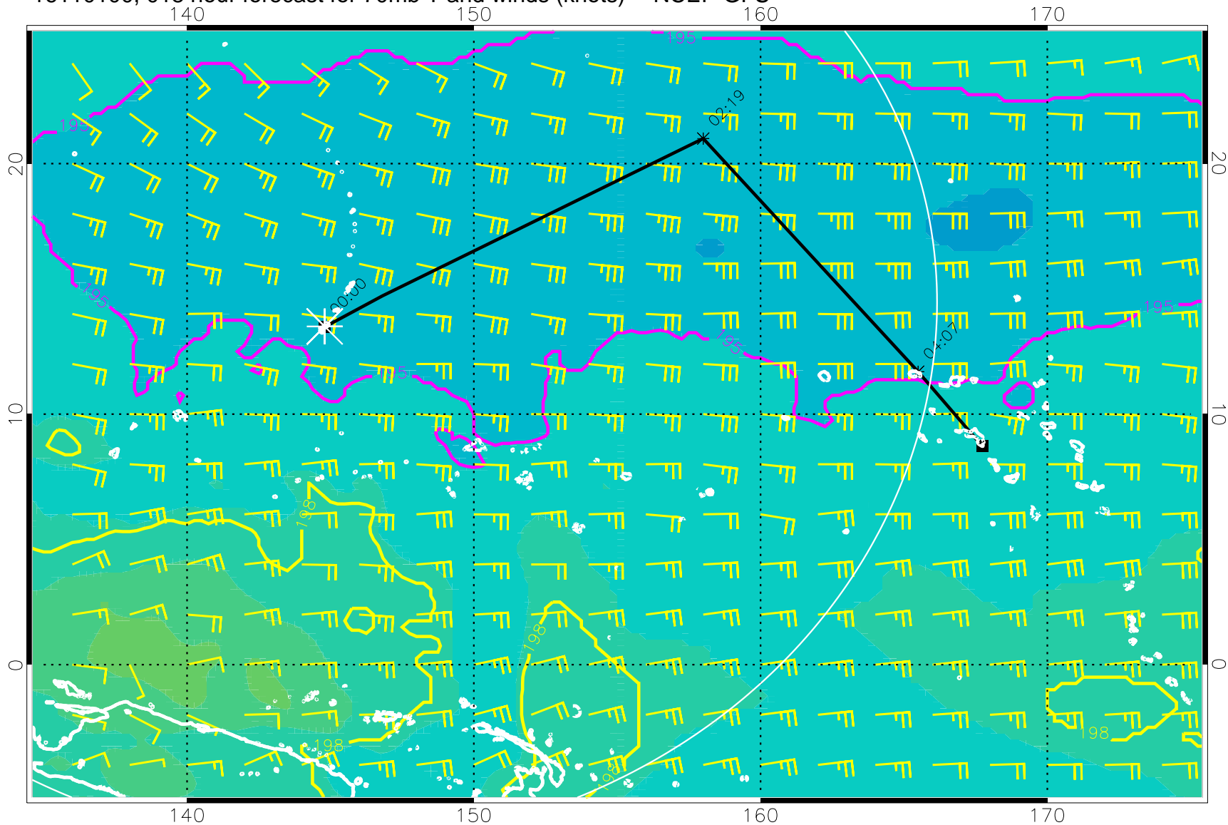
16110100, 018 hour forecast for 70mb T and winds (knots) -- NCEP GFS
