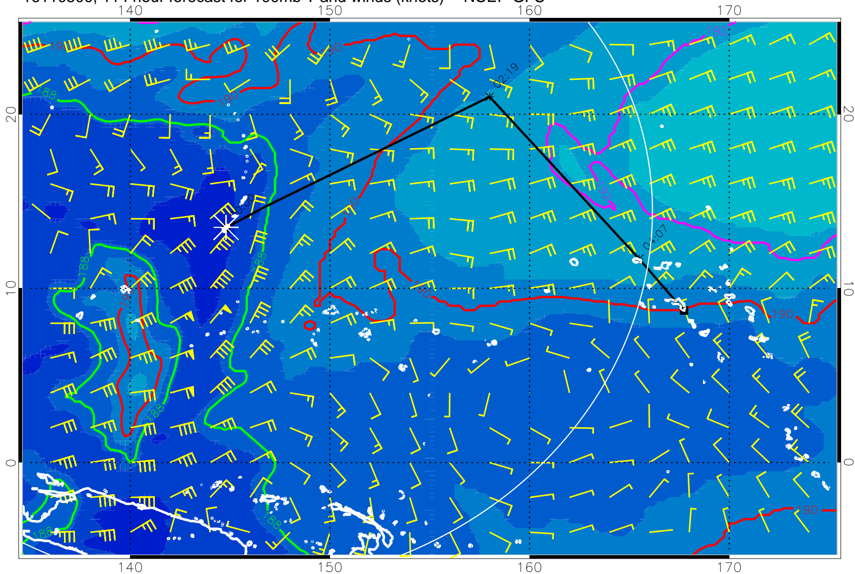
16110500, 114 hour forecast for 100mb T and winds (knots) -- NCEP GFS
