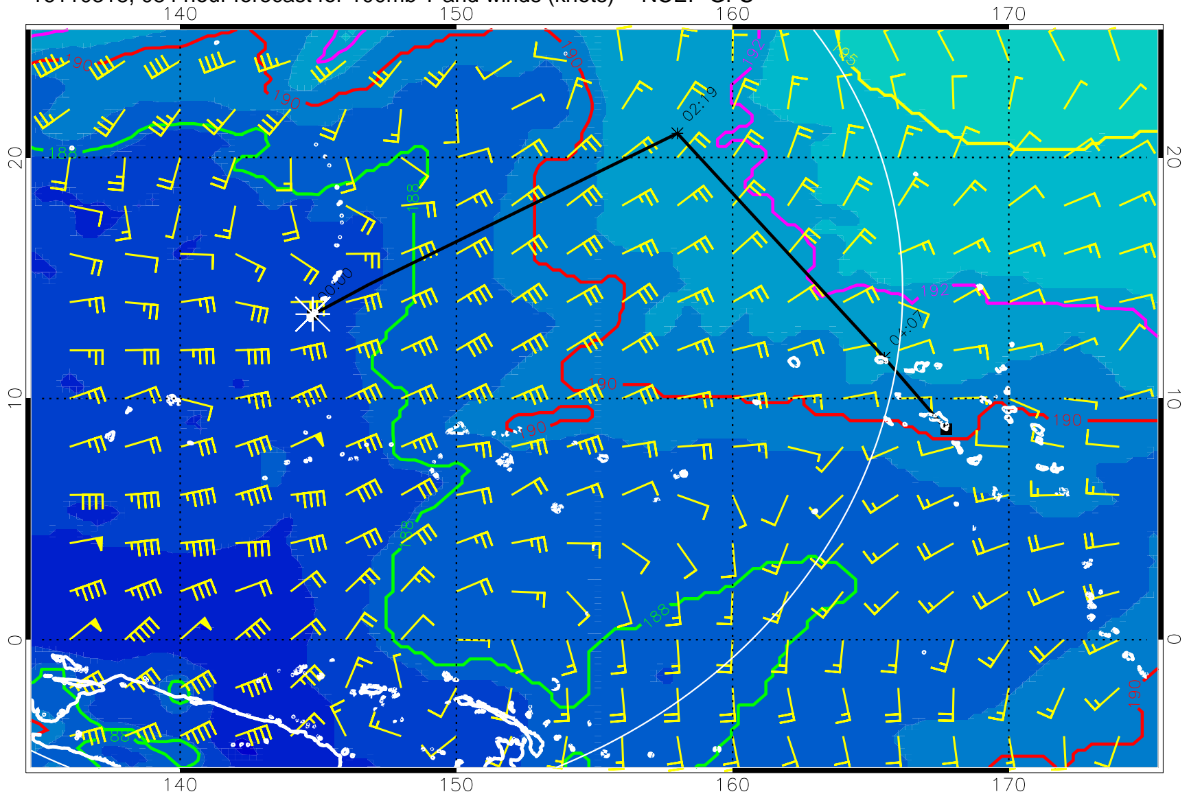
16110318, 084 hour forecast for 100mb T and winds (knots) -- NCEP GFS
