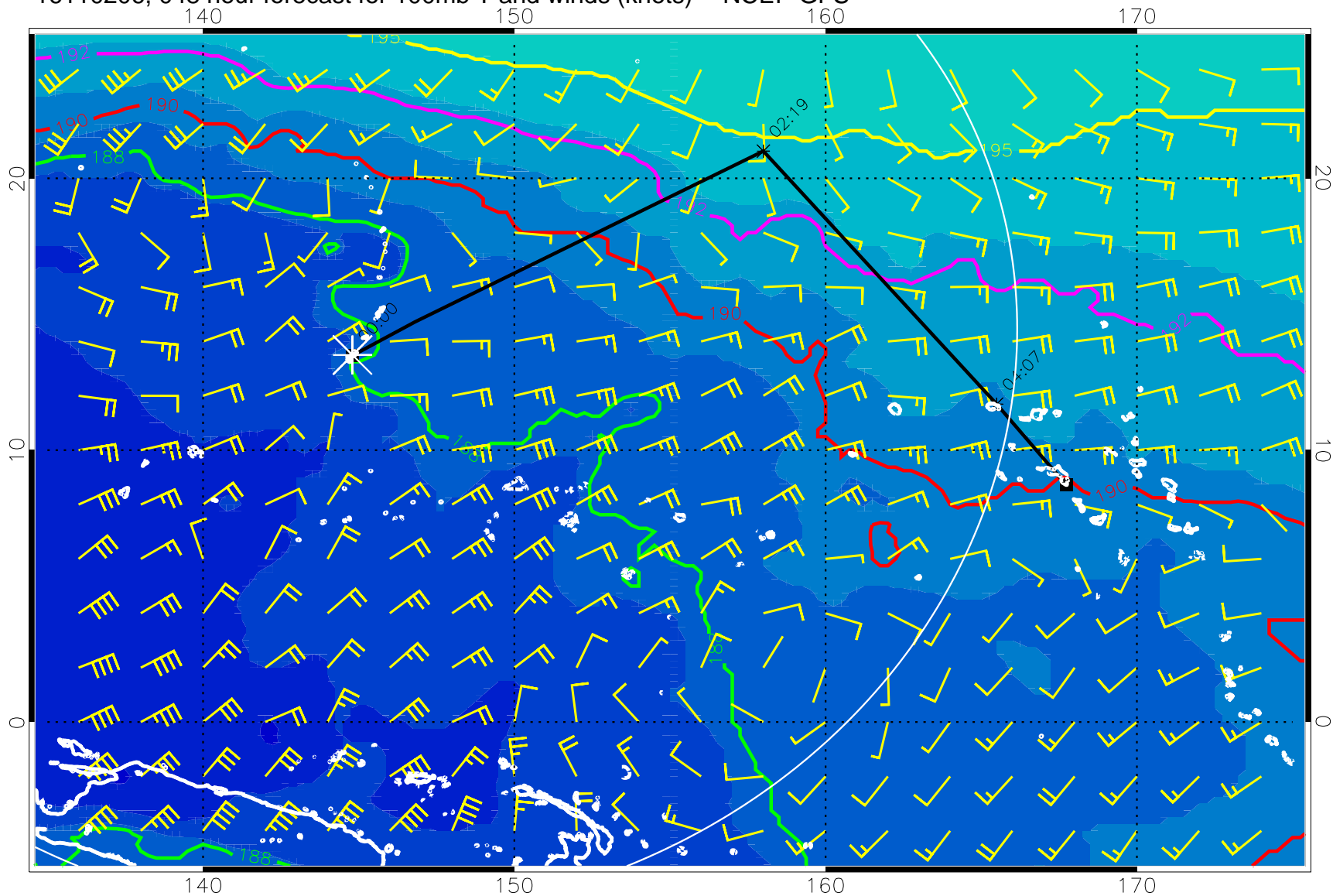
16110206, 048 hour forecast for 100mb T and winds (knots) -- NCEP GFS
