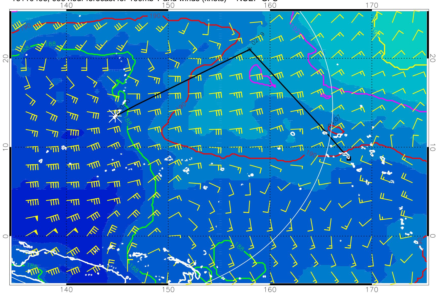
16110406, 096 hour forecast for 100mb T and winds (knots) -- NCEP GFS
