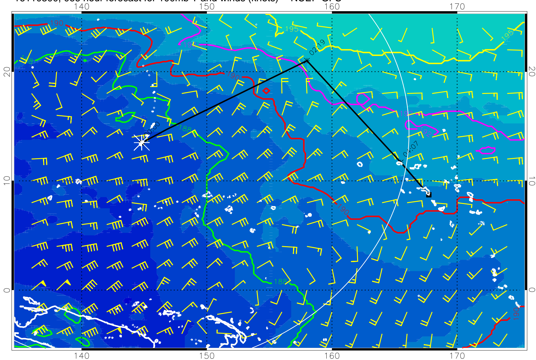
16110300, 066 hour forecast for 100mb T and winds (knots) -- NCEP GFS
