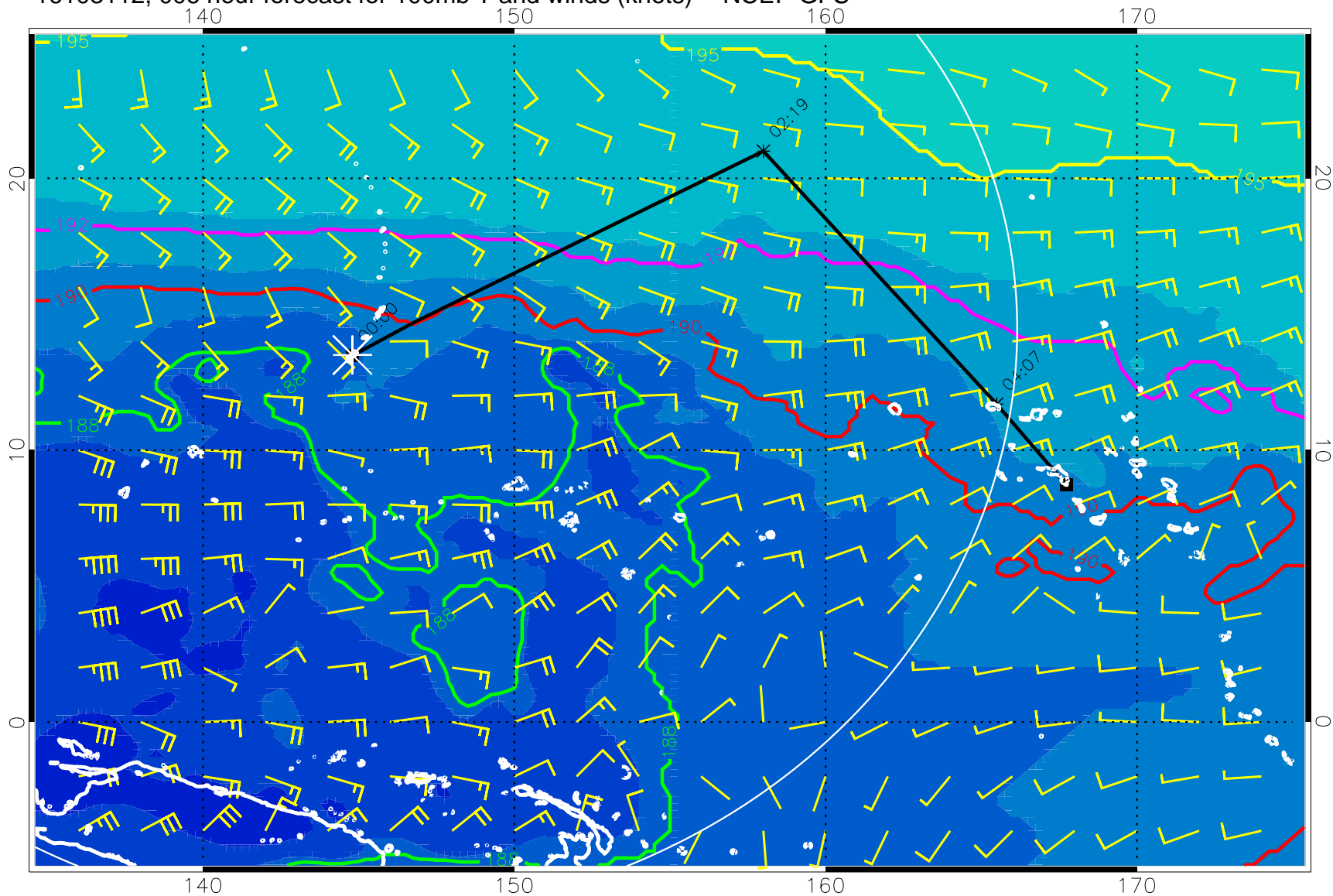
16103112, 006 hour forecast for 100mb T and winds (knots) -- NCEP GFS
