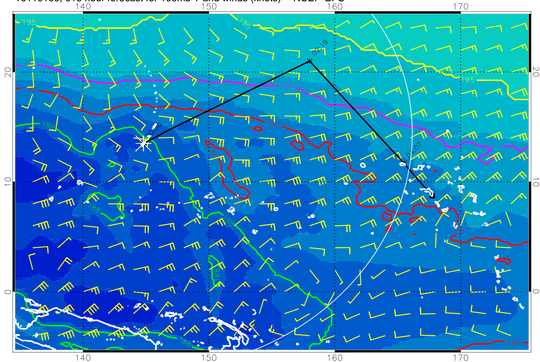
16110100, 018 hour forecast for 100mb T and winds (knots) -- NCEP GFS
