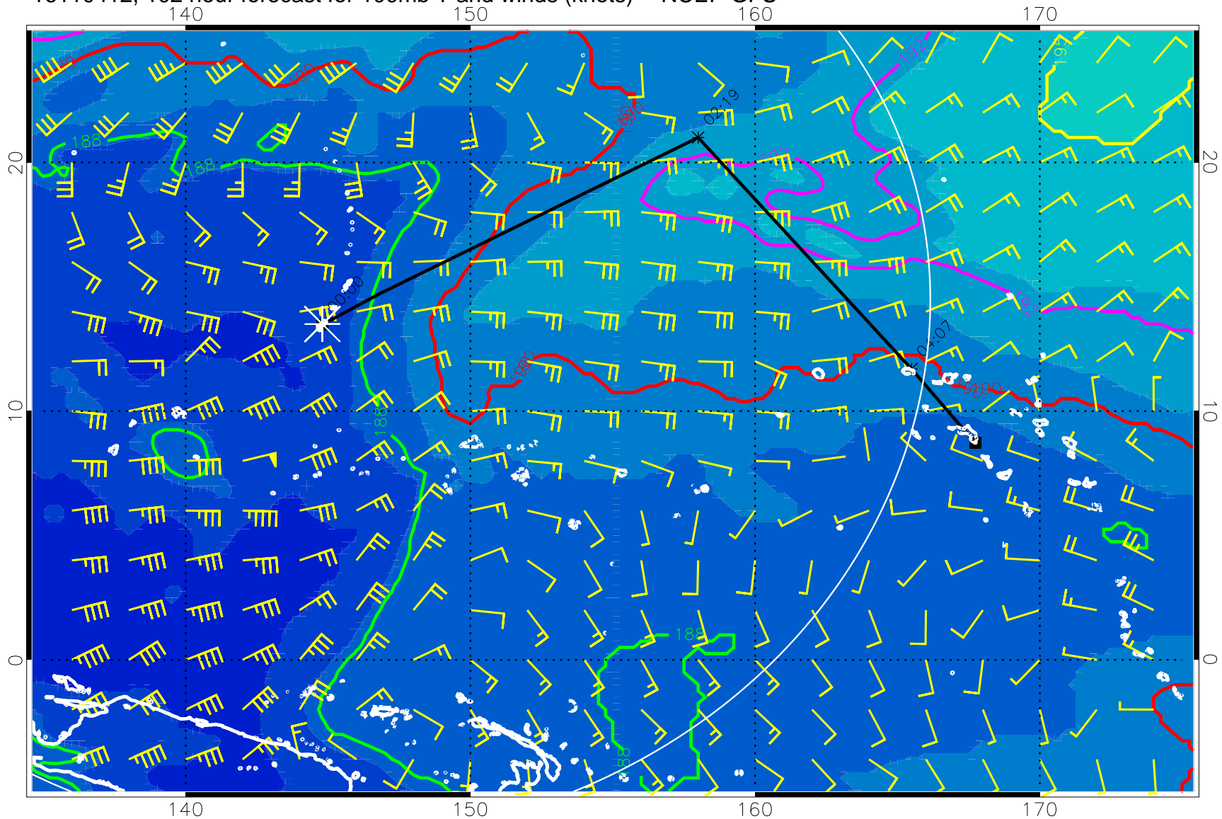
16110412, 102 hour forecast for 100mb T and winds (knots) -- NCEP GFS
