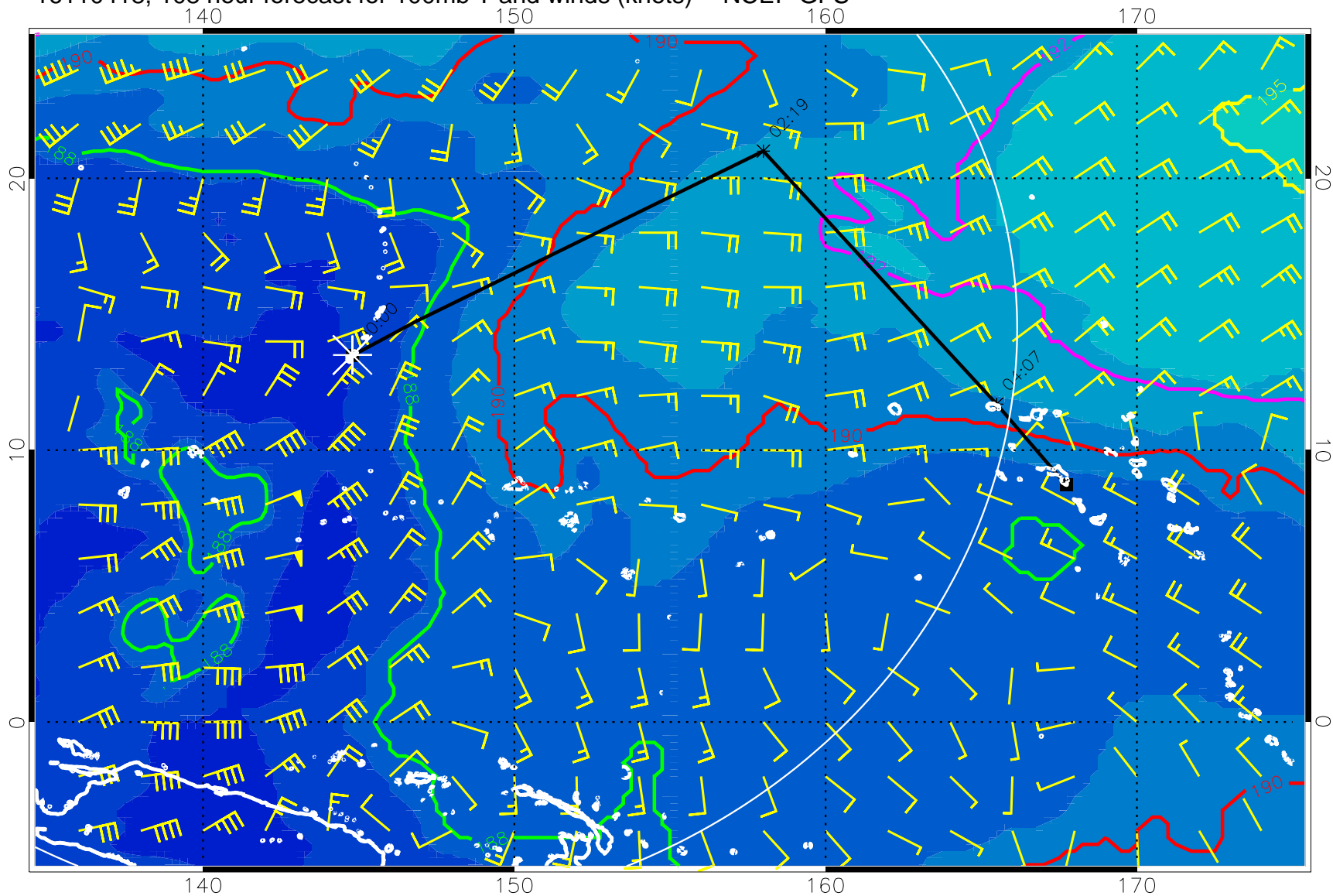
16110418, 108 hour forecast for 100mb T and winds (knots) -- NCEP GFS
