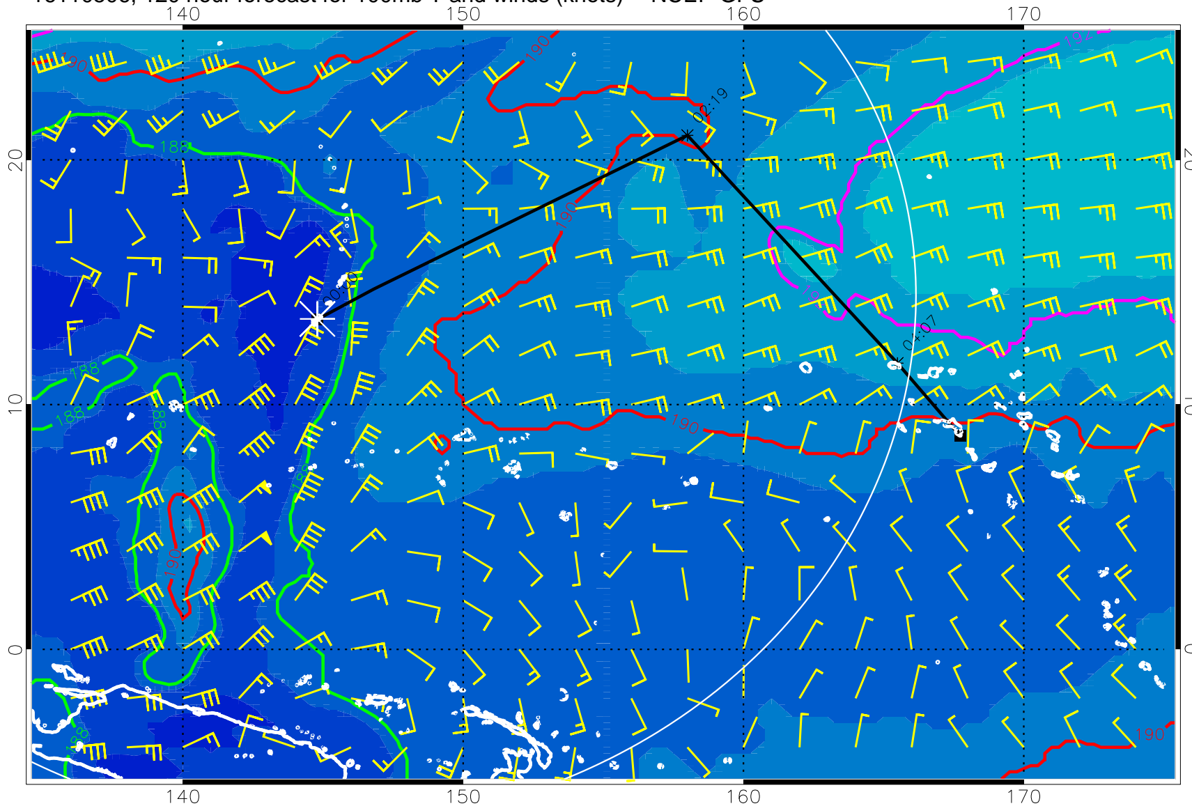
16110506, 120 hour forecast for 100mb T and winds (knots) -- NCEP GFS
