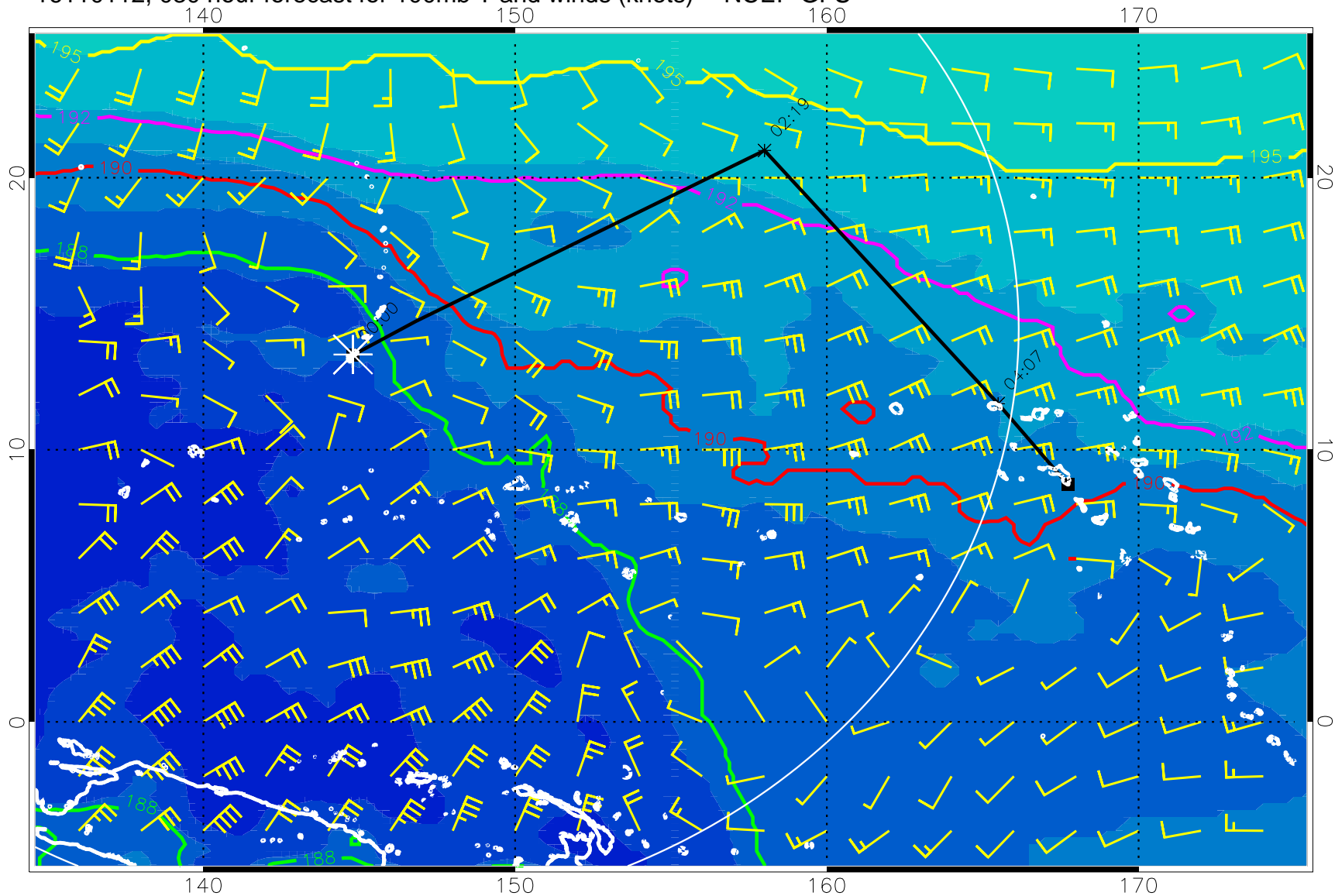
16110112, 0300 hour forecast for 100mb T and winds (knots) -- NCEP GFS
