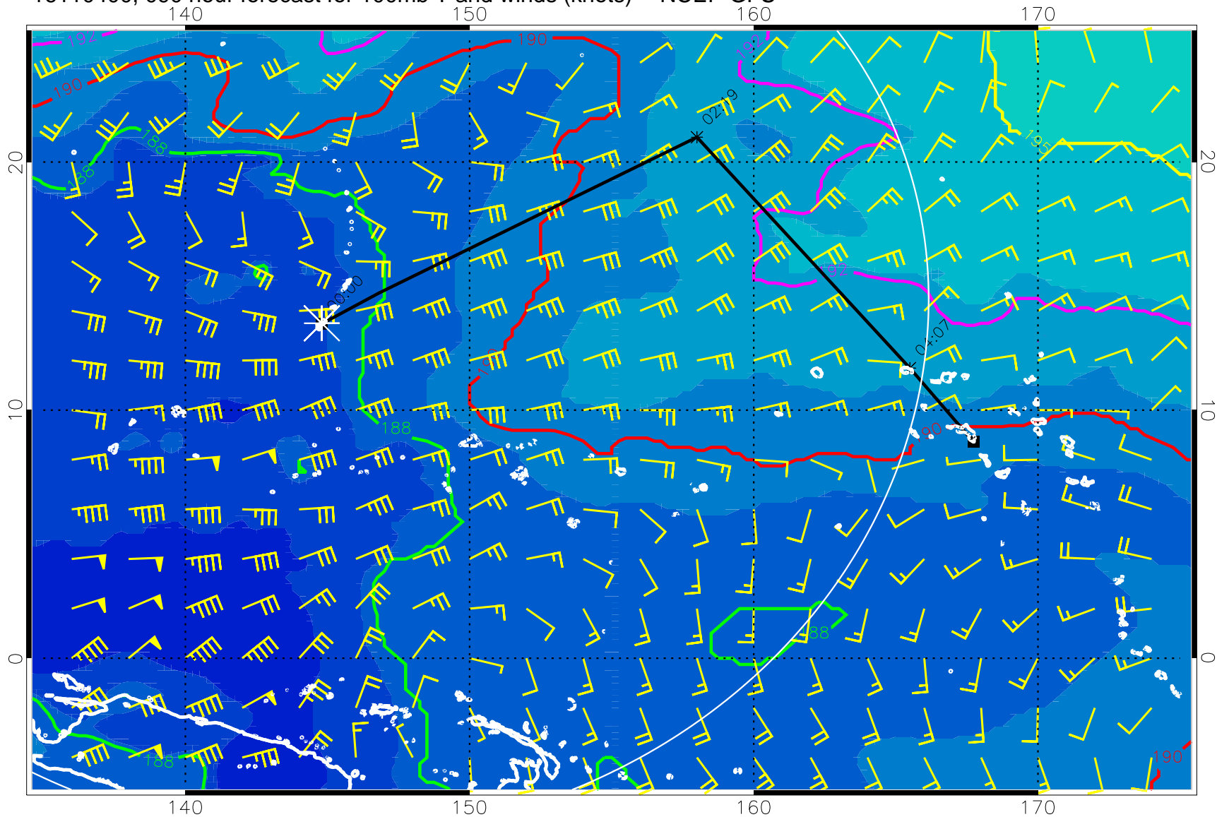
16110400, 090 hour forecast for 100mb T and winds (knots) -- NCEP GFS
