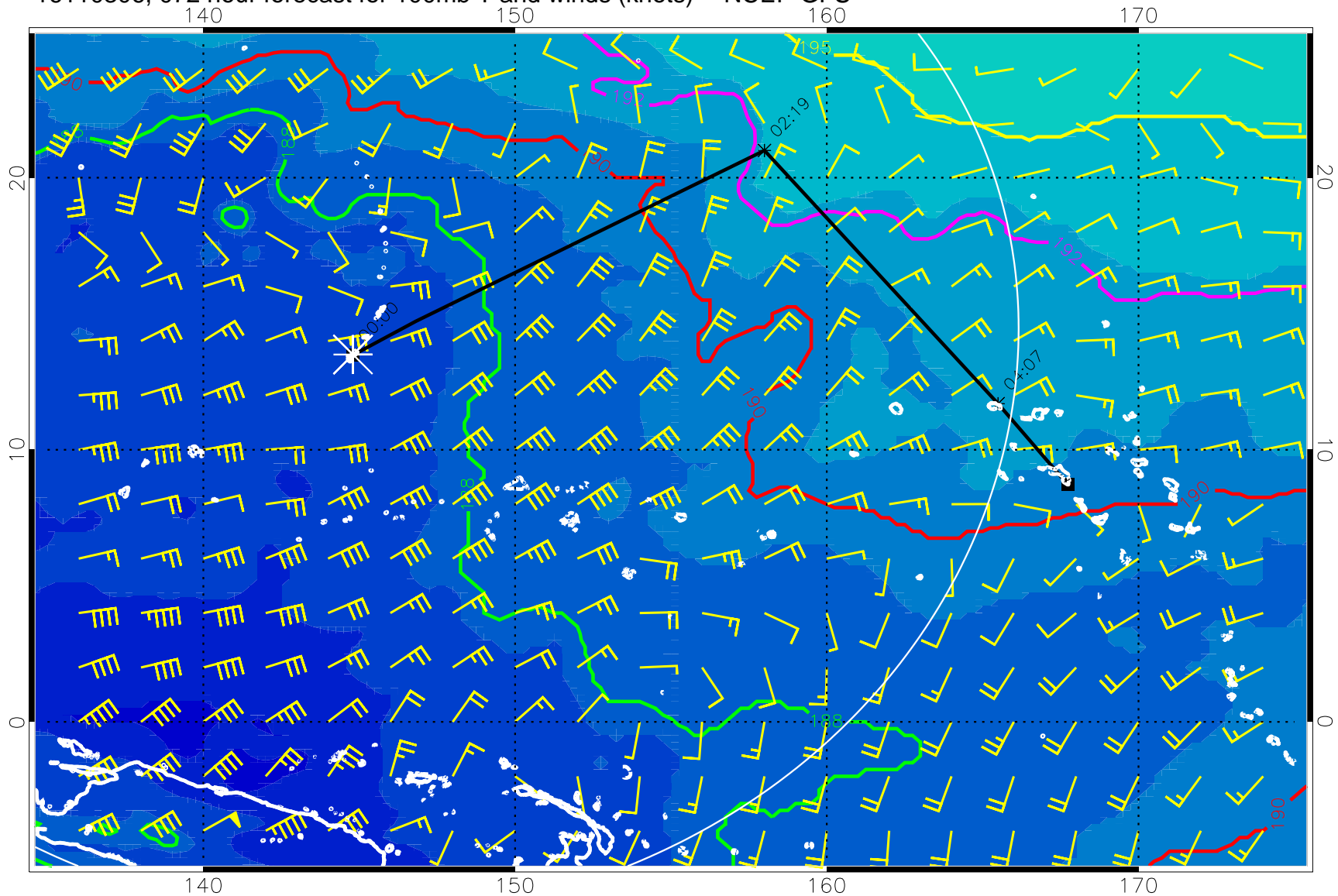
16110306, 072 hour forecast for 100mb T and winds (knots) -- NCEP GFS
