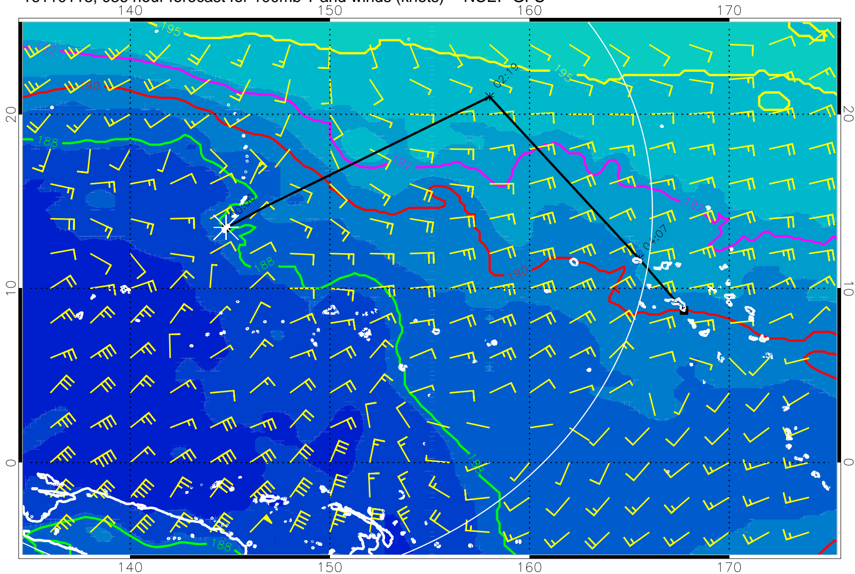
16110118, 036 hour forecast for 100mb T and winds (knots) -- NCEP GFS
