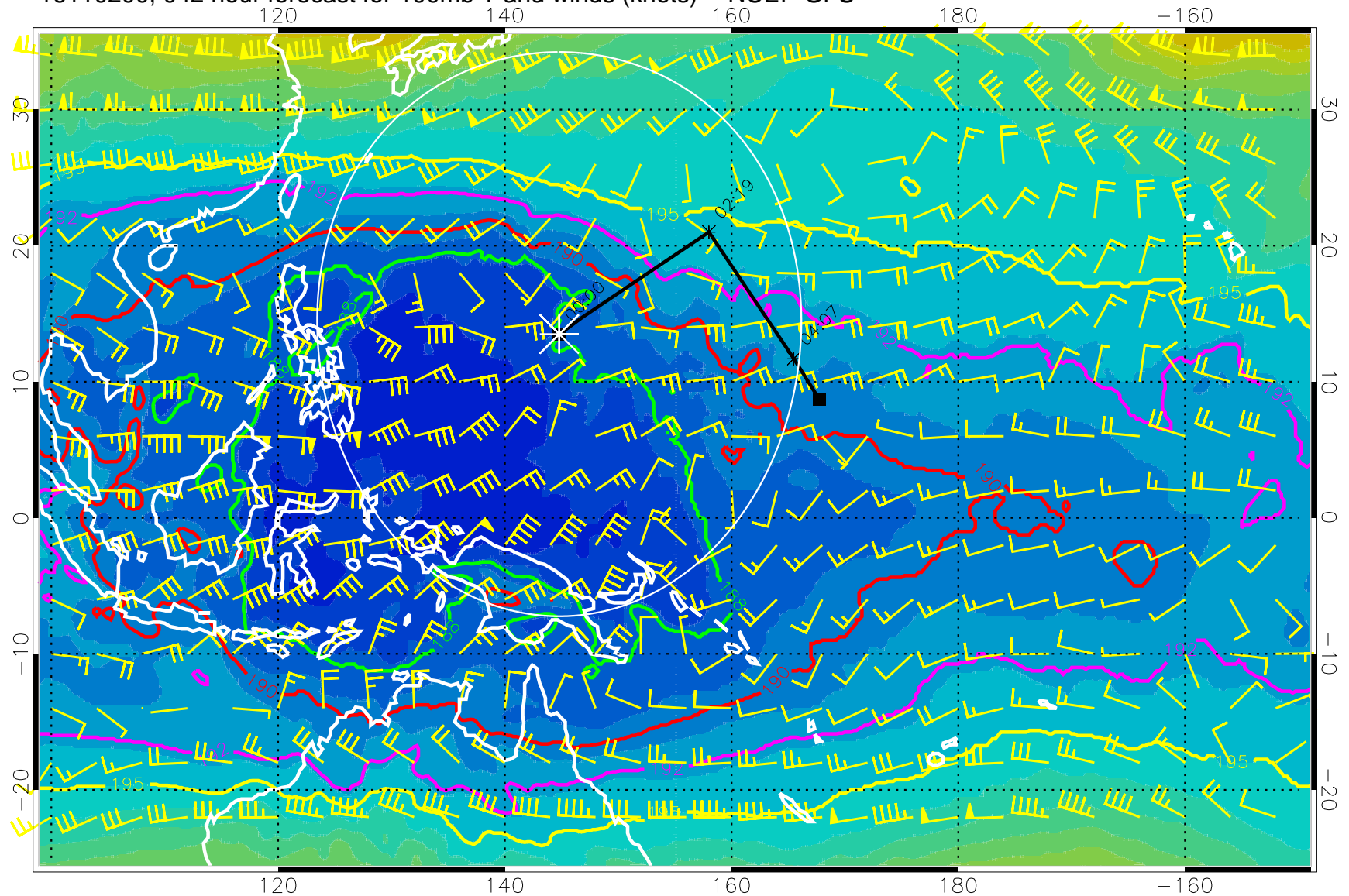
16110200, 042 hour forecast for 100mb T and winds (knots) -- NCEP GFS
