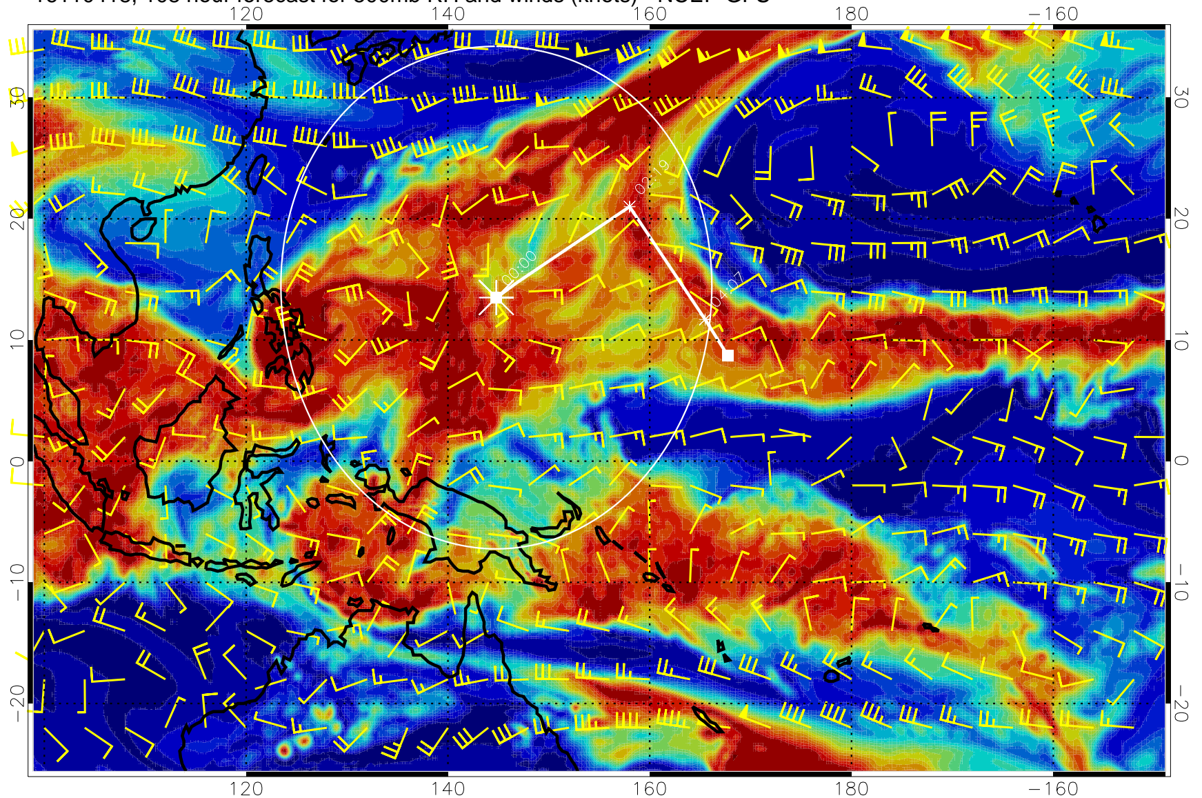
16110418, 108 hour forecast for 500mb RH and winds (knots) - NCEP GFS
