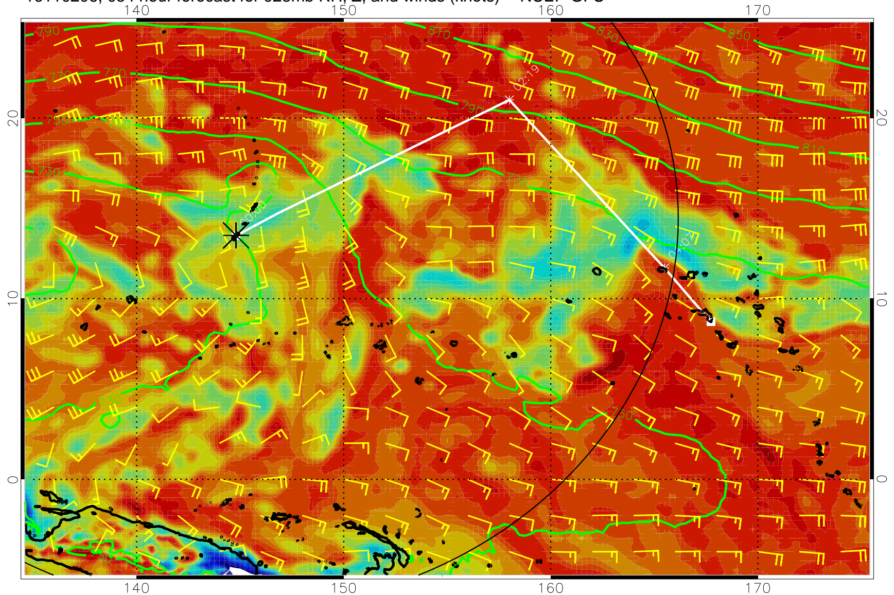
16110206, 054 hour forecast for 925mb RH, Z, and winds (knots) -- NCEP GFS
