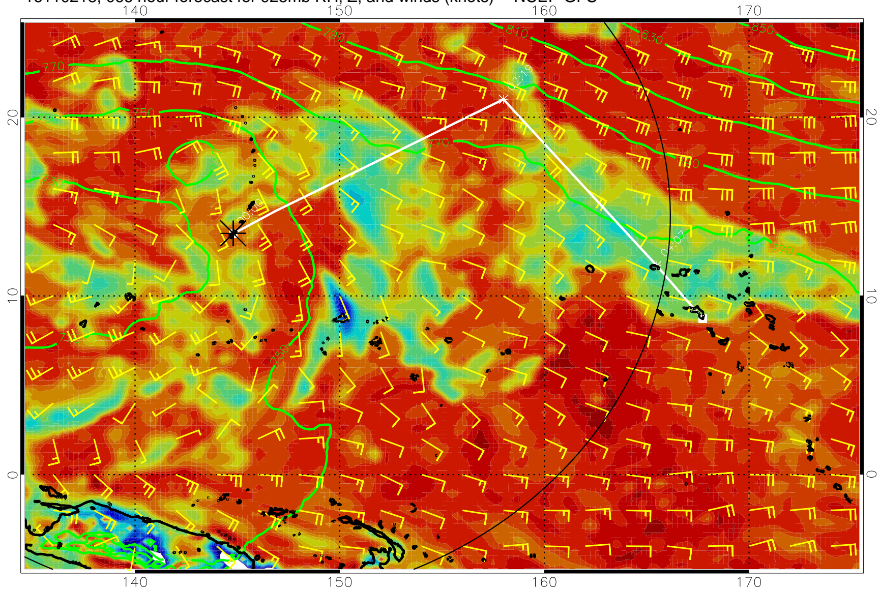
16110218, 066 hour forecast for 925mb RH, Z, and winds (knots) -- NCEP GFS
