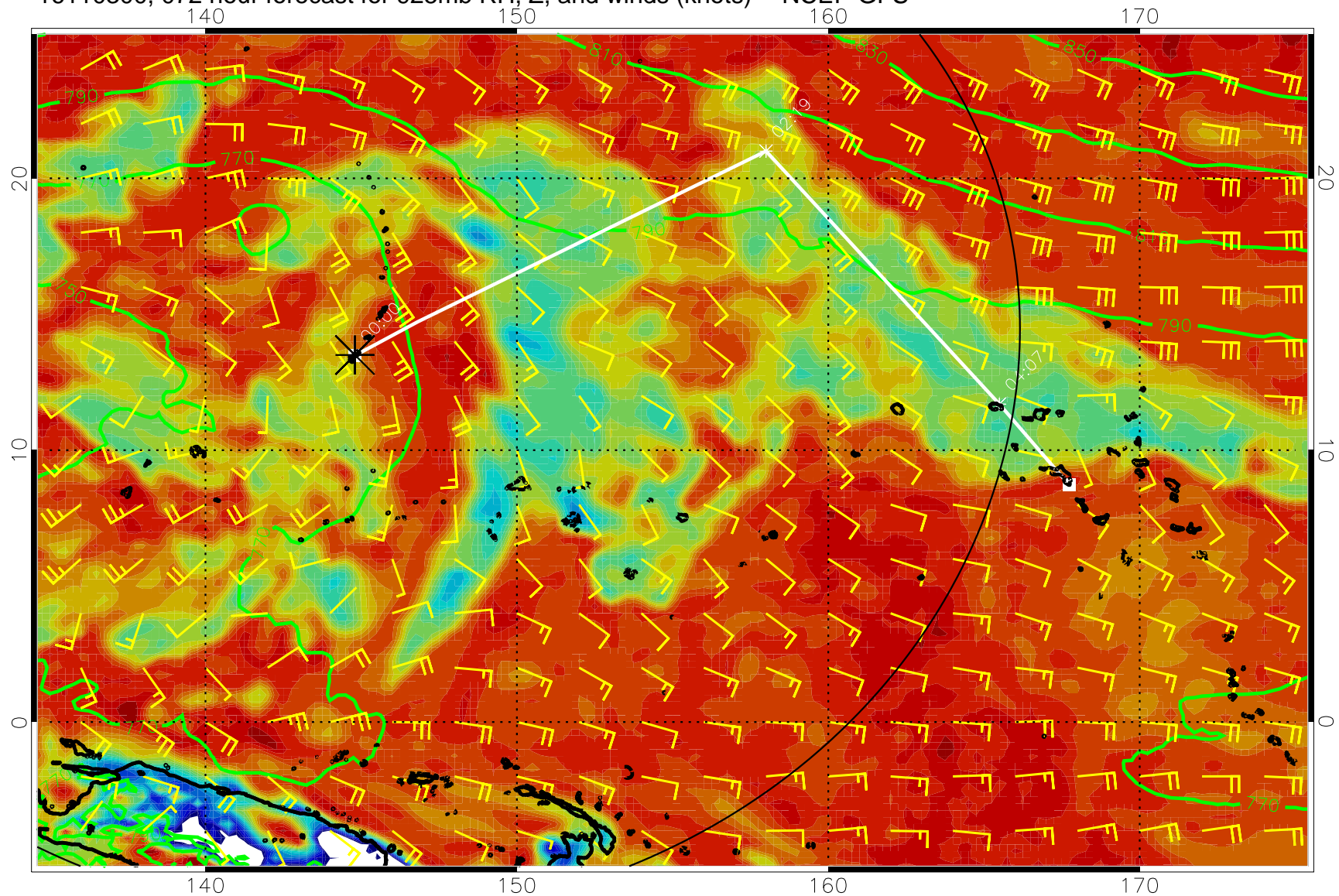
16110300, 072 hour forecast for 925mb RH, Z, and winds (knots) -- NCEP GFS
