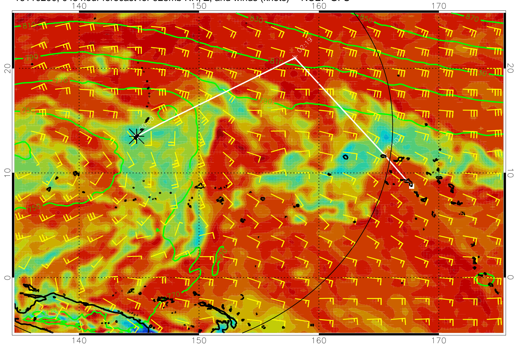
16110200, 048 hour forecast for 925mb RH, Z, and winds (knots) -- NCEP GFS
