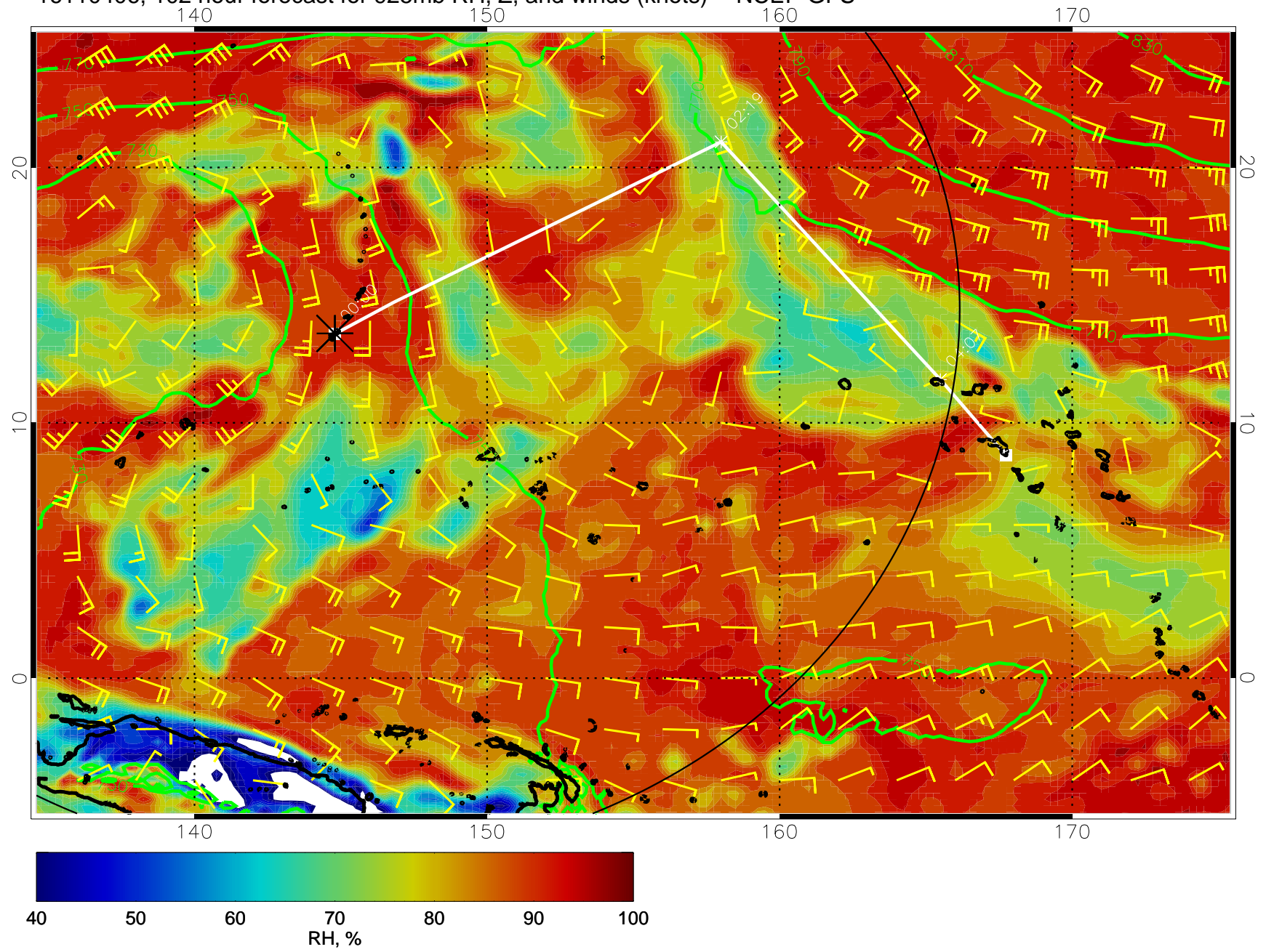
16110406, 102 hour forecast for 925mb RH, Z, and winds (knots) -- NCEP GFS
