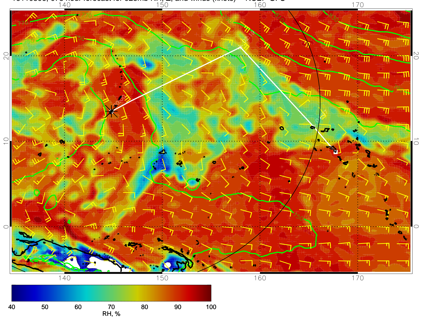
16110306, 078 hour forecast for 925mb RH, Z, and winds (knots) -- NCEP GFS
