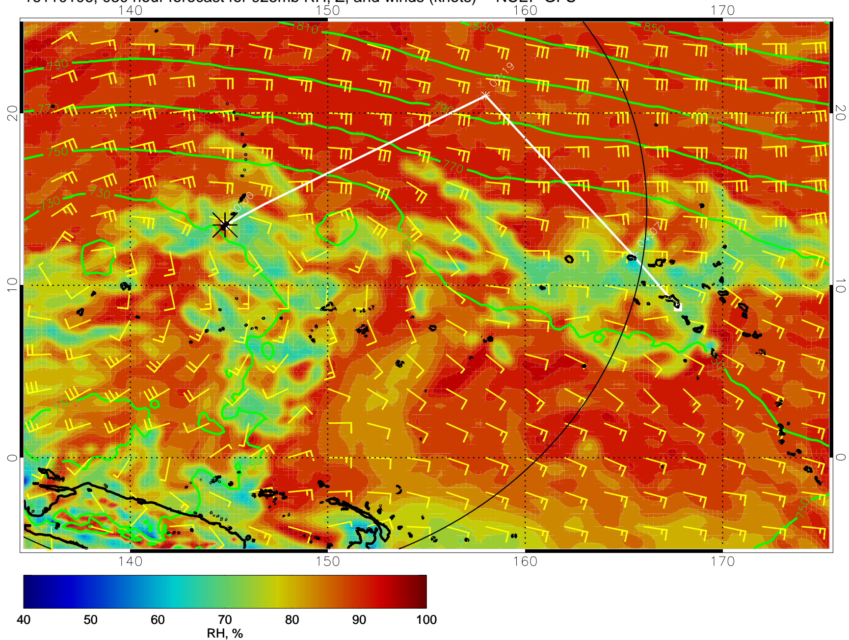
16110106, 030 hour forecast for 925mb RH, Z, and winds (knots) -- NCEP GFS
