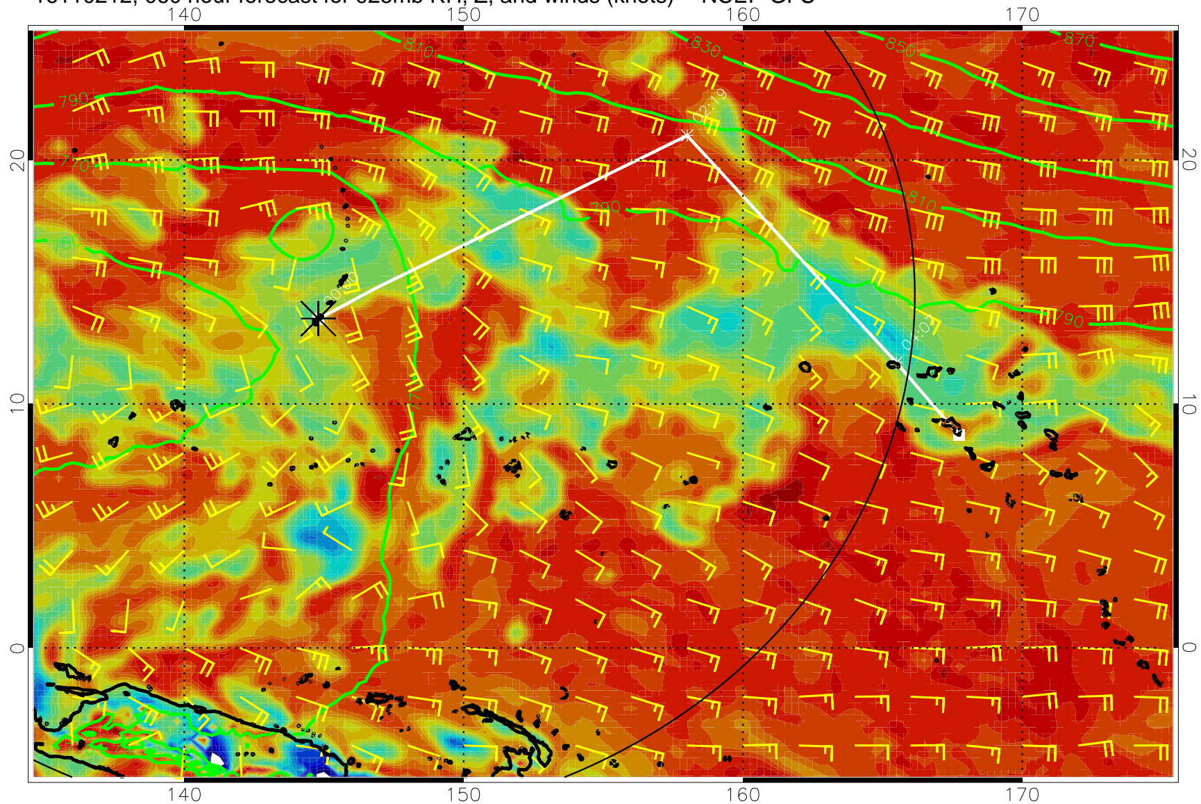
16110212, 060 hour forecast for 925mb RH, Z, and winds (knots) -- NCEP GFS
