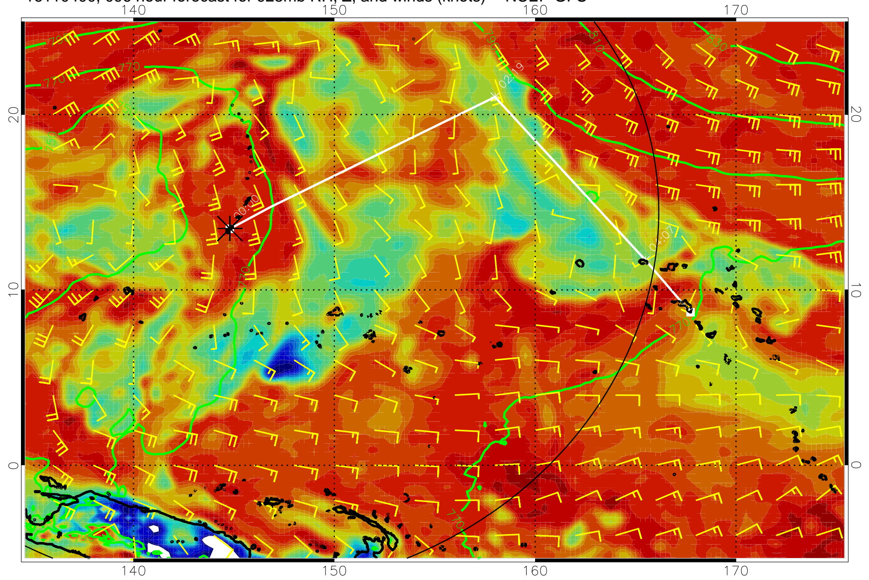
16110400, 096 hour forecast for 925mb RH, Z, and winds (knots) -- NCEP GFS
