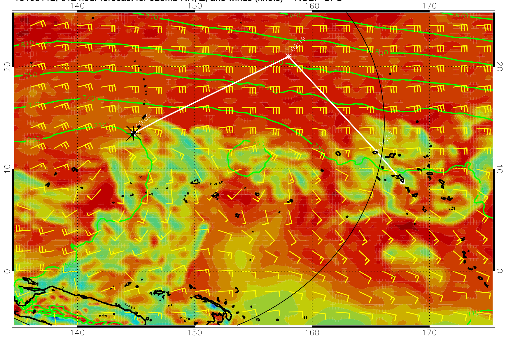
16103112, 012 hour forecast for 925mb RH, Z, and winds (knots) -- NCEP GFS
