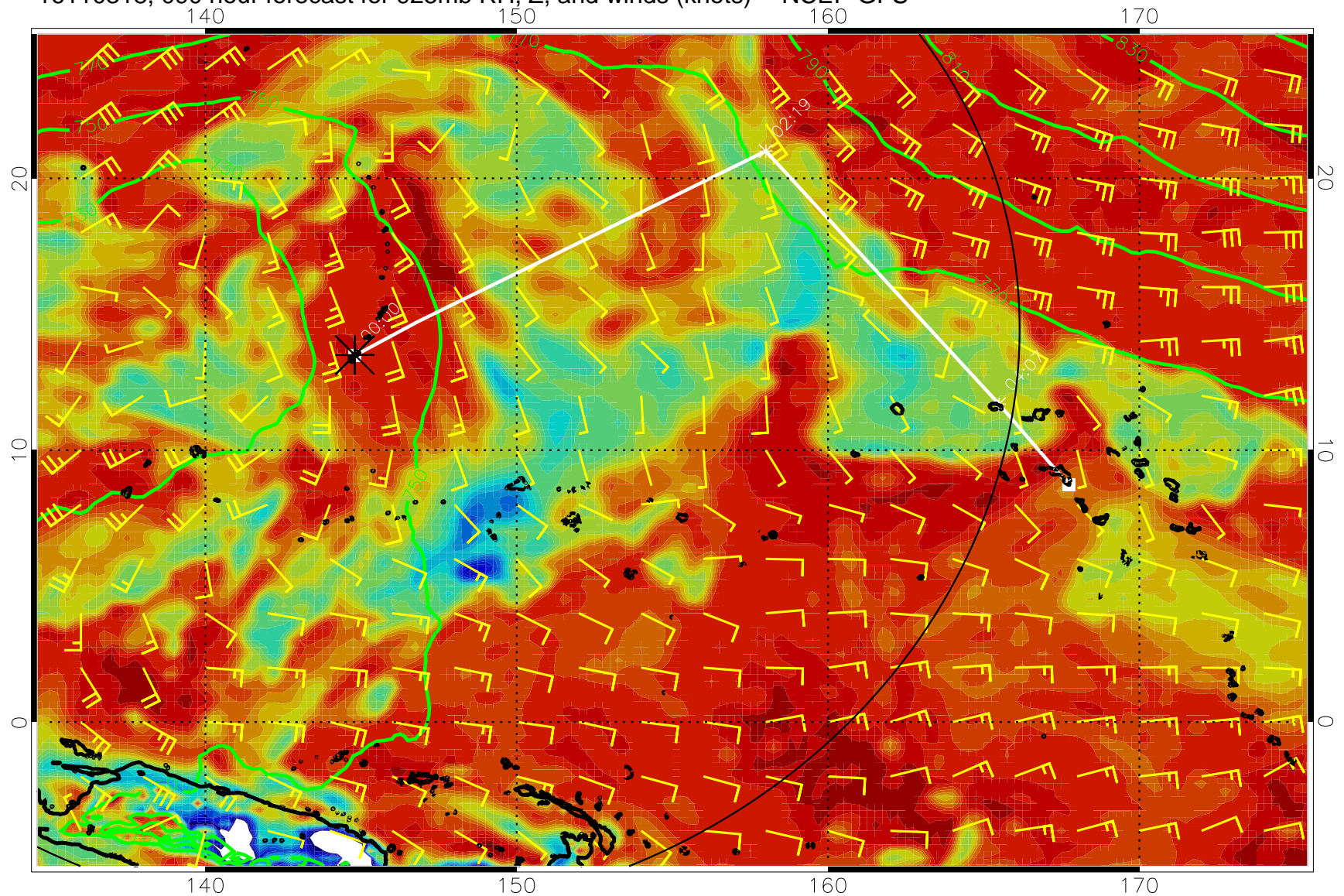
16110318, 090 hour forecast for 925mb RH, Z, and winds (knots) -- NCEP GFS
