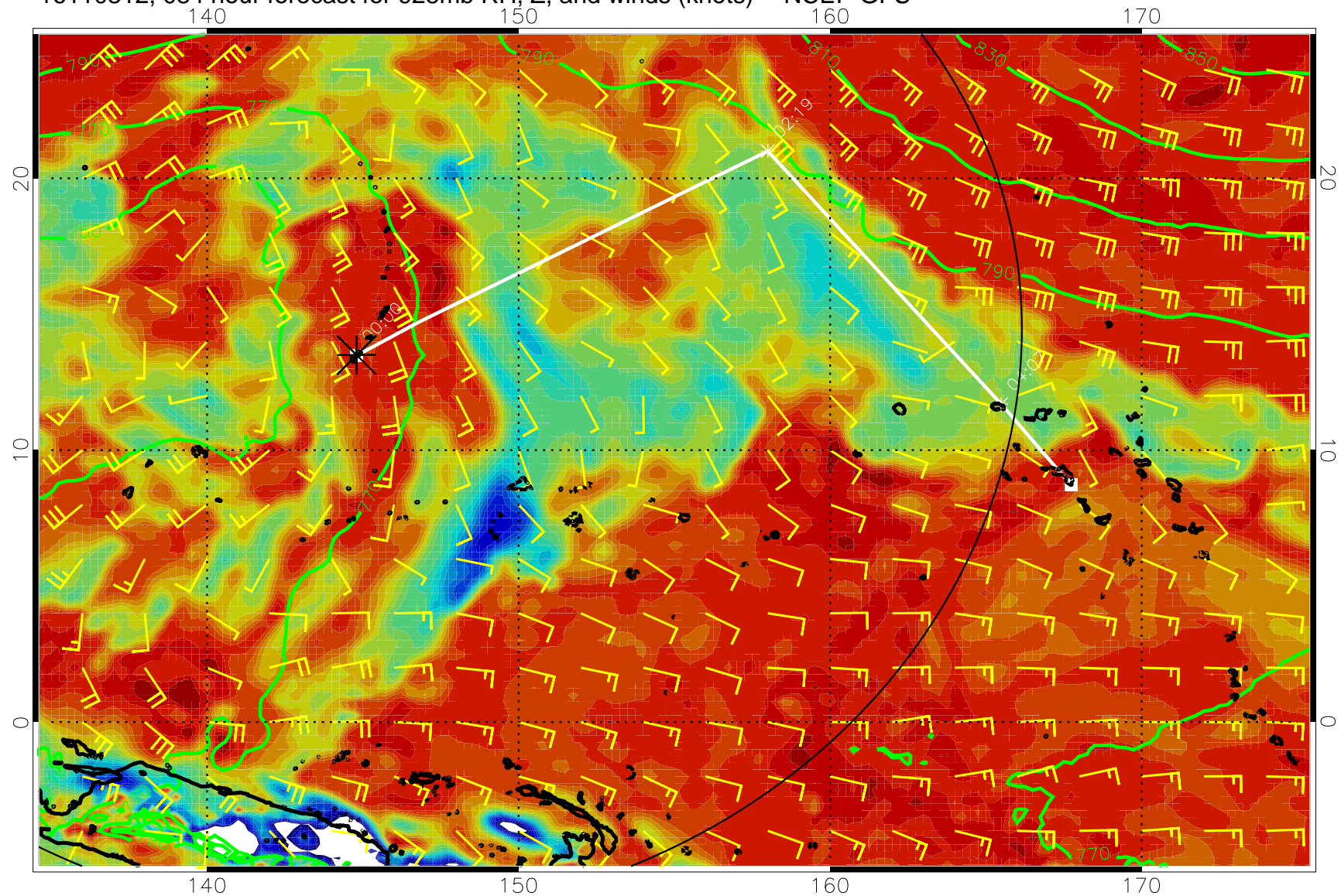
16110312, 084 hour forecast for 925mb RH, Z, and winds (knots) -- NCEP GFS
