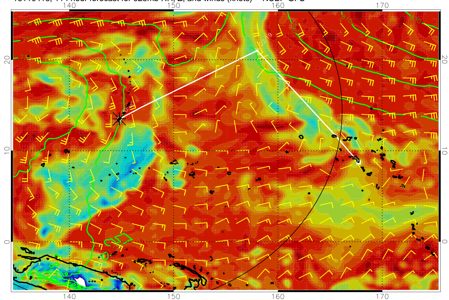
16110418, 114 hour forecast for 925mb RH, Z, and winds (knots) -- NCEP GFS
