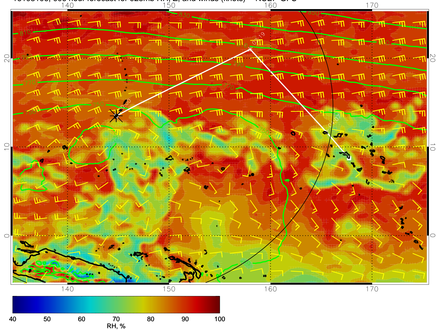
16103106, 006 hour forecast for 925mb RH, Z, and winds (knots) -- NCEP GFS
