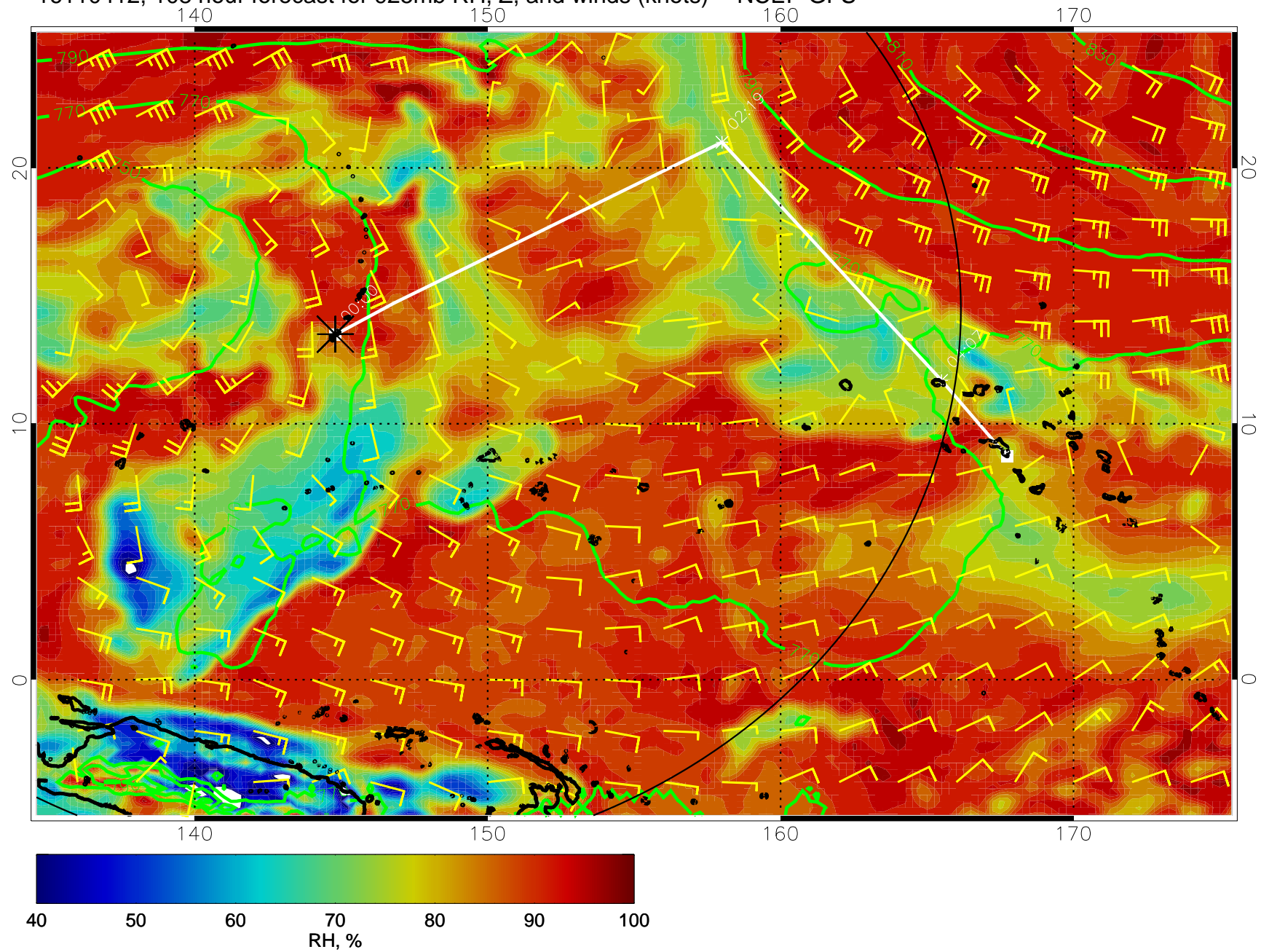
16110412, 108 hour forecast for 925mb RH, Z, and winds (knots) -- NCEP GFS
