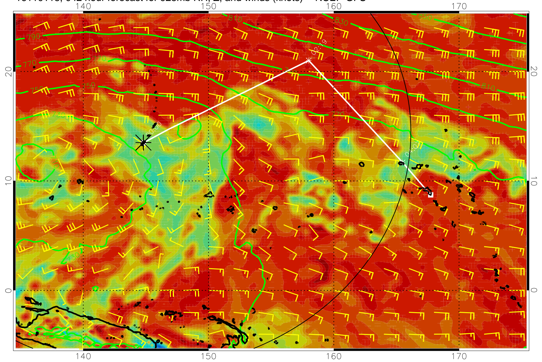
16110118, 042 hour forecast for 925mb RH, Z, and winds (knots) -- NCEP GFS
