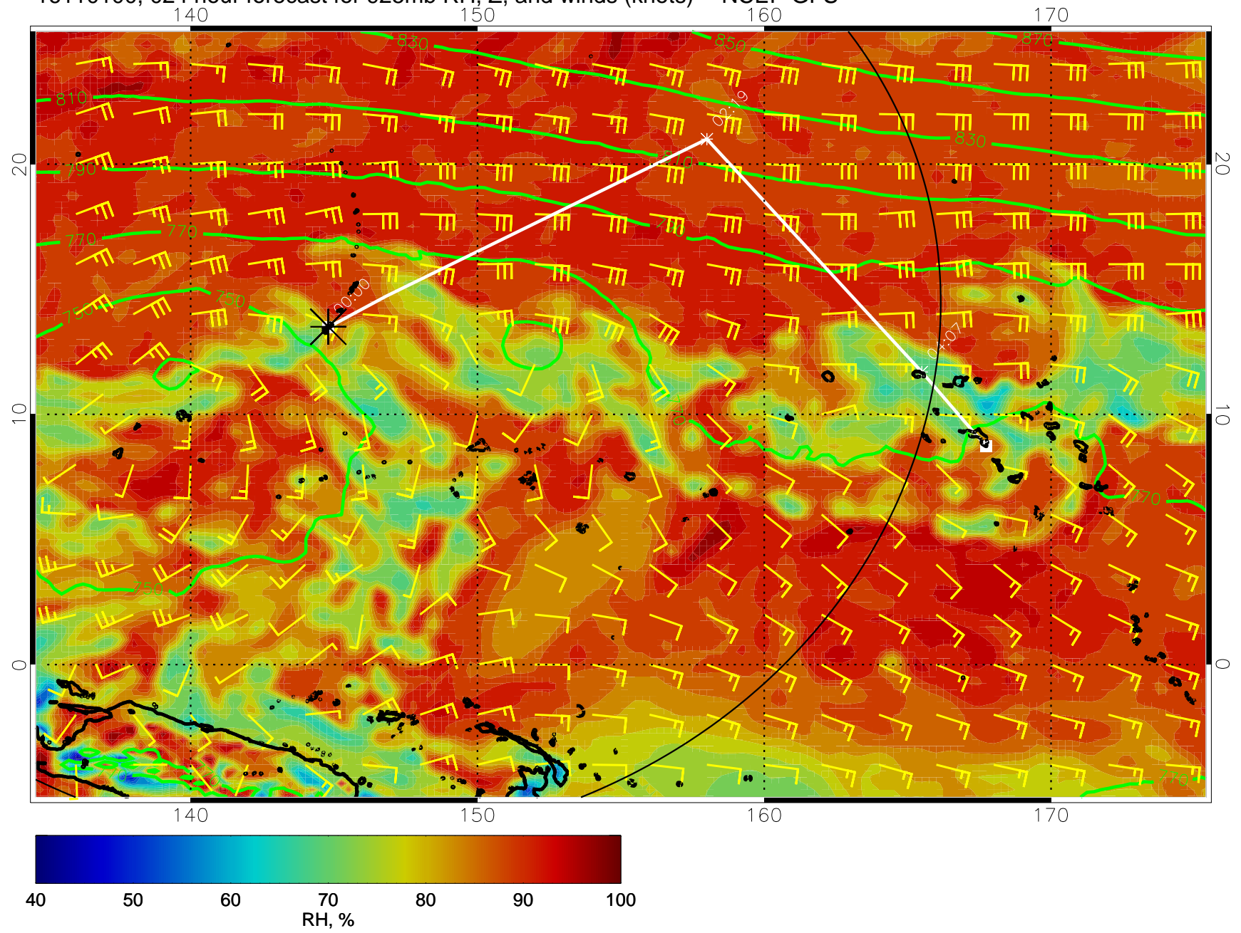
16110100, 024 hour forecast for 925mb RH, Z, and winds (knots) -- NCEP GFS
