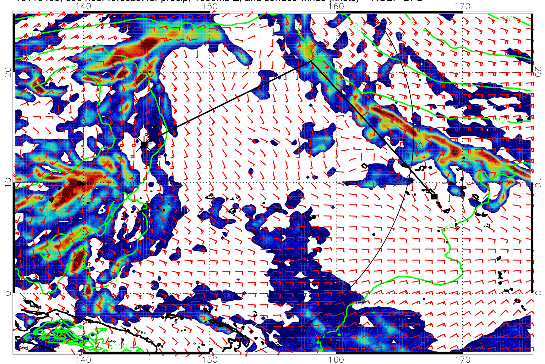
16110400, 096 hour forecast for precip, 1000mb Z, and surface winds (knots) -- NCEP GFS
