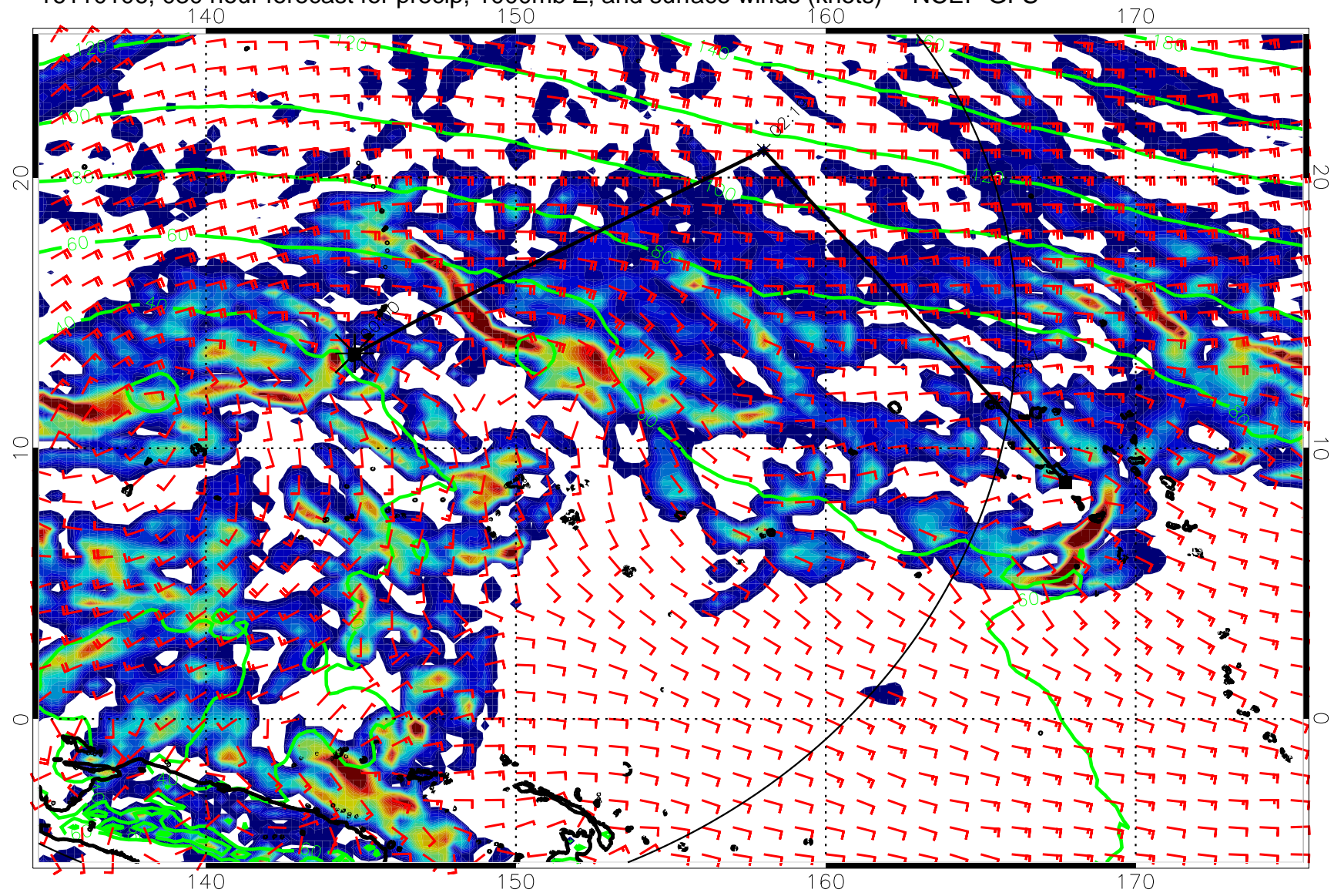
16110106, 030 hour forecast for precip, 1000mb Z, and surface winds (knots) -- NCEP GFS
