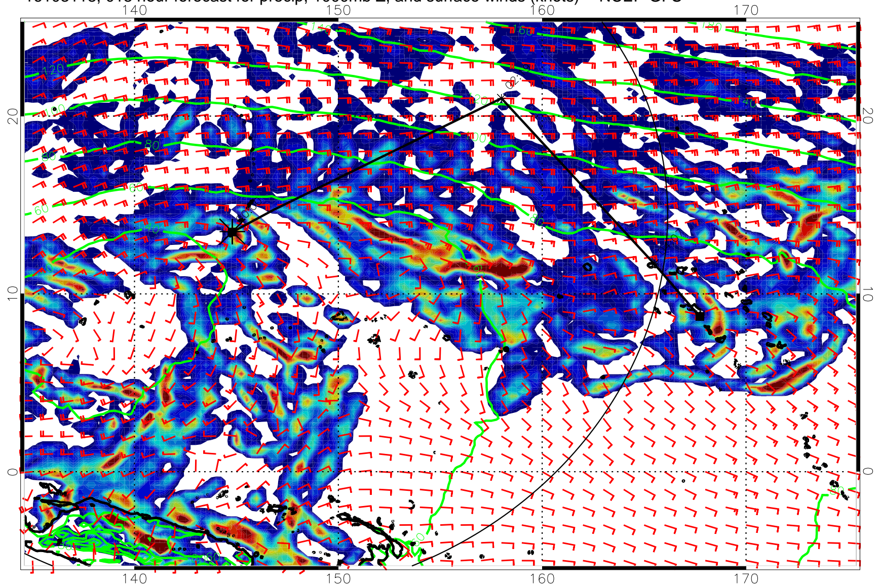
16103118, 018 hour forecast for precip, 1000mb Z, and surface winds (knots) -- NCEP GFS
