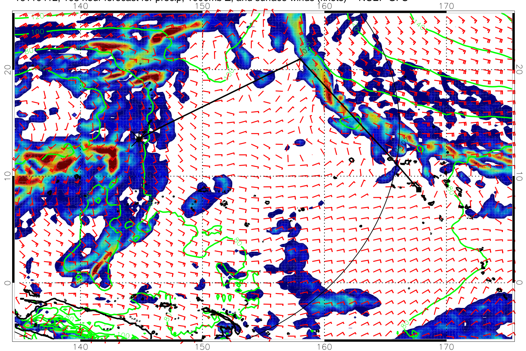
16110412, 108 hour forecast for precip, 1000mb Z, and surface winds (knots) -- NCEP GFS
