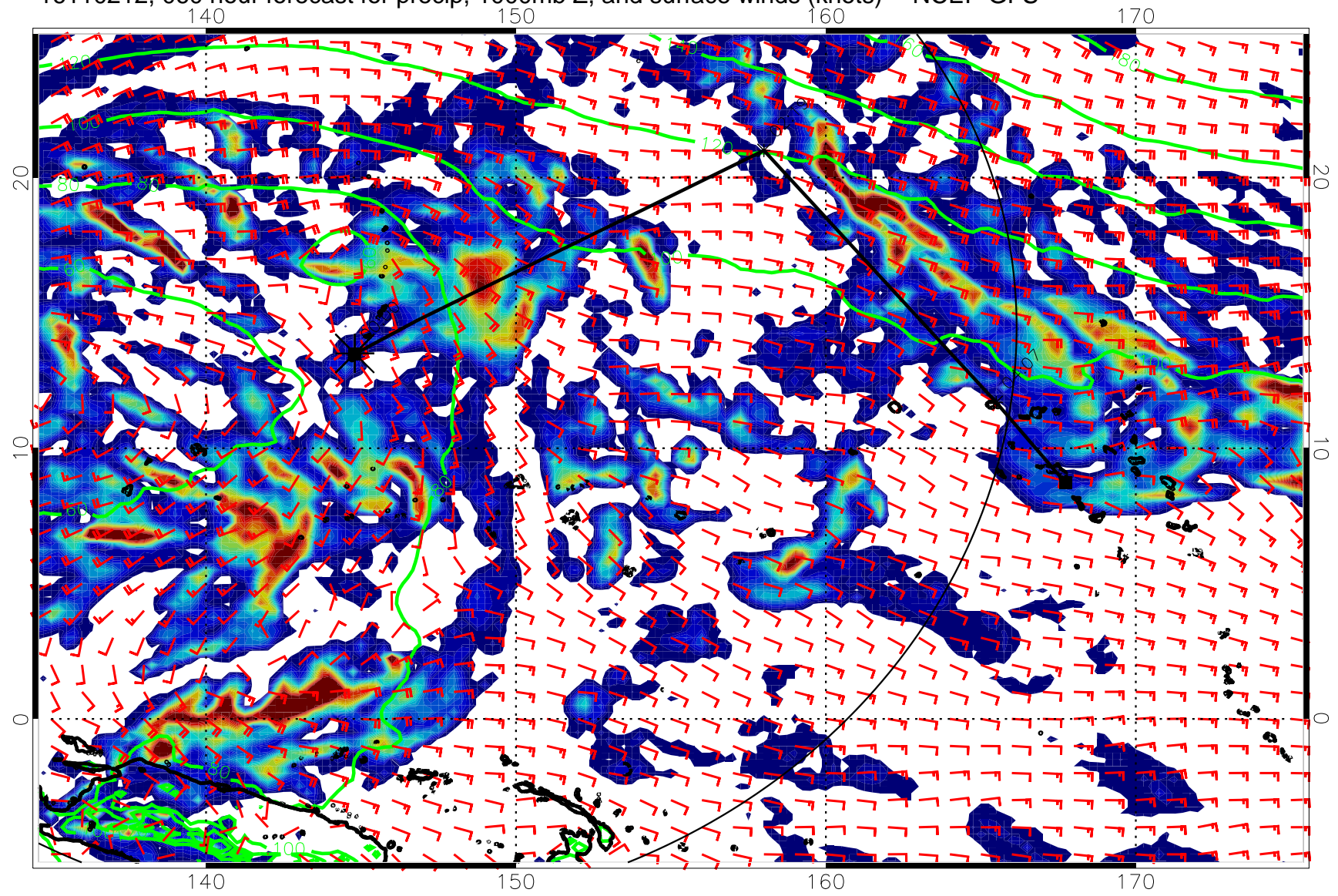
16110212, 060 hour forecast for precip, 1000mb Z, and surface winds (knots) -- NCEP GFS
