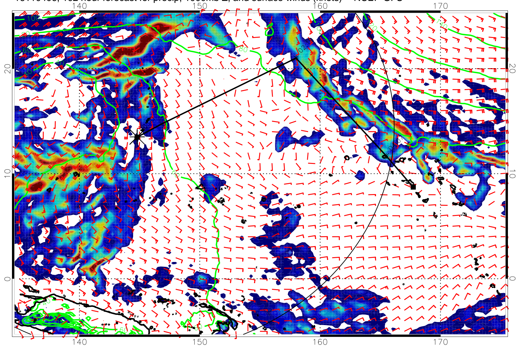
16110406, 102 hour forecast for precip, 1000mb Z, and surface winds (knots) -- NCEP GFS
