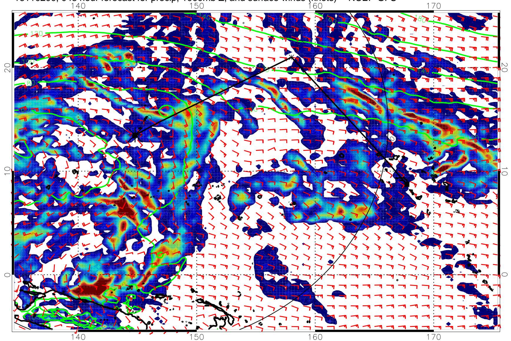
16110200, 048 hour forecast for precip, 1000mb Z, and surface winds (knots) -- NCEP GFS
