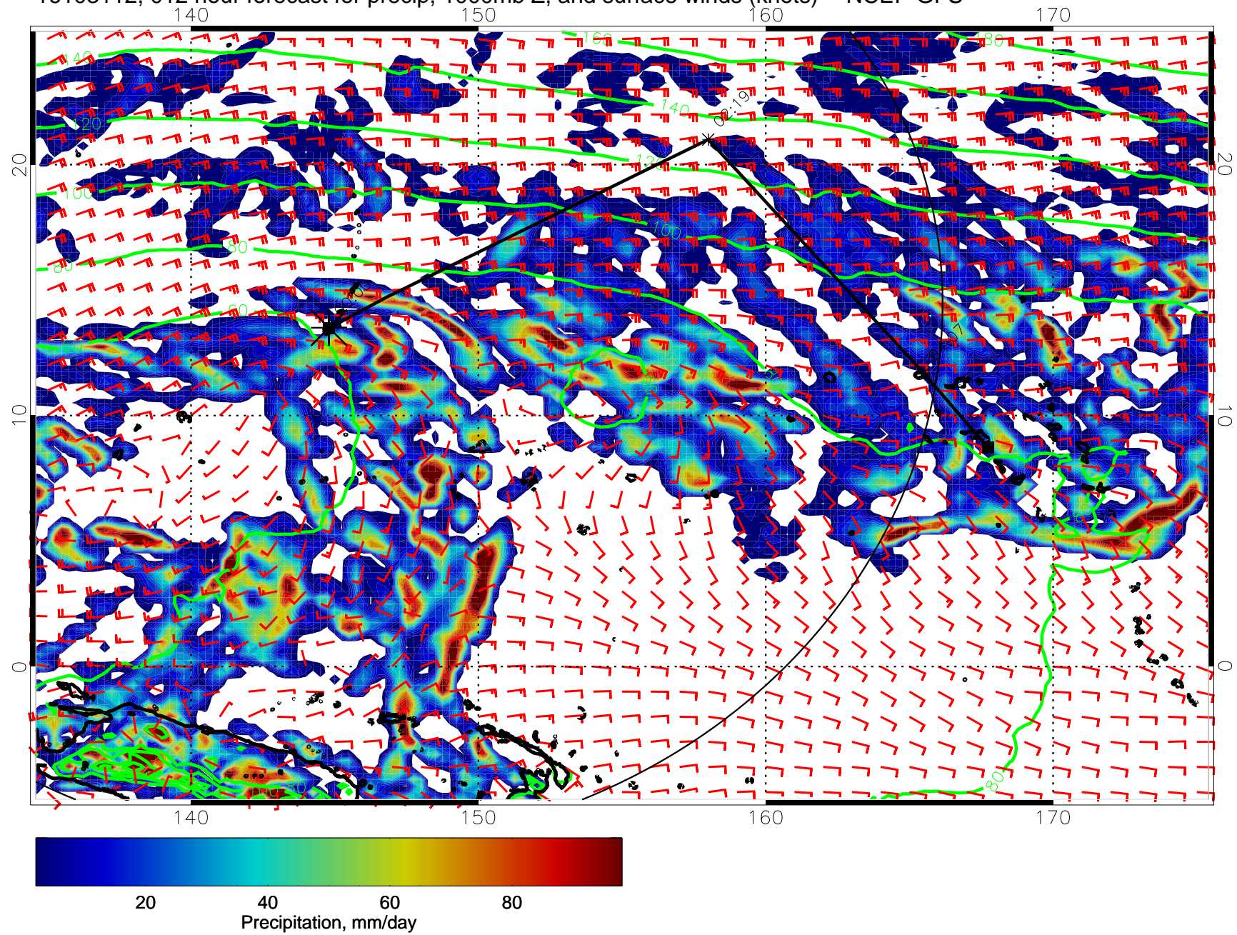
16103112, 012 hour forecast for precip, 1000mb Z, and surface winds (knots) -- NCEP GFS
