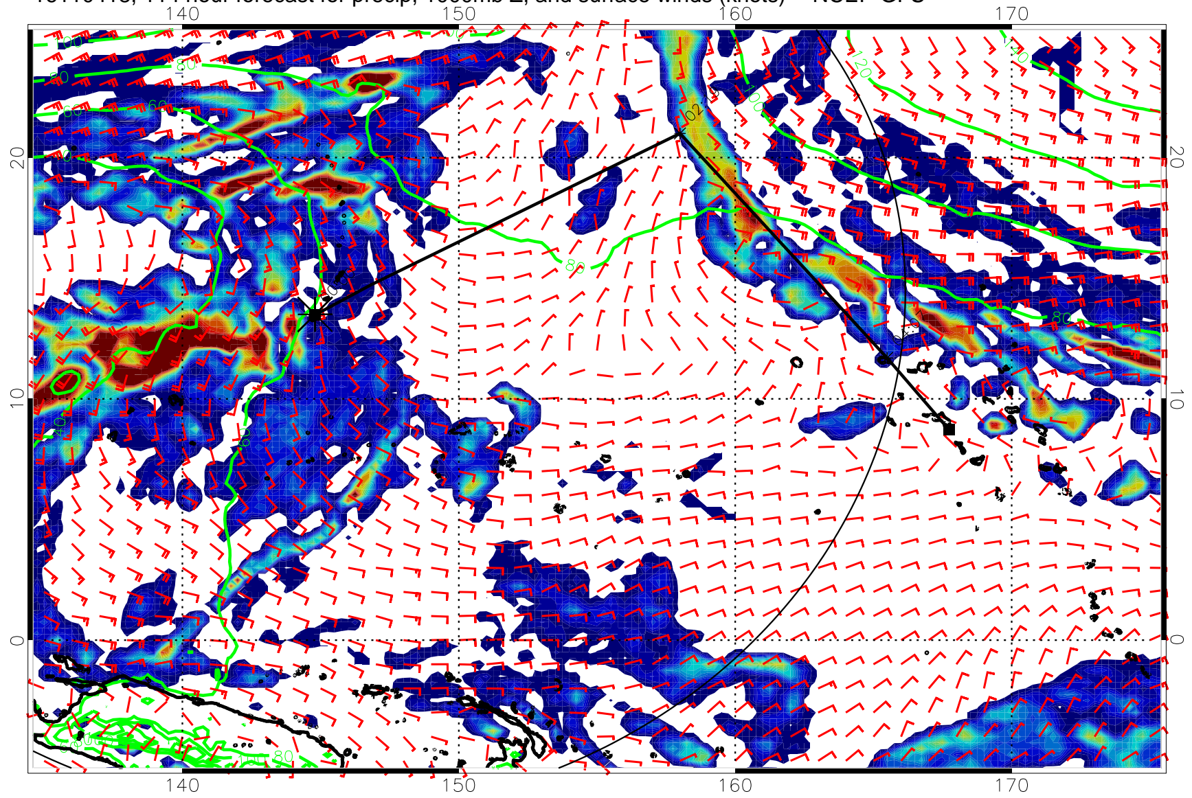
16110418, 114 hour forecast for precip, 1000mb Z, and surface winds (knots) -- NCEP GFS
