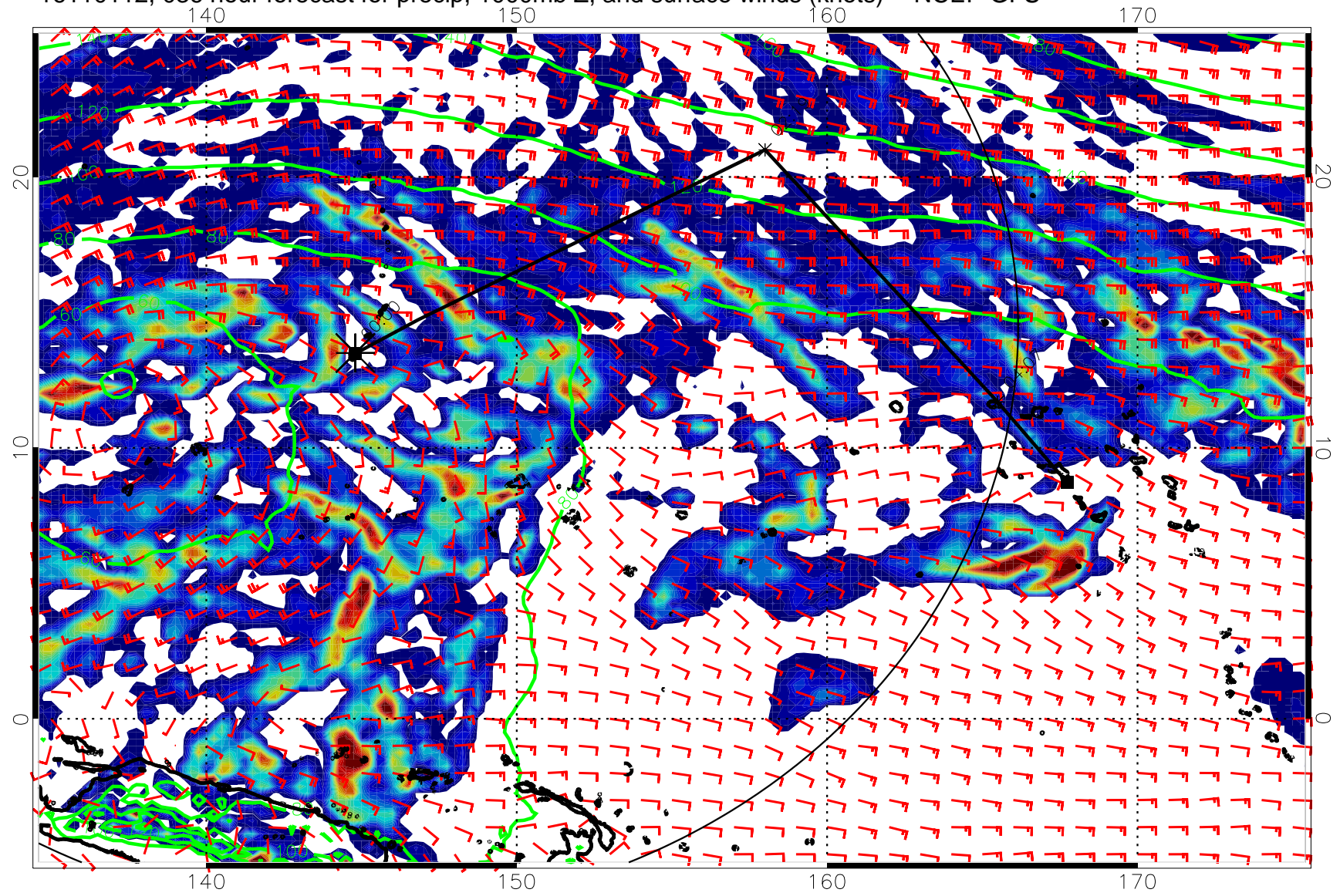
16110112, 036 hour forecast for precip, 1000mb Z, and surface winds (knots) -- NCEP GFS
