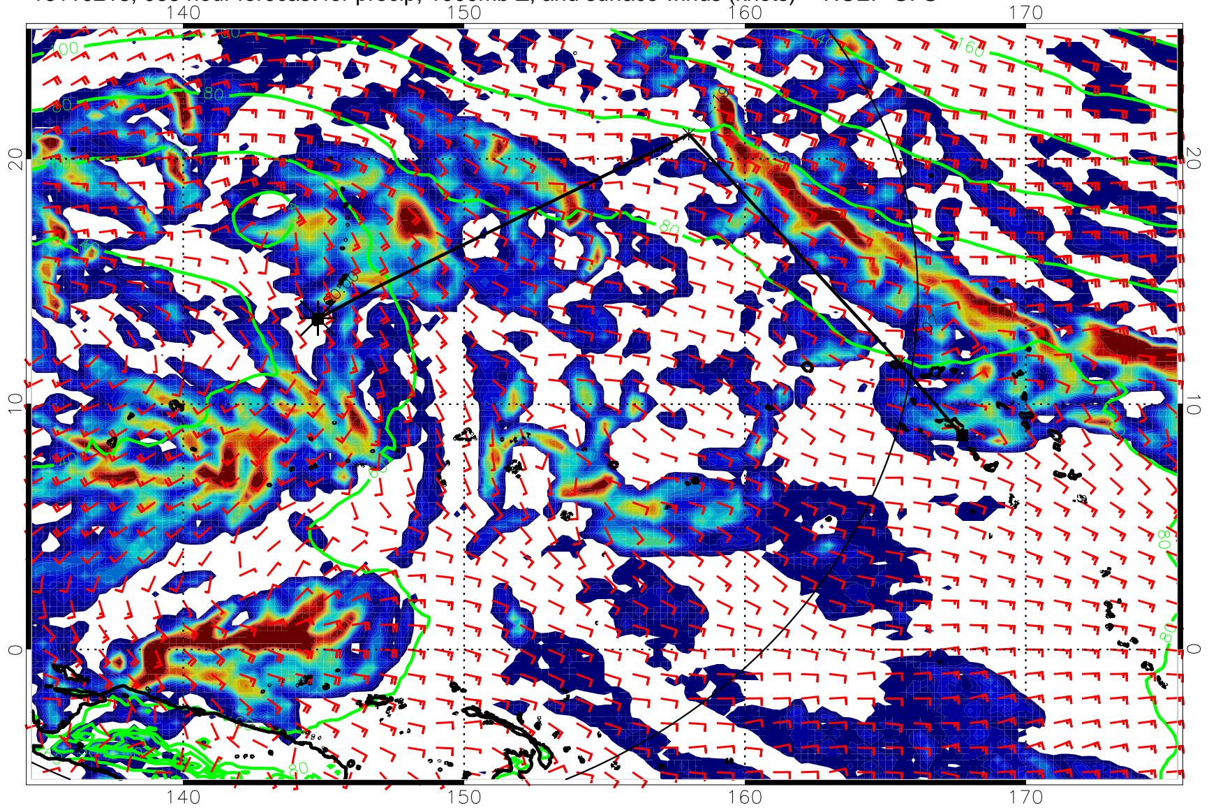
16110218, 066 hour forecast for precip, 1000mb Z, and surface winds (knots) -- NCEP GFS
