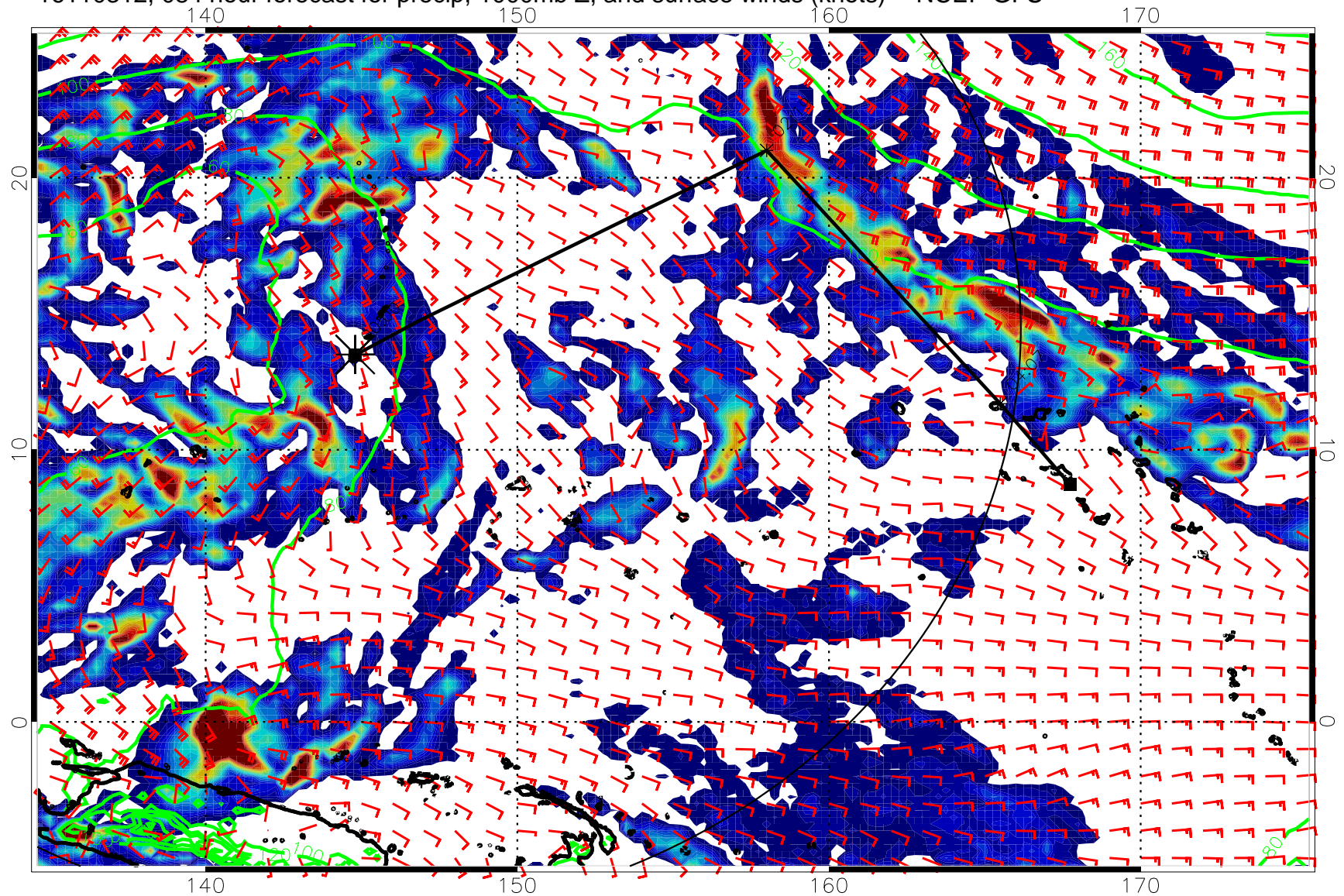
16110312, 084 hour forecast for precip, 1000mb Z, and surface winds (knots) -- NCEP GFS
