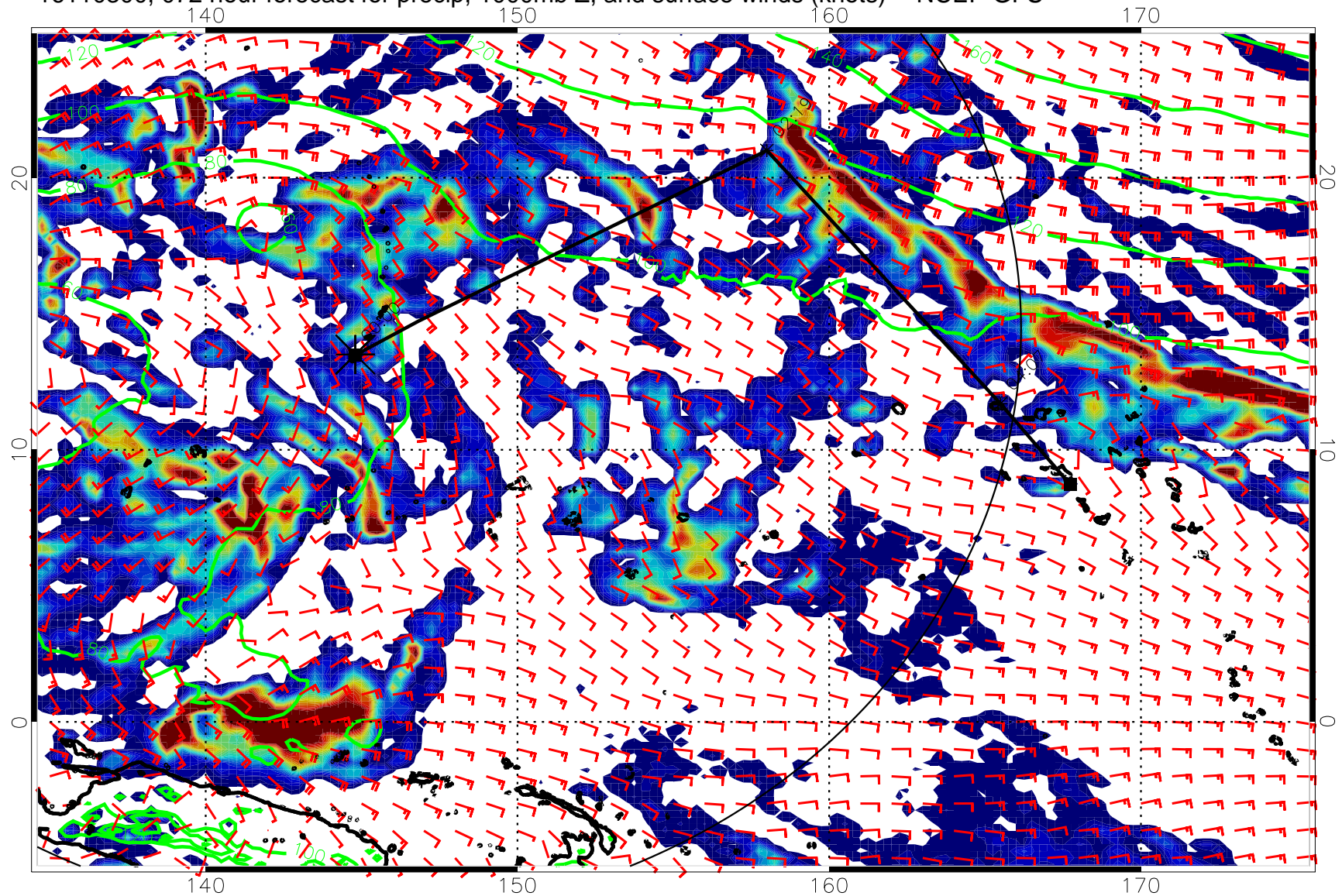
16110300, 072 hour forecast for precip, 1000mb Z, and surface winds (knots) -- NCEP GFS
