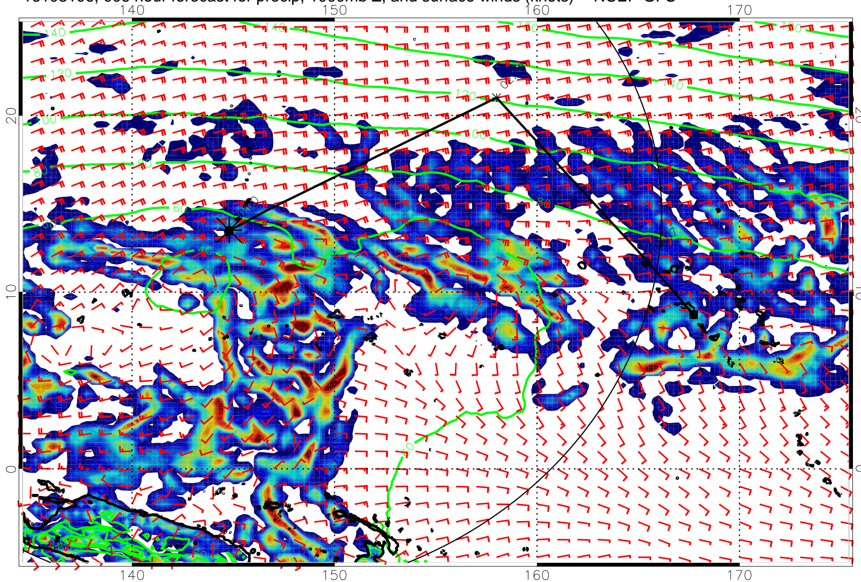
16103106, 006 hour forecast for precip, 1000mb Z, and surface winds (knots) -- NCEP GFS
