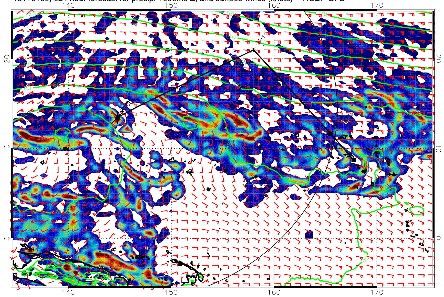
16110100, 024 hour forecast for precip, 1000mb Z, and surface winds (knots) -- NCEP GFS
