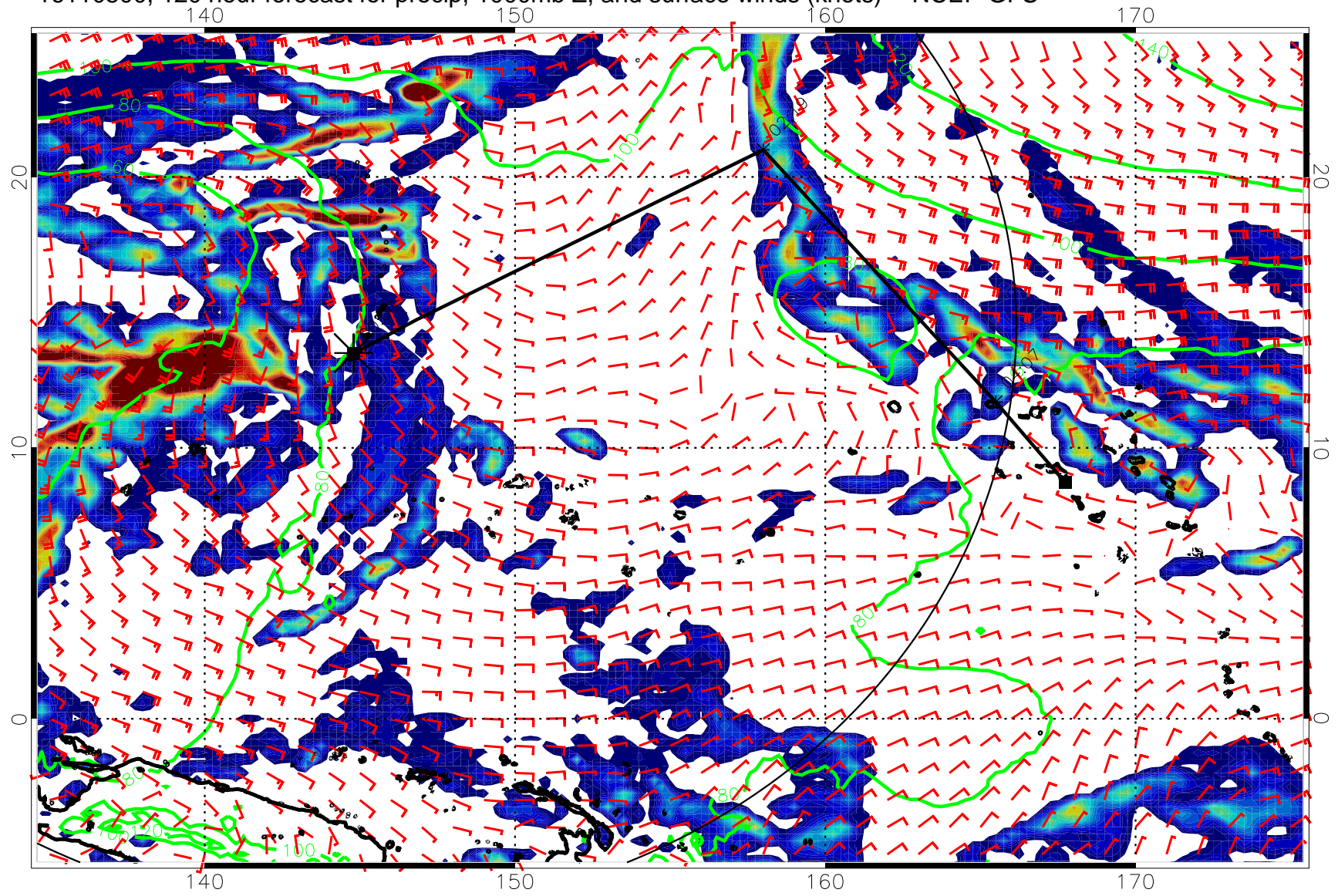
16110500, 120 hour forecast for precip, 1000mb Z, and surface winds (knots) -- NCEP GFS
