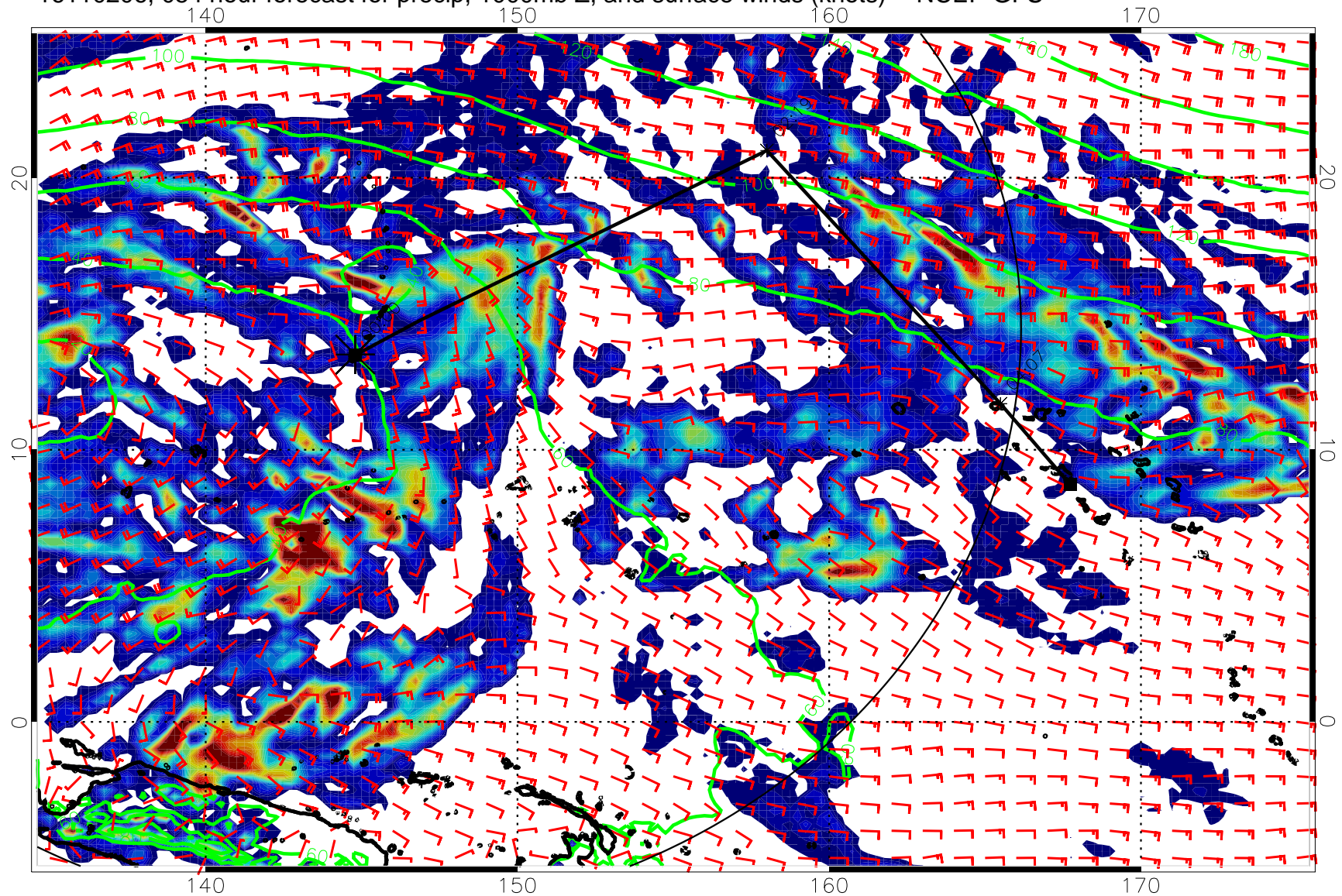
16110206, 054 hour forecast for precip, 1000mb Z, and surface winds (knots) -- NCEP GFS
