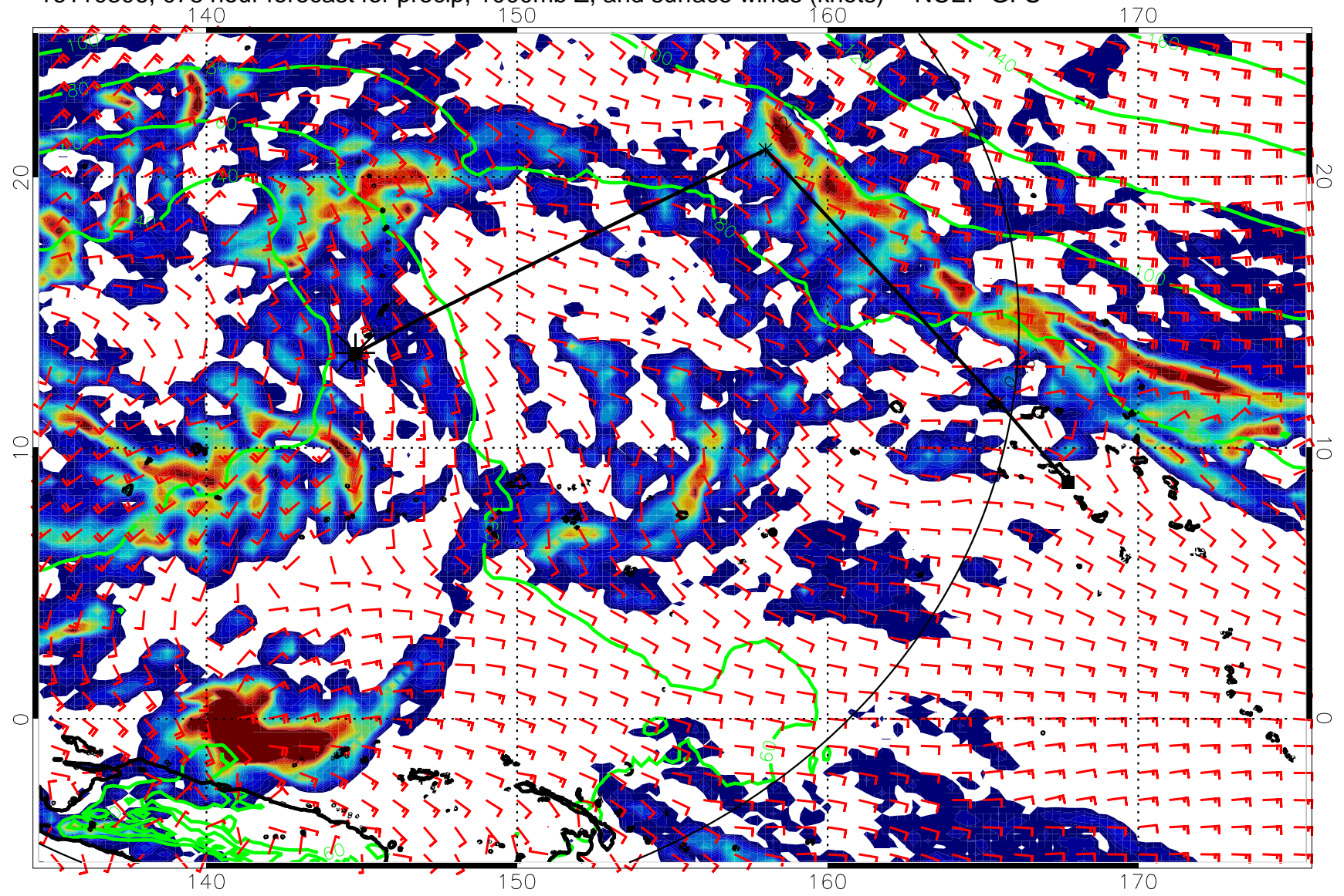
16110306, 078 hour forecast for precip, 1000mb Z, and surface winds (knots) -- NCEP GFS
