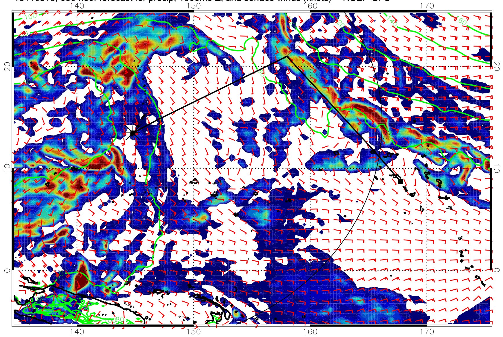
16110318, 090 hour forecast for precip, 1000mb Z, and surface winds (knots) -- NCEP GFS
