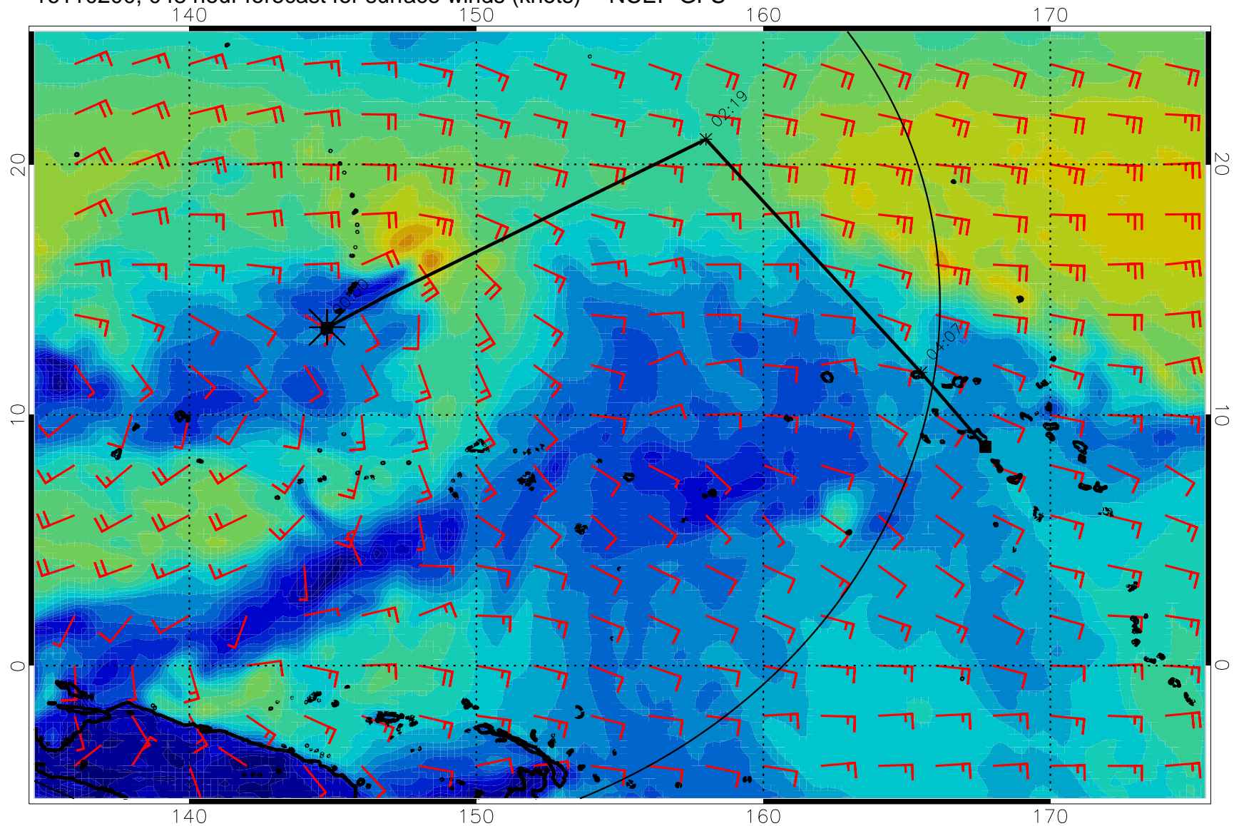
16110200, 048 hour forecast for surface winds (knots) -- NCEP GFS
