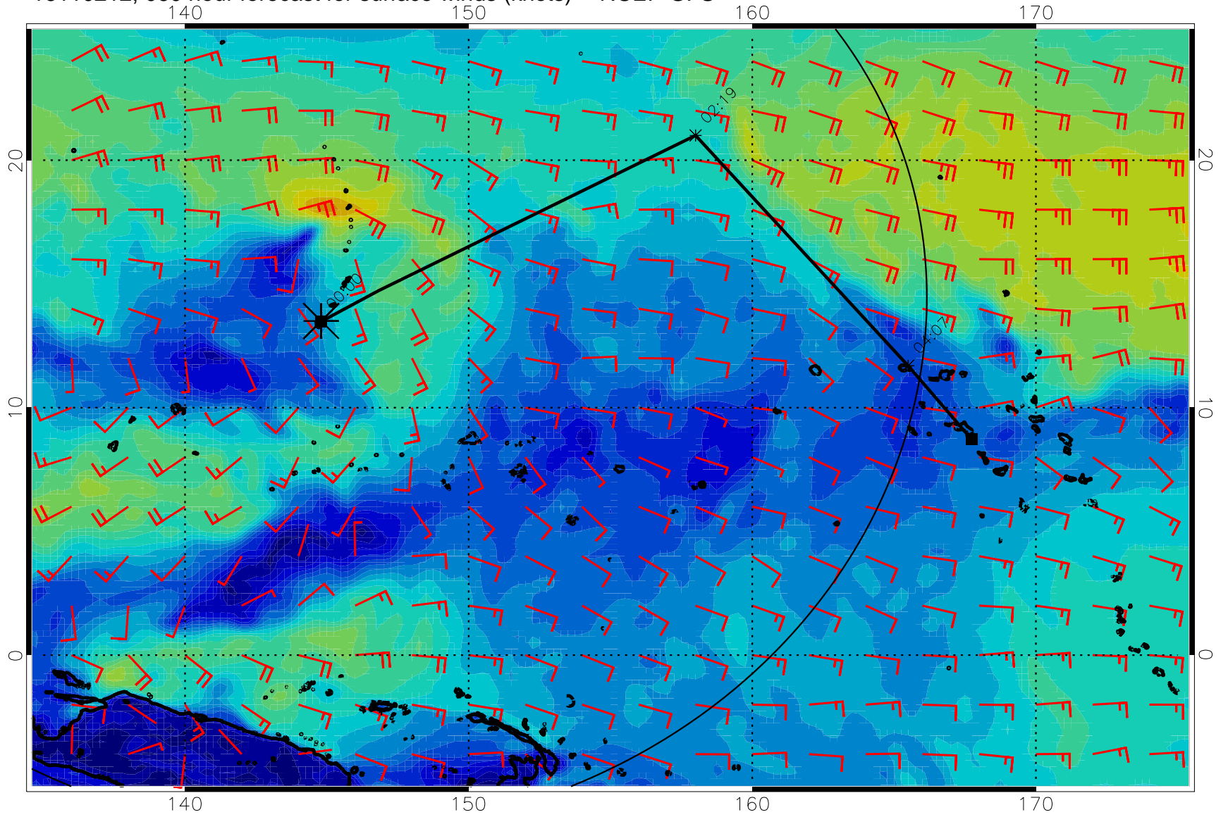
16110212, 060 hour forecast for surface winds (knots) -- NCEP GFS
