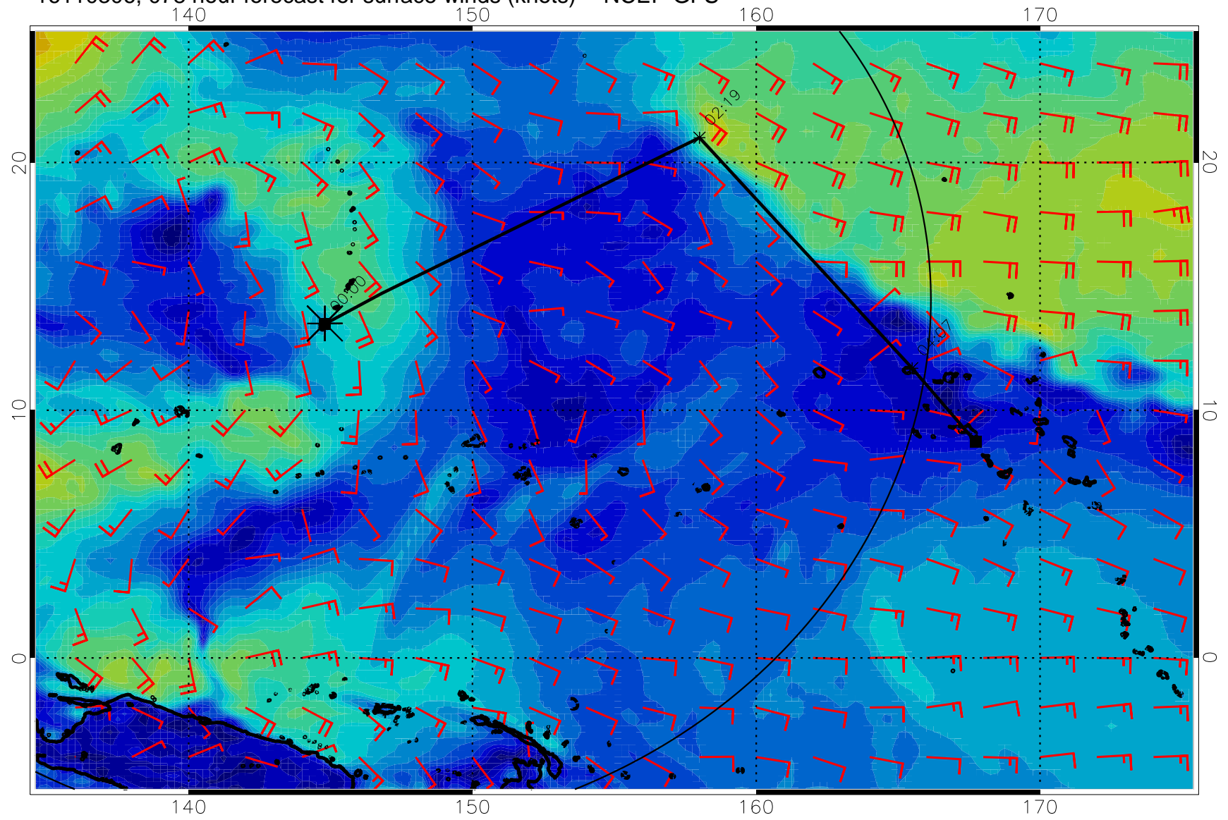
16110306, 078 hour forecast for surface winds (knots) -- NCEP GFS
