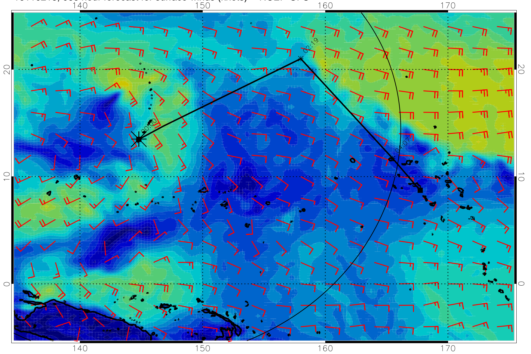
16110218, 066 hour forecast for surface winds (knots) -- NCEP GFS
