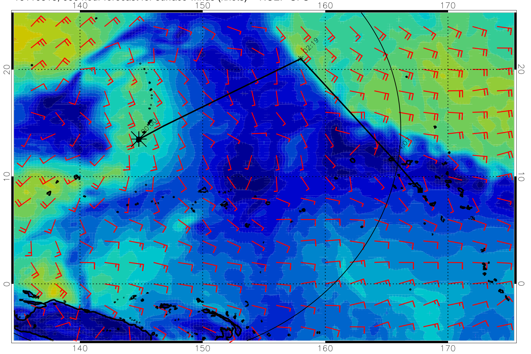
16110318, 090 hour forecast for surface winds (knots) -- NCEP GFS
