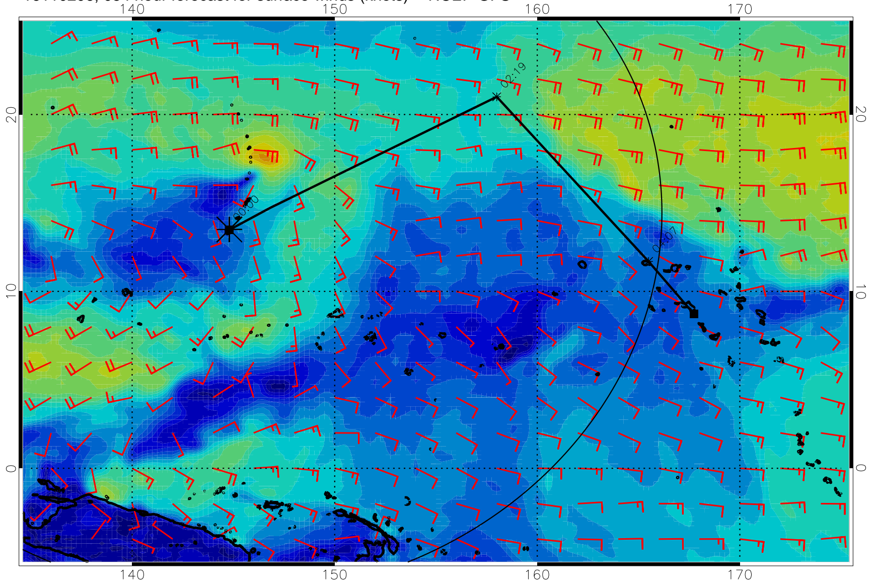
16110206, 054 hour forecast for surface winds (knots) -- NCEP GFS
