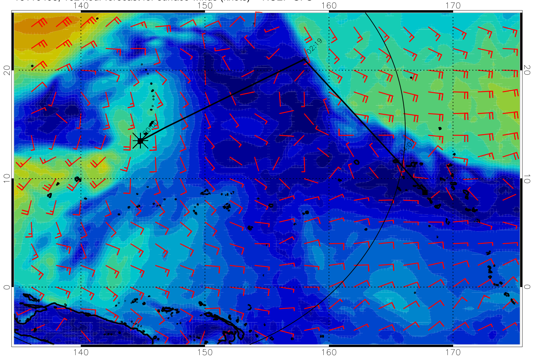
16110406, 102 hour forecast for surface winds (knots) -- NCEP GFS
