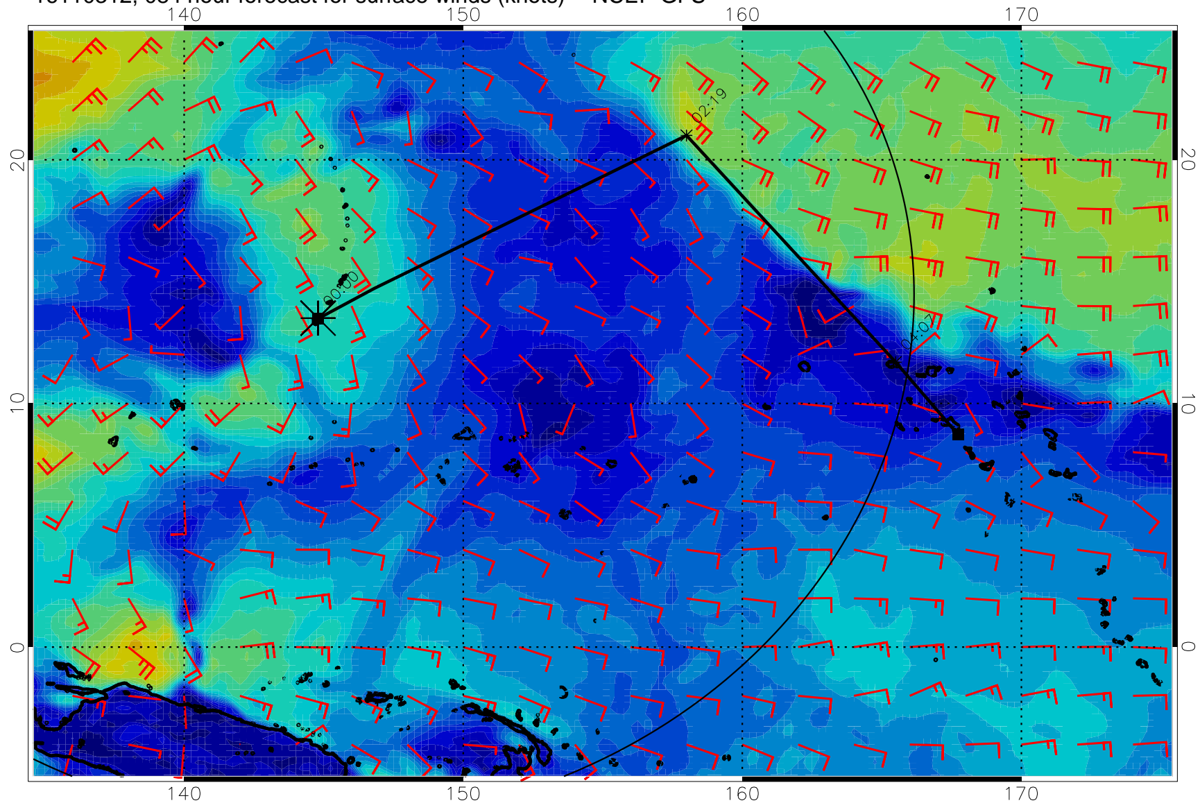
16110312, 084 hour forecast for surface winds (knots) -- NCEP GFS
