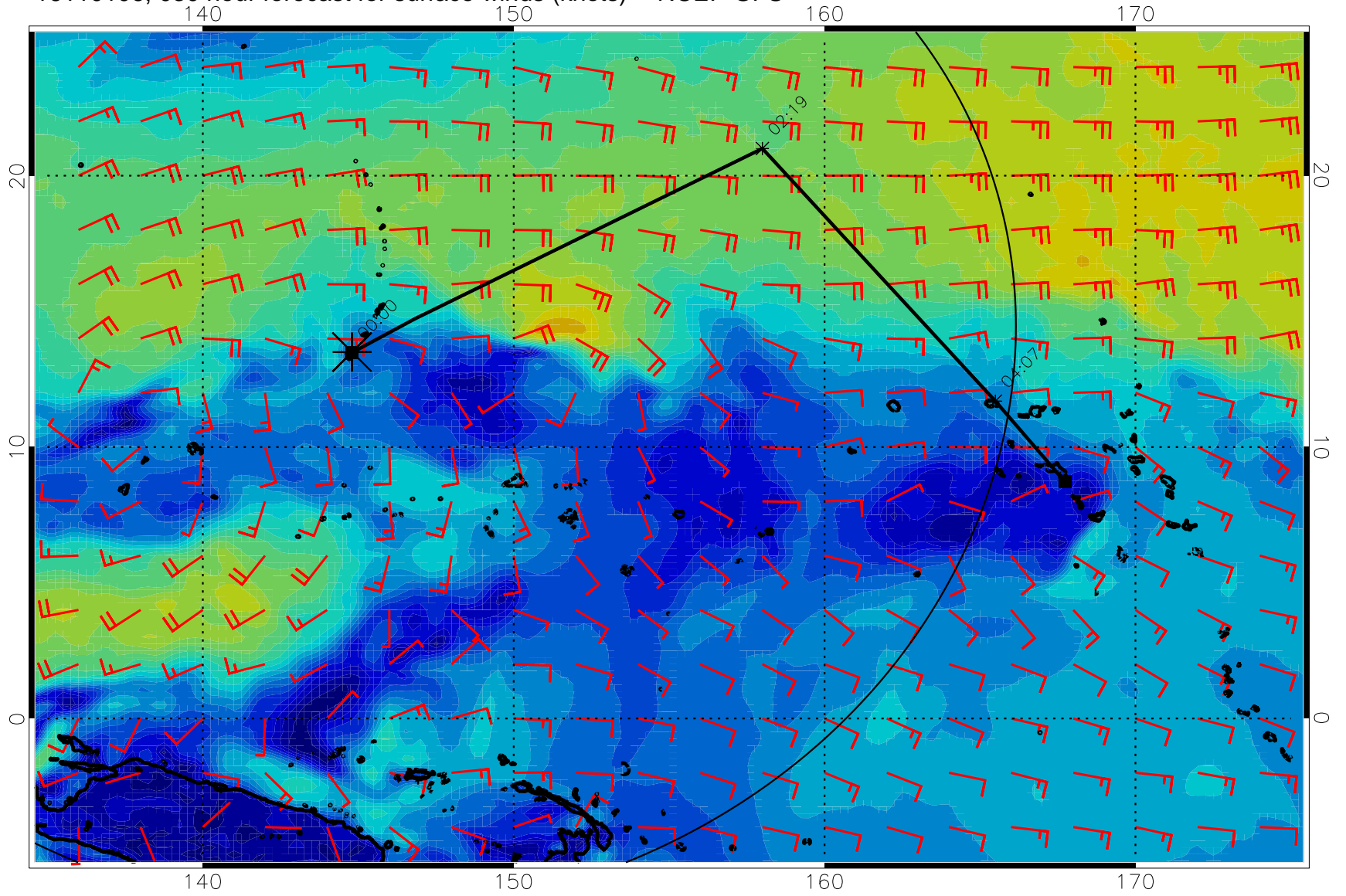
16110106, 0300 hour forecast for surface winds (knots) -- NCEP GFS
