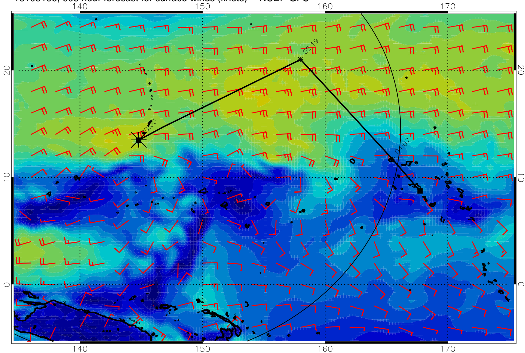
16103106, 006 hour forecast for surface winds (knots) -- NCEP GFS
