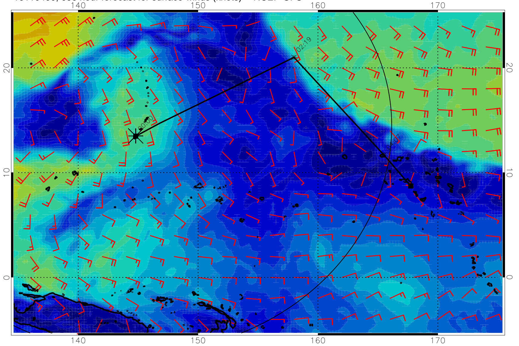
16110400, 096 hour forecast for surface winds (knots) -- NCEP GFS
