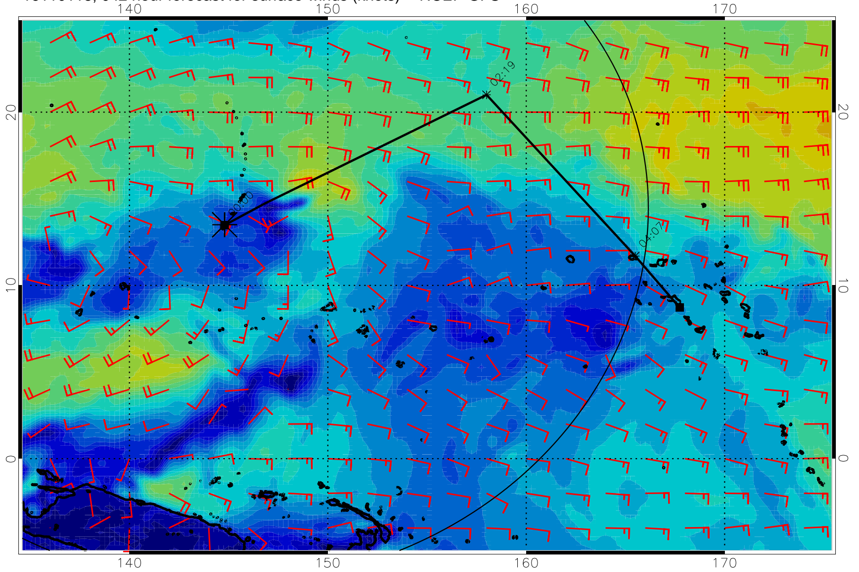
16110118, 042 hour forecast for surface winds (knots) -- NCEP GFS
