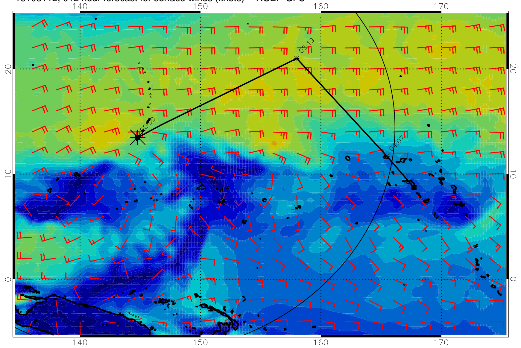
16103112, 012 hour forecast for surface winds (knots) -- NCEP GFS
