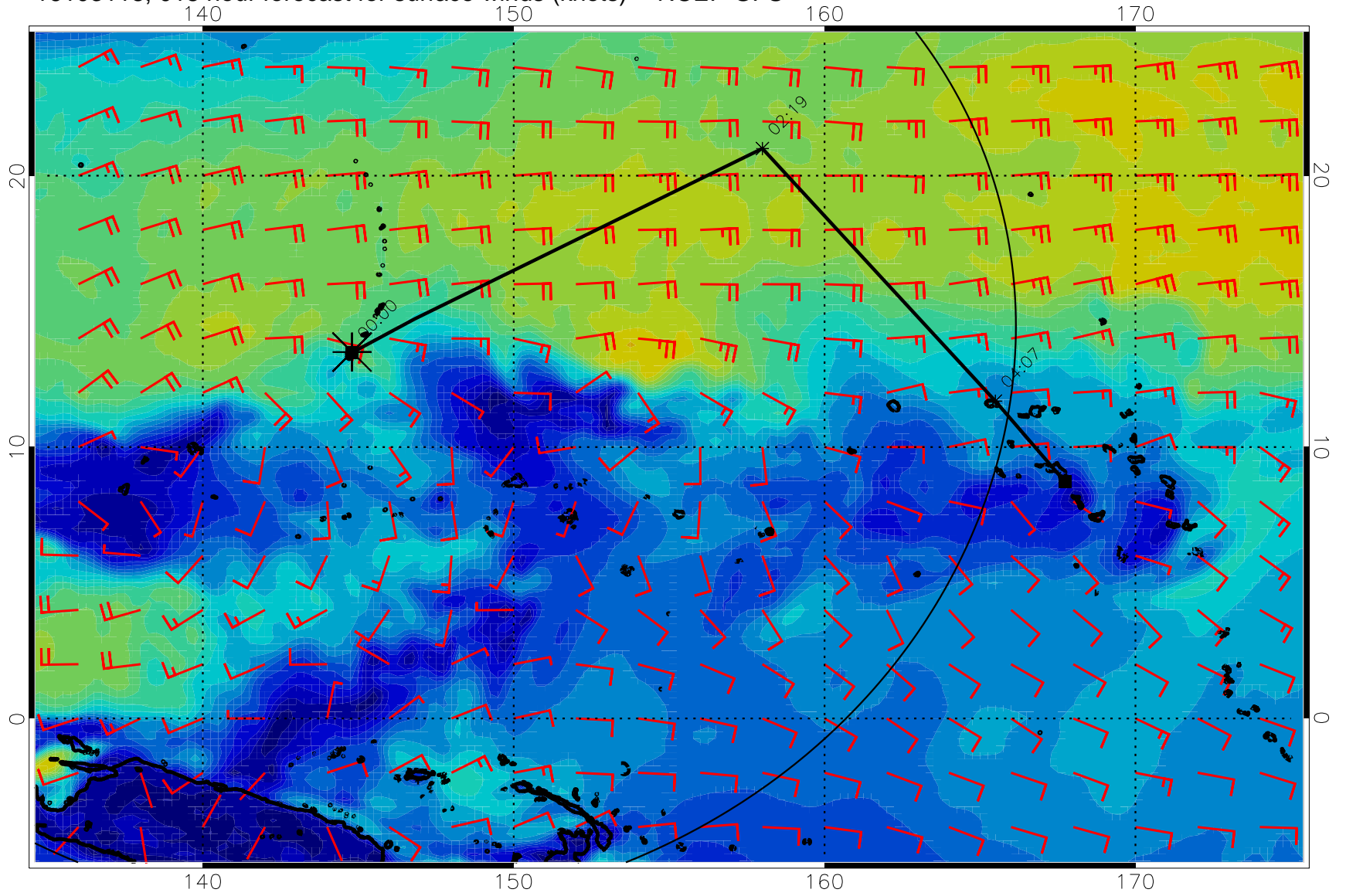
16103118, 018 hour forecast for surface winds (knots) -- NCEP GFS
