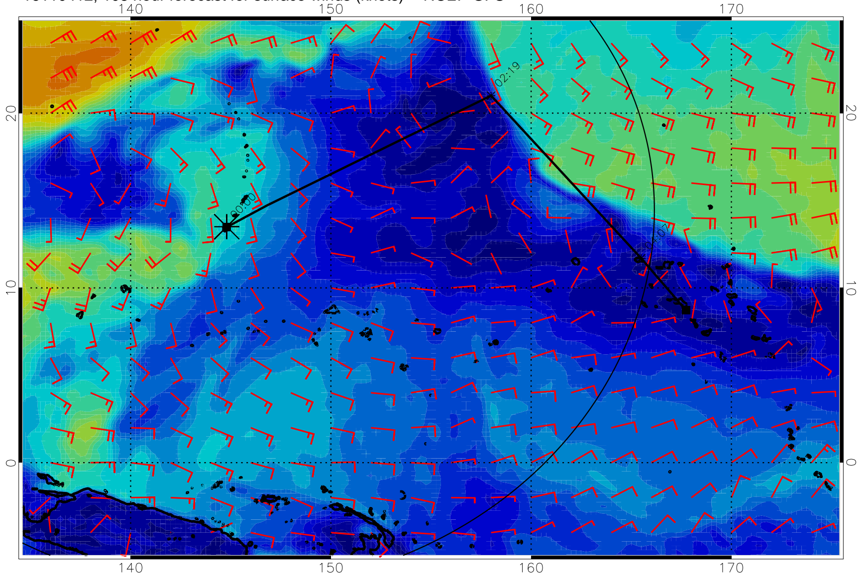
16110412, 108 hour forecast for surface winds (knots) -- NCEP GFS
