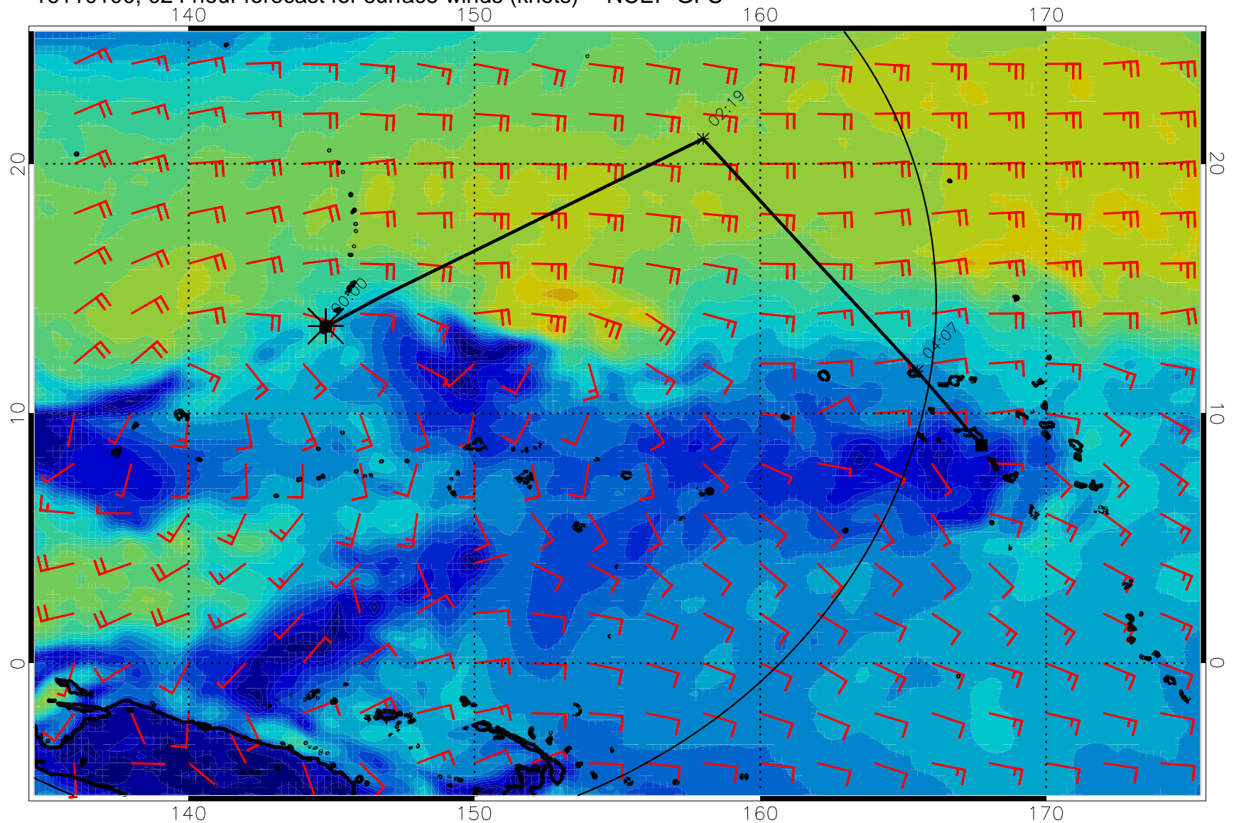
16110100, 024 hour forecast for surface winds (knots) -- NCEP GFS
