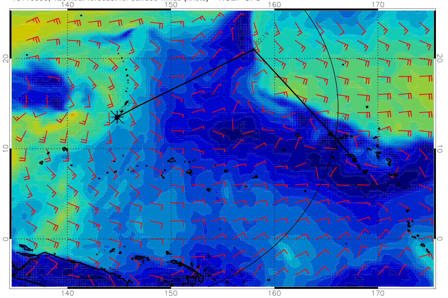
16110500, 120 hour forecast for surface winds (knots) -- NCEP GFS
