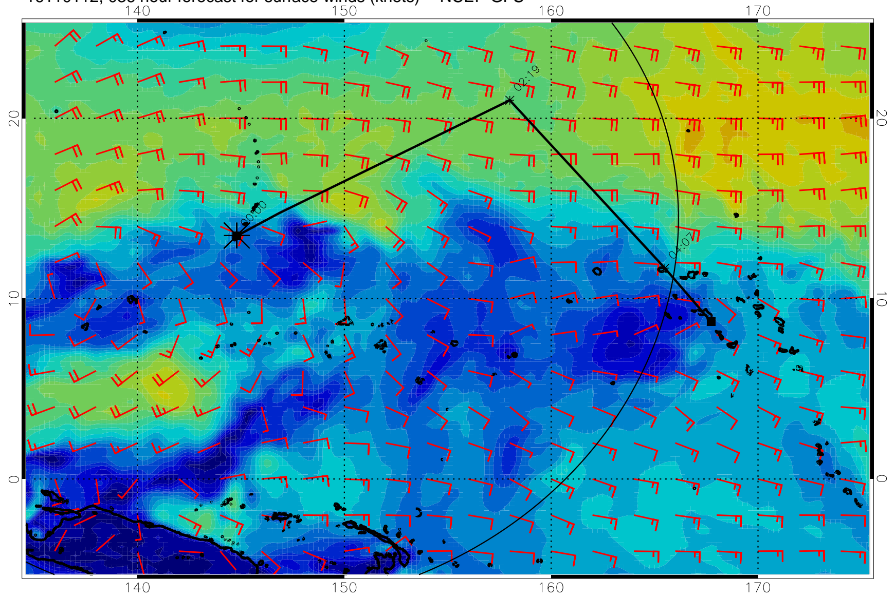
16110112, 036 hour forecast for surface winds (knots) -- NCEP GFS
