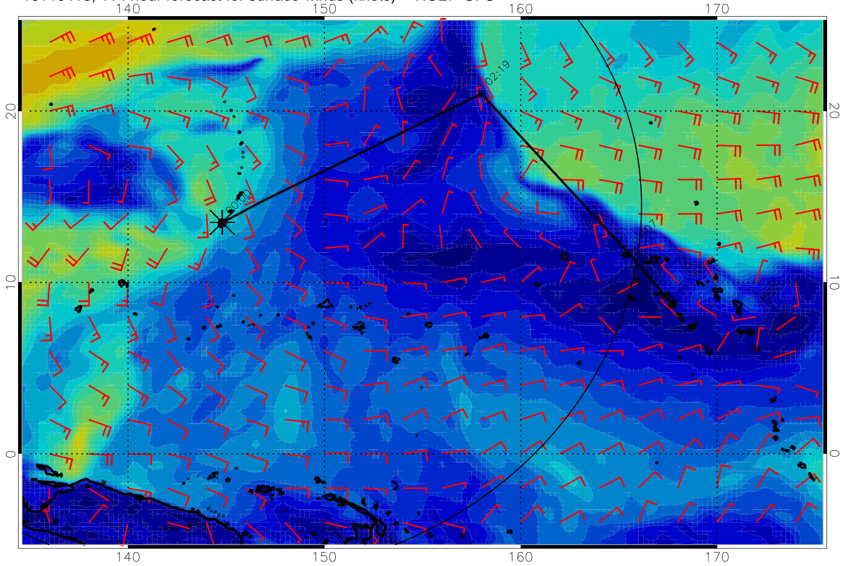
16110418, 114 hour forecast for surface winds (knots) -- NCEP GFS
