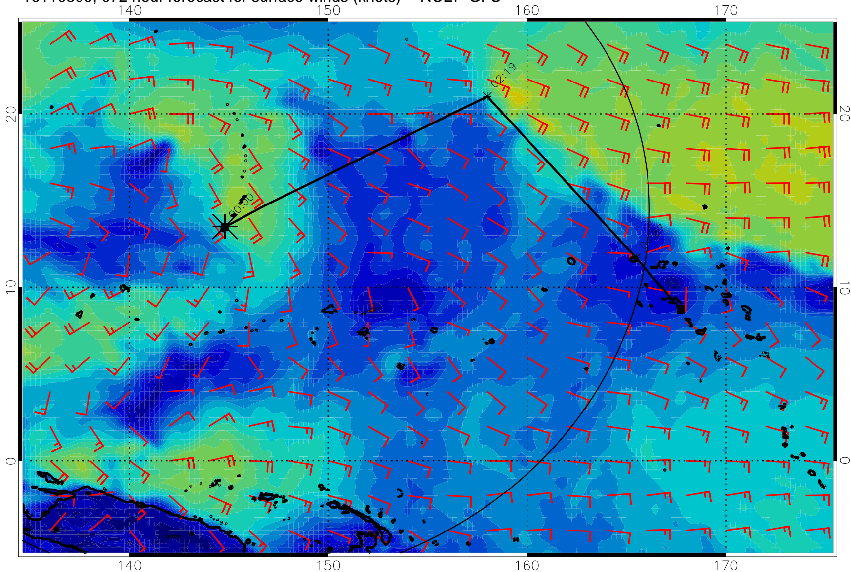
16110300, 072 hour forecast for surface winds (knots) -- NCEP GFS
