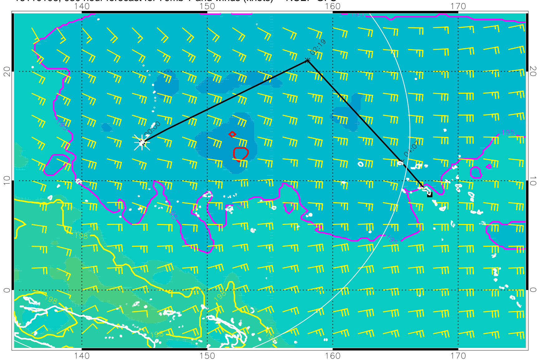
16110106, 030 hour forecast for 70mb T and winds (knots) -- NCEP GFS
