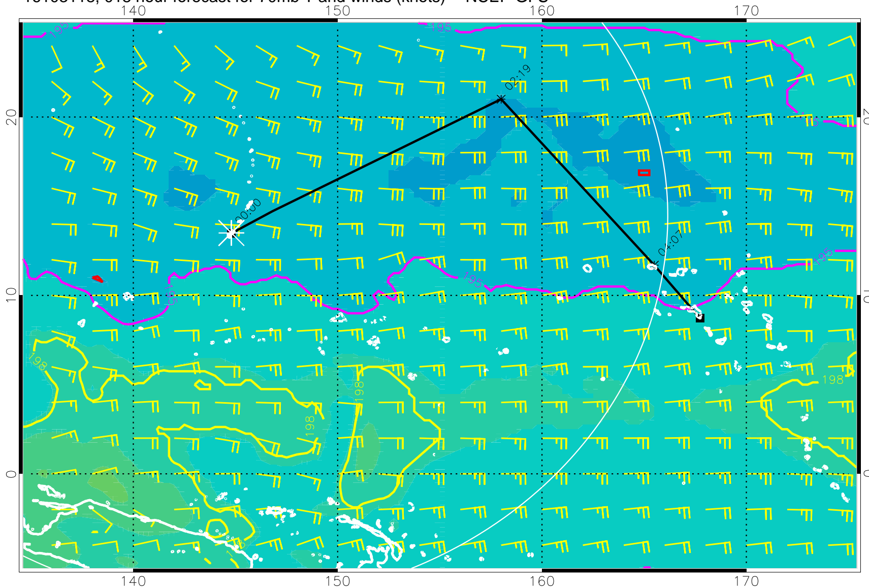
16103118, 018 hour forecast for 70mb T and winds (knots) -- NCEP GFS
