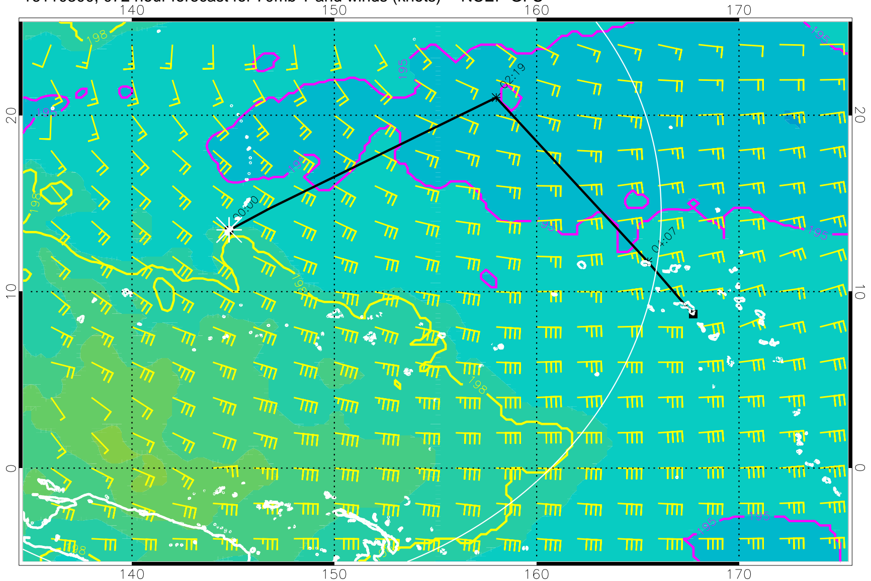
16110300, 072 hour forecast for 70mb T and winds (knots) -- NCEP GFS
