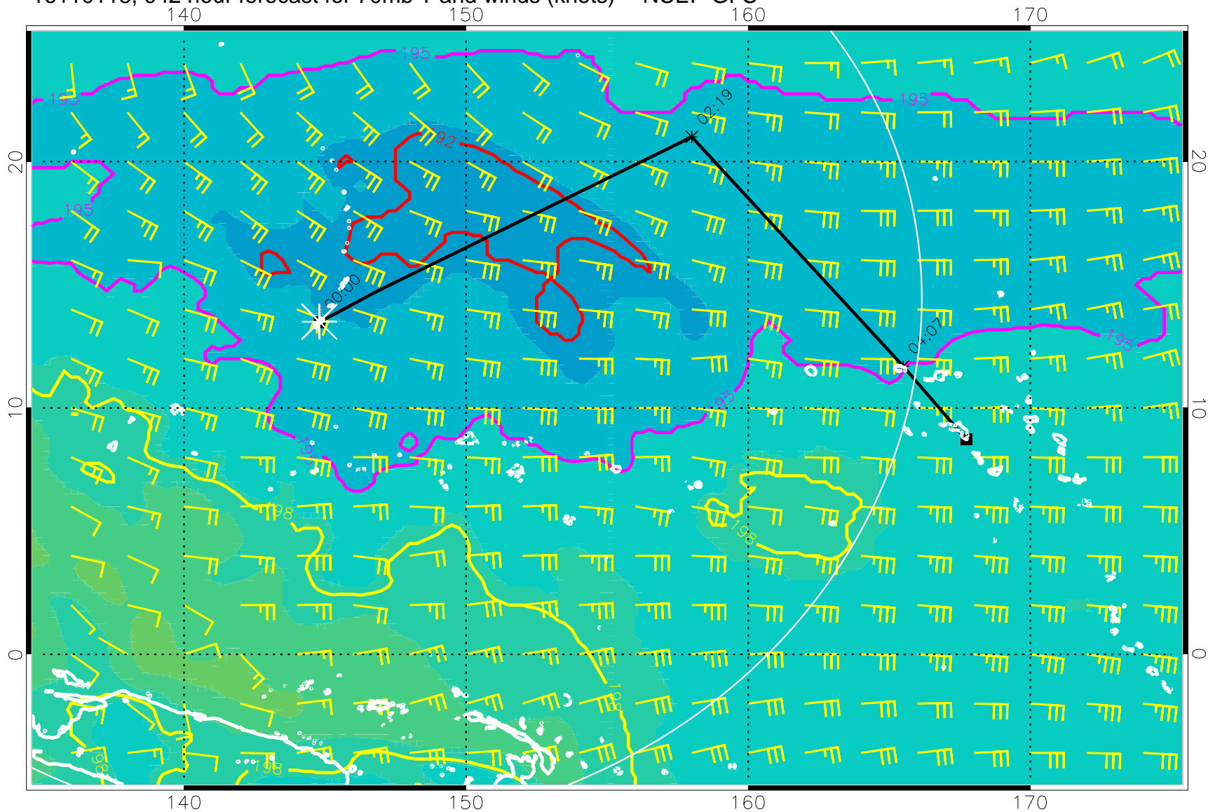
16110118, 04Z hour forecast for 70mb T and winds (knots) -- NCEP GFS
