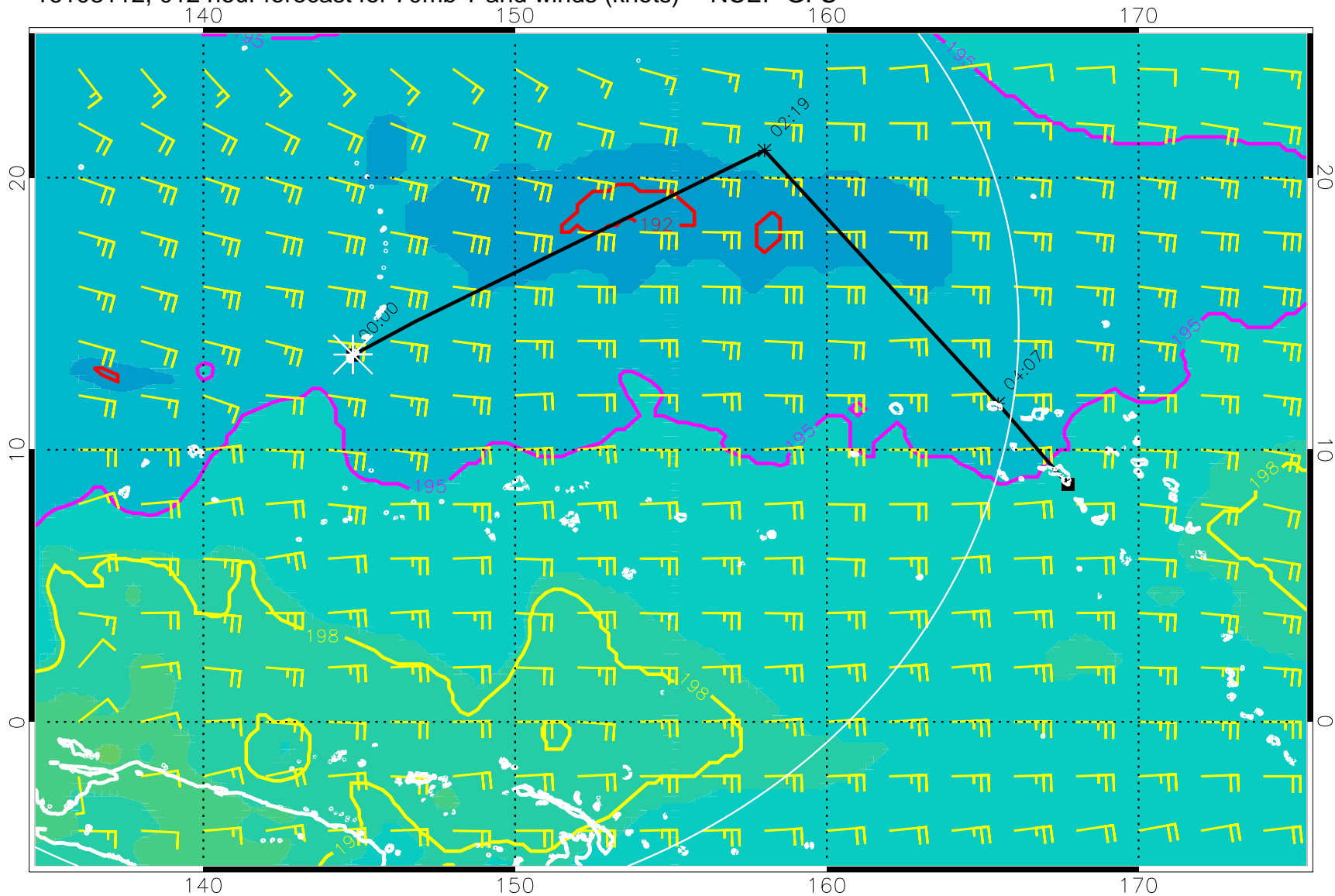
16103112, 012 hour forecast for 70mb T and winds (knots) -- NCEP GFS
