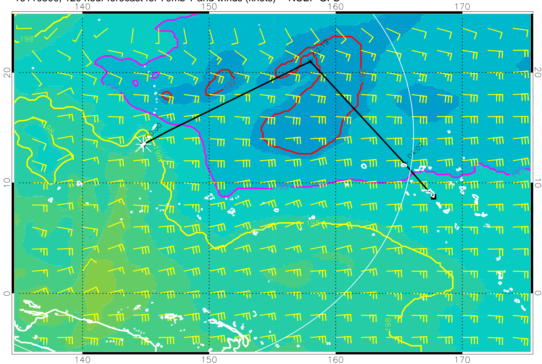
16110500, 120 hour forecast for 70mb T and winds (knots) -- NCEP GFS
