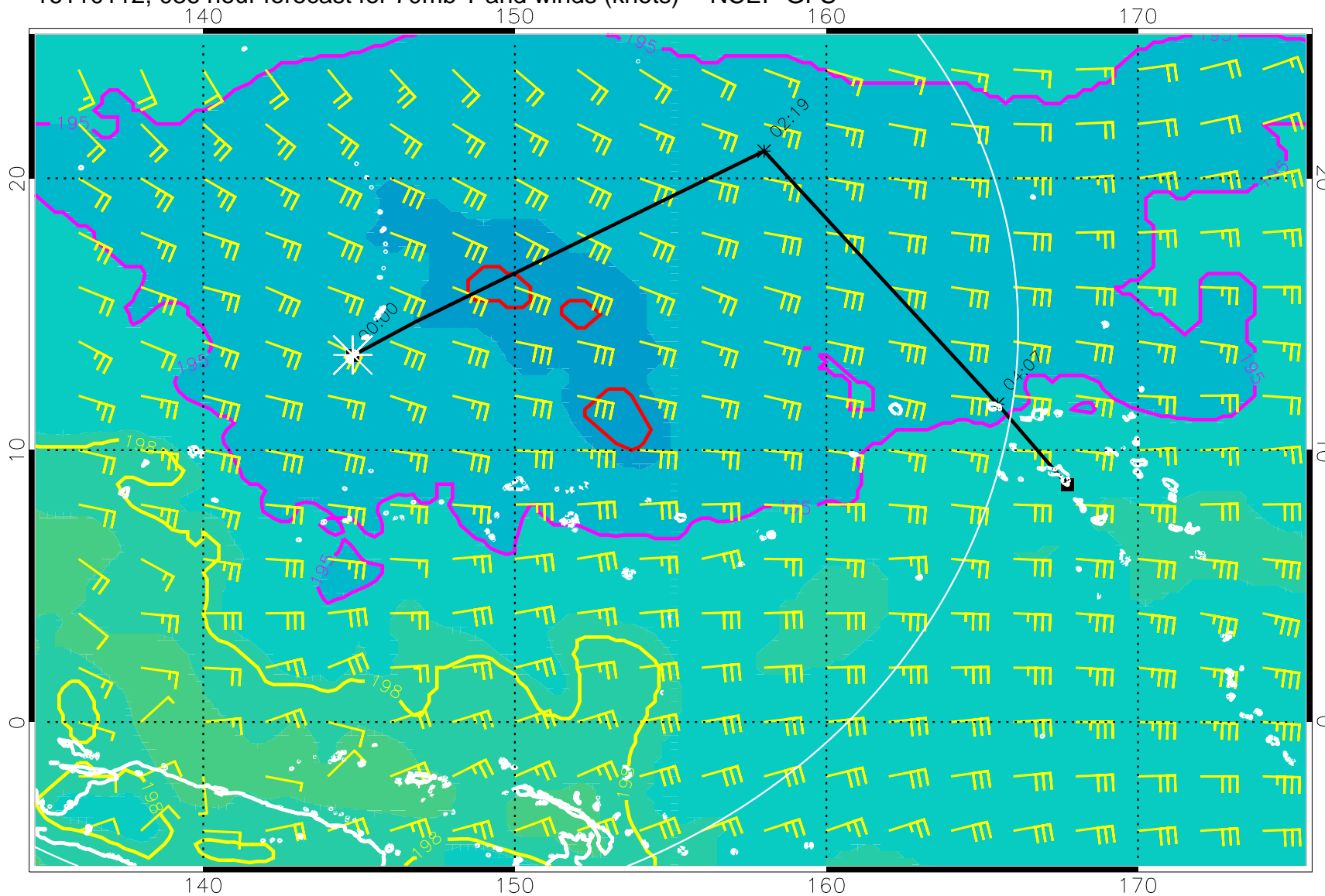
16110112, 036 hour forecast for 70mb T and winds (knots) -- NCEP GFS
