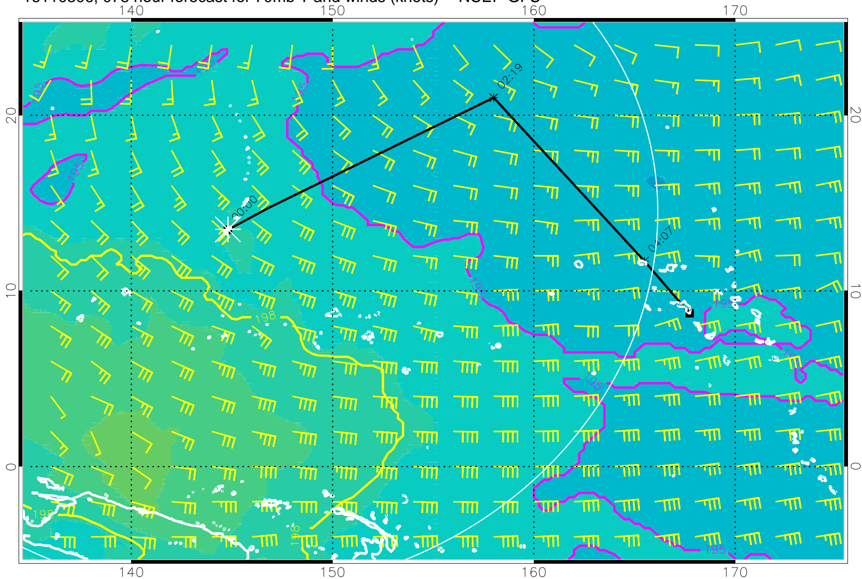
16110306, 078 hour forecast for 70mb T and winds (knots) -- NCEP GFS
