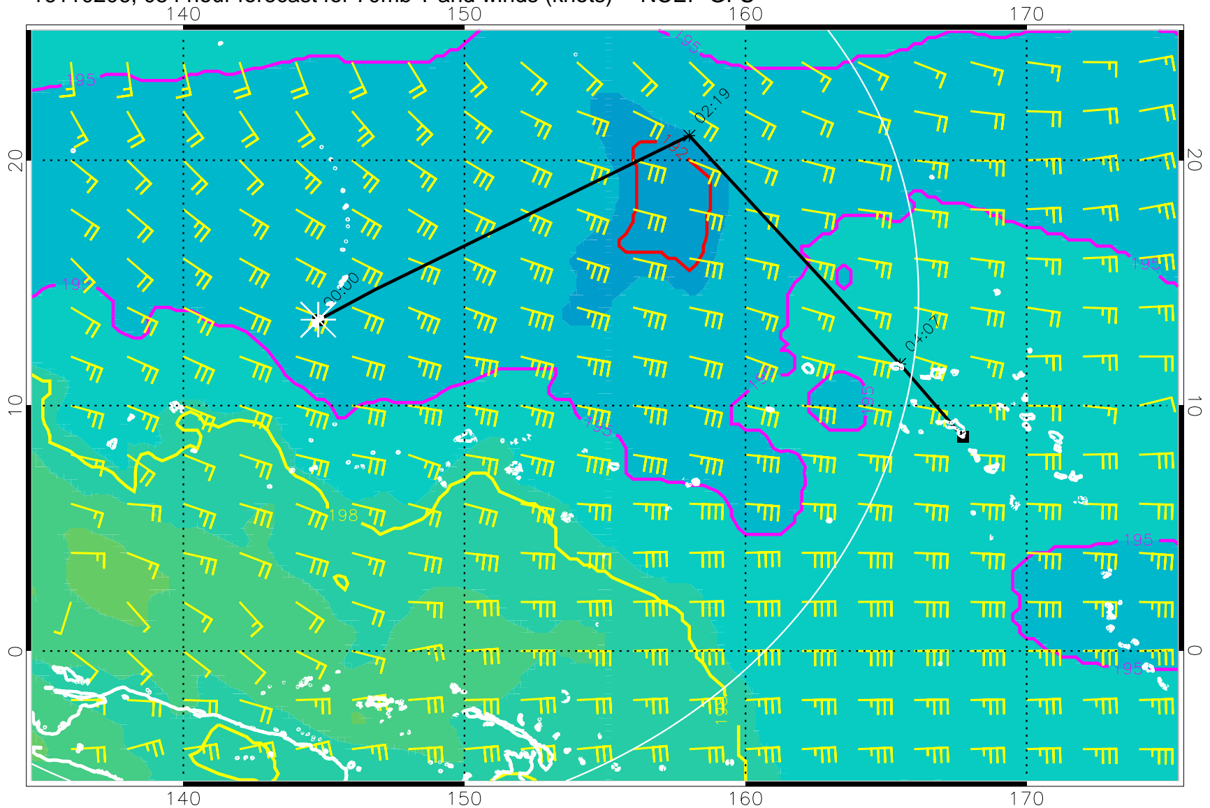
16110206, 054 hour forecast for 70mb T and winds (knots) -- NCEP GFS
