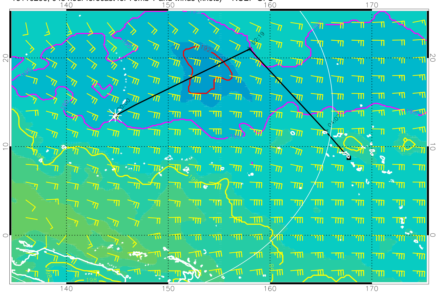
16110200, 048 hour forecast for 70mb T and winds (knots) -- NCEP GFS
