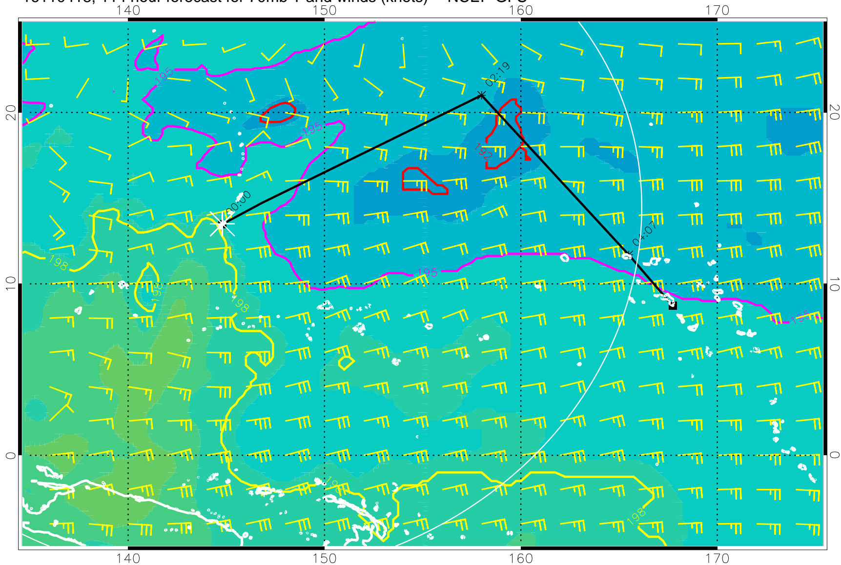
16110418, 114 hour forecast for 70mb T and winds (knots) -- NCEP GFS
