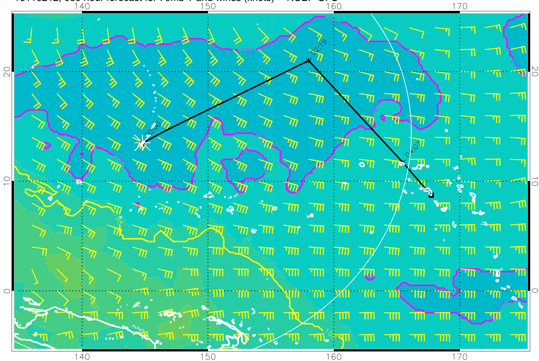
16110212, 060 hour forecast for 70mb T and winds (knots) -- NCEP GFS
