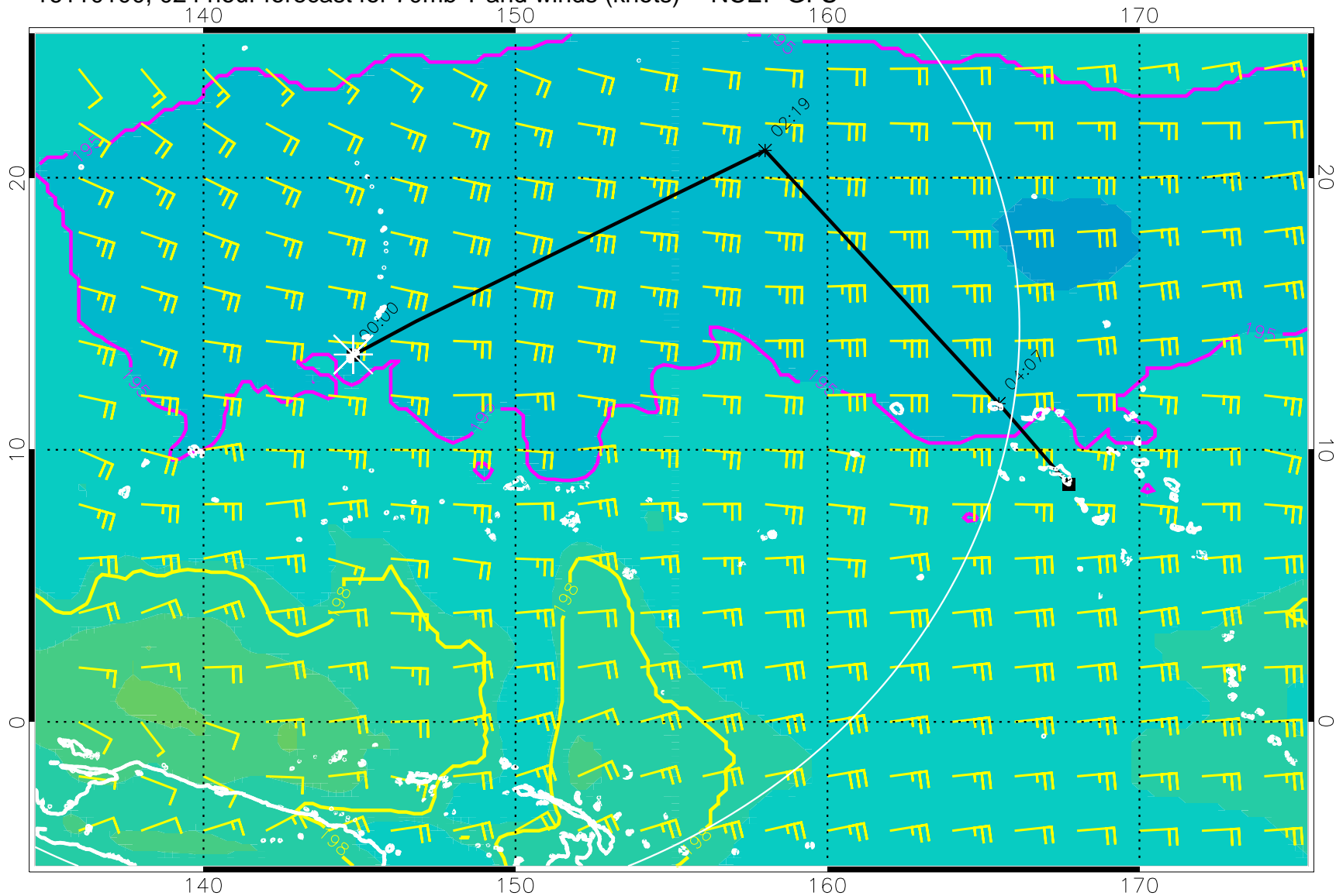
16110100, 024 hour forecast for 70mb T and winds (knots) -- NCEP GFS
