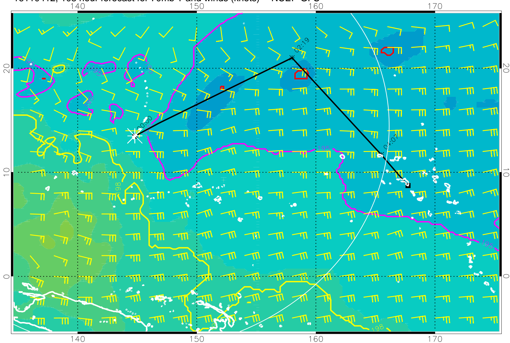
16110412, 108 hour forecast for 70mb T and winds (knots) -- NCEP GFS
