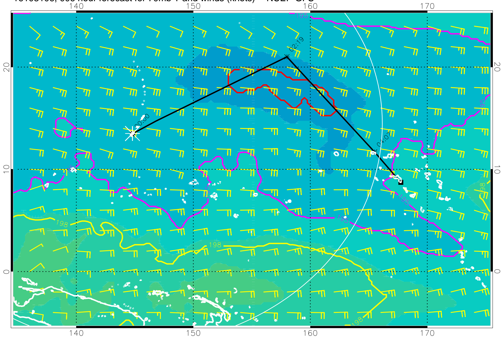
16103106, 006 hour forecast for 70mb T and winds (knots) -- NCEP GFS
