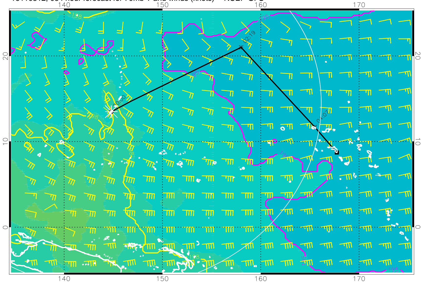
16110312, 084 hour forecast for 70mb T and winds (knots) -- NCEP GFS
