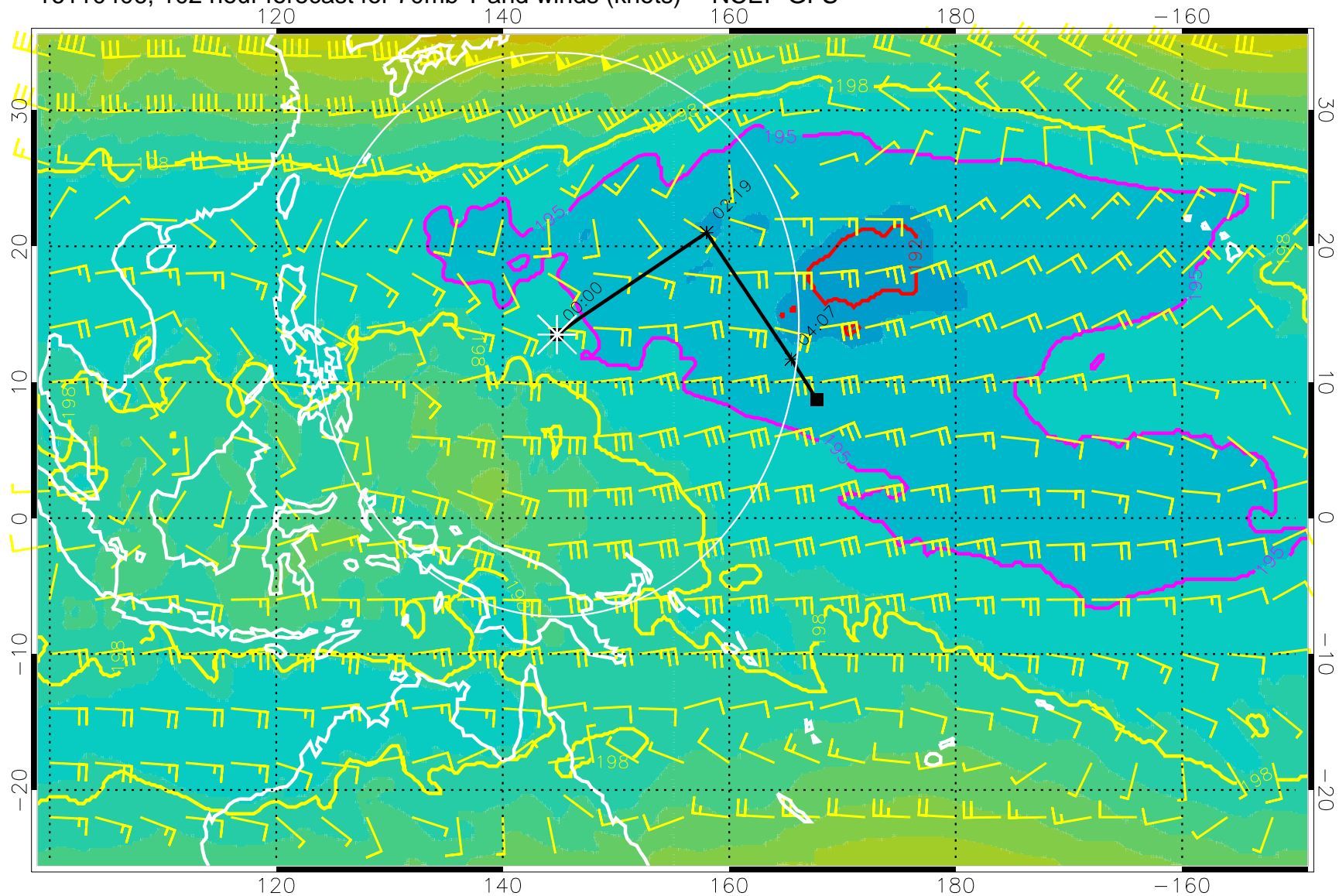
16110406, 102 hour forecast for 70mb T and winds (knots) -- NCEP GFS
