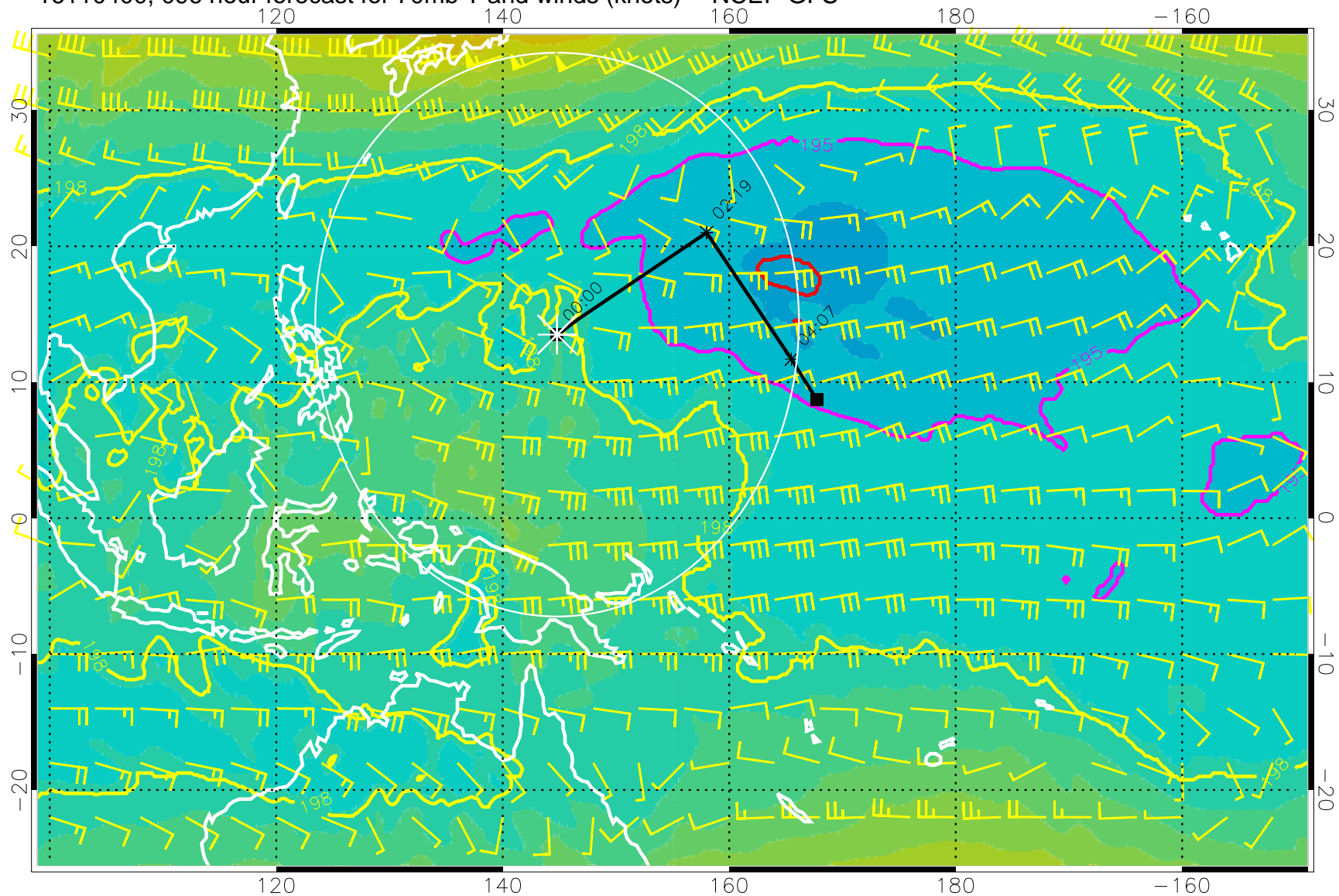
16110400, 096 hour forecast for 70mb T and winds (knots) -- NCEP GFS
