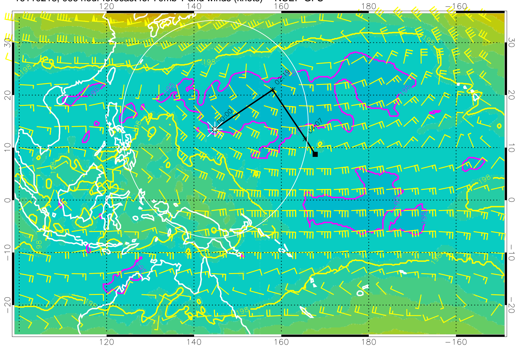
16110218, 066 hour forecast for 70mb T and winds (knots) -- NCEP GFS
