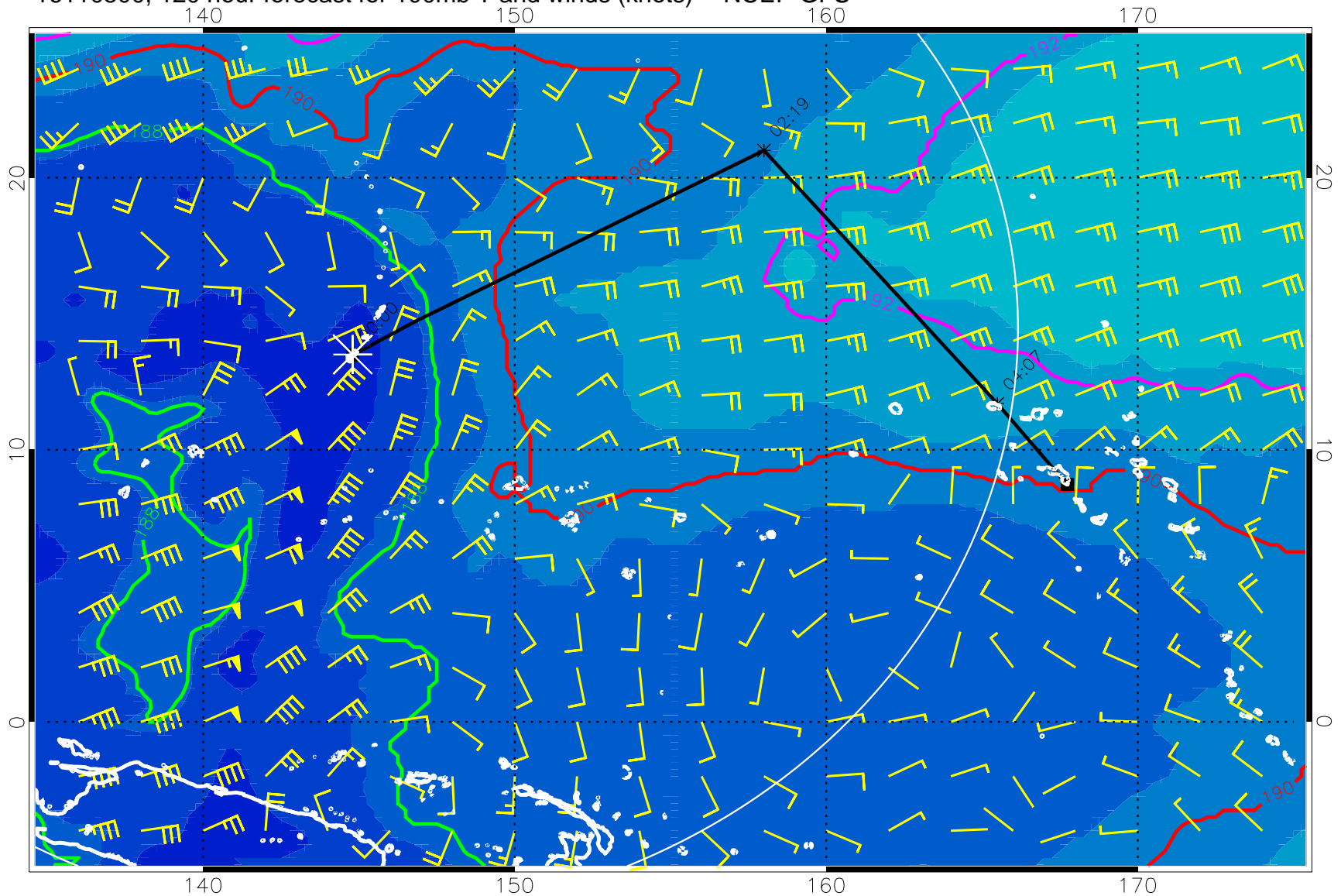
16110500, 120 hour forecast for 100mb T and winds (knots) -- NCEP GFS
