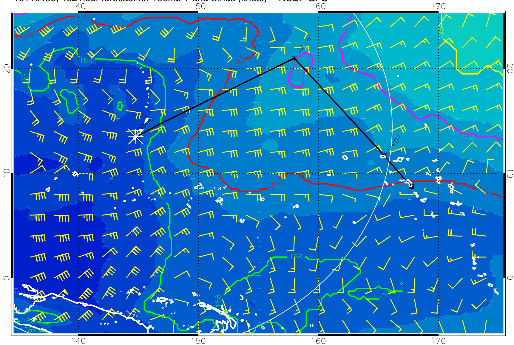
16110406, 102 hour forecast for 100mb T and winds (knots) -- NCEP GFS
