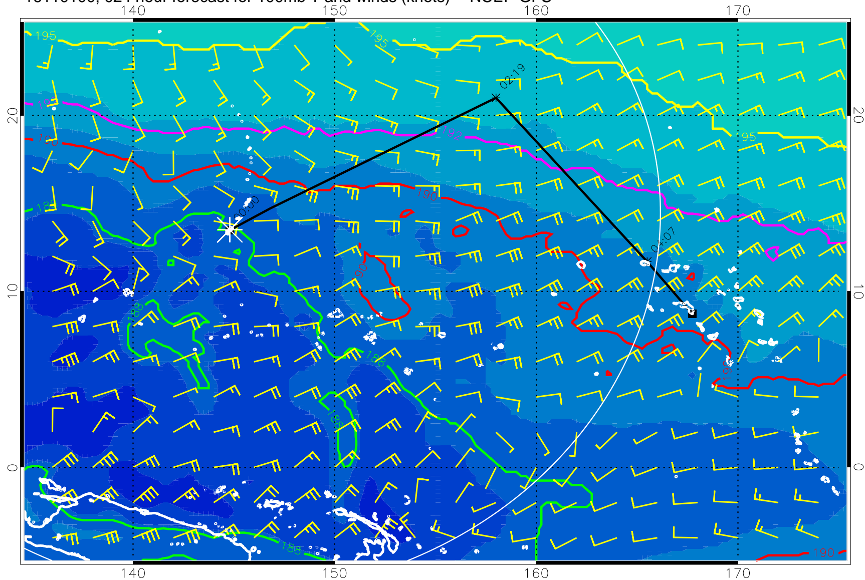
16110100, 024 hour forecast for 100mb T and winds (knots) -- NCEP GFS
