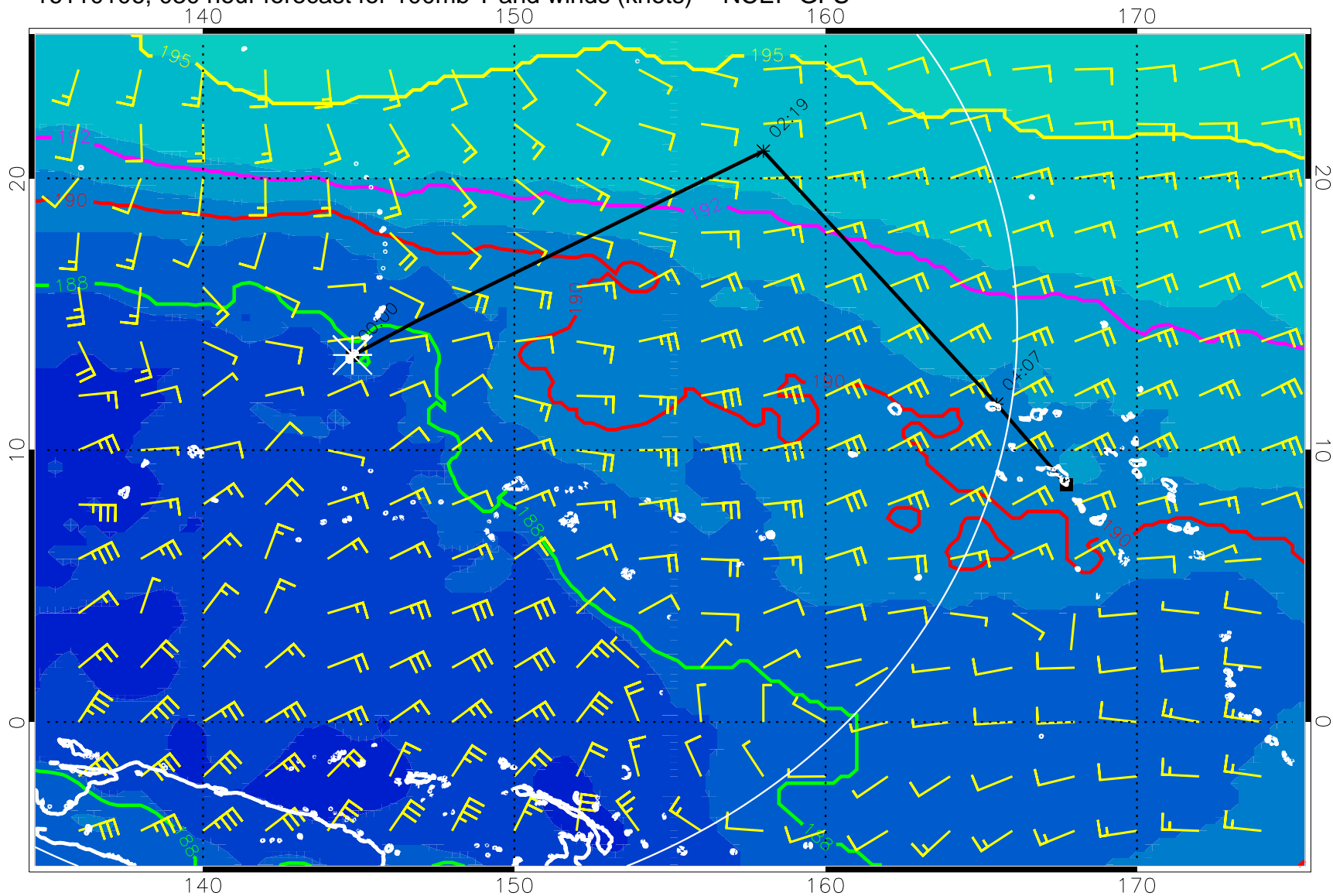
16110106, 030 hour forecast for 100mb T and winds (knots) -- NCEP GFS
