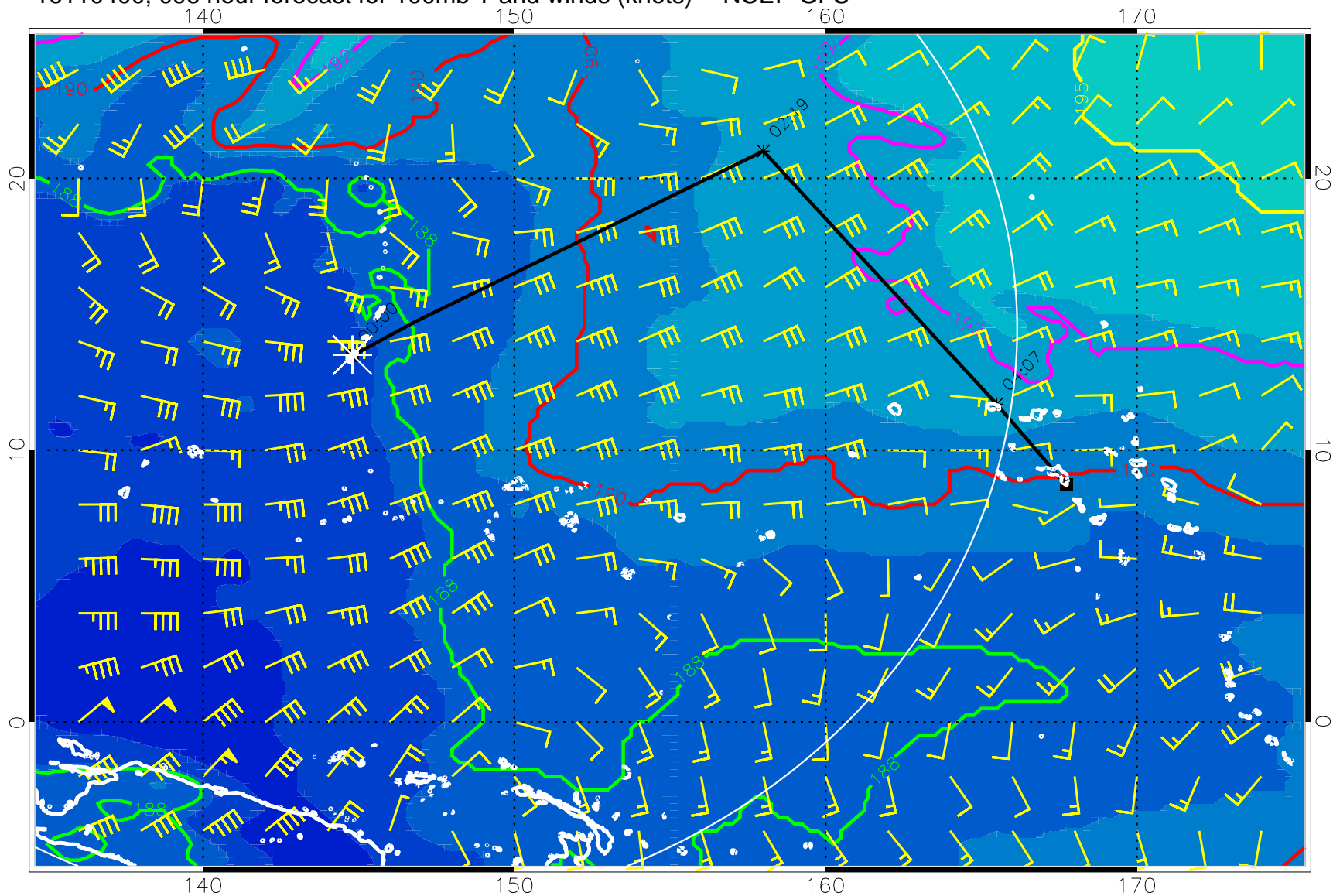
16110400, 096 hour forecast for 100mb T and winds (knots) -- NCEP GFS
