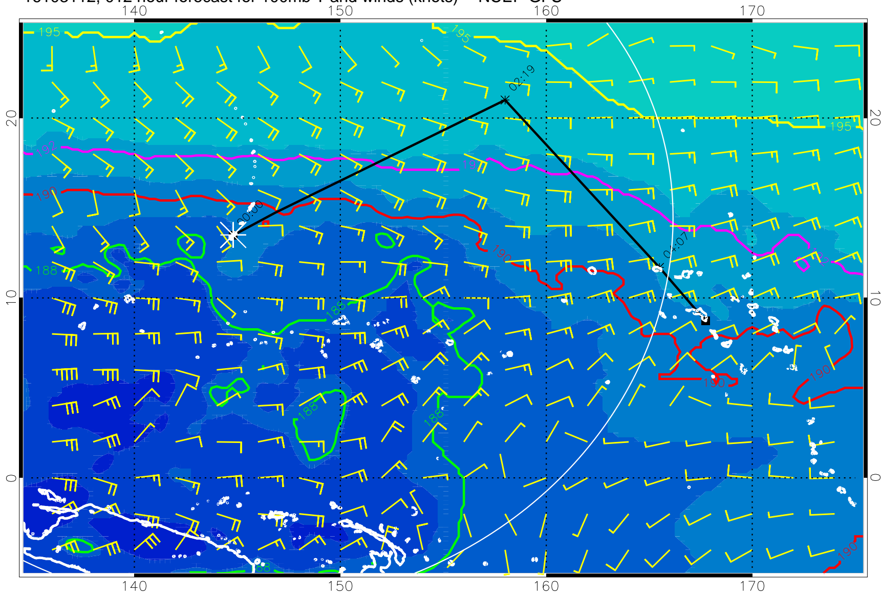
16103112, 012 hour forecast for 100mb T and winds (knots) -- NCEP GFS
