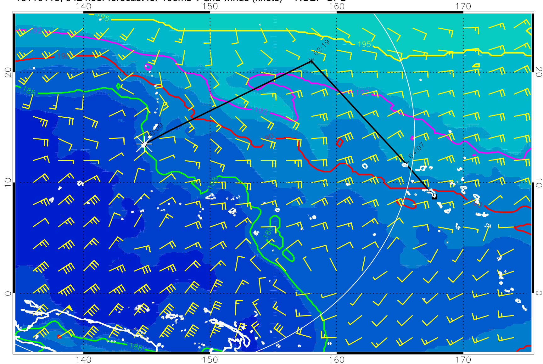
16110118, 042 hour forecast for 100mb T and winds (knots) -- NCEP GFS
