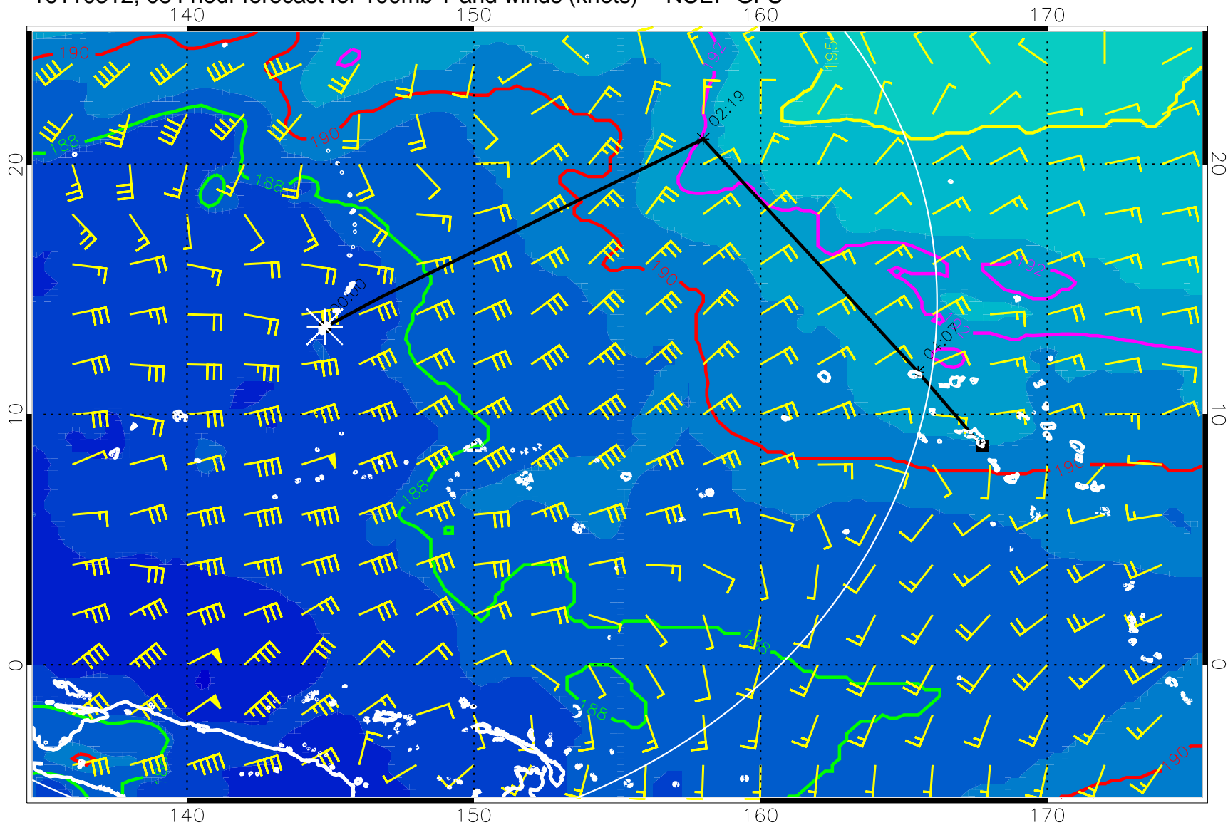
16110312, 084 hour forecast for 100mb T and winds (knots) -- NCEP GFS
