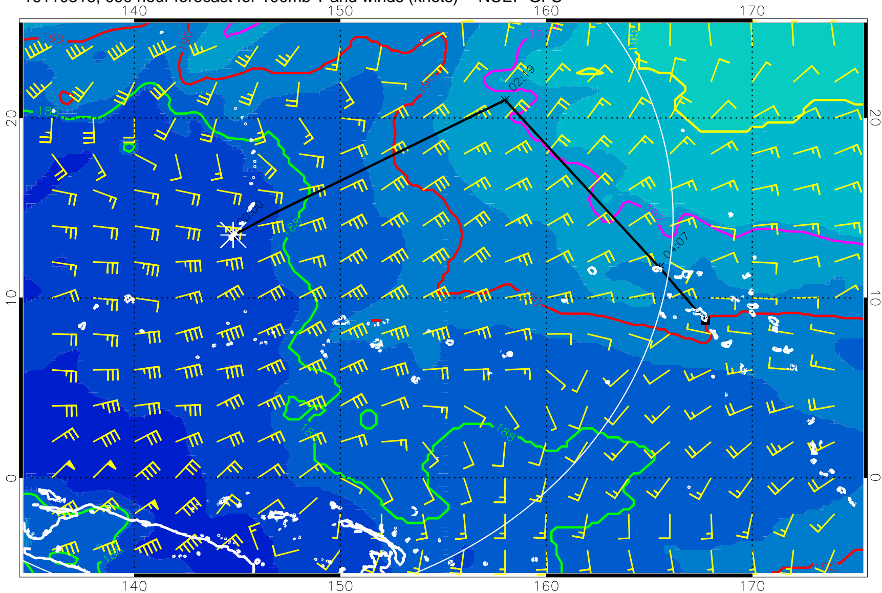
16110318, 090 hour forecast for 100mb T and winds (knots) -- NCEP GFS
