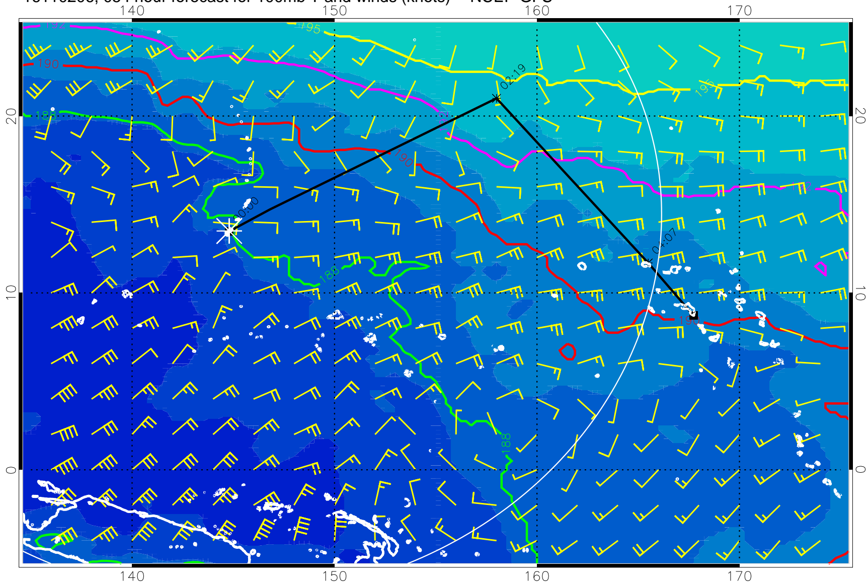
16110206, 054 hour forecast for 100mb T and winds (knots) -- NCEP GFS
