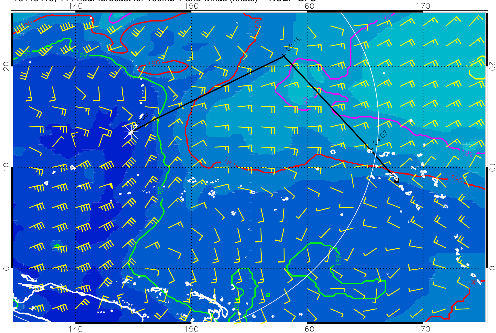
16110418, 114 hour forecast for 100mb T and winds (knots) -- NCEP GFS
