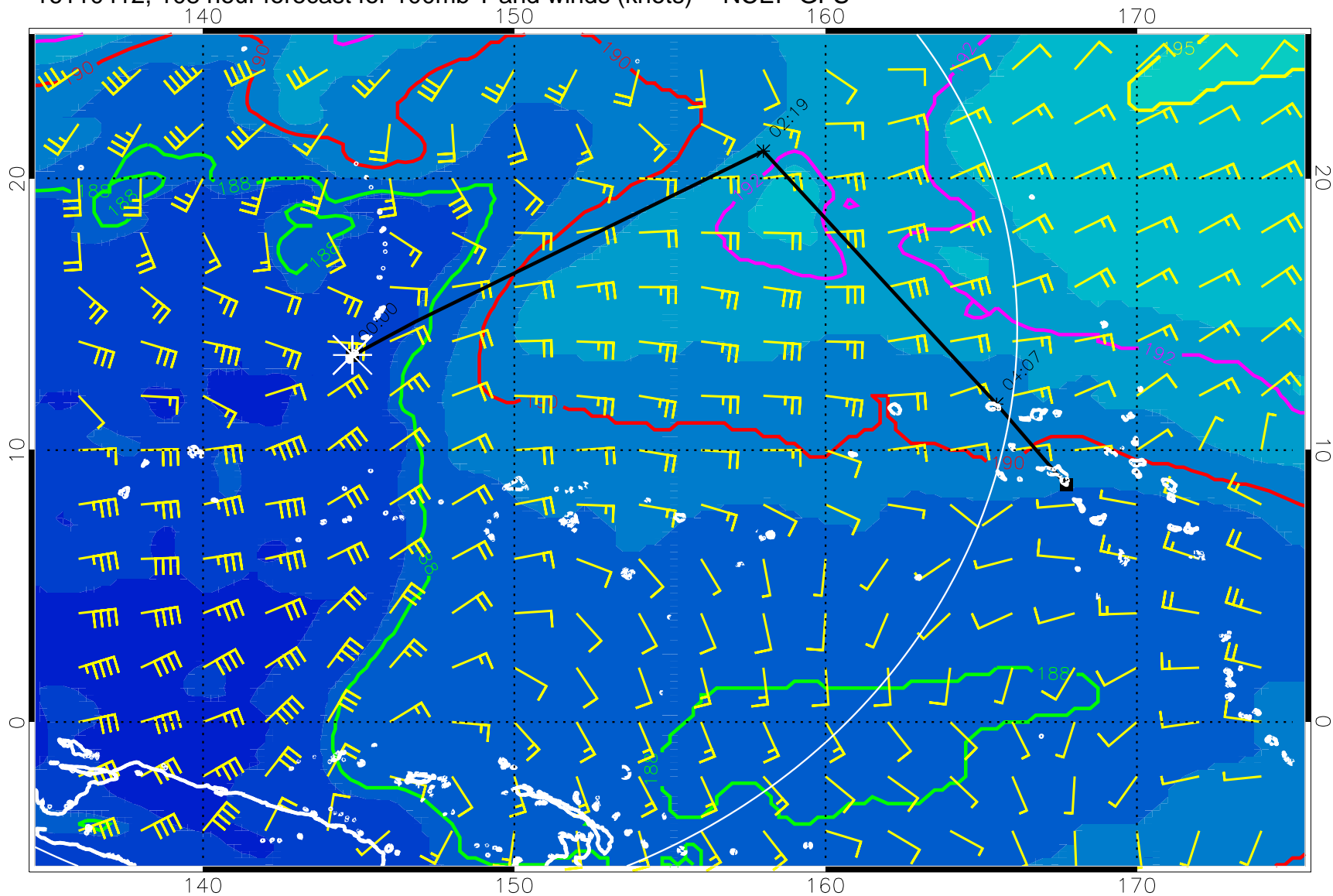
16110412, 108 hour forecast for 100mb T and winds (knots) -- NCEP GFS
