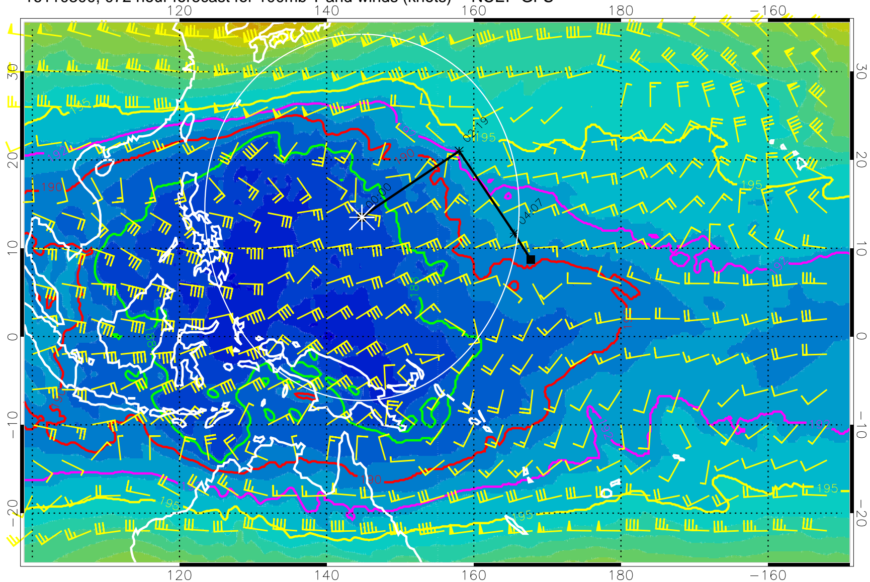
16110300, 072 hour forecast for 100mb T and winds (knots) -- NCEP GFS
