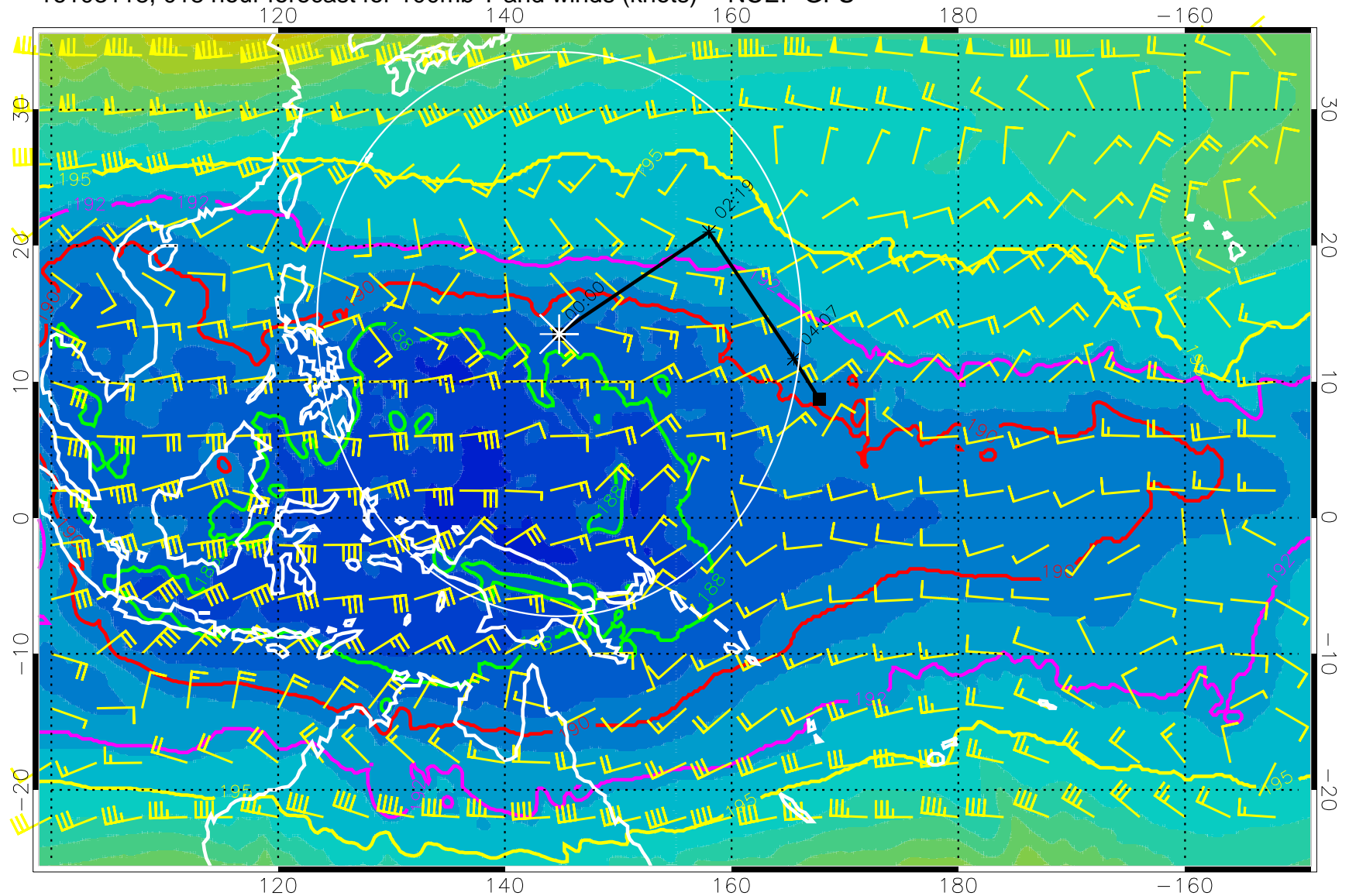
16103118, 018 hour forecast for 100mb T and winds (knots) -- NCEP GFS
