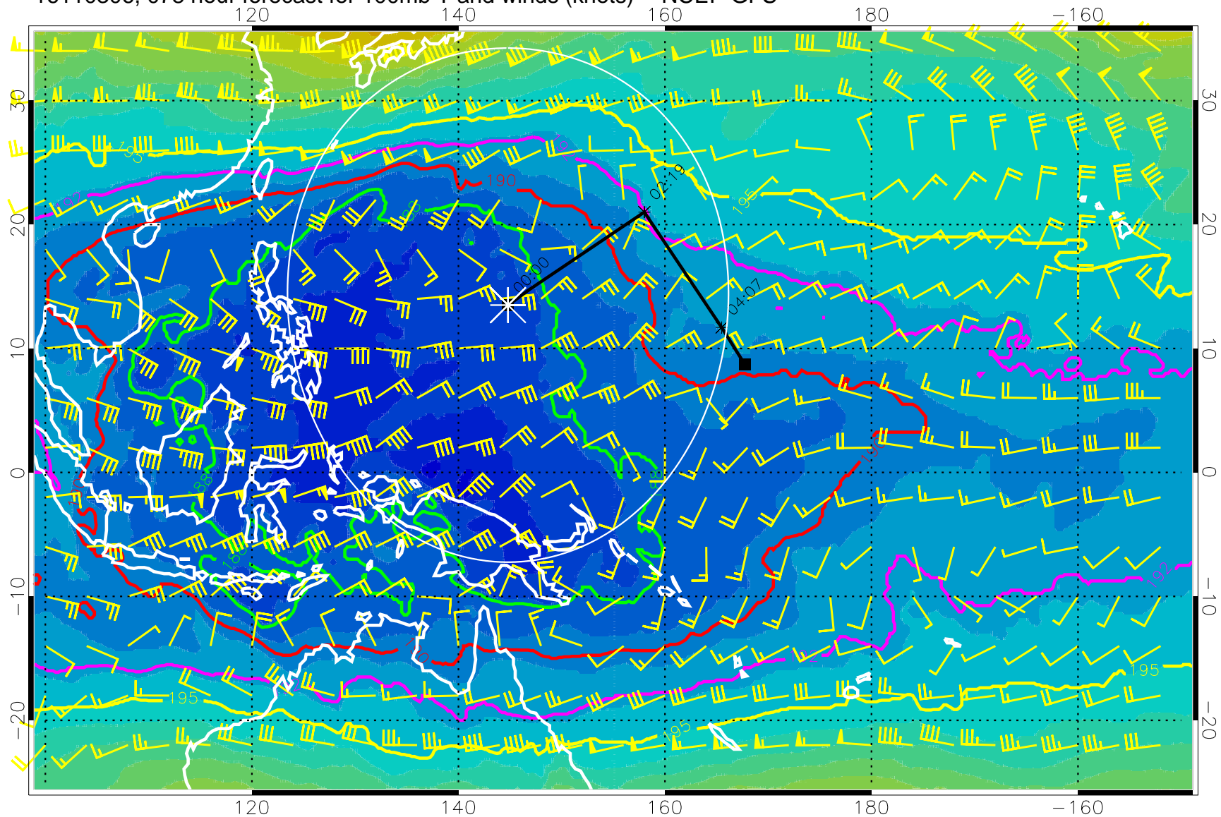
16110306, 078 hour forecast for 100mb T and winds (knots) -- NCEP GFS
