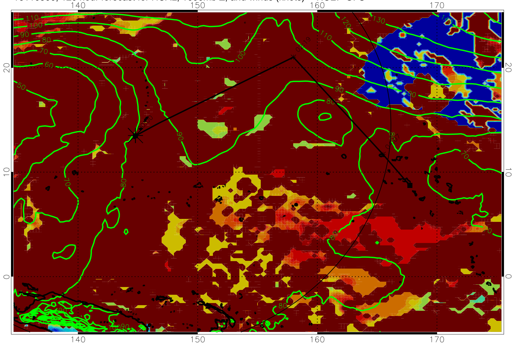
16110500, 120 hour forecast for HCAL, 1000mb Z, and winds (knots) -- NCEP GFS
