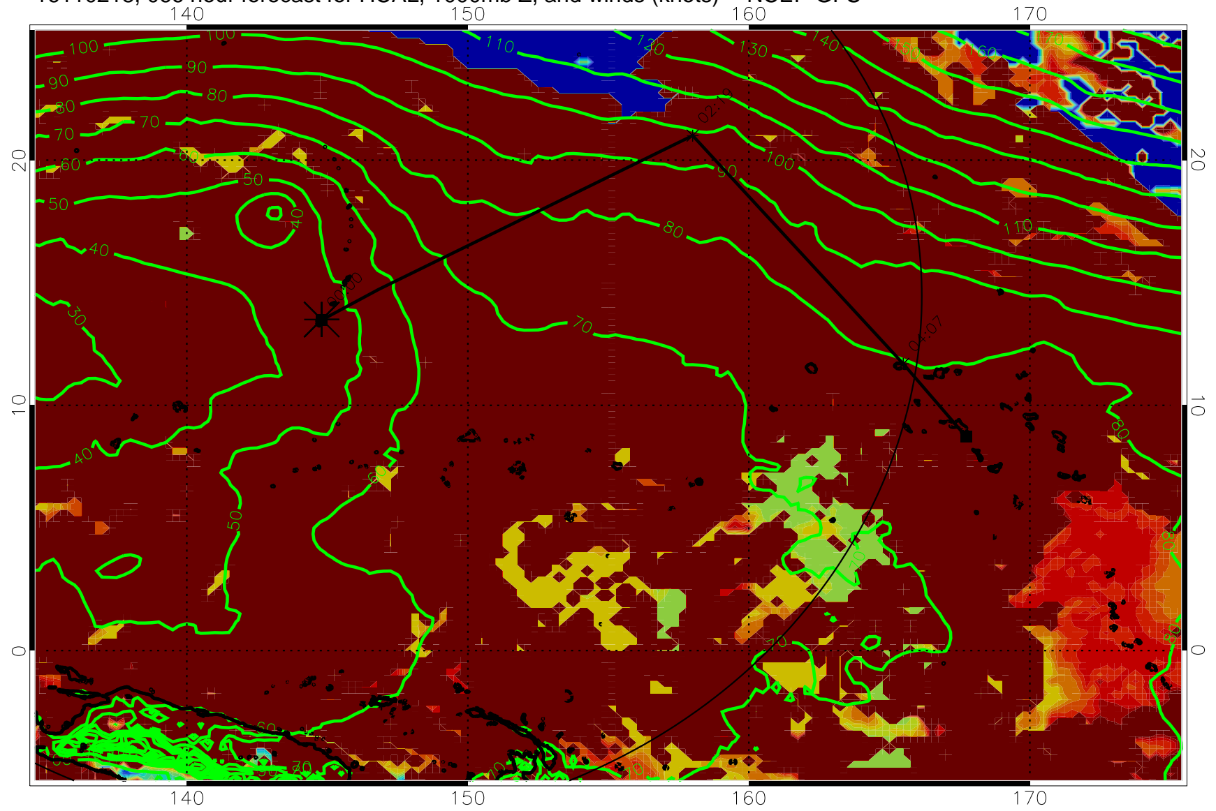
16110218, 066 hour forecast for HCAL, 1000mb Z, and winds (knots) -- NCEP GFS
