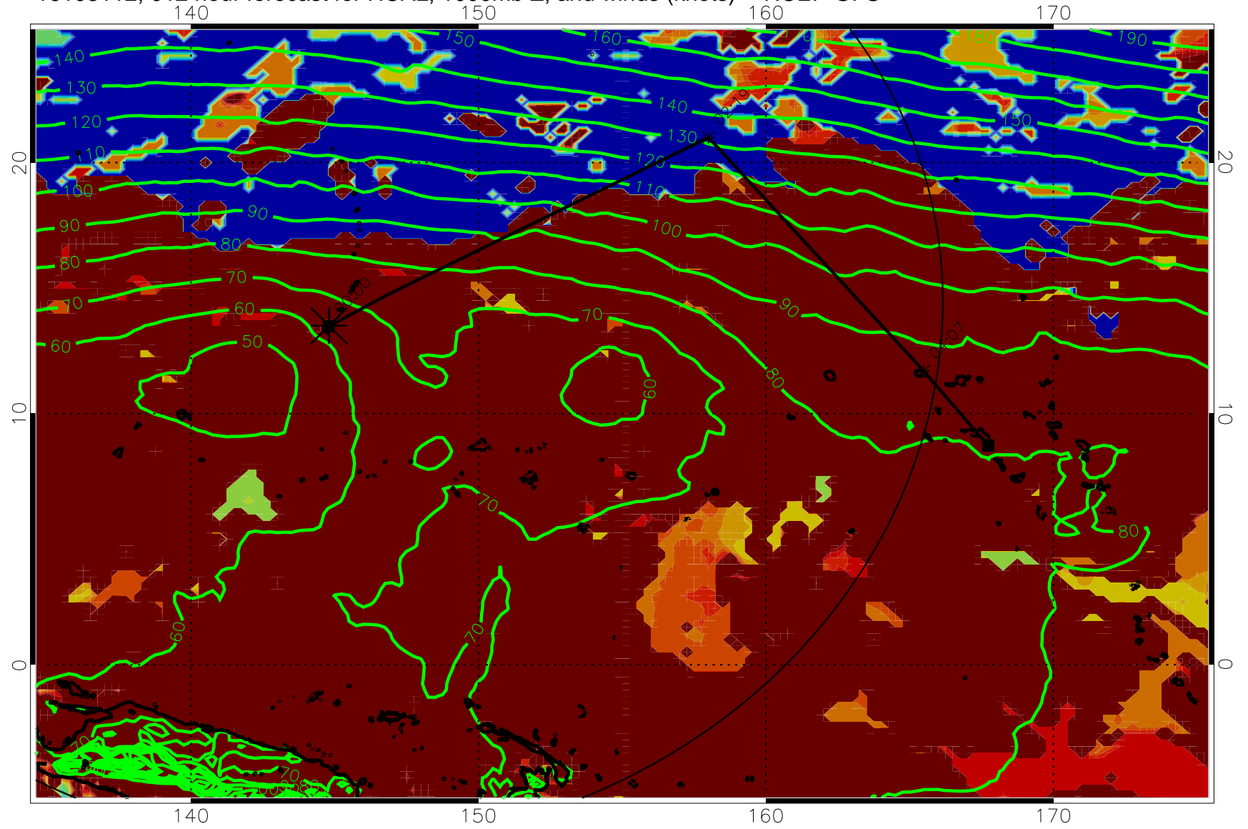
16103112, 012 hour forecast for HCAL, 1000mb Z, and winds (knots) -- NCEP GFS
