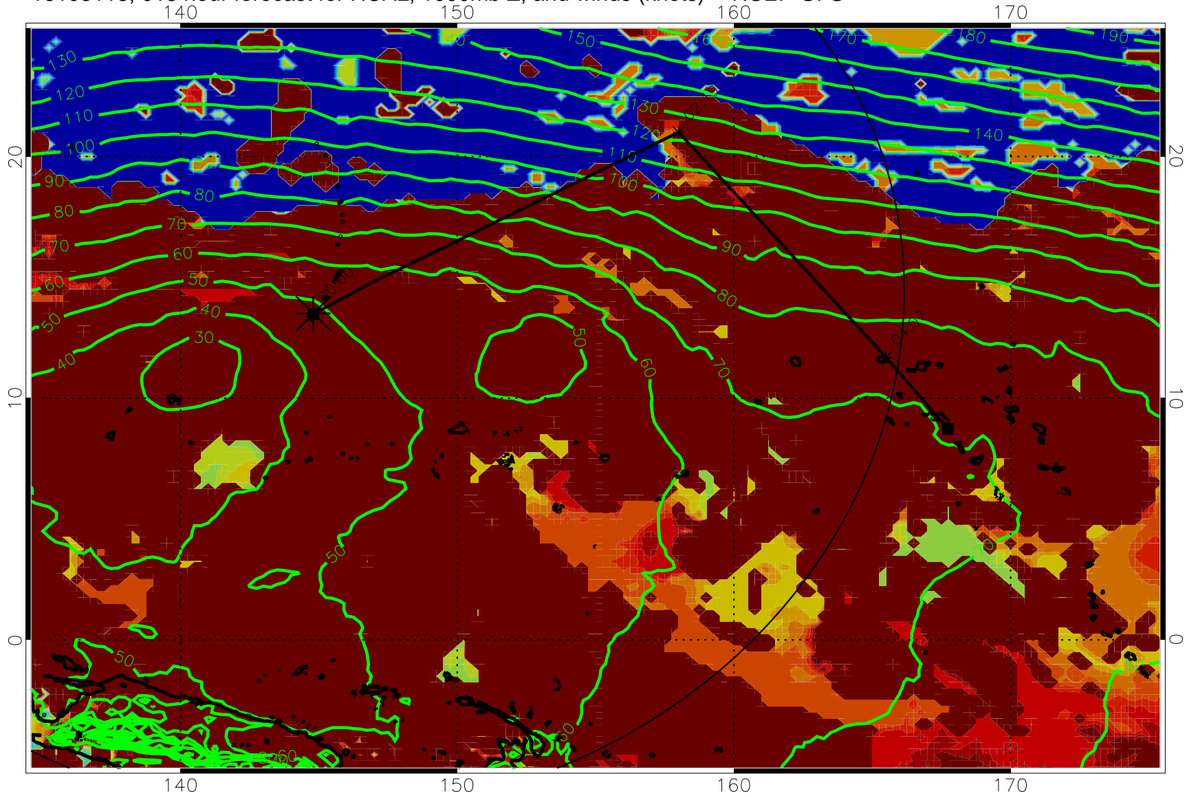
16103118, 018 hour forecast for HCAL, 1000mb Z, and winds (knots) -- NCEP GFS
