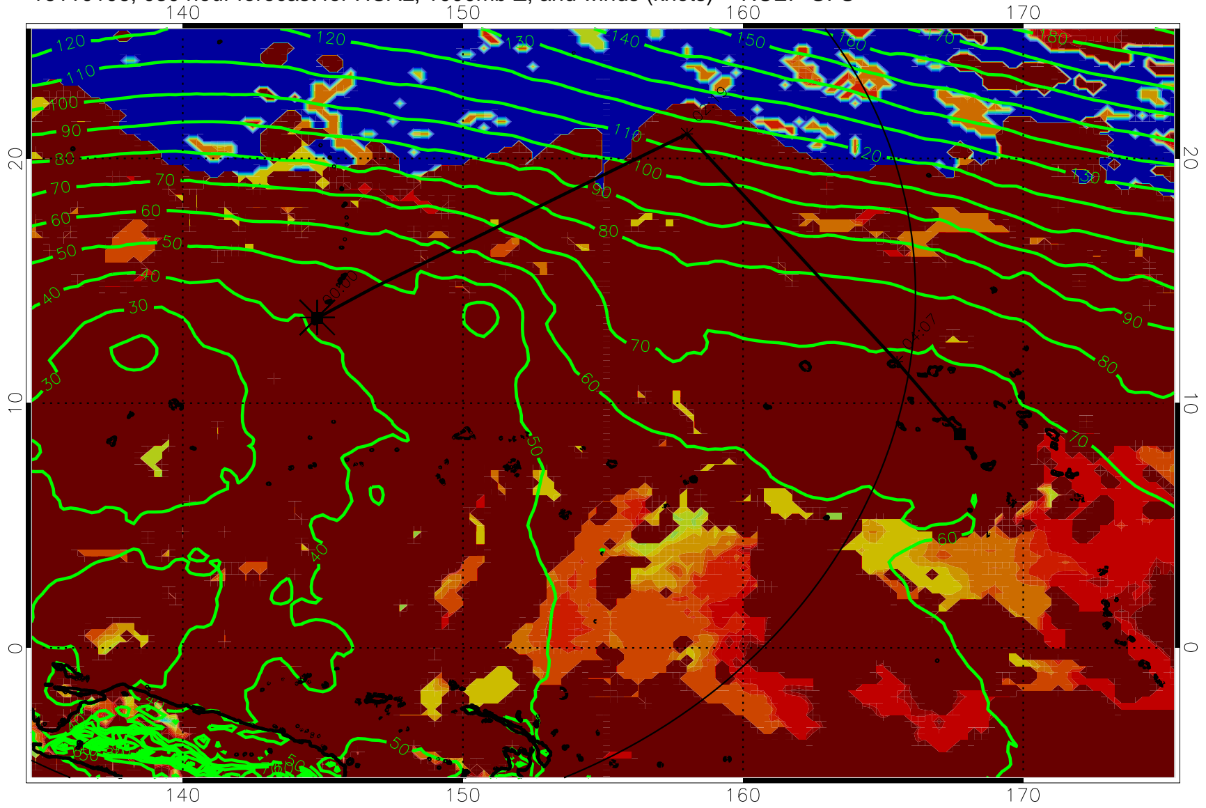
16110106, 030 hour forecast for HCAL, 1000mb Z, and winds (knots) -- NCEP GFS
