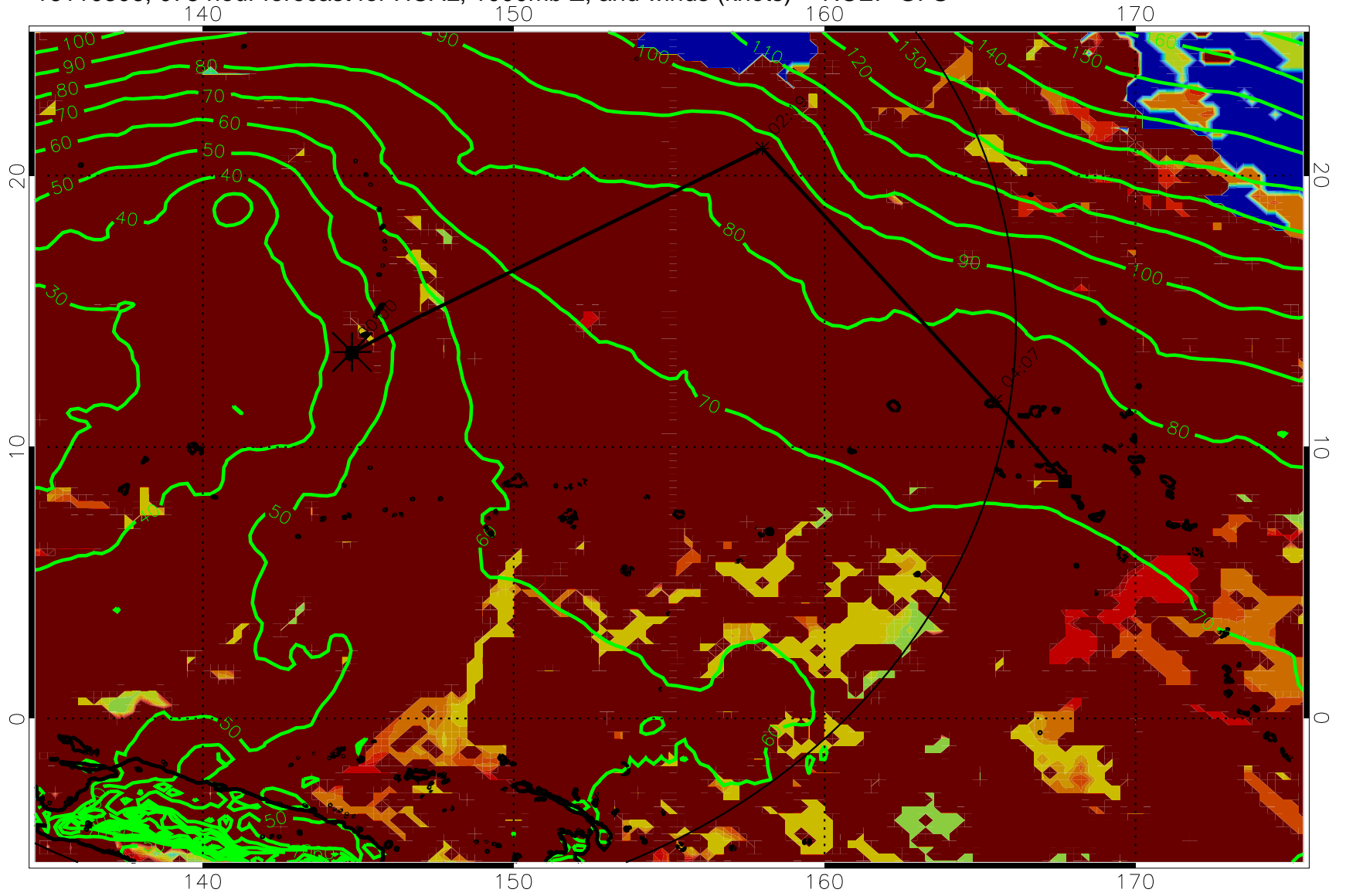
16110306, 078 hour forecast for HCAL, 1000mb Z, and winds (knots) -- NCEP GFS
