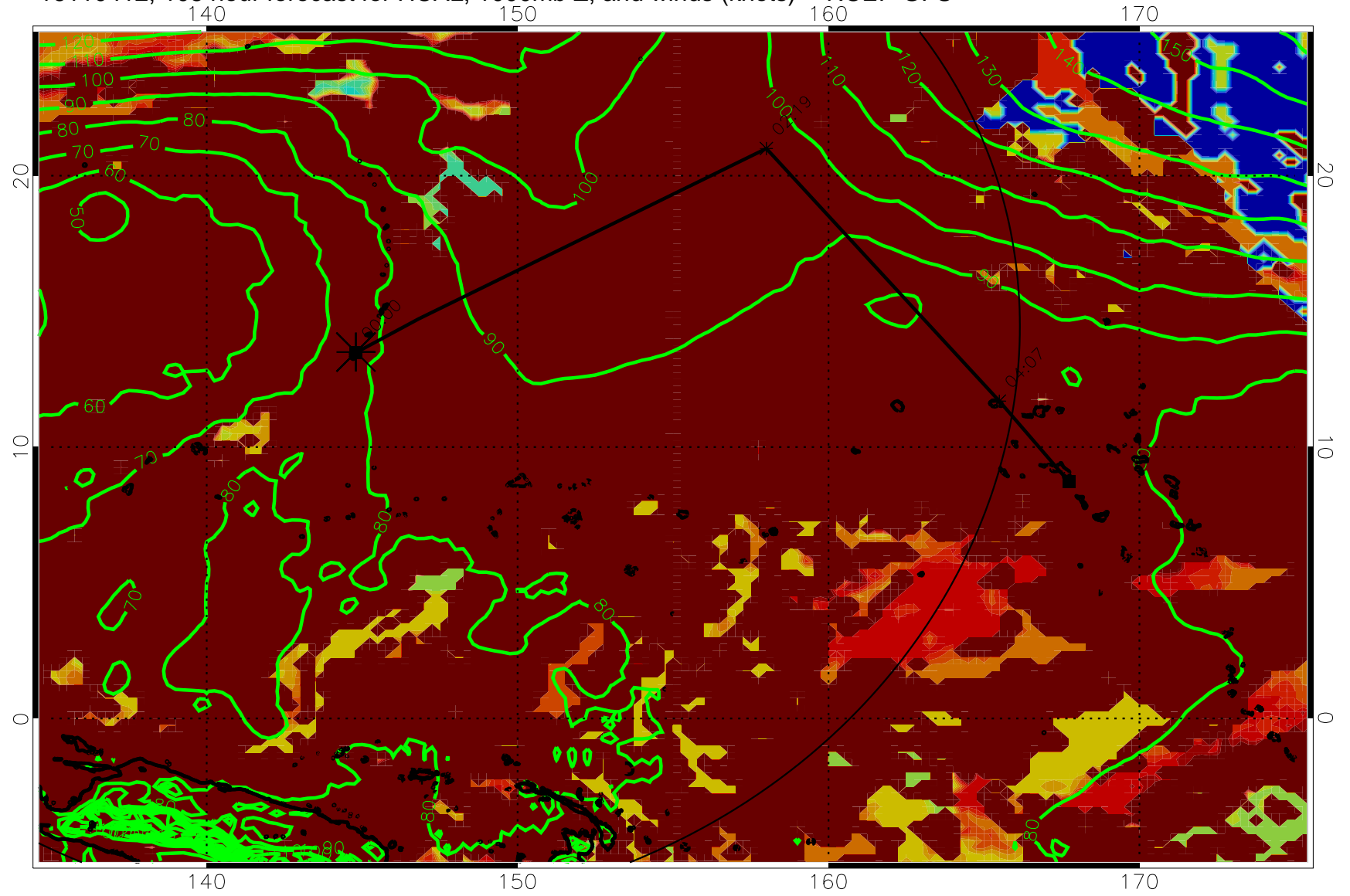
16110412, 108 hour forecast for HCAL, 1000mb Z, and winds (knots) -- NCEP GFS
