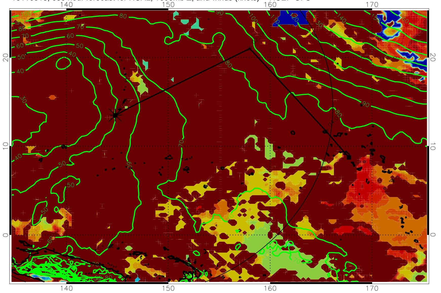
16110318, 090 hour forecast for HCAL, 1000mb Z, and winds (knots) -- NCEP GFS
