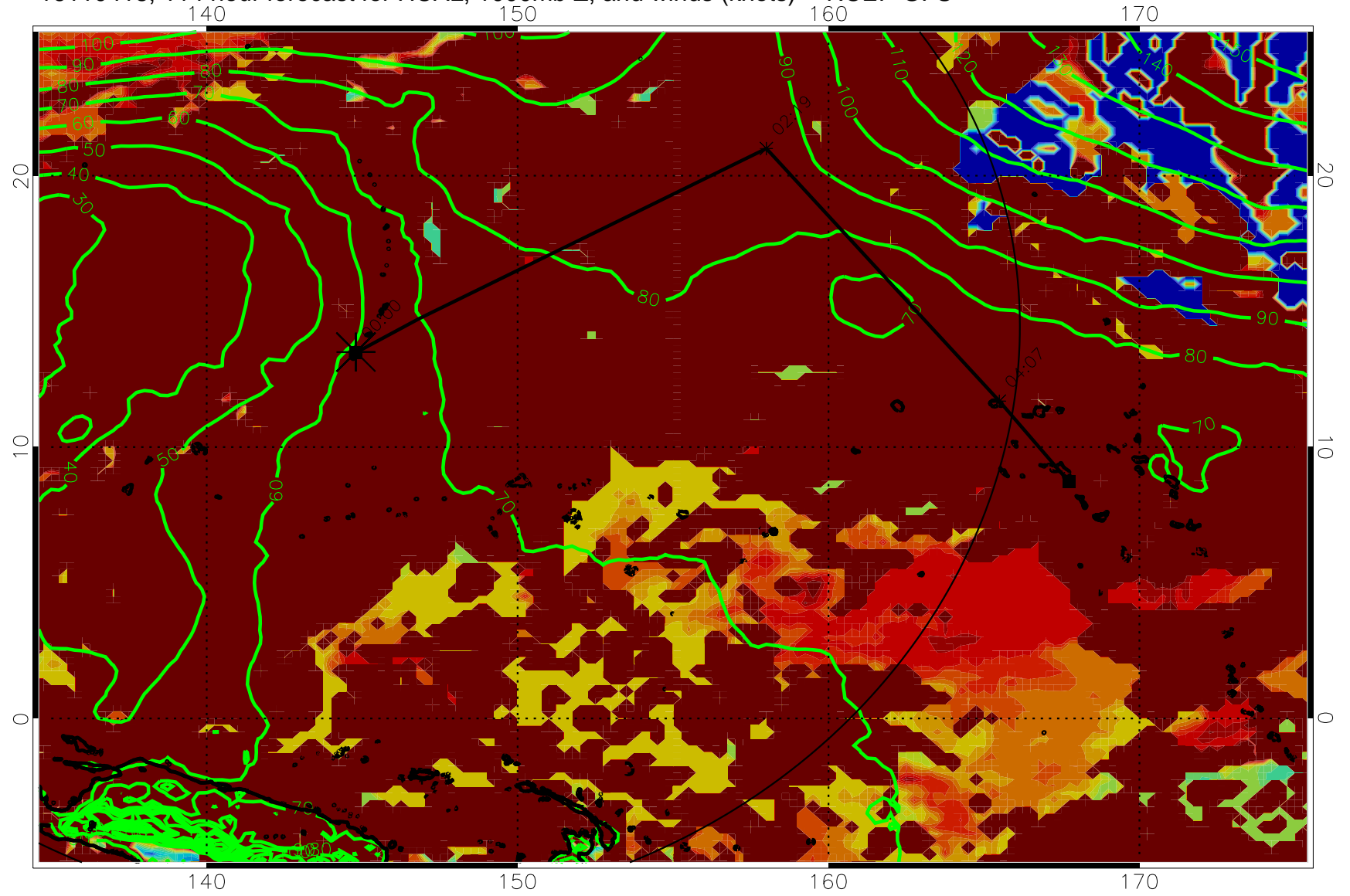
16110418, 114 hour forecast for HCAL, 1000mb Z, and winds (knots) -- NCEP GFS
