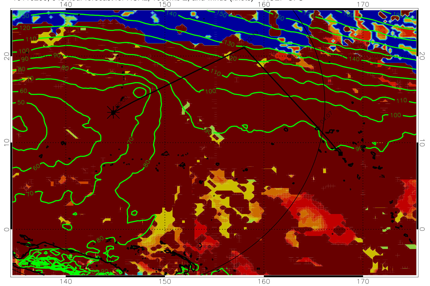
16110200, 048 hour forecast for HCAL, 1000mb Z, and winds (knots) -- NCEP GFS
