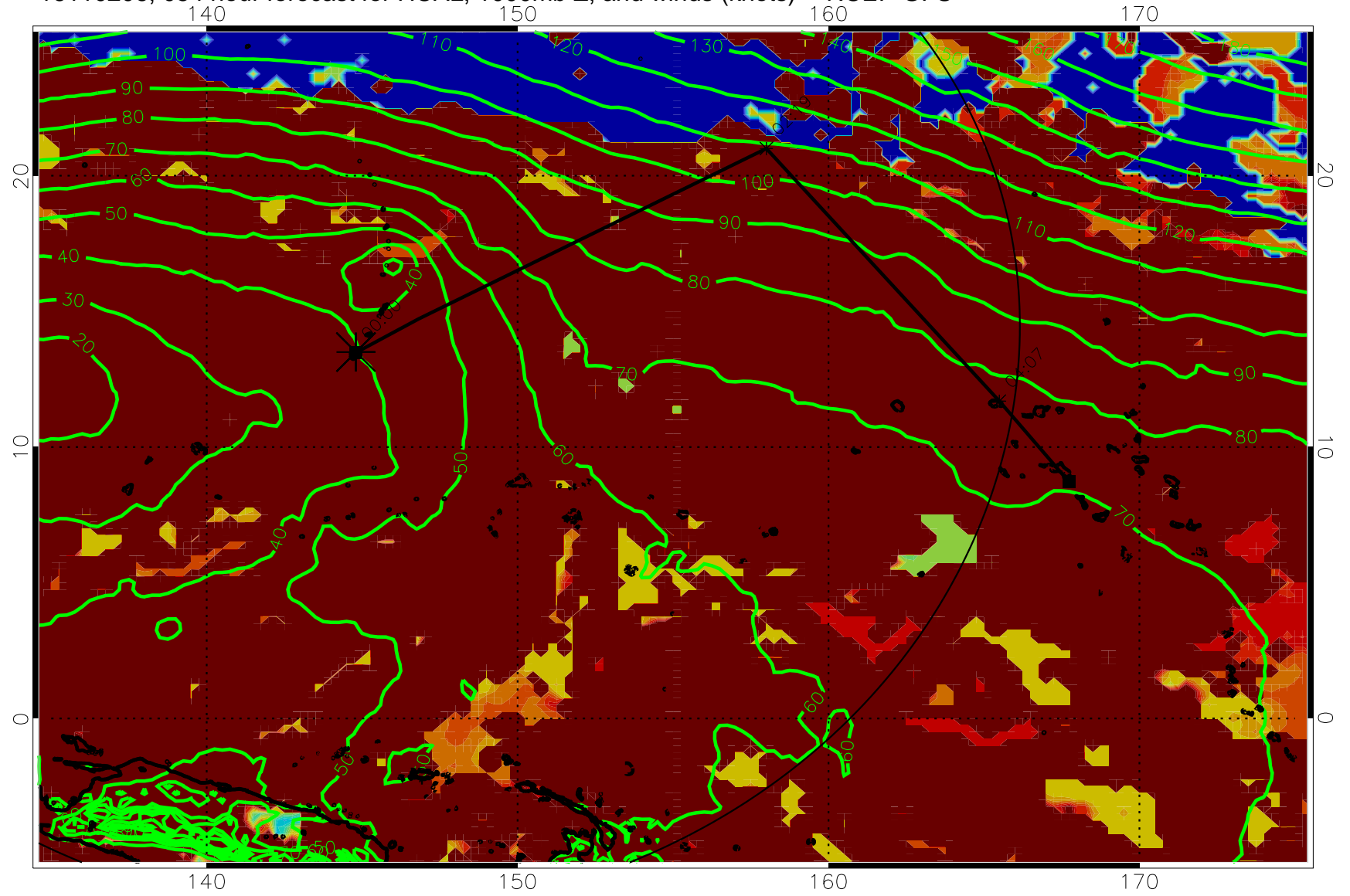
16110206, 054 hour forecast for HCAL, 1000mb Z, and winds (knots) -- NCEP GFS
