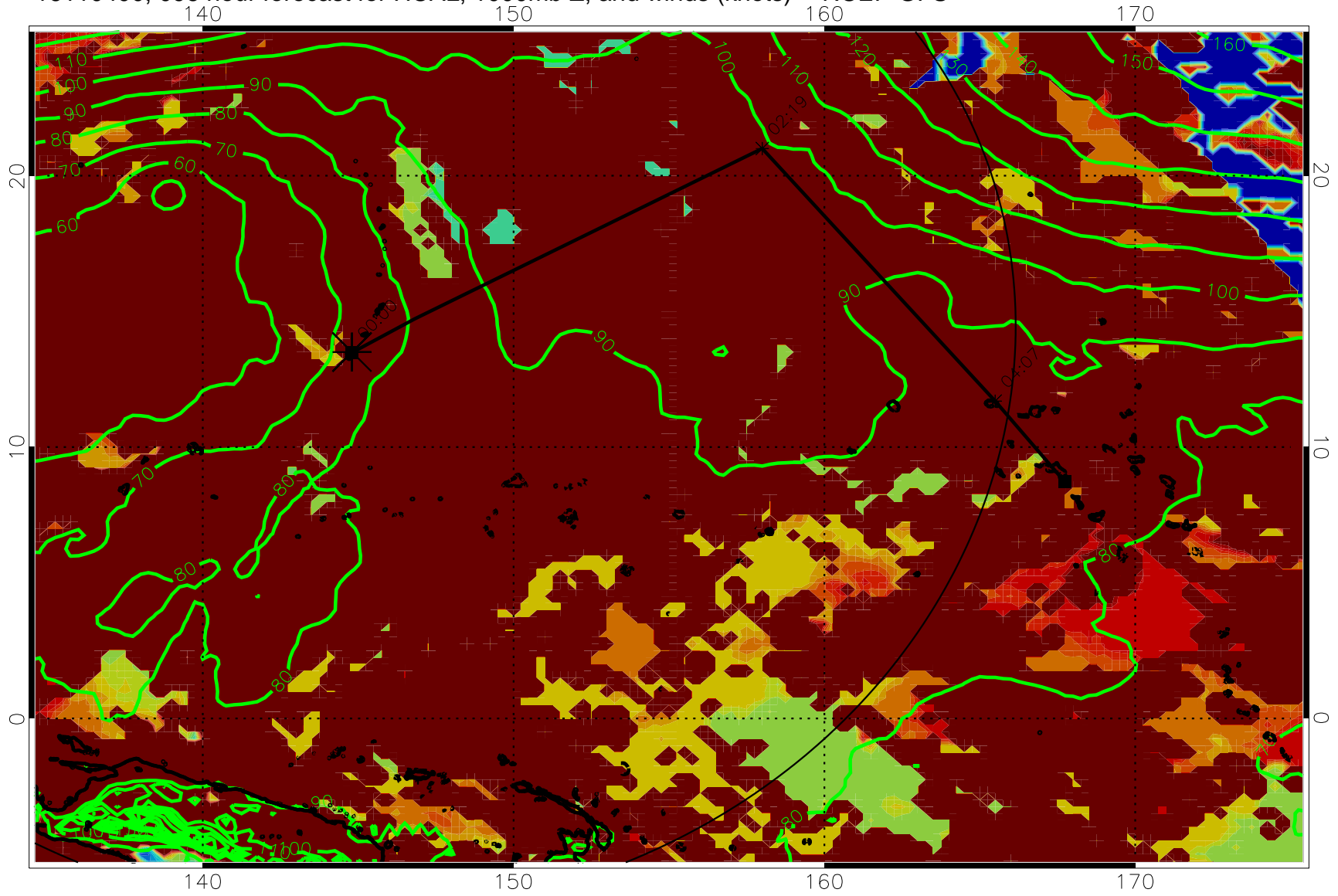
16110400, 096 hour forecast for HCAL, 1000mb Z, and winds (knots) -- NCEP GFS
