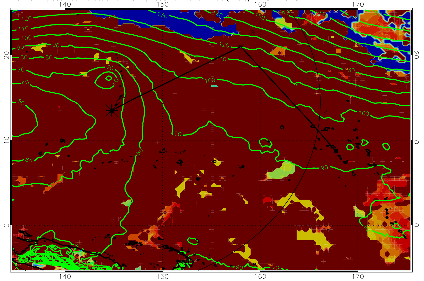
16110212, 060 hour forecast for HCAL, 1000mb Z, and winds (knots) -- NCEP GFS
