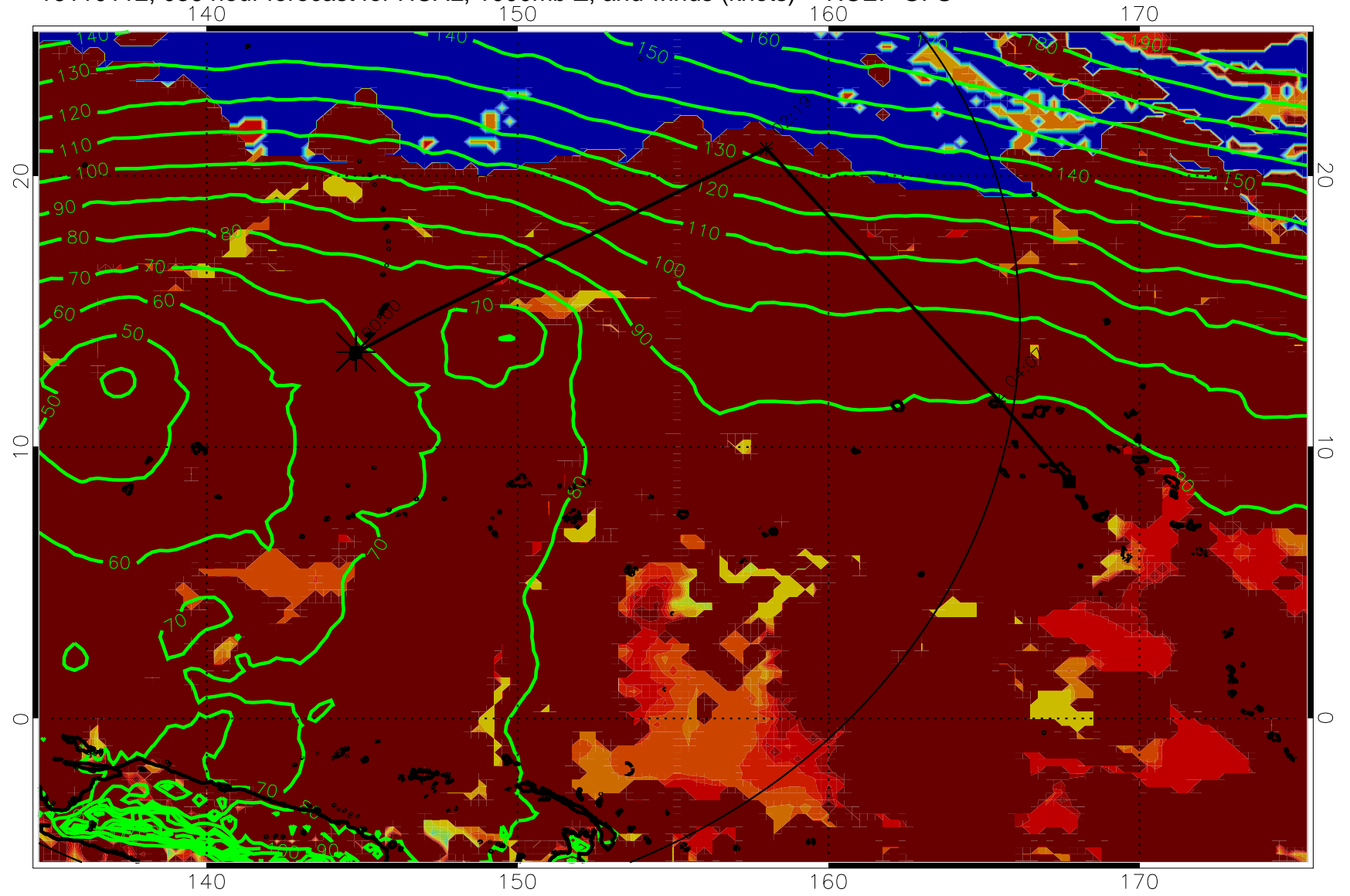
16110112, 036 hour forecast for HCAL, 1000mb Z, and winds (knots) -- NCEP GFS
