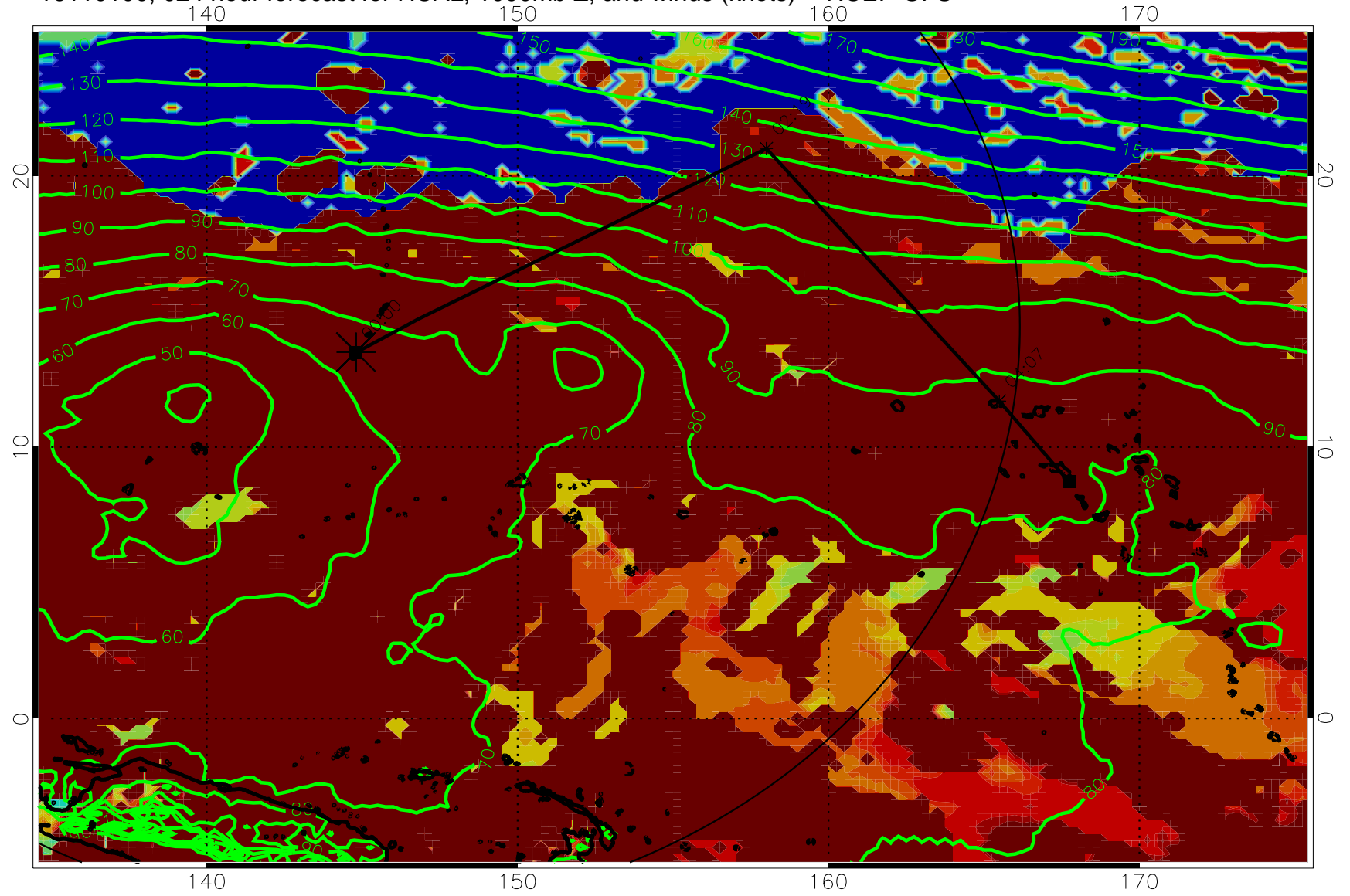
16110100, 024 hour forecast for HCAL, 1000mb Z, and winds (knots) -- NCEP GFS
