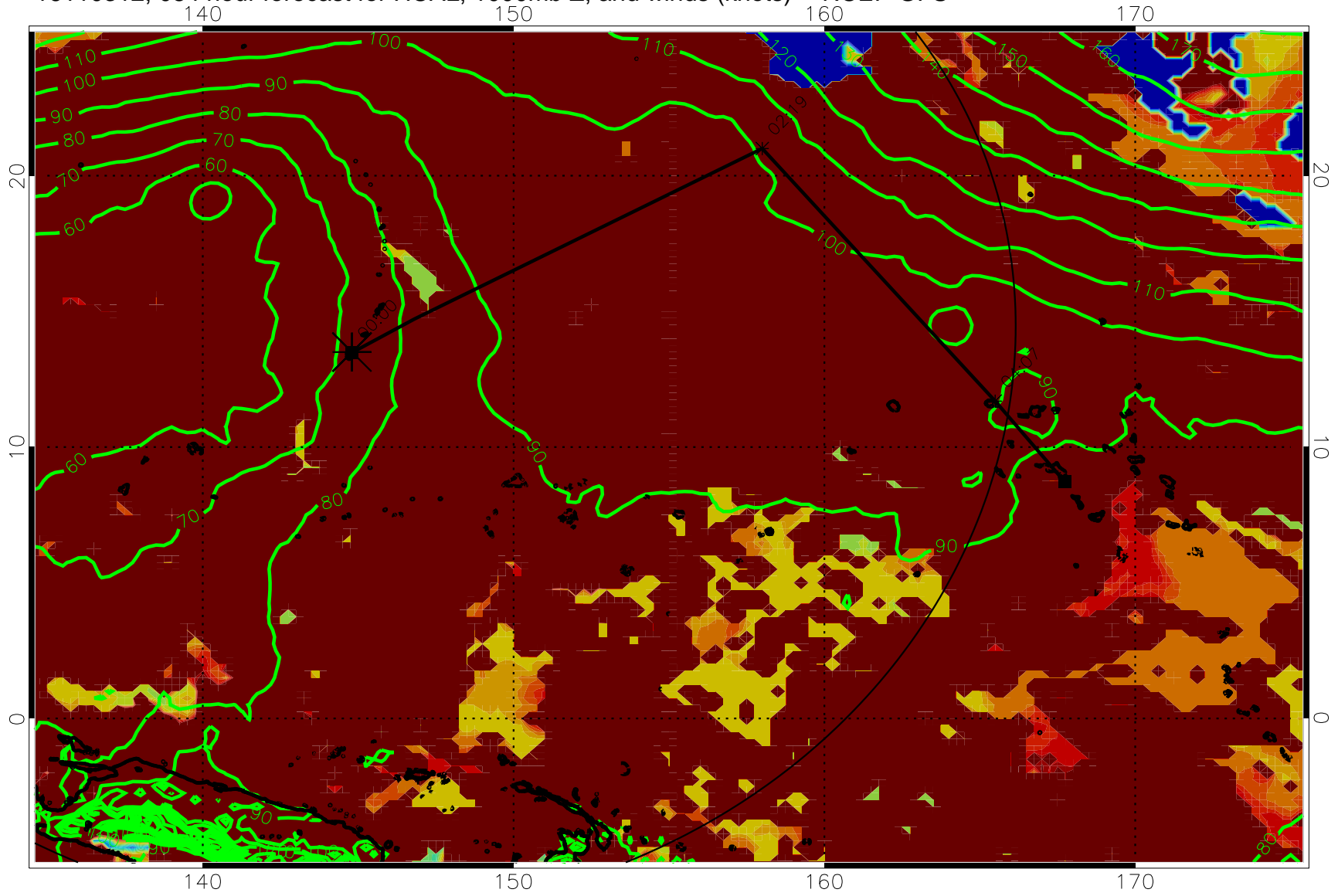
16110312, 084 hour forecast for HCAL, 1000mb Z, and winds (knots) -- NCEP GFS
