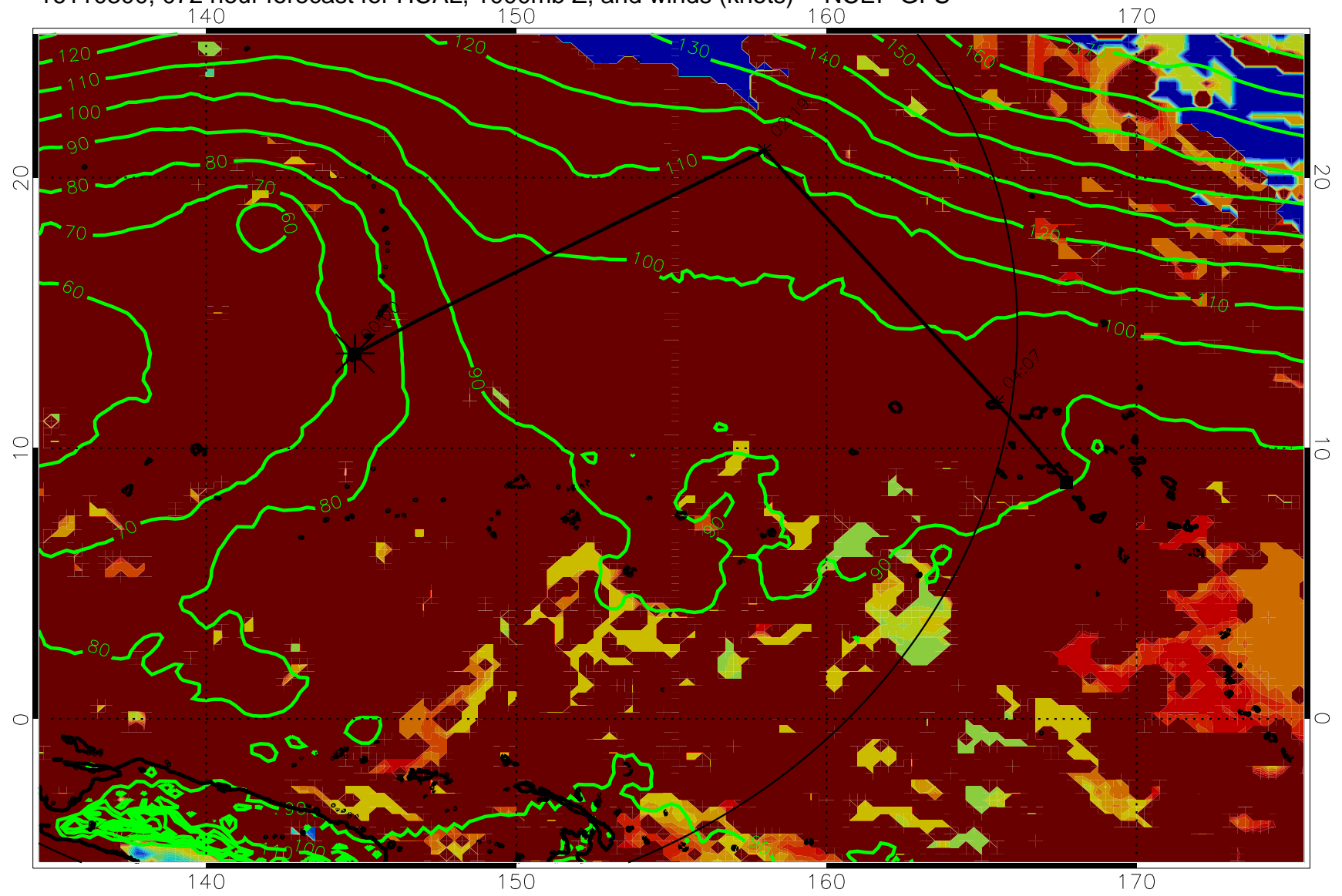
16110300, 072 hour forecast for HCAL, 1000mb Z, and winds (knots) -- NCEP GFS
