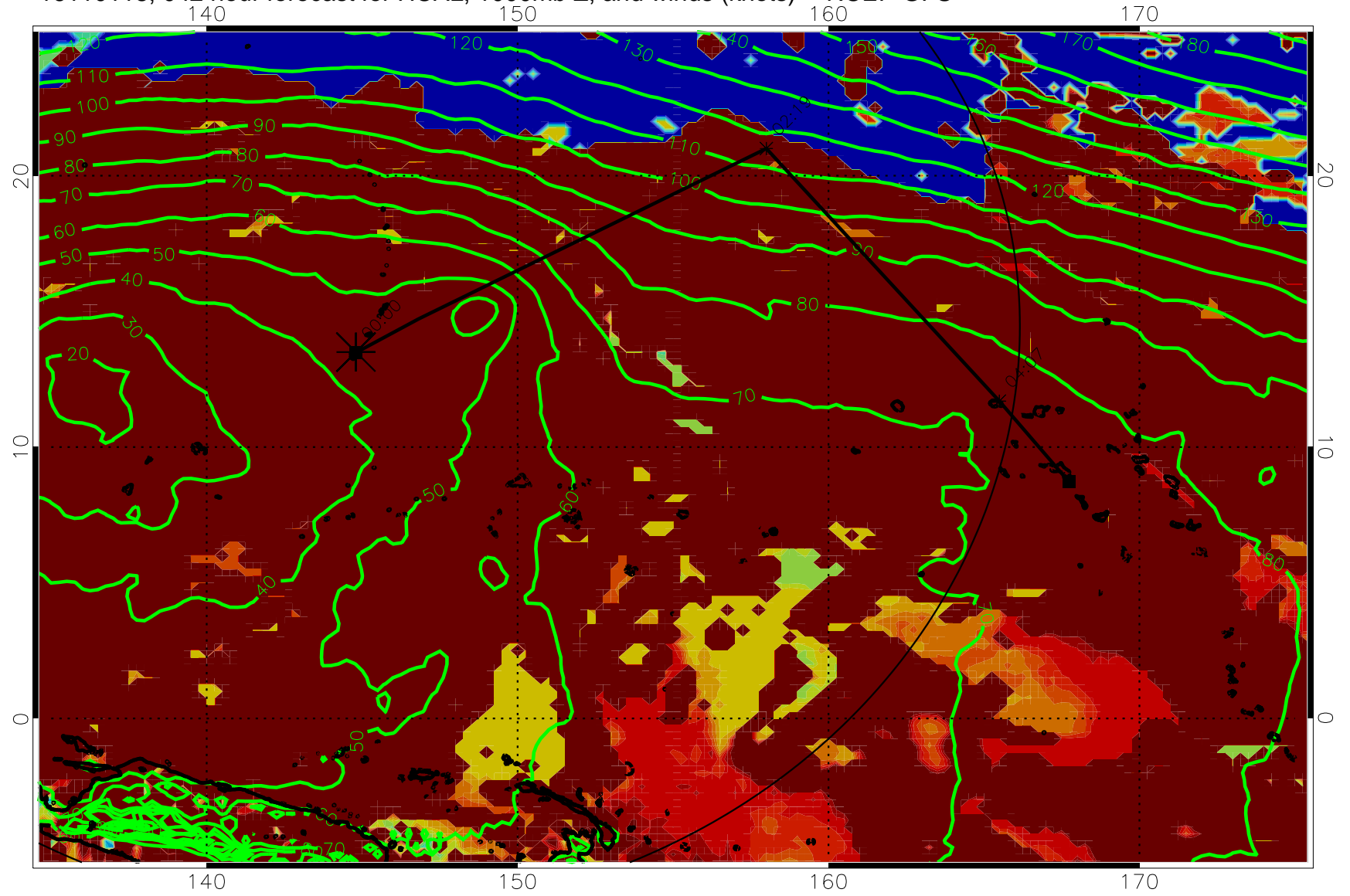
16110118, 042 hour forecast for HCAL, 1000mb Z, and winds (knots) -- NCEP GFS
