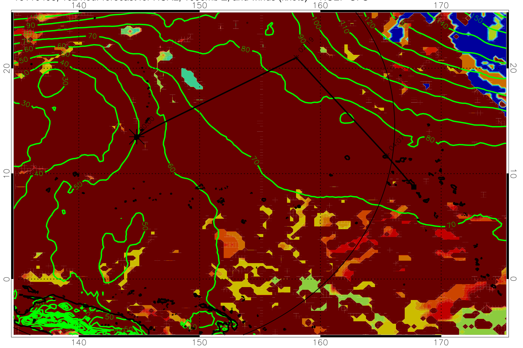
16110406, 102 hour forecast for HCAL, 1000mb Z, and winds (knots) -- NCEP GFS
