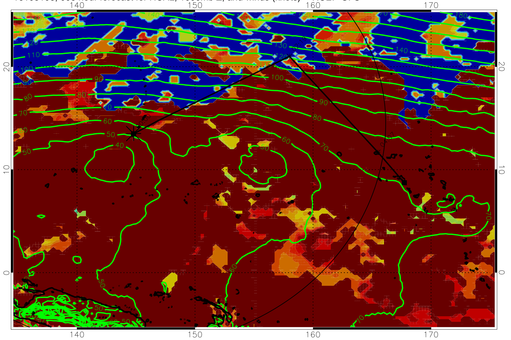
16103106, 006 hour forecast for HCAL, 1000mb Z, and winds (knots) -- NCEP GFS
