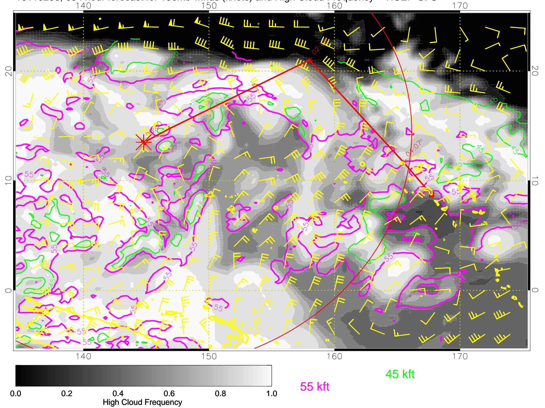
16110206, 054 hour forecast for 150mb winds (knots) and High Cloud Frequency -- NCEP GFS
