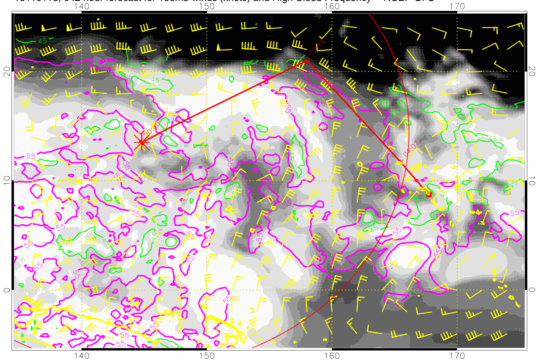
16110118, 04Z hour forecast for 150mb winds (knots) and High Cloud Frequency -- NCEP GFS
