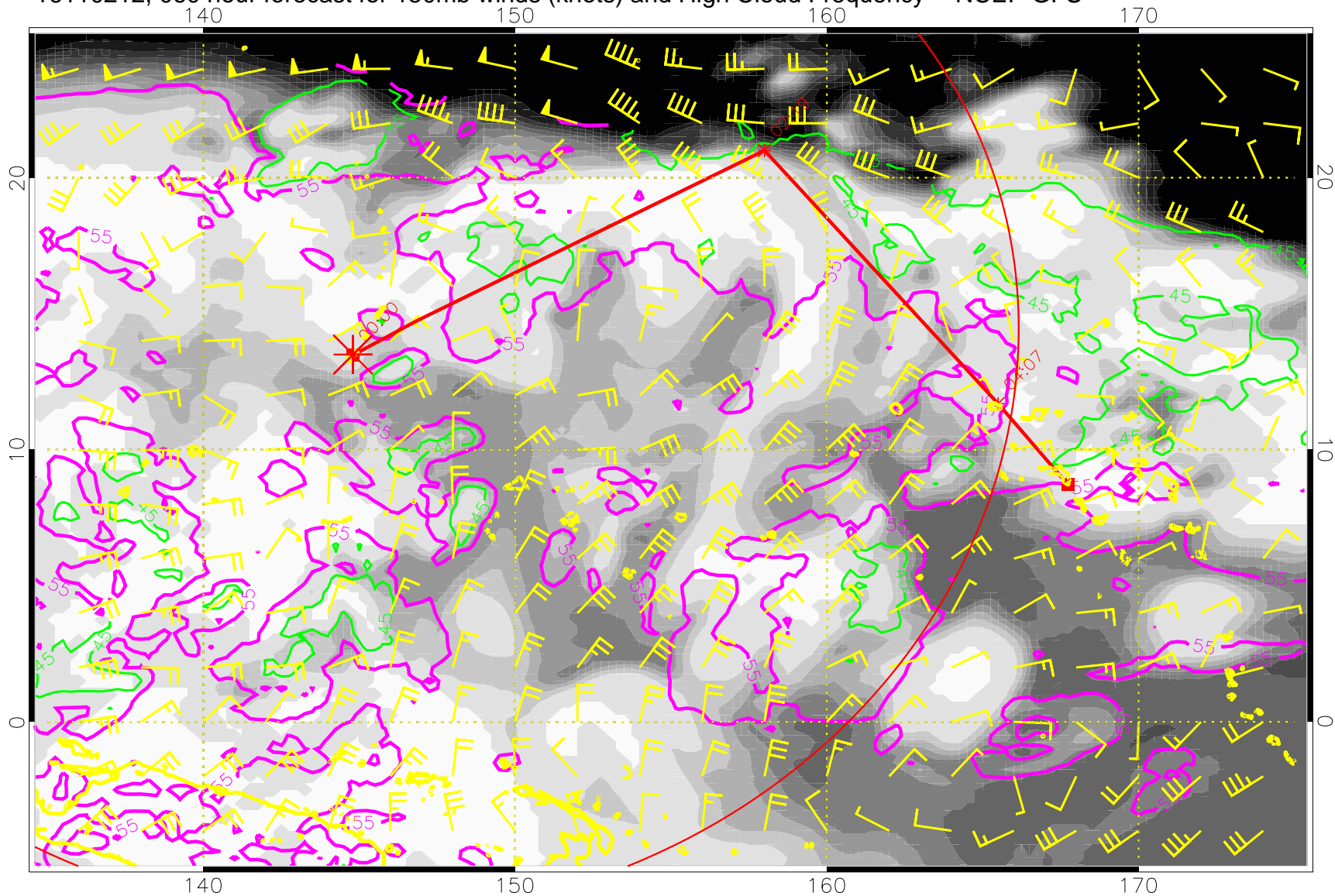
16110212, 060 hour forecast for 150mb winds (knots) and High Cloud Frequency -- NCEP GFS
