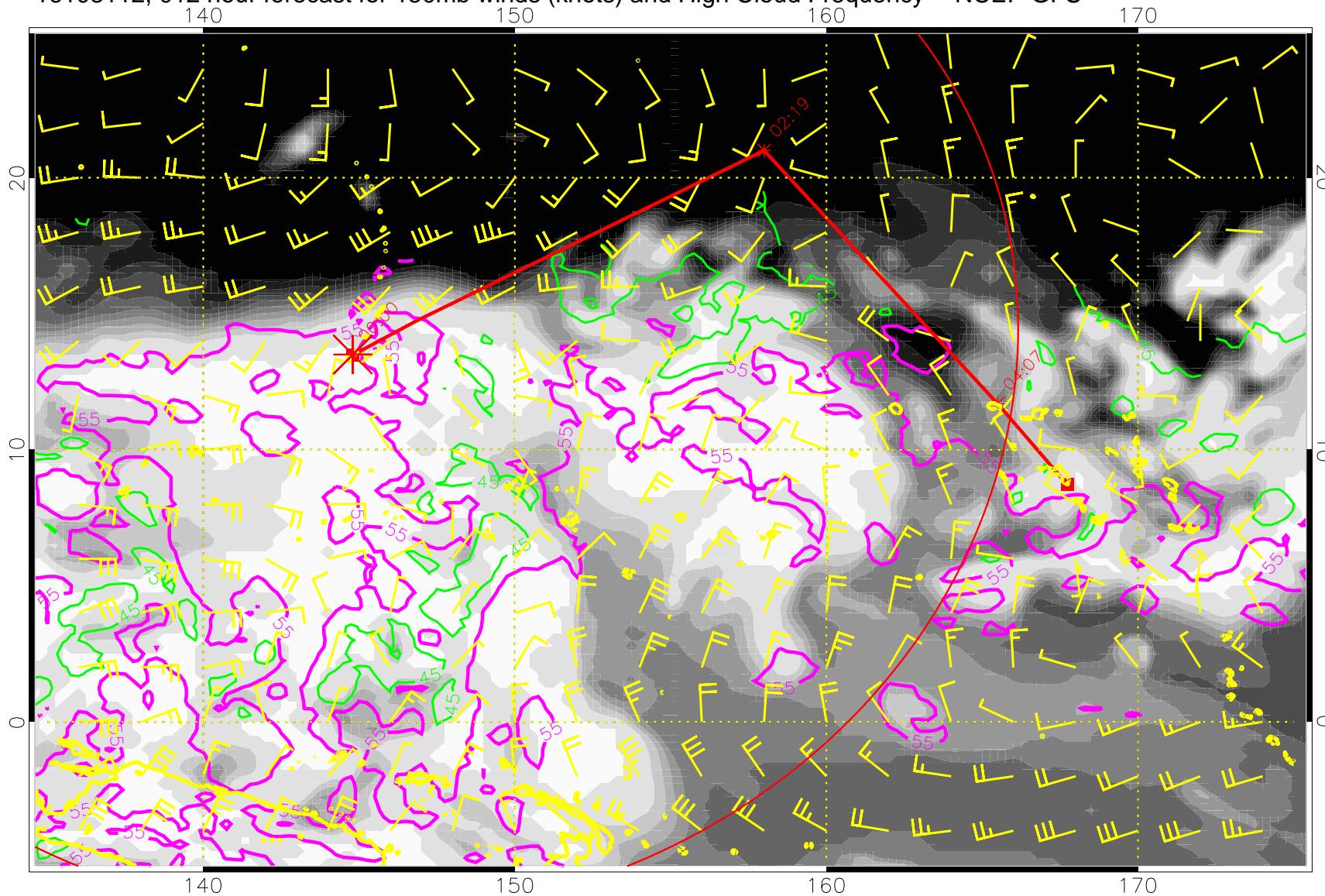
16103112, 012 hour forecast for 150mb winds (knots) and High Cloud Frequency -- NCEP GFS
