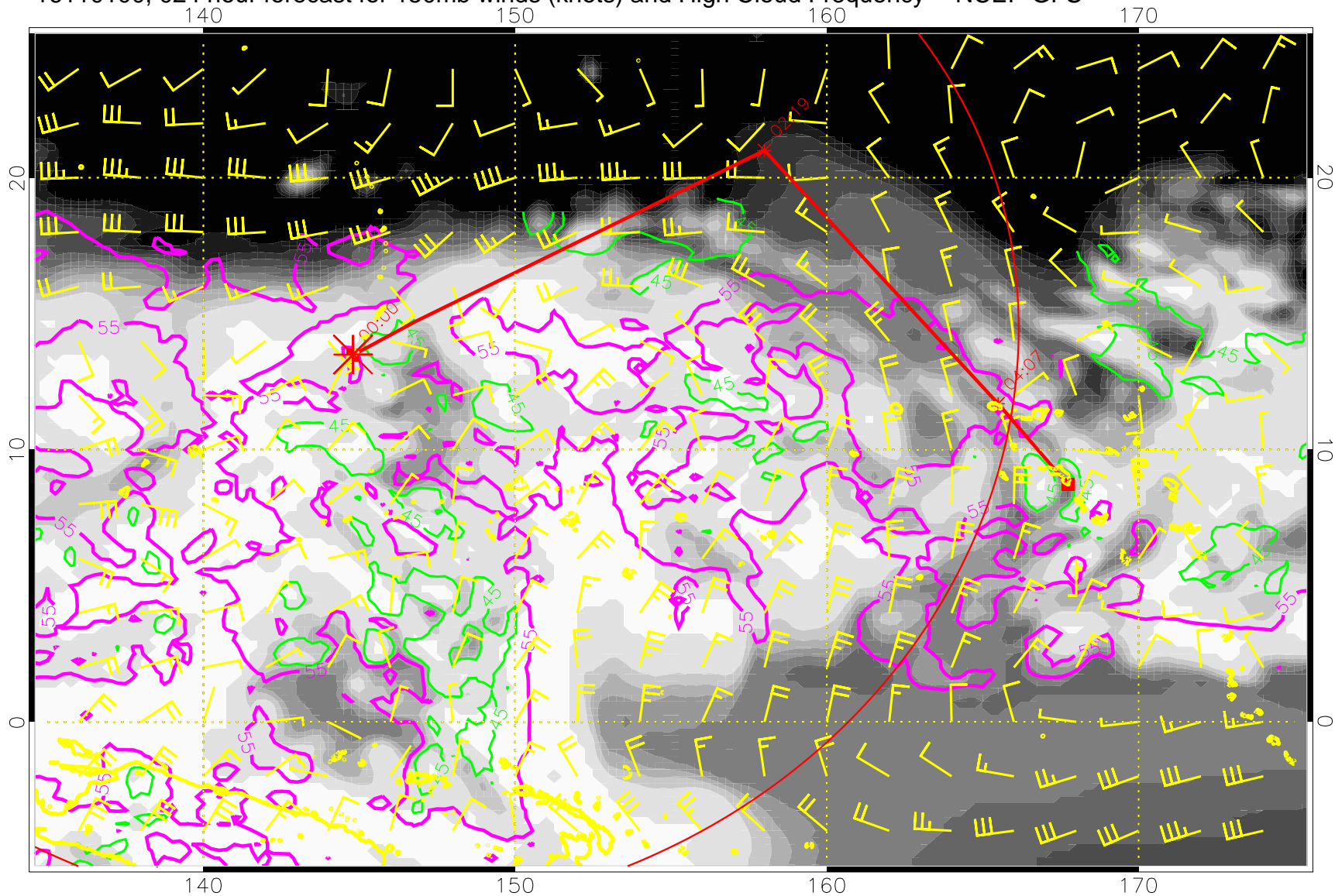
16110100, 024 hour forecast for 150mb winds (knots) and High Cloud Frequency -- NCEP GFS
