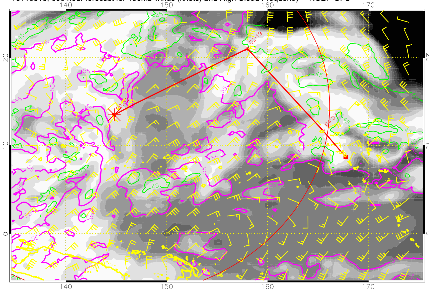
16110318, 090 hour forecast for 150mb winds (knots) and High Cloud Frequency -- NCEP GFS
