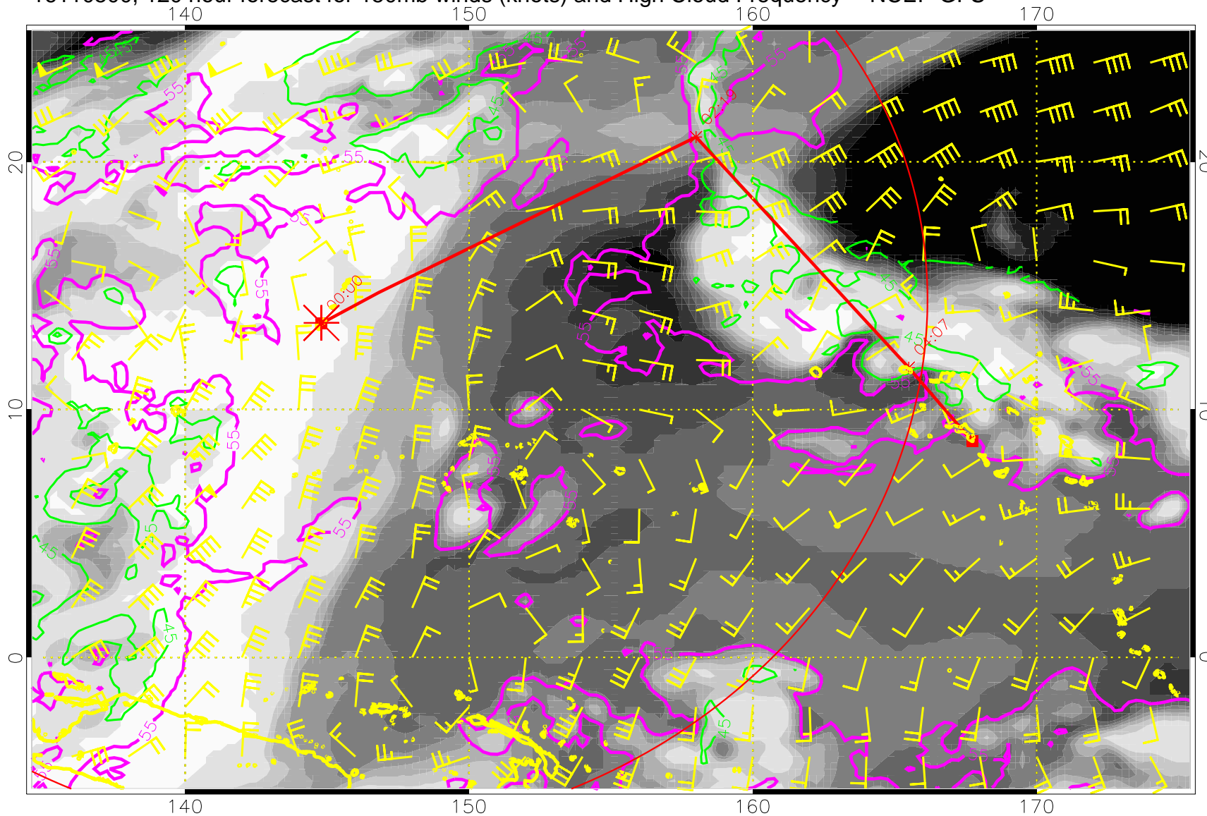
16110500, 120 hour forecast for 150mb winds (knots) and High Cloud Frequency -- NCEP GFS
