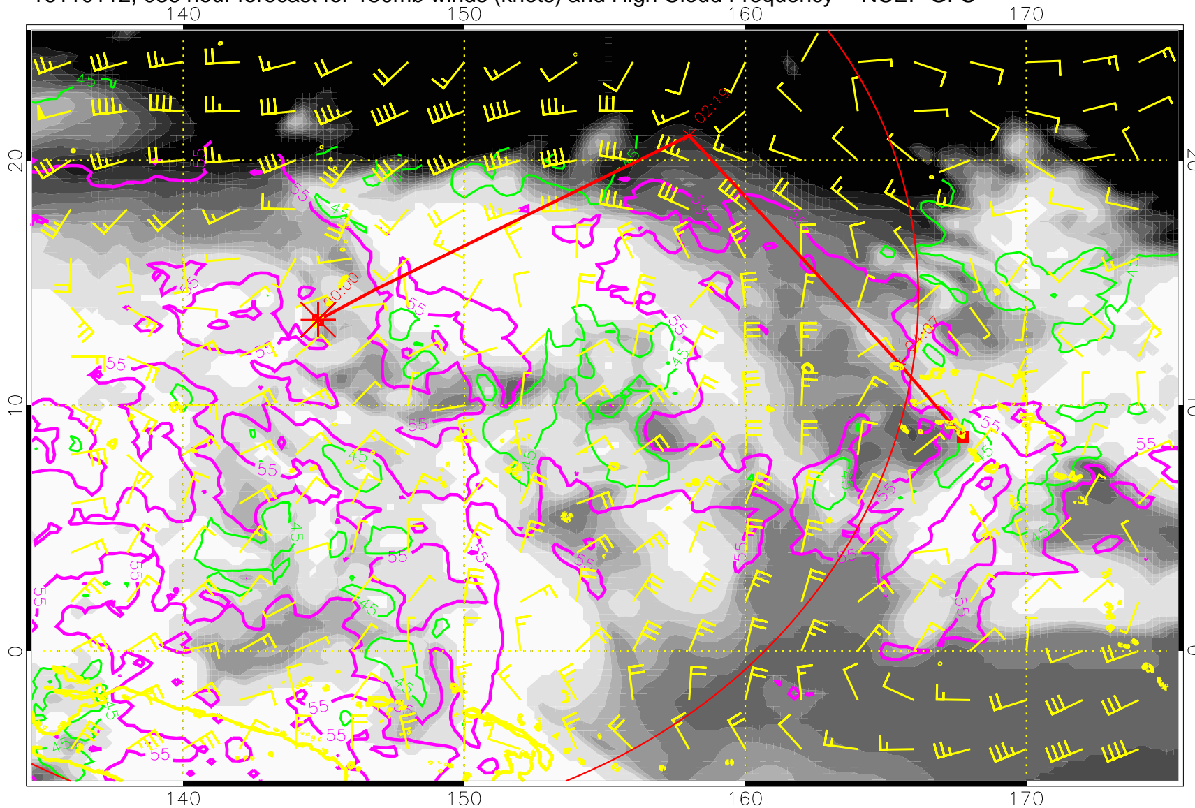
16110112, 036 hour forecast for 150mb winds (knots) and High Cloud Frequency -- NCEP GFS
