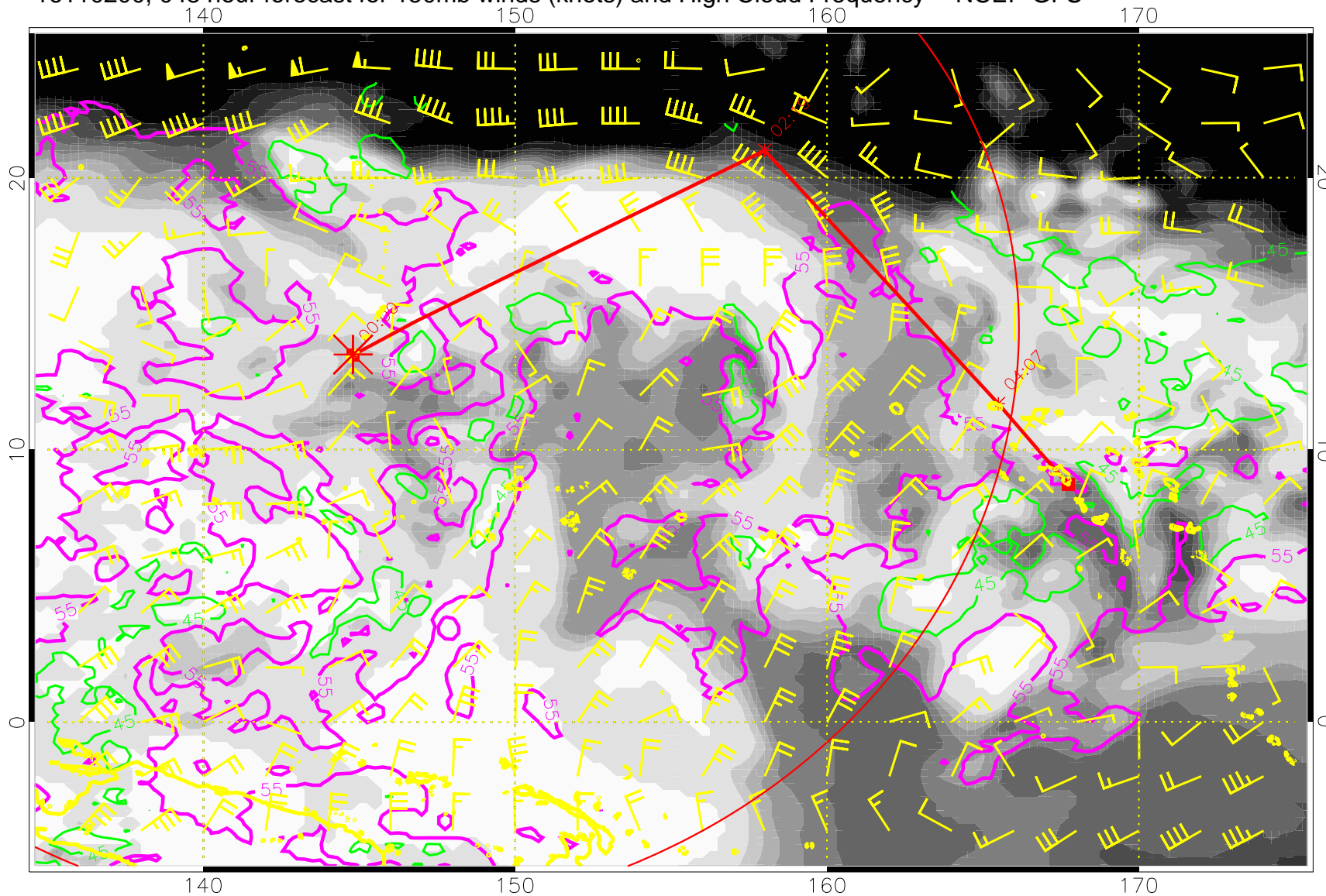
16110200, 048 hour forecast for 150mb winds (knots) and High Cloud Frequency -- NCEP GFS
