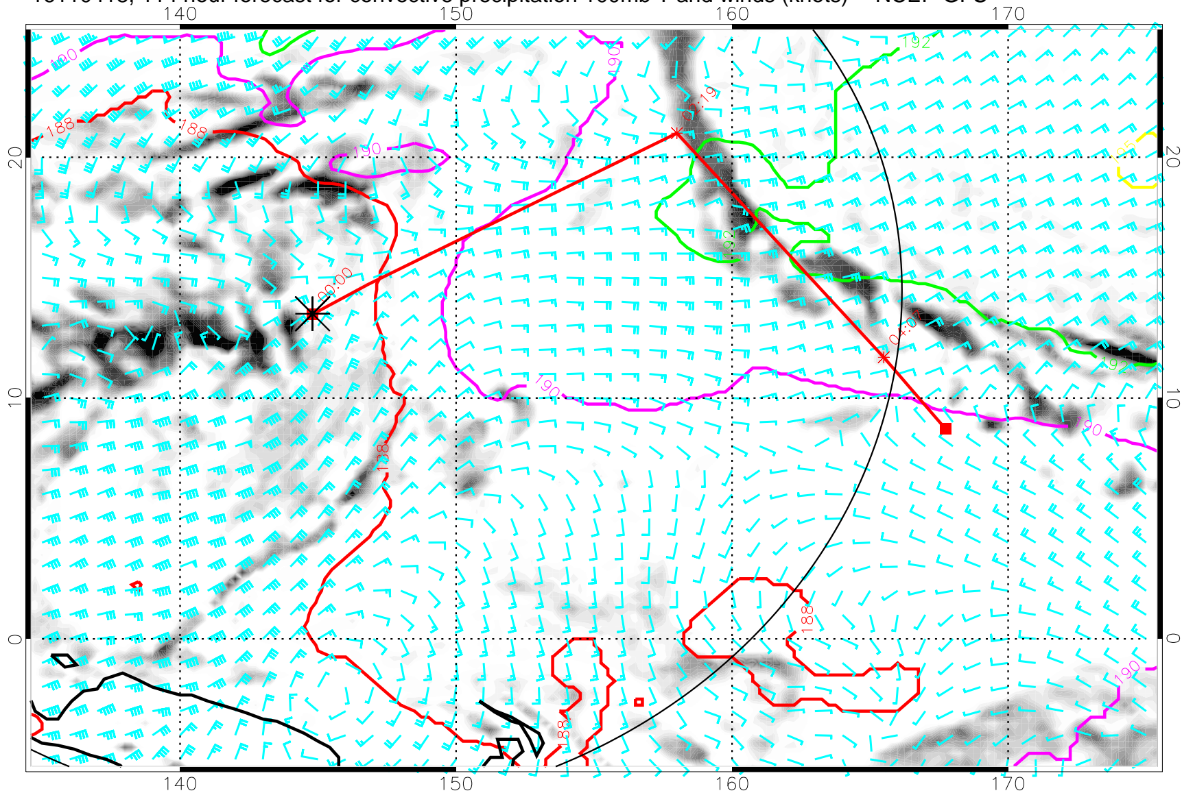
16110418, 114 hour forecast for convective precipitation 100mb T and winds (knots) -- NCEP GFS
