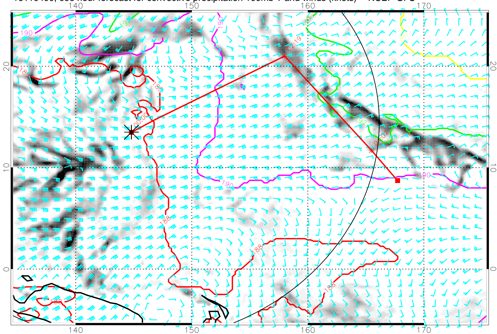
16110400, 096 hour forecast for convective precipitation 100mb T and winds (knots) -- NCEP GFS
