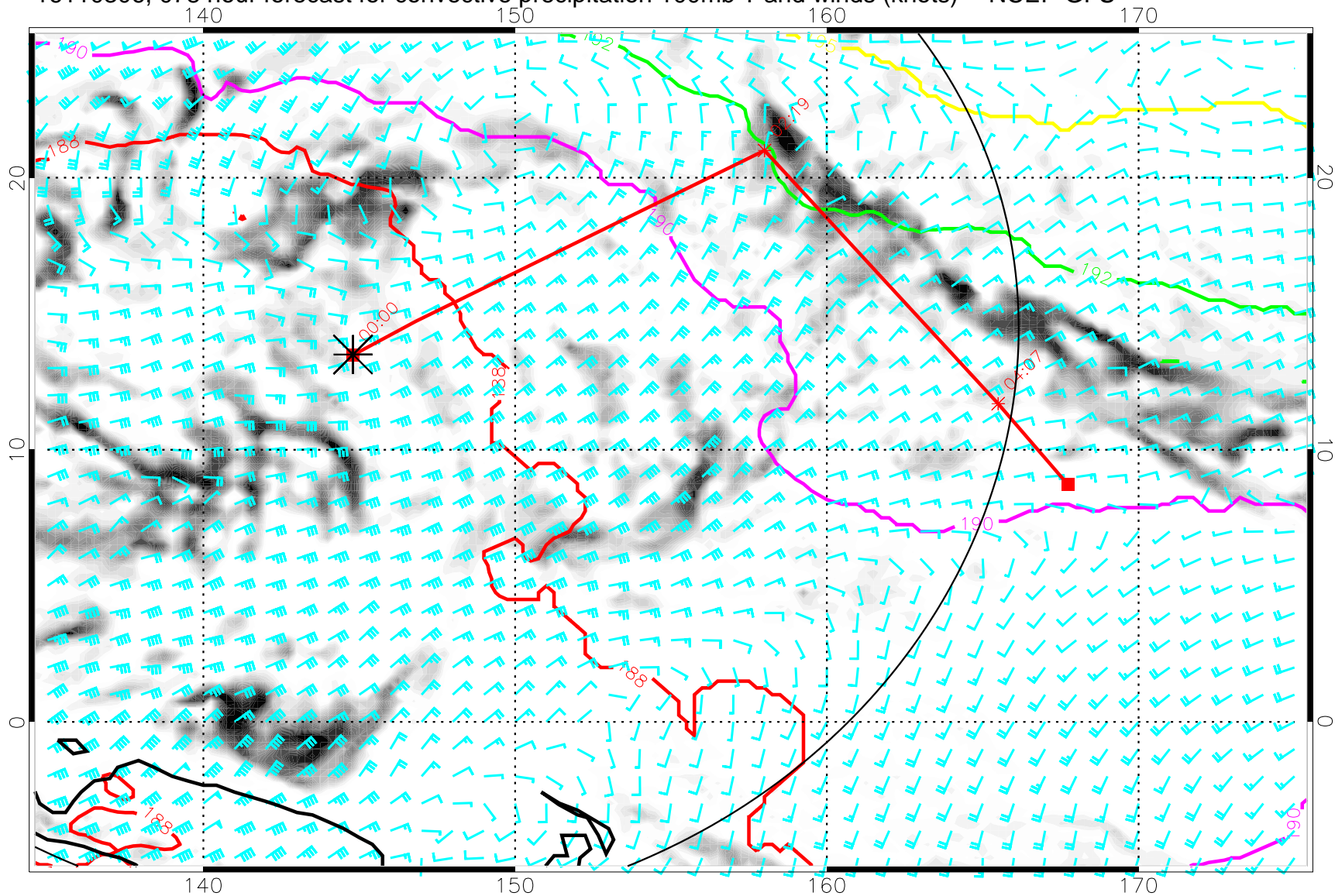
16110306, 078 hour forecast for convective precipitation 100mb T and winds (knots) -- NCEP GFS
