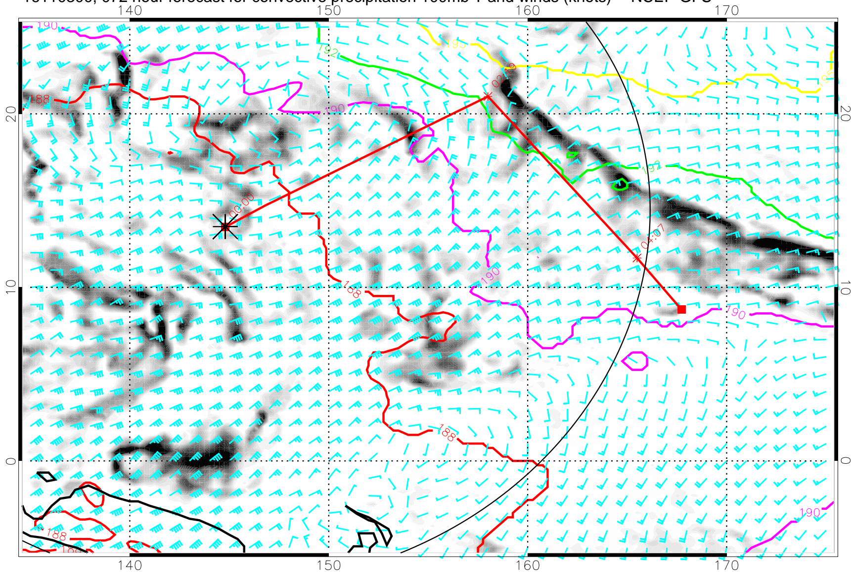
16110300, 072 hour forecast for convective precipitation 100mb T and winds (knots) -- NCEP GFS
