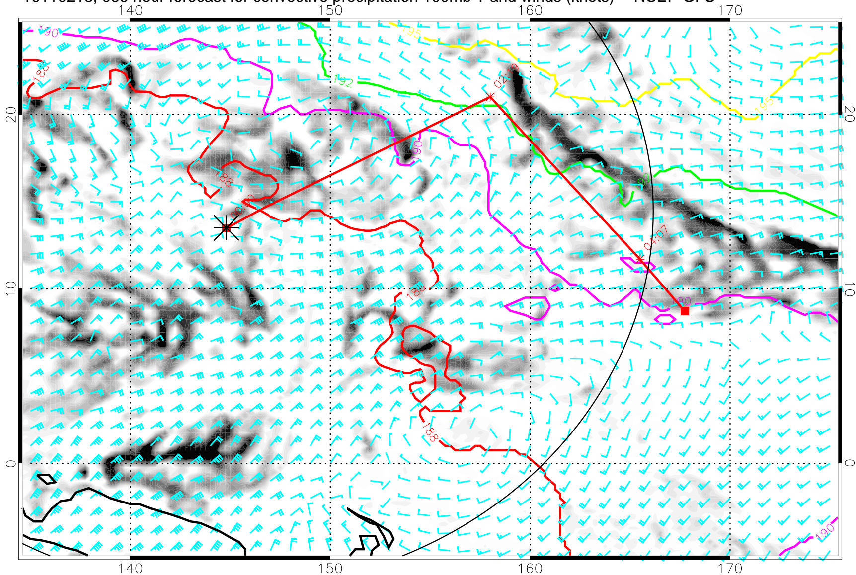
16110218, 066 hour forecast for convective precipitation 100mb T and winds (knots) -- NCEP GFS
