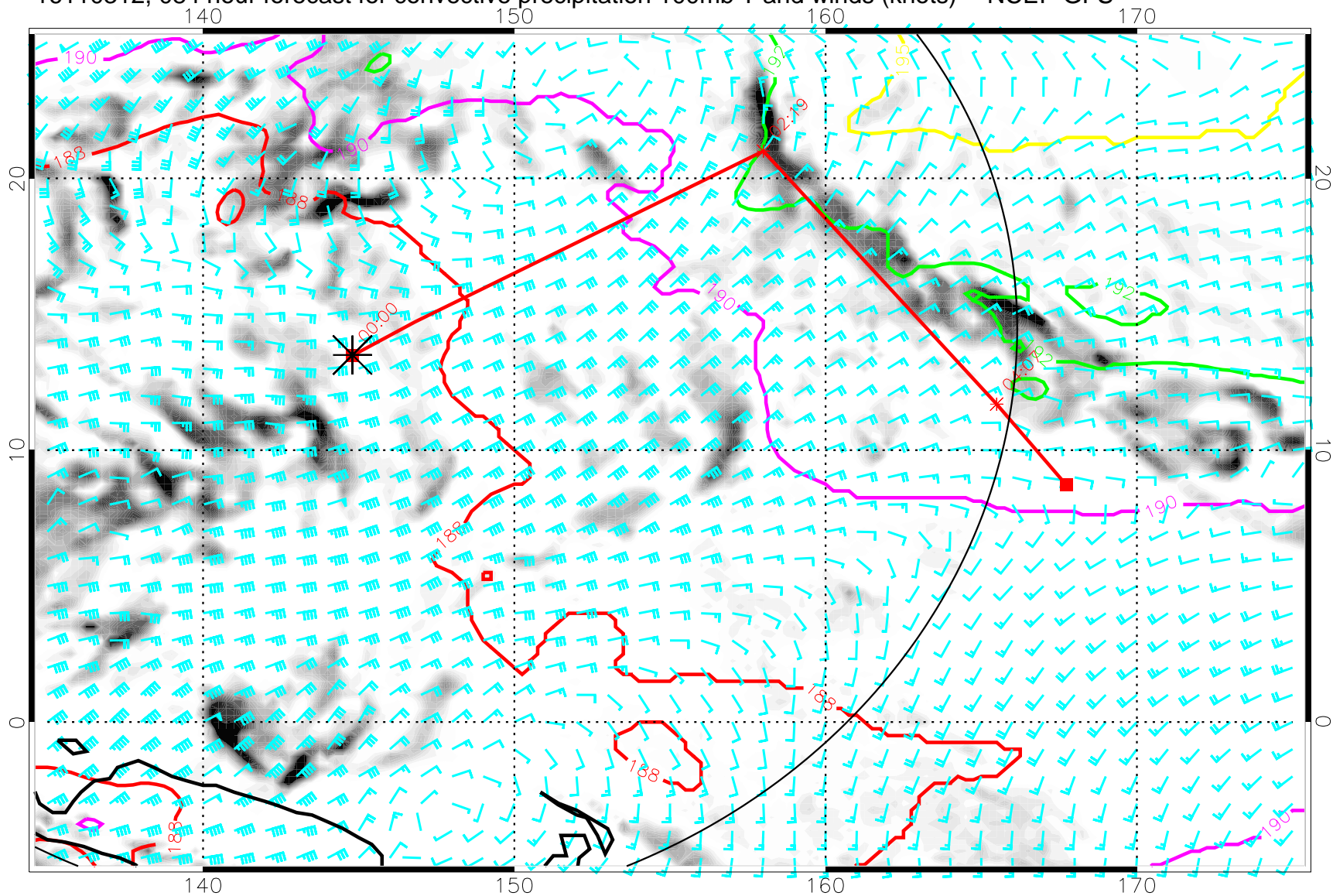
16110312, 084 hour forecast for convective precipitation 100mb T and winds (knots) -- NCEP GFS
