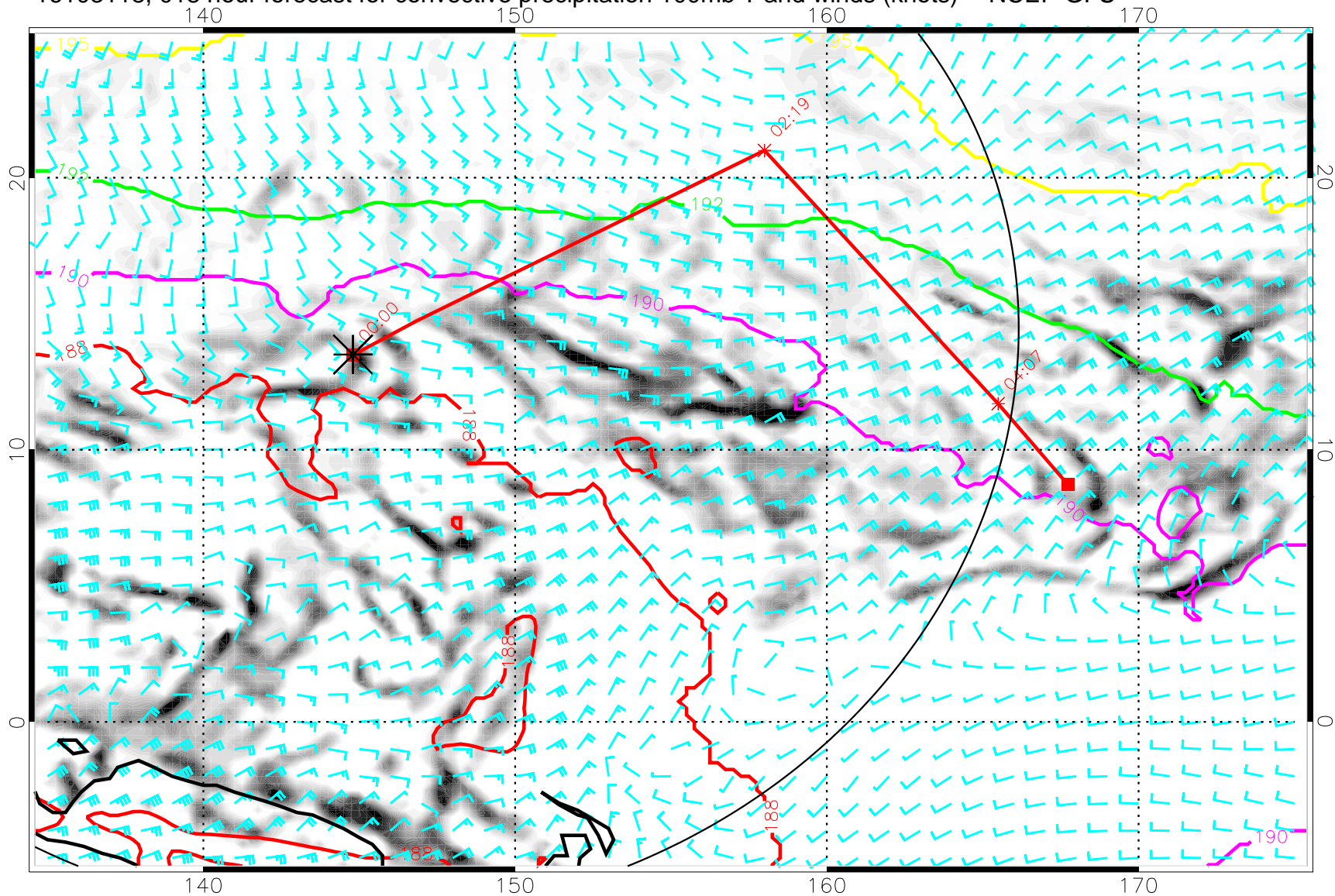
16103118, 018 hour forecast for convective precipitation 100mb T and winds (knots) -- NCEP GFS
