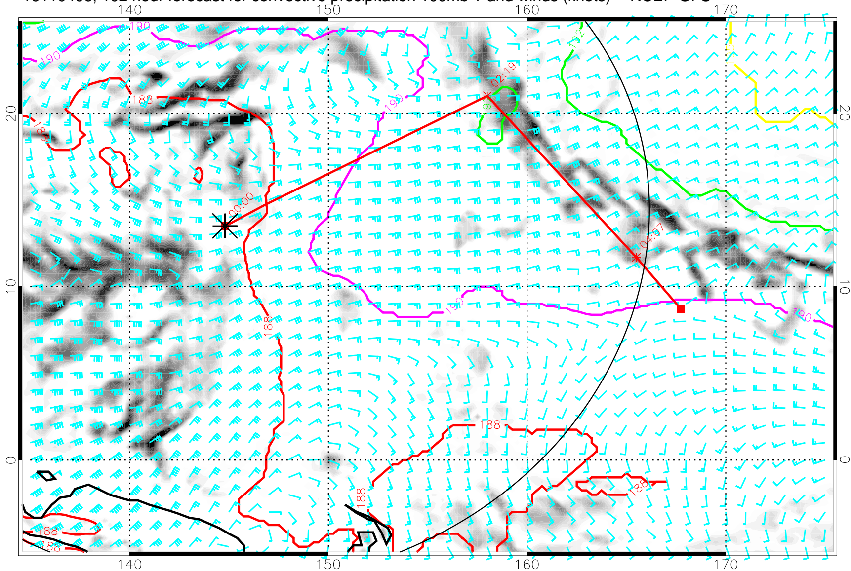
16110406, 102 hour forecast for convective precipitation 100mb T and winds (knots) -- NCEP GFS
