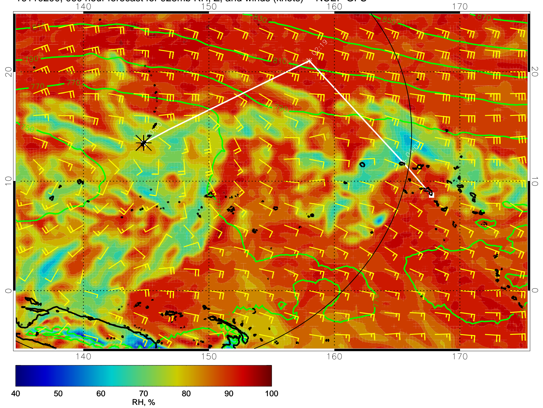
16110200, 060 hour forecast for 925mb RH, Z, and winds (knots) -- NCEP GFS
