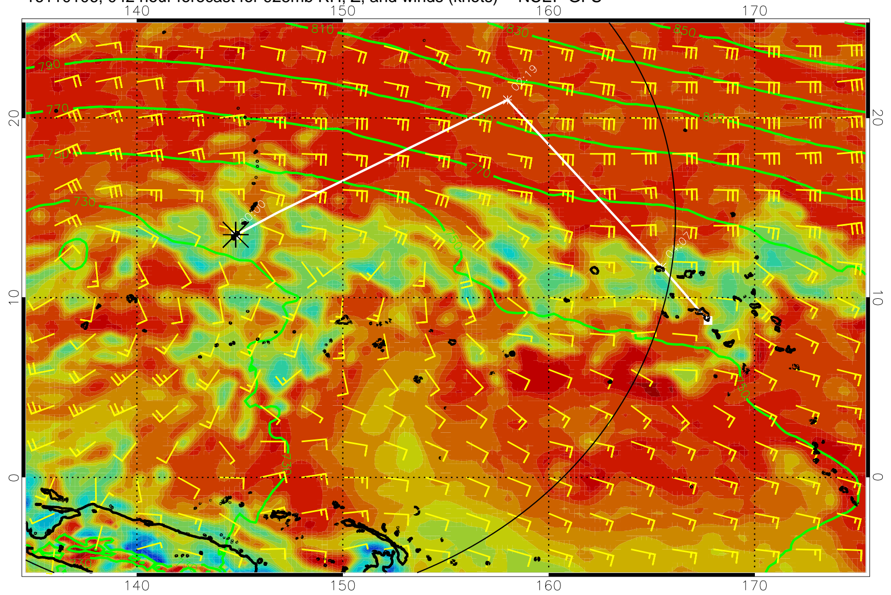
16110106, 042 hour forecast for 925mb RH, Z, and winds (knots) -- NCEP GFS
