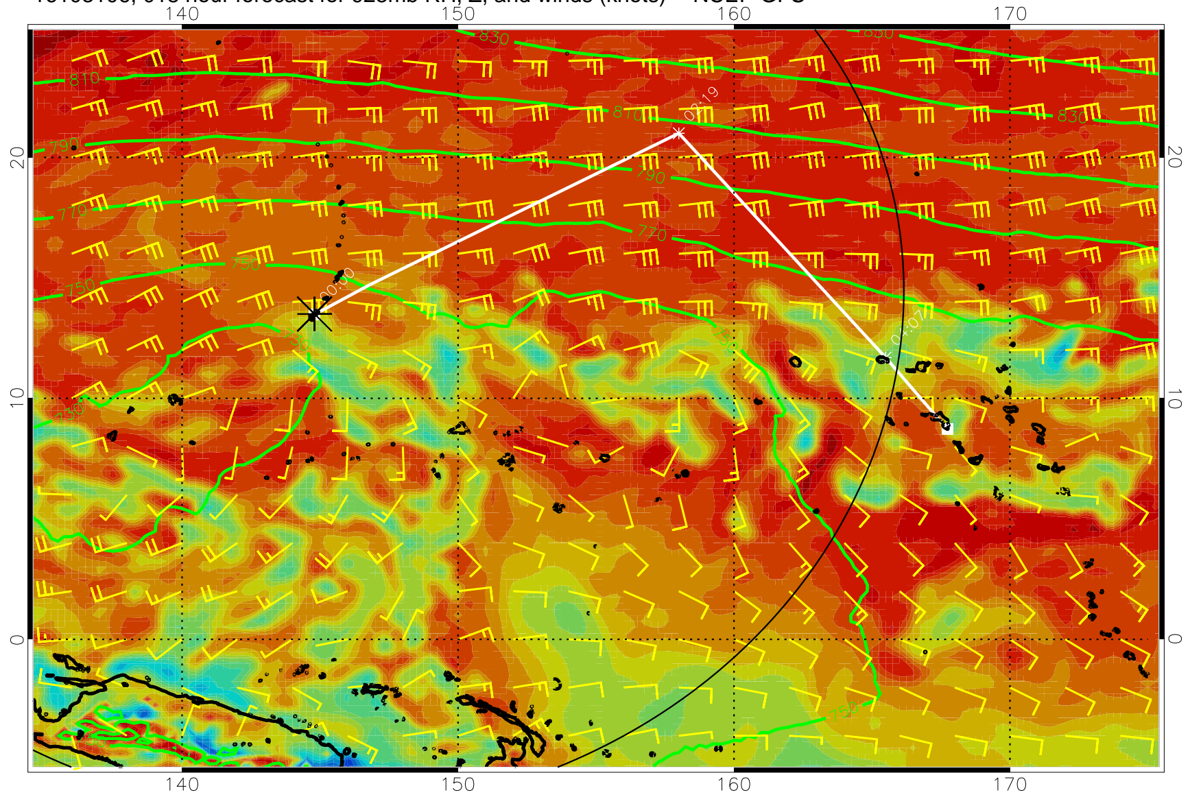
16103106, 018 hour forecast for 925mb RH, Z, and winds (knots) -- NCEP GFS
