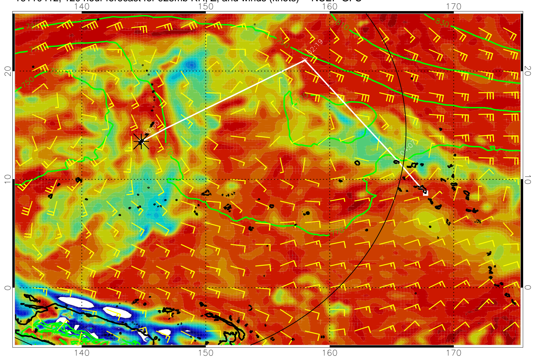
16110412, 120 hour forecast for 925mb RH, Z, and winds (knots) -- NCEP GFS
