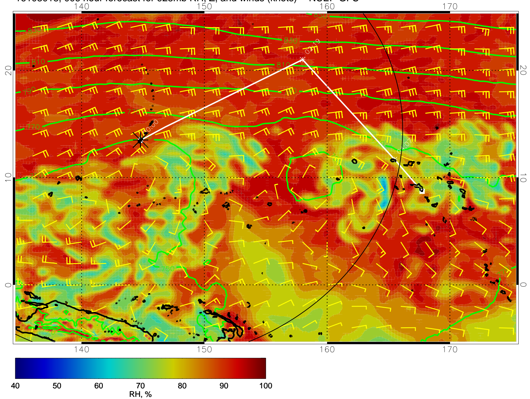
16103018, 006 hour forecast for 925mb RH, Z, and winds (knots) -- NCEP GFS
