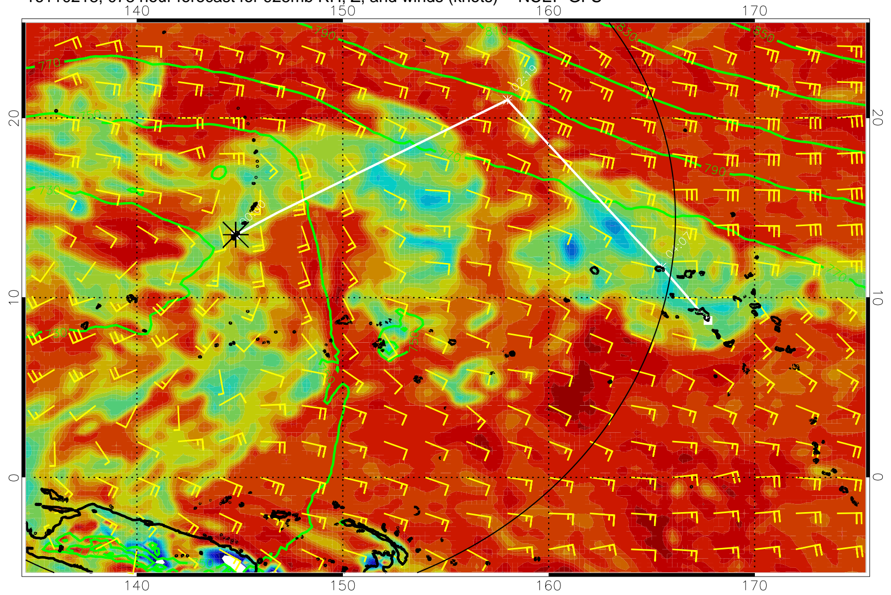
16110218, 078 hour forecast for 925mb RH, Z, and winds (knots) -- NCEP GFS
