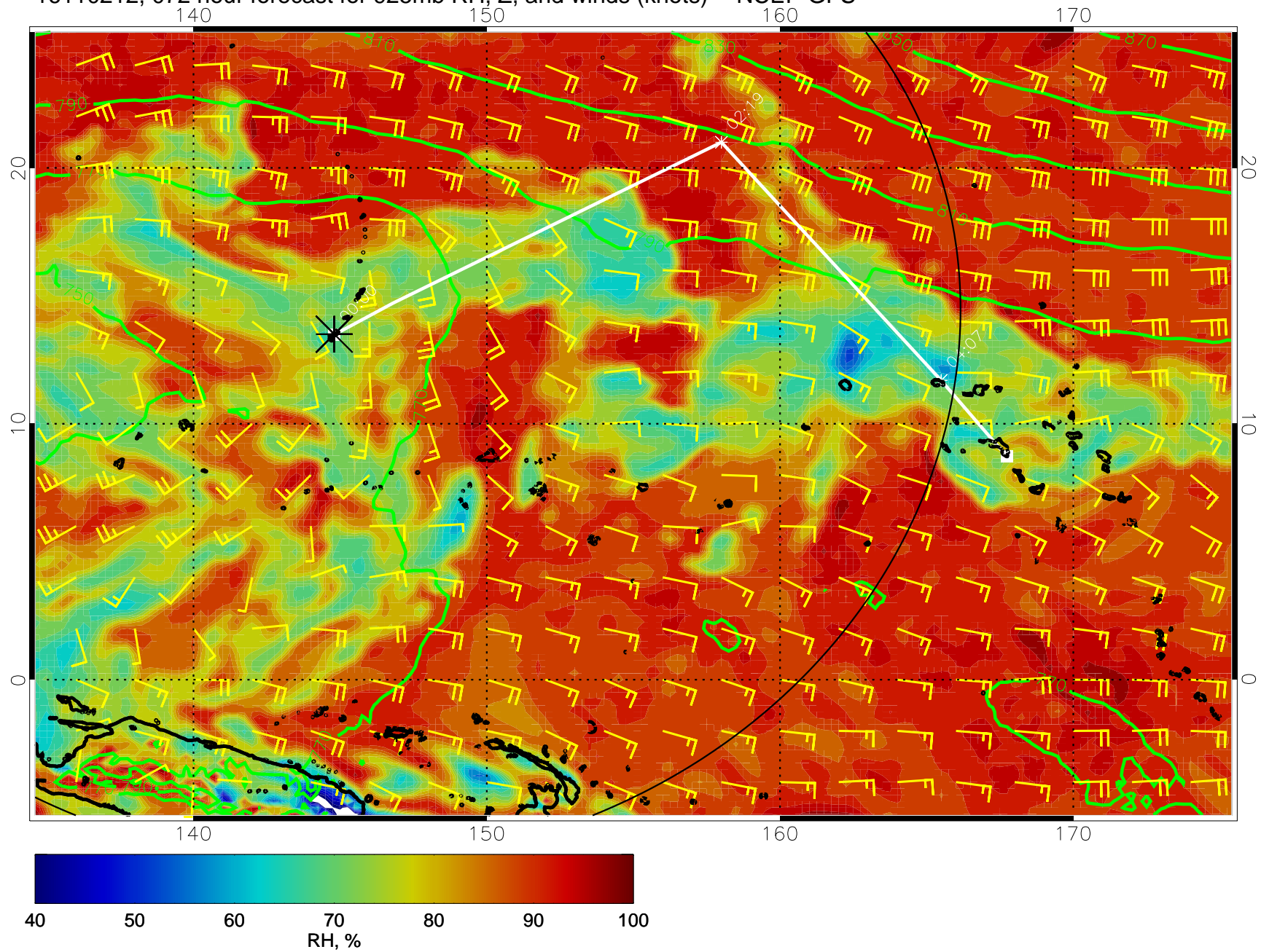
16110212, 072 hour forecast for 925mb RH, Z, and winds (knots) -- NCEP GFS
