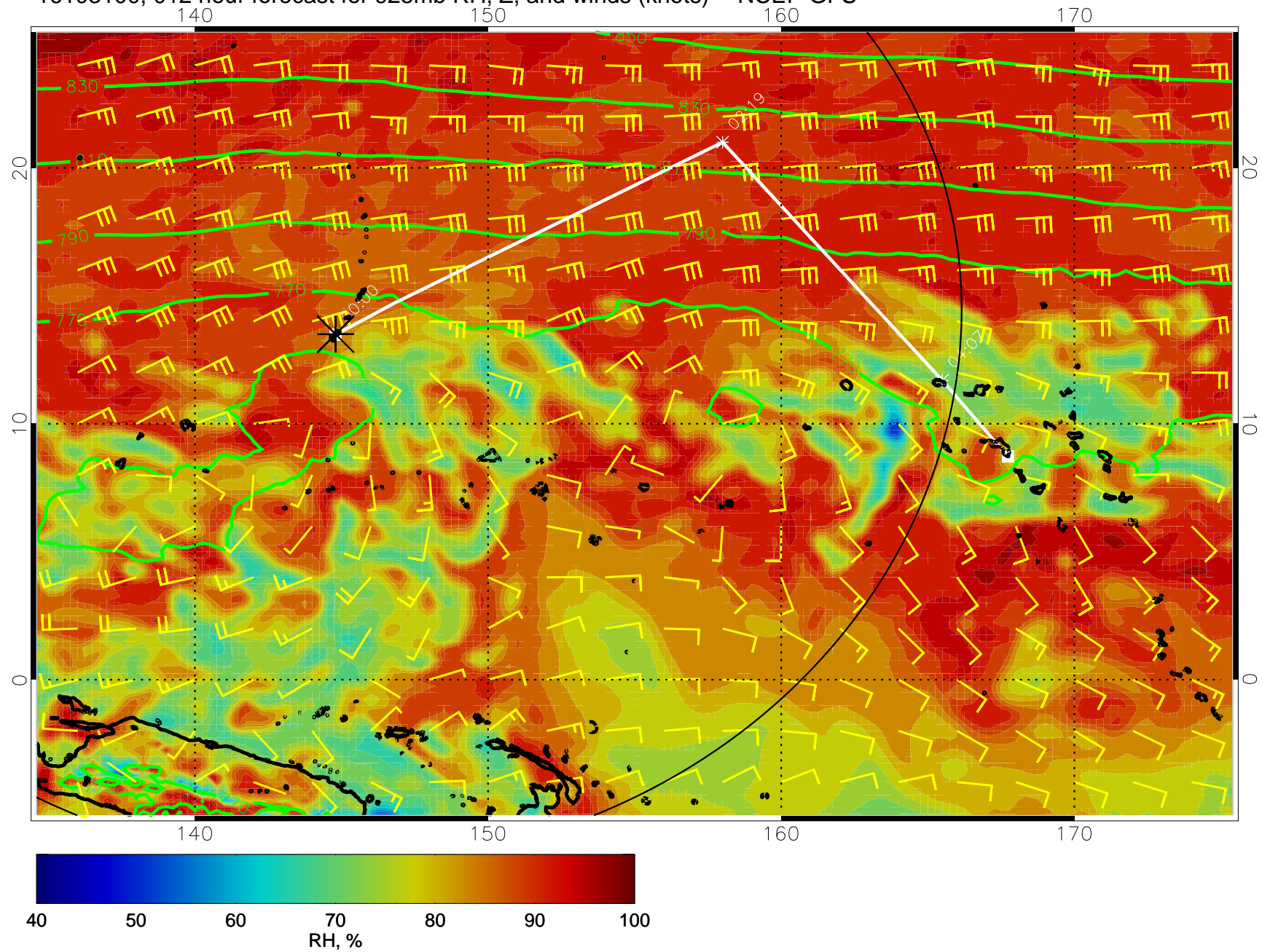
16103100, 012 hour forecast for 925mb RH, Z, and winds (knots) -- NCEP GFS
