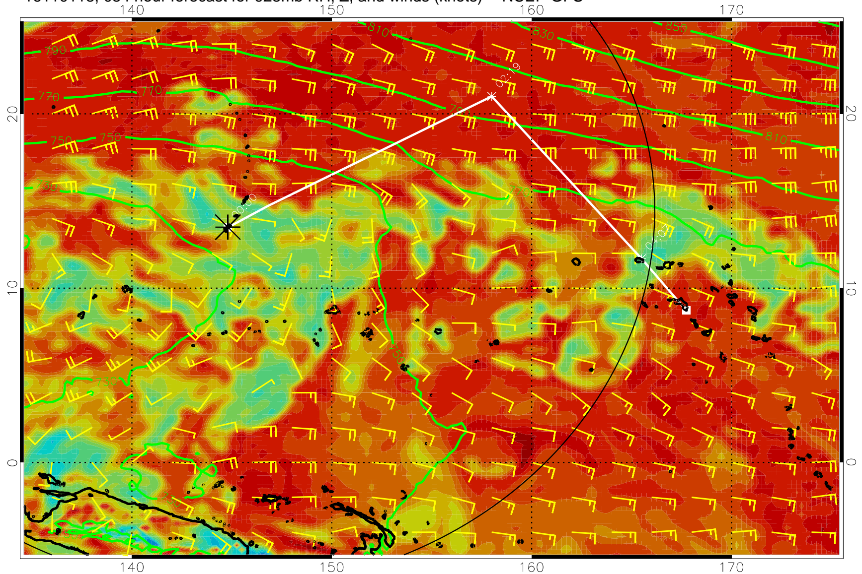
16110118, 054 hour forecast for 925mb RH, Z, and winds (knots) -- NCEP GFS
