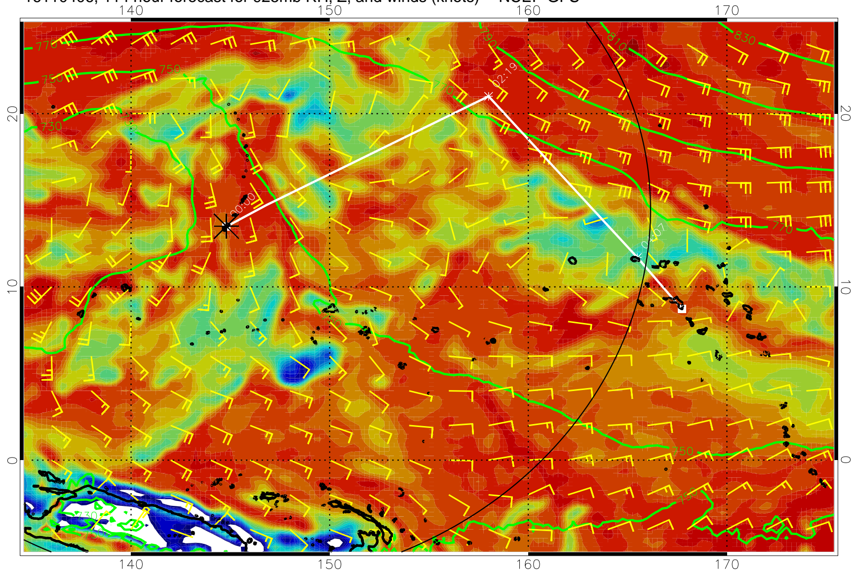
16110406, 114 hour forecast for 925mb RH, Z, and winds (knots) -- NCEP GFS
