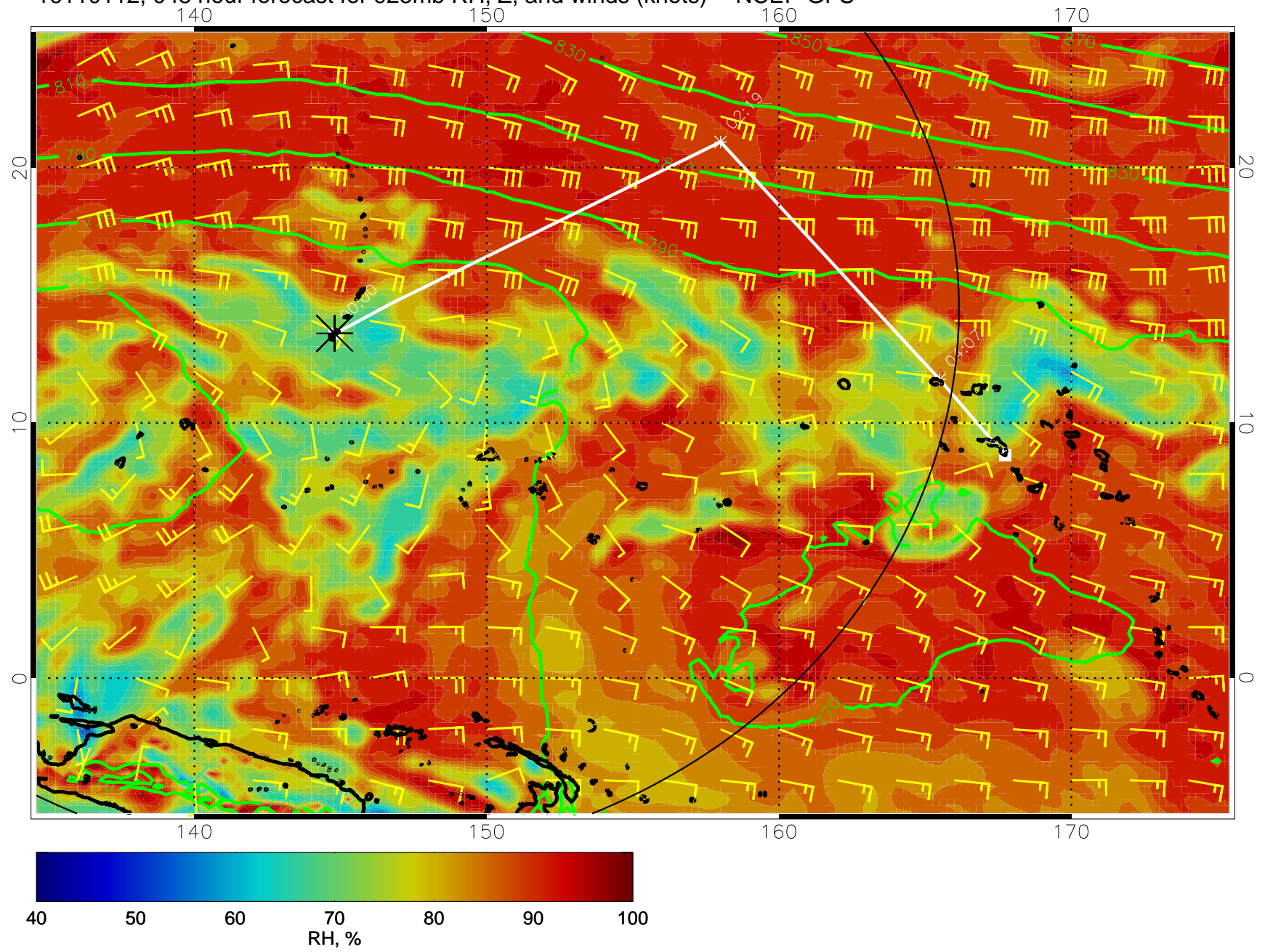
16110112, 048 hour forecast for 925mb RH, Z, and winds (knots) -- NCEP GFS
