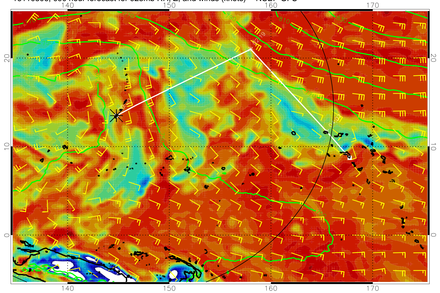
16110306, 090 hour forecast for 925mb RH, Z, and winds (knots) -- NCEP GFS
