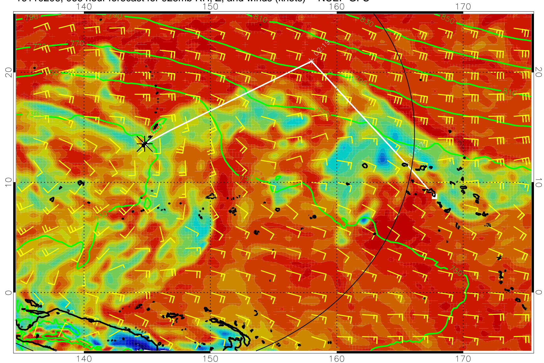
16110206, 066 hour forecast for 925mb RH, Z, and winds (knots) -- NCEP GFS
