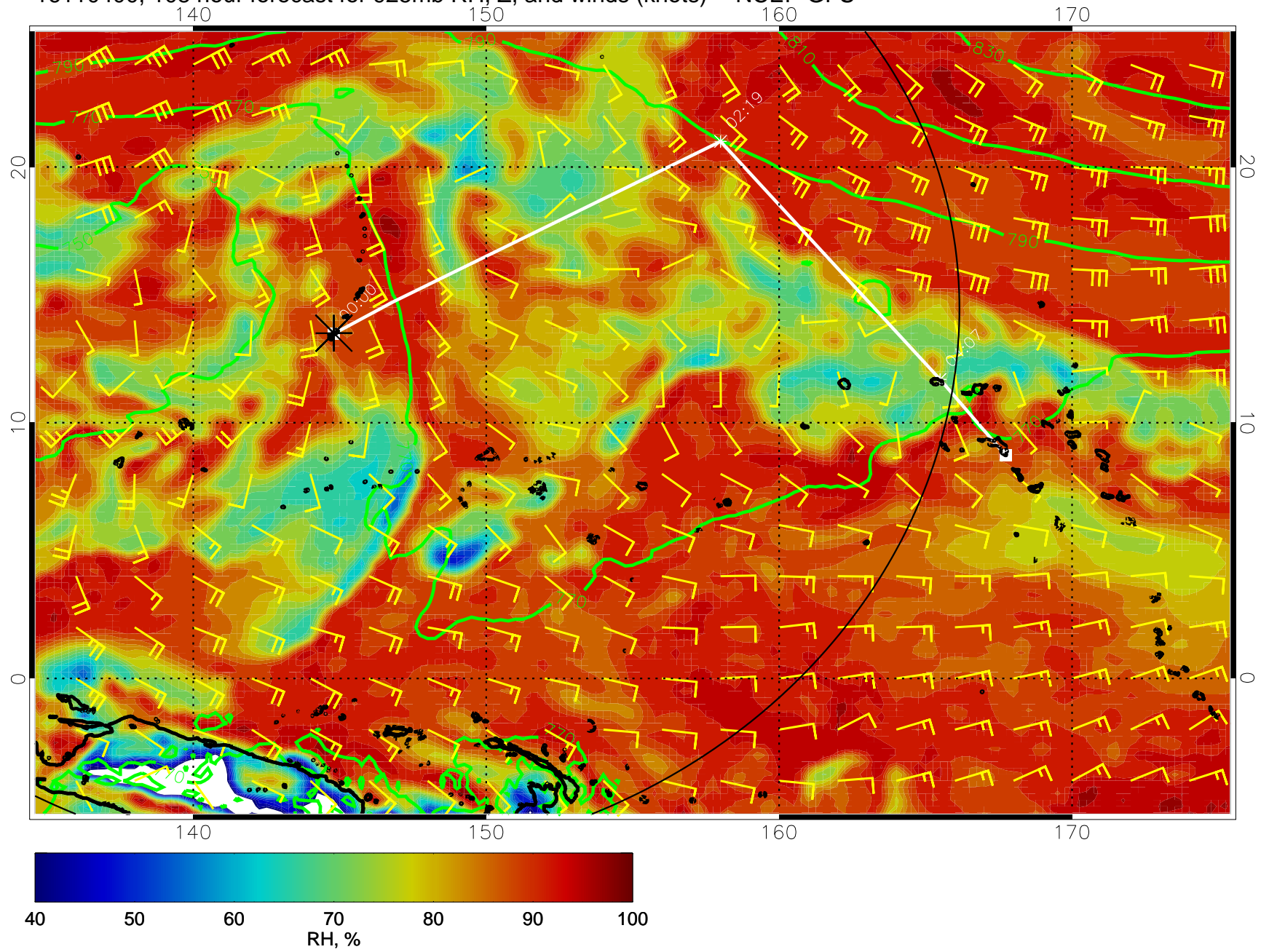
16110400, 108 hour forecast for 925mb RH, Z, and winds (knots) -- NCEP GFS
