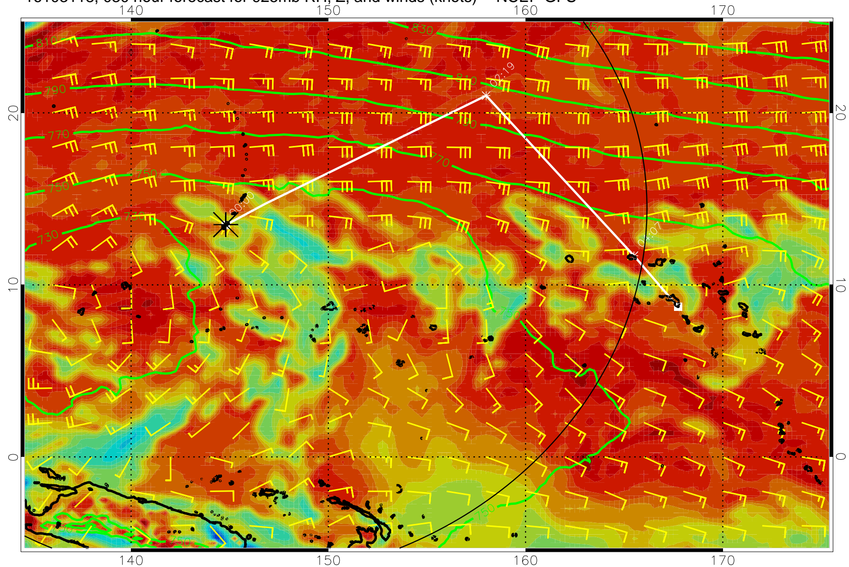
16103118, 030 hour forecast for 925mb RH, Z, and winds (knots) -- NCEP GFS
