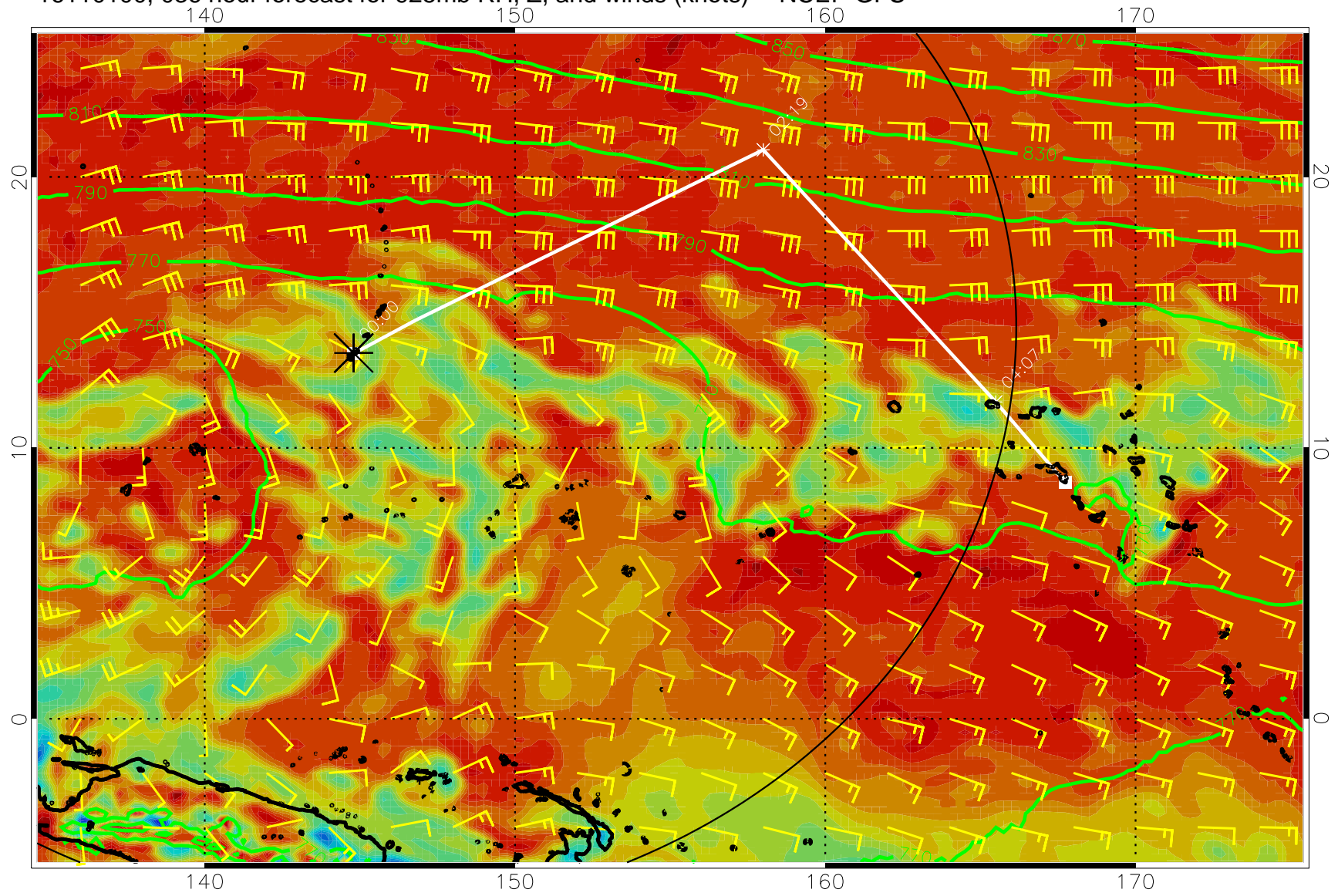
16110100, 036 hour forecast for 925mb RH, Z, and winds (knots) -- NCEP GFS
