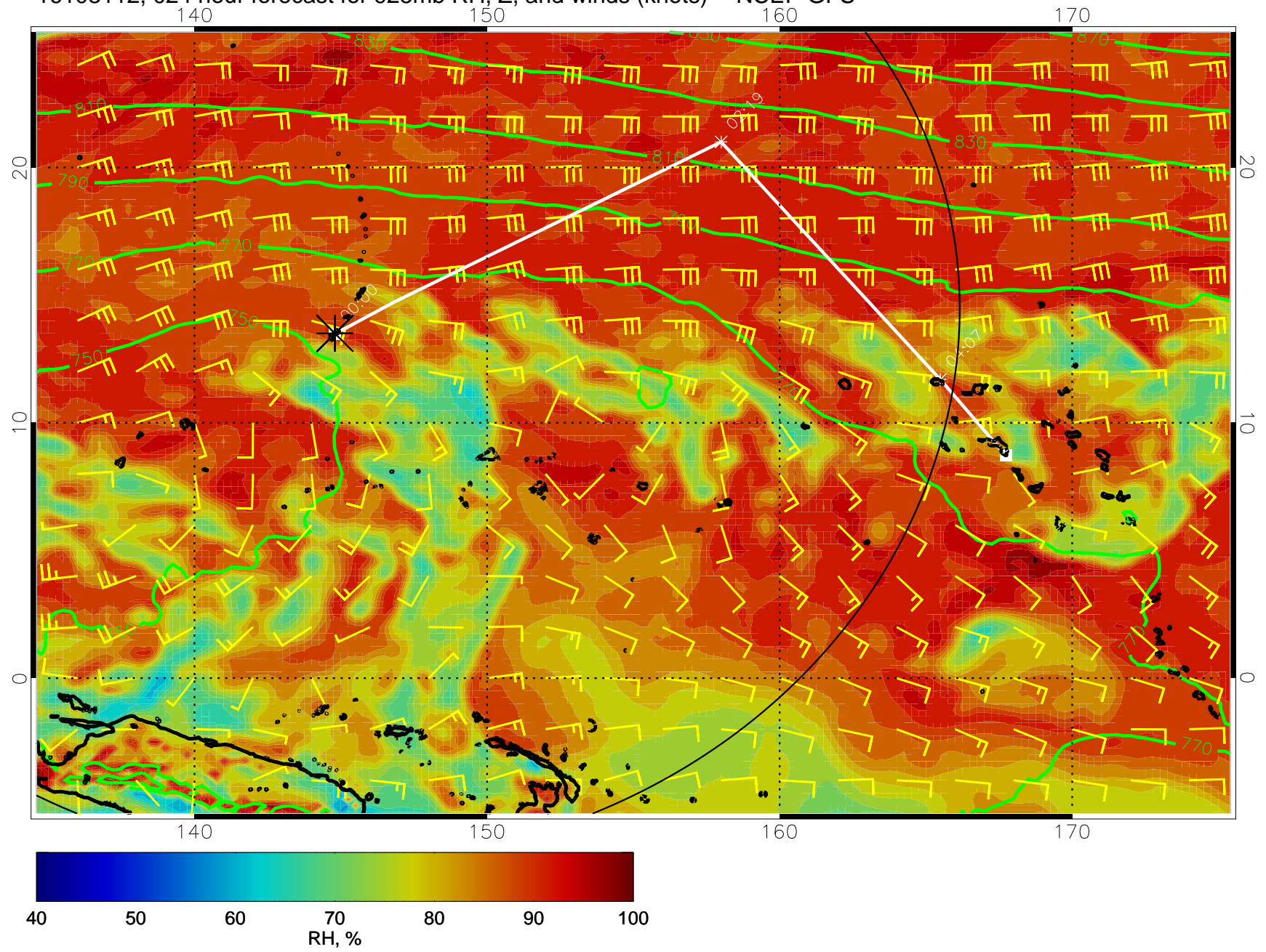
16103112, 024 hour forecast for 925mb RH, Z, and winds (knots) -- NCEP GFS
