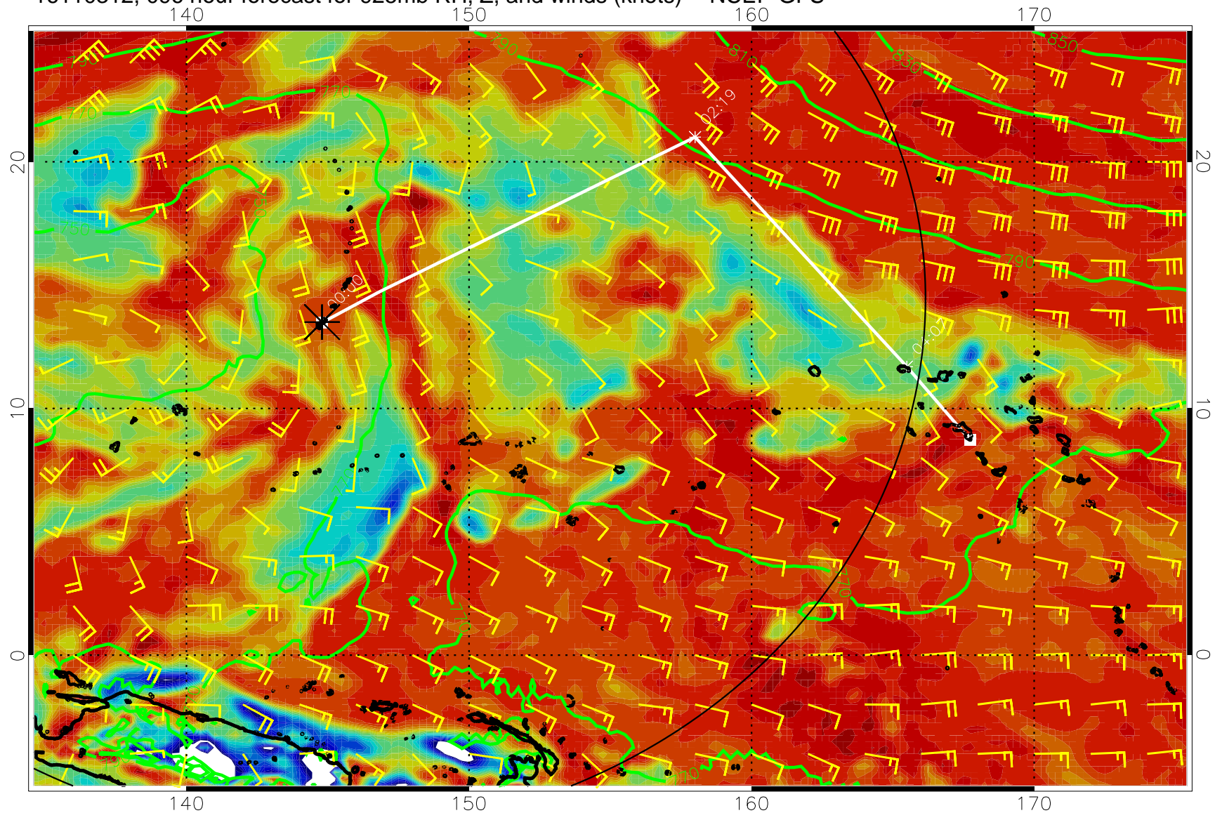
16110312, 096 hour forecast for 925mb RH, Z, and winds (knots) -- NCEP GFS
