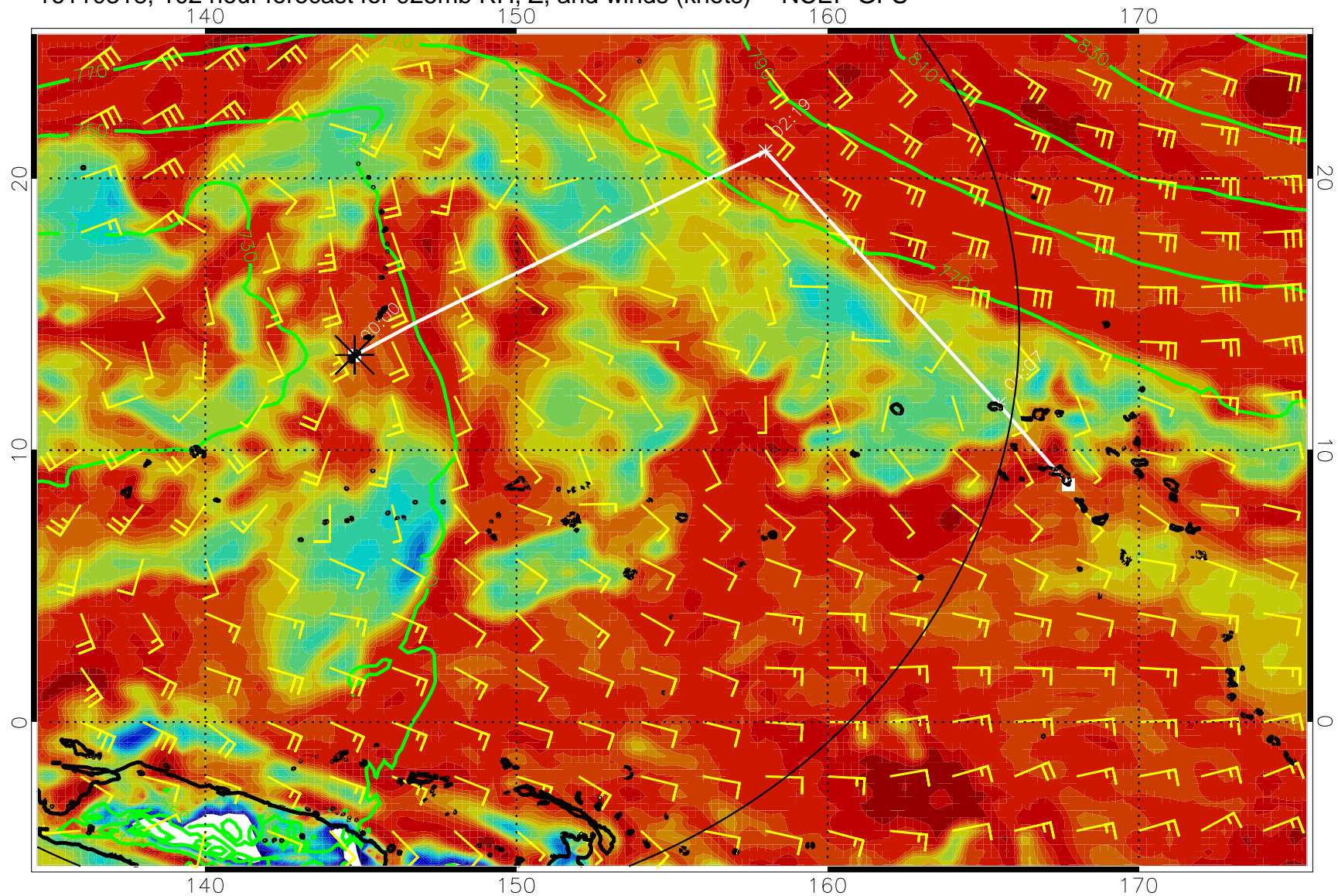
16110318, 102 hour forecast for 925mb RH, Z, and winds (knots) -- NCEP GFS
