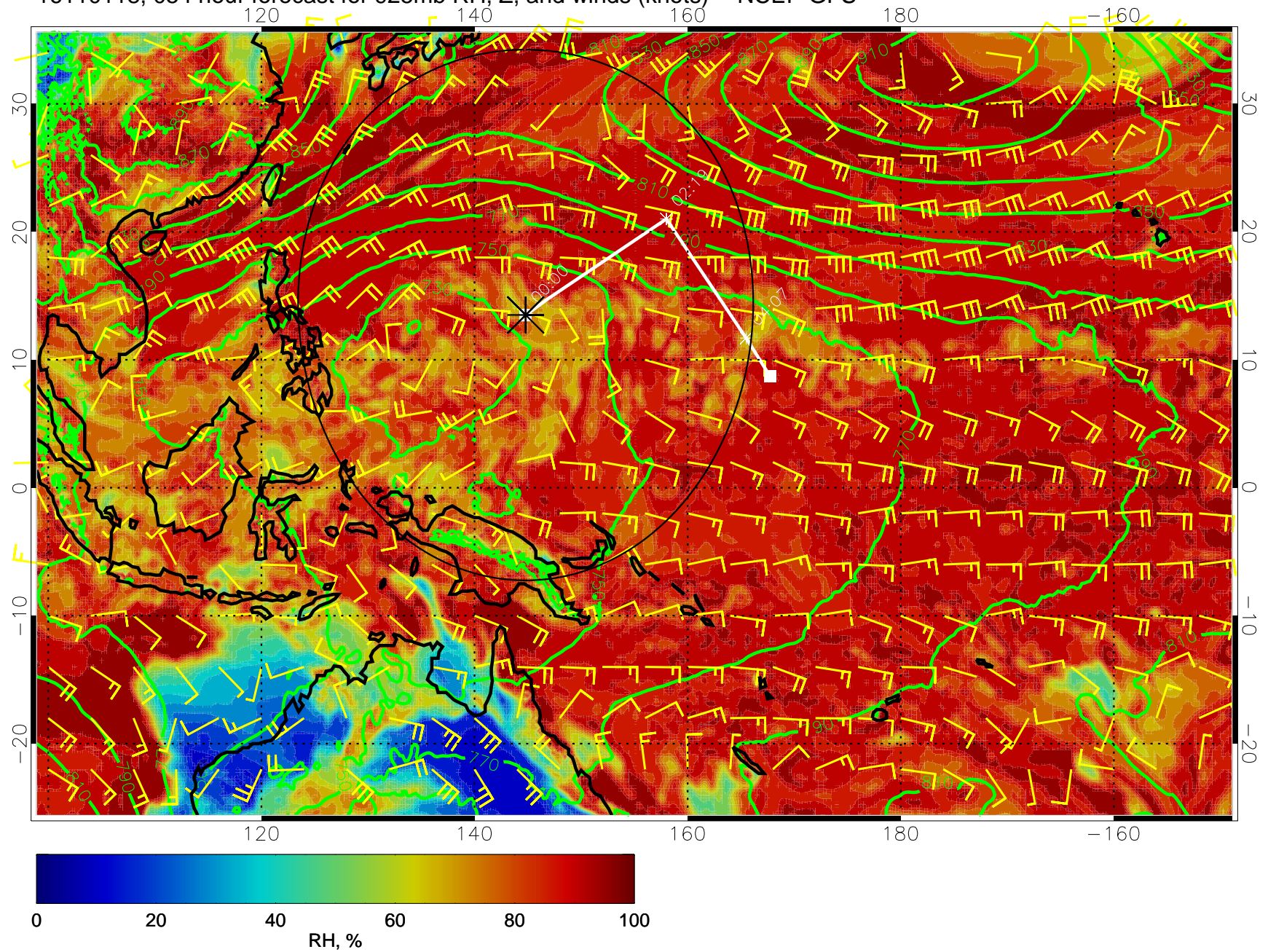
16110118, 054 hour forecast for 925mb RH, Z, and winds (knots) -- NCEP GFS
