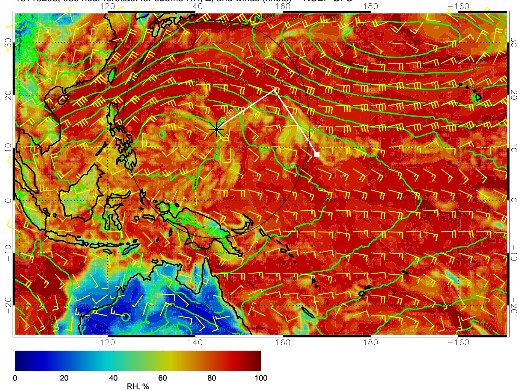
16110206, 066 hour forecast for 925mb RH, Z, and winds (knots) -- NCEP GFS
