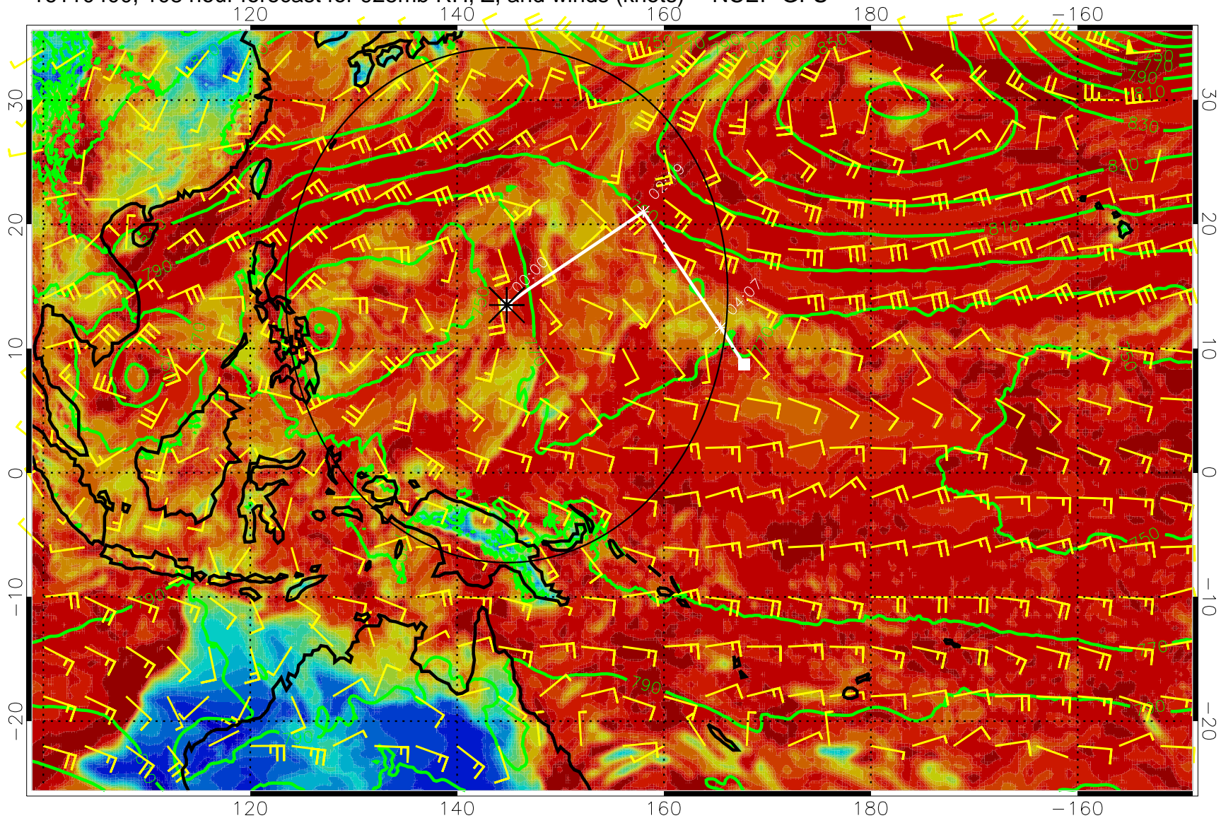
16110400, 108 hour forecast for 925mb RH, Z, and winds (knots) -- NCEP GFS
