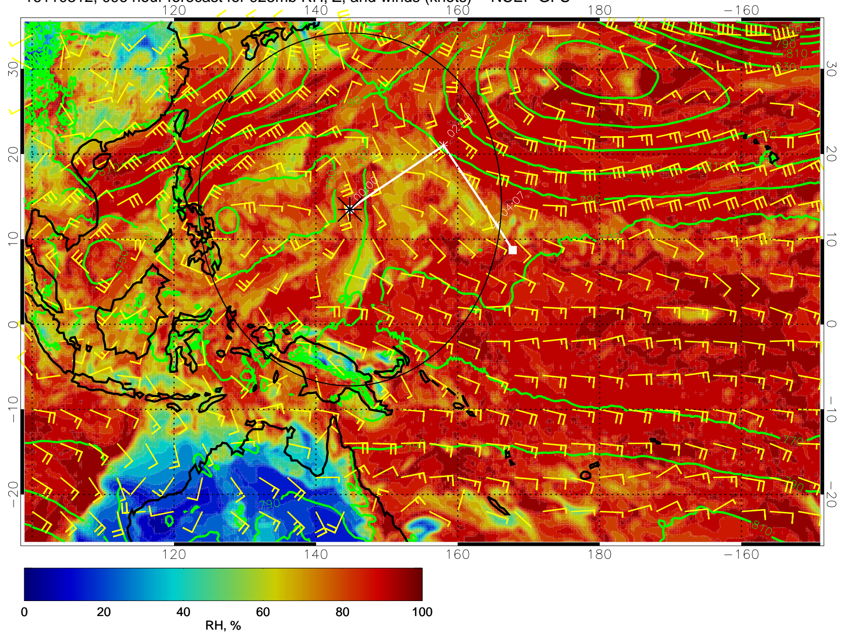
16110312, 096 hour forecast for 925mb RH, Z, and winds (knots) -- NCEP GFS
