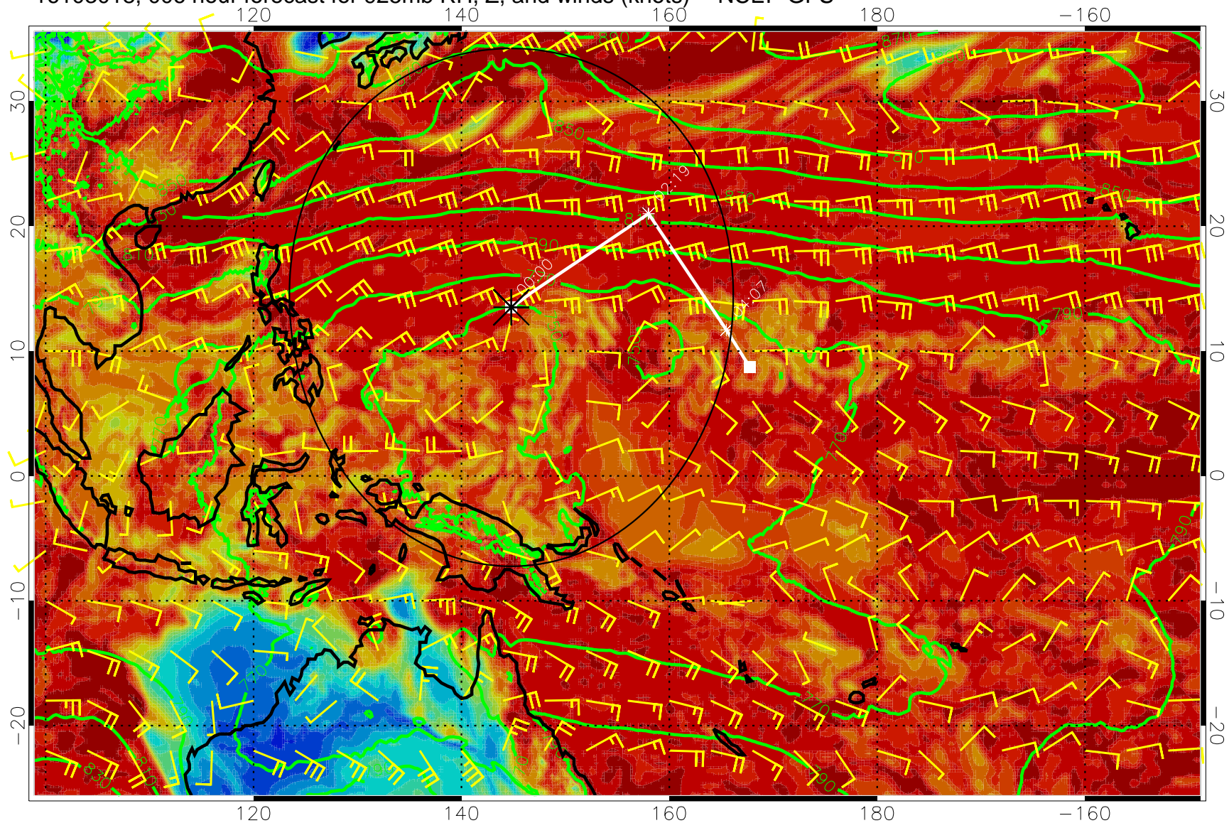
16103018, 006 hour forecast for 925mb RH, Z, and winds (knots) -- NCEP GFS
