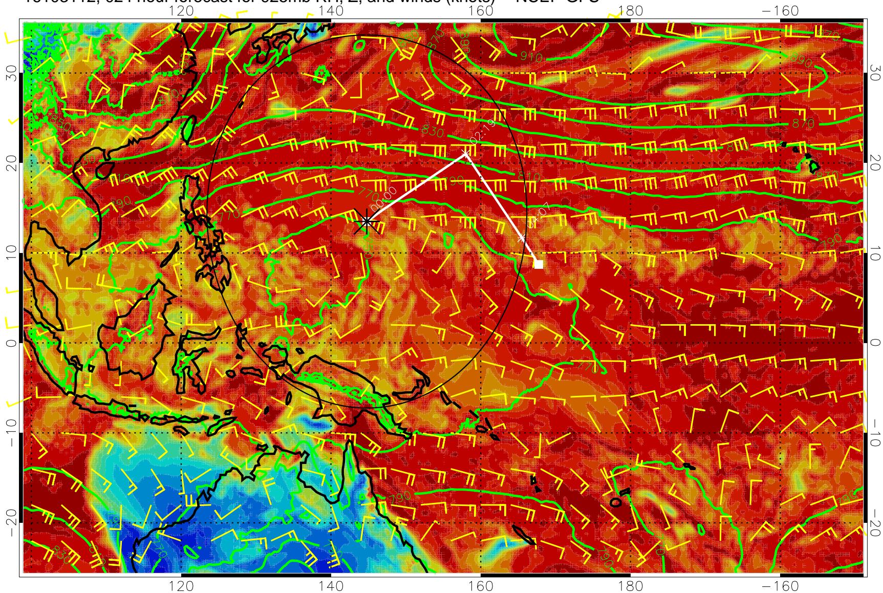
16103112, 024 hour forecast for 925mb RH, Z, and winds (knots) -- NCEP GFS
