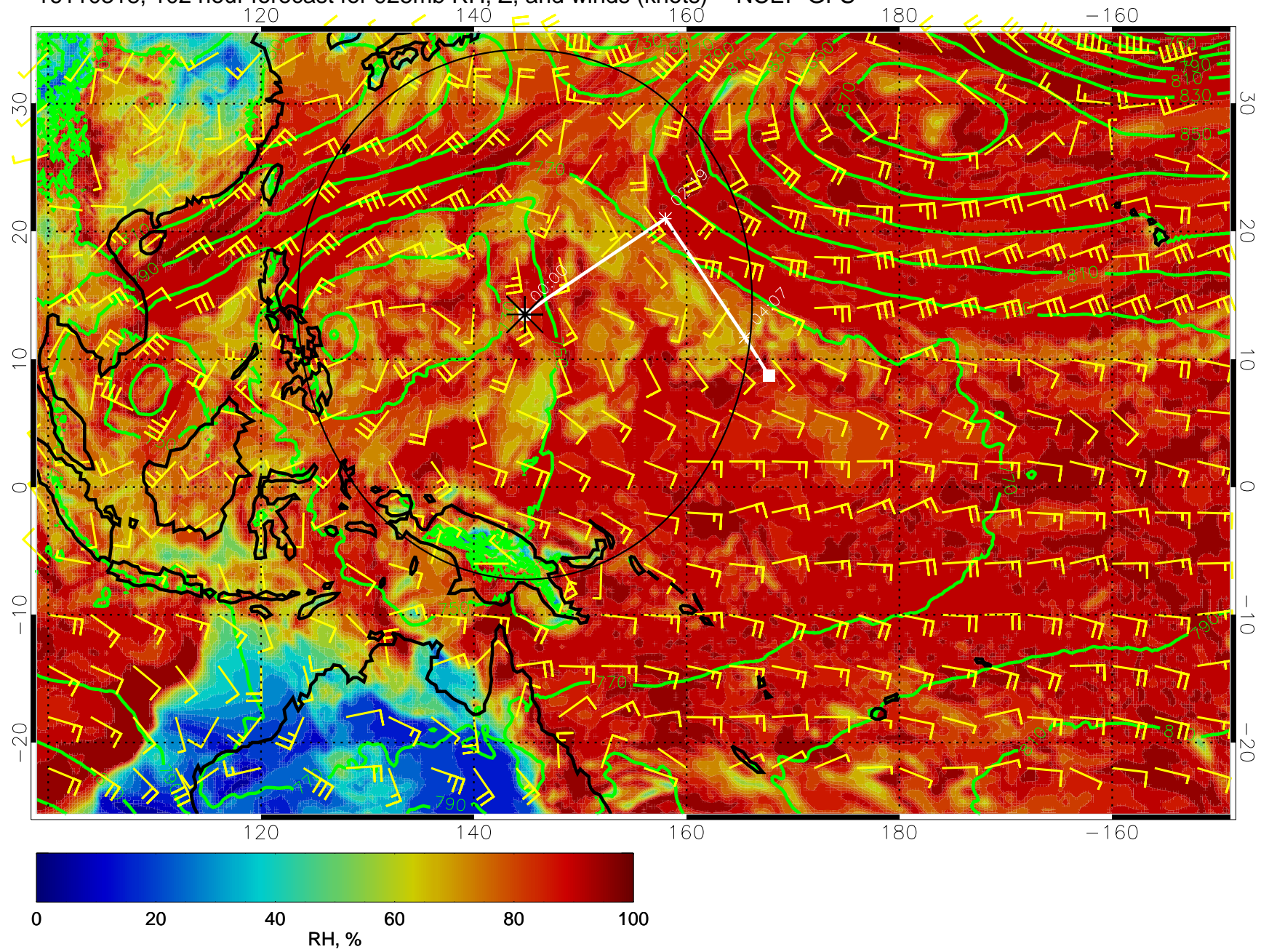
16110318, 102 hour forecast for 925mb RH, Z, and winds (knots) -- NCEP GFS
