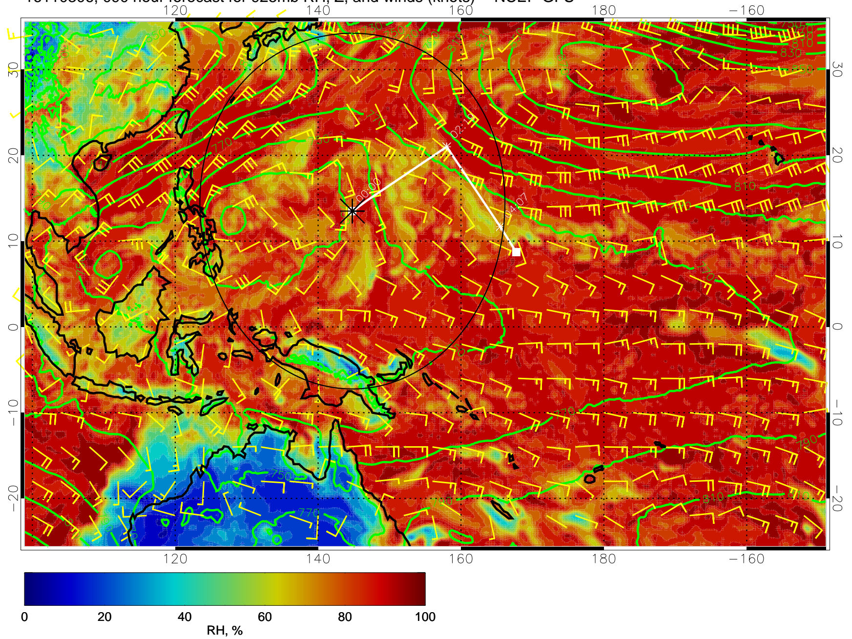
16110306, 090 hour forecast for 925mb RH, Z, and winds (knots) -- NCEP GFS
