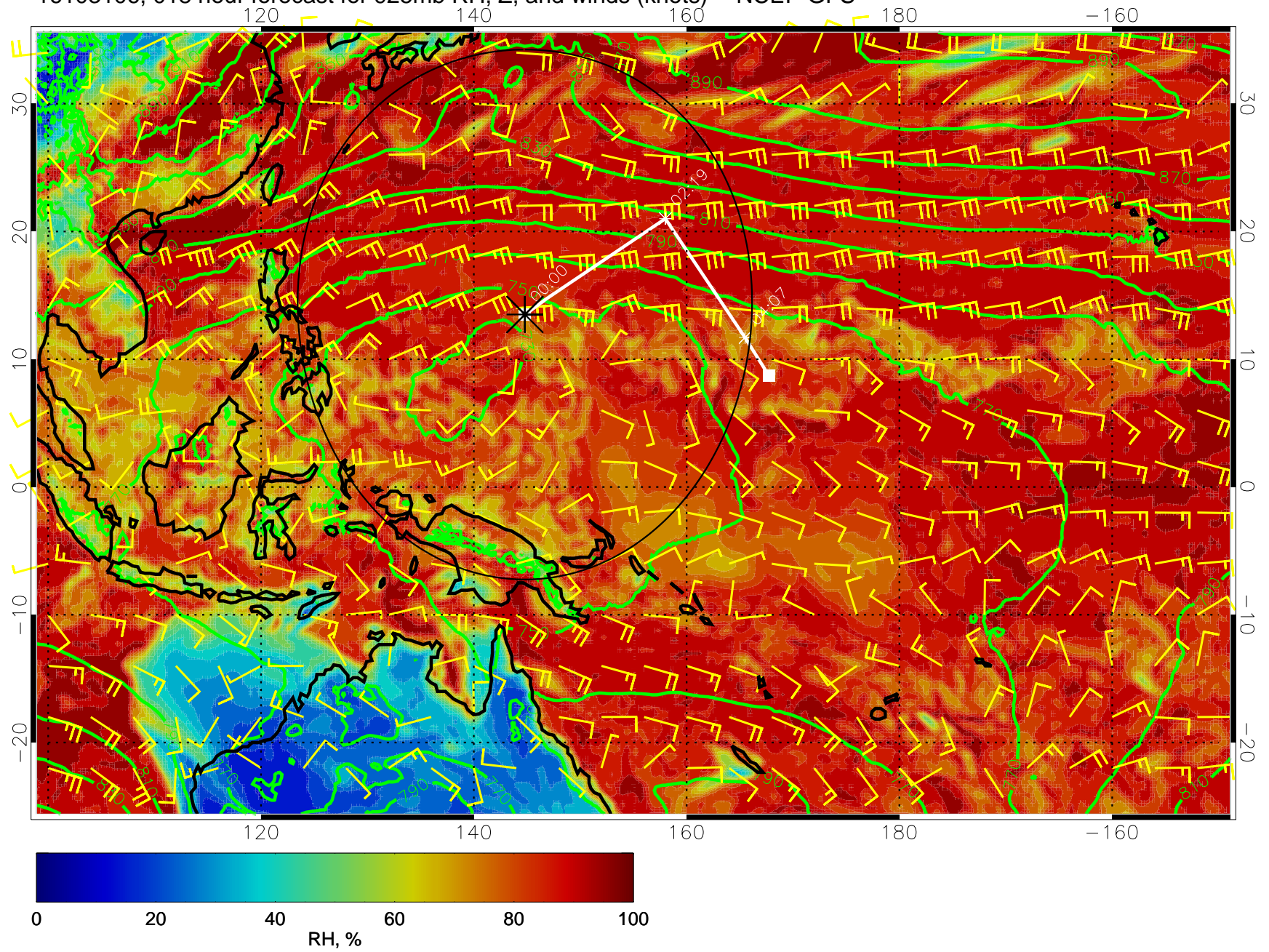
16103106, 018 hour forecast for 925mb RH, Z, and winds (knots) -- NCEP GFS
