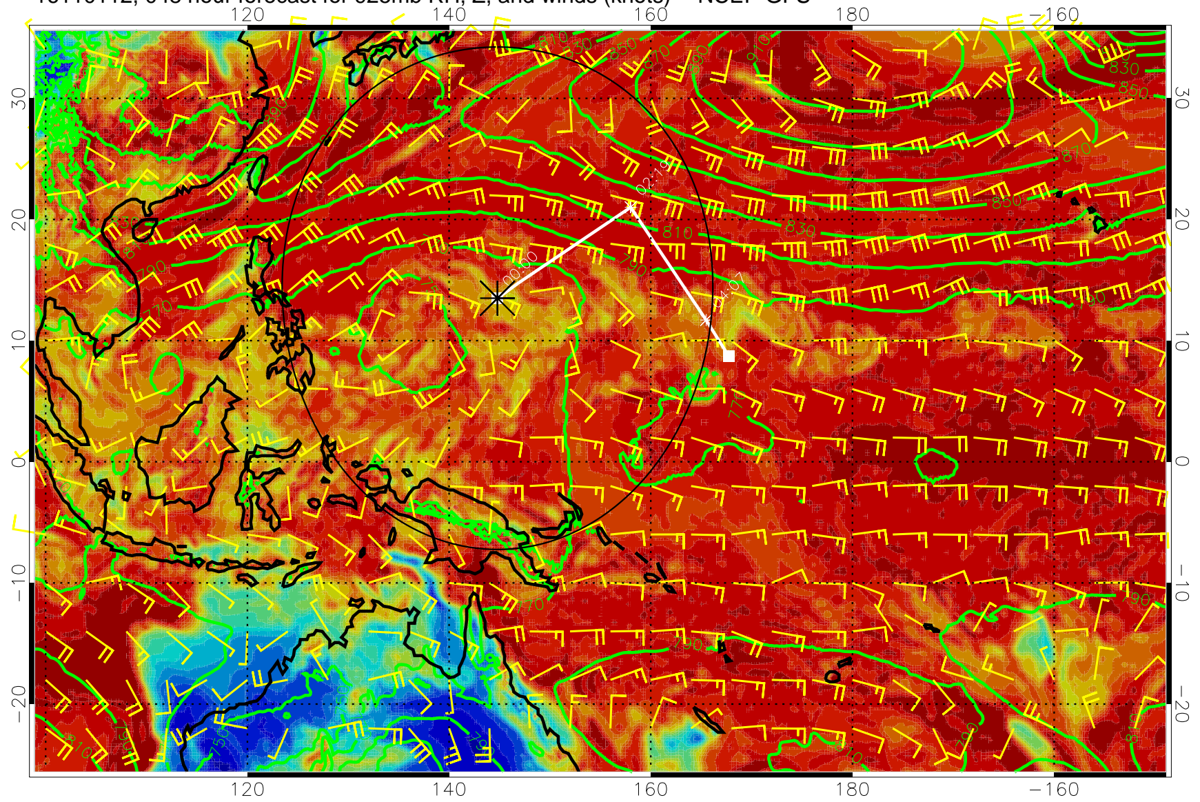
16110112, 048 hour forecast for 925mb RH, Z, and winds (knots) -- NCEP GFS
