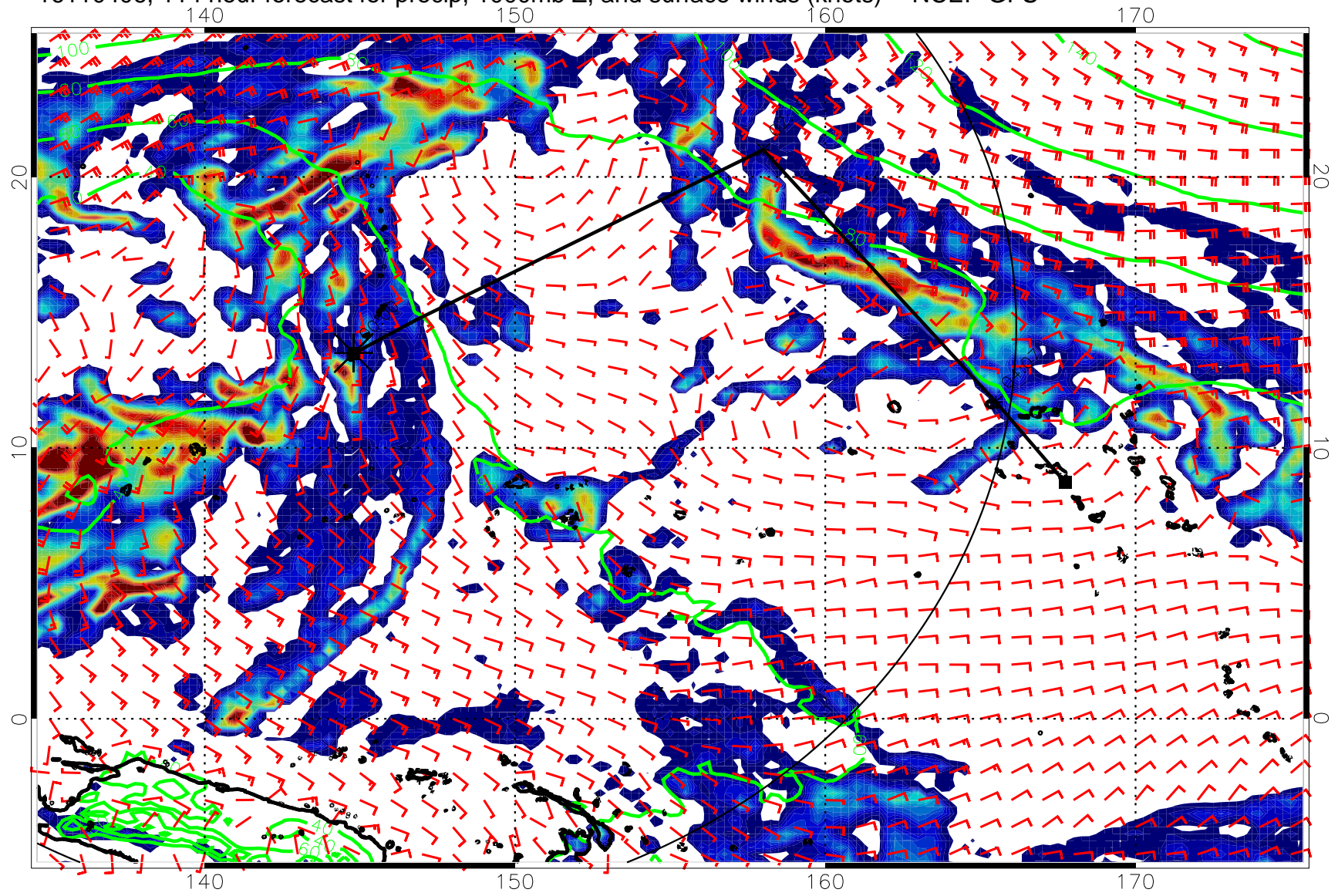
16110406, 114 hour forecast for precip, 1000mb Z, and surface winds (knots) -- NCEP GFS
