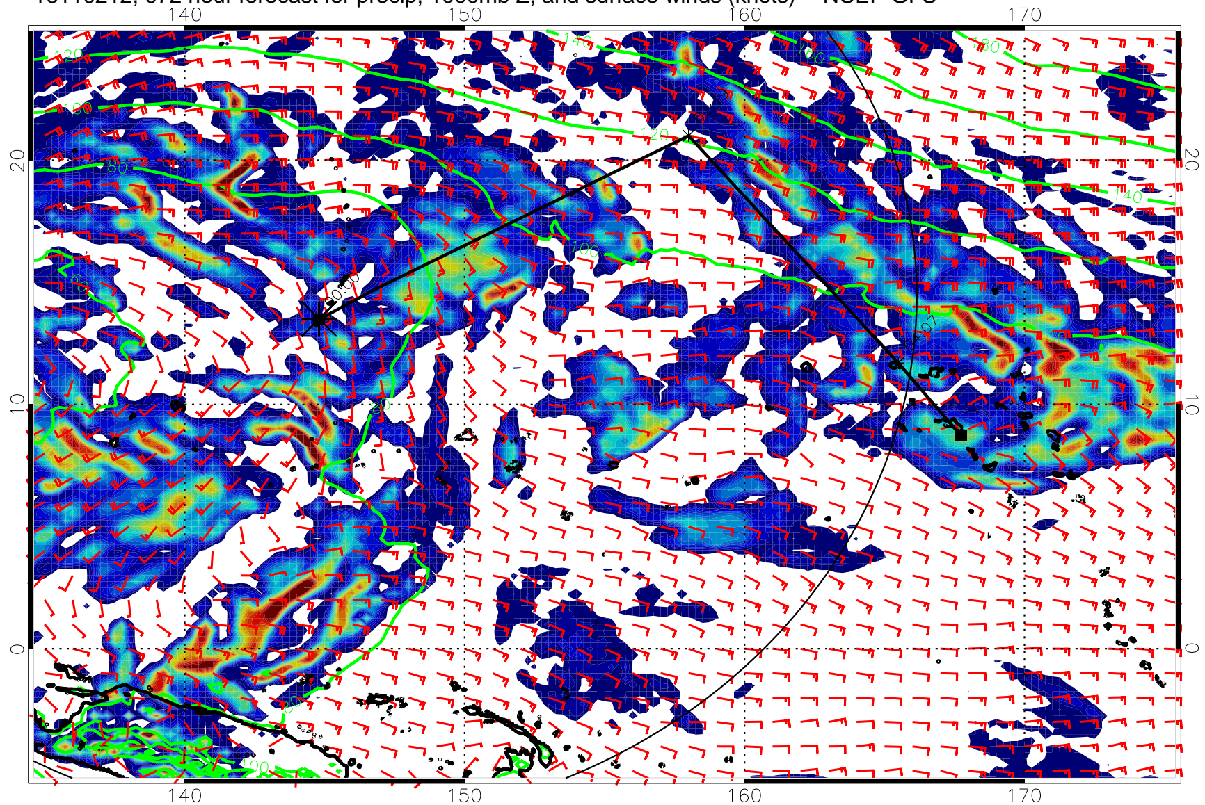
16110212, 072 hour forecast for precip, 1000mb Z, and surface winds (knots) -- NCEP GFS
