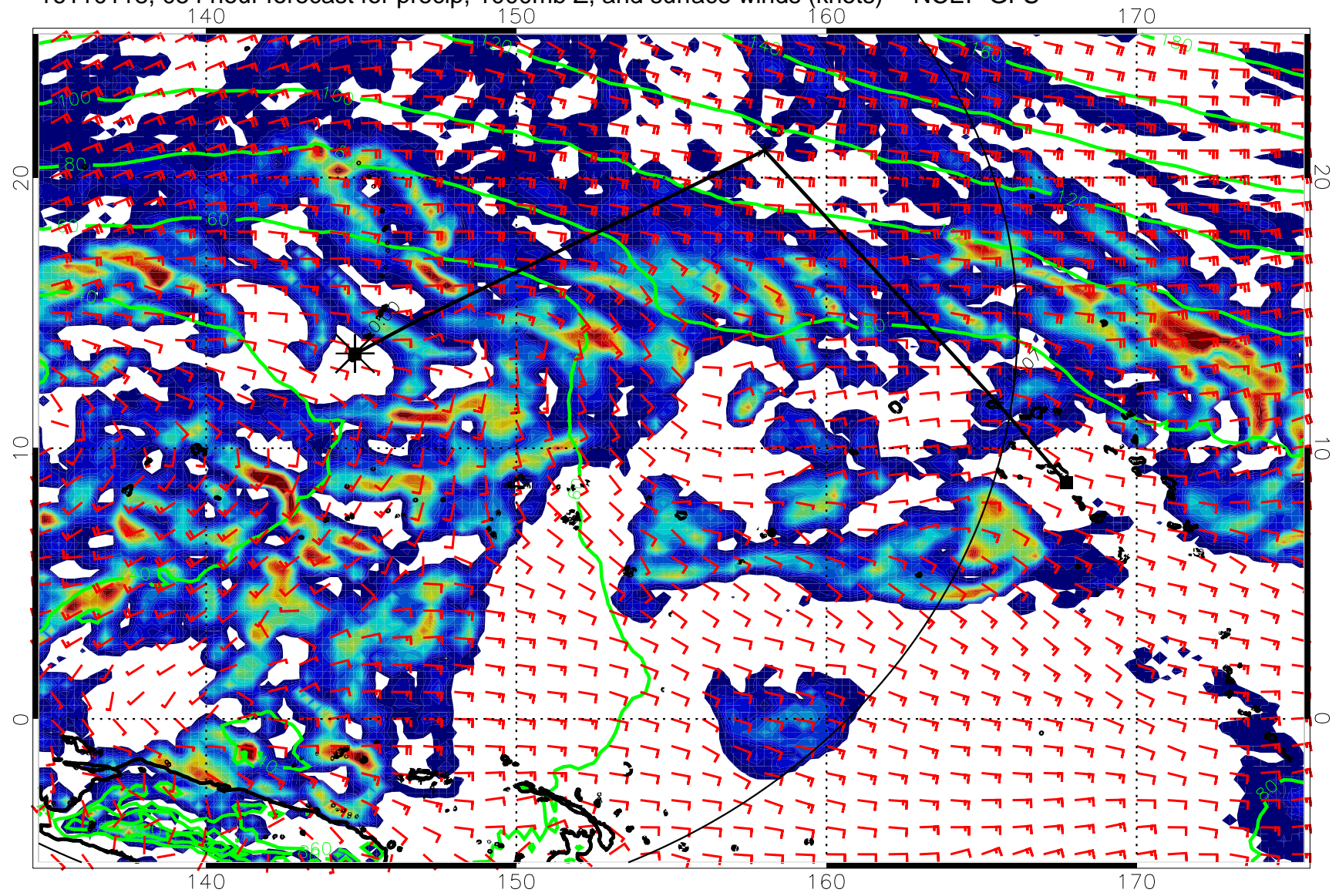
16110118, 054 hour forecast for precip, 1000mb Z, and surface winds (knots) -- NCEP GFS
