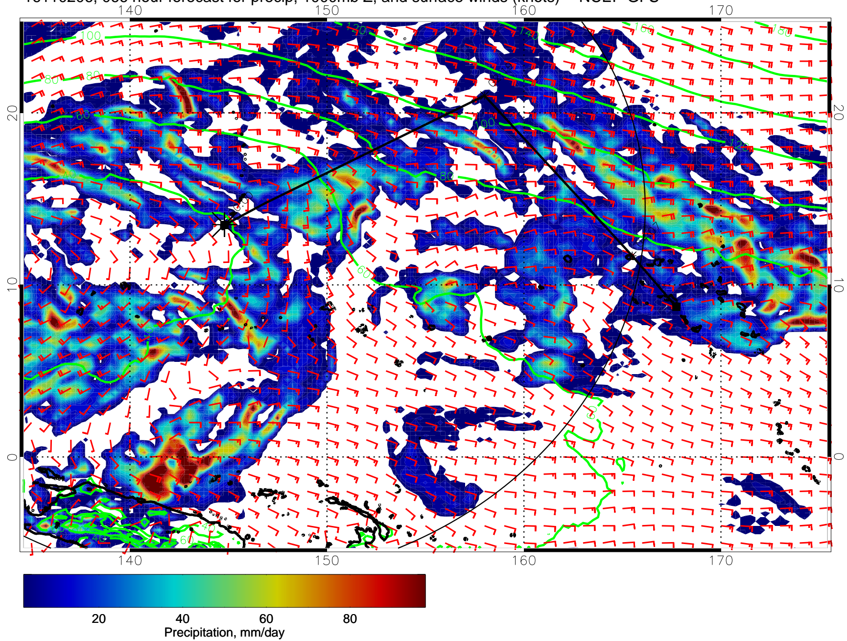
16110206, 066 hour forecast for precip, 1000mb Z, and surface winds (knots) -- NCEP GFS
