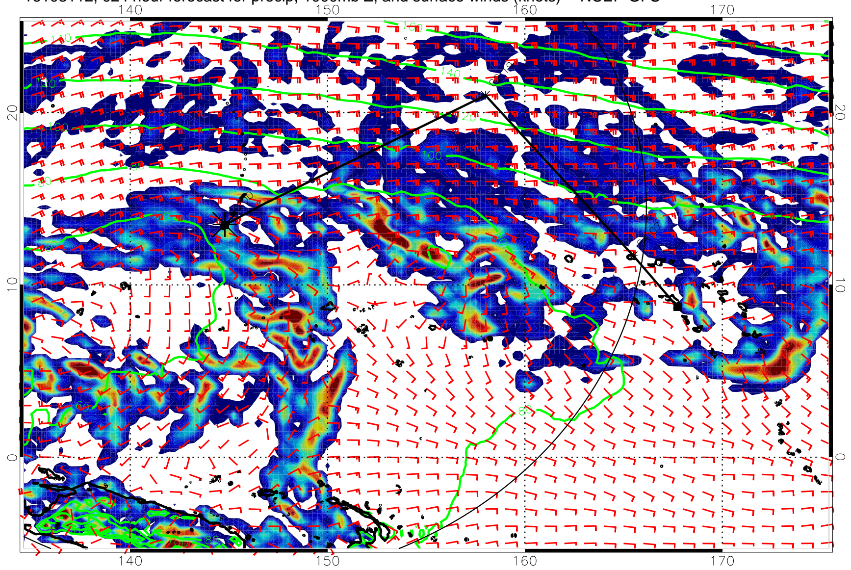
16103112, 024 hour forecast for precip, 1000mb Z, and surface winds (knots) -- NCEP GFS
