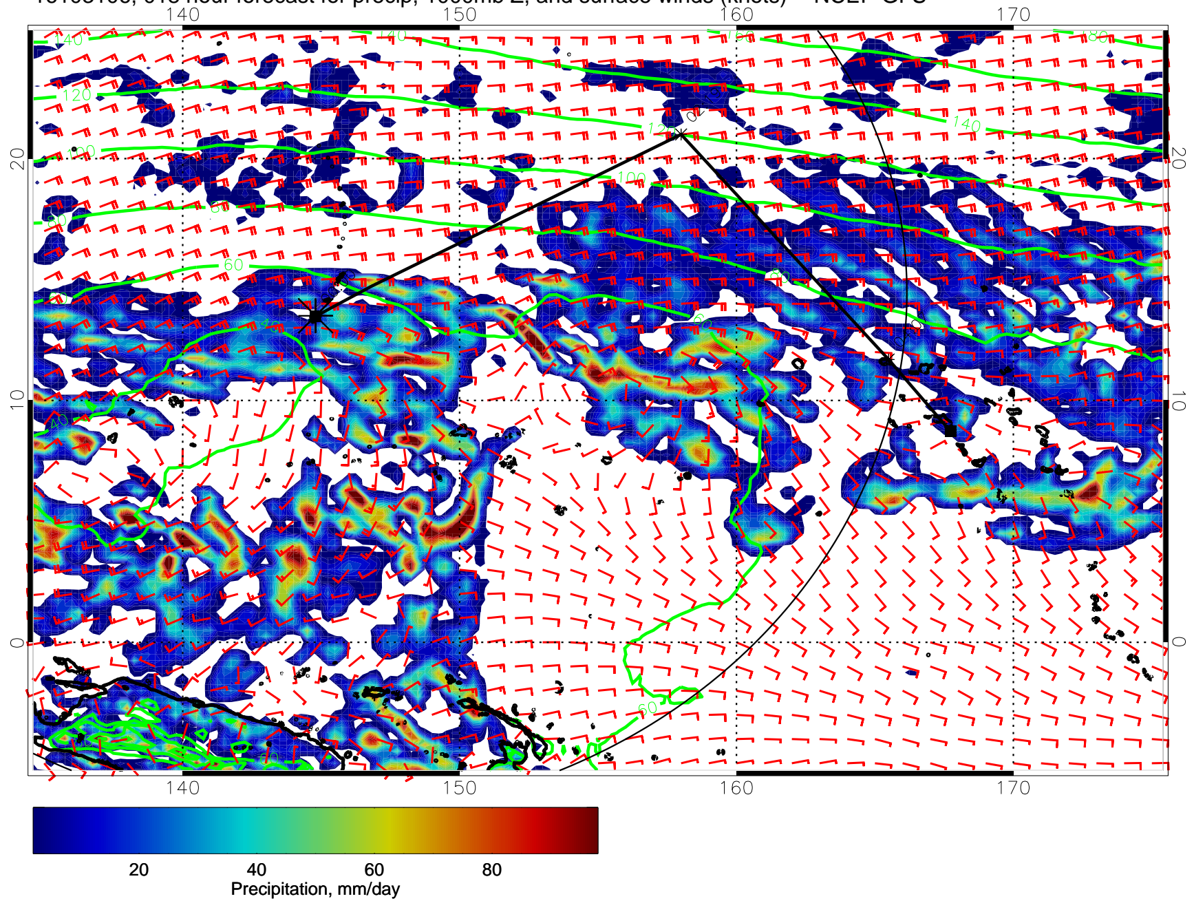
16103106, 018 hour forecast for precip, 1000mb Z, and surface winds (knots) -- NCEP GFS
