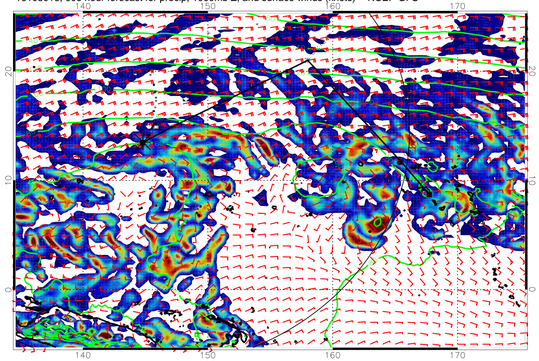
16103018, 006 hour forecast for precip, 1000mb Z, and surface winds (knots) -- NCEP GFS
