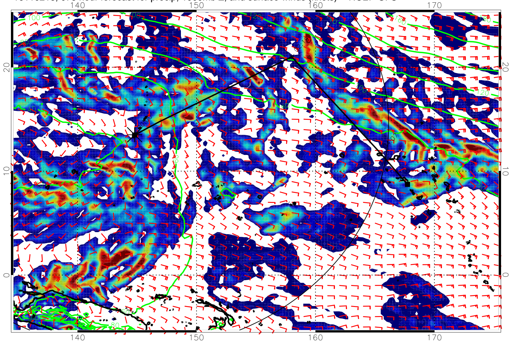
16110218, 078 hour forecast for precip, 1000mb Z, and surface winds (knots) -- NCEP GFS
