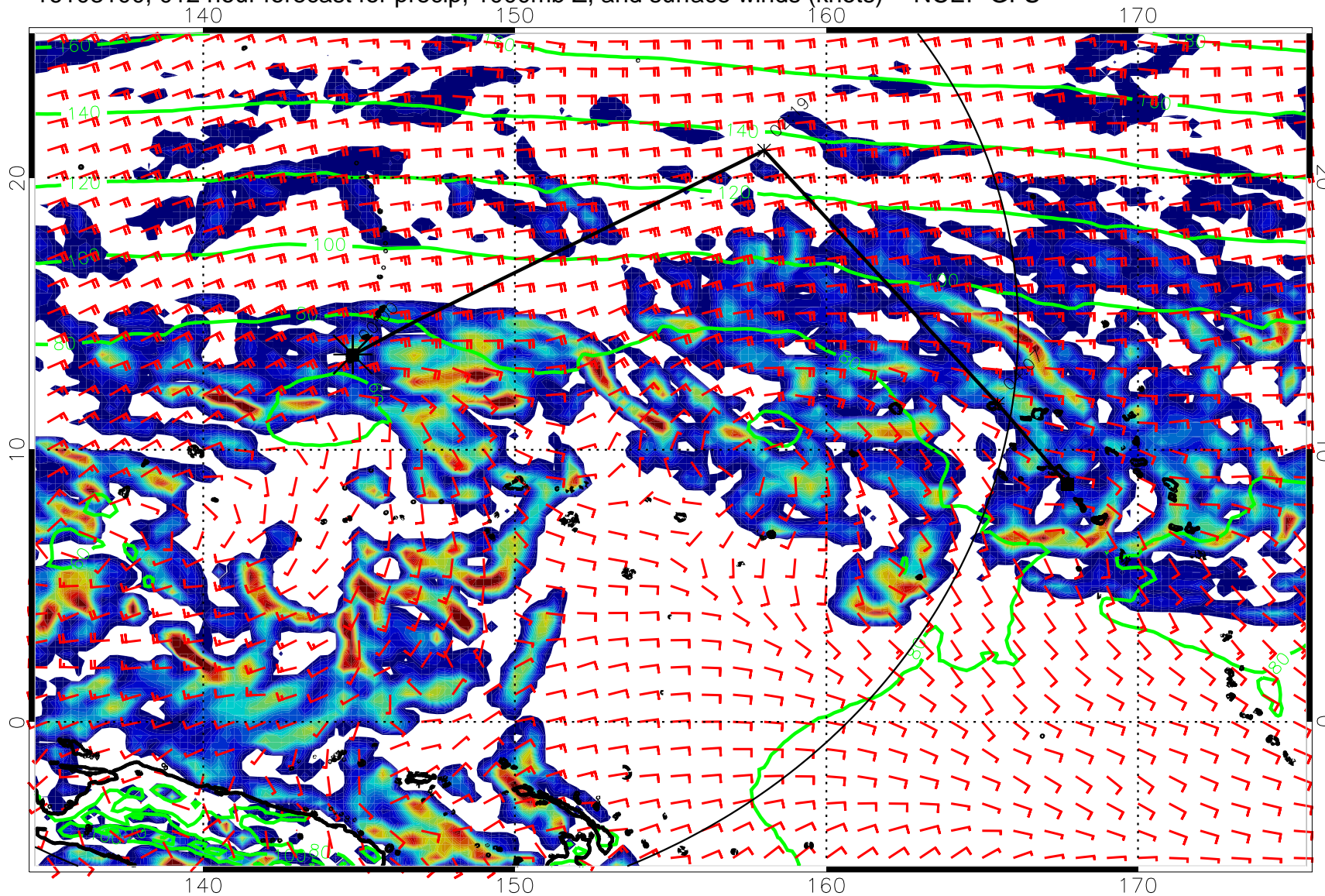
16103100, 012 hour forecast for precip, 1000mb Z, and surface winds (knots) -- NCEP GFS
