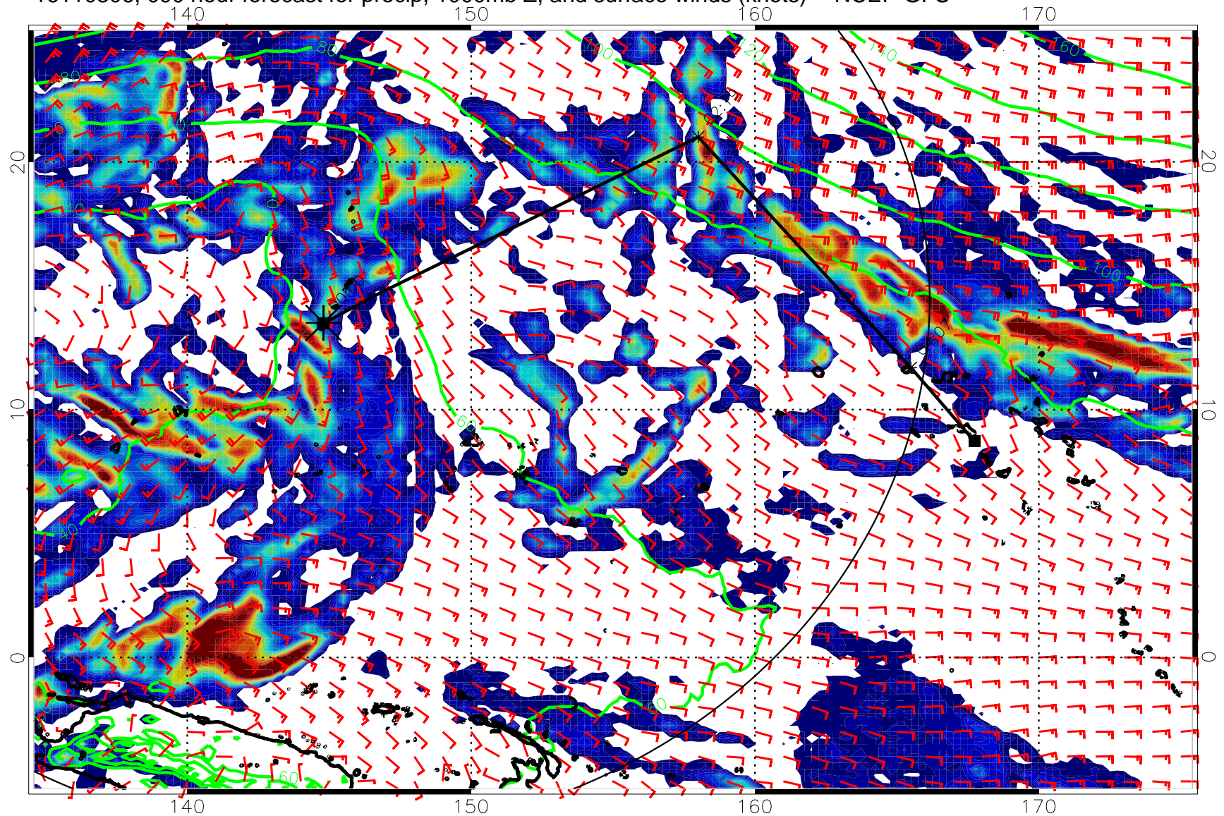
16110306, 090 hour forecast for precip, 1000mb Z, and surface winds (knots) -- NCEP GFS
