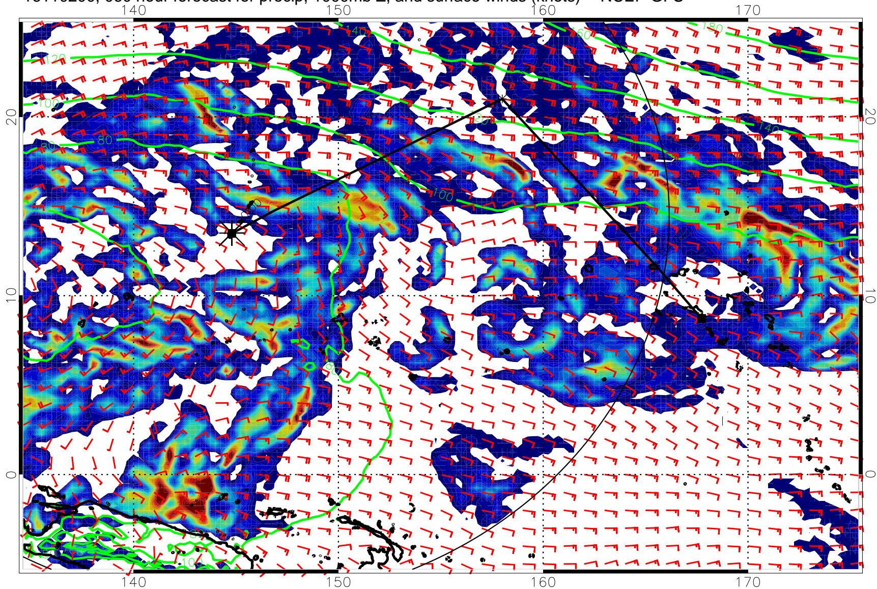
16110200, 060 hour forecast for precip, 1000mb Z, and surface winds (knots) -- NCEP GFS
