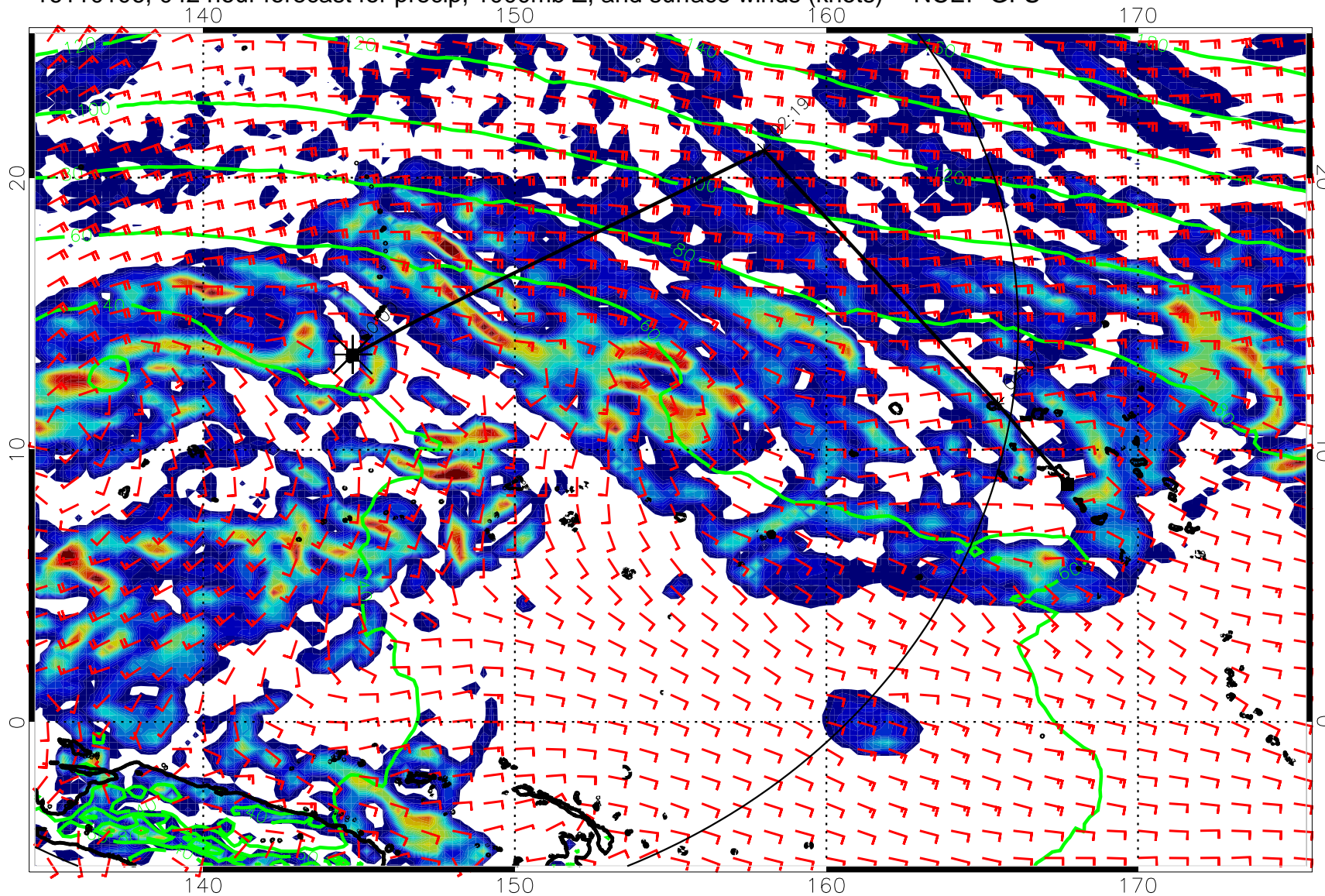
16110106, 042 hour forecast for precip, 1000mb Z, and surface winds (knots) -- NCEP GFS
