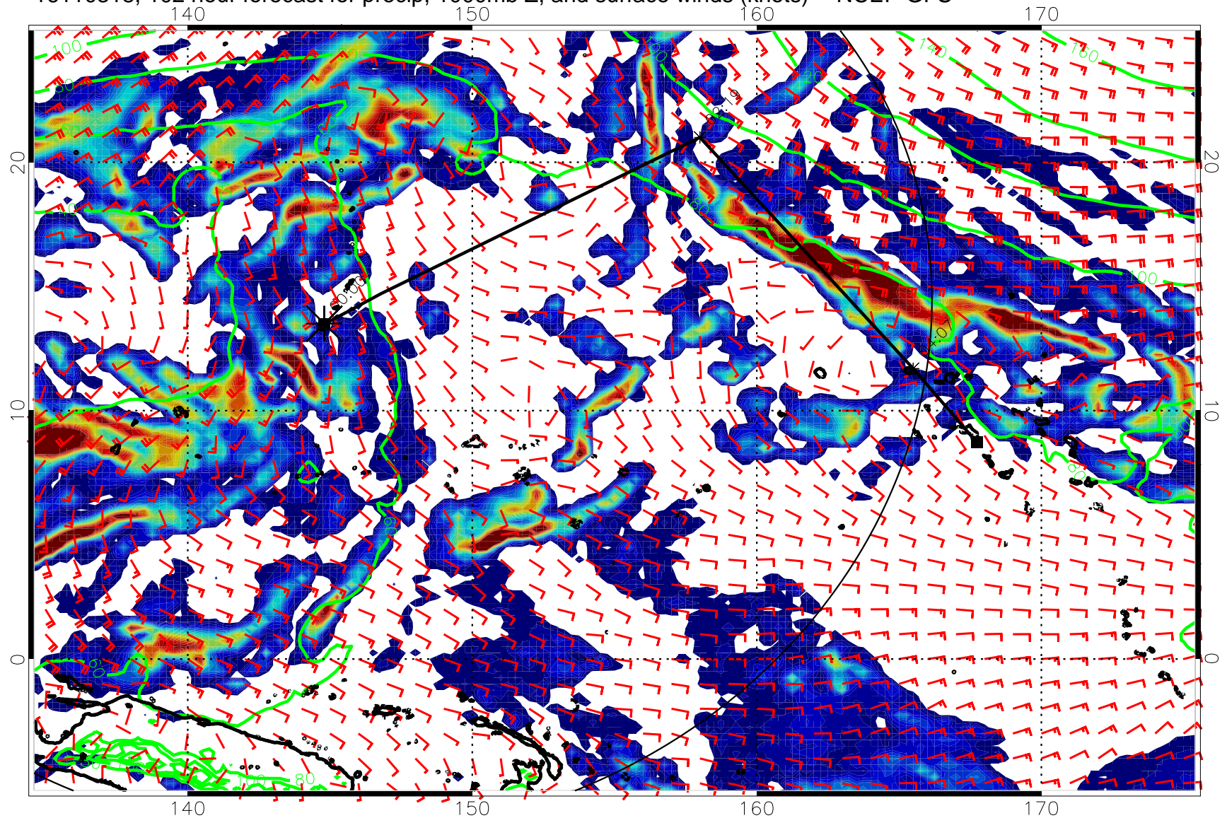
16110318, 102 hour forecast for precip, 1000mb Z, and surface winds (knots) -- NCEP GFS
