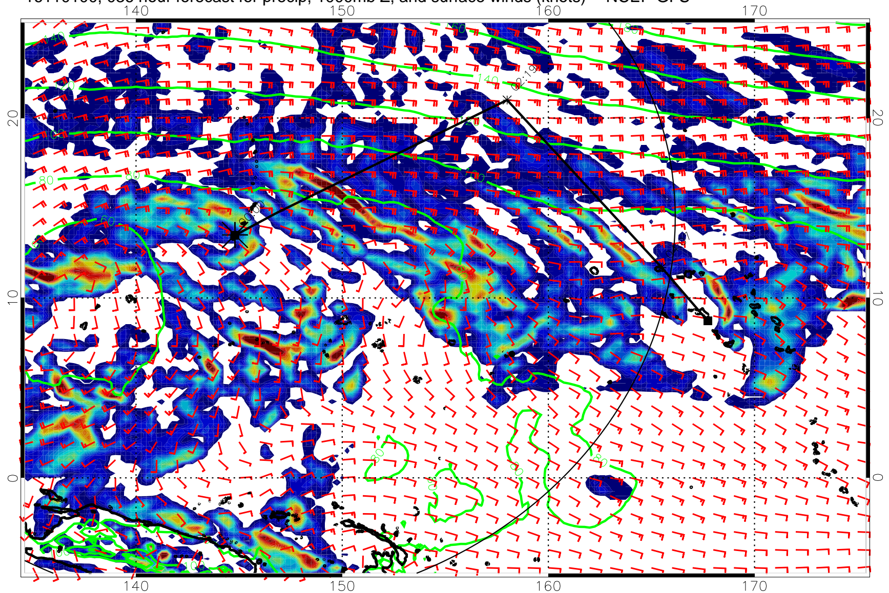
16110100, 036 hour forecast for precip, 1000mb Z, and surface winds (knots) -- NCEP GFS
