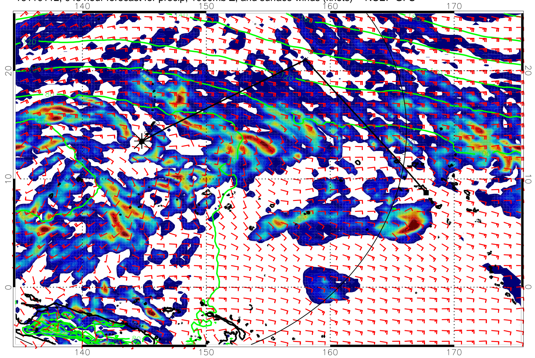
16110112, 048 hour forecast for precip, 1000mb Z, and surface winds (knots) -- NCEP GFS
