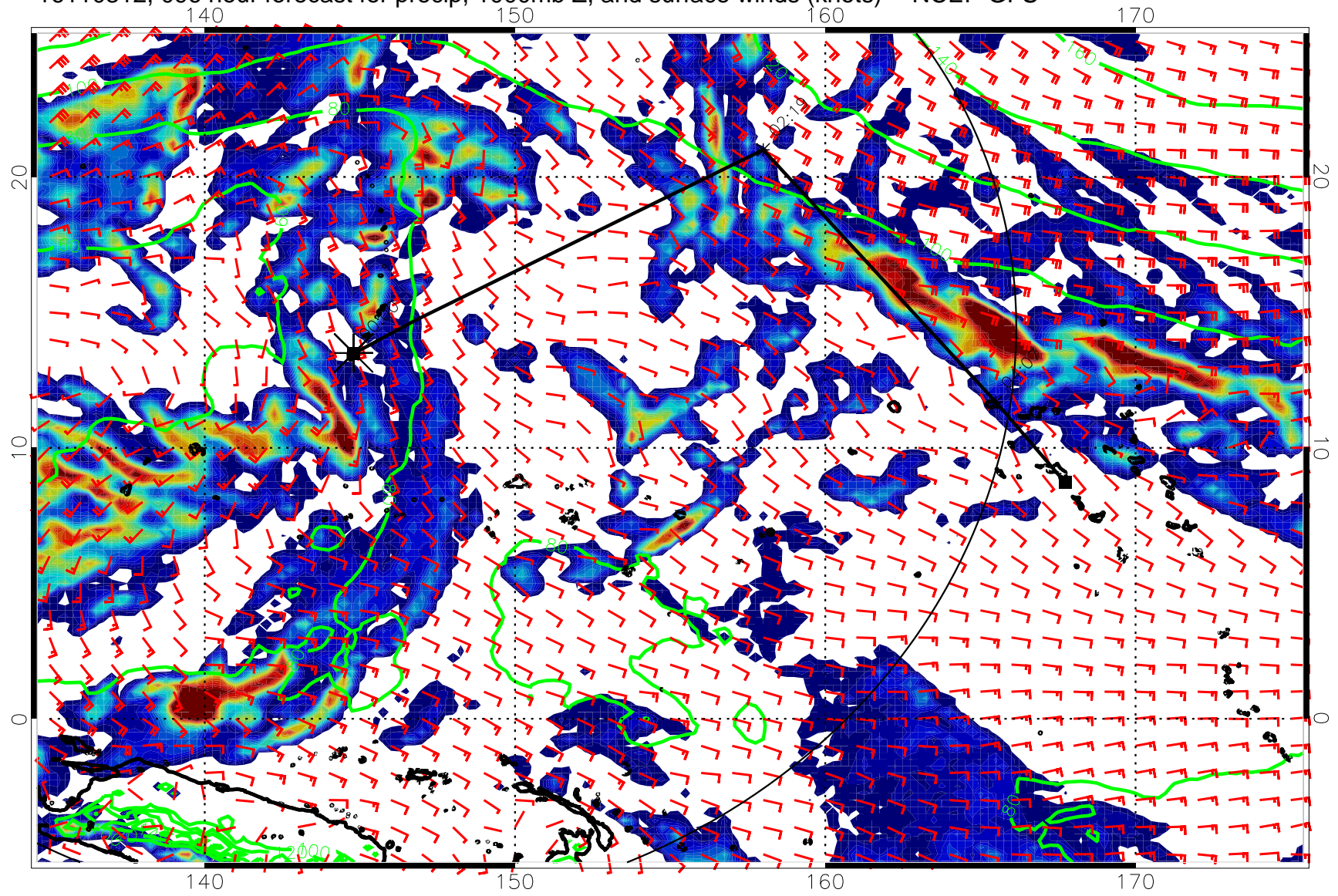
16110312, 096 hour forecast for precip, 1000mb Z, and surface winds (knots) -- NCEP GFS
