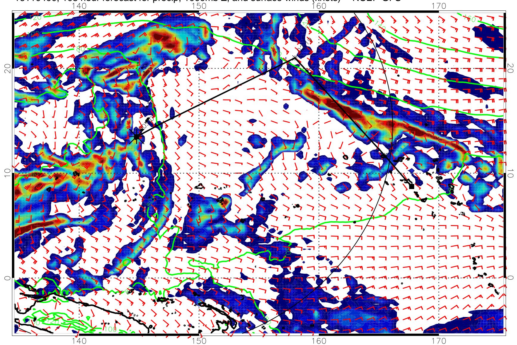
16110400, 108 hour forecast for precip, 1000mb Z, and surface winds (knots) -- NCEP GFS
