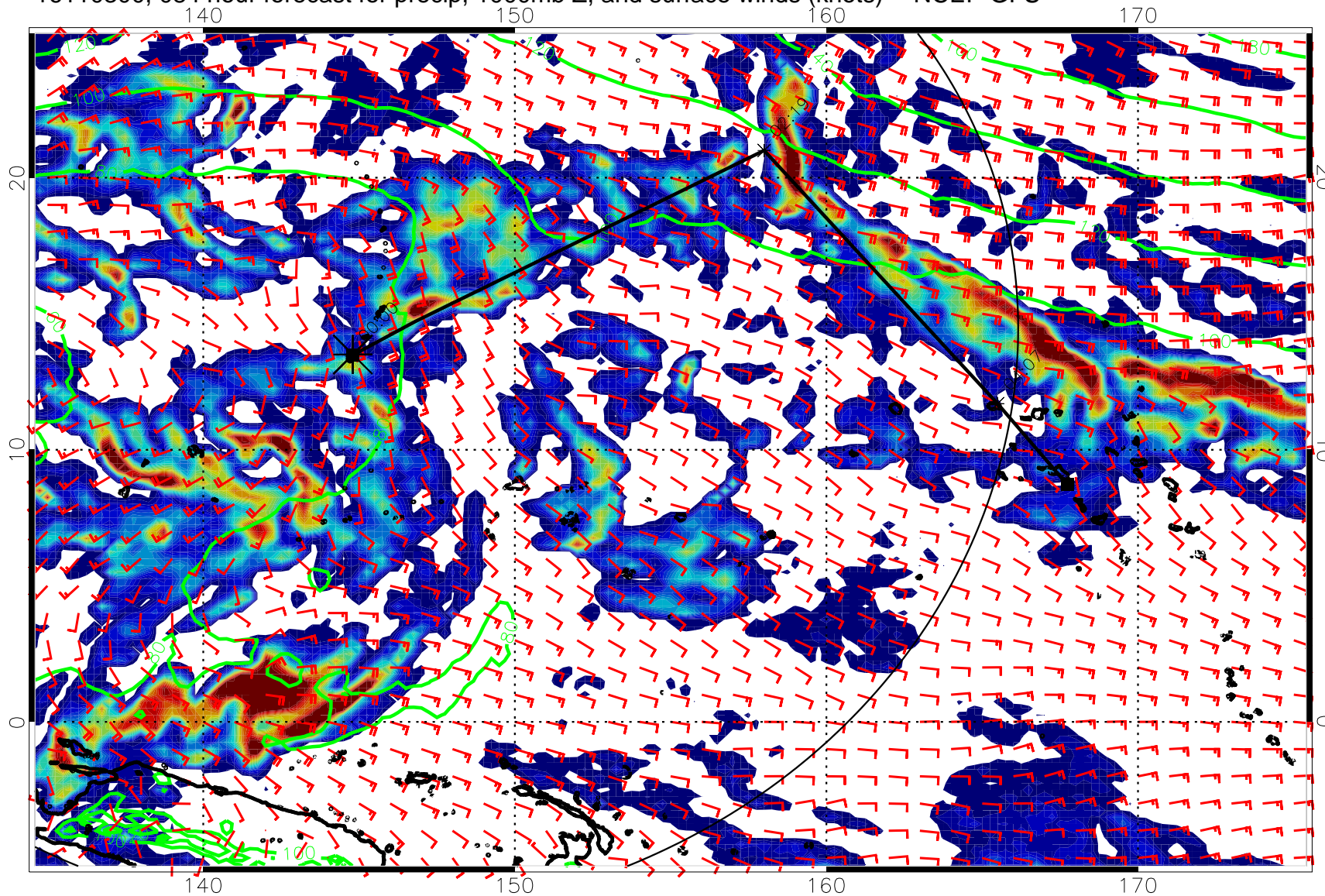
16110300, 084 hour forecast for precip, 1000mb Z, and surface winds (knots) -- NCEP GFS
