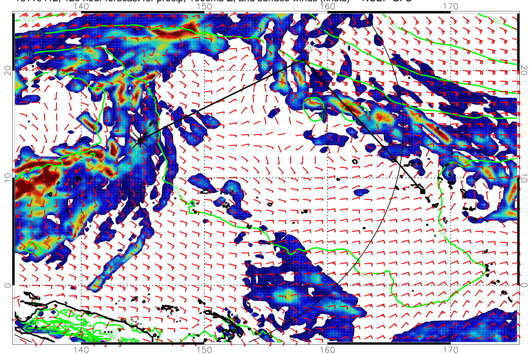
16110412, 120 hour forecast for precip, 1000mb Z, and surface winds (knots) -- NCEP GFS
