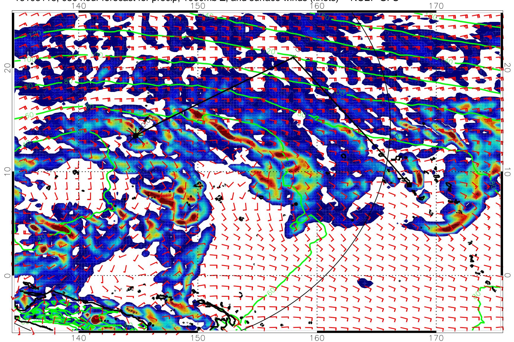
16103118, 030 hour forecast for precip, 1000mb Z, and surface winds (knots) -- NCEP GFS
