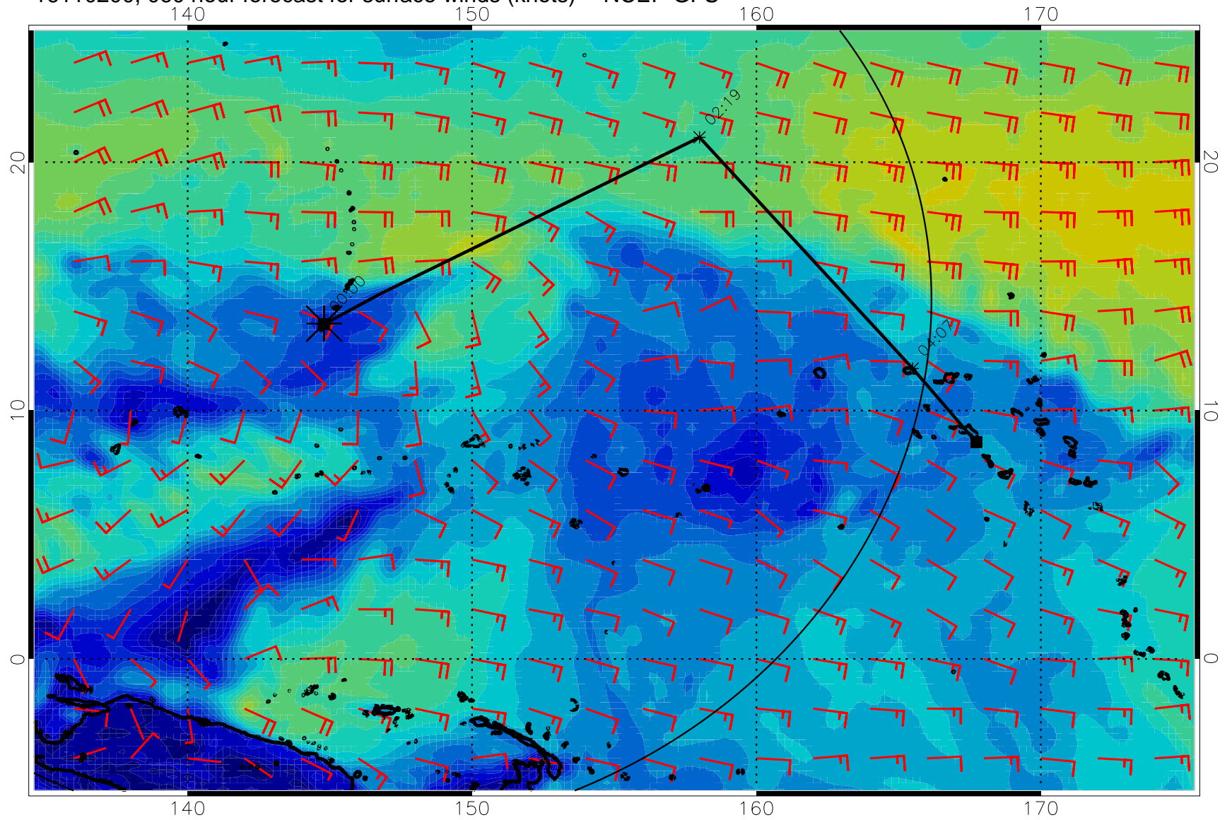
16110200, 060 hour forecast for surface winds (knots) -- NCEP GFS
