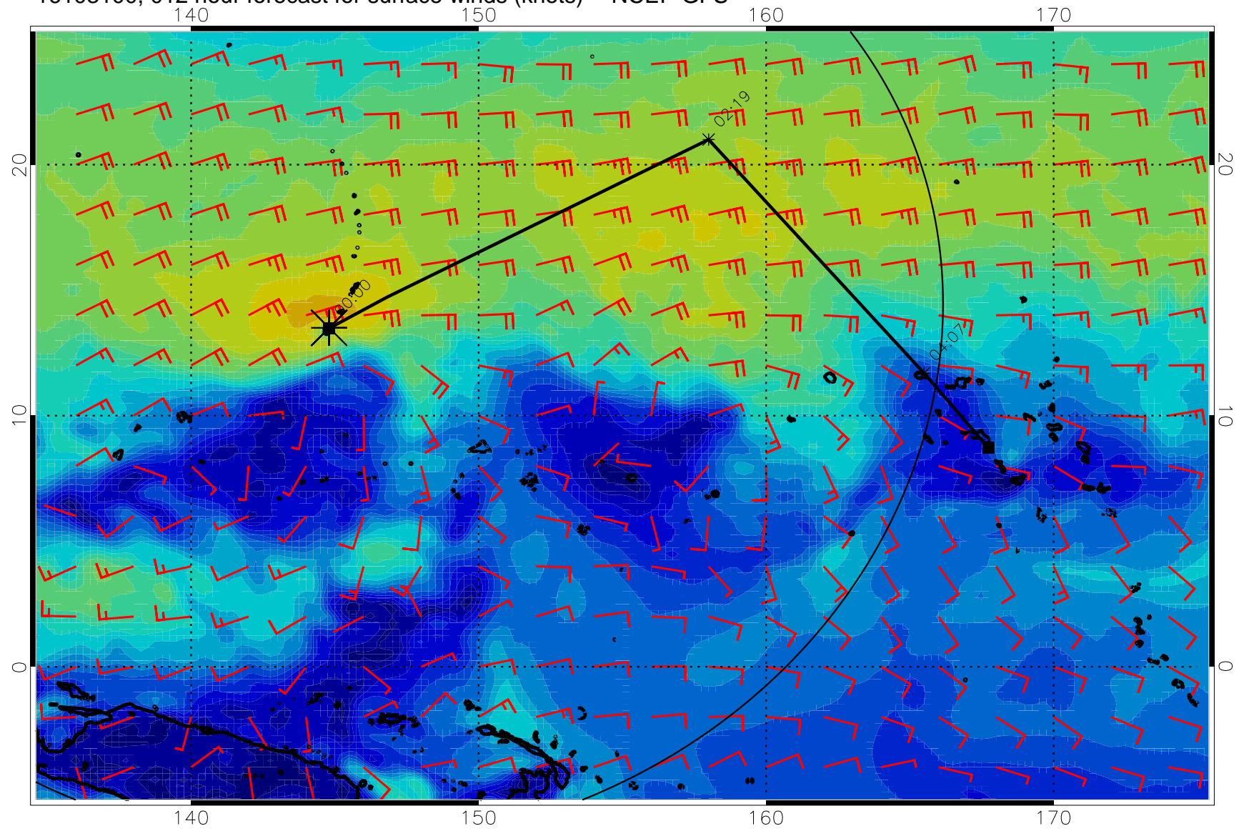
16103100, 012 hour forecast for surface winds (knots) -- NCEP GFS
