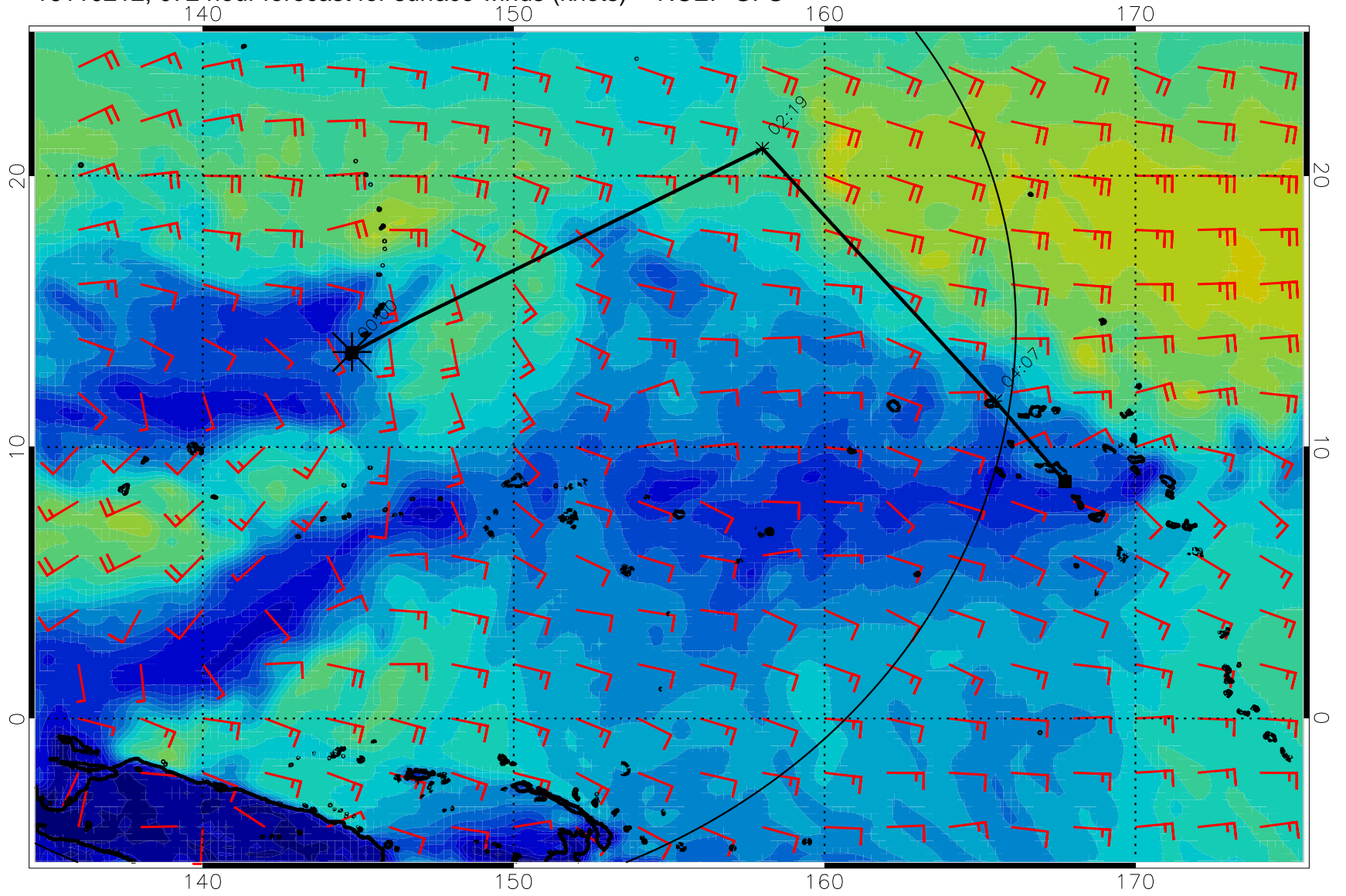
16110212, 072 hour forecast for surface winds (knots) -- NCEP GFS
