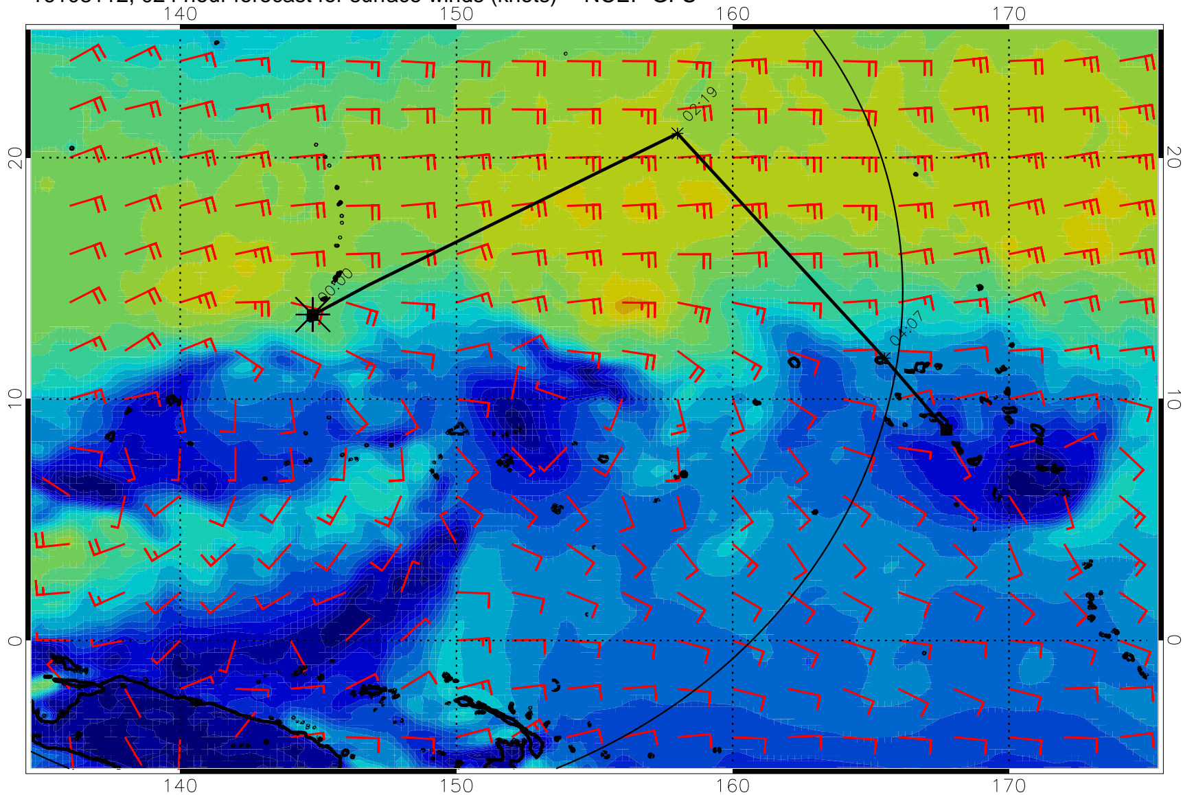
16103112, 024 hour forecast for surface winds (knots) -- NCEP GFS
