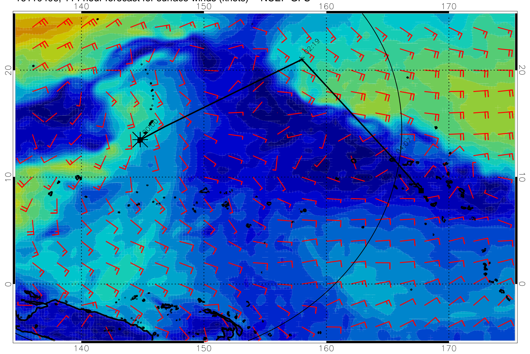
16110406, 114 hour forecast for surface winds (knots) -- NCEP GFS
