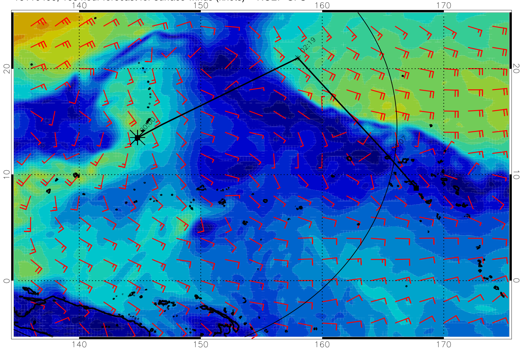
16110400, 108 hour forecast for surface winds (knots) -- NCEP GFS
