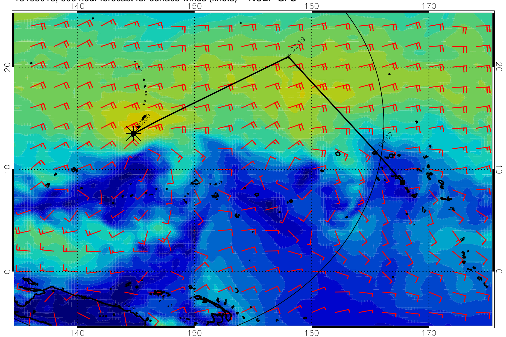
16103018, 006 hour forecast for surface winds (knots) -- NCEP GFS
