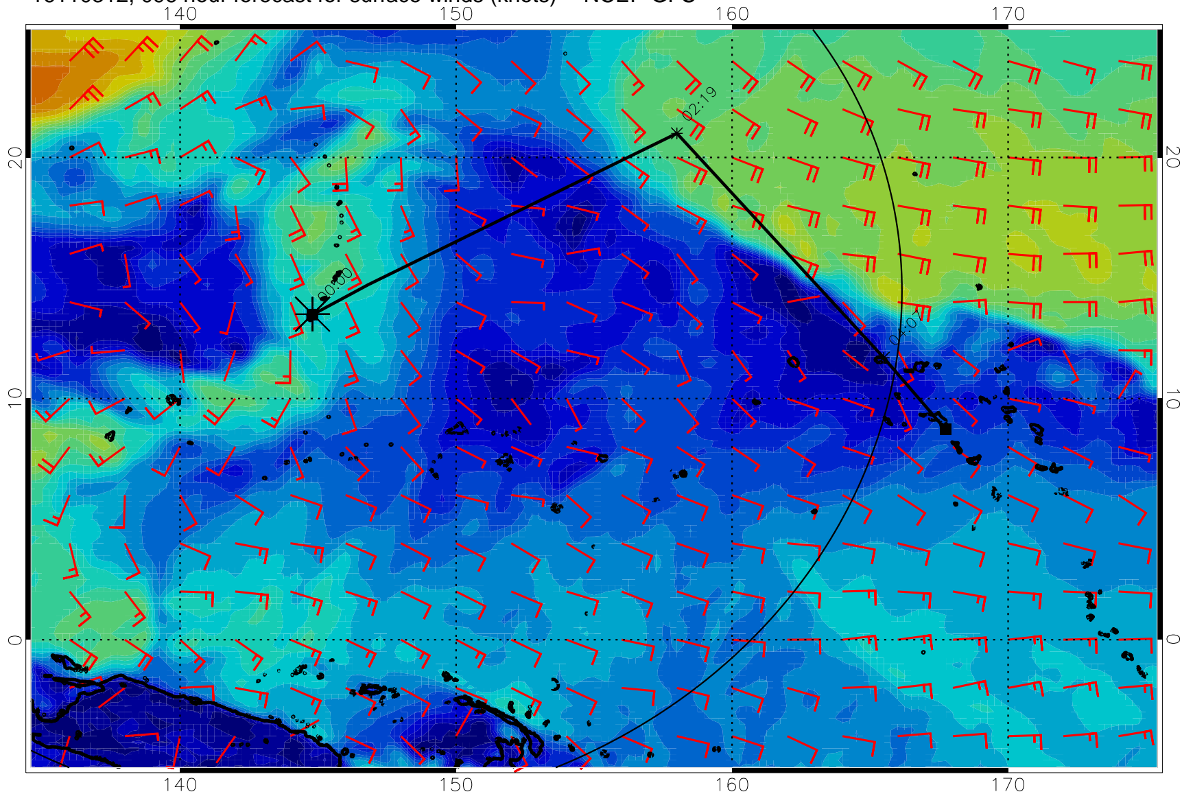
16110312, 096 hour forecast for surface winds (knots) -- NCEP GFS
