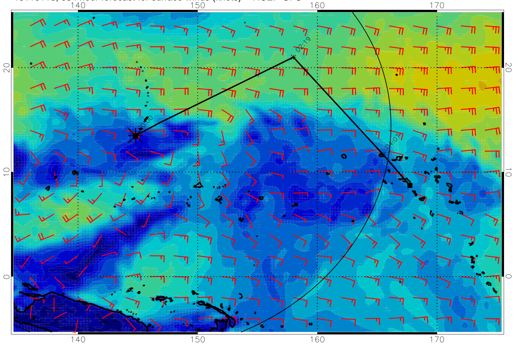
16110118, 054 hour forecast for surface winds (knots) -- NCEP GFS
