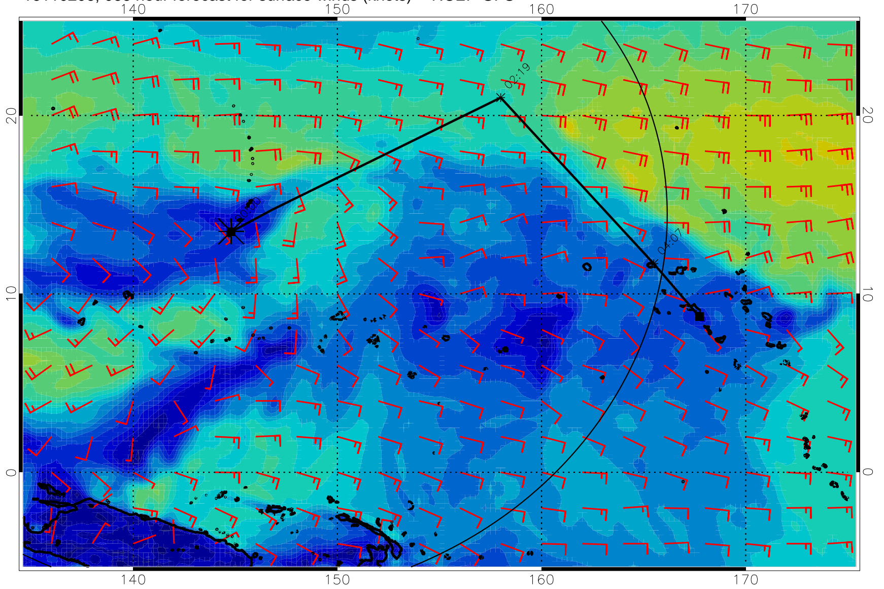
16110206, 066 hour forecast for surface winds (knots) -- NCEP GFS
