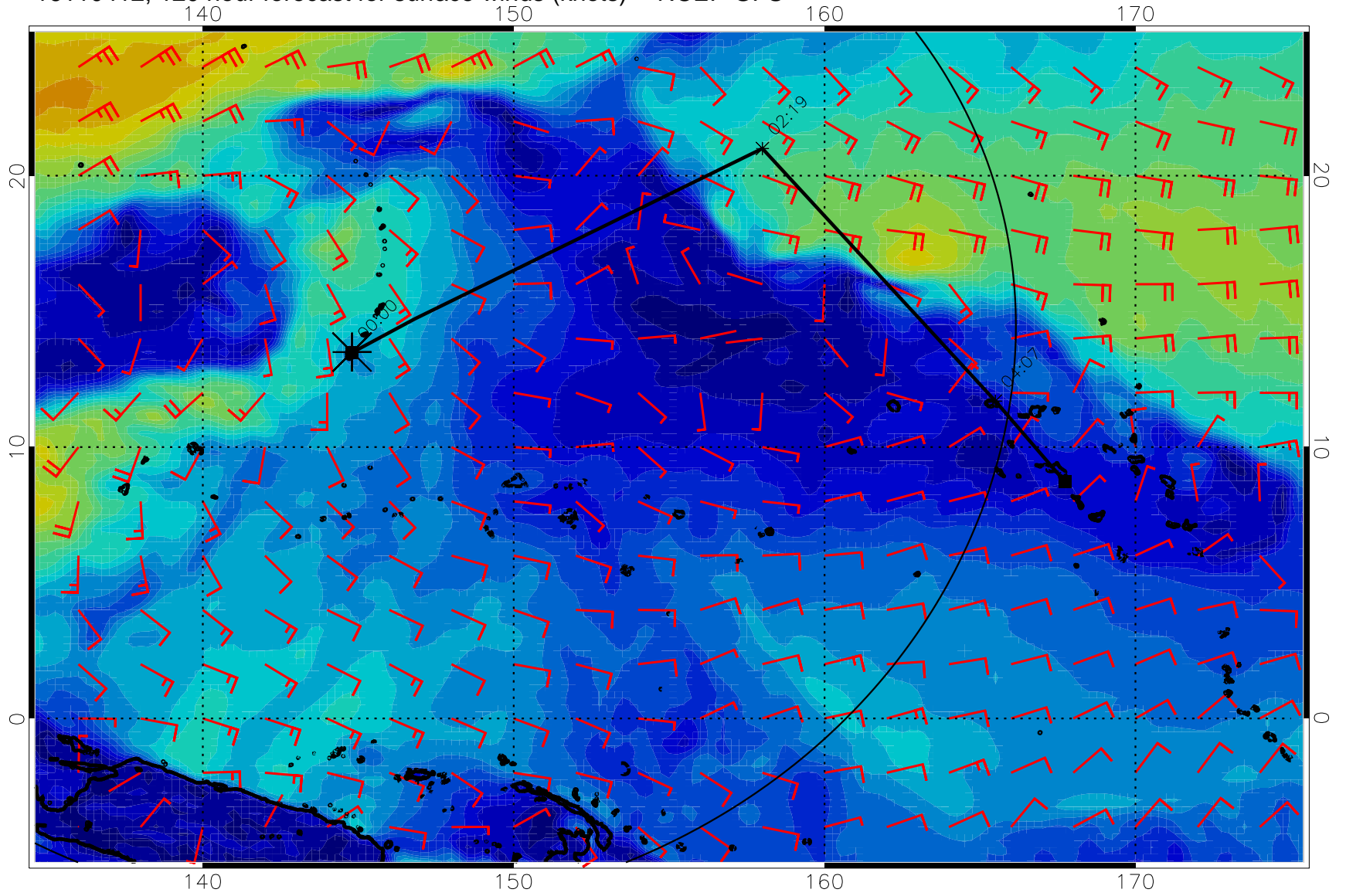
16110412, 120 hour forecast for surface winds (knots) -- NCEP GFS
