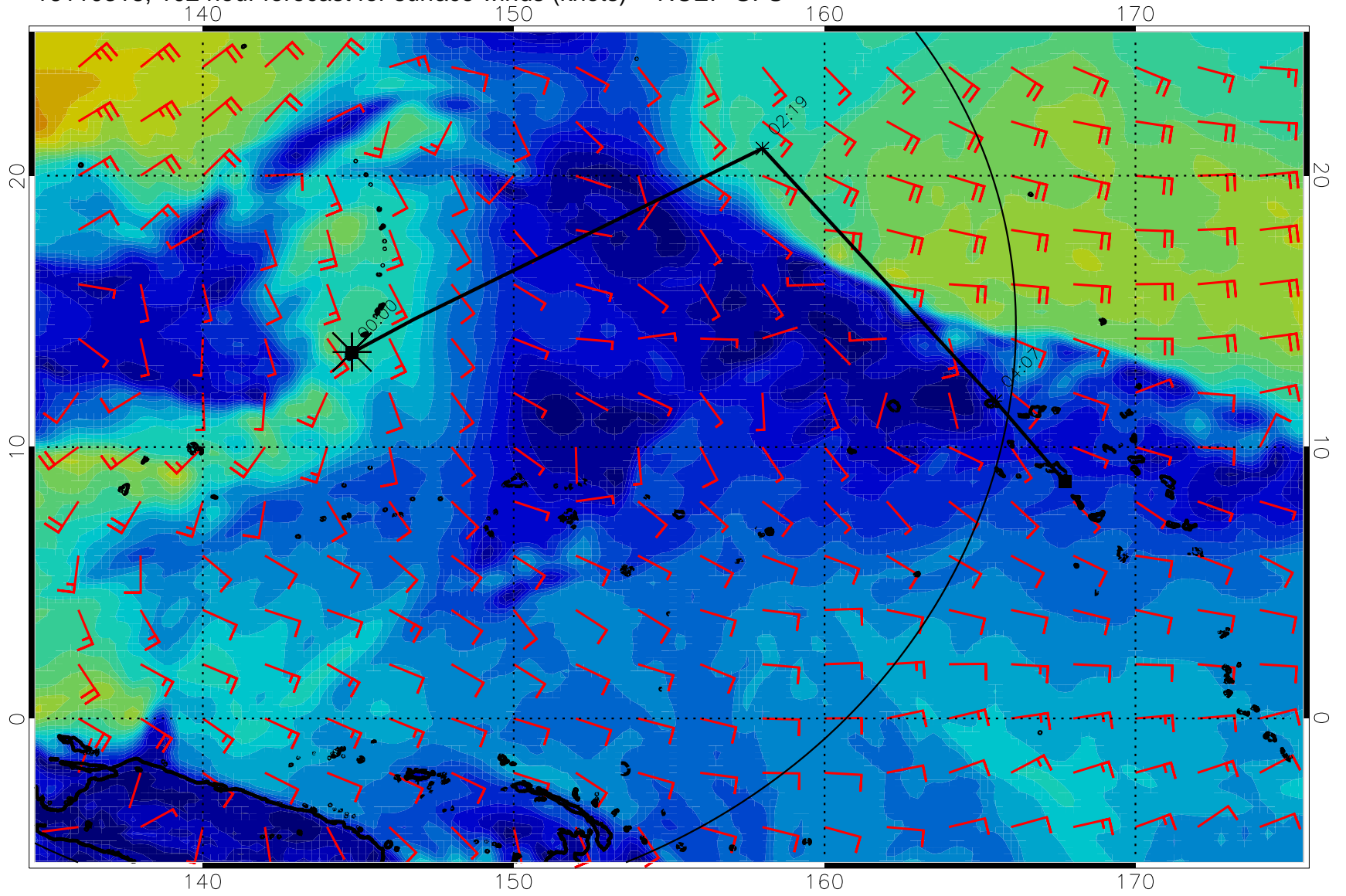
16110318, 102 hour forecast for surface winds (knots) -- NCEP GFS
