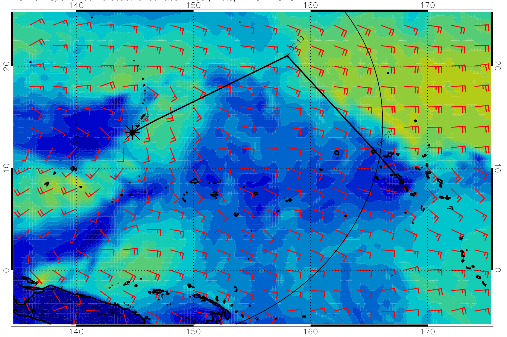
16110218, 078 hour forecast for surface winds (knots) -- NCEP GFS
