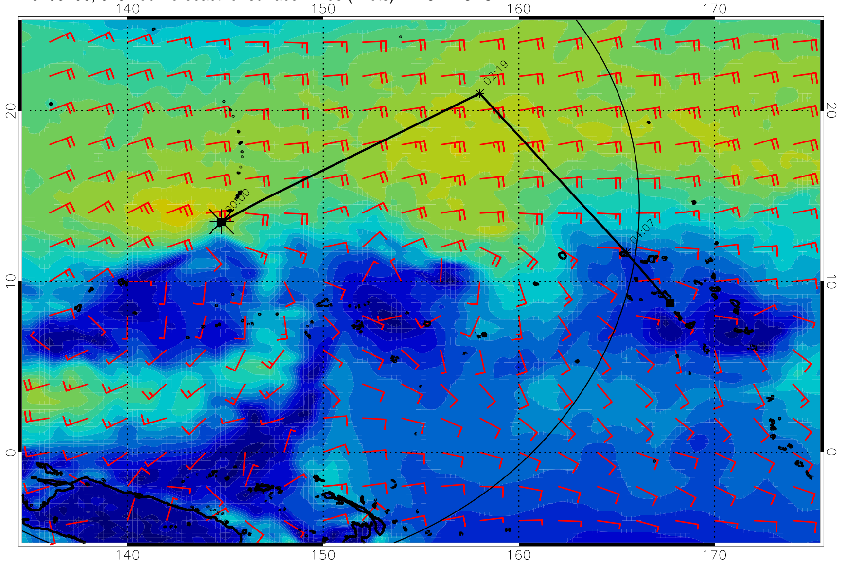
16103106, 018 hour forecast for surface winds (knots) -- NCEP GFS
