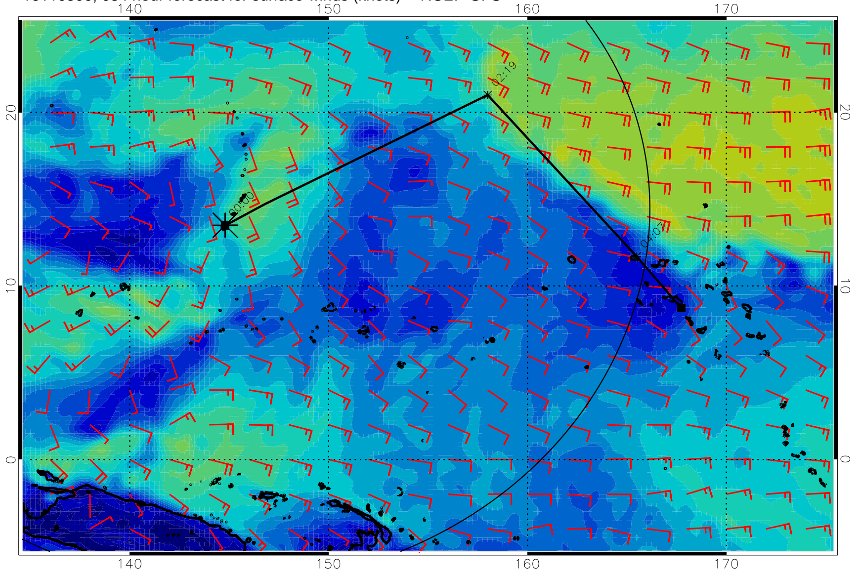
16110300, 084 hour forecast for surface winds (knots) -- NCEP GFS
