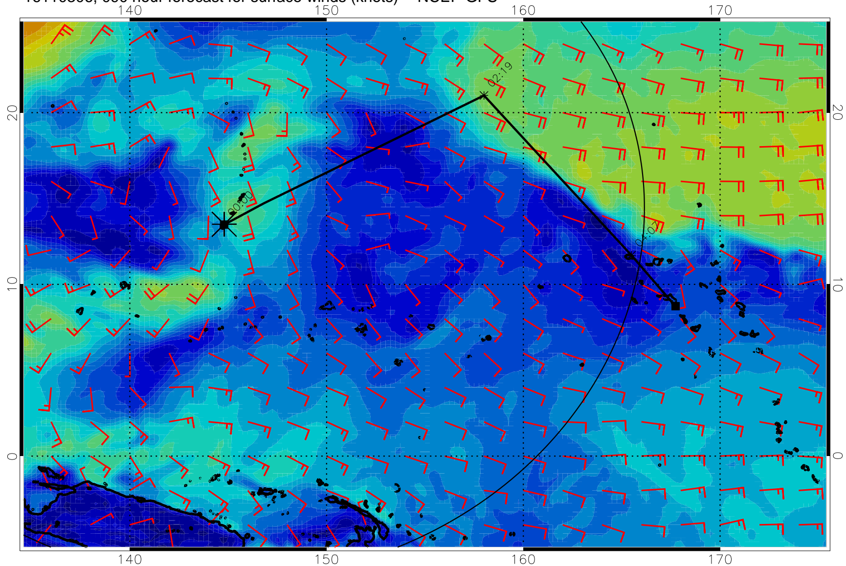
16110306, 090 hour forecast for surface winds (knots) -- NCEP GFS
