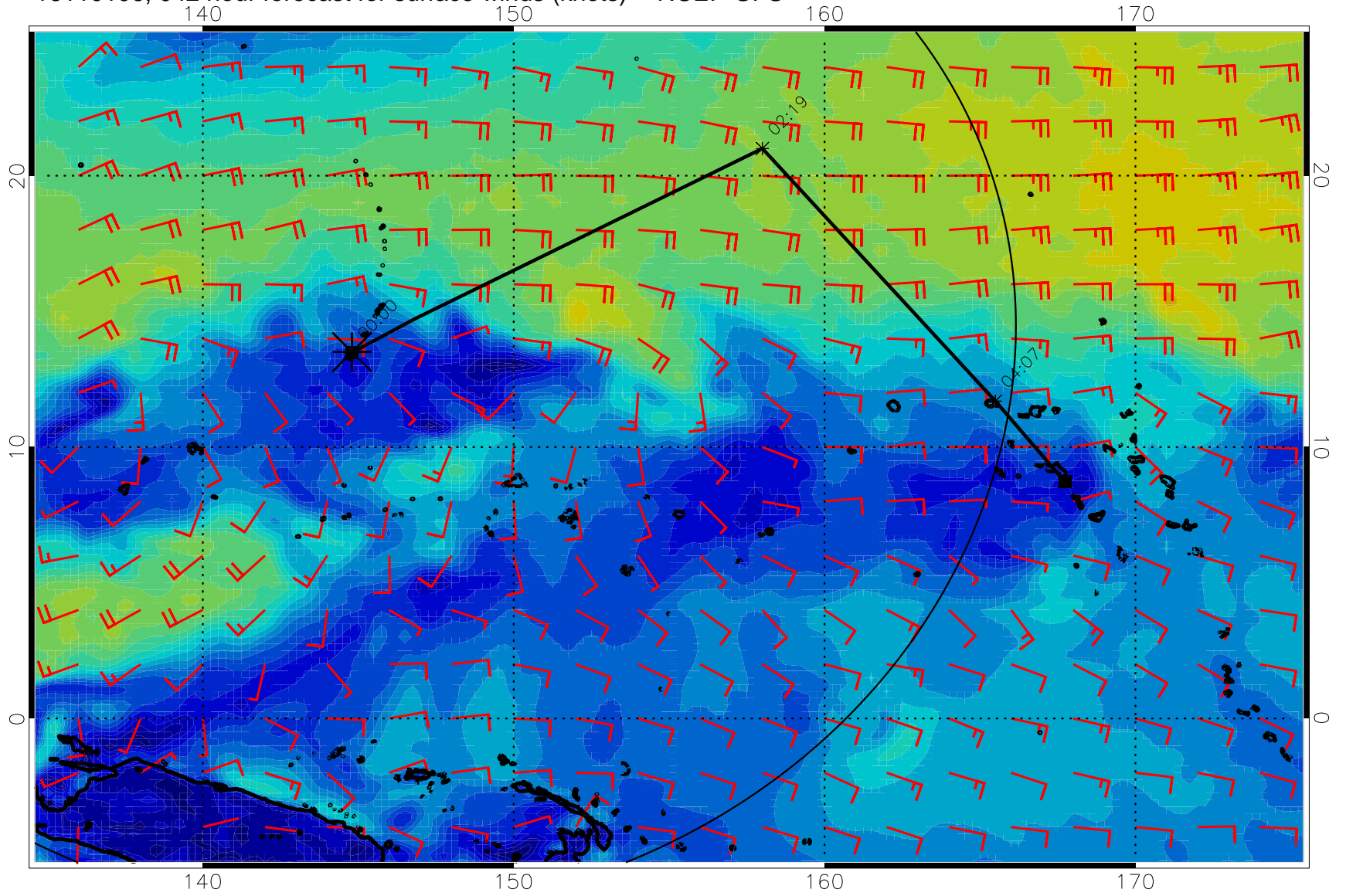
16110106, 042 hour forecast for surface winds (knots) -- NCEP GFS
