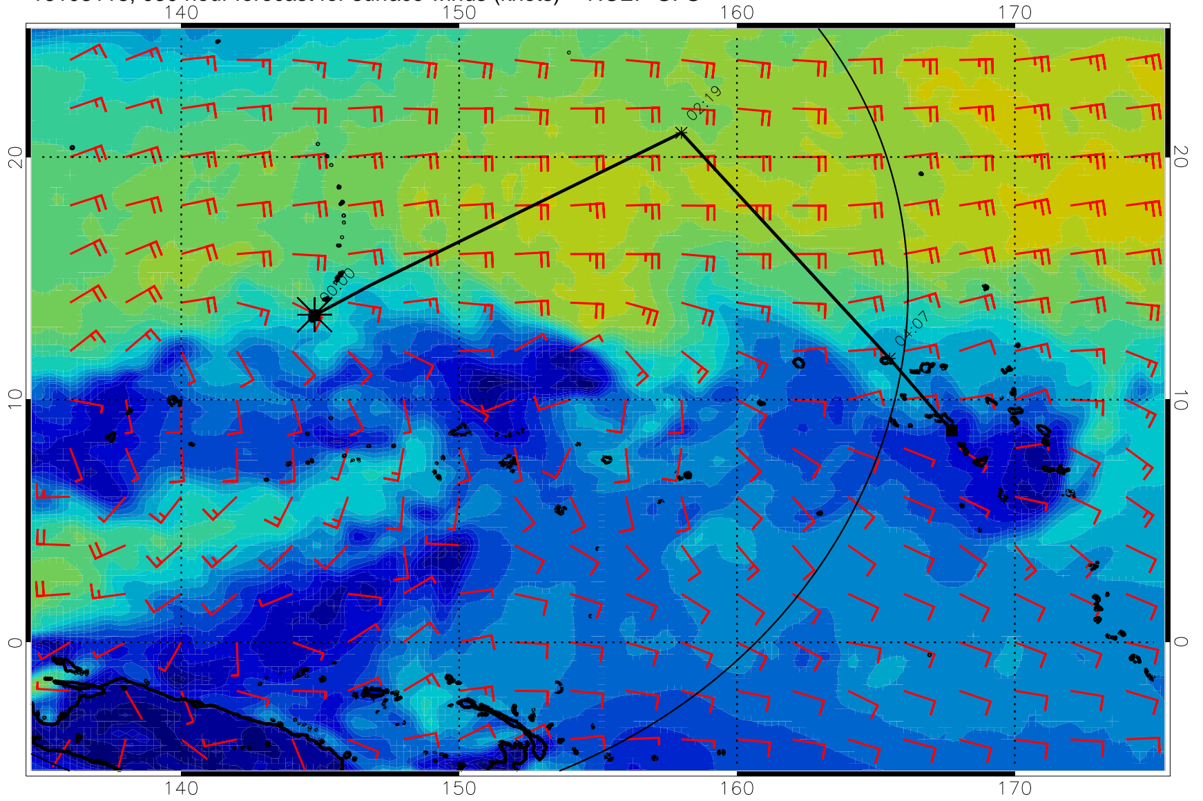
16103118, 030 hour forecast for surface winds (knots) -- NCEP GFS
