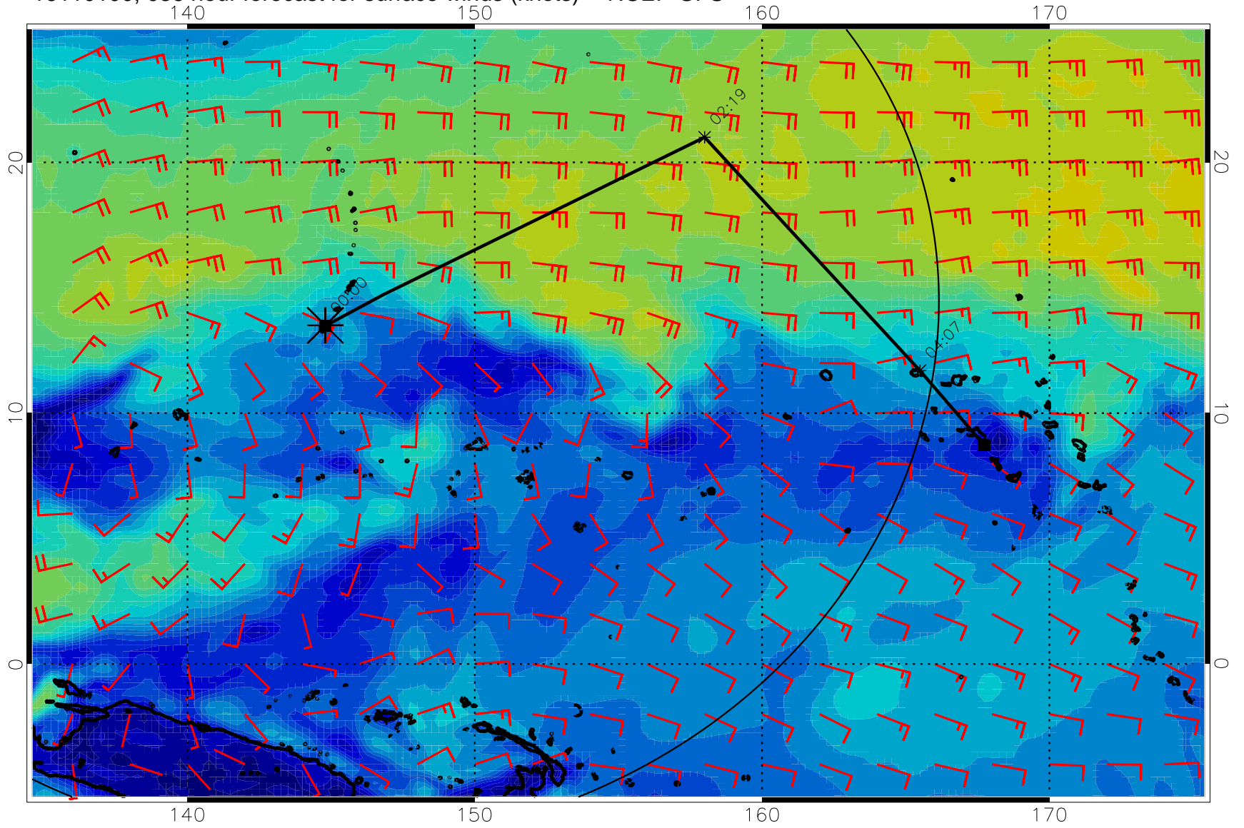
16110100, 036 hour forecast for surface winds (knots) -- NCEP GFS
