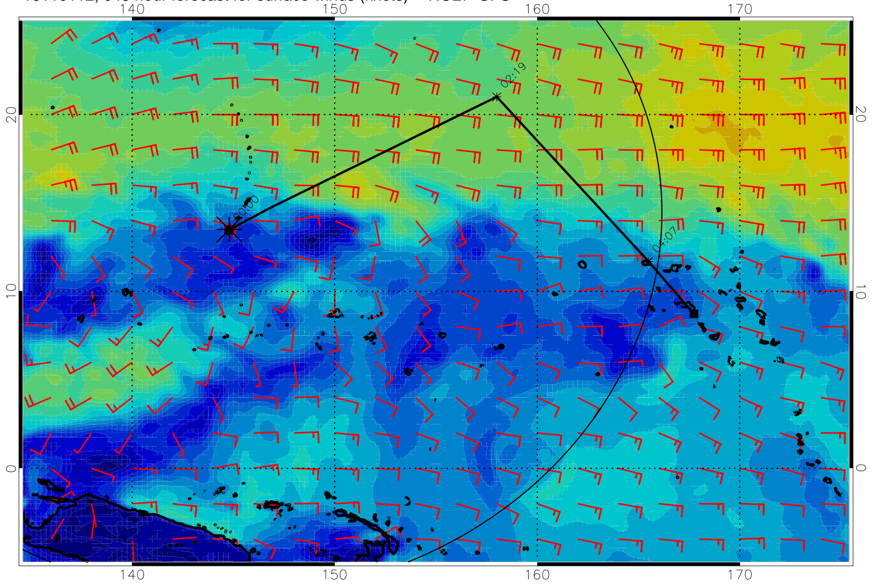
16110112, 048 hour forecast for surface winds (knots) -- NCEP GFS
