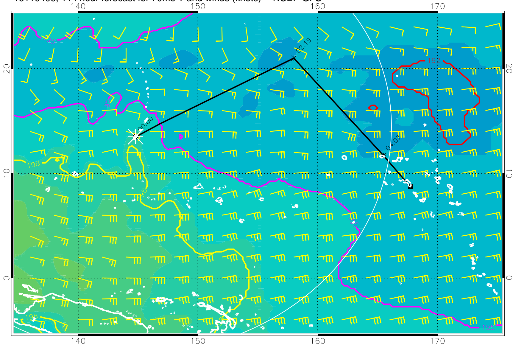
16110406, 114 hour forecast for 70mb T and winds (knots) -- NCEP GFS
