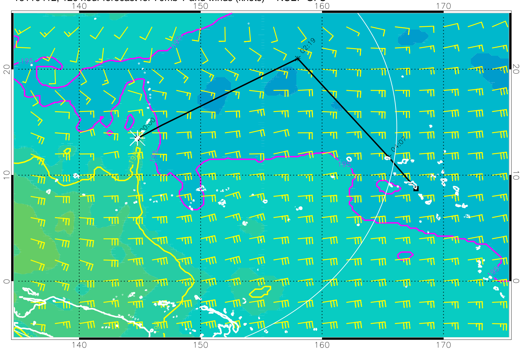
16110412, 120 hour forecast for 70mb T and winds (knots) -- NCEP GFS
