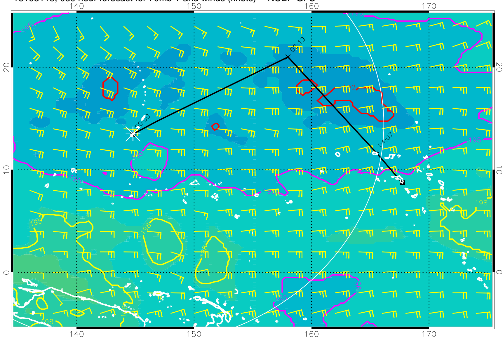
16103118, 030 hour forecast for 70mb T and winds (knots) -- NCEP GFS
