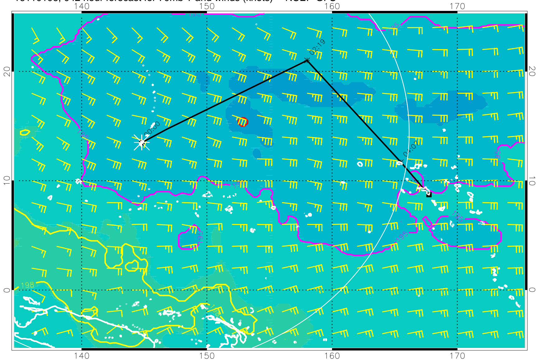
16110106, 042 hour forecast for 70mb T and winds (knots) -- NCEP GFS
