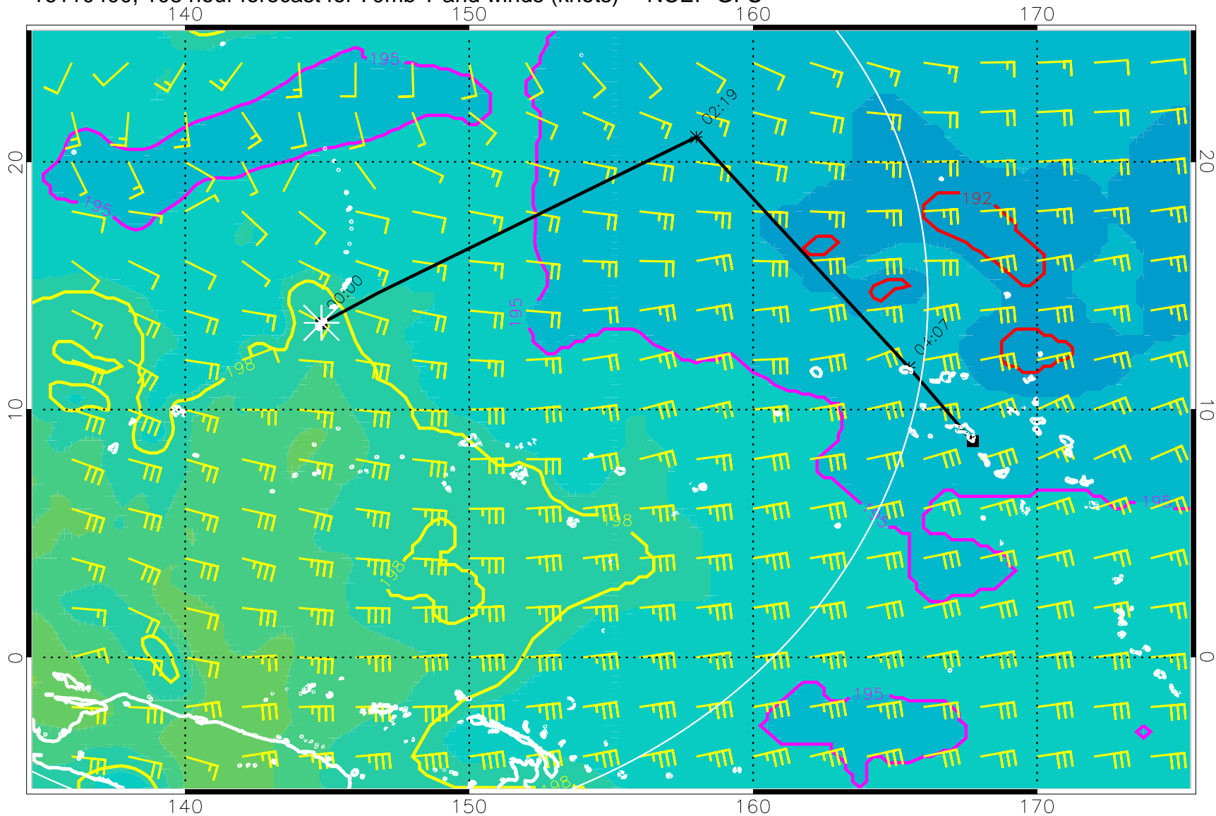
16110400, 108 hour forecast for 70mb T and winds (knots) -- NCEP GFS
