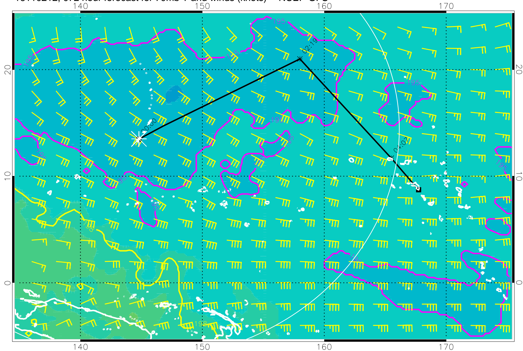
16110212, 072 hour forecast for 70mb T and winds (knots) -- NCEP GFS
