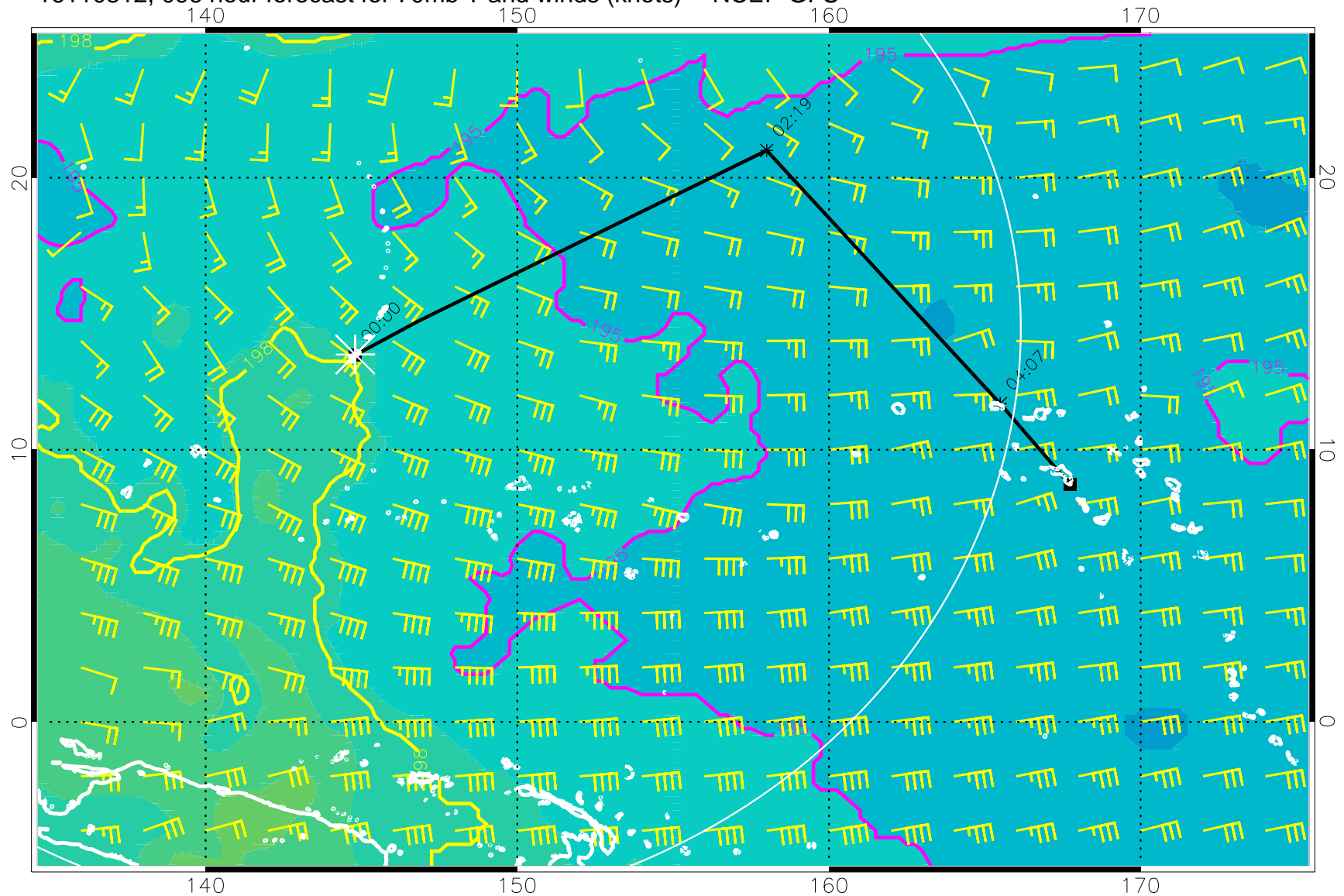
16110312, 096 hour forecast for 70mb T and winds (knots) -- NCEP GFS
