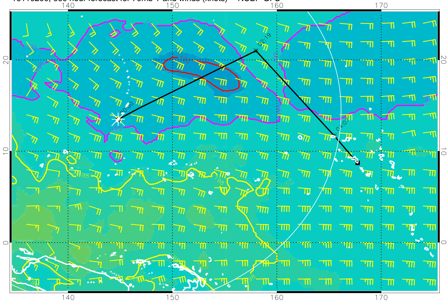
16110200, 060 hour forecast for 70mb T and winds (knots) -- NCEP GFS
