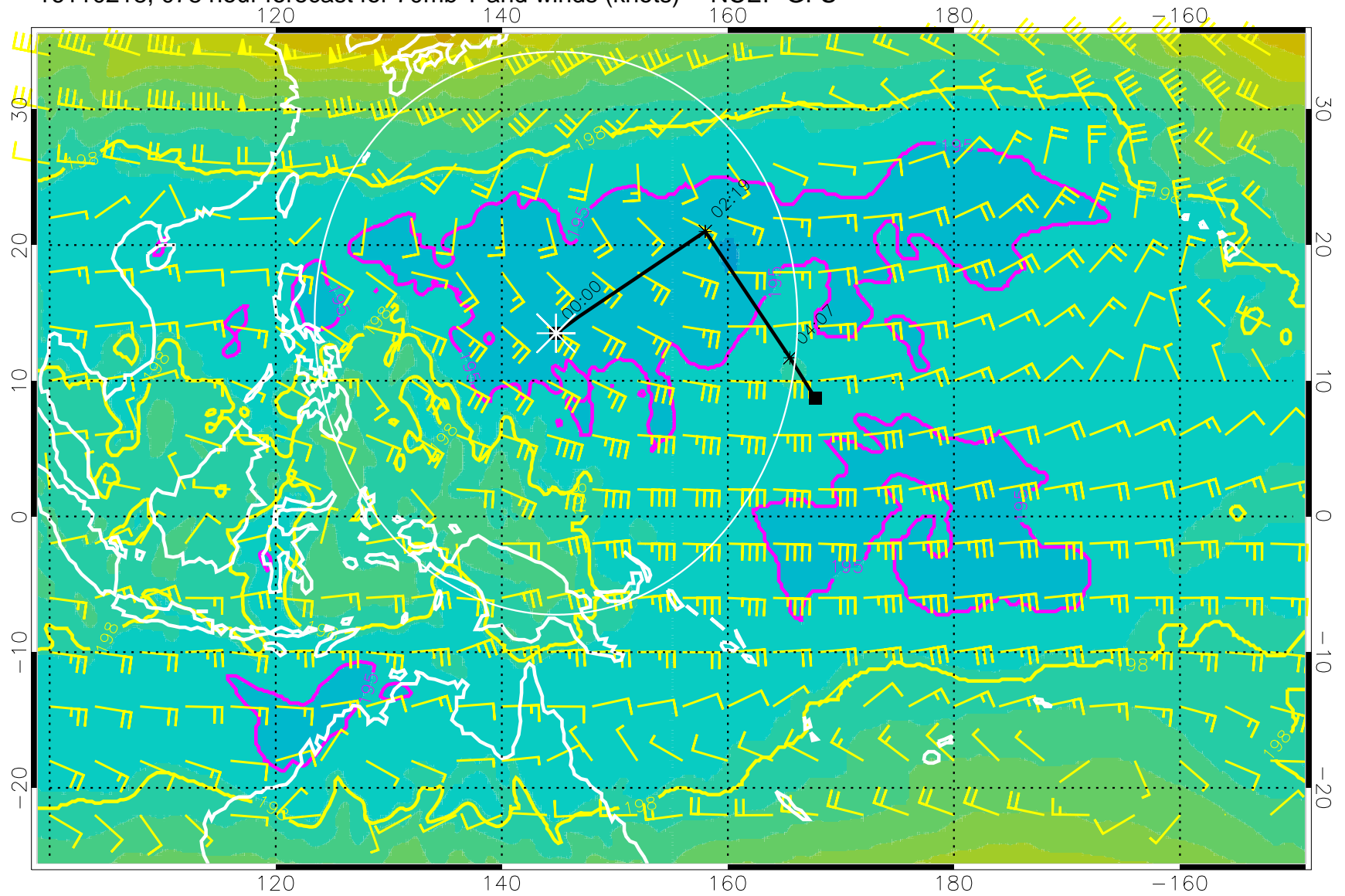
16110218, 078 hour forecast for 70mb T and winds (knots) -- NCEP GFS
