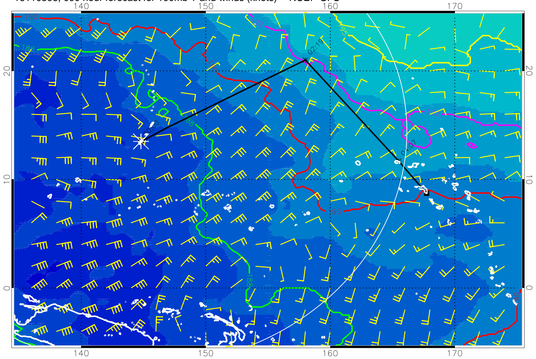
16110306, 090 hour forecast for 100mb T and winds (knots) -- NCEP GFS
