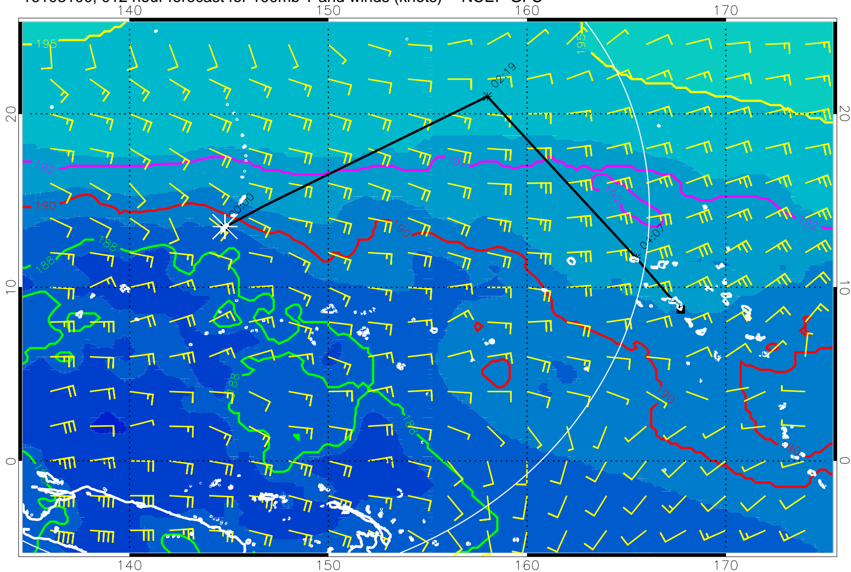
16103100, 012 hour forecast for 100mb T and winds (knots) -- NCEP GFS
