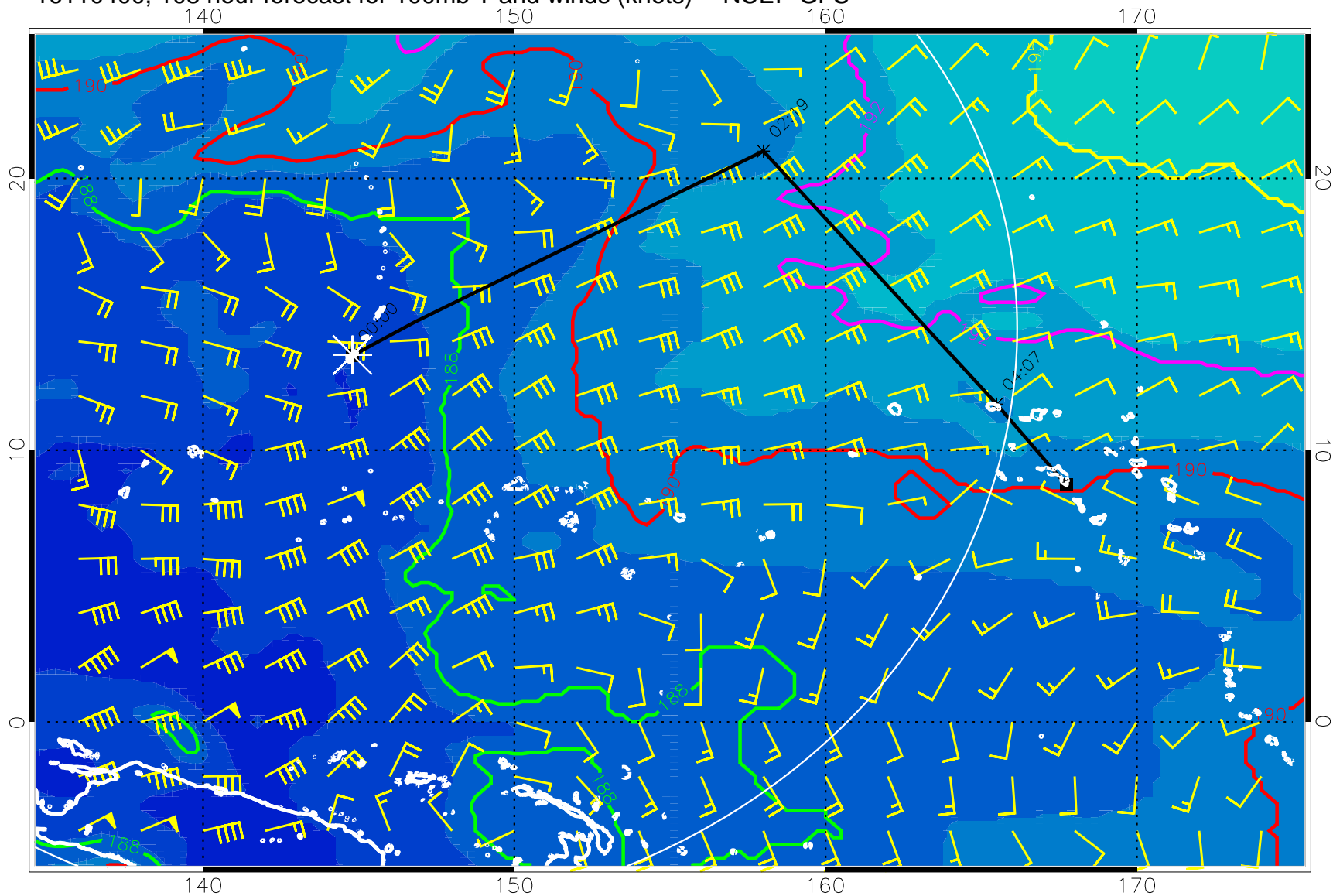
16110400, 108 hour forecast for 100mb T and winds (knots) -- NCEP GFS
