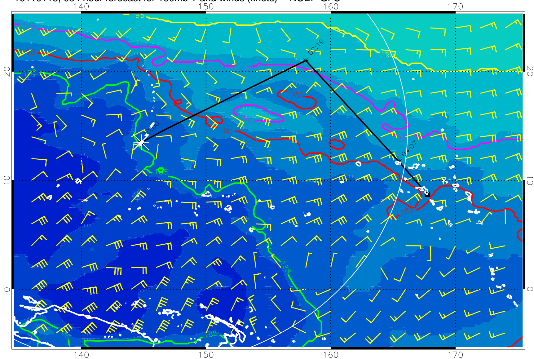
16110118, 054 hour forecast for 100mb T and winds (knots) -- NCEP GFS
