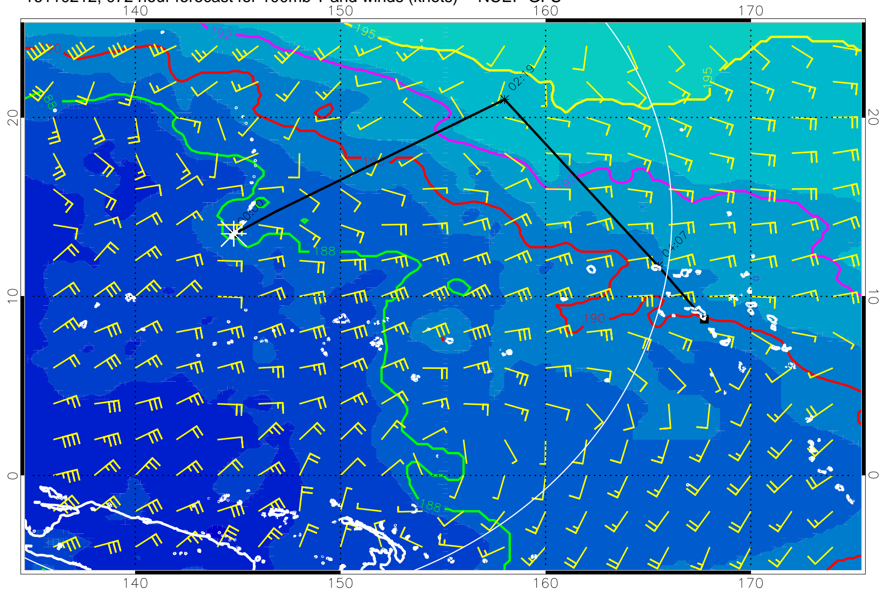
16110212, 072 hour forecast for 100mb T and winds (knots) -- NCEP GFS
