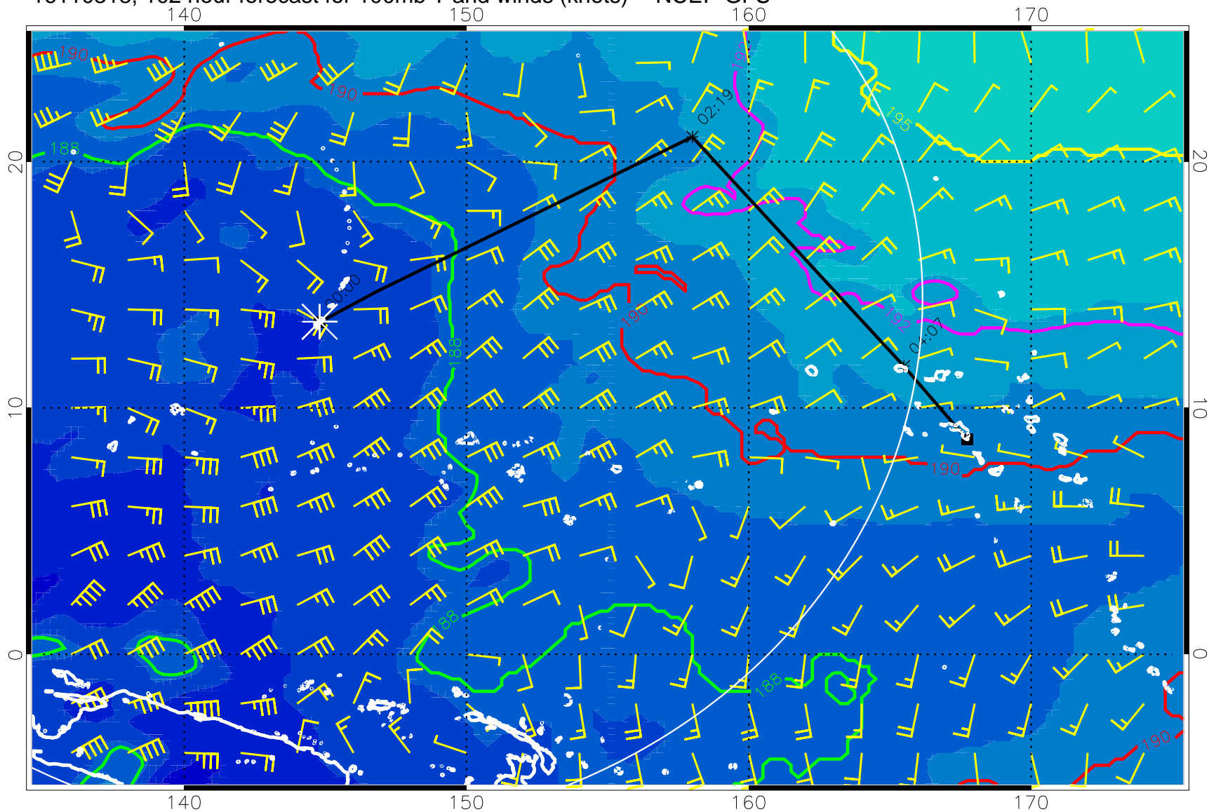
16110318, 102 hour forecast for 100mb T and winds (knots) -- NCEP GFS
