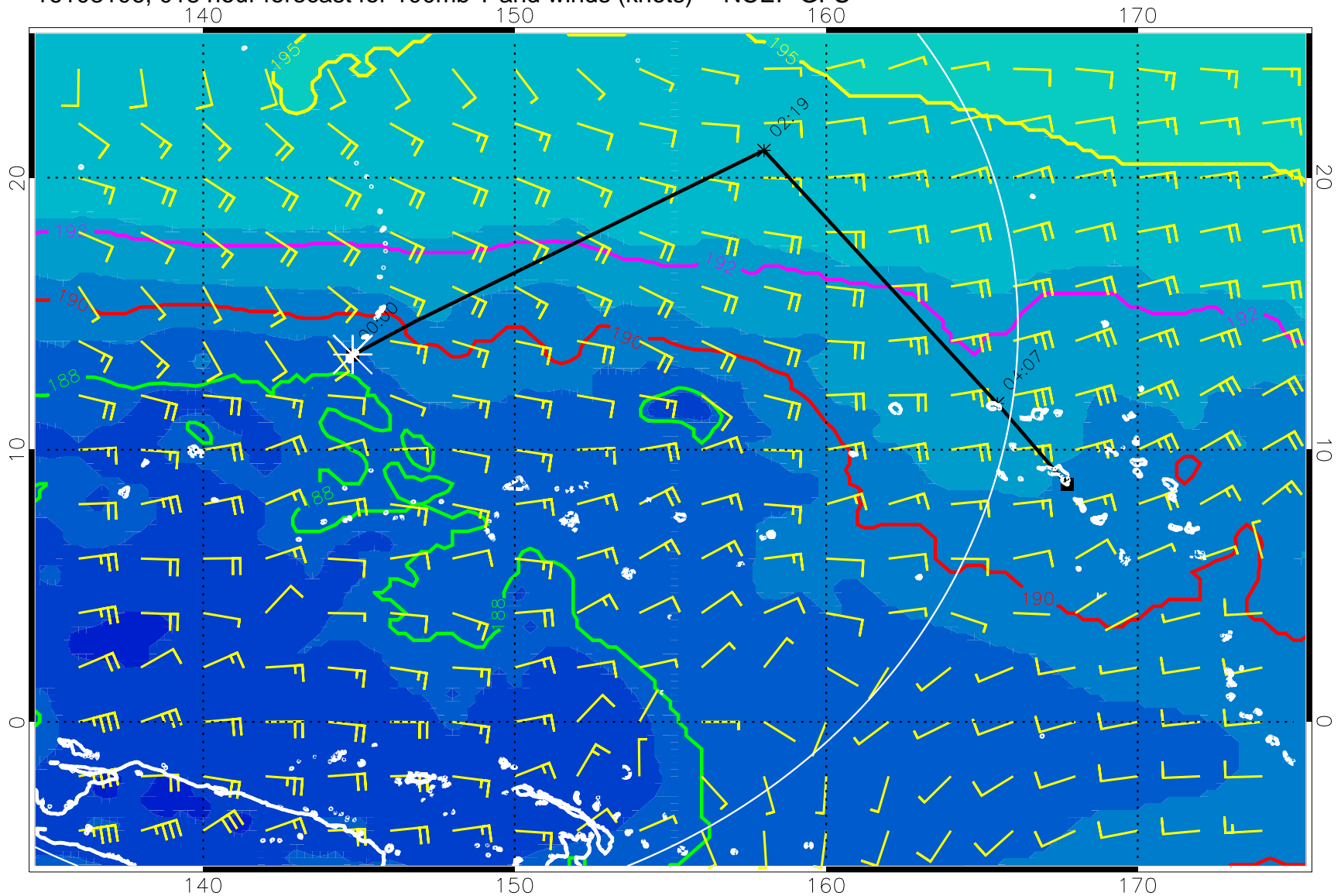
16103106, 018 hour forecast for 100mb T and winds (knots) -- NCEP GFS
