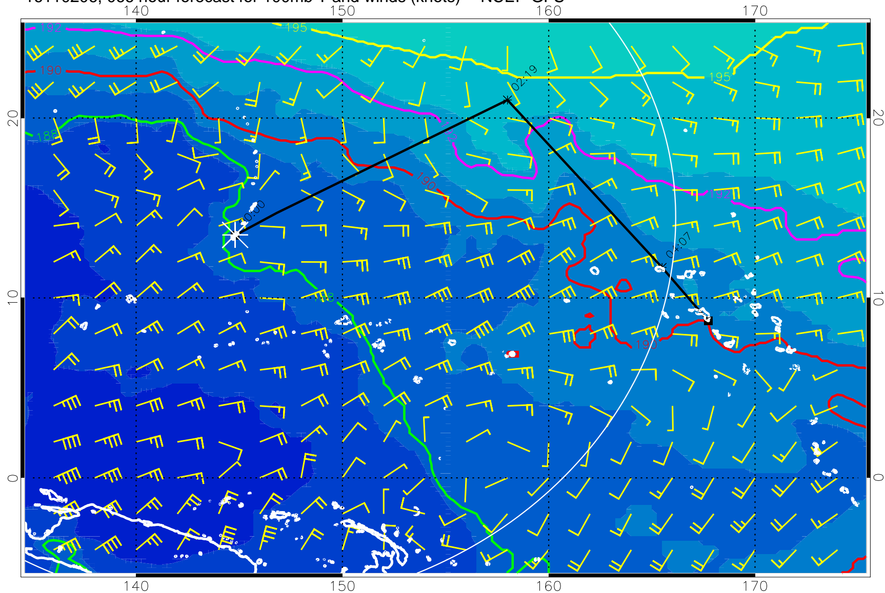
16110206, 066 hour forecast for 100mb T and winds (knots) -- NCEP GFS
