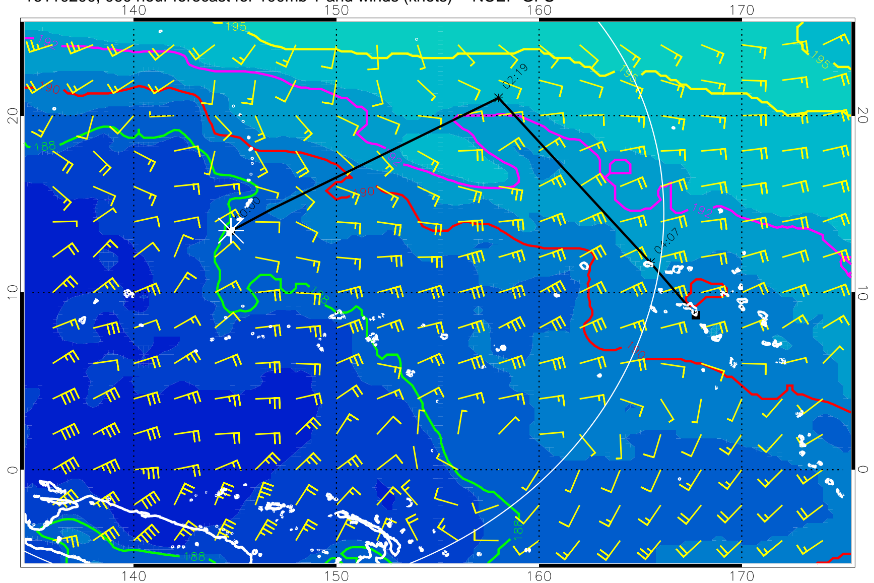
16110200, 060 hour forecast for 100mb T and winds (knots) -- NCEP GFS
