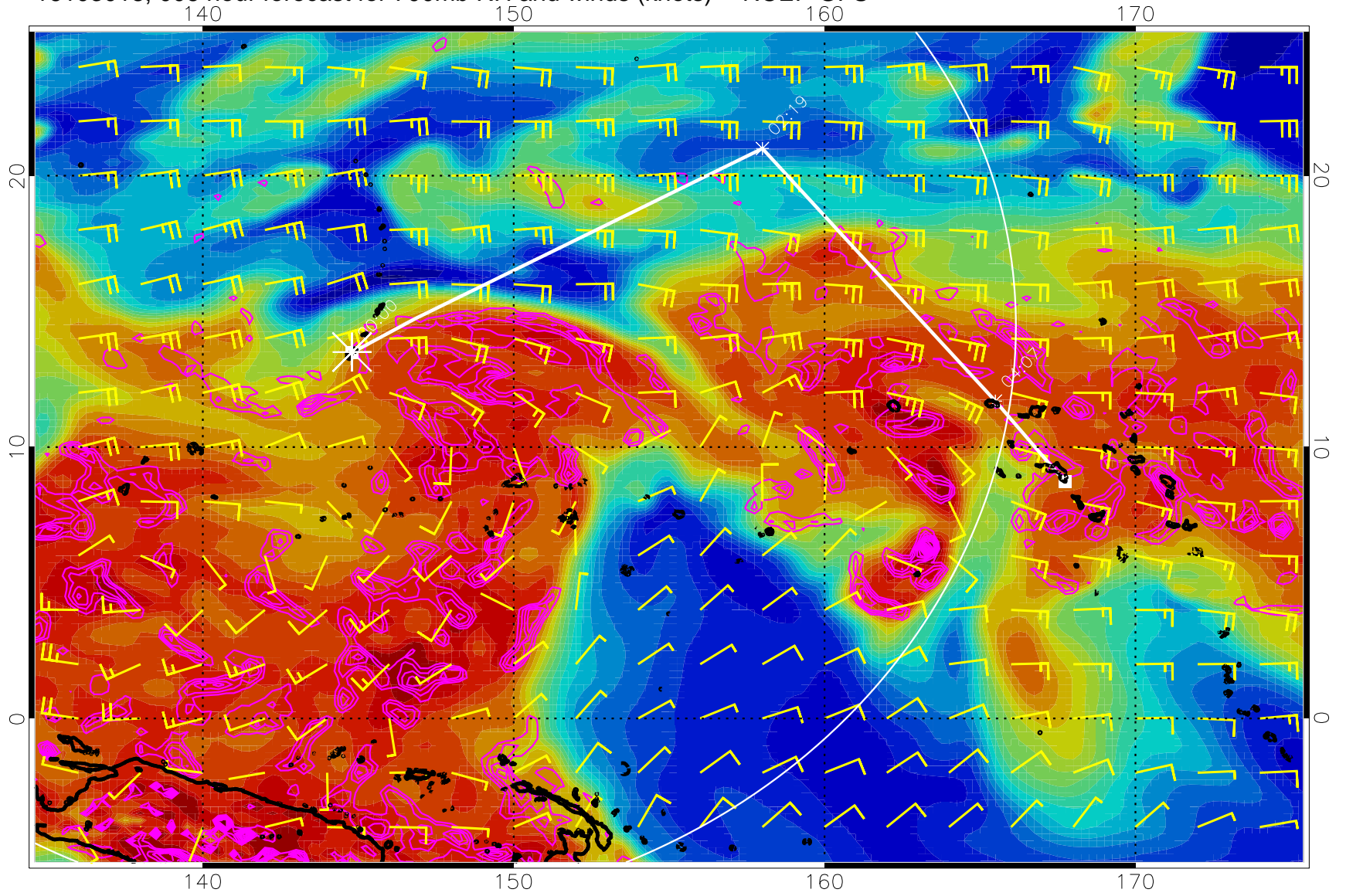
16103018, 006 hour forecast for 700mb RH and winds (knots) -- NCEP GFS
