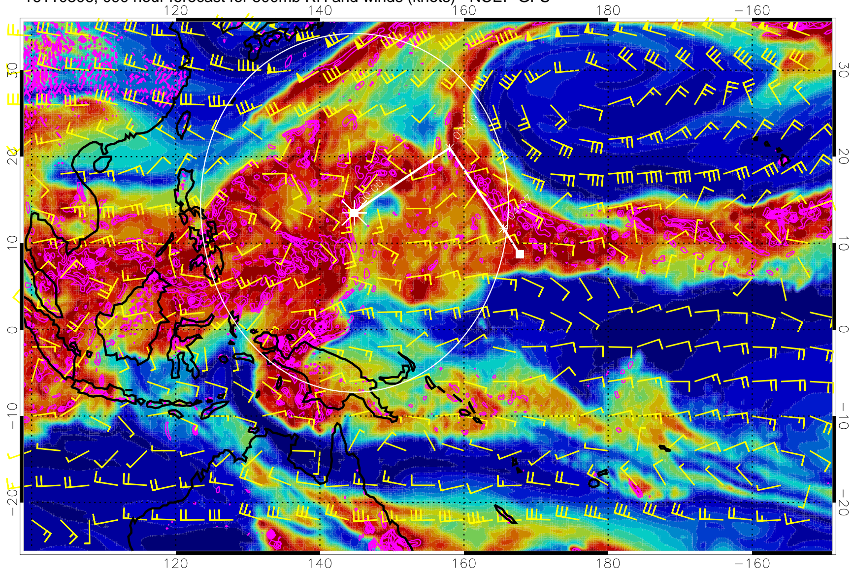
16110306, 090 hour forecast for 500mb RH and winds (knots) - NCEP GFS
