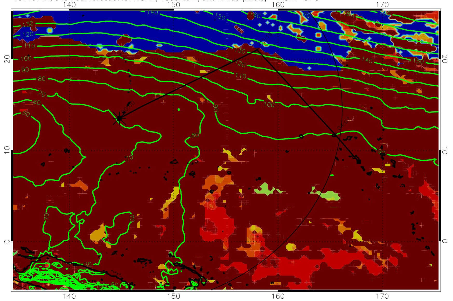
16110112, 048 hour forecast for HCAL, 1000mb Z, and winds (knots) -- NCEP GFS
