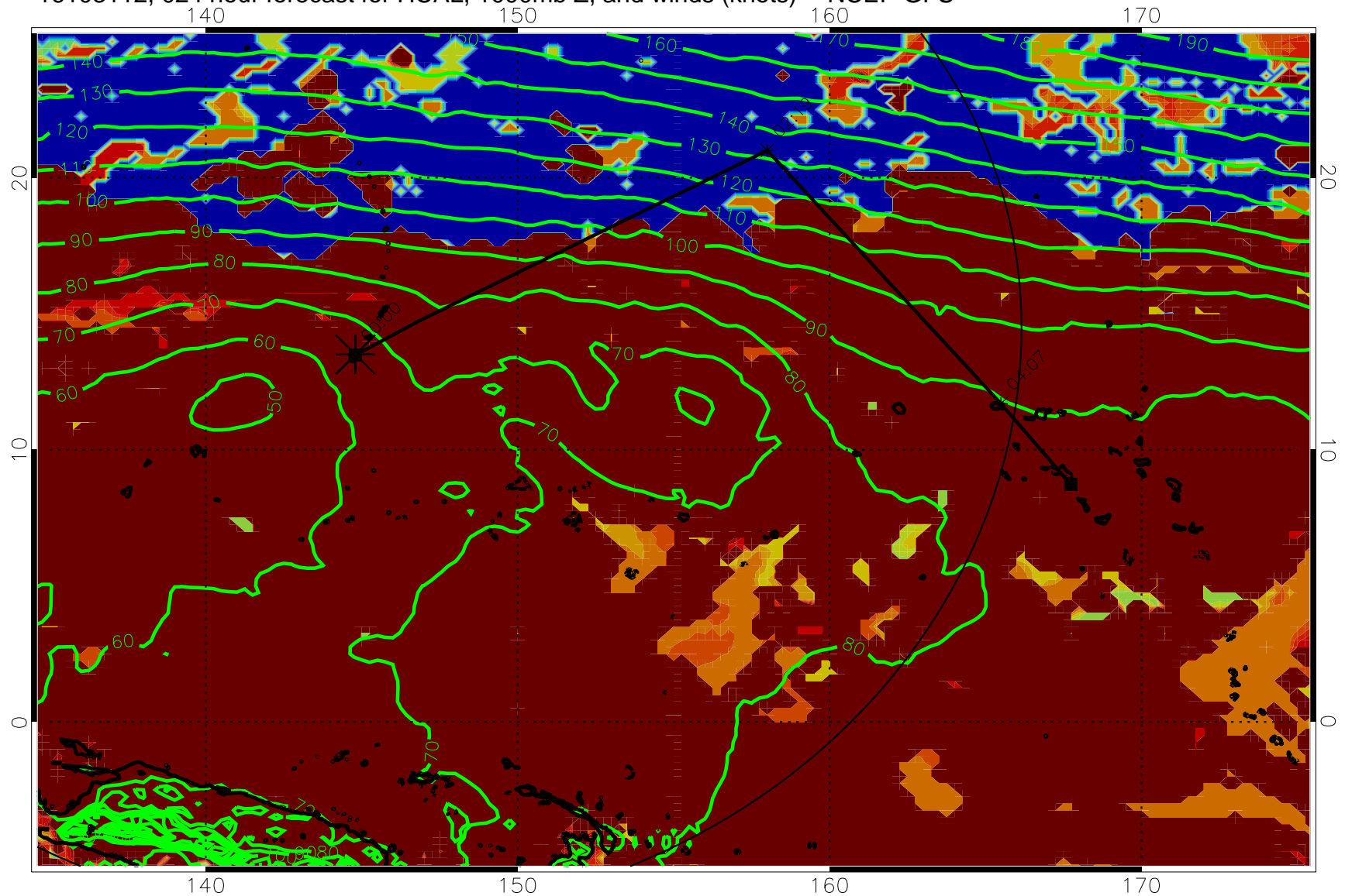
16103112, 024 hour forecast for HCAL, 1000mb Z, and winds (knots) -- NCEP GFS
