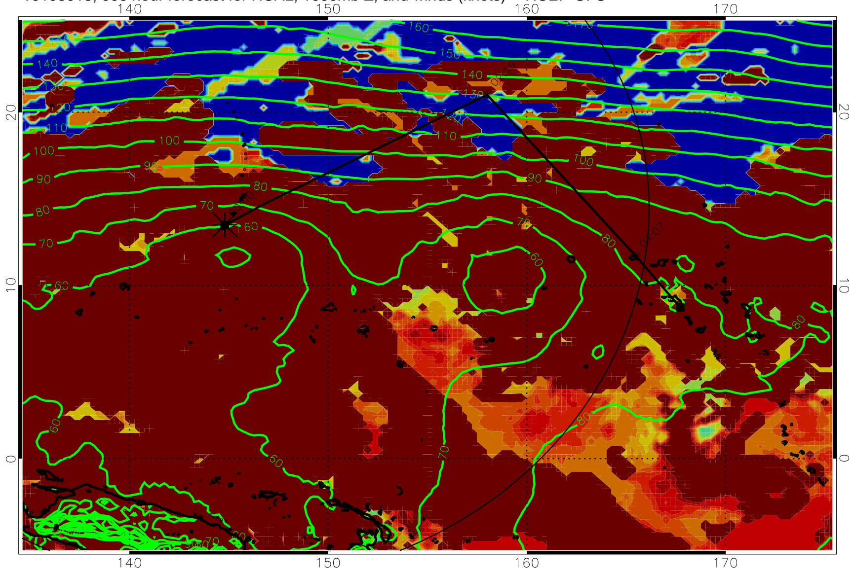
16103018, 006 hour forecast for HCAL, 1000mb Z, and winds (knots) -- NCEP GFS
