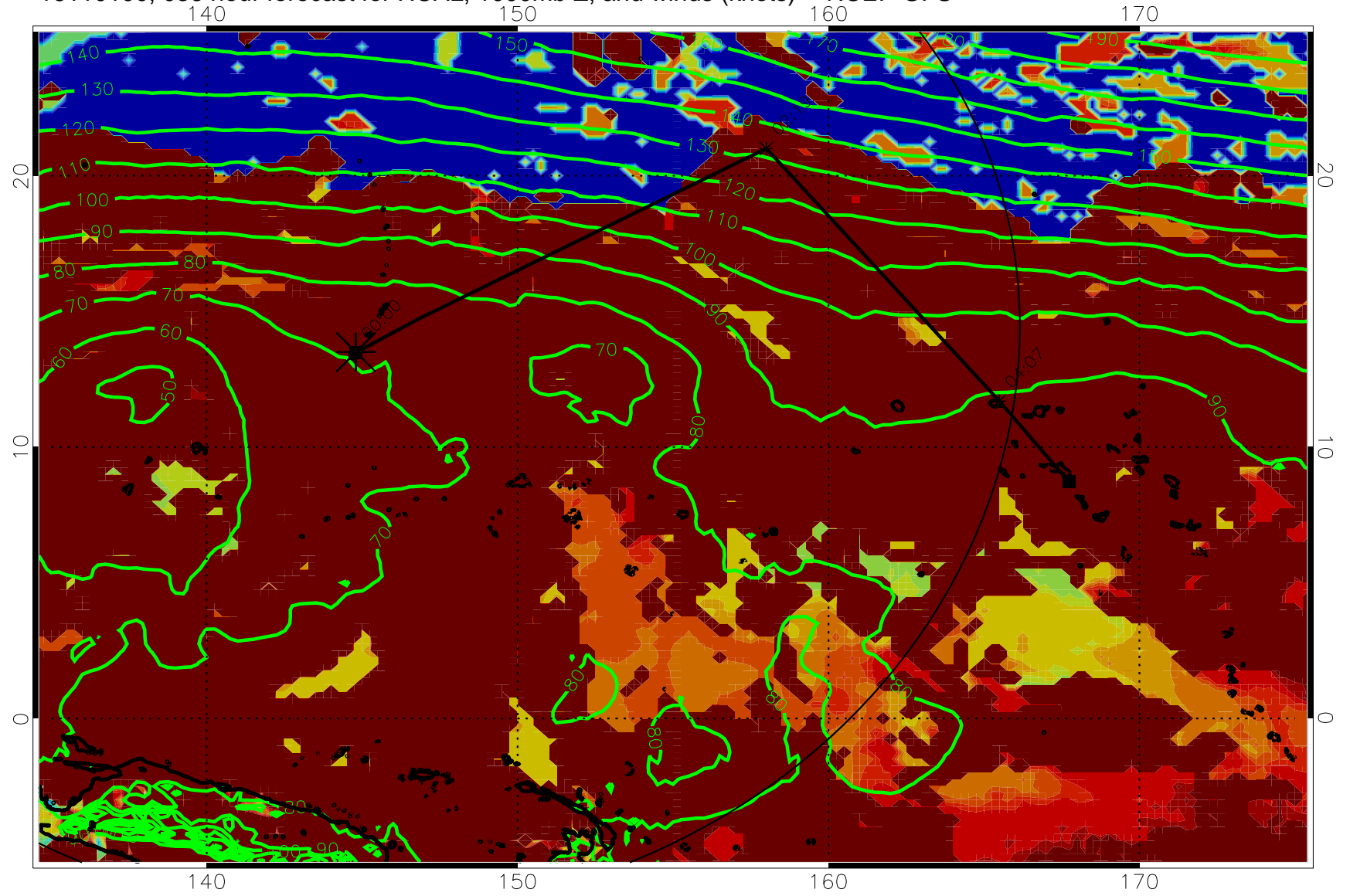
16110100, 036 hour forecast for HCAL, 1000mb Z, and winds (knots) -- NCEP GFS
