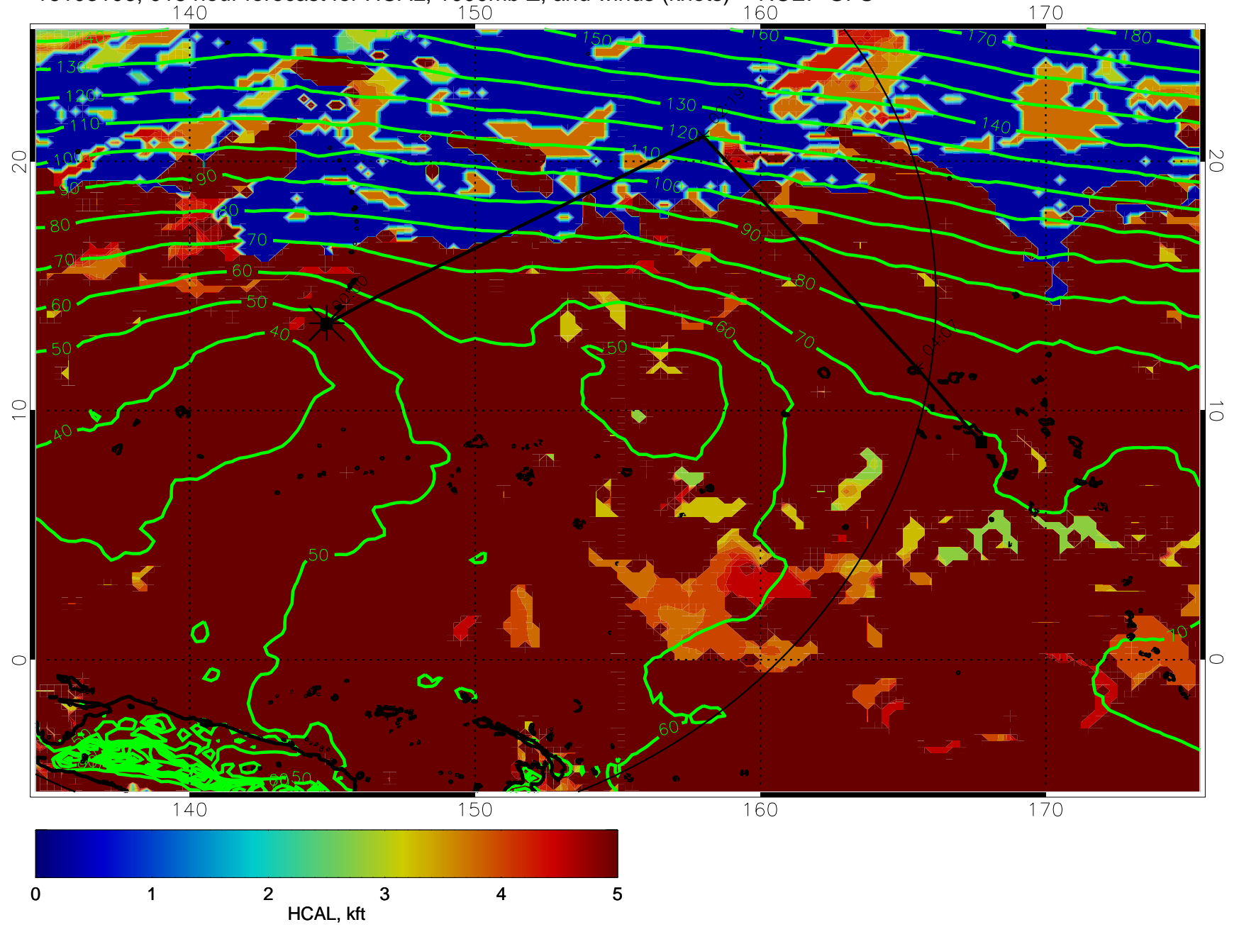
16103106, 018 hour forecast for HCAL, 1000mb Z, and winds (knots) -- NCEP GFS
