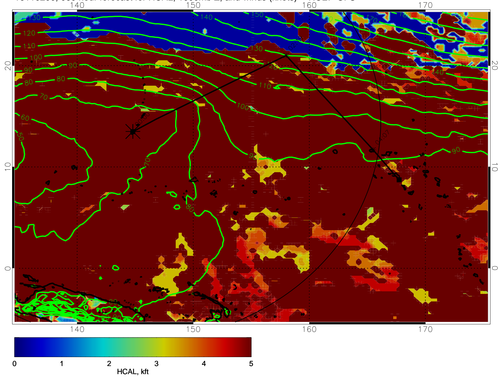
16110200, 060 hour forecast for HCAL, 1000mb Z, and winds (knots) -- NCEP GFS
