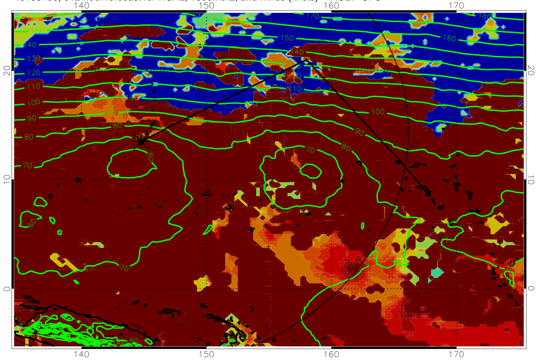
16103100, 012 hour forecast for HCAL, 1000mb Z, and winds (knots) -- NCEP GFS
