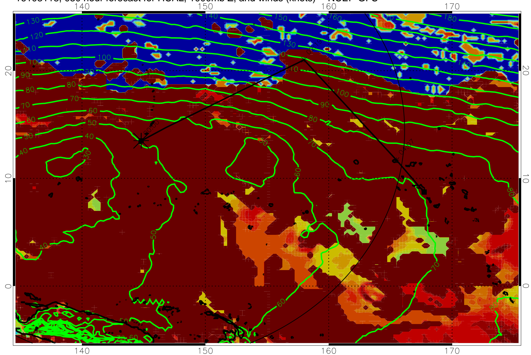
16103118, 030 hour forecast for HCAL, 1000mb Z, and winds (knots) -- NCEP GFS
