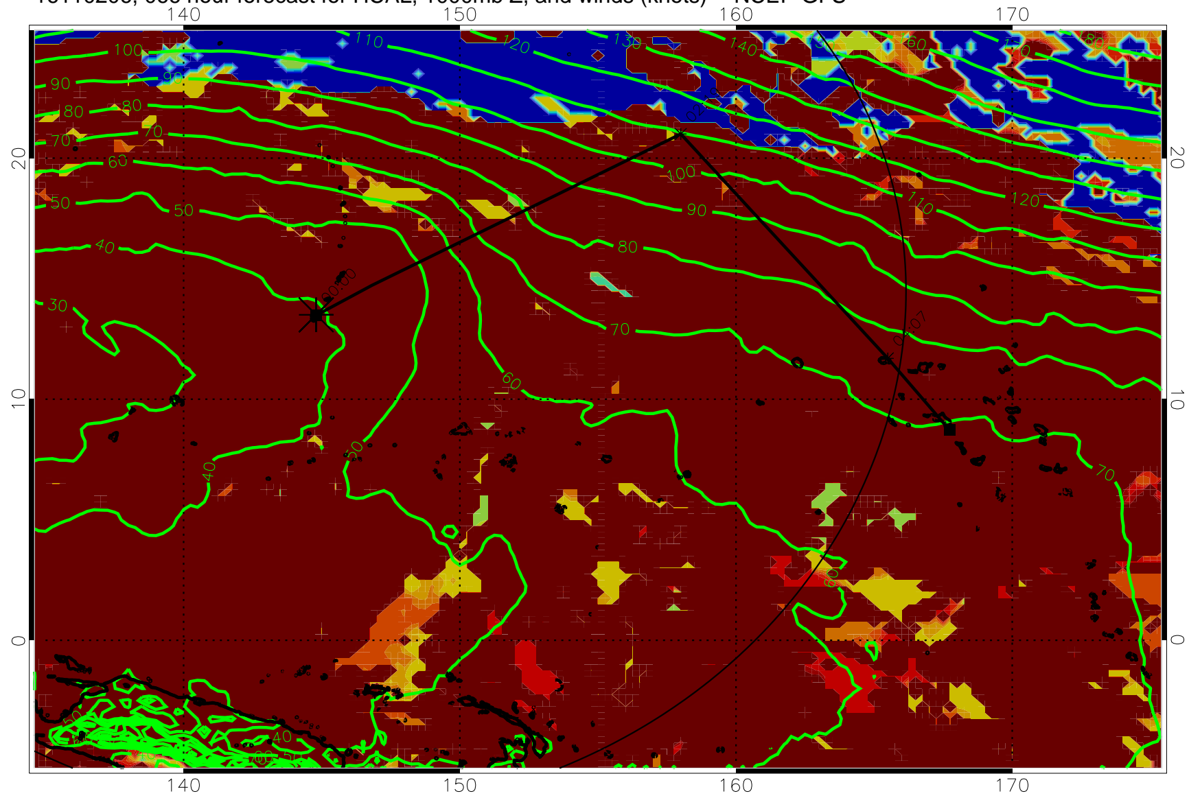
16110206, 066 hour forecast for HCAL, 1000mb Z, and winds (knots) -- NCEP GFS
