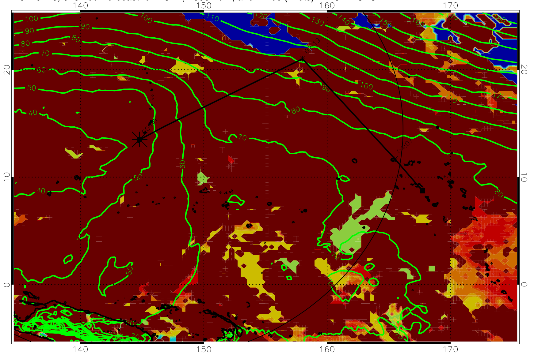
16110218, 078 hour forecast for HCAL, 1000mb Z, and winds (knots) -- NCEP GFS
