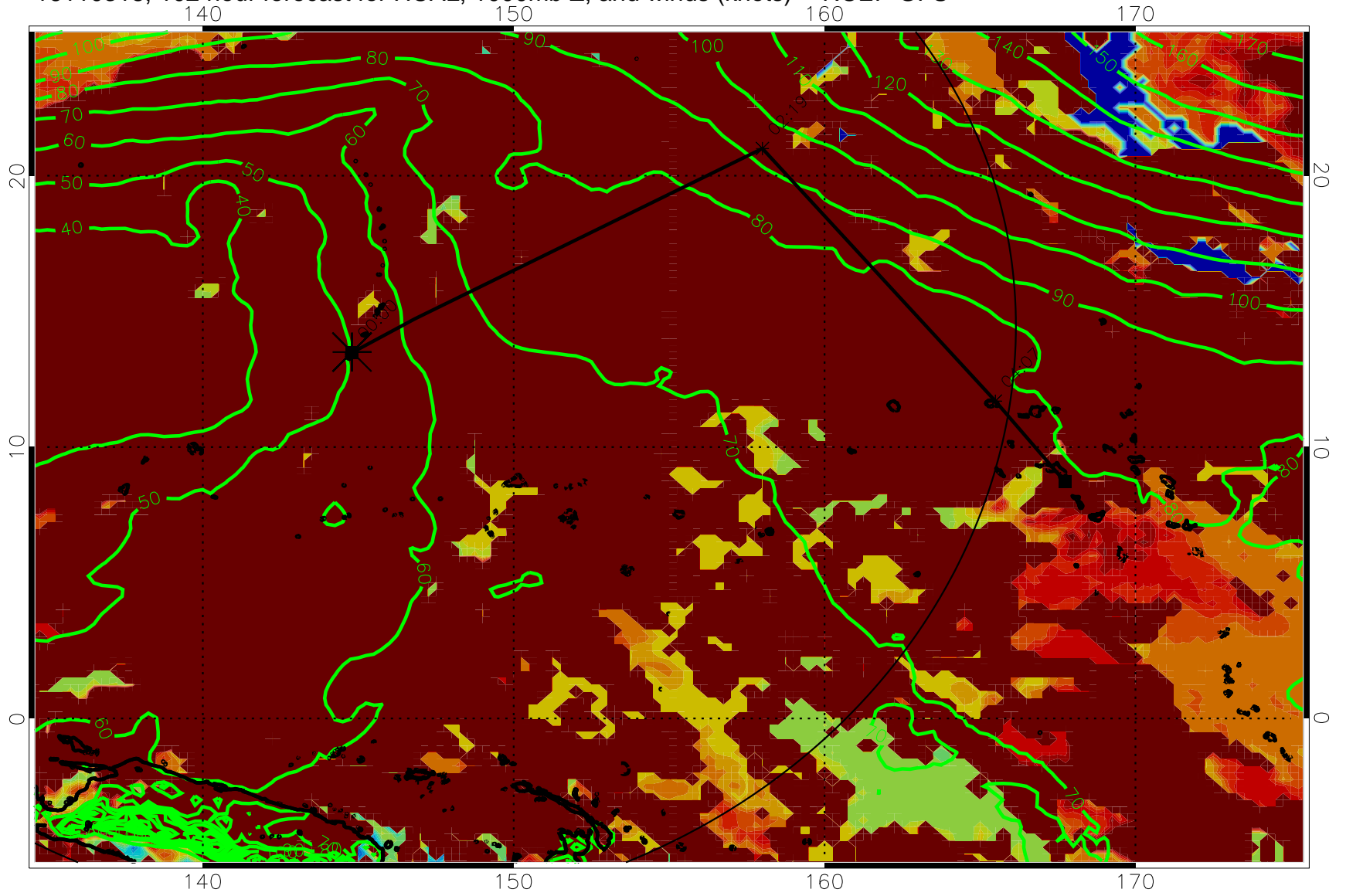
16110318, 102 hour forecast for HCAL, 1000mb Z, and winds (knots) -- NCEP GFS
