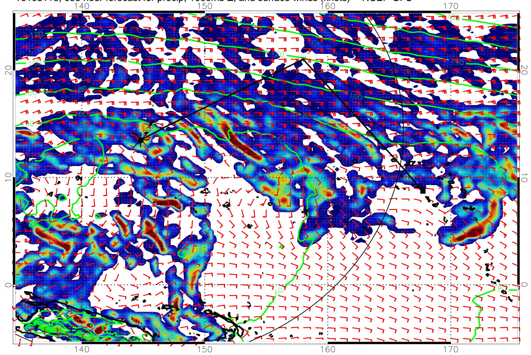
16103118, 036 hour forecast for precip, 1000mb Z, and surface winds (knots) -- NCEP GFS
