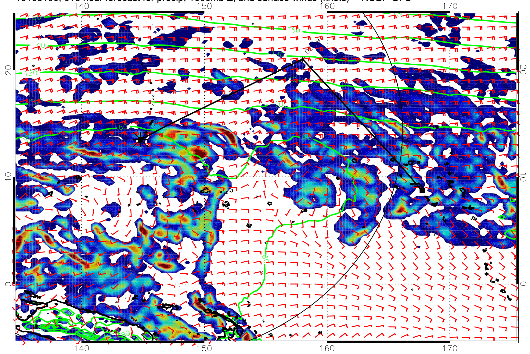
16103100, 018 hour forecast for precip, 1000mb Z, and surface winds (knots) -- NCEP GFS
