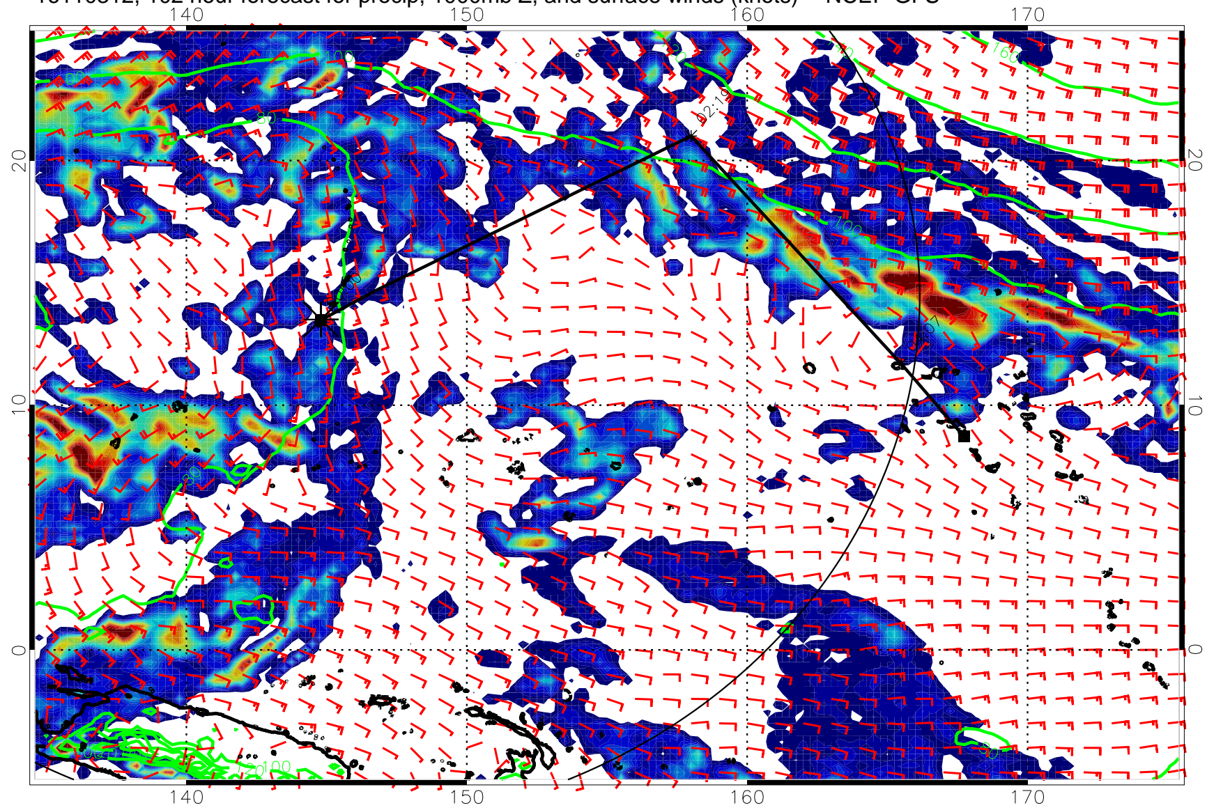
16110312, 102 hour forecast for precip, 1000mb Z, and surface winds (knots) -- NCEP GFS
