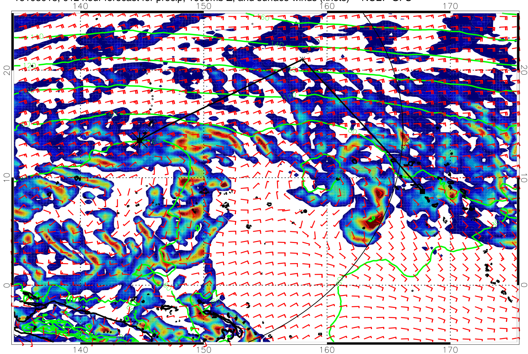
16103018, 012 hour forecast for precip, 1000mb Z, and surface winds (knots) -- NCEP GFS
