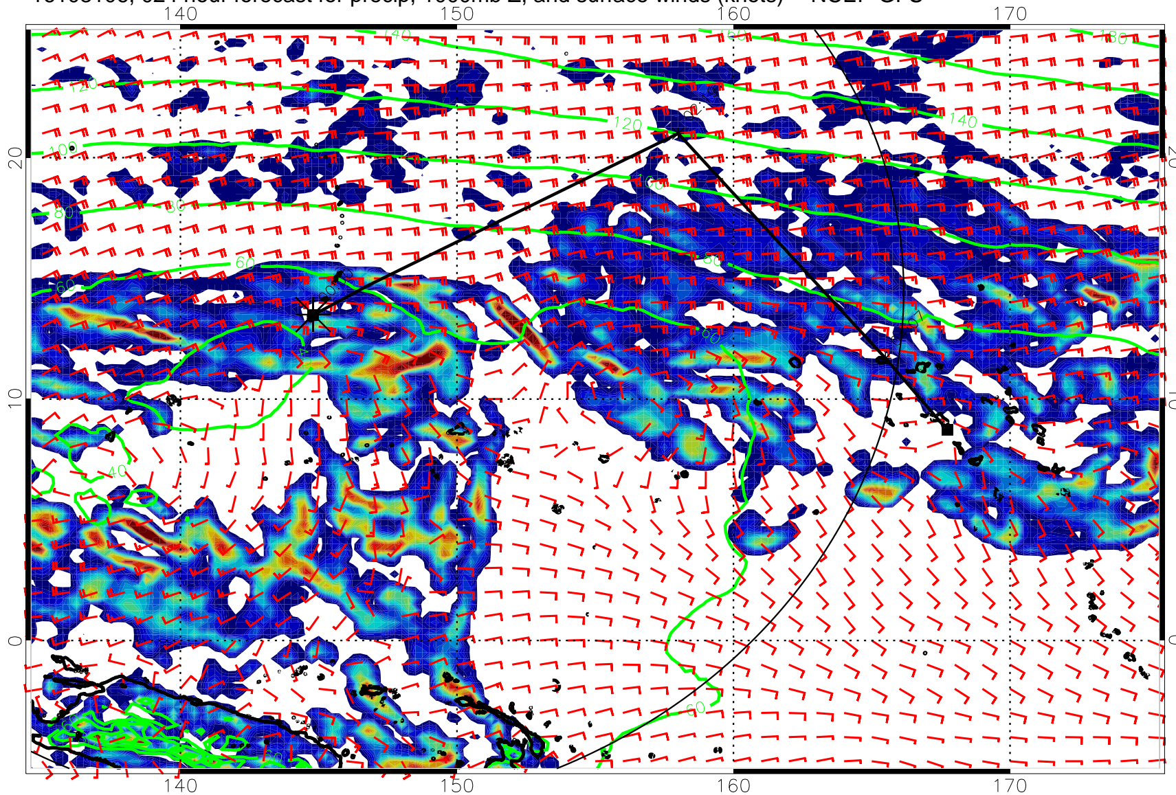
16103106, 024 hour forecast for precip, 1000mb Z, and surface winds (knots) -- NCEP GFS
