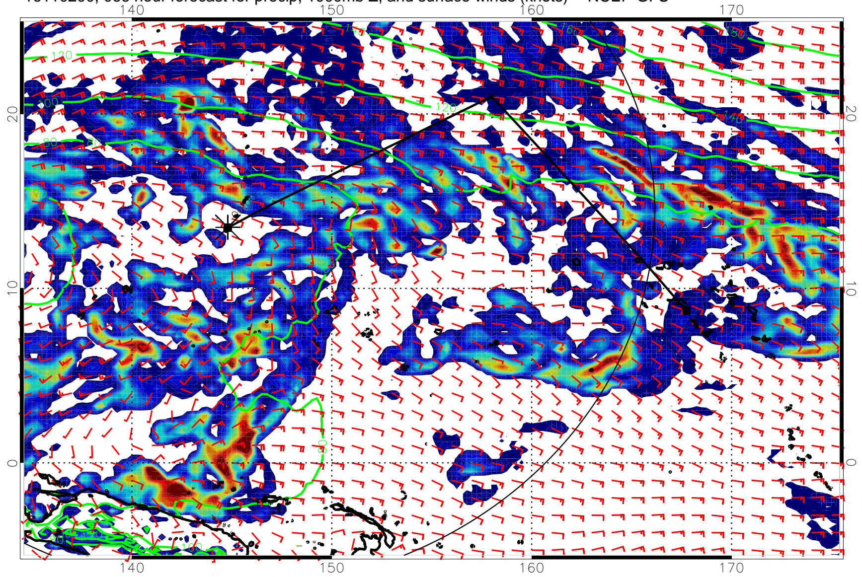
16110200, 066 hour forecast for precip, 1000mb Z, and surface winds (knots) -- NCEP GFS
