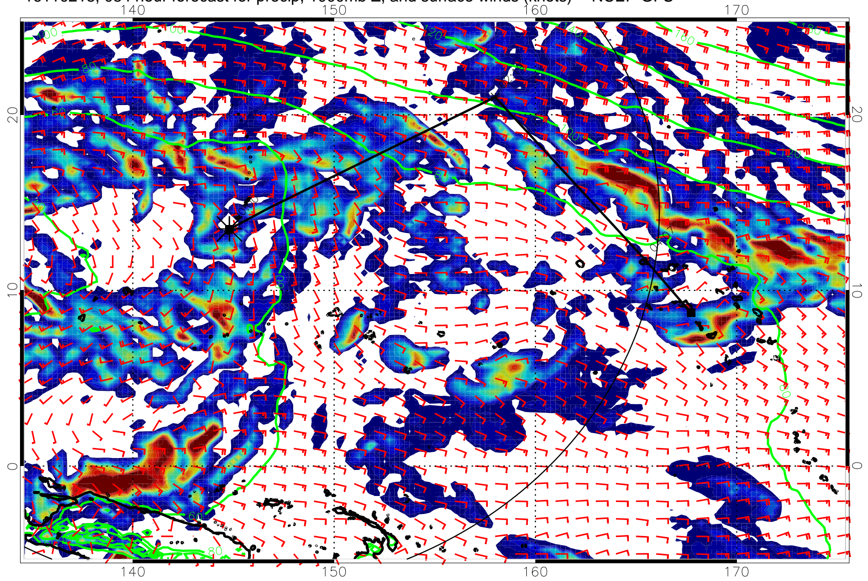
16110218, 084 hour forecast for precip, 1000mb Z, and surface winds (knots) -- NCEP GFS
