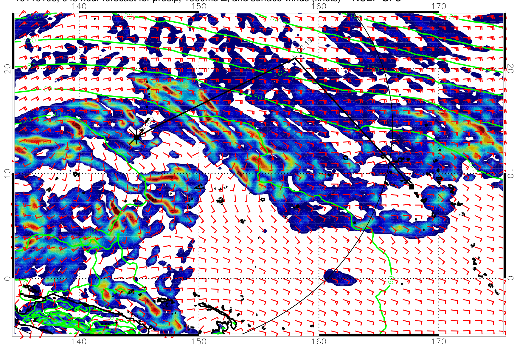
16110106, 048 hour forecast for precip, 1000mb Z, and surface winds (knots) -- NCEP GFS
