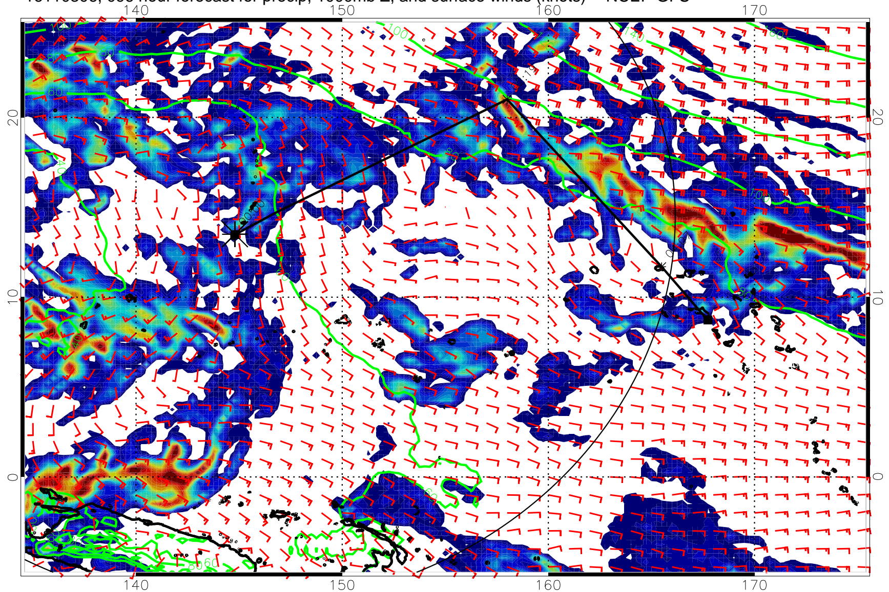
16110306, 096 hour forecast for precip, 1000mb Z, and surface winds (knots) -- NCEP GFS
