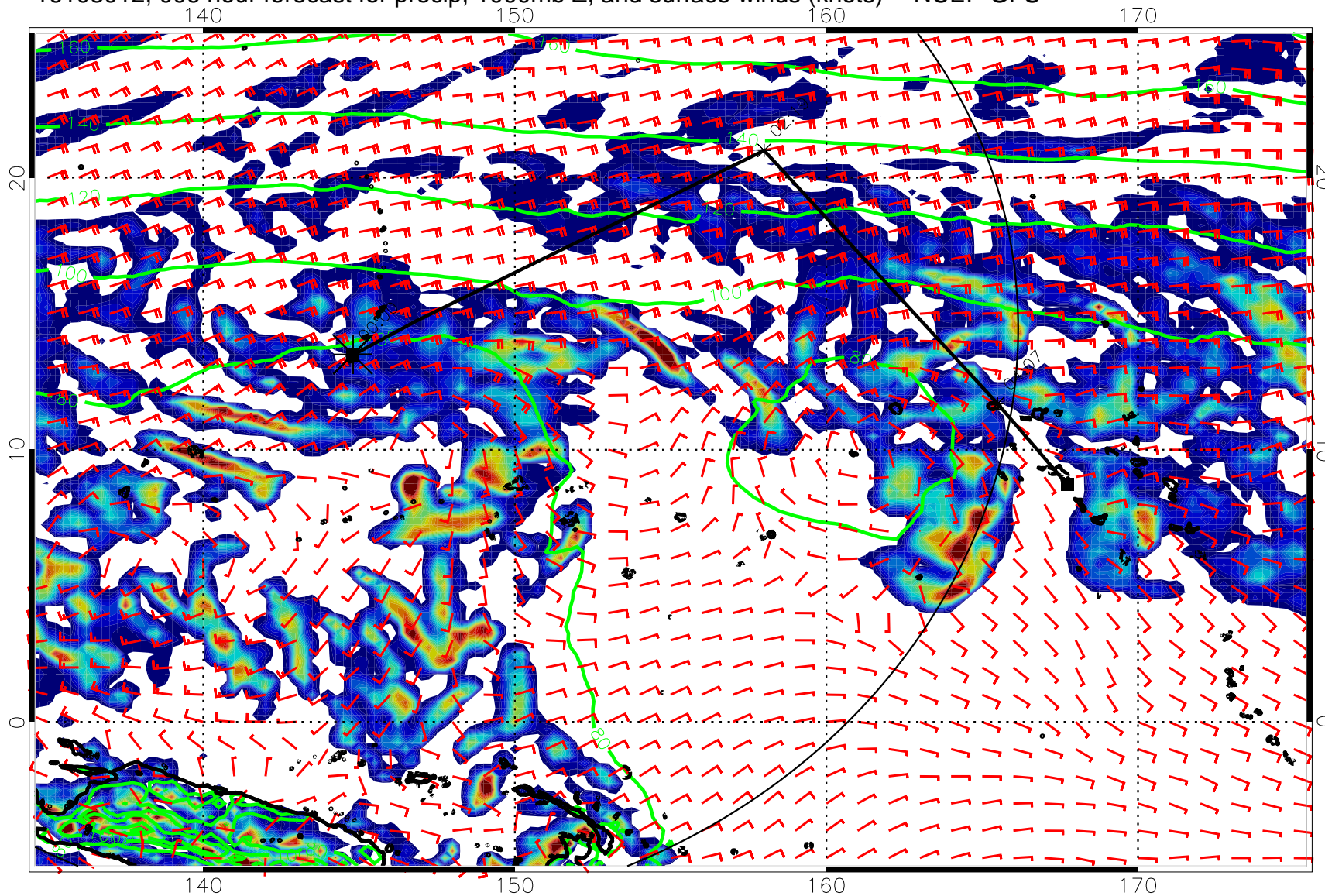
16103012, 006 hour forecast for precip, 1000mb Z, and surface winds (knots) -- NCEP GFS
