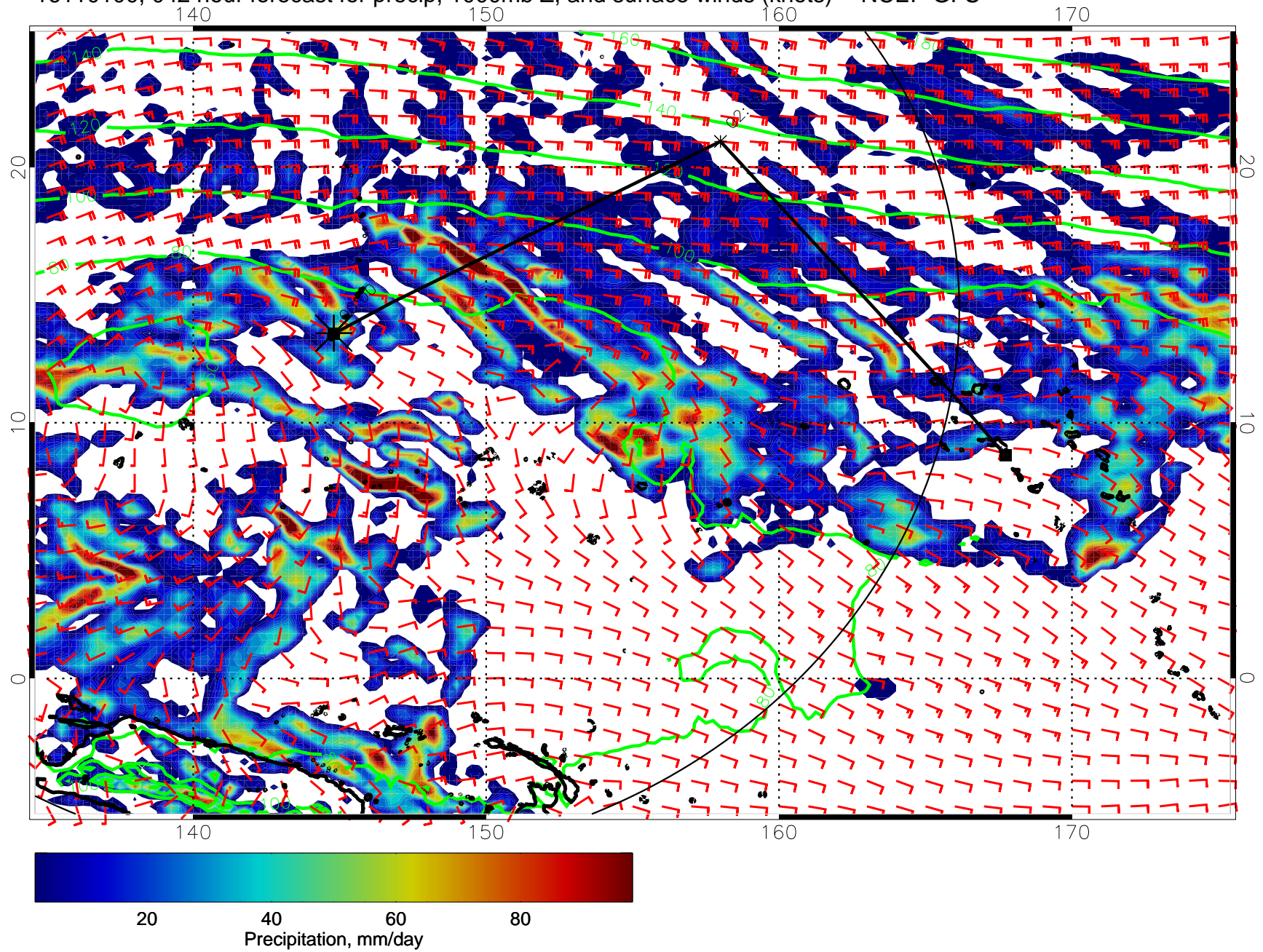
16110100, 042 hour forecast for precip, 1000mb Z, and surface winds (knots) -- NCEP GFS
