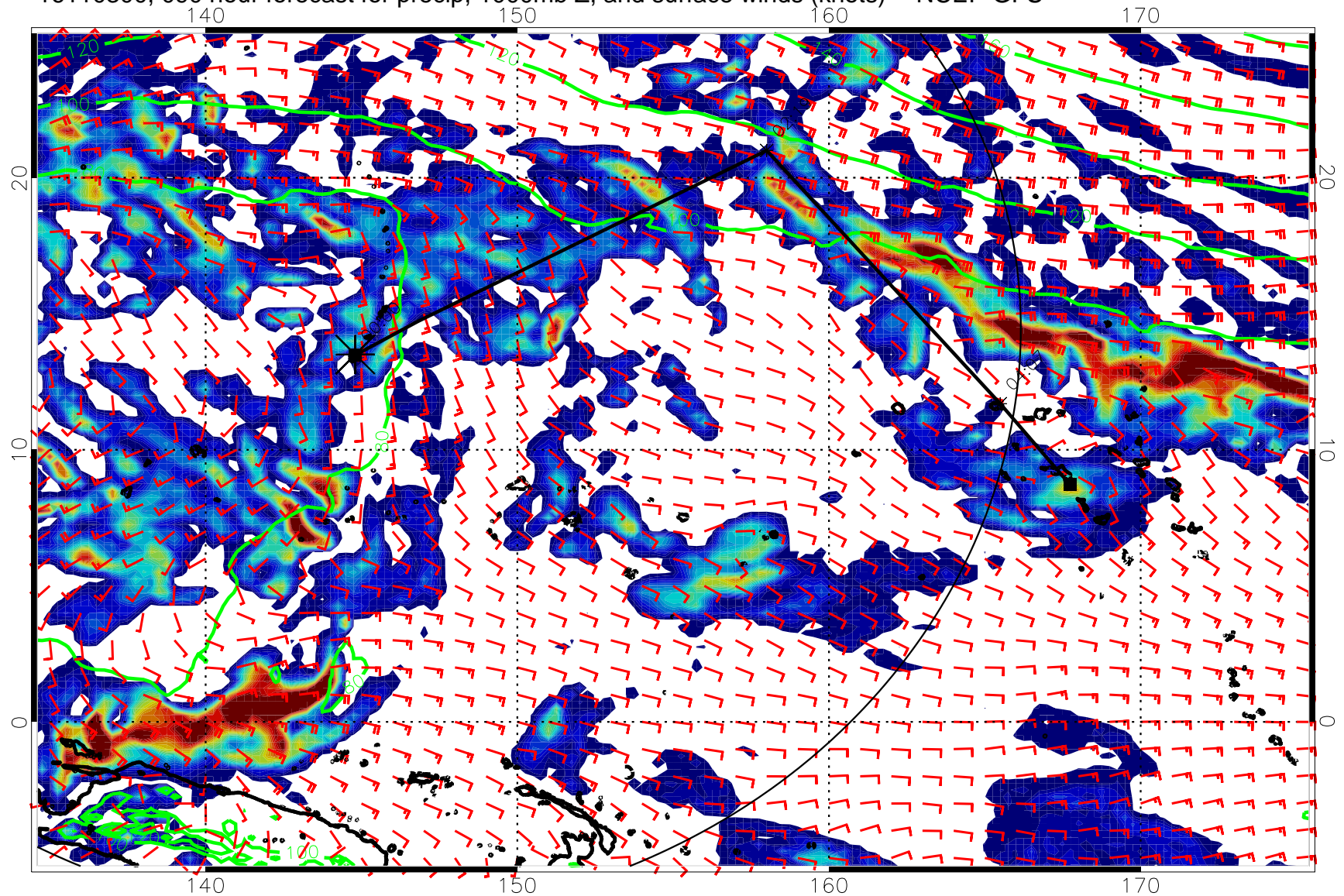
16110300, 090 hour forecast for precip, 1000mb Z, and surface winds (knots) -- NCEP GFS
