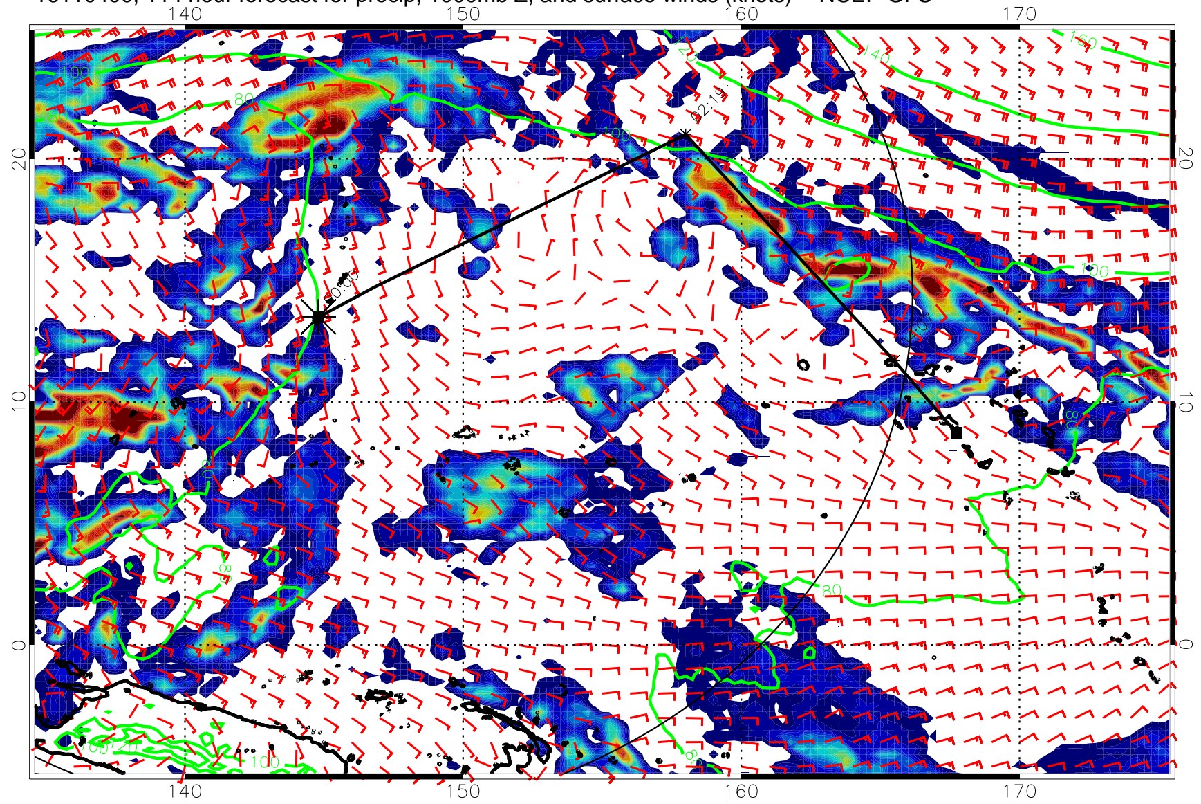
16110400, 114 hour forecast for precip, 1000mb Z, and surface winds (knots) -- NCEP GFS
