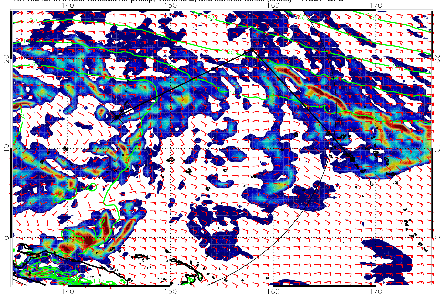
16110212, 078 hour forecast for precip, 1000mb Z, and surface winds (knots) -- NCEP GFS
