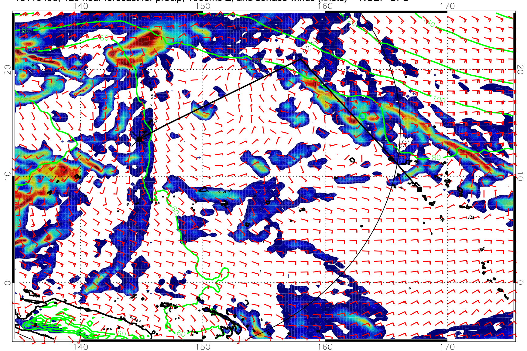
16110406, 120 hour forecast for precip, 1000mb Z, and surface winds (knots) -- NCEP GFS
