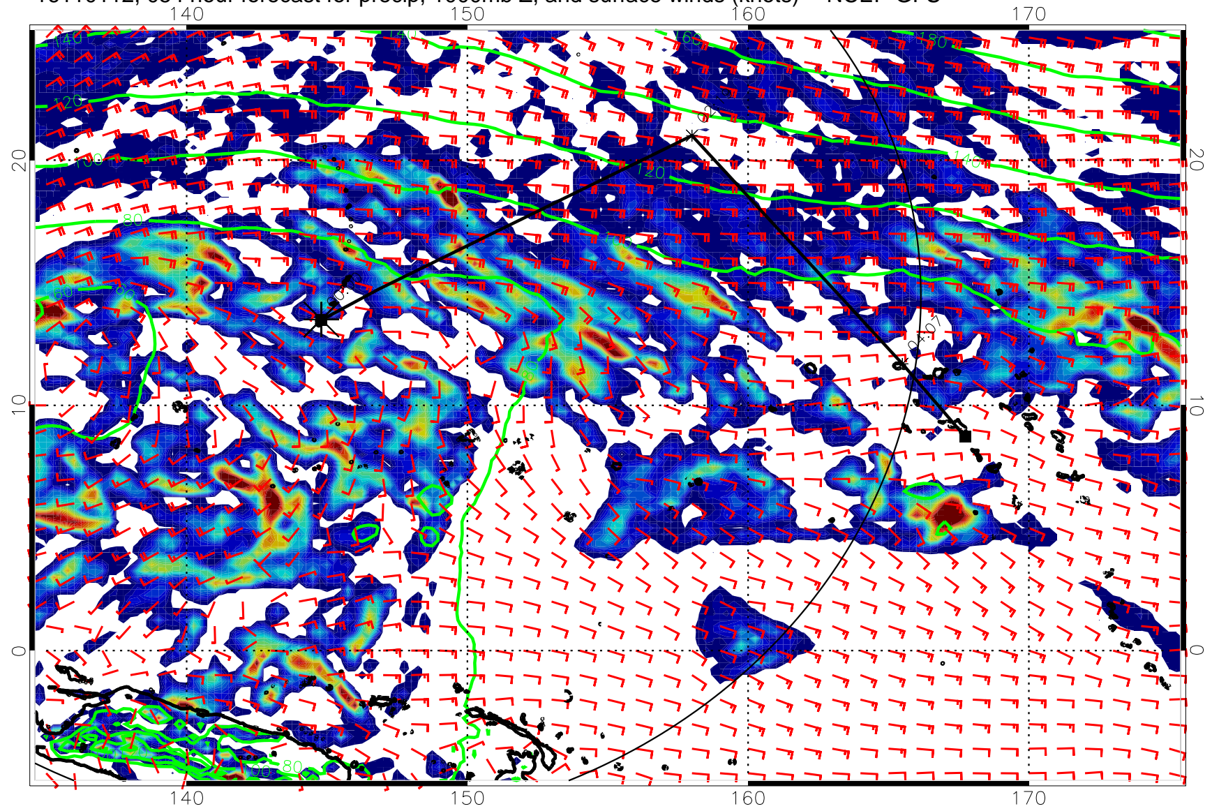
16110112, 054 hour forecast for precip, 1000mb Z, and surface winds (knots) -- NCEP GFS
