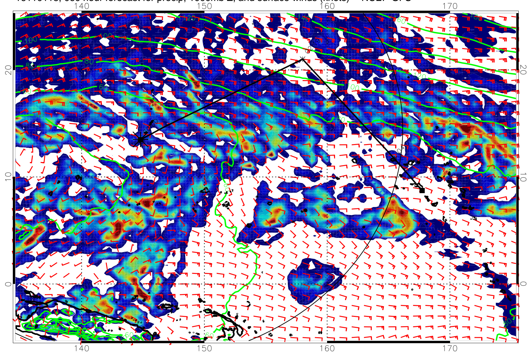
16110118, 060 hour forecast for precip, 1000mb Z, and surface winds (knots) -- NCEP GFS
