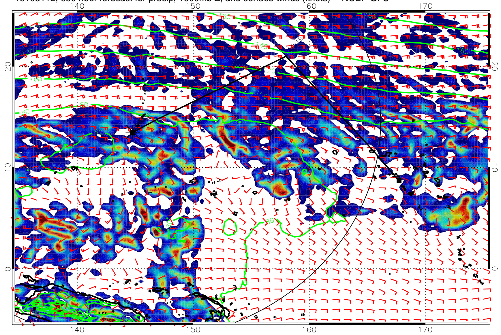
16103112, 030 hour forecast for precip, 1000mb Z, and surface winds (knots) -- NCEP GFS
