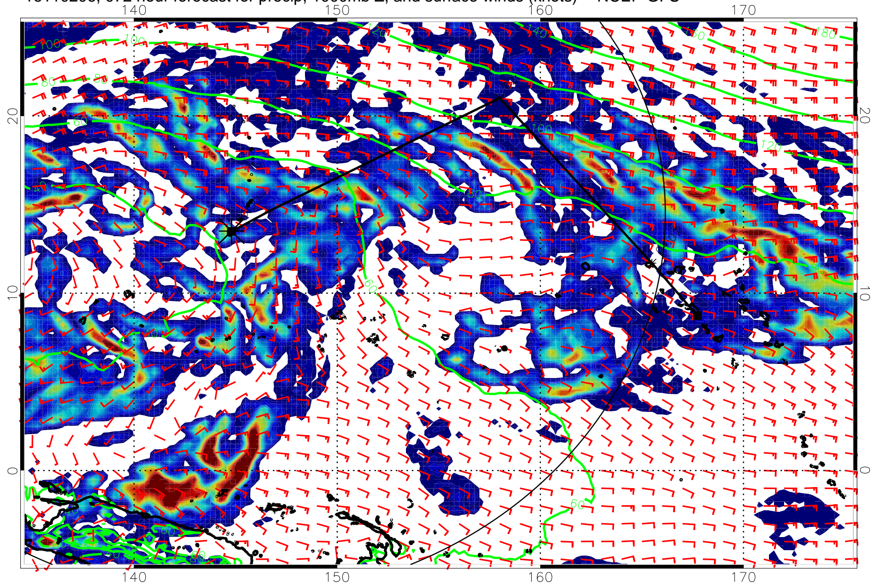
16110206, 072 hour forecast for precip, 1000mb Z, and surface winds (knots) -- NCEP GFS
