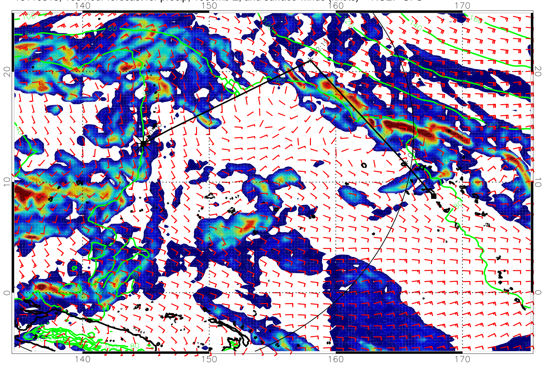
16110318, 108 hour forecast for precip, 1000mb Z, and surface winds (knots) -- NCEP GFS
