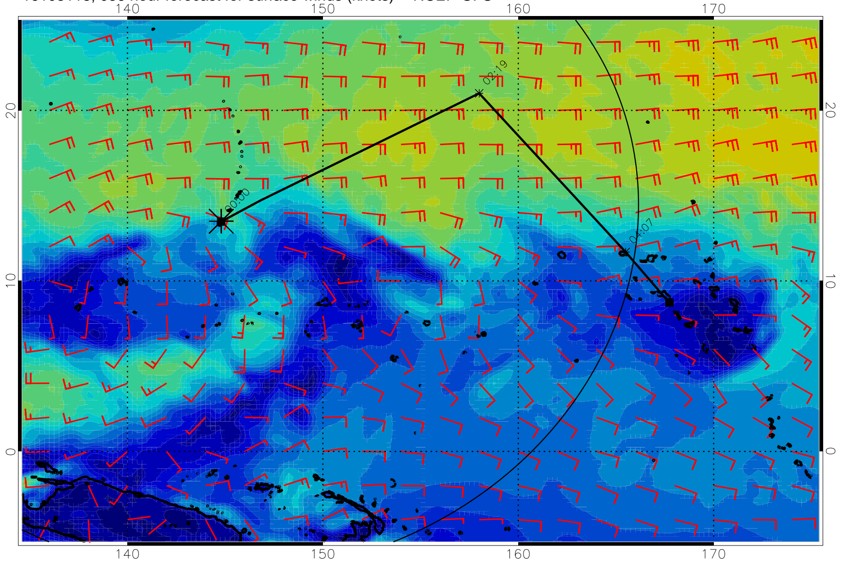
16103118, 036 hour forecast for surface winds (knots) -- NCEP GFS
