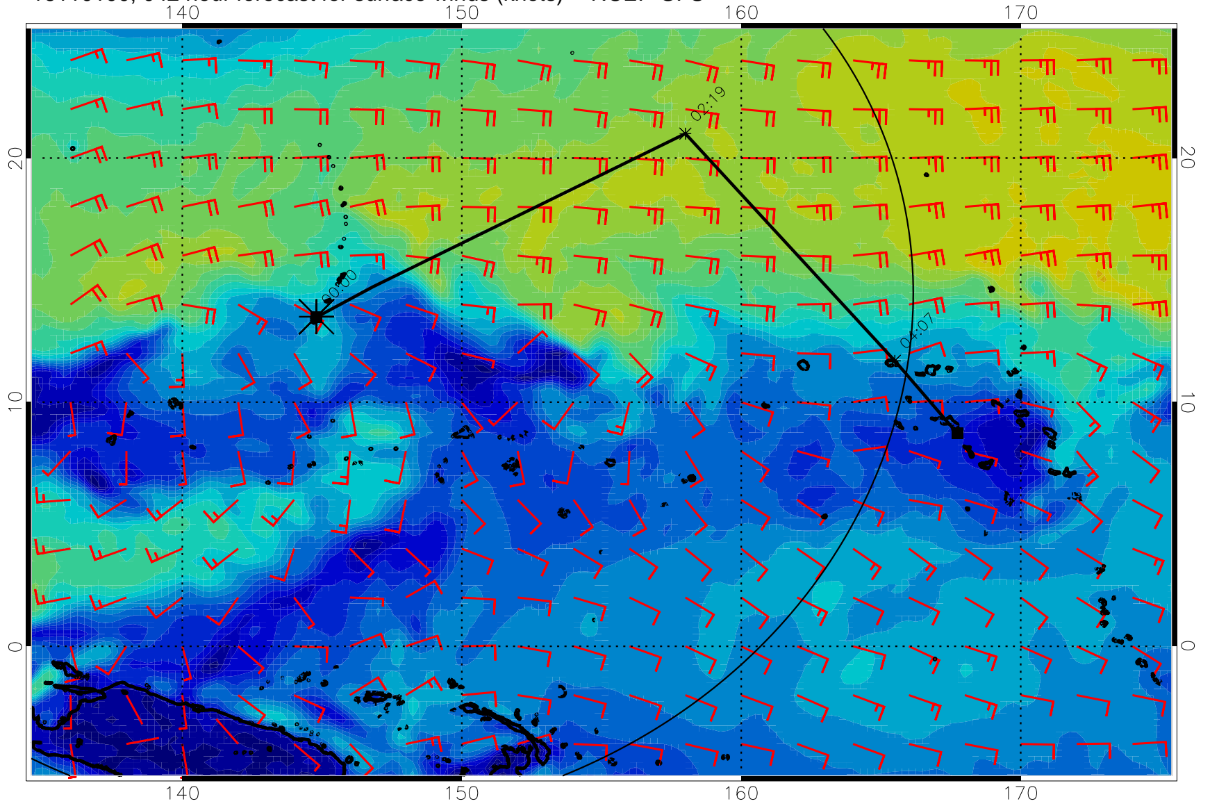
16110100, 042 hour forecast for surface winds (knots) -- NCEP GFS
