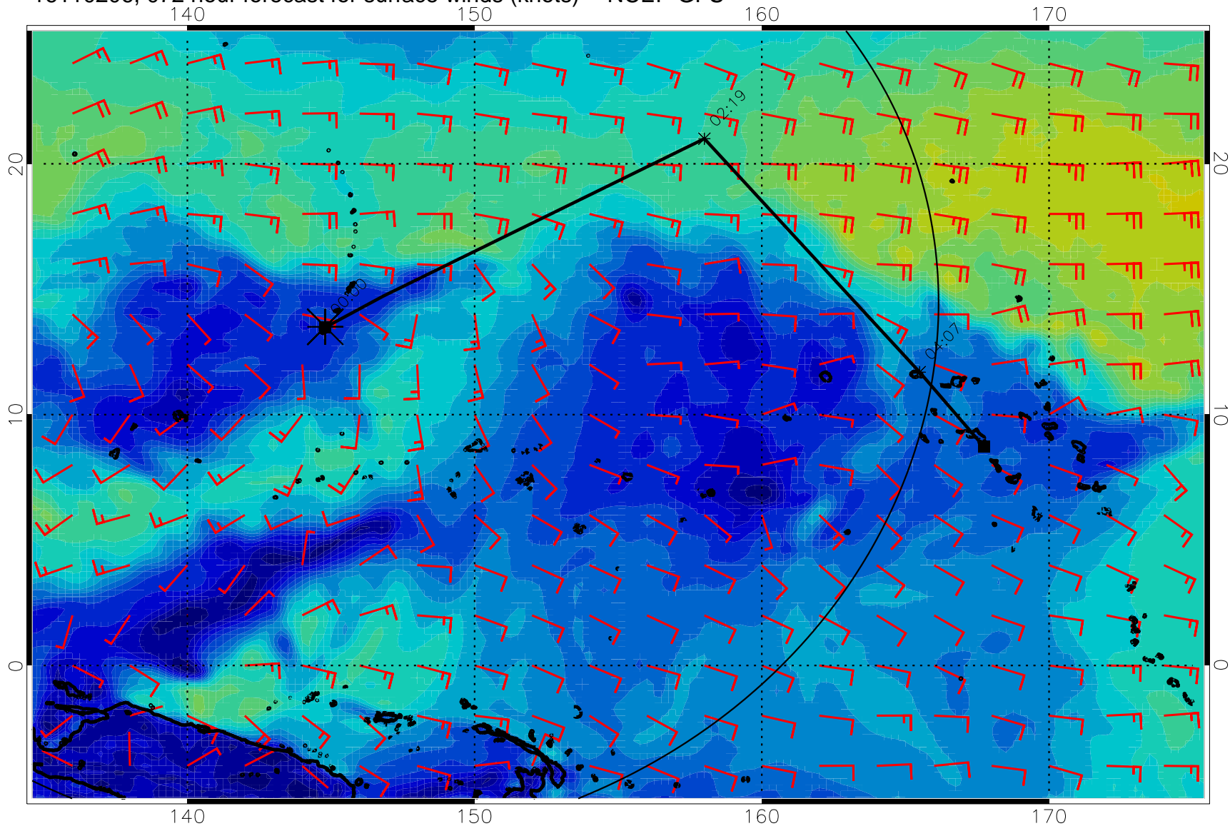
16110206, 072 hour forecast for surface winds (knots) -- NCEP GFS
