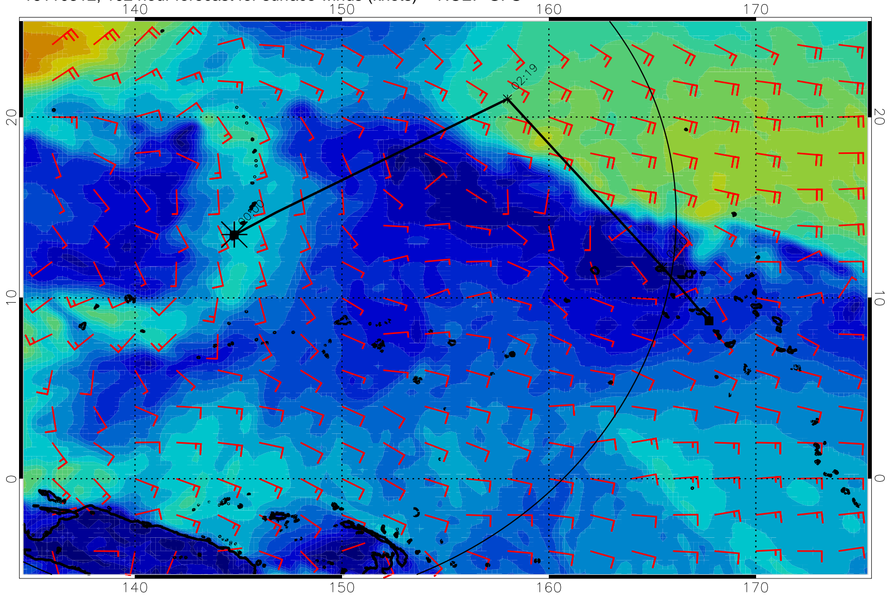
16110312, 102 hour forecast for surface winds (knots) -- NCEP GFS
