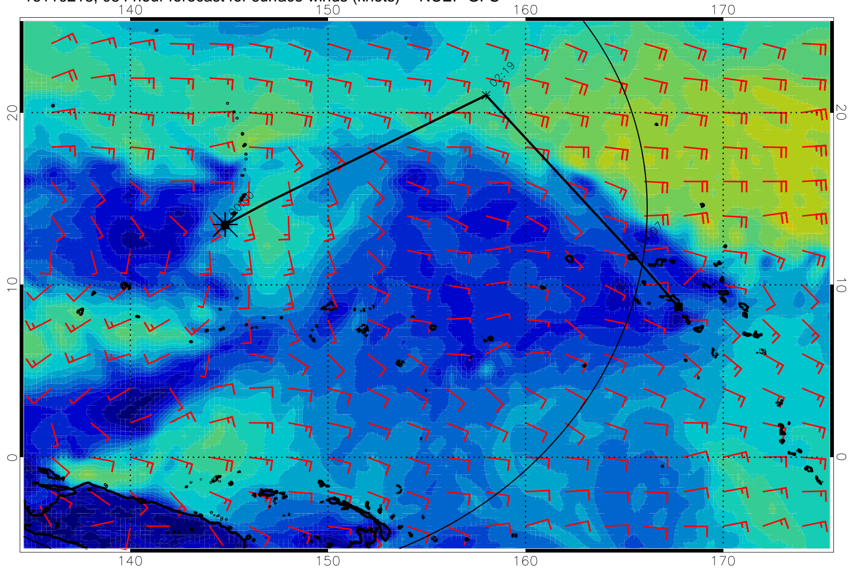
16110218, 084 hour forecast for surface winds (knots) -- NCEP GFS
