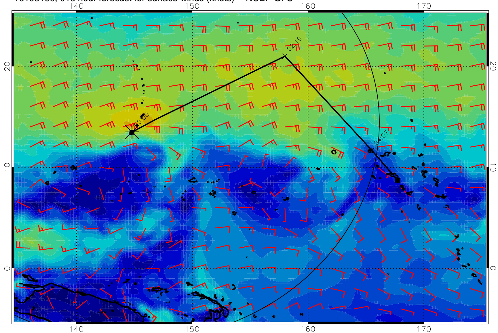
16103100, 018 hour forecast for surface winds (knots) -- NCEP GFS
