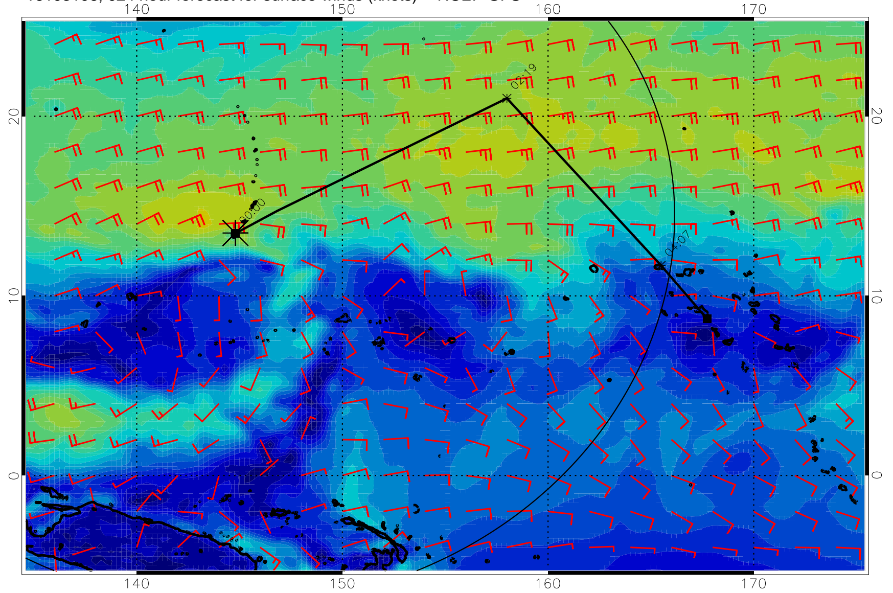
16103106, 024 hour forecast for surface winds (knots) -- NCEP GFS
