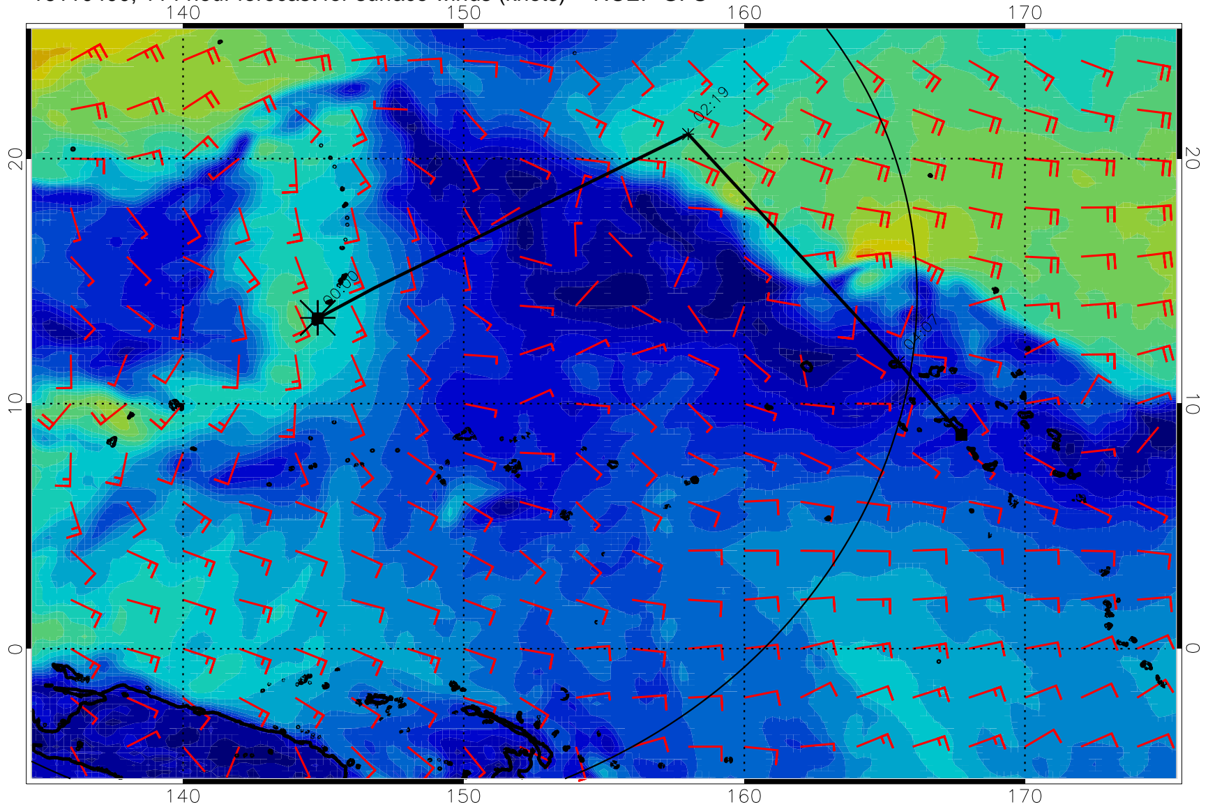
16110400, 114 hour forecast for surface winds (knots) -- NCEP GFS
