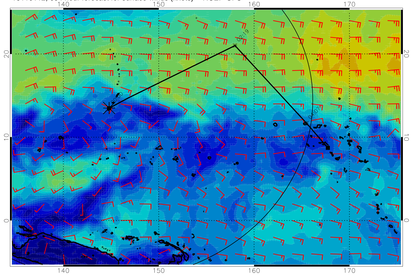
16110112, 054 hour forecast for surface winds (knots) -- NCEP GFS
