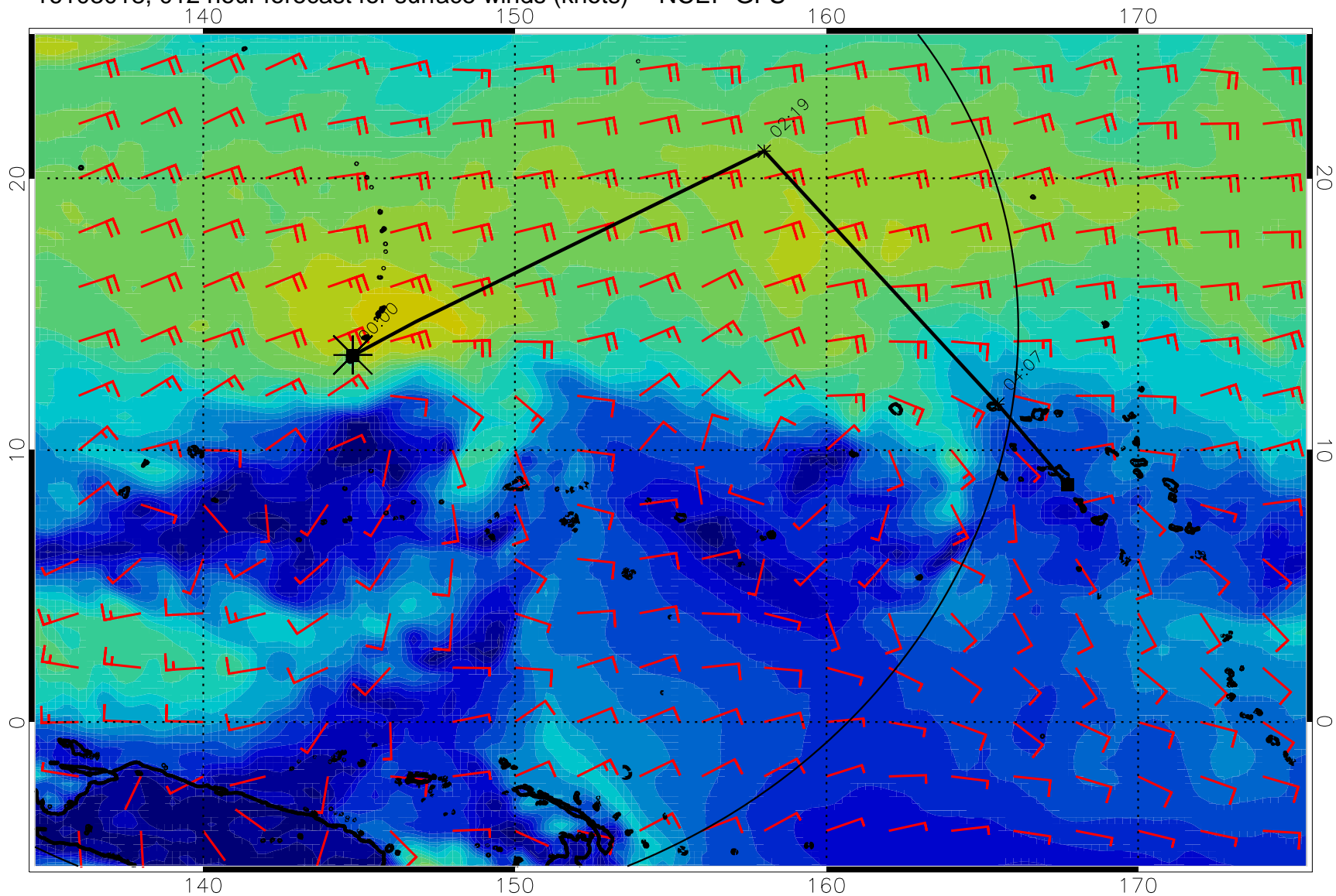
16103018, 012 hour forecast for surface winds (knots) -- NCEP GFS
