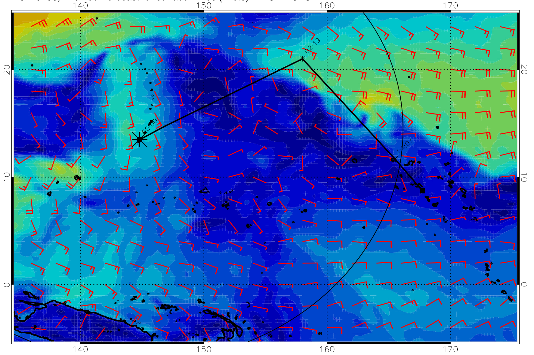
16110406, 120 hour forecast for surface winds (knots) -- NCEP GFS
