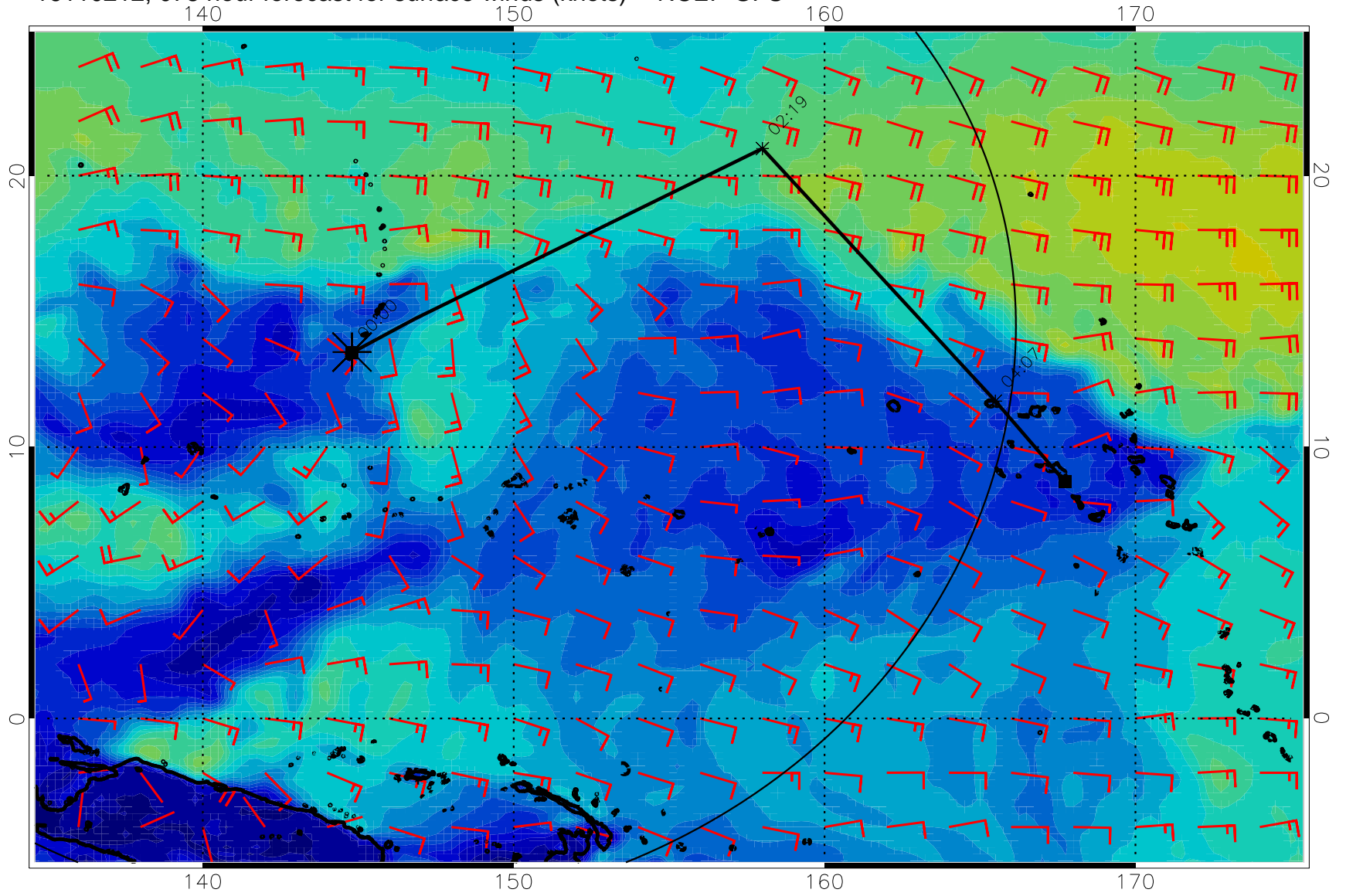
16110212, 078 hour forecast for surface winds (knots) -- NCEP GFS
