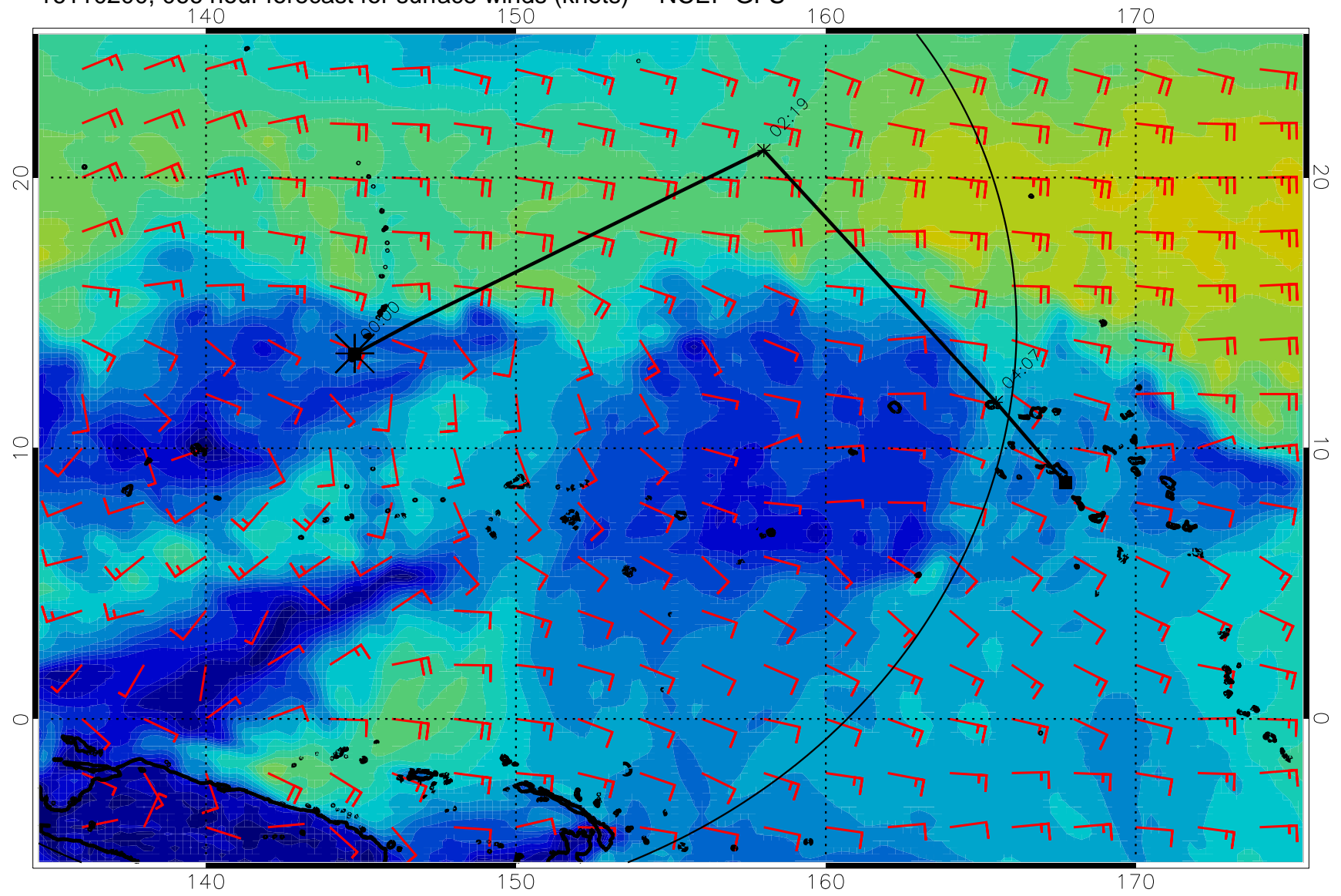
16110200, 066 hour forecast for surface winds (knots) -- NCEP GFS
