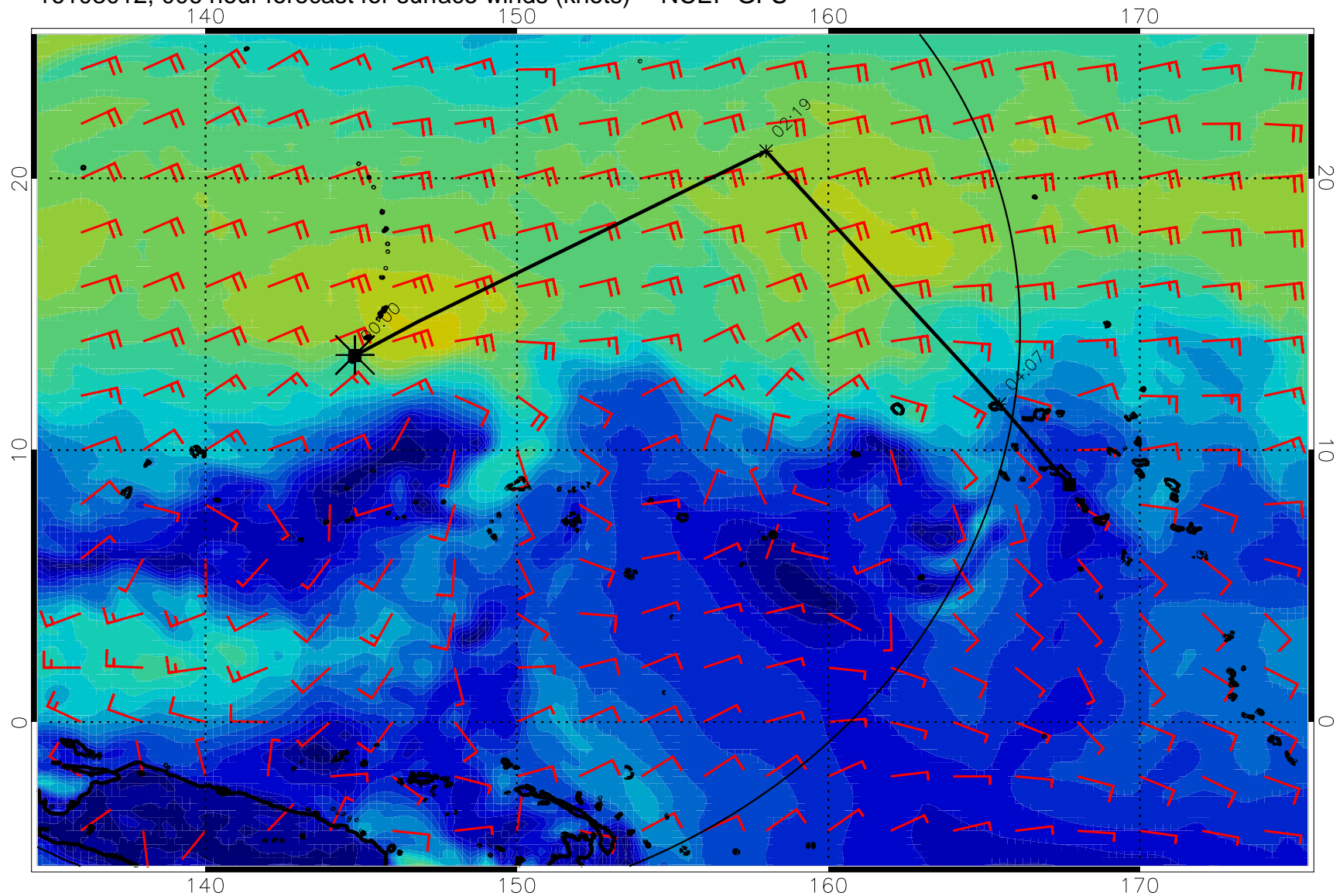
16103012, 006 hour forecast for surface winds (knots) -- NCEP GFS
