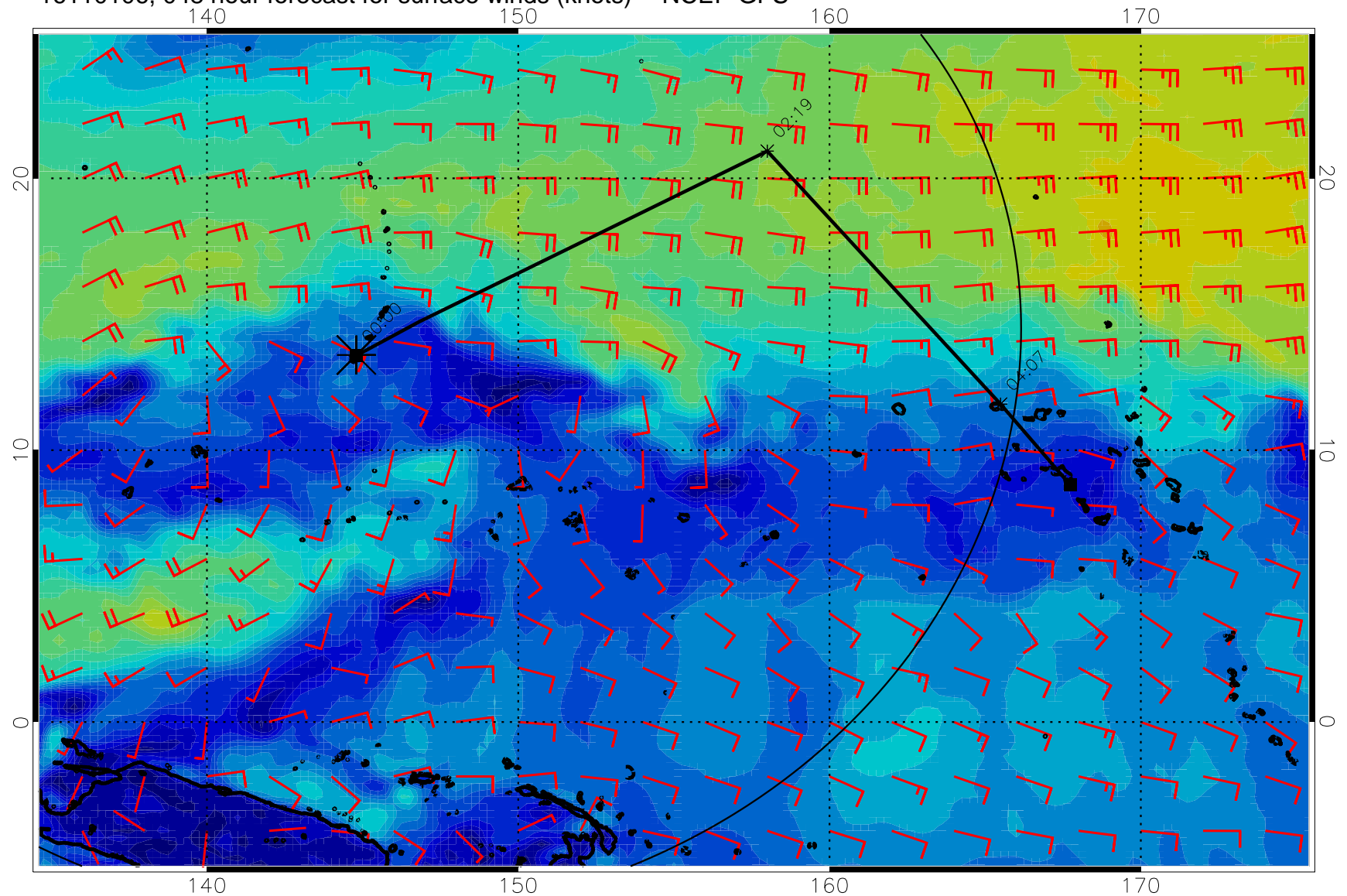
16110106, 048 hour forecast for surface winds (knots) -- NCEP GFS
