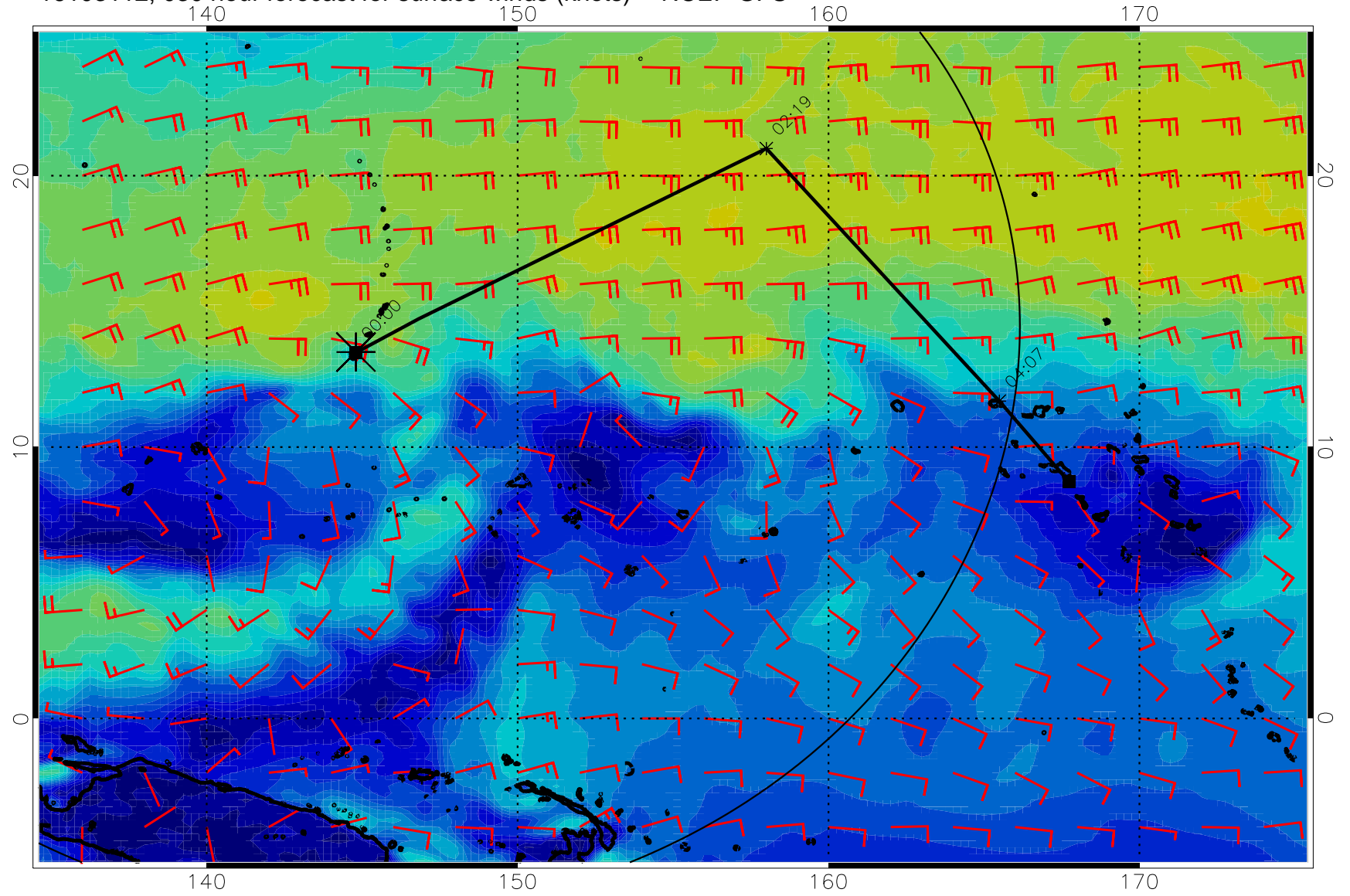
16103112, 030 hour forecast for surface winds (knots) -- NCEP GFS
