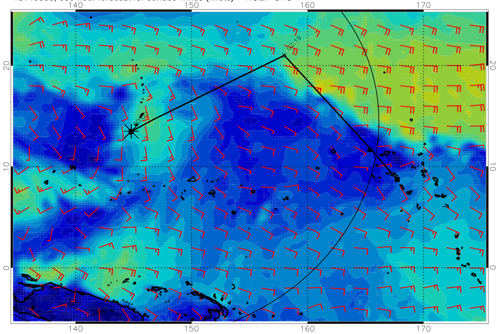
16110300, 090 hour forecast for surface winds (knots) -- NCEP GFS
