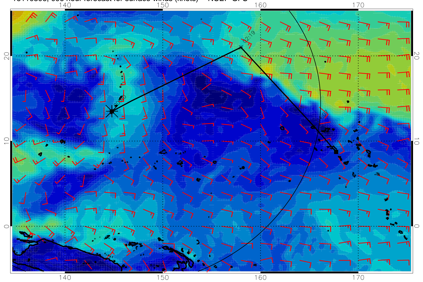
16110306, 096 hour forecast for surface winds (knots) -- NCEP GFS
