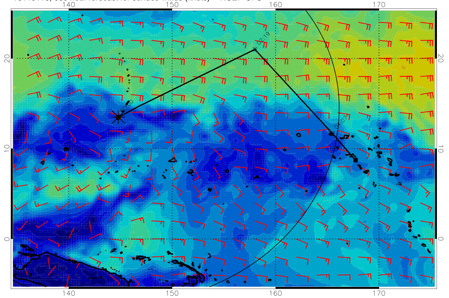
16110118, 060 hour forecast for surface winds (knots) -- NCEP GFS
