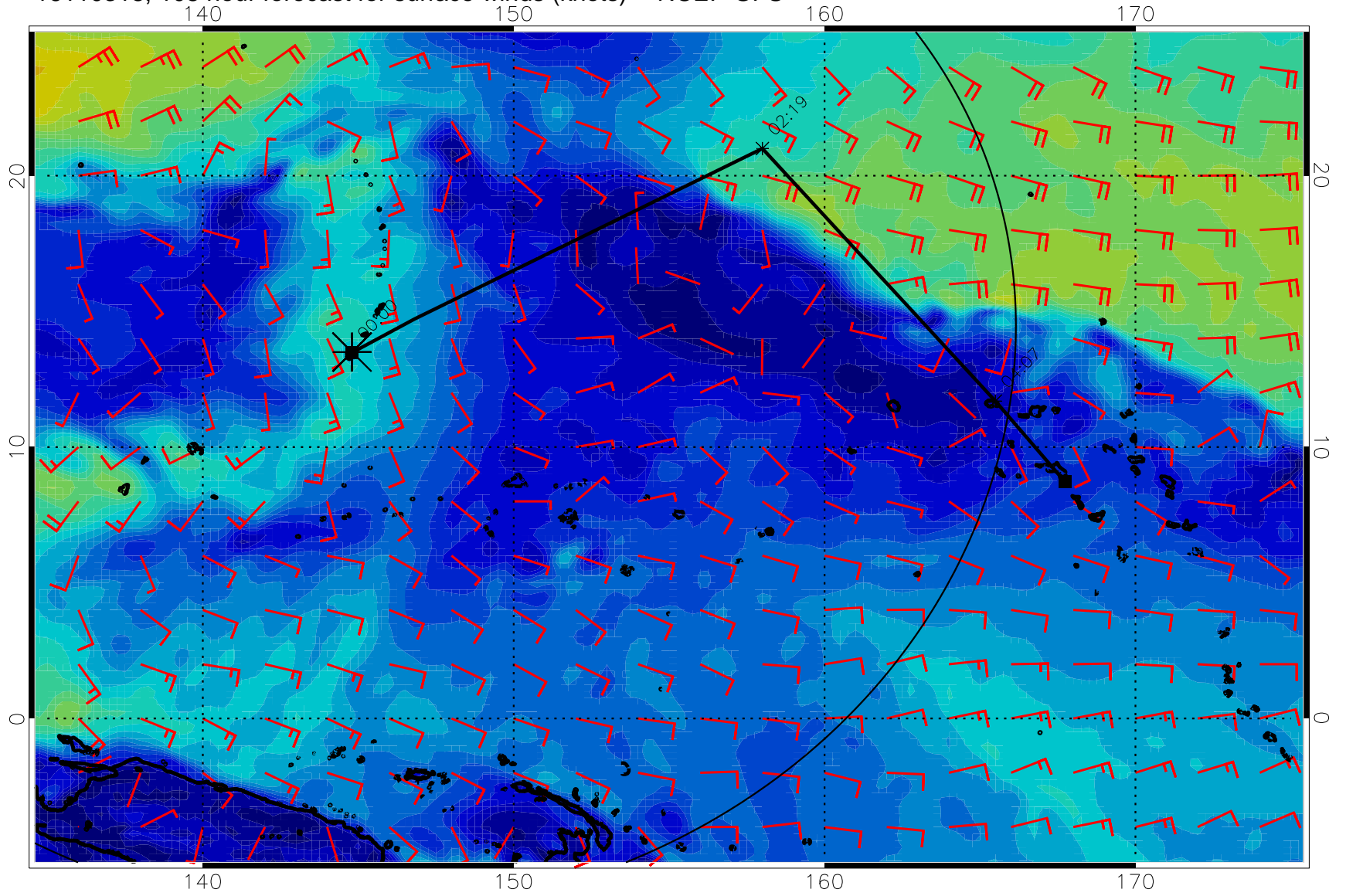
16110318, 108 hour forecast for surface winds (knots) -- NCEP GFS
