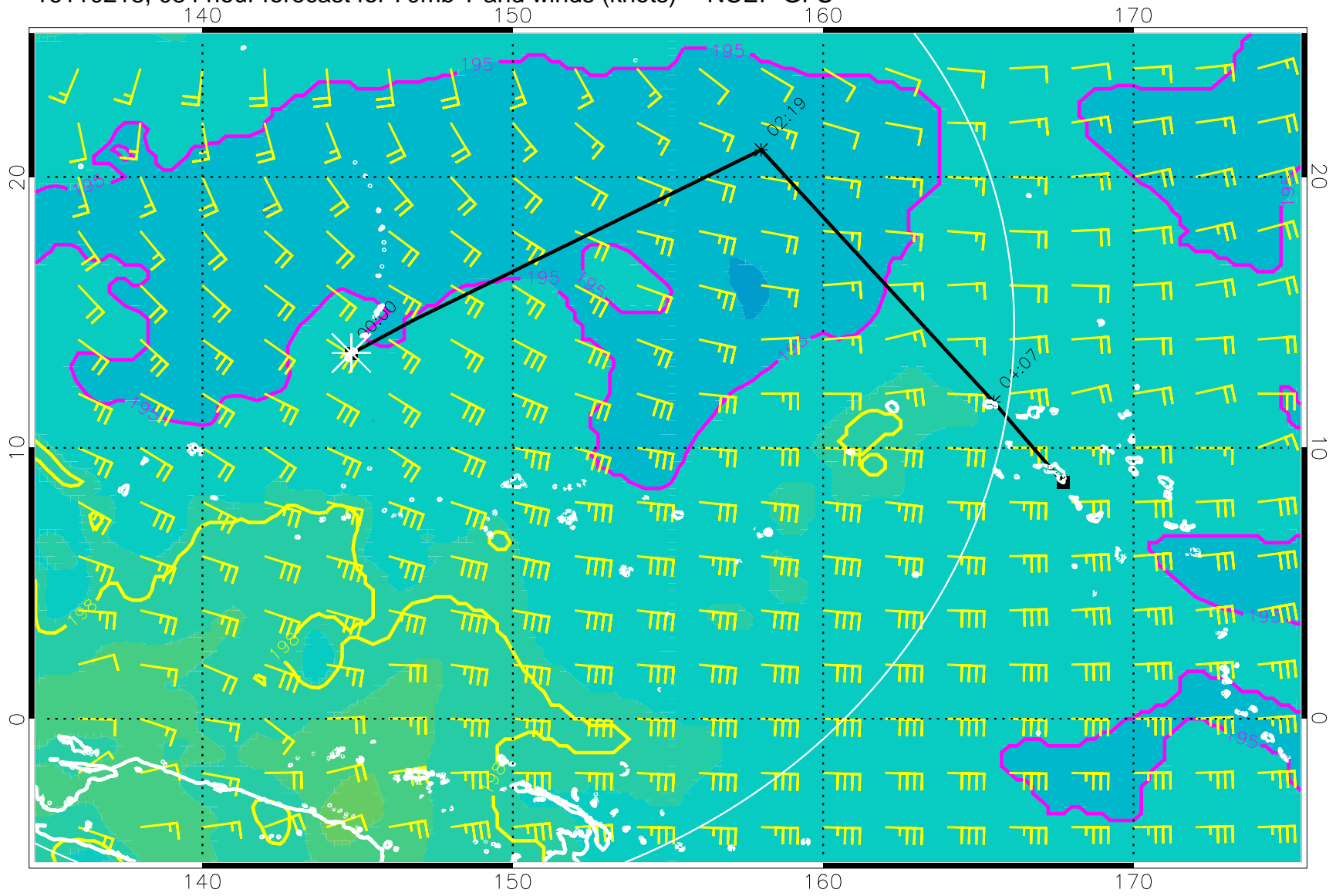
16110218, 084 hour forecast for 70mb T and winds (knots) -- NCEP GFS
