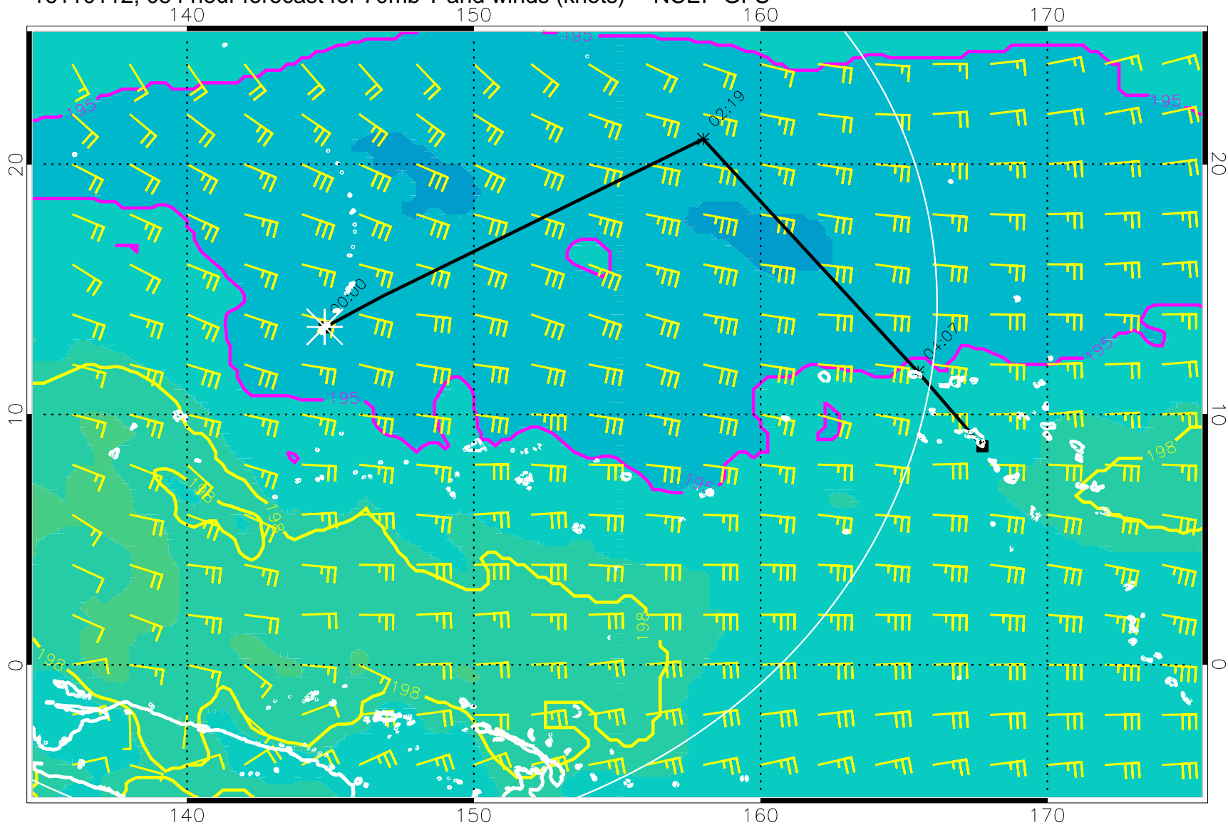
16110112, 054 hour forecast for 70mb T and winds (knots) -- NCEP GFS
