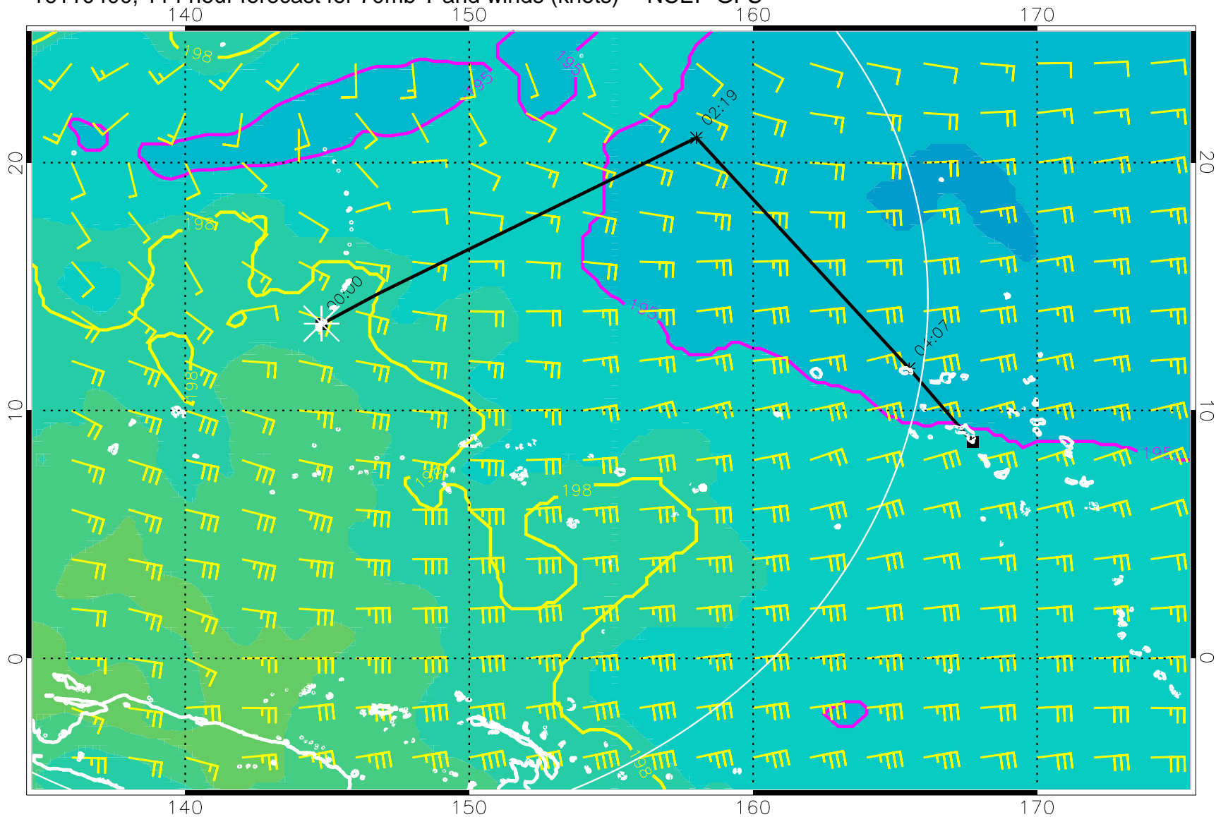
16110400, 114 hour forecast for 70mb T and winds (knots) -- NCEP GFS
