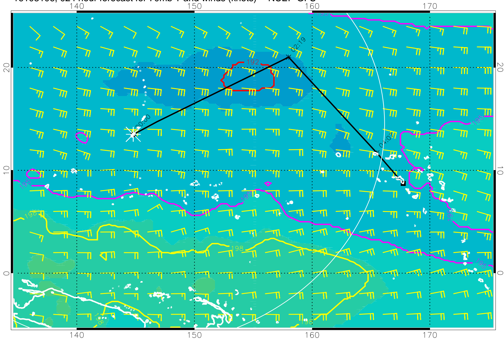
16103106, 024 hour forecast for 70mb T and winds (knots) -- NCEP GFS
