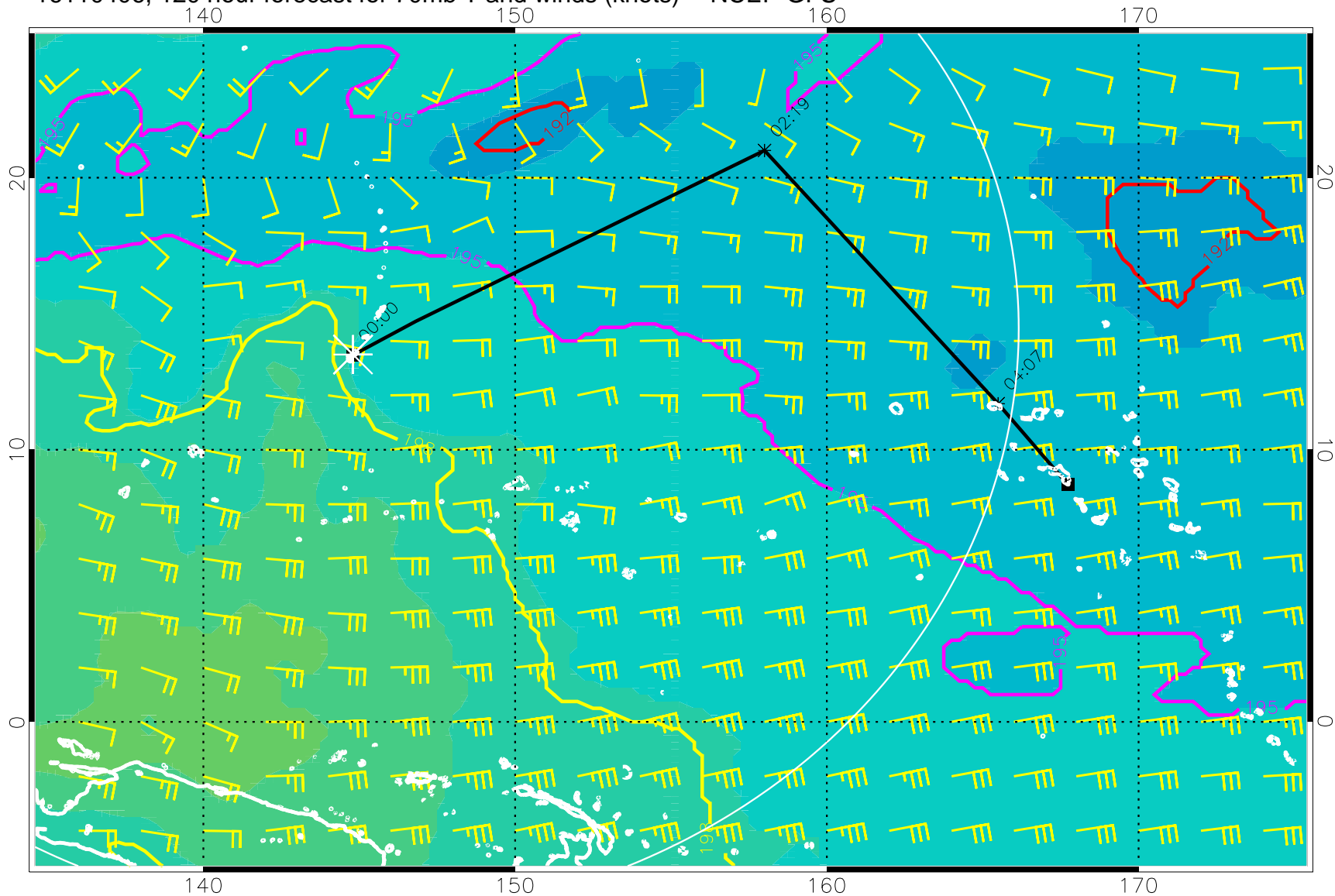
16110406, 120 hour forecast for 70mb T and winds (knots) -- NCEP GFS
