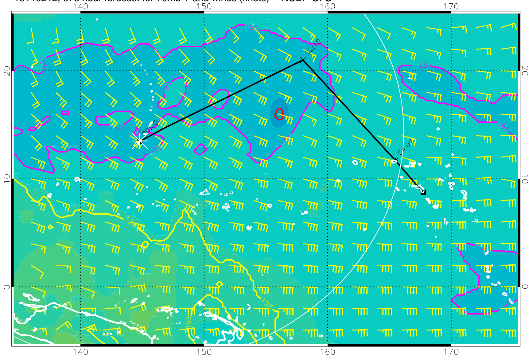
16110212, 078 hour forecast for 70mb T and winds (knots) -- NCEP GFS
