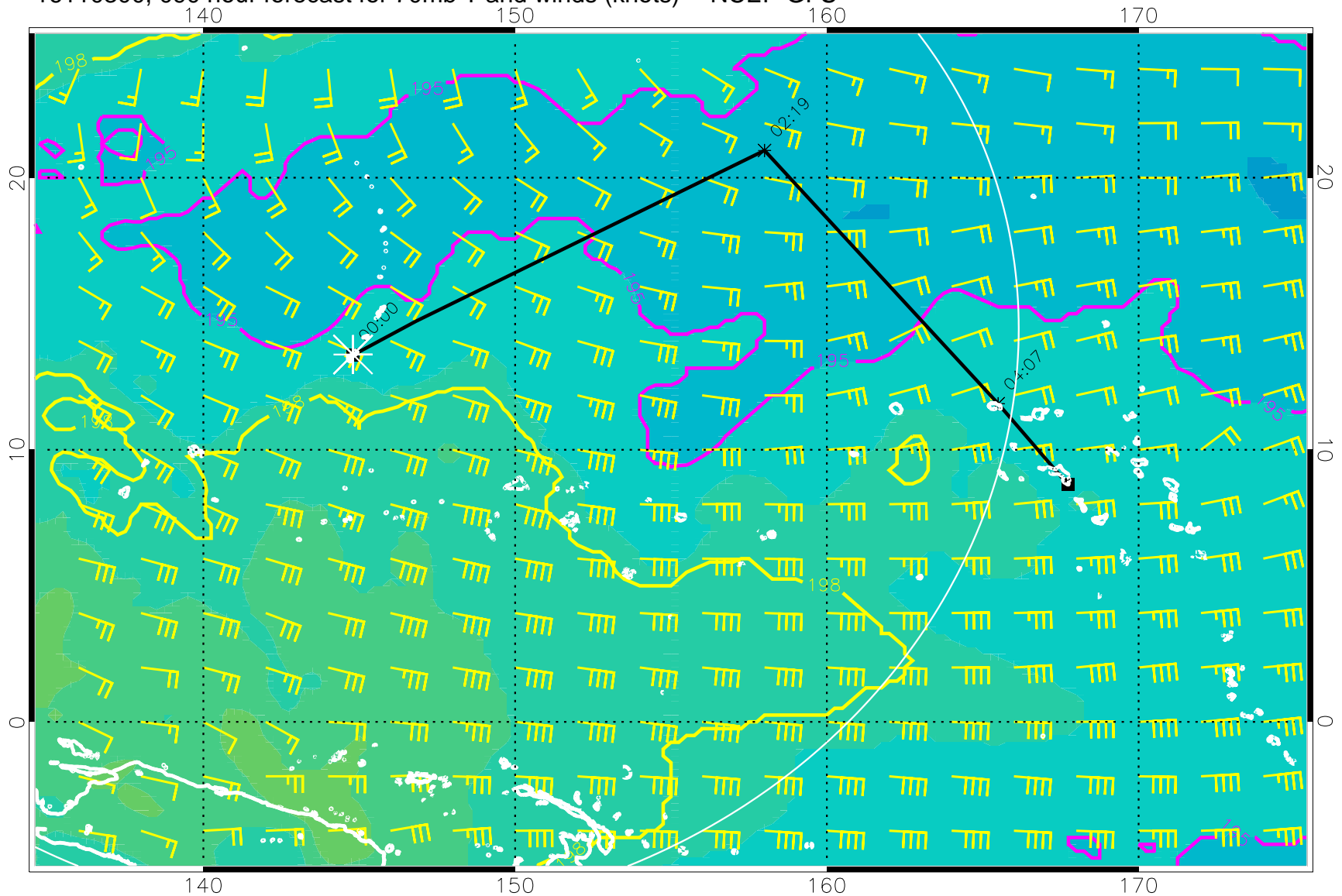
16110300, 090 hour forecast for 70mb T and winds (knots) -- NCEP GFS
