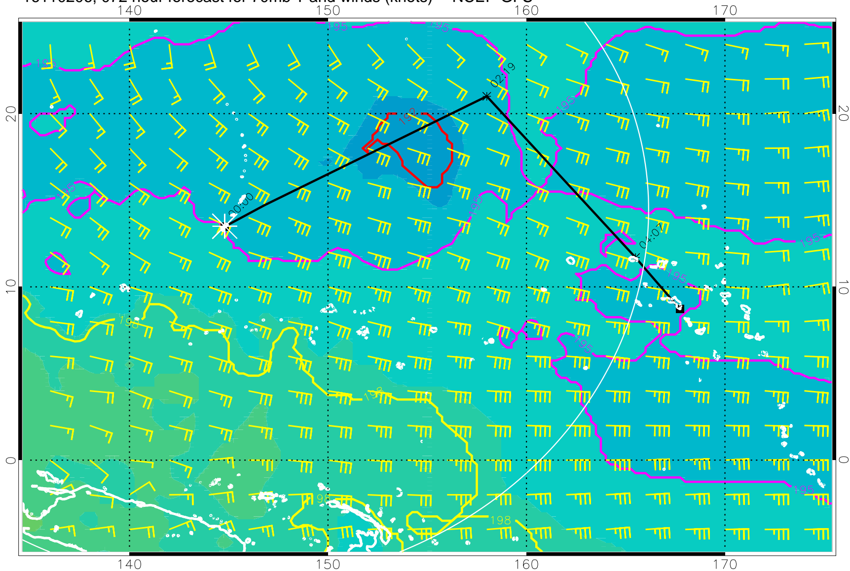
16110206, 072 hour forecast for 70mb T and winds (knots) -- NCEP GFS
