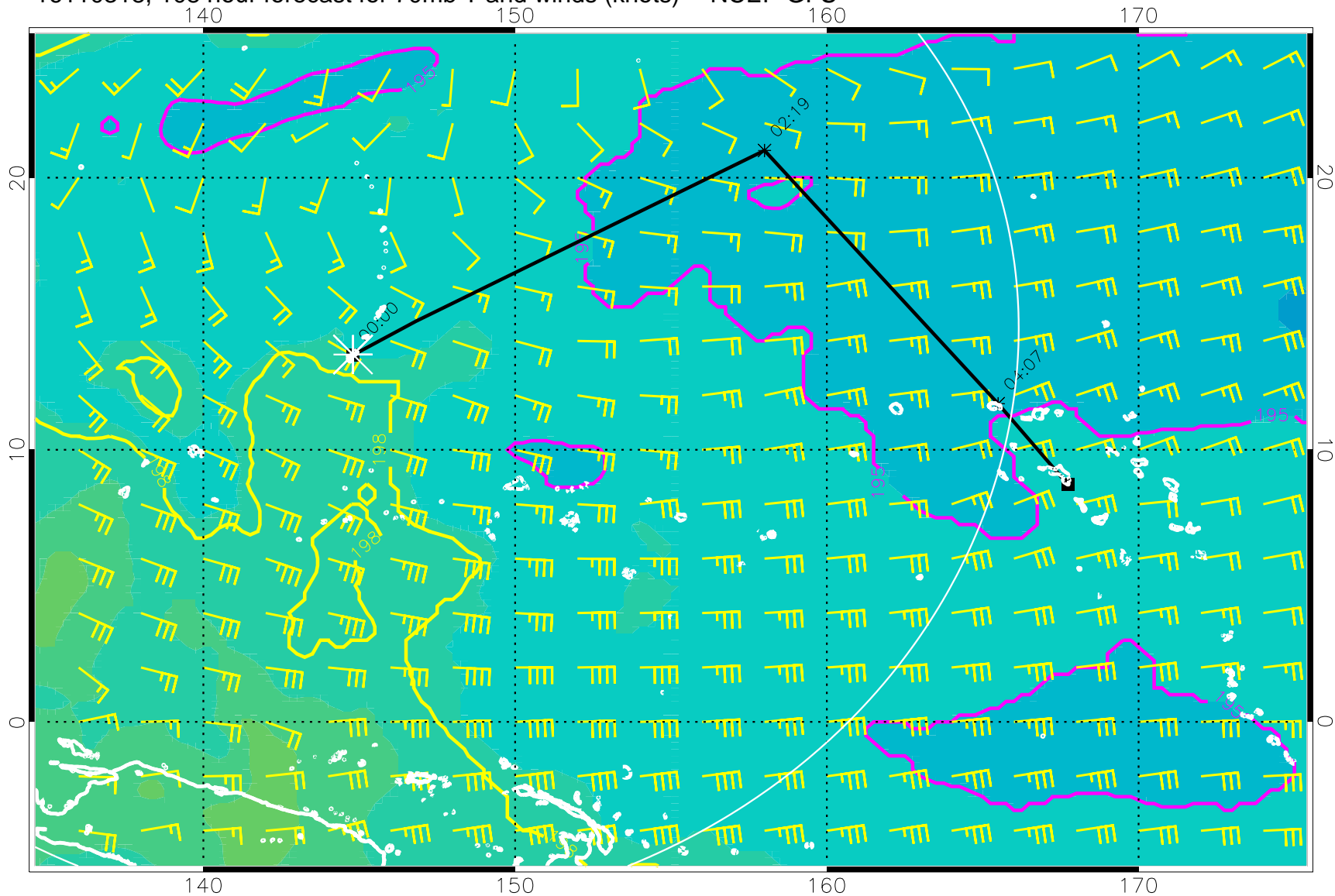
16110318, 108 hour forecast for 70mb T and winds (knots) -- NCEP GFS
