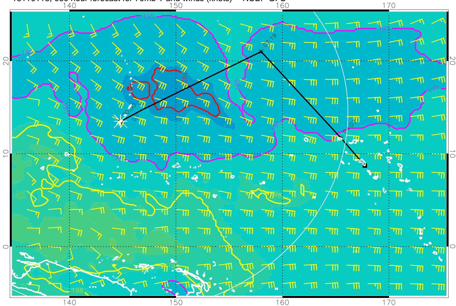
16110118, 060 hour forecast for 70mb T and winds (knots) -- NCEP GFS
