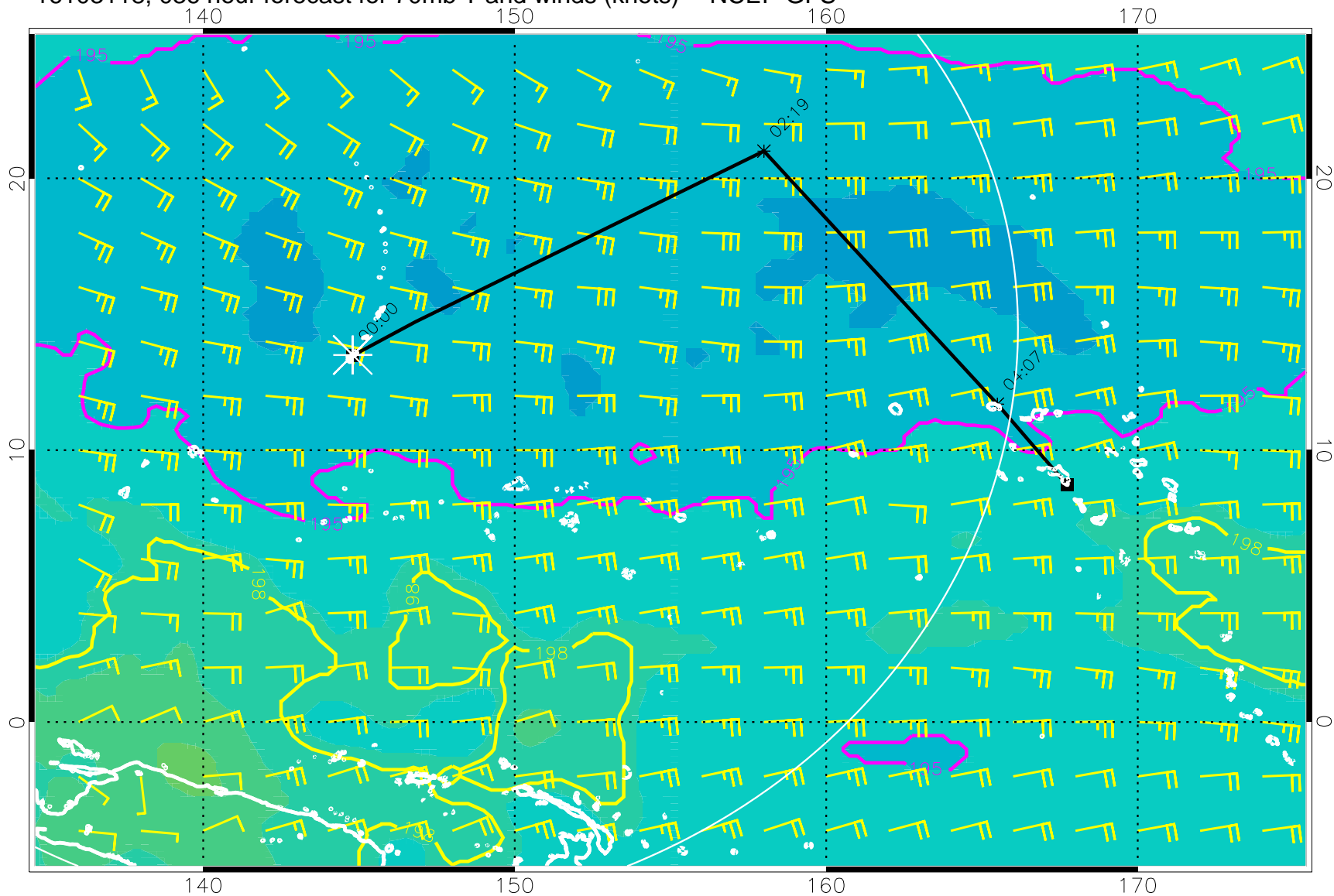
16103118, 036 hour forecast for 70mb T and winds (knots) -- NCEP GFS
