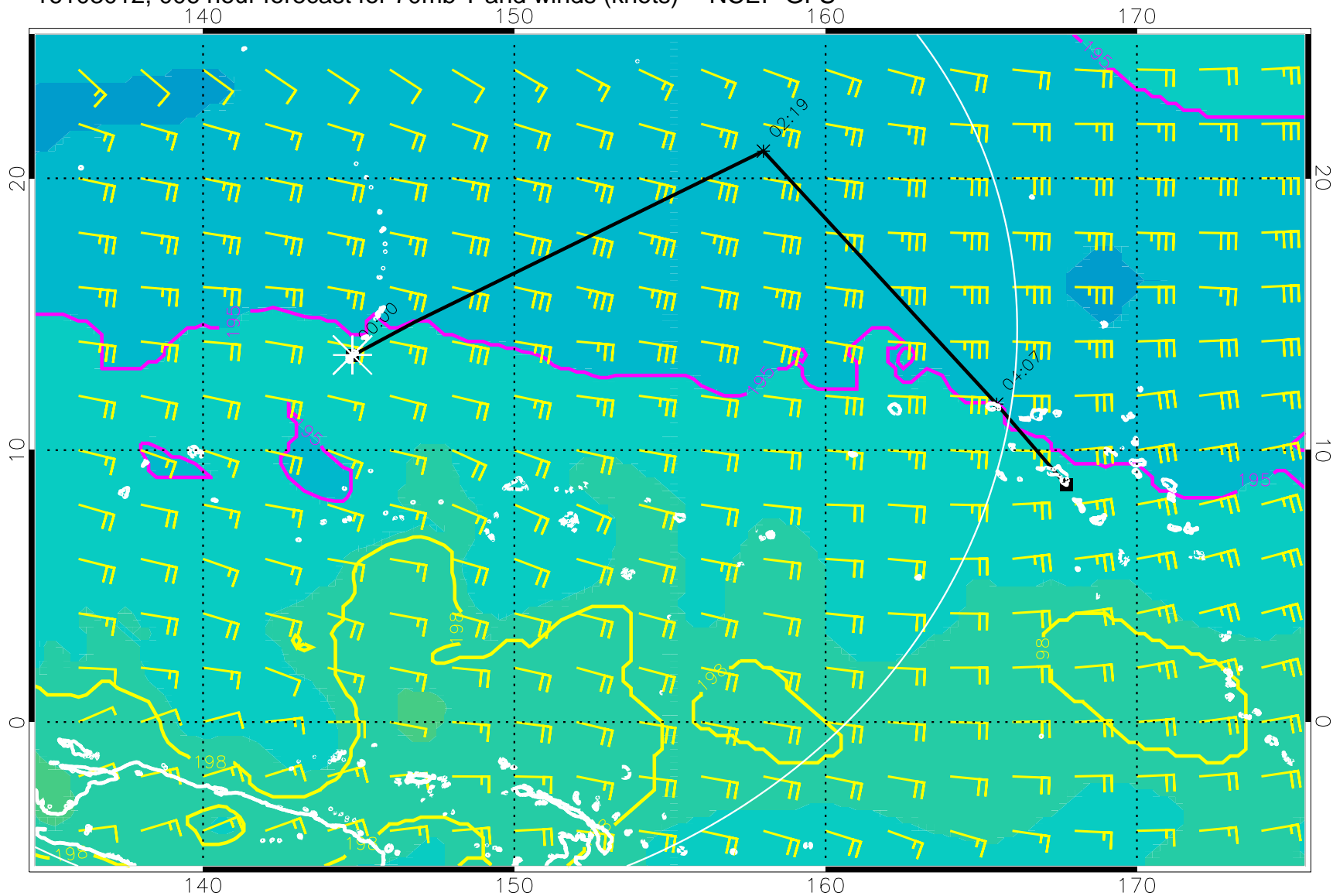
16103012, 006 hour forecast for 70mb T and winds (knots) -- NCEP GFS
