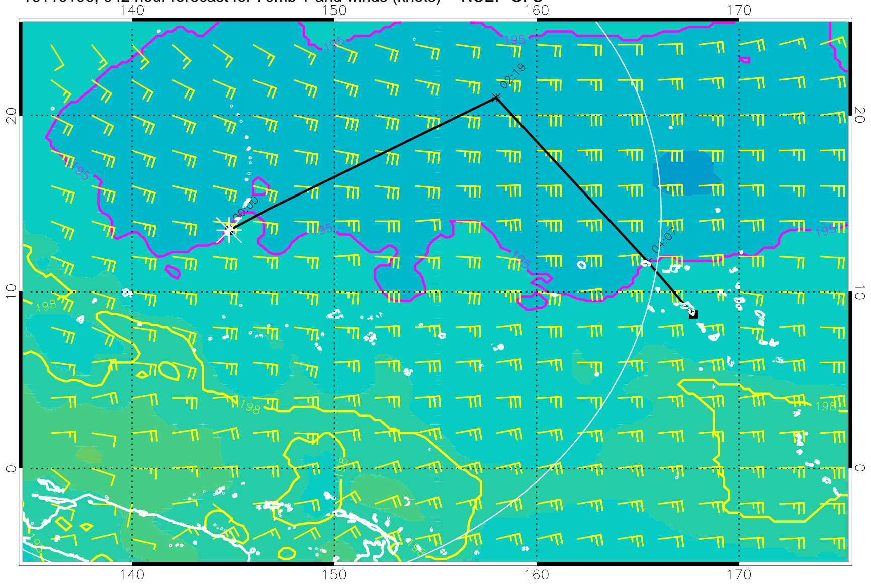
16110100, 042 hour forecast for 70mb T and winds (knots) -- NCEP GFS
