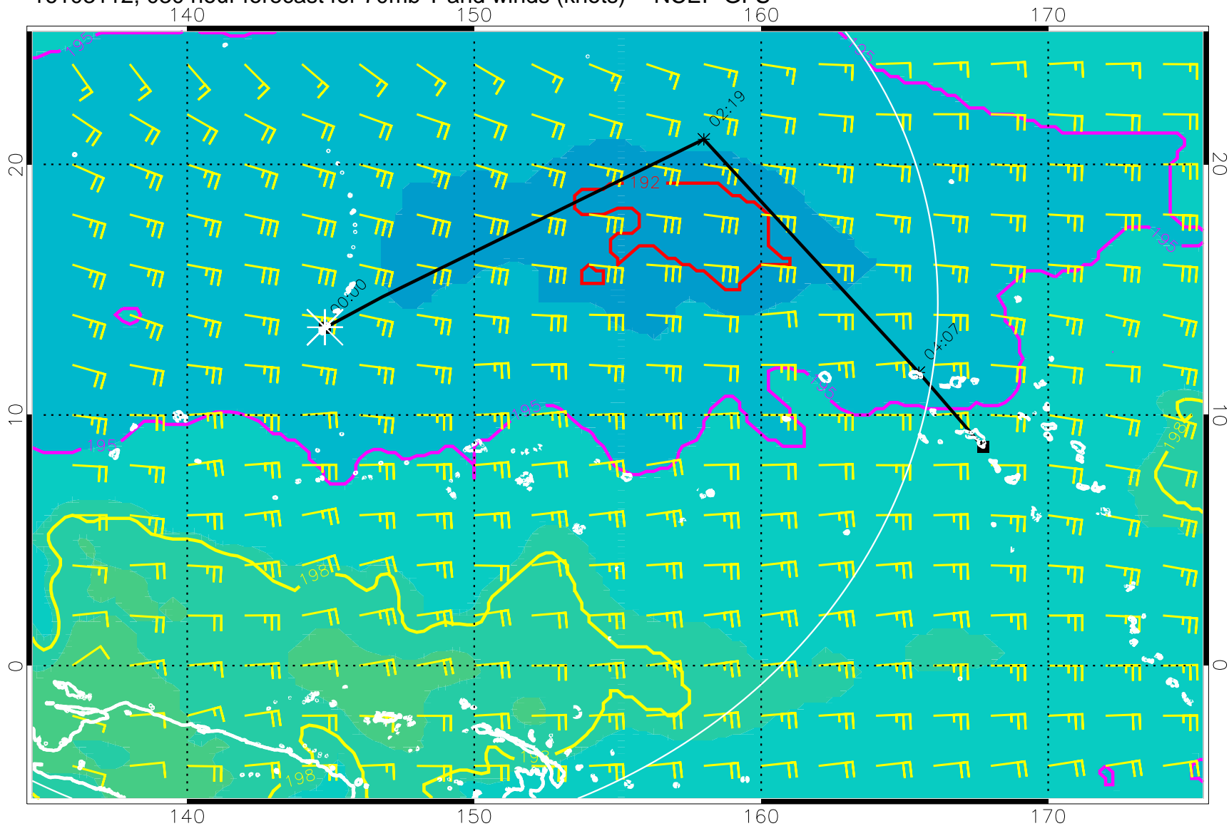
16103112, 030 hour forecast for 70mb T and winds (knots) -- NCEP GFS
