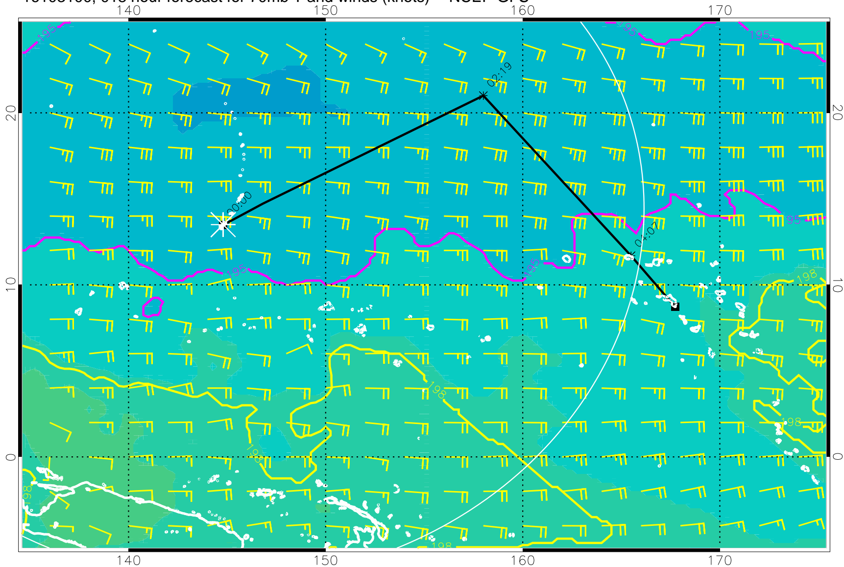
16103100, 018 hour forecast for 70mb T and winds (knots) -- NCEP GFS
