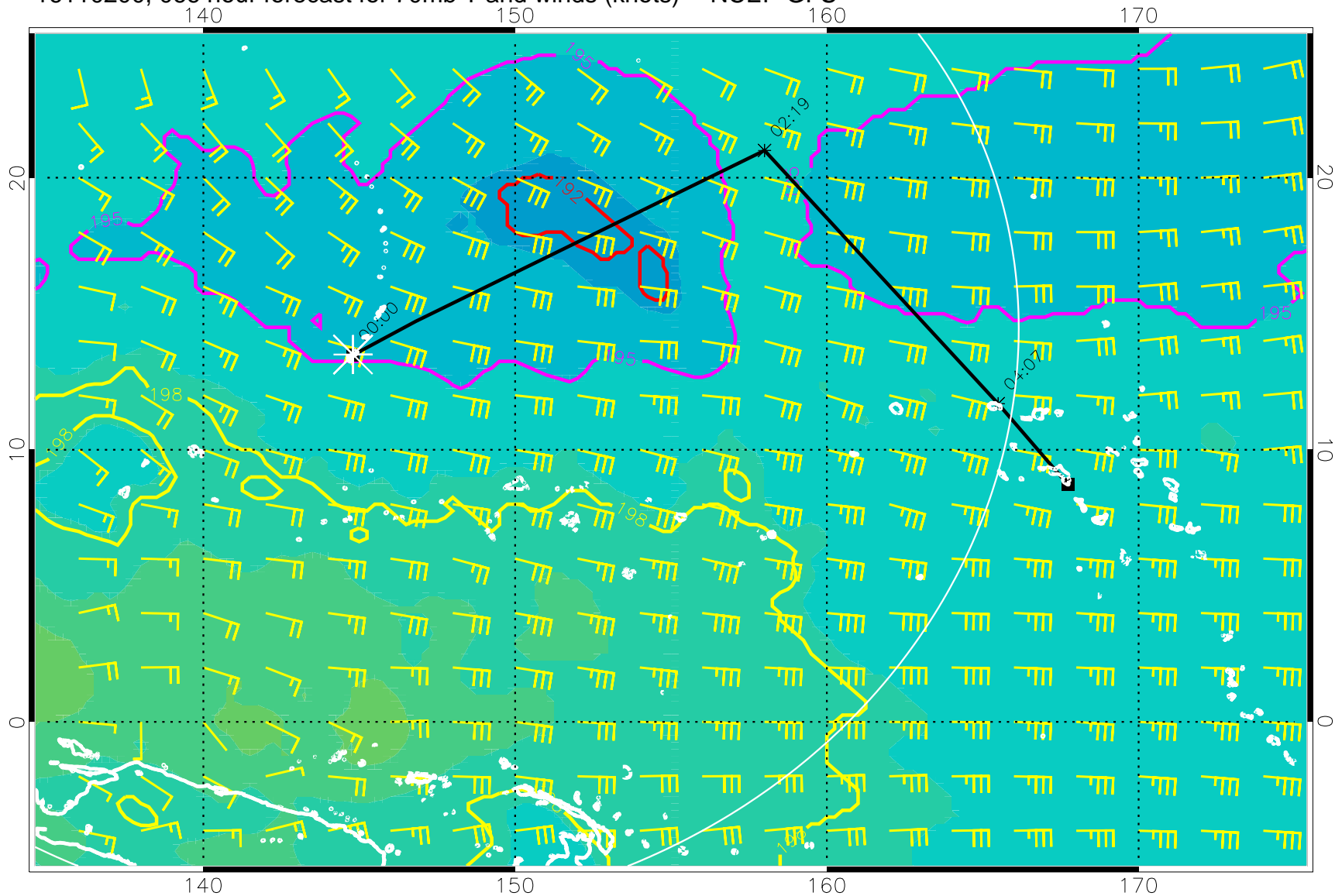
16110200, 066 hour forecast for 70mb T and winds (knots) -- NCEP GFS
