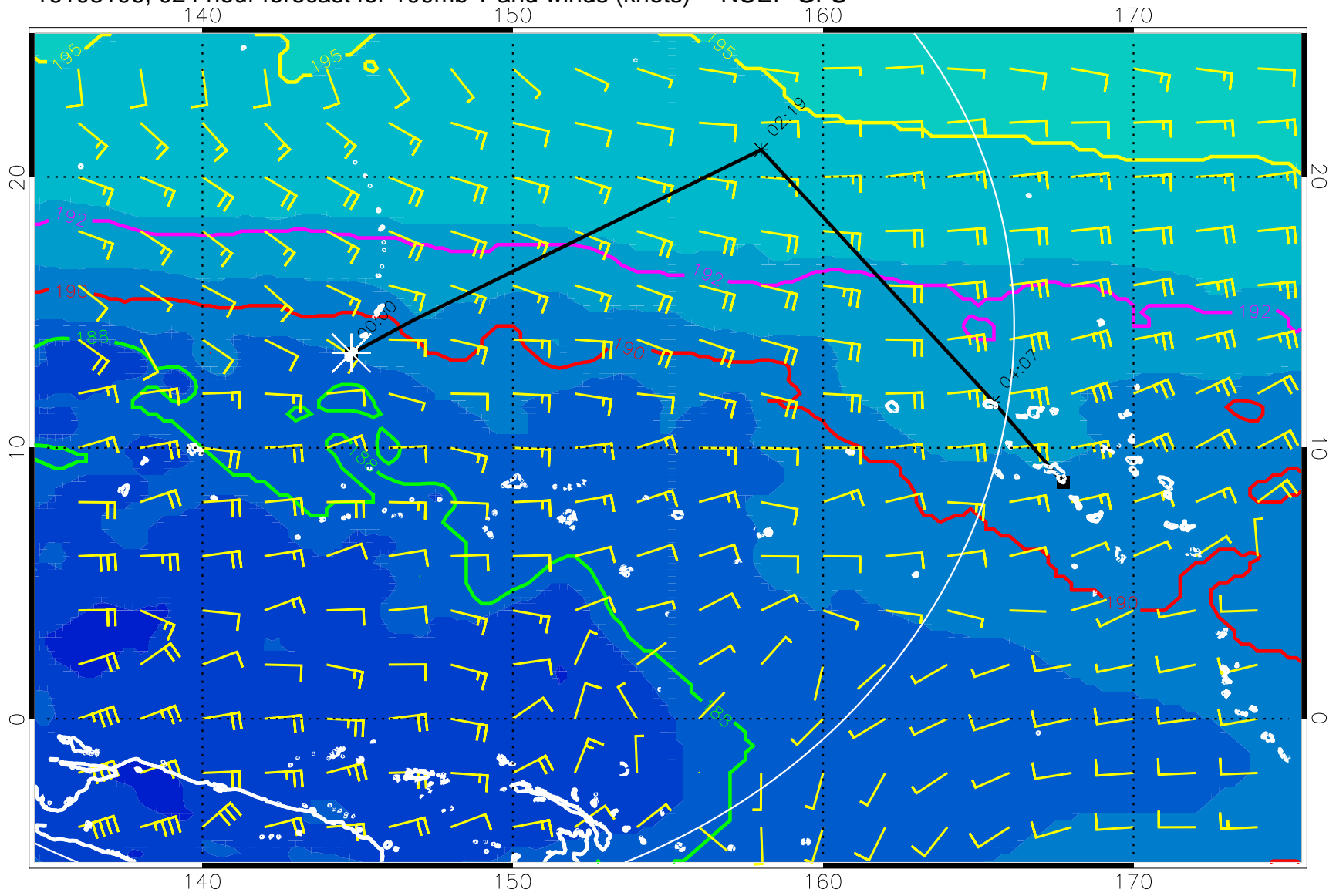
16103106, 024 hour forecast for 100mb T and winds (knots) -- NCEP GFS
