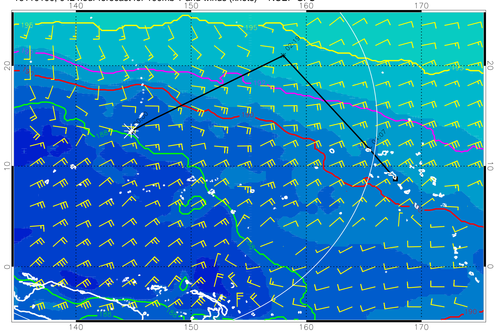
16110100, 042 hour forecast for 100mb T and winds (knots) -- NCEP GFS
