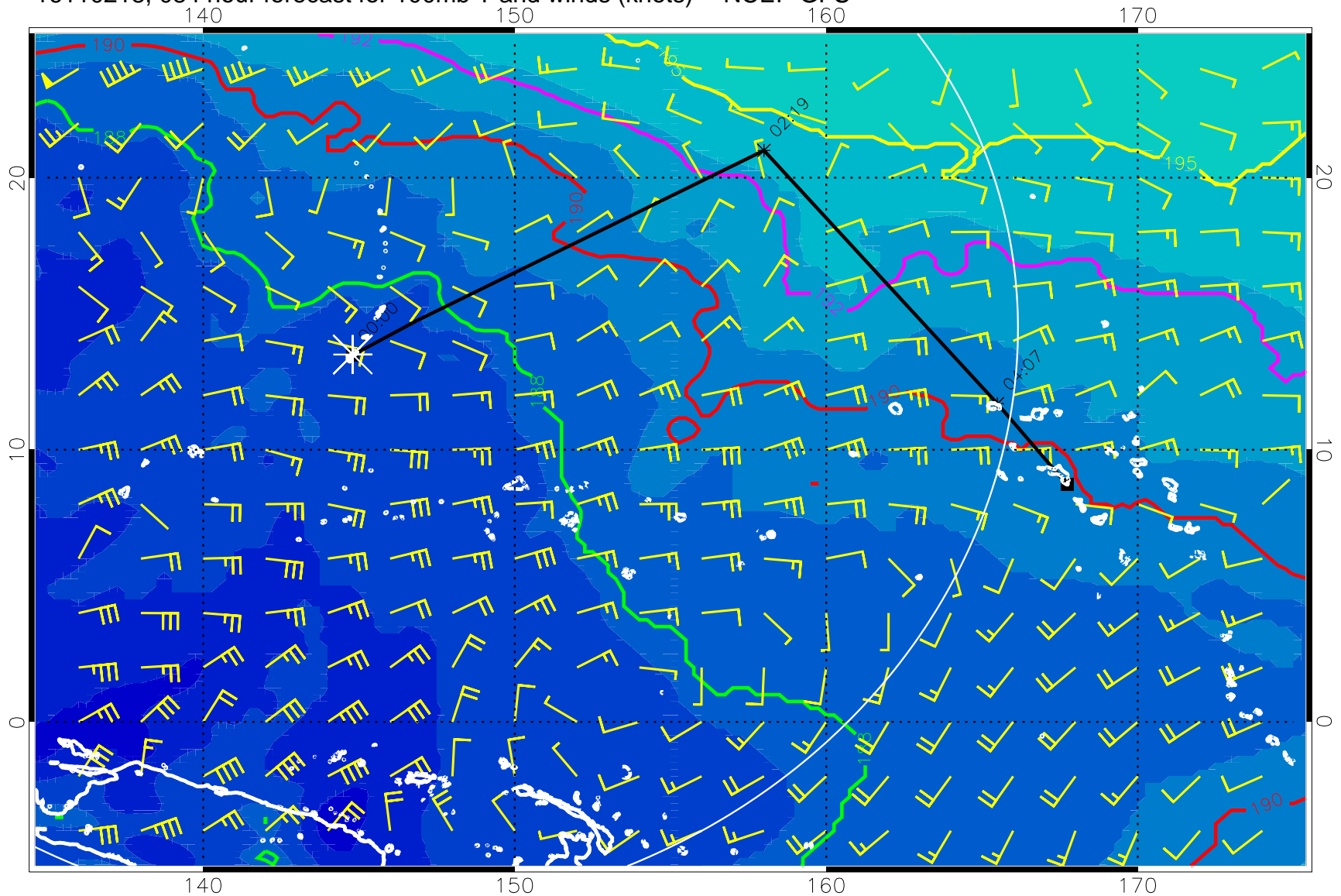
16110218, 084 hour forecast for 100mb T and winds (knots) -- NCEP GFS
