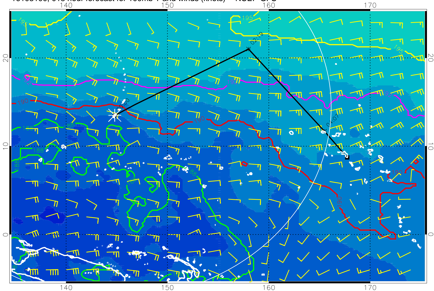
16103100, 018 hour forecast for 100mb T and winds (knots) -- NCEP GFS
