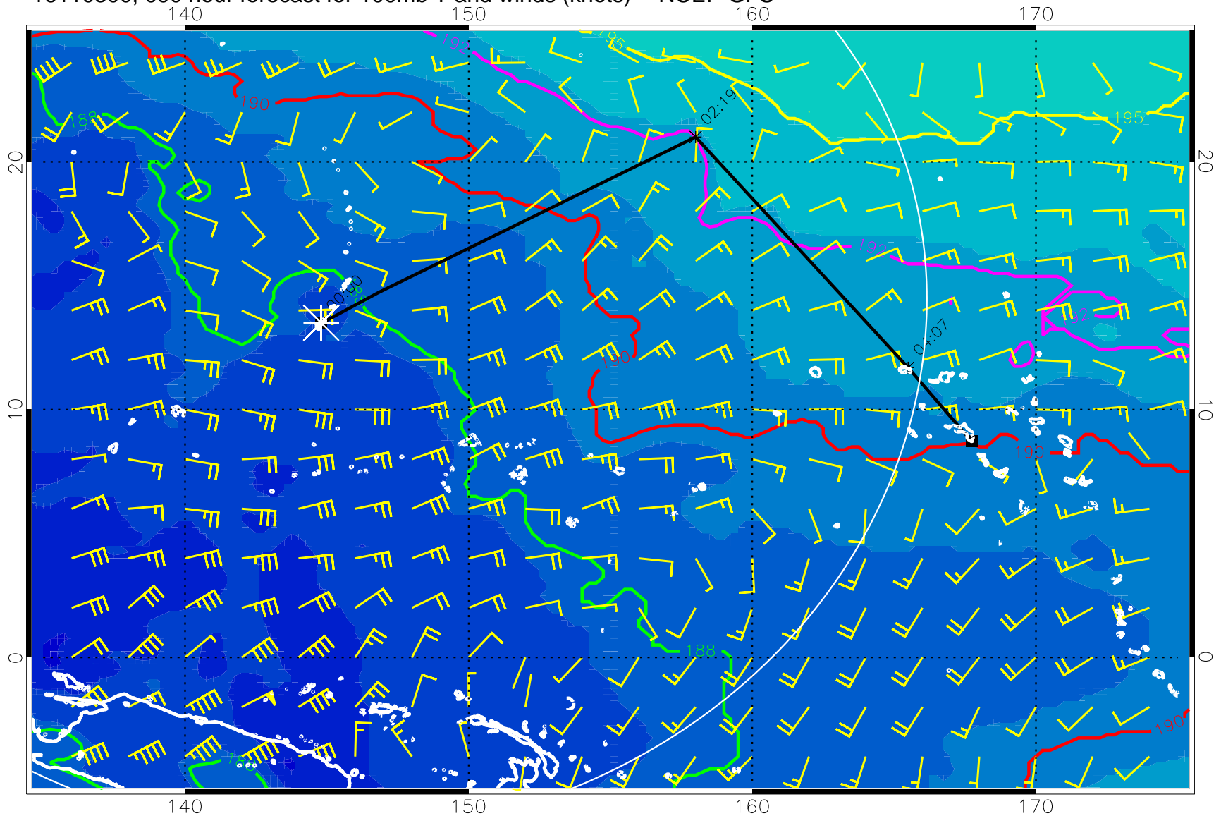
16110300, 090 hour forecast for 100mb T and winds (knots) -- NCEP GFS
