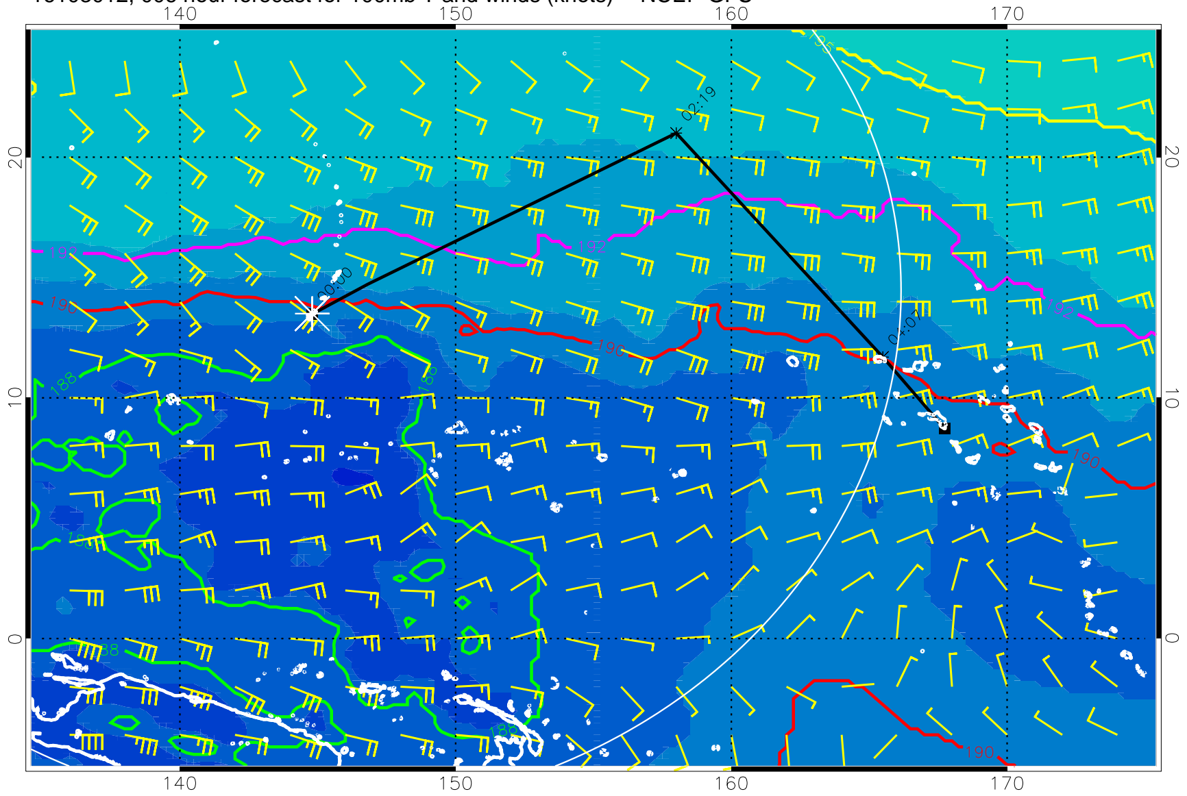
16103012, 006 hour forecast for 100mb T and winds (knots) -- NCEP GFS
