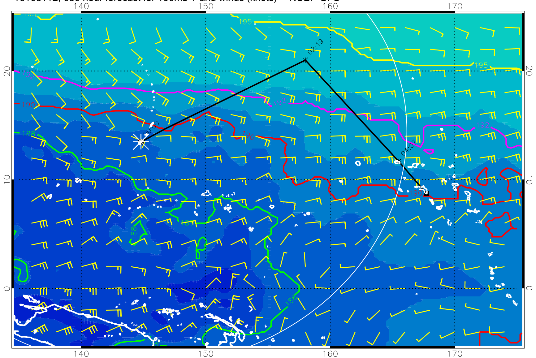
16103112, 030 hour forecast for 100mb T and winds (knots) -- NCEP GFS
