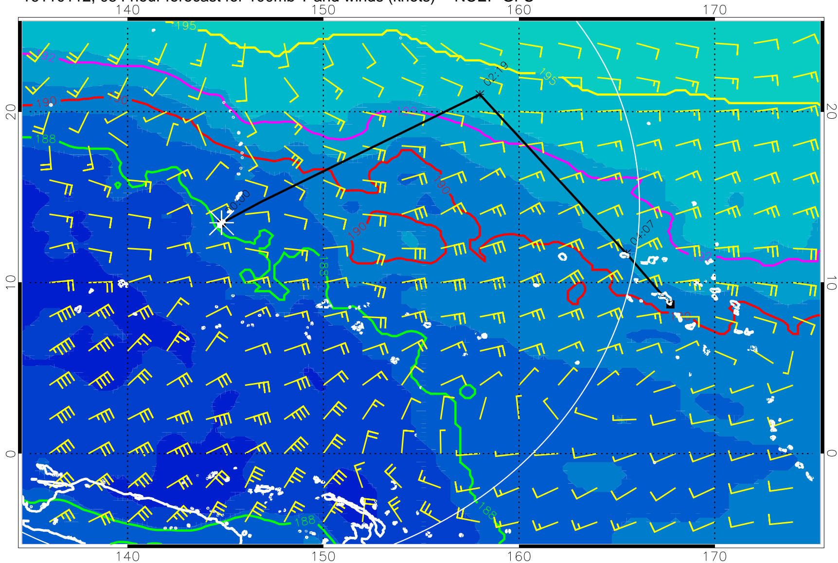
16110112, 054 hour forecast for 100mb T and winds (knots) -- NCEP GFS
