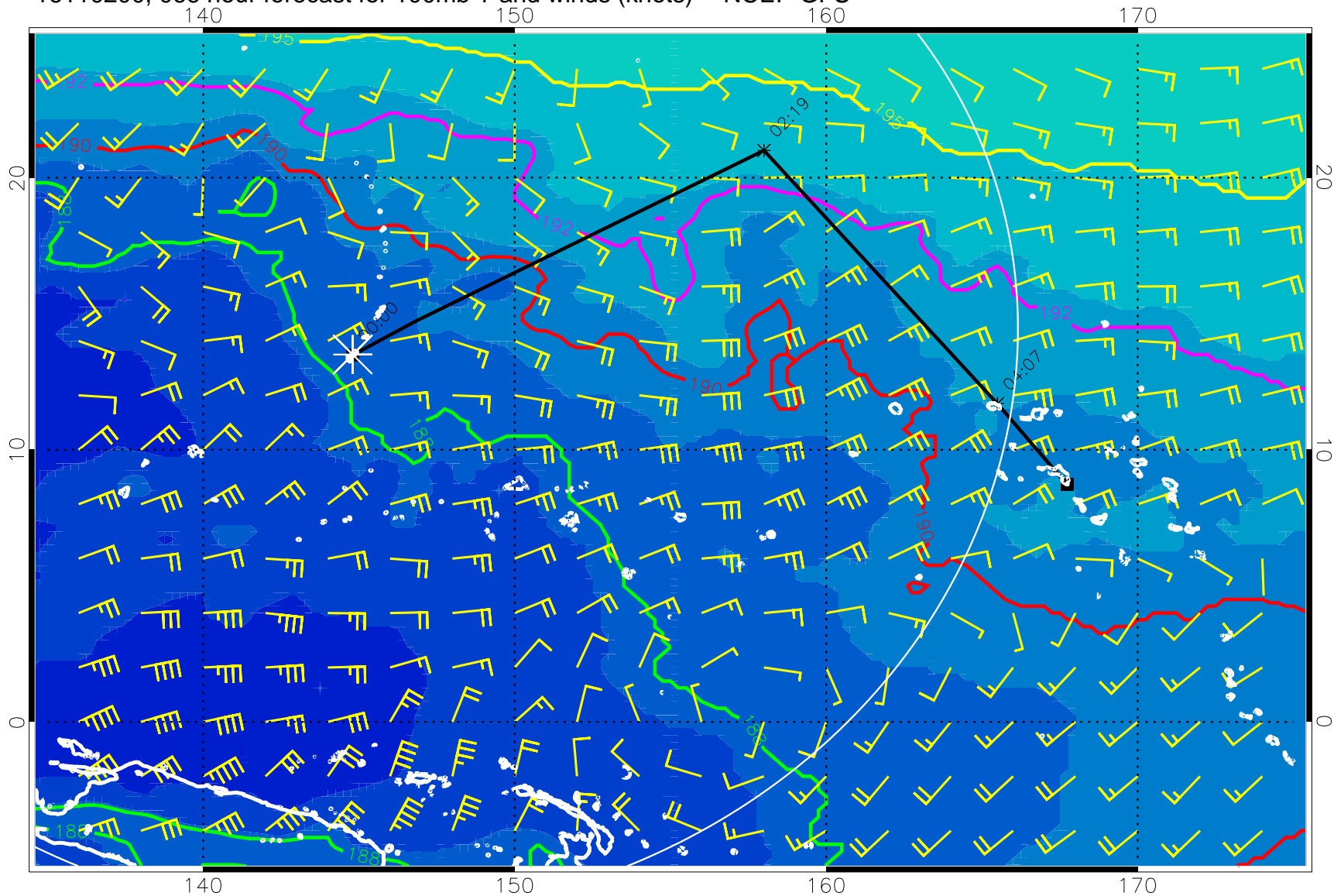
16110200, 066 hour forecast for 100mb T and winds (knots) -- NCEP GFS
