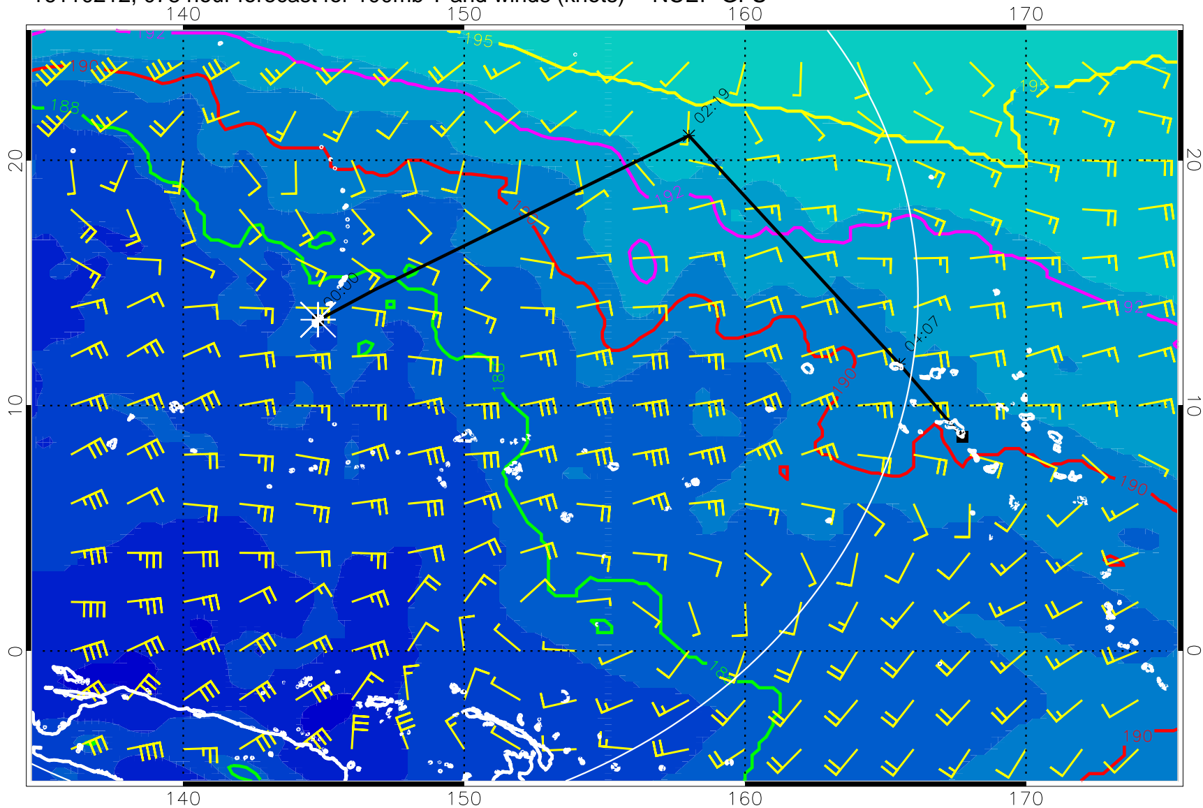
16110212, 078 hour forecast for 100mb T and winds (knots) -- NCEP GFS
