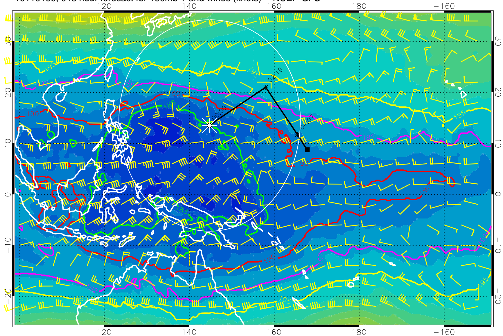
16110106, 048 hour forecast for 100mb T and winds (knots) -- NCEP GFS
