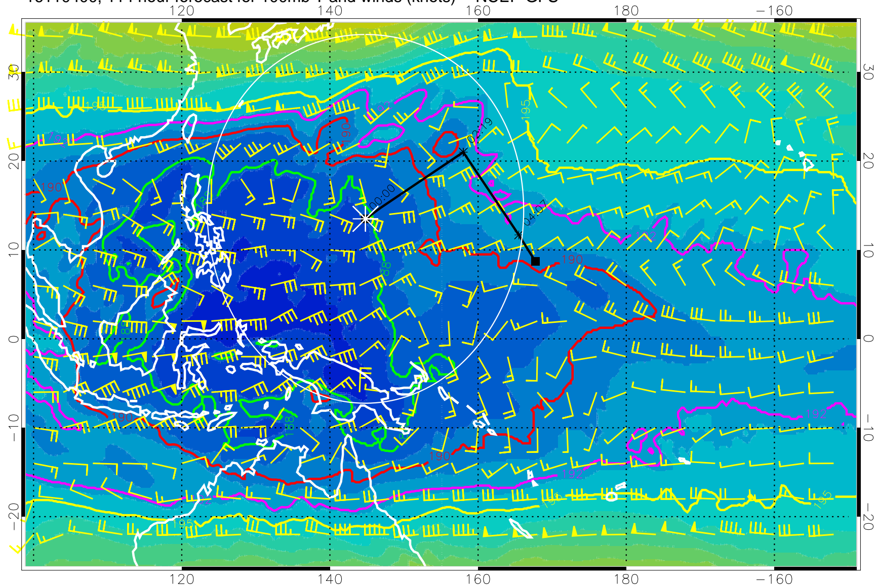
16110400, 114 hour forecast for 100mb T and winds (knots) -- NCEP GFS
