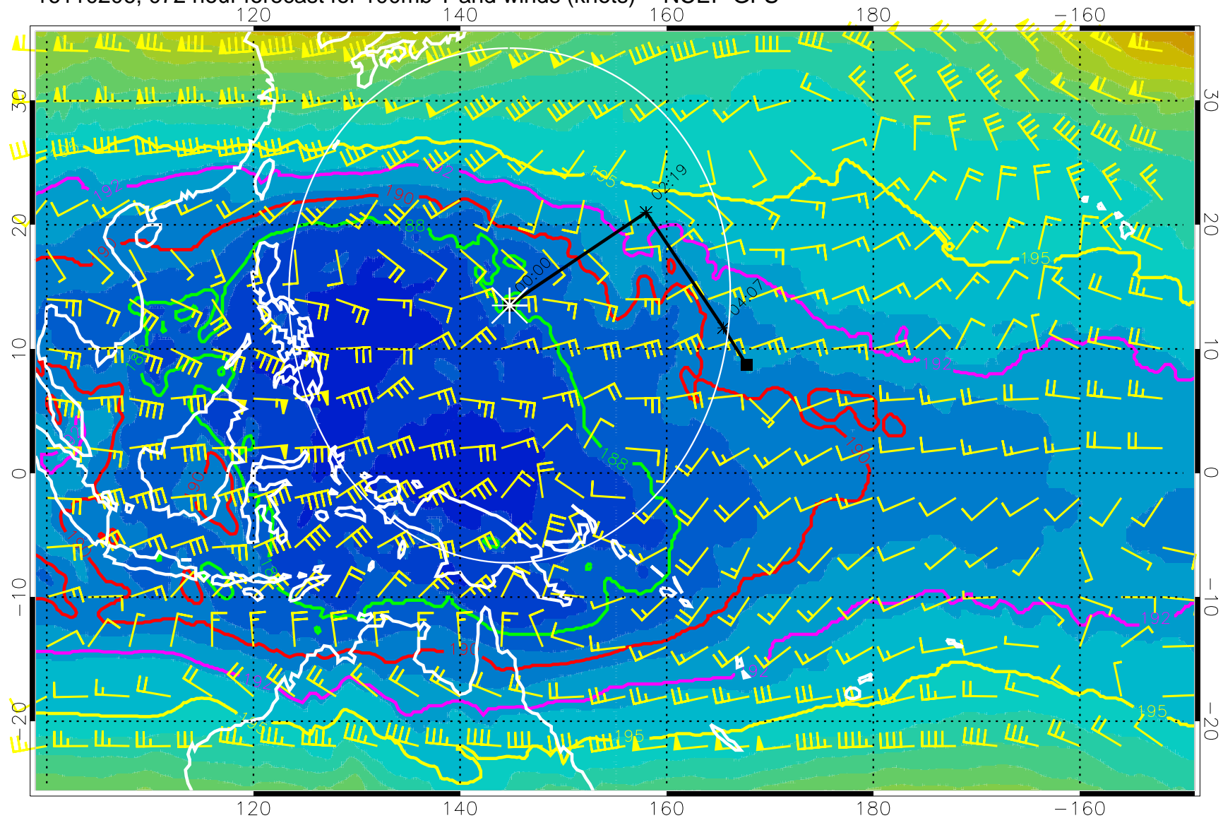
16110206, 072 hour forecast for 100mb T and winds (knots) -- NCEP GFS
