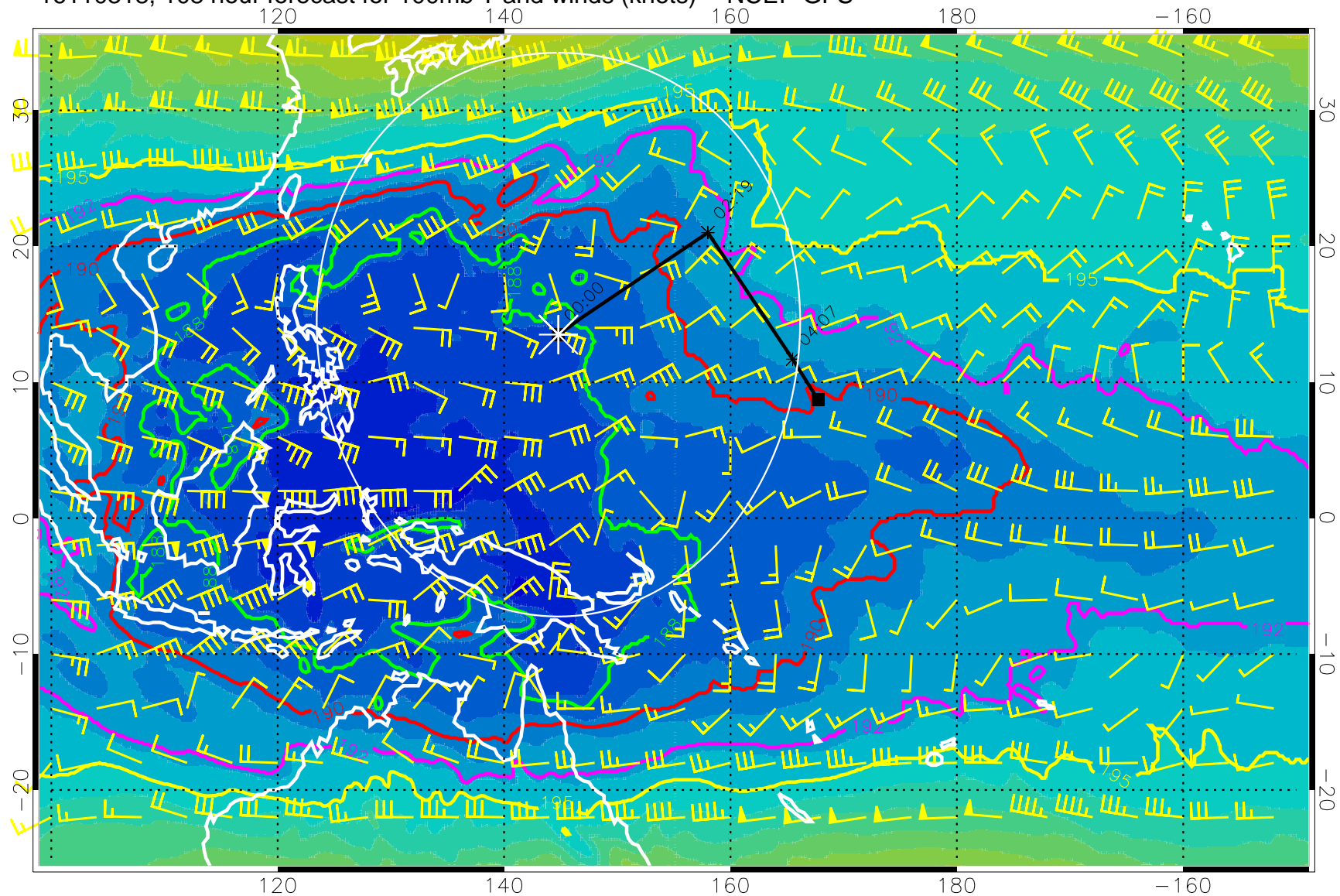
16110318, 108 hour forecast for 100mb T and winds (knots) -- NCEP GFS
