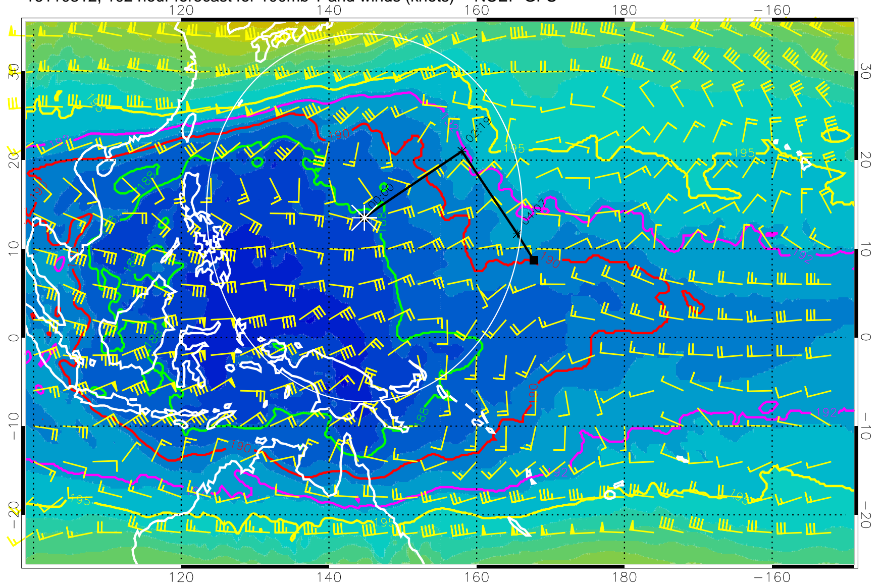
16110312, 102 hour forecast for 100mb T and winds (knots) -- NCEP GFS
