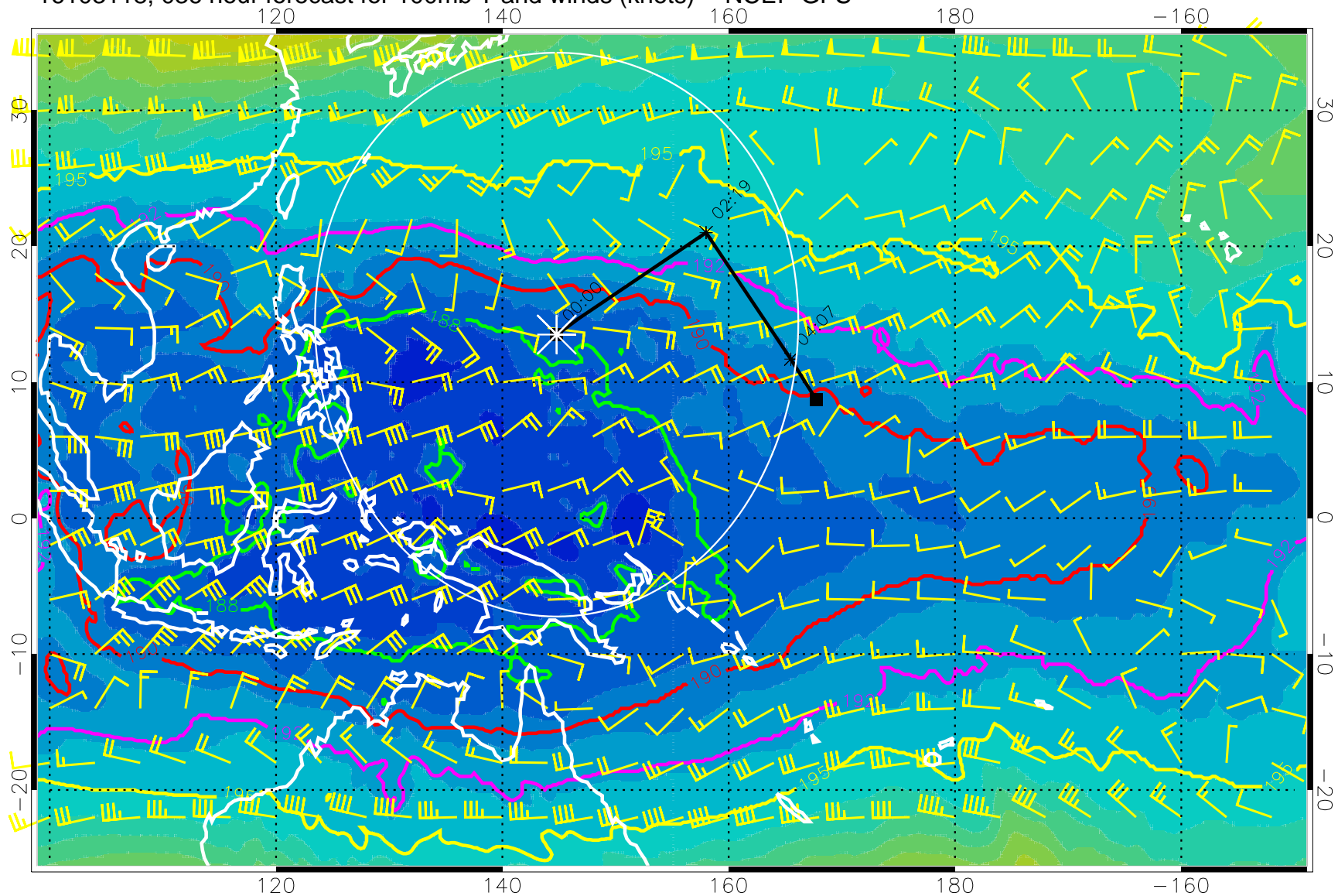
16103118, 036 hour forecast for 100mb T and winds (knots) -- NCEP GFS
