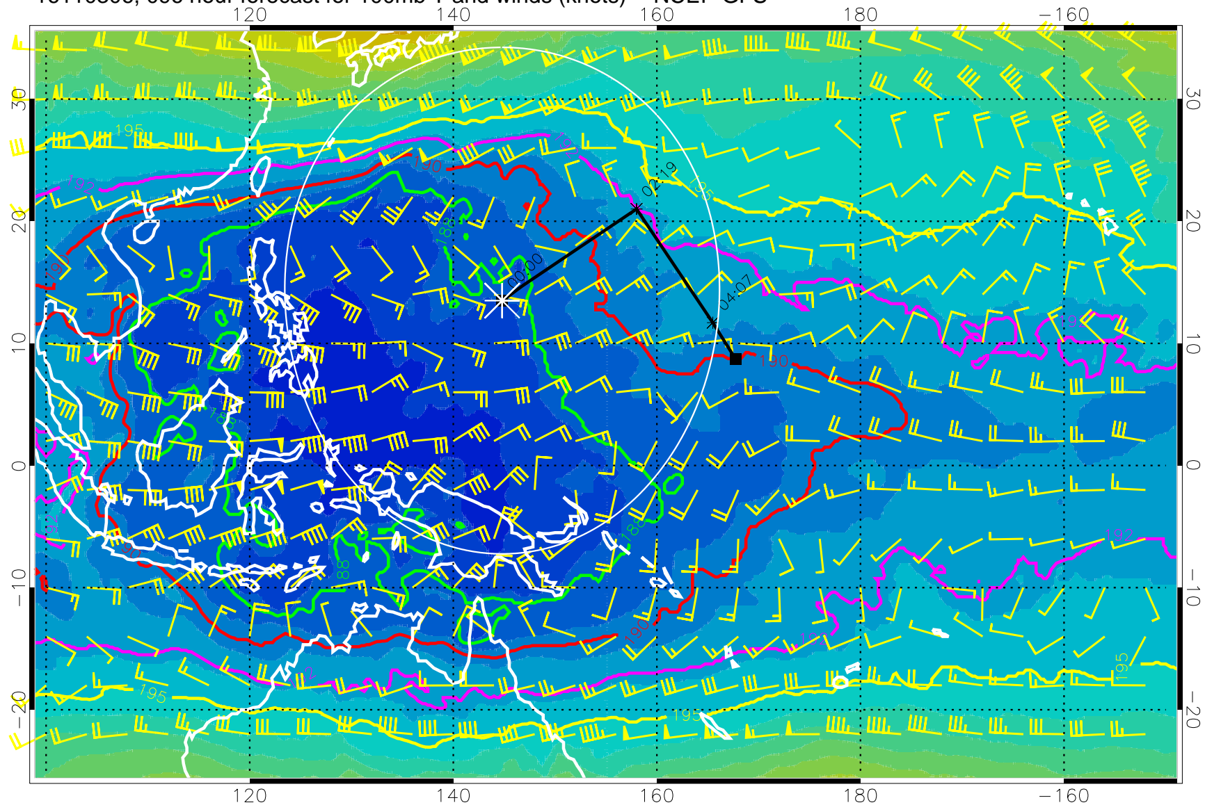
16110306, 096 hour forecast for 100mb T and winds (knots) -- NCEP GFS
