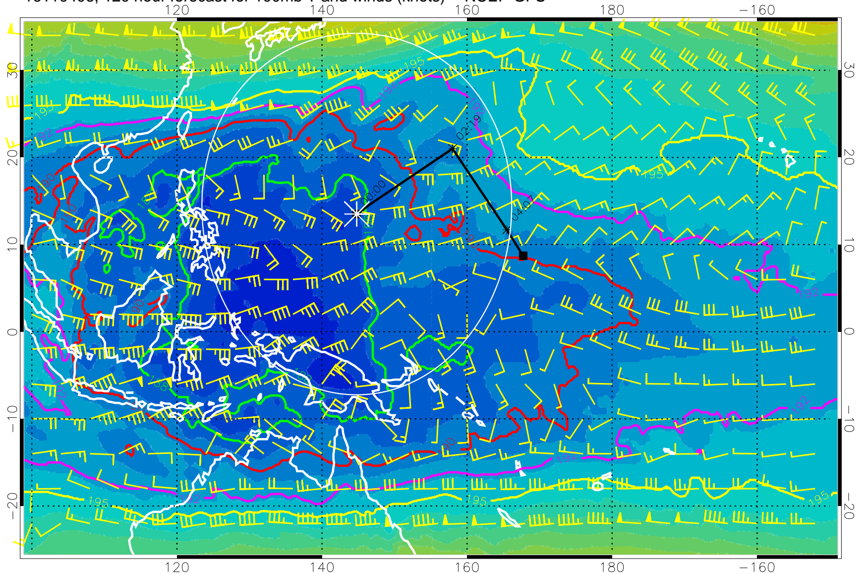
16110406, 120 hour forecast for 100mb T and winds (knots) -- NCEP GFS
